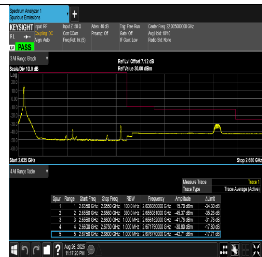
Band41(2555-2655)-20MHz-16QAM-41140-1RB#0-PASS
