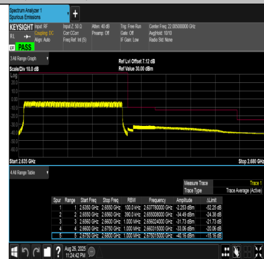
Band41(2555-2655)-20MHz-16QAM-41140-100RB#0-PASS
