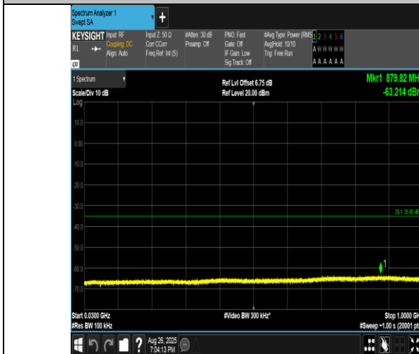
Band41(2555-2655)-5MHz-QPSK-40265-25RB#0-30~1000-PASS
