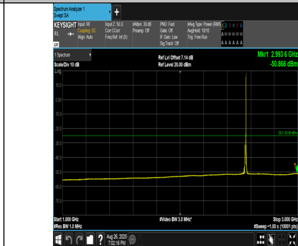
Band41(2555-2655)-5MHz-16QAM-40265-1RB#24-1000~3000-PASS
