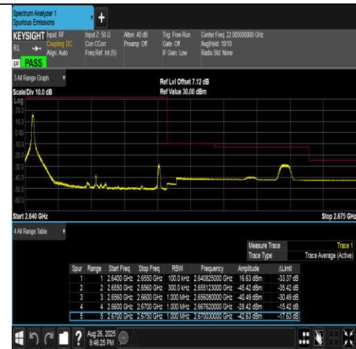
Band41(2555-2655)-15MHz-16QAM-41165-1RB#0-PASS
