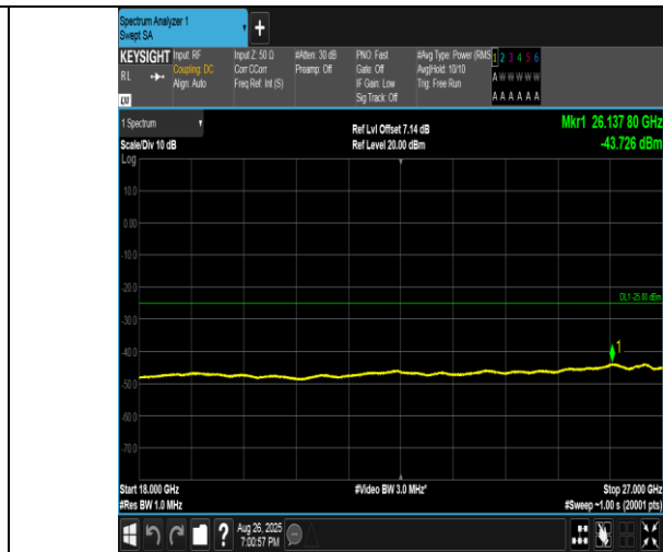
Band41(2555-2655)-5MHz-QPSK-40265-1RB#24-18000~27000-PASS
