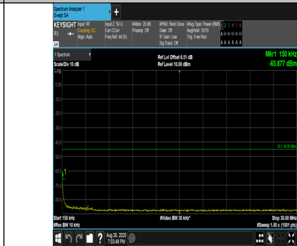
Band41(2555-2655)-5MHz-QPSK-40265-25RB#0-0.15~30-PASS
