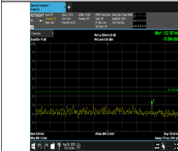
Band41(2555-2655)-5MHz-16QAM-40265-1RB#24-0.009~0.15-PASS
