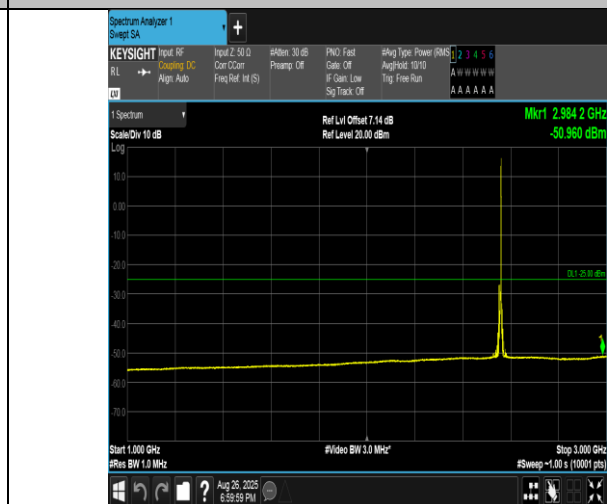
Band41(2555-2655)-5MHz-QPSK-40265-1RB#24-1000~3000-PASS
