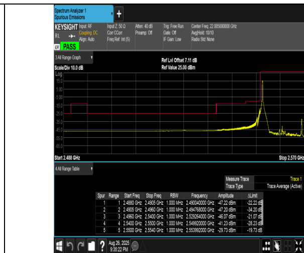
Band41(2555-2655)-15MHz-16QAM-40315-1RB#0-PASS
