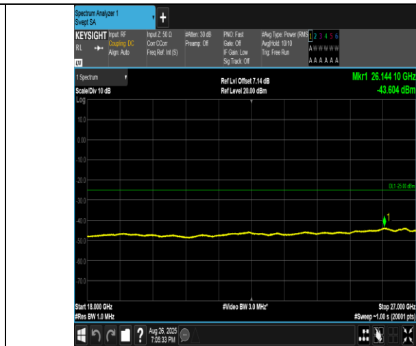
Band41(2555-2655)-5MHz-QPSK-40265-25RB#0-18000~27000-PASS
