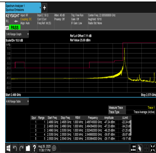
Band41(2555-2655)-20MHz-16QAM-40340-1RB#0-PASS
