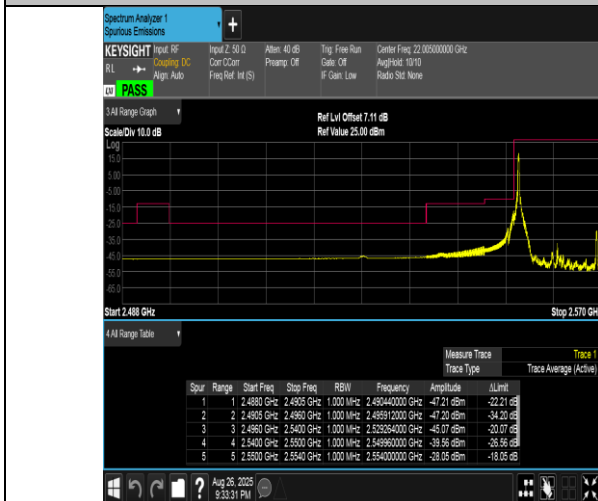
Band41(2555-2655)-15MHz-QPSK-40315-1RB#0-PASS
