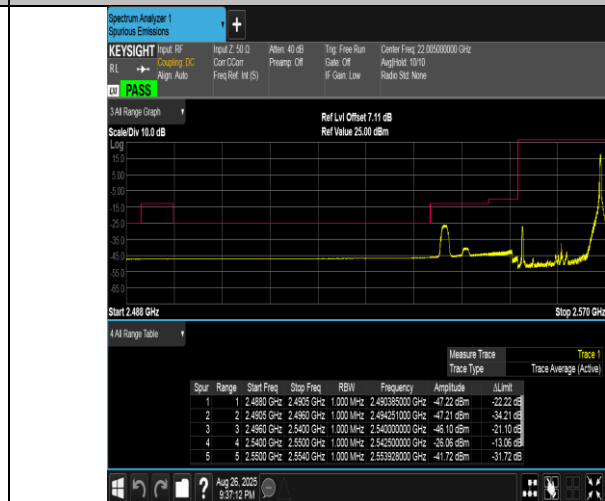
Band41(2555-2655)-15MHz-QPSK-40315-1RB#74-PASS
