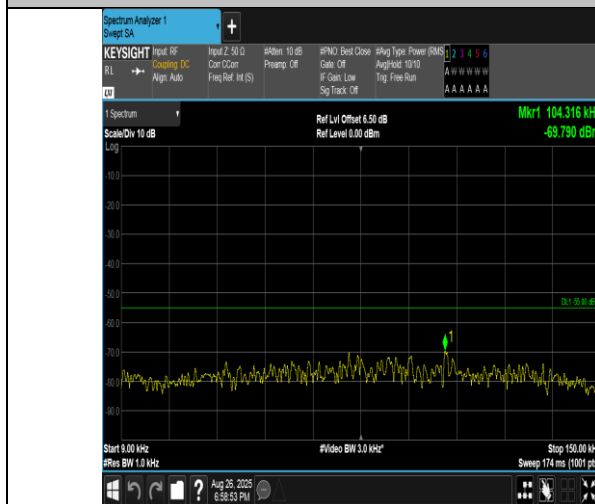
Band41(2555-2655)-5MHz-QPSK-40265-1RB#24-0.009~0.15-PASS
