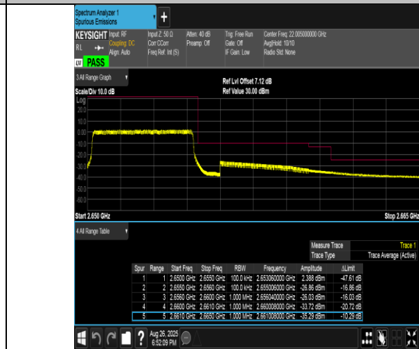
Band41(2555-2655)-5MHz-16QAM-41215-25RB#0-PASS
