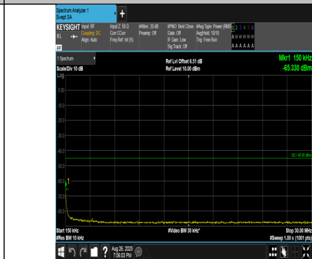
Band41(2555-2655)-5MHz-16QAM-40265-25RB#0-0.15~30-PASS
