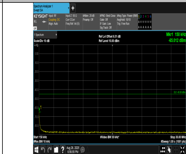
Band41(2555-2655)-5MHz-16QAM-40265-1RB#0-0.15~30-PASS
