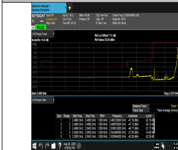
Band41(2555-2655)-15MHz-16QAM-40315-1RB#74-PASS
