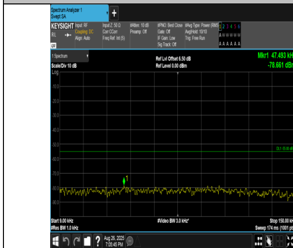
Band41(2555-2655)-5MHz-16QAM-40265-25RB#0-0.009~0.15-PASS
