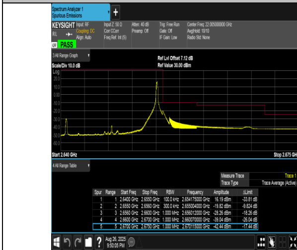
Band41(2555-2655)-15MHz-16QAM-41165-1RB#74-PASS
