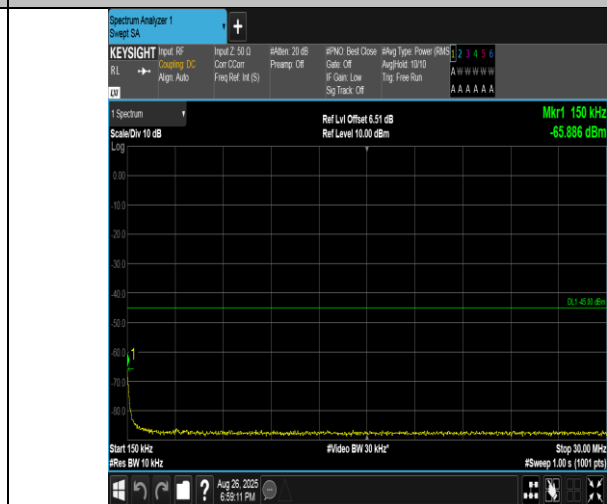
Band41(2555-2655)-5MHz-QPSK-40265-1RB#24-0.15~30-PASS
