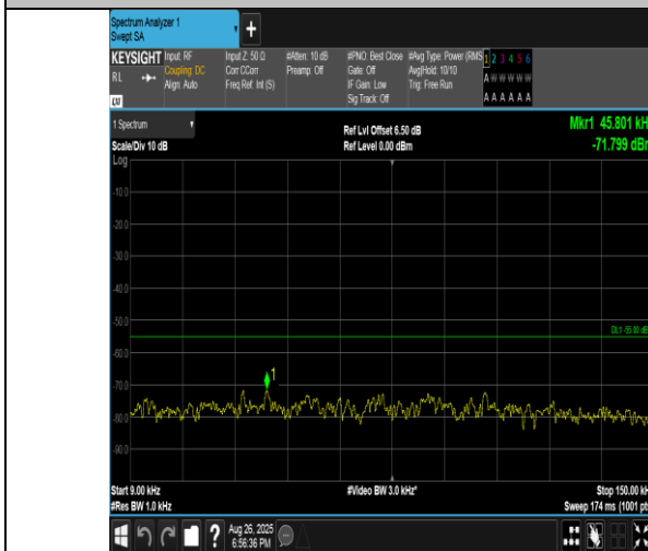
Band41(2555-2655)-5MHz-16QAM-40265-1RB#0-0.009~0.15-PASS
