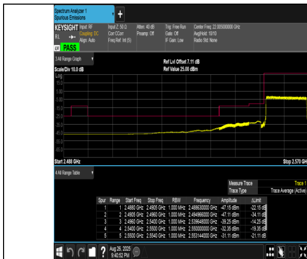
Band41(2555-2655)-15MHz-QPSK-40315-75RB#0-PASS
