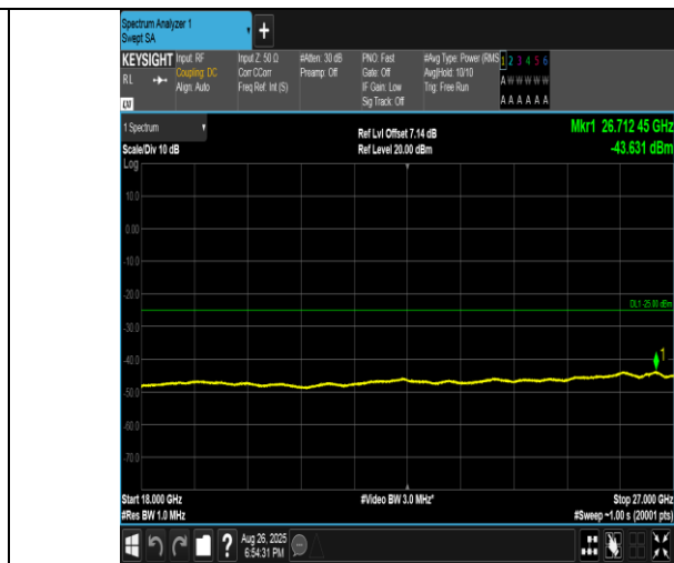
Band41(2555-2655)-5MHz-QPSK-40265-1RB#0-18000~27000-PASS
