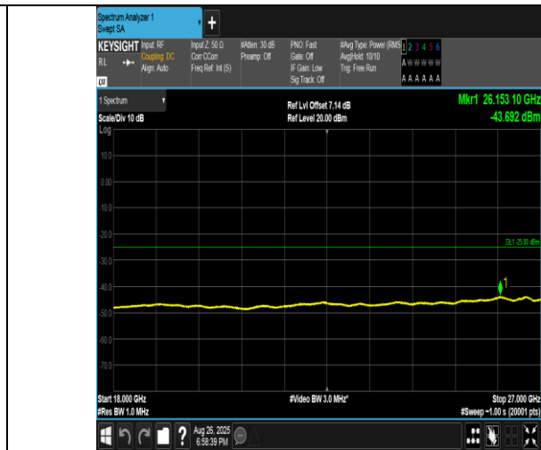
Band41(2555-2655)-5MHz-16QAM-40265-1RB#0-18000~27000-PASS
