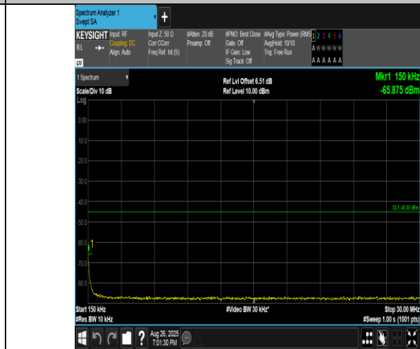
Band41(2555-2655)-5MHz-16QAM-40265-1RB#24-0.15~30-PASS
