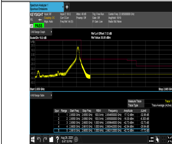
Band41(2555-2655)-5MHz-16QAM-41215-1RB#24-PASS
