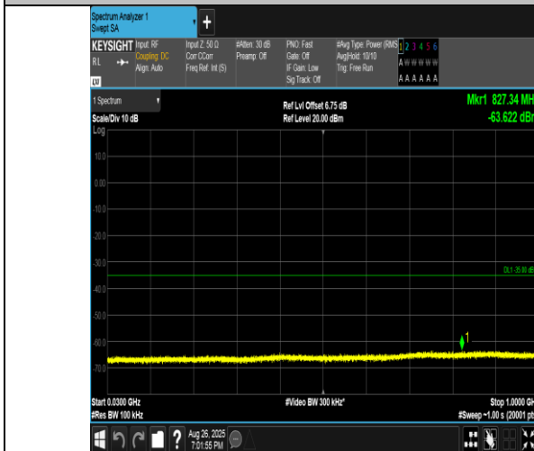
Band41(2555-2655)-5MHz-16QAM-40265-1RB#24-30~1000-PASS
