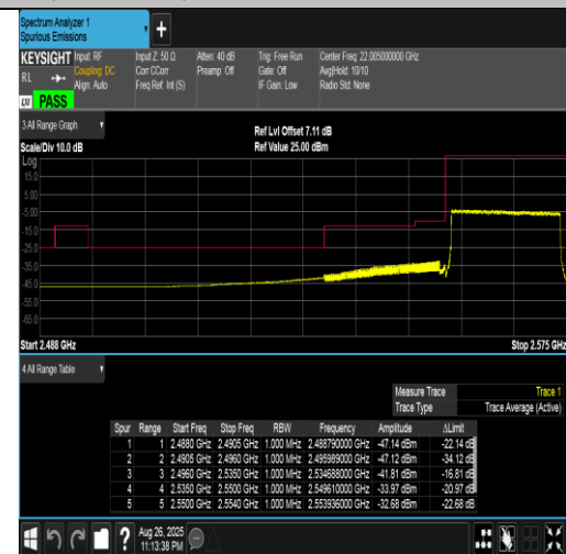
Band41(2555-2655)-20MHz-16QAM-40340-100RB#0-PASS
