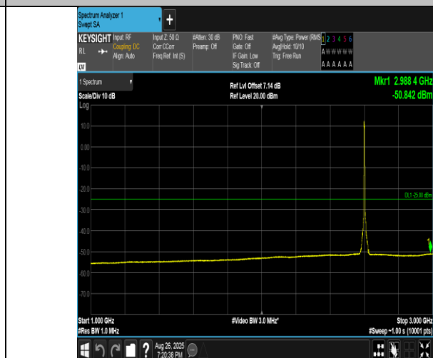
Band41(2555-2655)-5MHz-16QAM-40690-25RB#0-1000~3000-PASS
