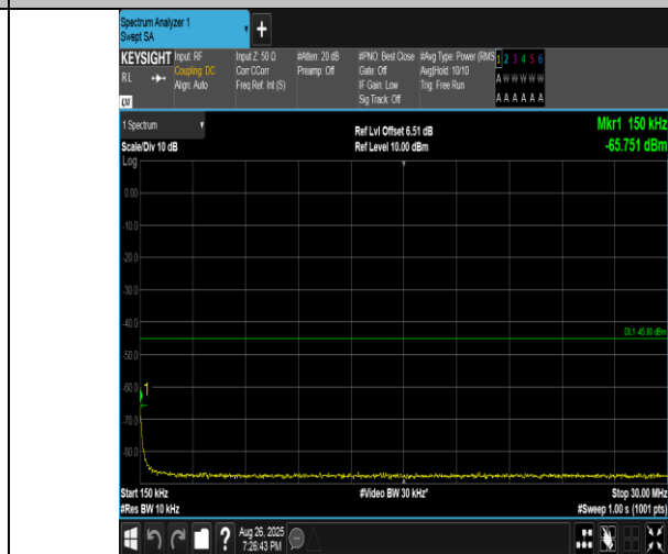
Band41(2555-2655)-5MHz-QPSK-41215-1RB#24-0.15~30-PASS
