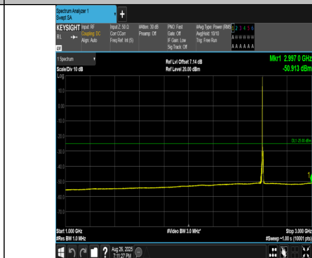
Band41(2555-2655)-5MHz-16QAM-40690-1RB#0-1000~3000-PASS
