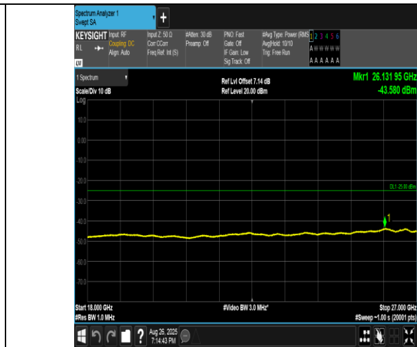
Band41(2555-2655)-5MHz-QPSK-40690-1RB#24-18000~27000-PASS
