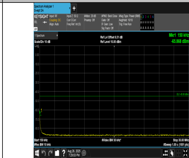
Band41(2555-2655)-5MHz-16QAM-41215-1RB#24-0.15~30-PASS
