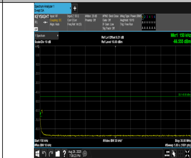
Band41(2555-2655)-5MHz-QPSK-40690-1RB#0-0.15~30-PASS
