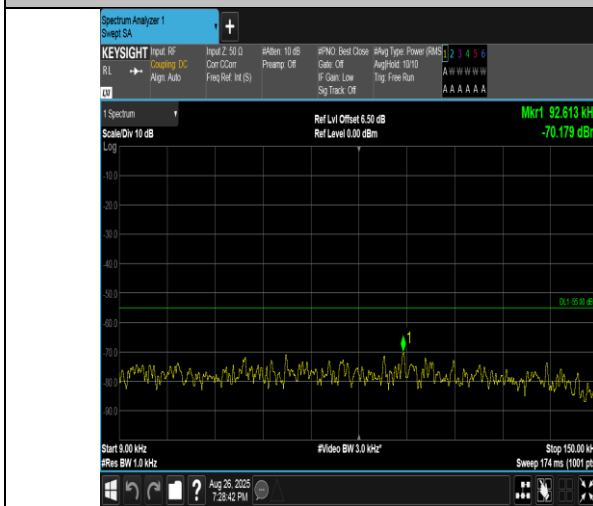
Band41(2555-2655)-5MHz-16QAM-41215-1RB#24-0.009~0.15-PASS
