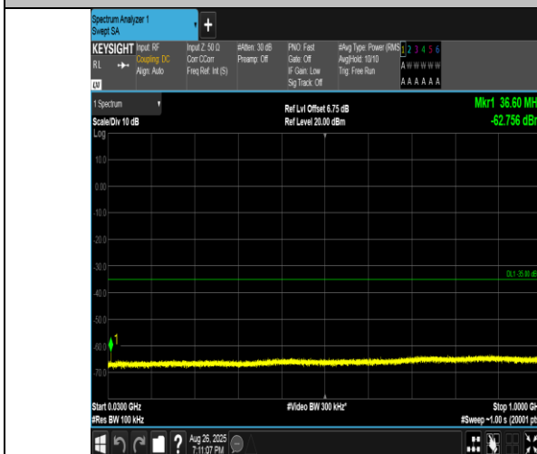
Band41(2555-2655)-5MHz-16QAM-40690-1RB#0-30~1000-PASS
