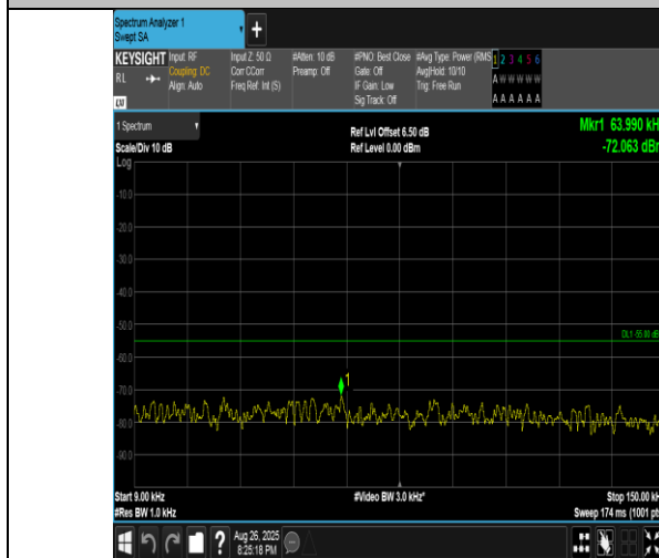
Band41(2555-2655)-10MHz-16QAM-40290-1RB#0-0.009~0.15-PASS
