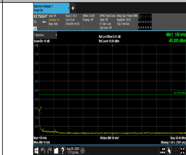
Band41(2555-2655)-5MHz-QPSK-40690-25RB#0-0.15~30-PASS
