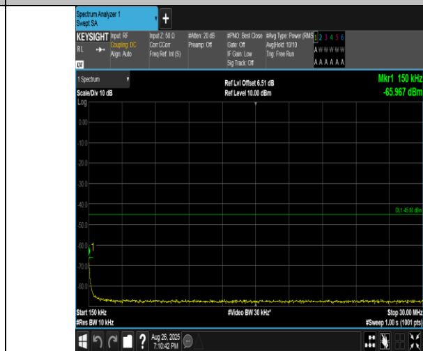
Band41(2555-2655)-5MHz-16QAM-40690-1RB#0-0.15~30-PASS
