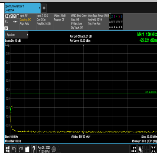
Band41(2555-2655)-5MHz-QPSK-40690-1RB#24-0.15~30-PASS
