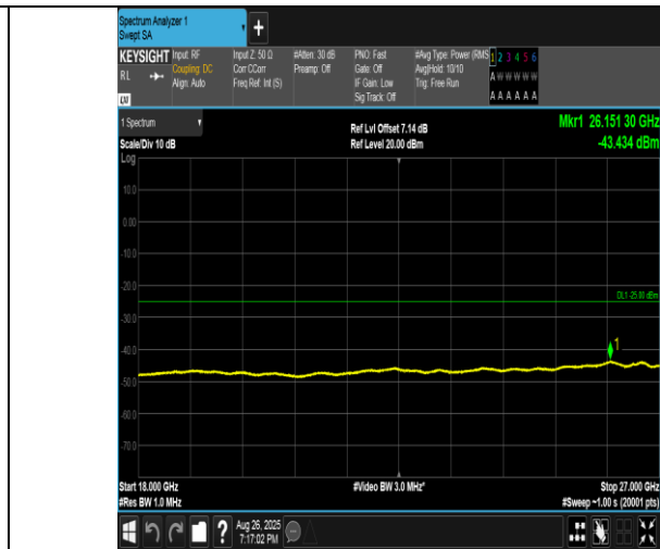
Band41(2555-2655)-5MHz-16QAM-40690-1RB#24-18000~27000-PASS
