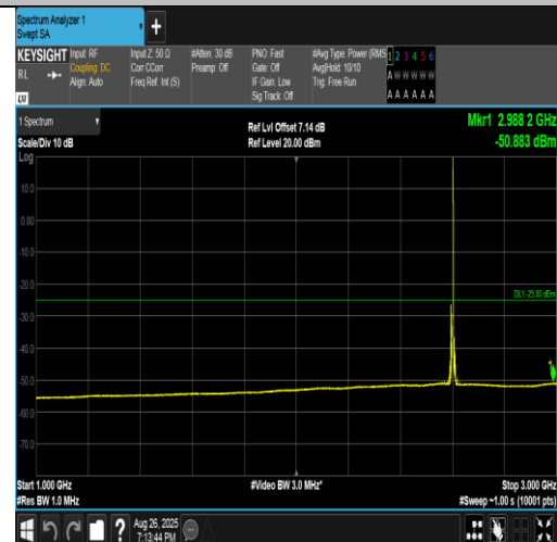
Band41(2555-2655)-5MHz-QPSK-40690-1RB#24-1000~3000-PASS
