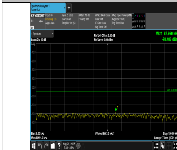
Band41(2555-2655)-5MHz-16QAM-41215-25RB#0-0.009~0.15-PASS
