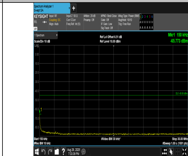
Band41(2555-2655)-5MHz-16QAM-41215-25RB#0-0.15~30-PASS
