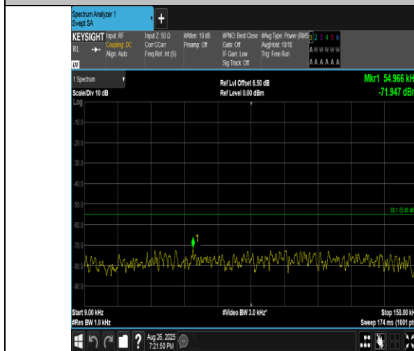
Band41(2555-2655)-5MHz-QPSK-41215-1RB#0-0.009~0.15-PASS
