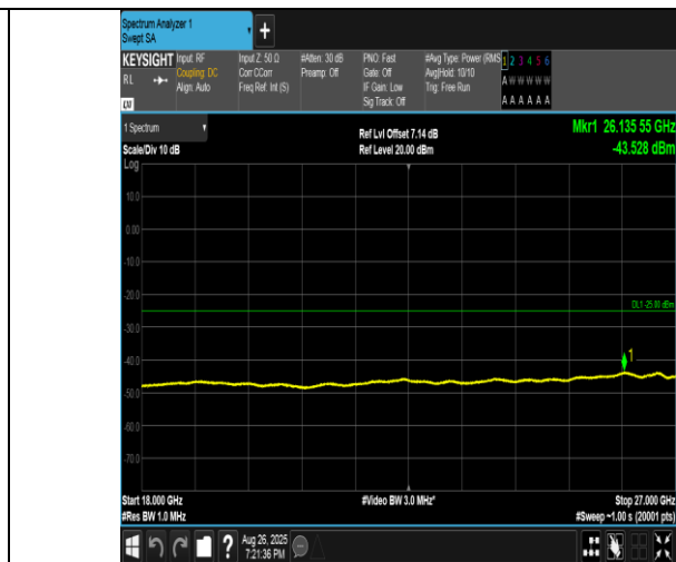
Band41(2555-2655)-5MHz-16QAM-40690-25RB#0-18000~27000-PASS
