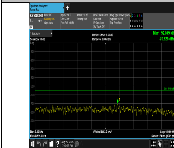
Band41(2555-2655)-5MHz-16QAM-40690-1RB#0-0.009~0.15-PASS
