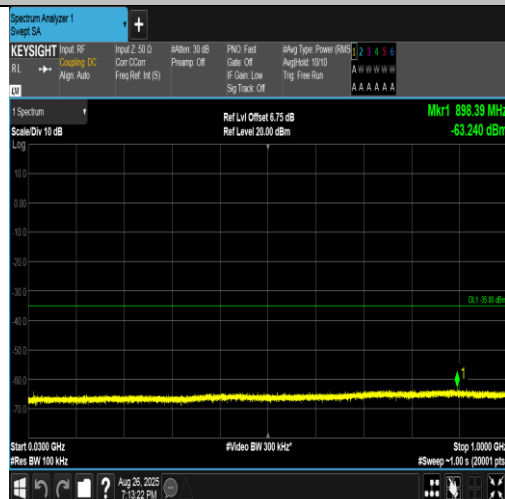
Band41(2555-2655)-5MHz-QPSK-40690-1RB#24-30~1000-PASS
