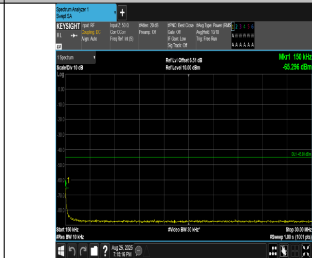
Band41(2555-2655)-5MHz-16QAM-40690-1RB#24-0.15~30-PASS
