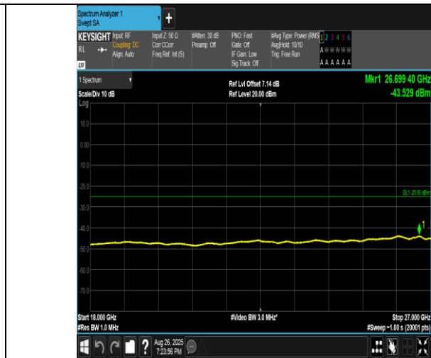
Band41(2555-2655)-5MHz-QPSK-41215-1RB#0-18000~27000-PASS
