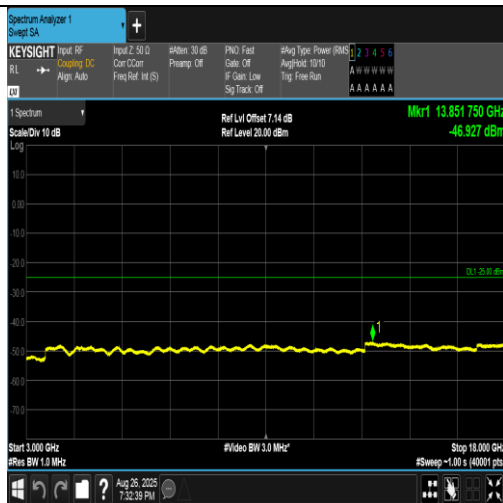
Band41(2555-2655)-5MHz-QPSK-41215-25RB#0-3000~18000-PASS
