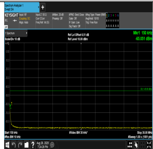
Band41(2555-2655)-5MHz-16QAM-41215-1RB#0-0.15~30-PASS
