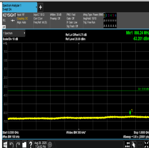
Band41(2555-2655)-5MHz-16QAM-41215-1RB#0-30~1000-PASS
