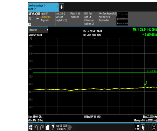
Band41(2555-2655)-5MHz-16QAM-41215-1RB#24-18000~27000-PASS
