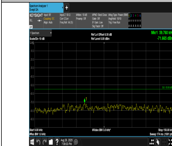
Band41(2555-2655)-5MHz-QPSK-40690-1RB#0-0.009~0.15-PASS
