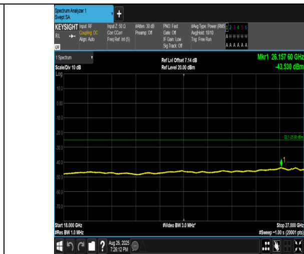
Band41(2555-2655)-5MHz-16QAM-41215-1RB#0-18000~27000-PASS
