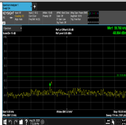
Band41(2555-2655)-5MHz-QPSK-40690-1RB#24-0.009~0.15-PASS
