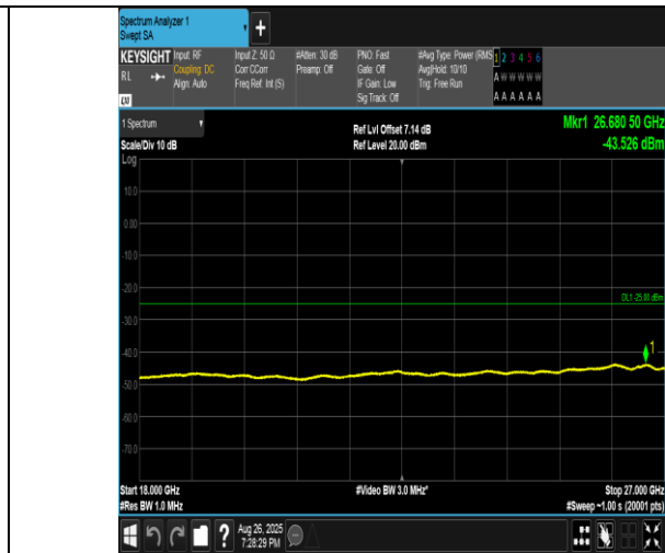
Band41(2555-2655)-5MHz-QPSK-41215-1RB#24-18000~27000-PASS
