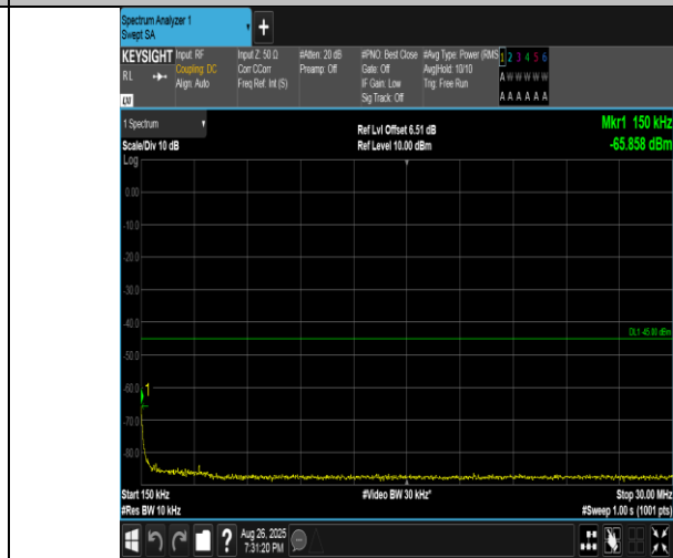
Band41(2555-2655)-5MHz-QPSK-41215-25RB#0-0.15~30-PASS
