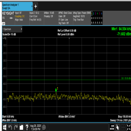
Band41(2555-2655)-5MHz-16QAM-41215-1RB#0-0.009~0.15-PASS
