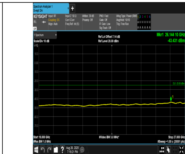
Band41(2555-2655)-5MHz-QPSK-40690-25RB#0-18000~27000-PASS
