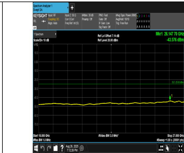
Band41(2555-2655)-5MHz-16QAM-40690-1RB#0-18000~27000-PASS
