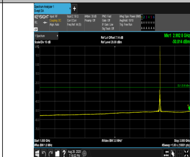
Band41(2555-2655)-5MHz-16QAM-40690-1RB#24-1000~3000-PASS
