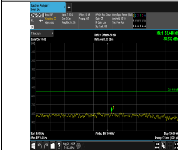
Band41(2555-2655)-5MHz-16QAM-40690-25RB#0-0.009~0.15-PASS
