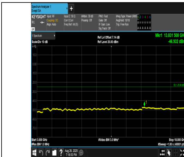
Band41(2555-2655)-5MHz-QPSK-40690-25RB#0-3000~18000-PASS
