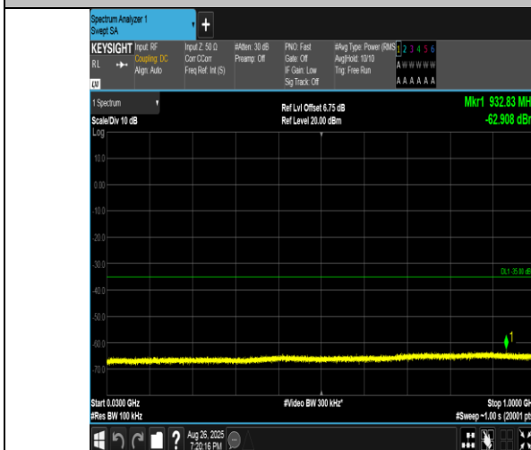
Band41(2555-2655)-5MHz-16QAM-40690-25RB#0-30~1000-PASS
