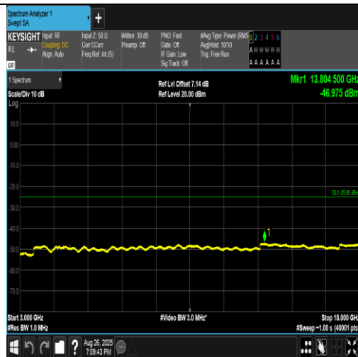
Band41(2555-2655)-5MHz-QPSK-40690-1RB#0-3000~18000-PASS
