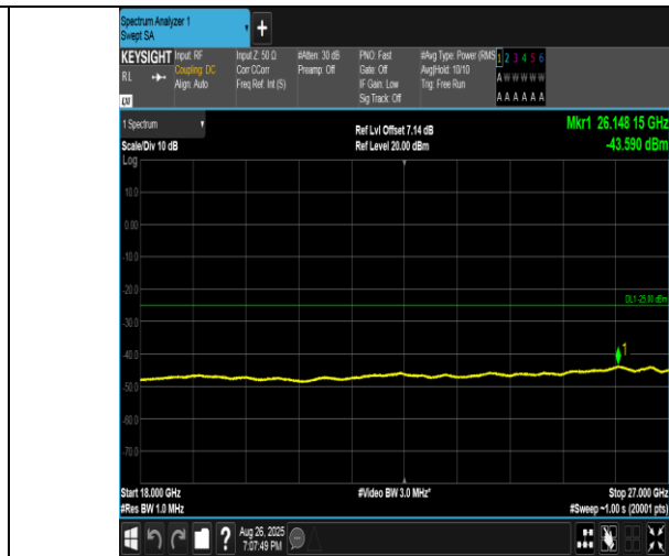
Band41(2555-2655)-5MHz-16QAM-40265-25RB#0-18000~27000-PASS
