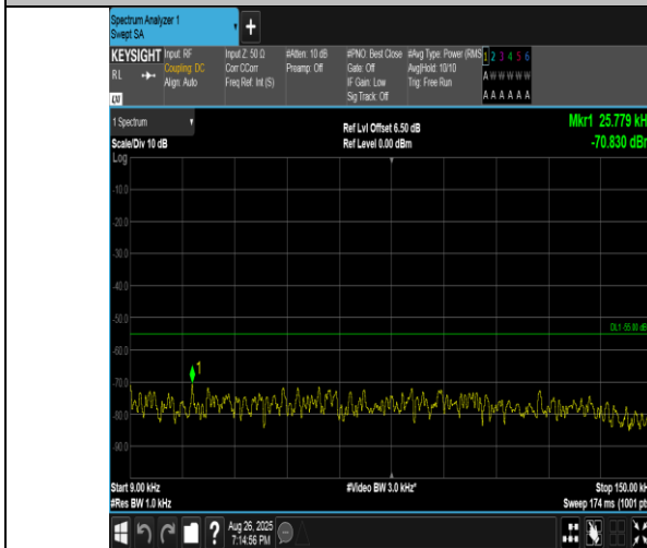
Band41(2555-2655)-5MHz-16QAM-40690-1RB#24-0.009~0.15-PASS
