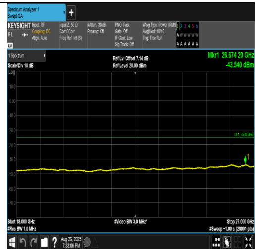
Band41(2555-2655)-5MHz-QPSK-41215-25RB#0-18000~27000-PASS
