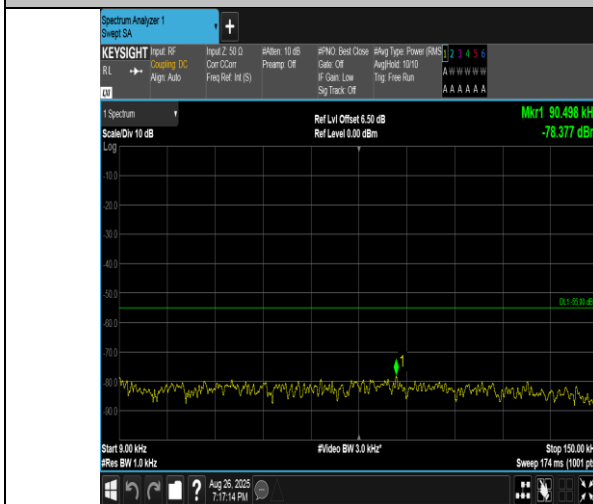
Band41(2555-2655)-5MHz-QPSK-40690-25RB#0-0.009~0.15-PASS
