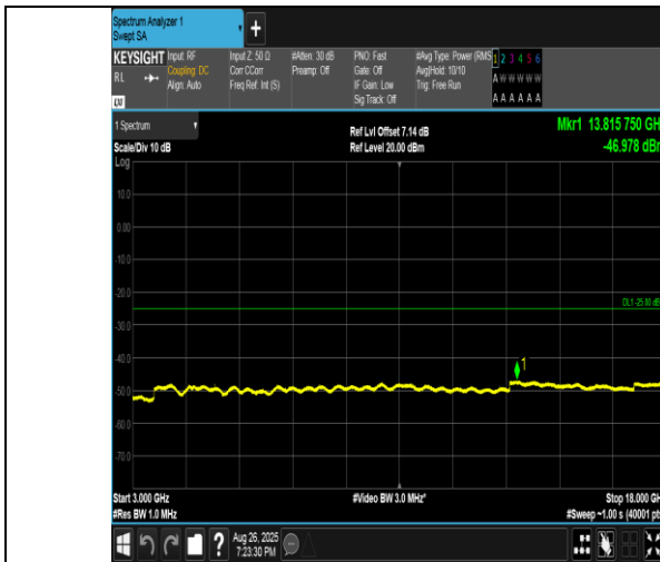
Band41(2555-2655)-5MHz-QPSK-41215-1RB#0-3000~18000-PASS
