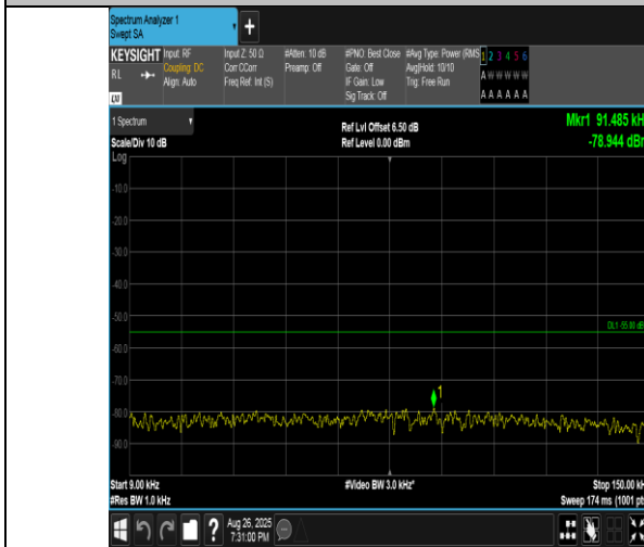
Band41(2555-2655)-5MHz-QPSK-41215-25RB#0-0.009~0.15-PASS
