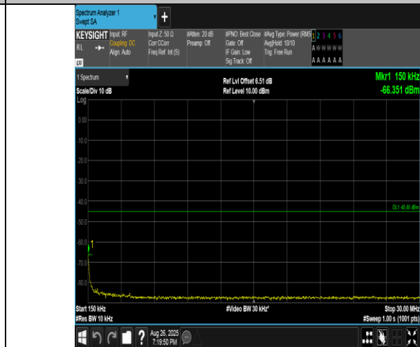
Band41(2555-2655)-5MHz-16QAM-40690-25RB#0-0.15~30-PASS
