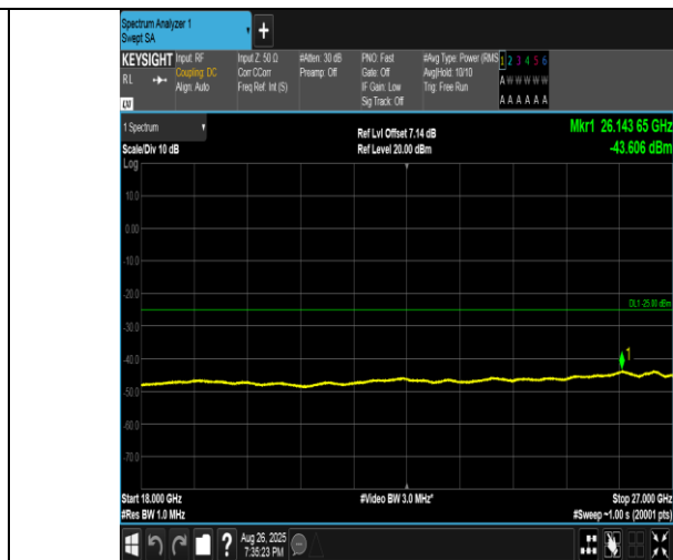
Band41(2555-2655)-5MHz-16QAM-41215-25RB#0-18000~27000-PASS
