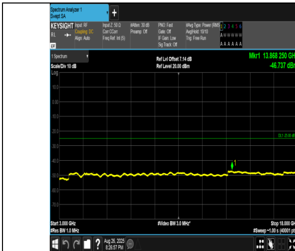
Band41(2555-2655)-10MHz-16QAM-40290-1RB#0-3000~18000-PASS
