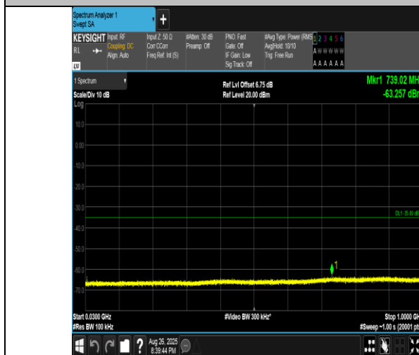
Band41(2555-2655)-10MHz-16QAM-40690-1RB#0-30~1000-PASS
