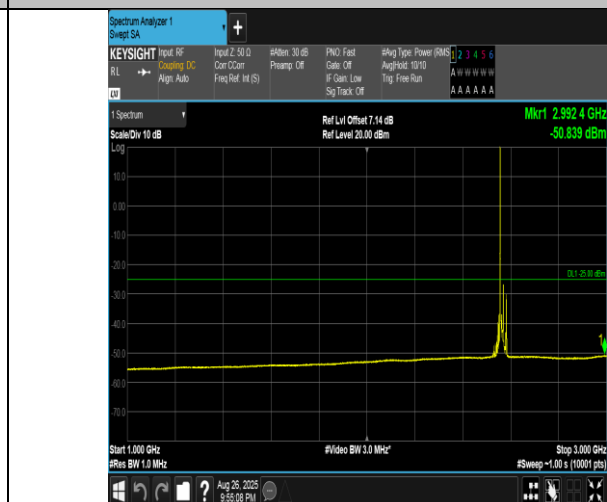
Band41(2555-2655)-15MHz-QPSK-40315-1RB#0-1000~3000-PASS
