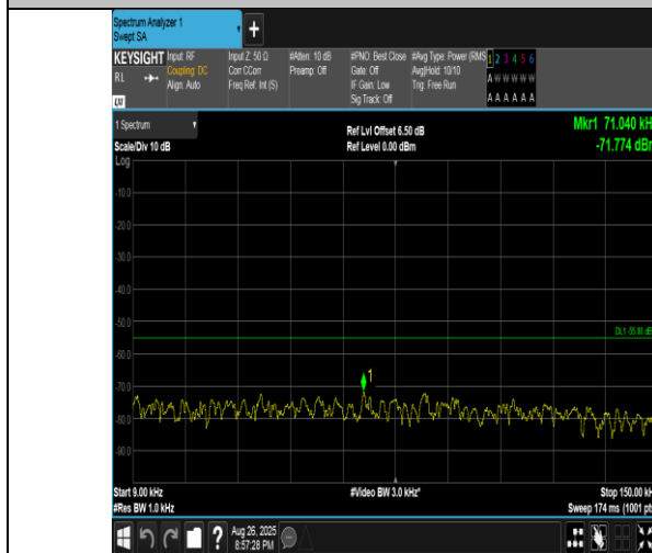
Band41(2555-2655)-10MHz-16QAM-41190-1RB#49-0.009~0.15-PASS
