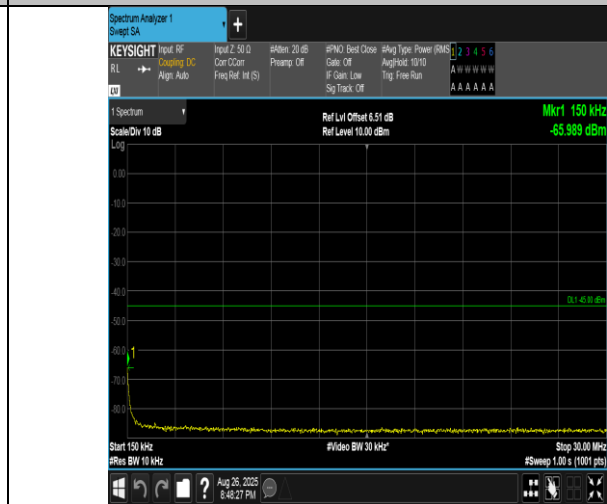
Band41(2555-2655)-10MHz-16QAM-40690-50RB#0-0.15~30-PASS
