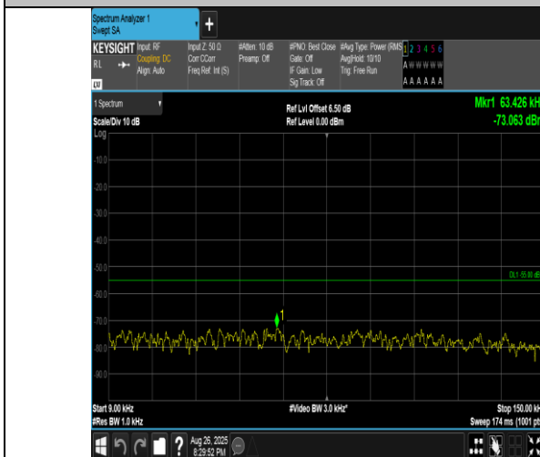
Band41(2555-2655)-10MHz-16QAM-40290-1RB#49-0.009~0.15-PASS
