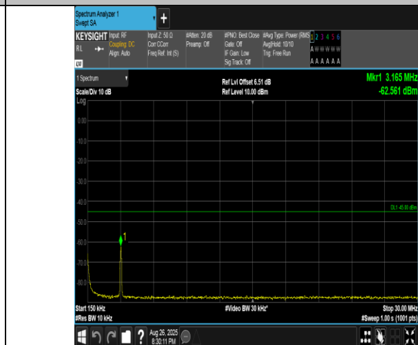
Band41(2555-2655)-10MHz-16QAM-40290-1RB#49-0.15~30-PASS
