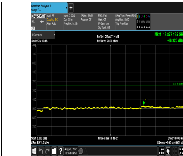
Band41(2555-2655)-10MHz-16QAM-40290-50RB#0-3000~18000-PASS
