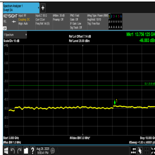
Band41(2555-2655)-15MHz-QPSK-40315-1RB#0-3000~18000-PASS
