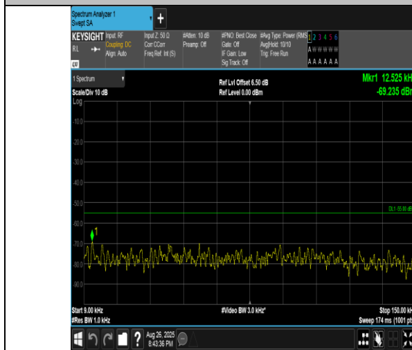
Band41(2555-2655)-10MHz-16QAM-40690-1RB#49-0.009~0.15-PASS
