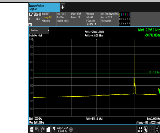
Band41(2555-2655)-10MHz-16QAM-40690-1RB#49-1000~3000-PASS
