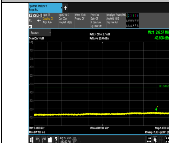
Band41(2555-2655)-10MHz-16QAM-41190-1RB#0-30~1000-PASS
