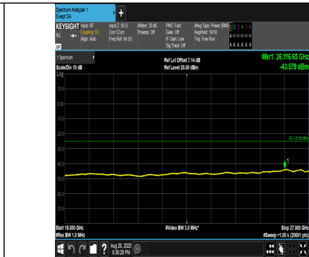
Band41(2555-2655)-10MHz-16QAM-40290-50RB#0-18000~27000-PASS
