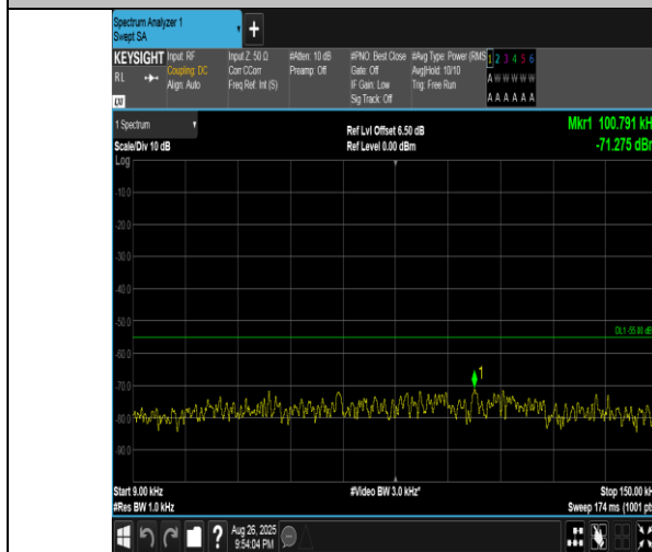
Band41(2555-2655)-15MHz-QPSK-40315-1RB#0-0.009~0.15-PASS
