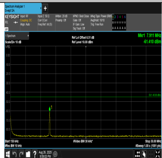
Band41(2555-2655)-15MHz-QPSK-40315-1RB#74-0.15~30-PASS
