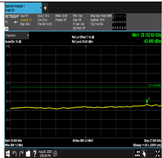
Band41(2555-2655)-15MHz-QPSK-40315-1RB#0-18000~27000-PASS
