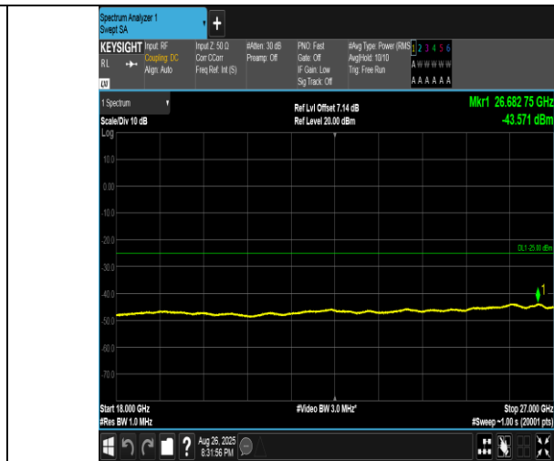
Band41(2555-2655)-10MHz-16QAM-40290-1RB#49-18000~27000-PASS
