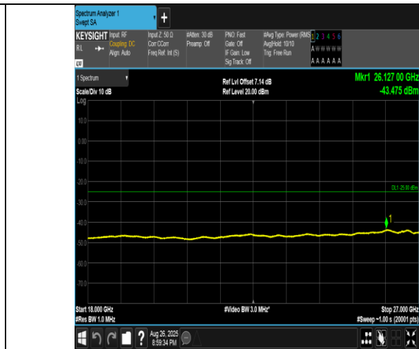
Band41(2555-2655)-10MHz-16QAM-41190-1RB#49-18000~27000-PASS
