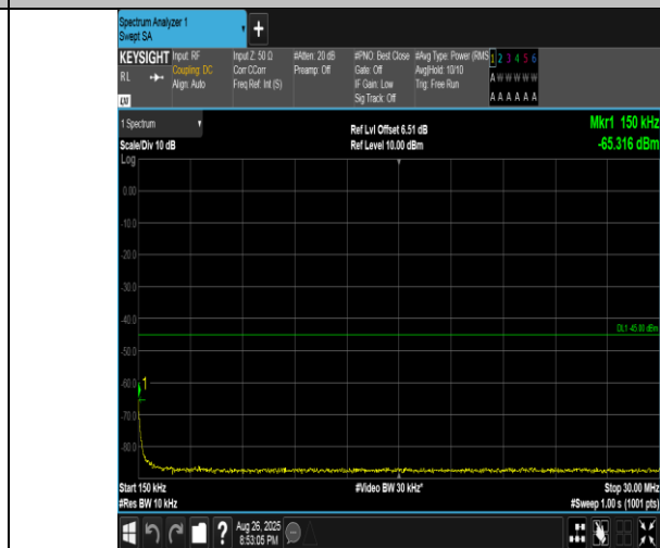
Band41(2555-2655)-10MHz-16QAM-41190-1RB#0-0.15~30-PASS
