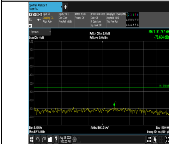
Band41(2555-2655)-10MHz-16QAM-41190-50RB#0-0.009~0.15-PASS
