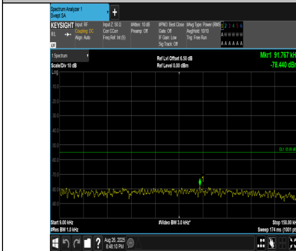
Band41(2555-2655)-10MHz-16QAM-40690-50RB#0-0.009~0.15-PASS
