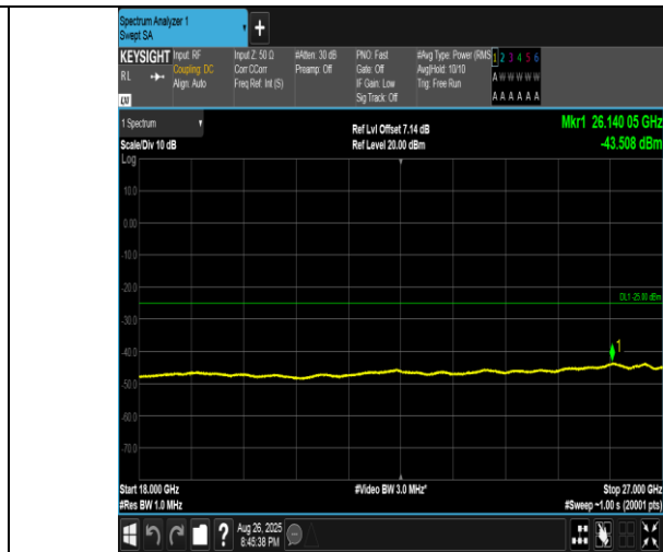
Band41(2555-2655)-10MHz-16QAM-40690-1RB#49-18000~27000-PASS
