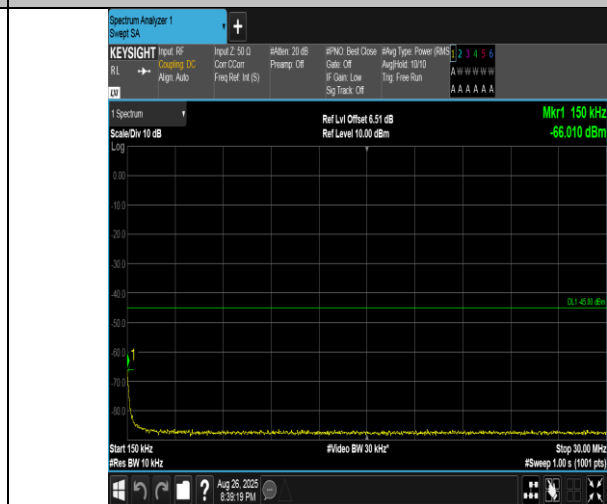
Band41(2555-2655)-10MHz-16QAM-40690-1RB#0-0.15~30-PASS
