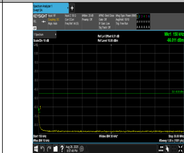
Band41(2555-2655)-10MHz-16QAM-41190-1RB#49-0.15~30-PASS
