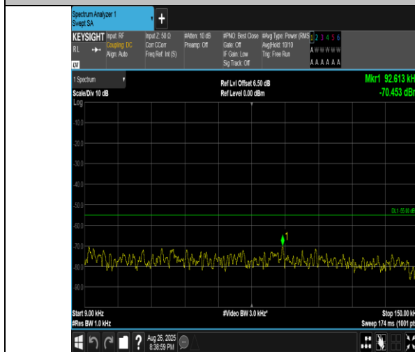
Band41(2555-2655)-10MHz-16QAM-40690-1RB#0-0.009~0.15-PASS
