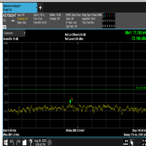
Band41(2555-2655)-15MHz-QPSK-40315-1RB#74-0.009~0.15-PASS
