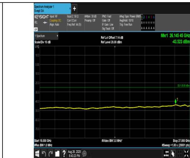
Band41(2555-2655)-10MHz-QPSK-40690-1RB#49-18000~27000-PASS
