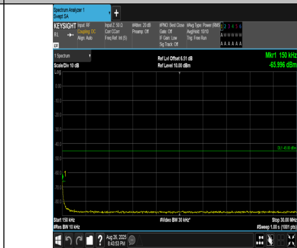
Band41(2555-2655)-10MHz-16QAM-40690-1RB#49-0.15~30-PASS
