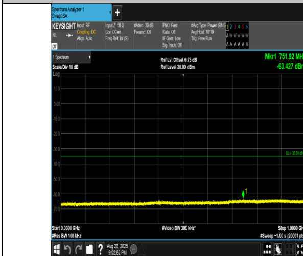
Band41(2555-2655)-10MHz-16QAM-41190-50RB#0-30~1000-PASS
