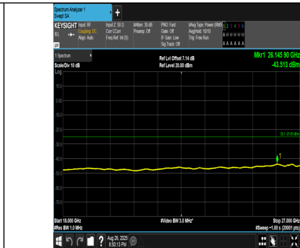
Band41(2555-2655)-10MHz-16QAM-40690-50RB#0-18000~27000-PASS
