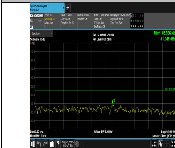
Band41(2555-2655)-10MHz-16QAM-41190-1RB#0-0.009~0.15-PASS
