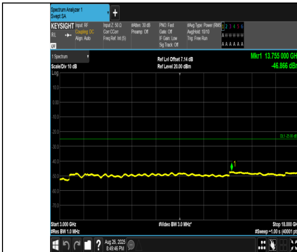
Band41(2555-2655)-10MHz-16QAM-40690-50RB#0-3000~18000-PASS
