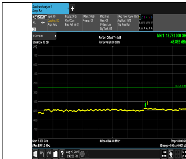
Band41(2555-2655)-10MHz-16QAM-40690-1RB#0-3000~18000-PASS
