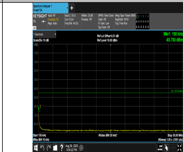
Band41(2555-2655)-15MHz-QPSK-40315-1RB#0-0.15~30-PASS
