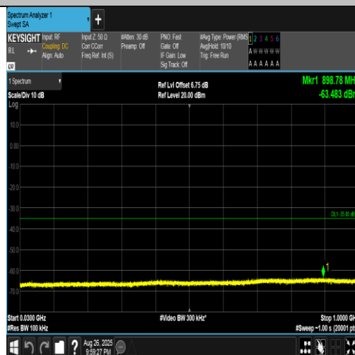
Band41(2555-2655)-15MHz-QPSK-40315-1RB#74-30~1000-PASS
