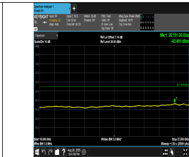
Band41(2555-2655)-10MHz-16QAM-40690-1RB#0-18000~27000-PASS
