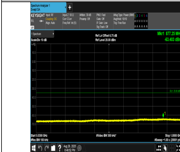
Band41(2555-2655)-10MHz-16QAM-40690-50RB#0-30~1000-PASS
