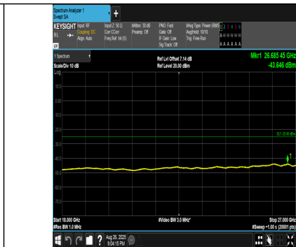
Band41(2555-2655)-10MHz-16QAM-41190-50RB#0-18000~27000-PASS
