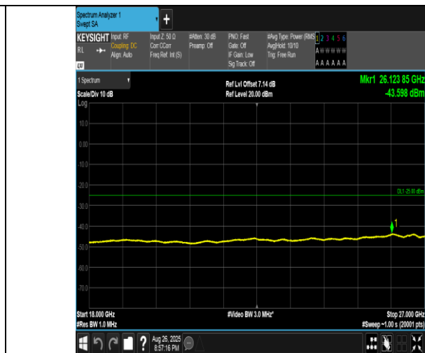
Band41(2555-2655)-10MHz-QPSK-41190-1RB#49-18000~27000-PASS
