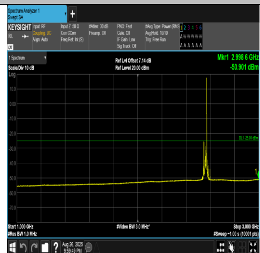
Band41(2555-2655)-15MHz-QPSK-40315-1RB#74-1000~3000-PASS
