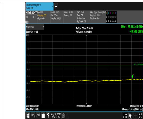
Band41(2555-2655)-10MHz-16QAM-41190-1RB#0-18000~27000-PASS
