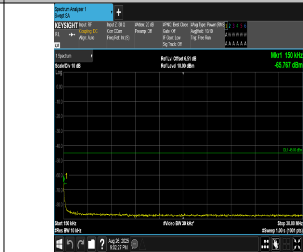
Band41(2555-2655)-10MHz-16QAM-41190-50RB#0-0.15~30-PASS
