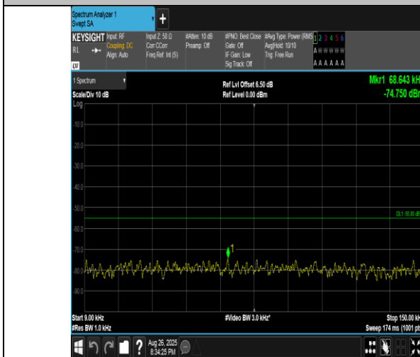
Band41(2555-2655)-10MHz-16QAM-40290-50RB#0-0.009~0.15-PASS
