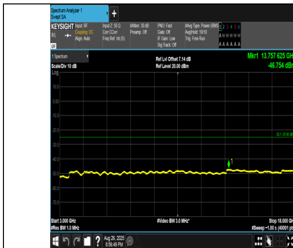
Band41(2555-2655)-10MHz-QPSK-41190-1RB#49-3000~18000-PASS
