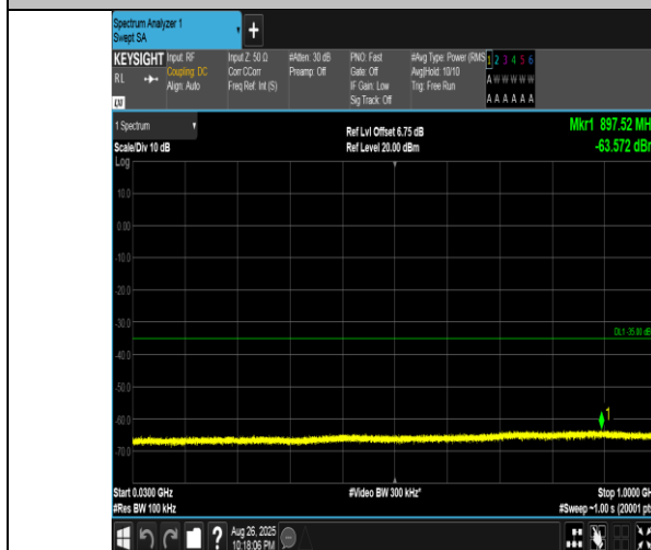
Band41(2555-2655)-15MHz-QPSK-40690-75RB#0-30~1000-PASS
