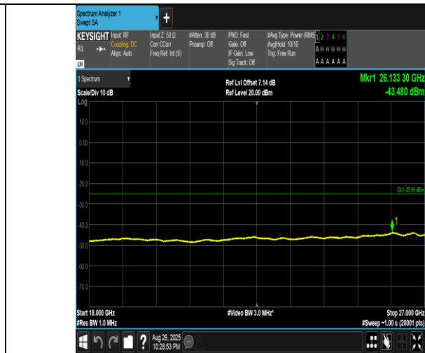
Band41(2555-2655)-15MHz-QPSK-41165-1RB#74-18000~27000-PASS
