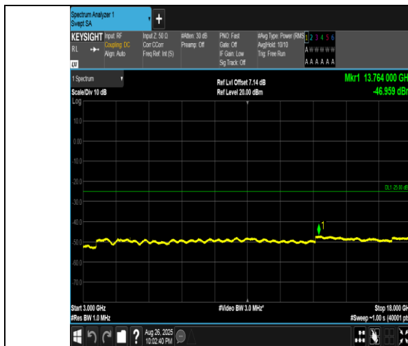
Band41(2555-2655)-15MHz-16QAM-40315-1RB#74-3000~18000-PASS
