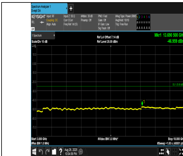
Band41(2555-2655)-15MHz-QPSK-40315-75RB#0-3000~18000-PASS
