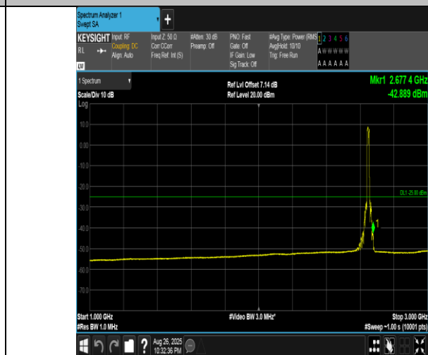
Band41(2555-2655)-15MHz-QPSK-41165-75RB#0-1000~3000-PASS
