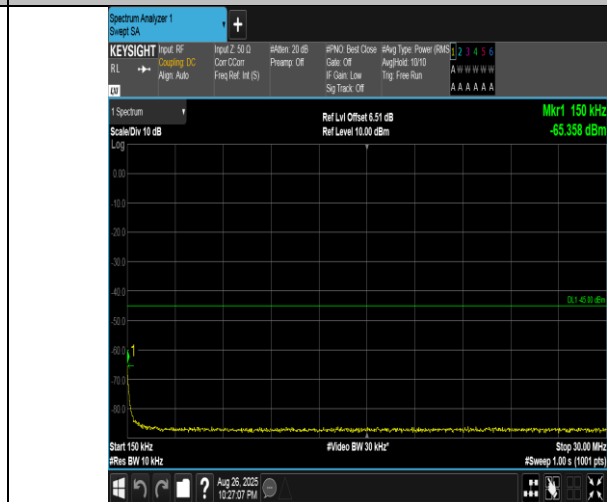
Band41(2555-2655)-15MHz-QPSK-41165-1RB#74-0.15~30-PASS
