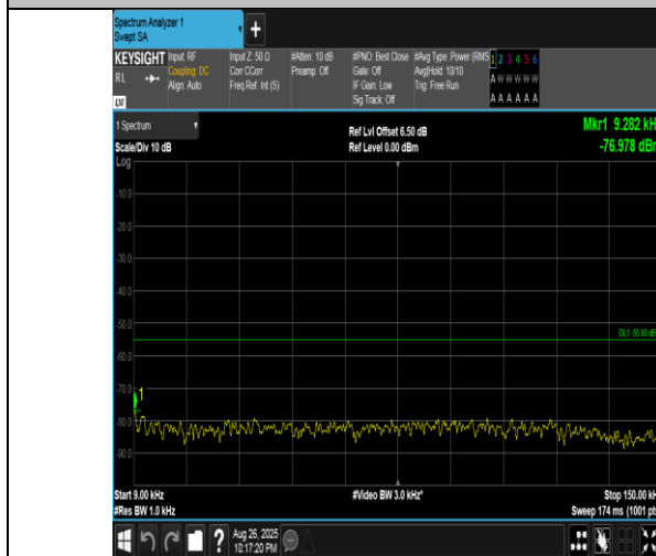
Band41(2555-2655)-15MHz-QPSK-40690-75RB#0-0.009~0.15-PASS
