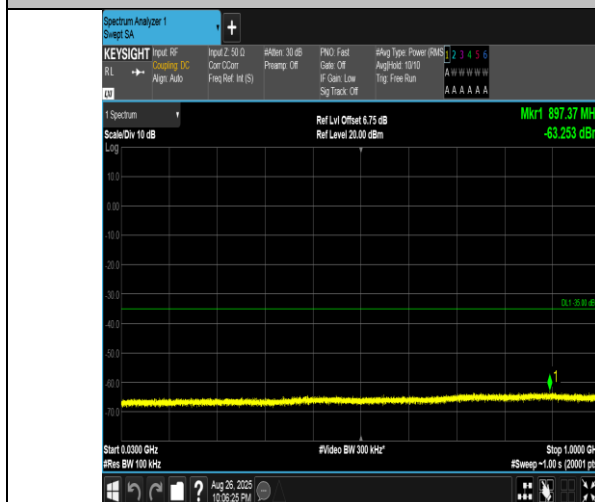
Band41(2555-2655)-15MHz-16QAM-40315-75RB#0-30~1000-PASS
