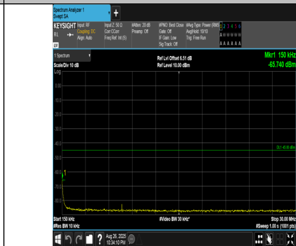
Band41(2555-2655)-15MHz-16QAM-41165-75RB#0-0.15~30-PASS
