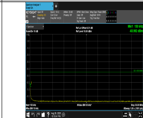
Band41(2555-2655)-15MHz-16QAM-40690-1RB#0-0.15~30-PASS
