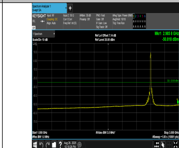
Band41(2555-2655)-15MHz-QPSK-40690-75RB#0-1000~3000-PASS
