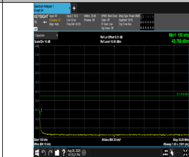
Band41(2555-2655)-15MHz-16QAM-40690-1RB#74-0.15~30-PASS
