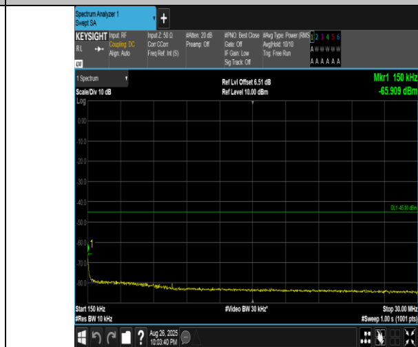
Band41(2555-2655)-15MHz-QPSK-40315-75RB#0-0.15~30-PASS
