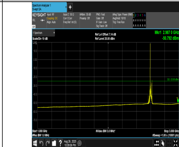
Band41(2555-2655)-15MHz-QPSK-40690-1RB#0-1000~3000-PASS
