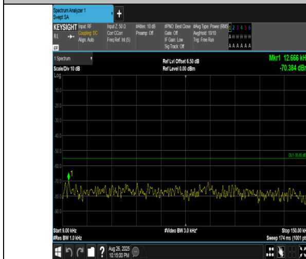
Band41(2555-2655)-15MHz-16QAM-40690-1RB#74-0.009~0.15-PASS
