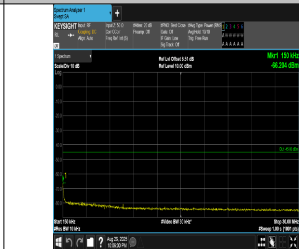
Band41(2555-2655)-15MHz-16QAM-40315-75RB#0-0.15~30-PASS
