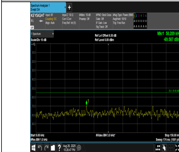
Band41(2555-2655)-15MHz-QPSK-41165-1RB#74-0.009~0.15-PASS
