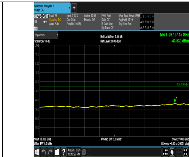
Band41(2555-2655)-15MHz-QPSK-40690-75RB#0-18000~27000-PASS
