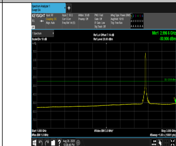
Band41(2555-2655)-15MHz-16QAM-40315-75RB#0-1000~3000-PASS
