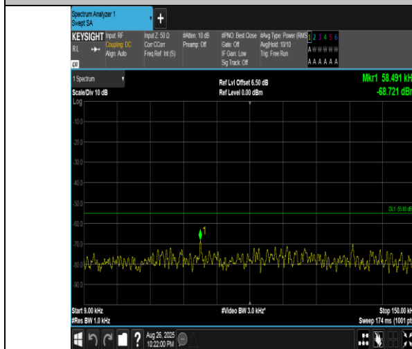
Band41(2555-2655)-15MHz-QPSK-41165-1RB#0-0.009~0.15-PASS
