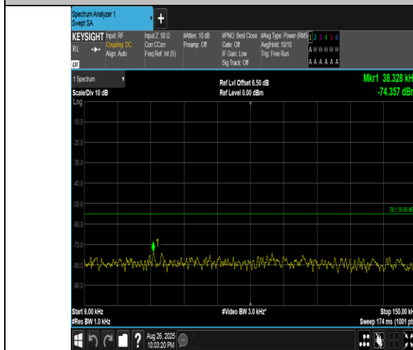
Band41(2555-2655)-15MHz-QPSK-40315-75RB#0-0.009~0.15-PASS
