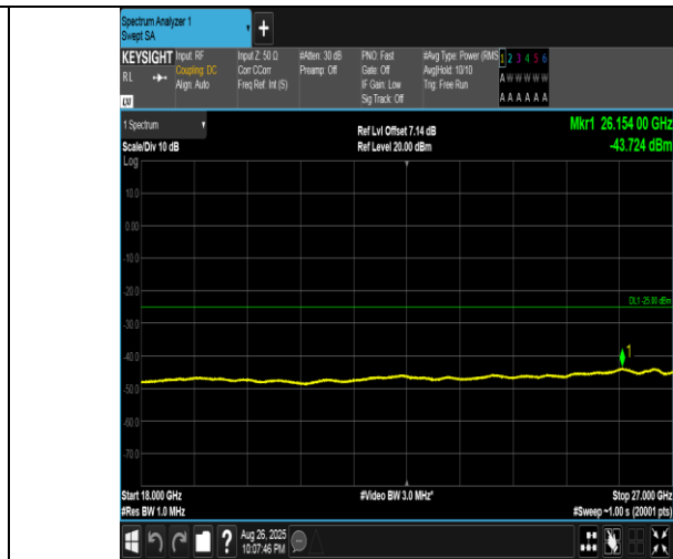
Band41(2555-2655)-15MHz-16QAM-40315-75RB#0-18000~27000-PASS
