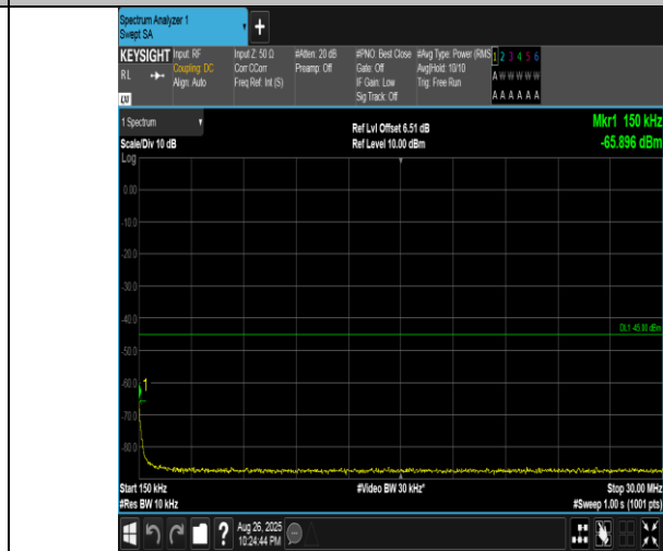
Band41(2555-2655)-15MHz-16QAM-41165-1RB#0-0.15~30-PASS
