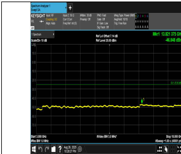
Band41(2555-2655)-15MHz-QPSK-41165-1RB#74-3000~18000-PASS
