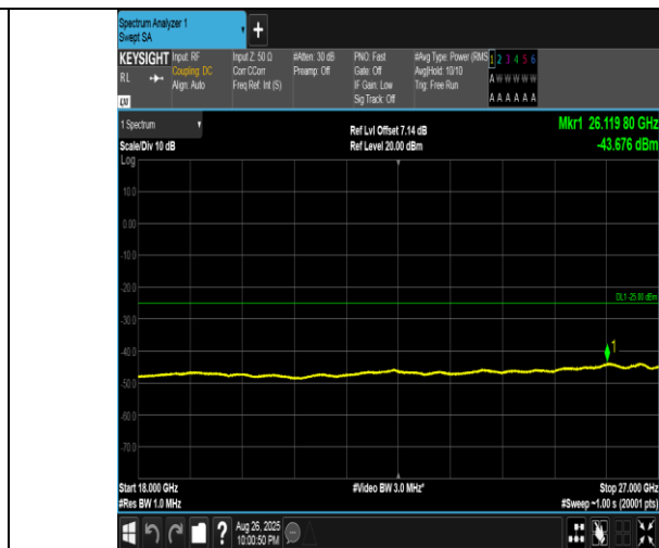
Band41(2555-2655)-15MHz-QPSK-40315-1RB#74-18000~27000-PASS
