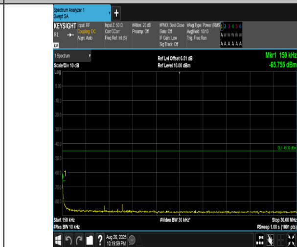
Band41(2555-2655)-15MHz-16QAM-40690-75RB#0-0.15~30-PASS
