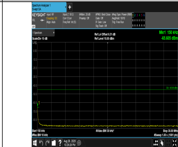
Band41(2555-2655)-15MHz-16QAM-41165-1RB#74-0.15~30-PASS
