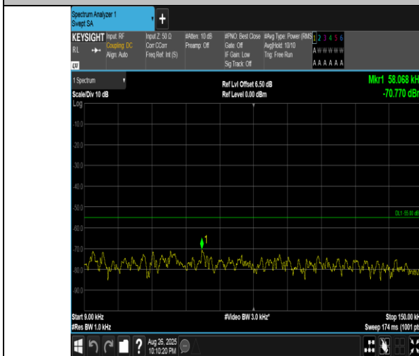
Band41(2555-2655)-15MHz-16QAM-40690-1RB#0-0.009~0.15-PASS
