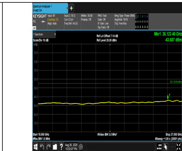
Band41(2555-2655)-15MHz-16QAM-40315-1RB#74-18000~27000-PASS
