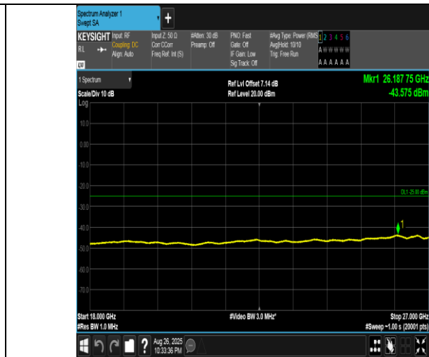
Band41(2555-2655)-15MHz-QPSK-41165-75RB#0-18000~27000-PASS
