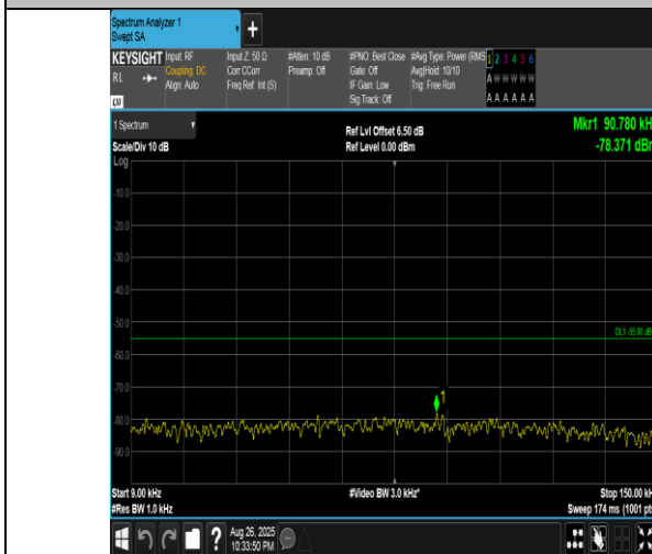
Band41(2555-2655)-15MHz-16QAM-41165-75RB#0-0.009~0.15-PASS
