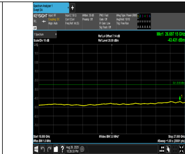
Band41(2555-2655)-15MHz-16QAM-41165-1RB#0-18000~27000-PASS
