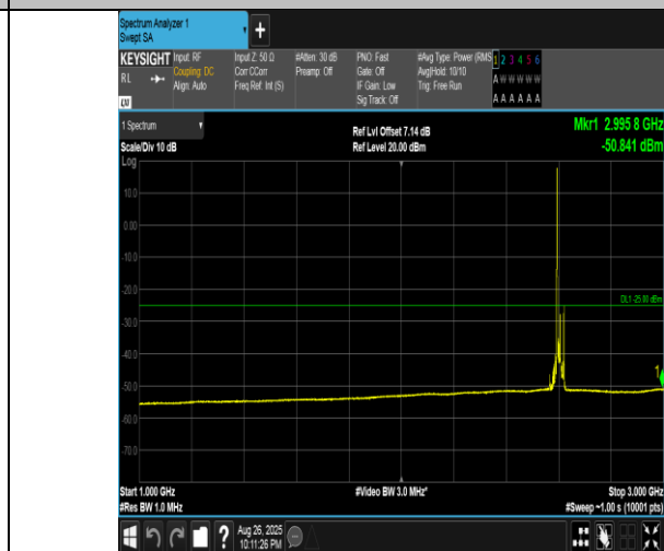
Band41(2555-2655)-15MHz-16QAM-40690-1RB#0-1000~3000-PASS
