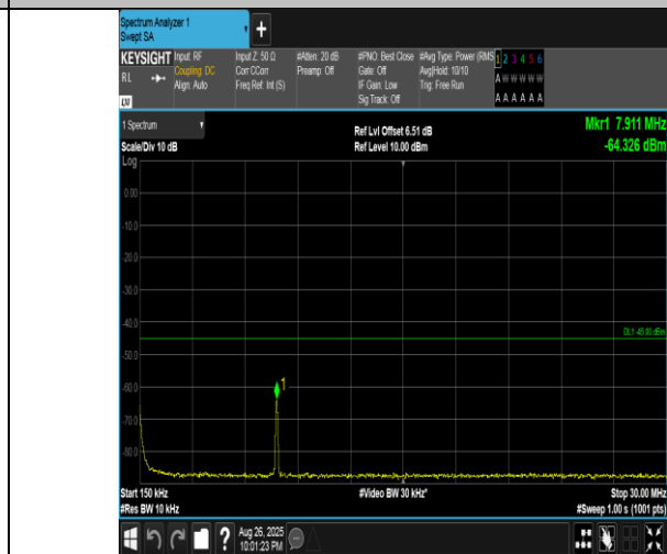
Band41(2555-2655)-15MHz-16QAM-40315-1RB#74-0.15~30-PASS
