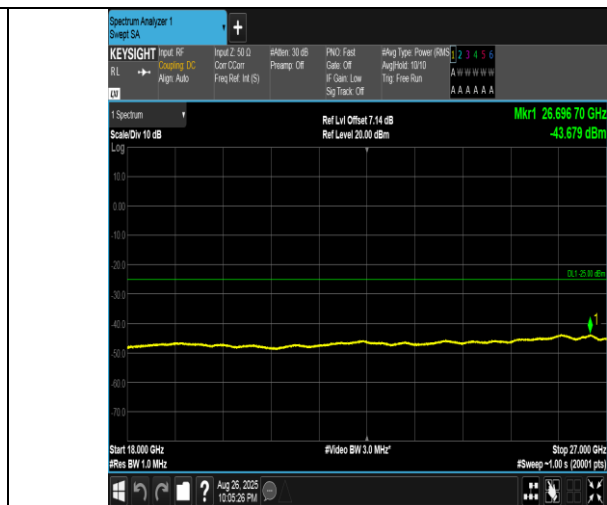
Band41(2555-2655)-15MHz-QPSK-40315-75RB#0-18000~27000-PASS
