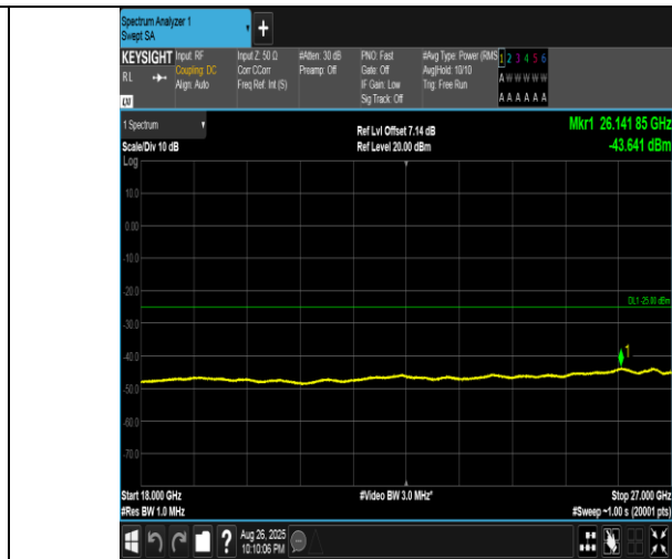
Band41(2555-2655)-15MHz-QPSK-40690-1RB#0-18000~27000-PASS
