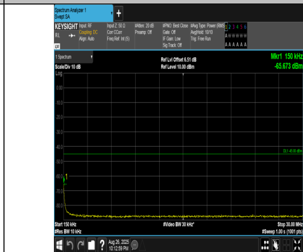
Band41(2555-2655)-15MHz-QPSK-40690-1RB#74-0.15~30-PASS
