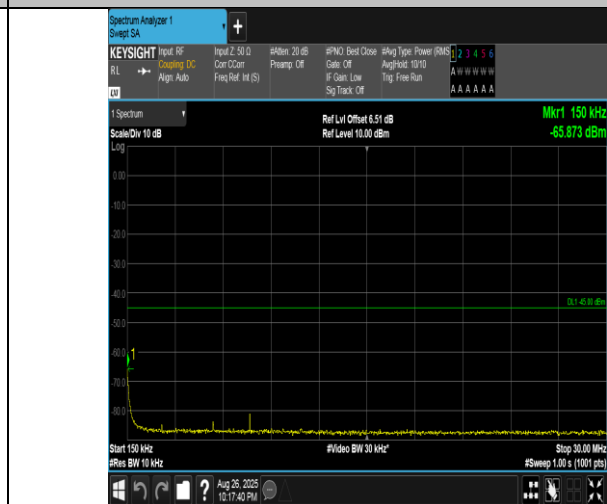
Band41(2555-2655)-15MHz-QPSK-40690-75RB#0-0.15~30-PASS
