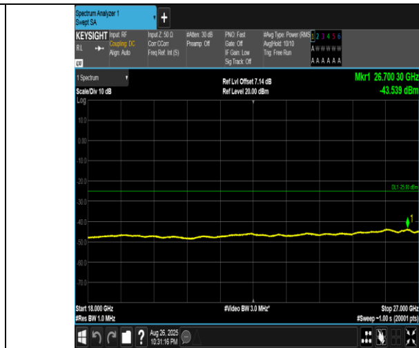
Band41(2555-2655)-15MHz-16QAM-41165-1RB#74-18000~27000-PASS
