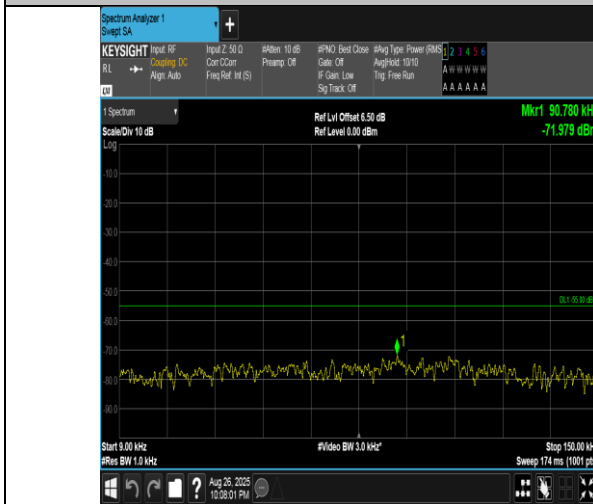
Band41(2555-2655)-15MHz-QPSK-40690-1RB#0-0.009~0.15-PASS
