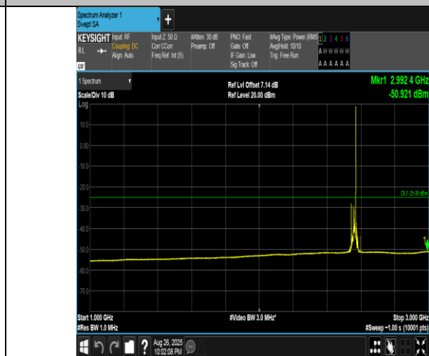
Band41(2555-2655)-15MHz-16QAM-40315-1RB#74-1000~3000-PASS
