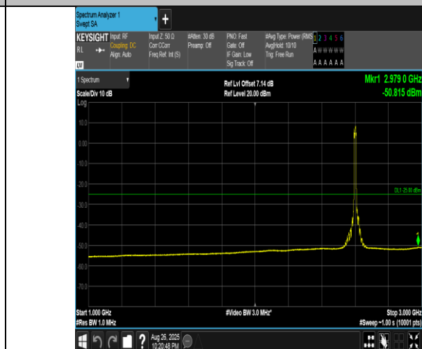
Band41(2555-2655)-15MHz-16QAM-40690-75RB#0-1000~3000-PASS
