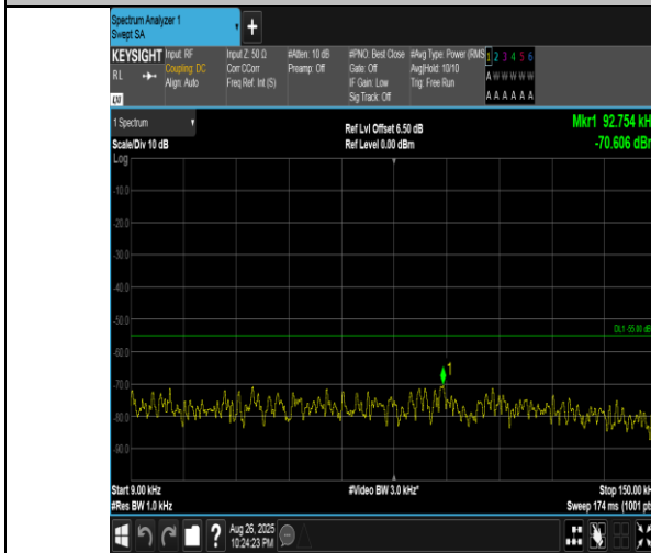
Band41(2555-2655)-15MHz-16QAM-41165-1RB#0-0.009~0.15-PASS
