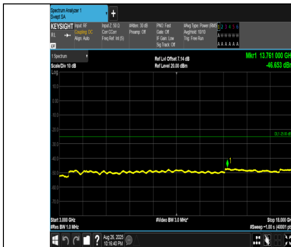
Band41(2555-2655)-15MHz-16QAM-40690-1RB#74-3000~18000-PASS
