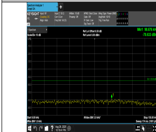
Band41(2555-2655)-15MHz-16QAM-40690-75RB#0-0.009~0.15-PASS
