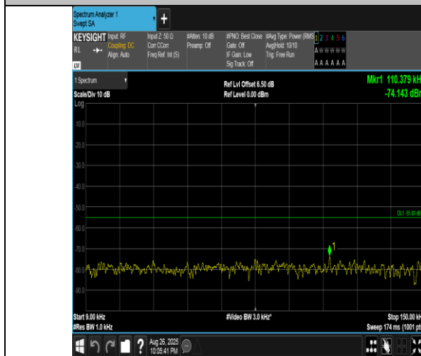
Band41(2555-2655)-15MHz-16QAM-40315-75RB#0-0.009~0.15-PASS
