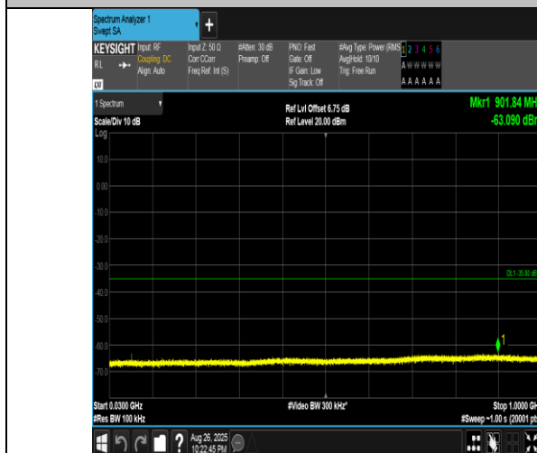
Band41(2555-2655)-15MHz-QPSK-41165-1RB#0-30~1000-PASS
