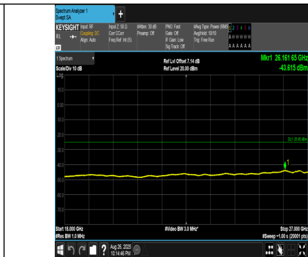
Band41(2555-2655)-15MHz-QPSK-40690-1RB#74-18000~27000-PASS
