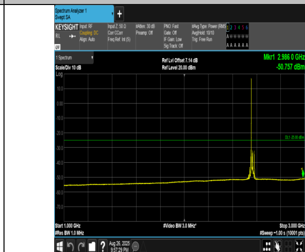
Band41(2555-2655)-15MHz-16QAM-40315-1RB#0-1000~3000-PASS
