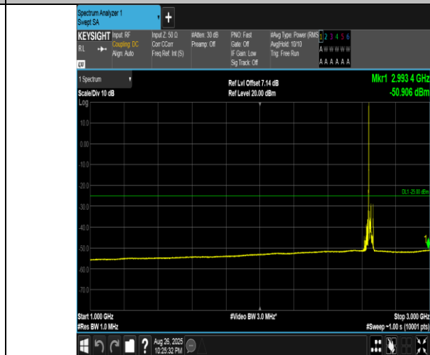
Band41(2555-2655)-15MHz-16QAM-41165-1RB#0-1000~3000-PASS
