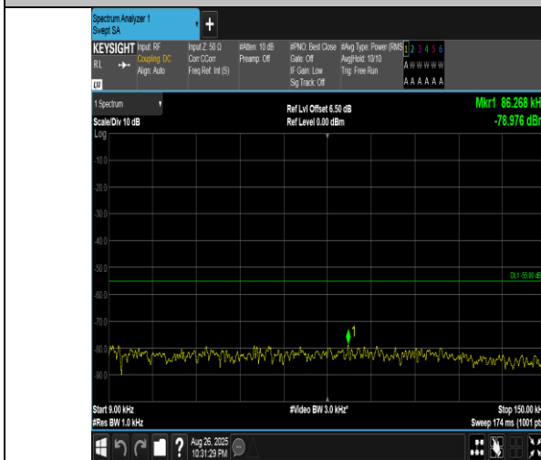
Band41(2555-2655)-15MHz-QPSK-41165-75RB#0-0.009~0.15-PASS
