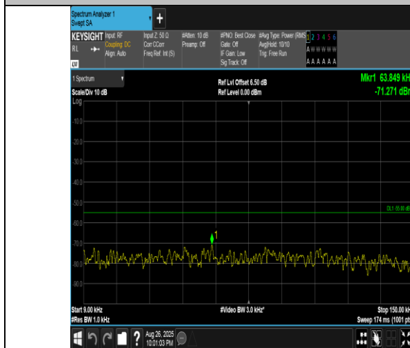
Band41(2555-2655)-15MHz-16QAM-40315-1RB#74-0.009~0.15-PASS
