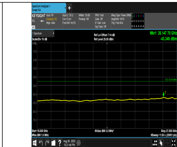
Band41(2555-2655)-15MHz-16QAM-40690-75RB#0-18000~27000-PASS
