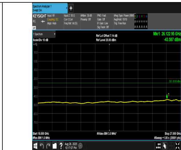
Band41(2555-2655)-15MHz-16QAM-40690-1RB#74-18000~27000-PASS
