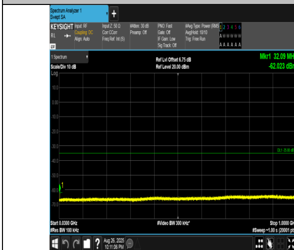
Band41(2555-2655)-15MHz-16QAM-40690-1RB#0-30~1000-PASS
