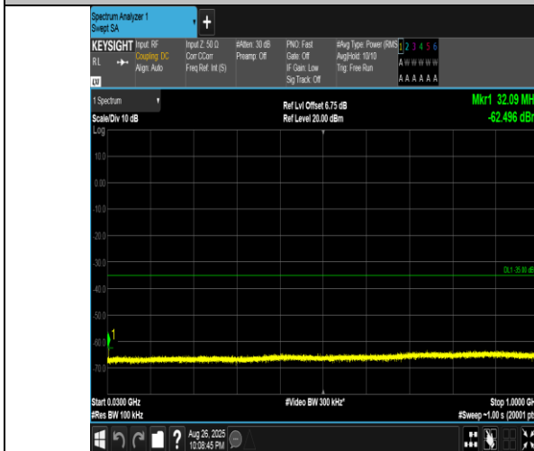
Band41(2555-2655)-15MHz-QPSK-40690-1RB#0-30~1000-PASS
