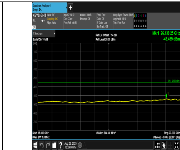
Band41(2555-2655)-15MHz-QPSK-41165-1RB#0-18000~27000-PASS
