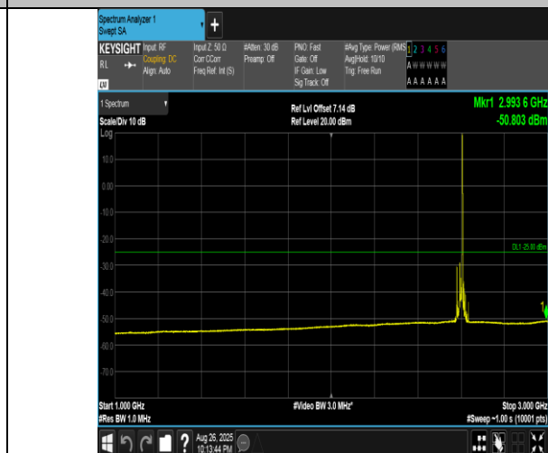
Band41(2555-2655)-15MHz-QPSK-40690-1RB#74-1000~3000-PASS
