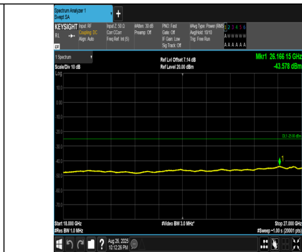
Band41(2555-2655)-15MHz-16QAM-40690-1RB#0-18000~27000-PASS
