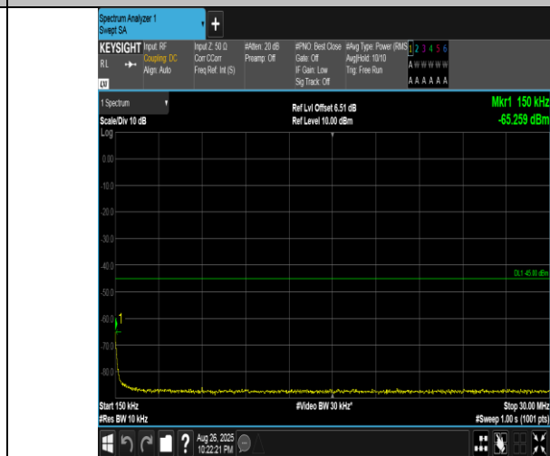
Band41(2555-2655)-15MHz-QPSK-41165-1RB#0-0.15~30-PASS
