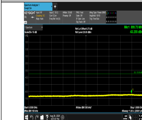
Band41(2555-2655)-15MHz-16QAM-40315-1RB#0-30~1000-PASS
