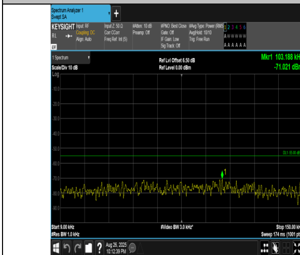
Band41(2555-2655)-15MHz-QPSK-40690-1RB#74-0.009~0.15-PASS
