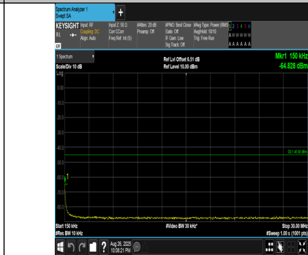
Band41(2555-2655)-15MHz-QPSK-40690-1RB#0-0.15~30-PASS
