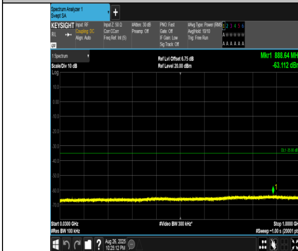
Band41(2555-2655)-15MHz-16QAM-41165-1RB#0-30~1000-PASS
