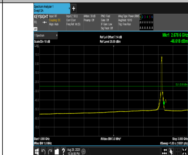
Band41(2555-2655)-15MHz-16QAM-41165-75RB#0-1000~3000-PASS
