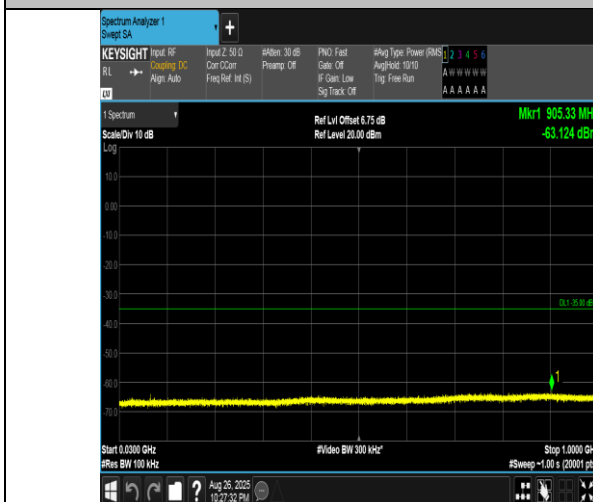
Band41(2555-2655)-15MHz-QPSK-41165-1RB#74-30~1000-PASS
