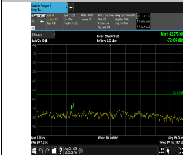
Band41(2555-2655)-15MHz-16QAM-41165-1RB#74-0.009~0.15-PASS
