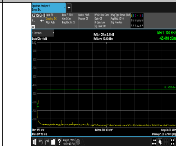
Band41(2555-2655)-15MHz-QPSK-41165-75RB#0-0.15~30-PASS
