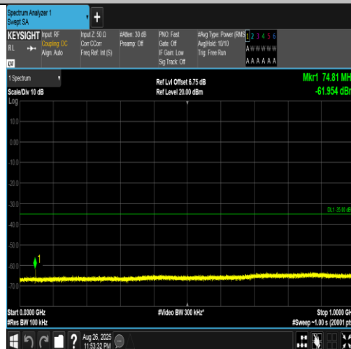
Band41(2555-2655)-20MHz-QPSK-41140-1RB#0-30~1000-PASS
