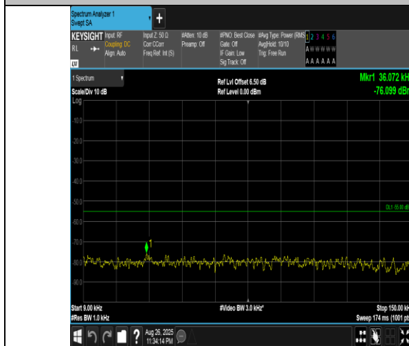
Band41(2555-2655)-20MHz-QPSK-40340-100RB#0-0.009~0.15-PASS
