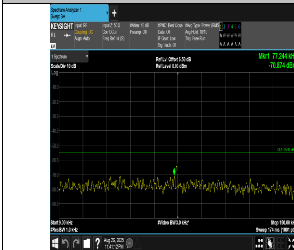
Band41(2555-2655)-20MHz-16QAM-40690-1RB#0-0.009~0.15-PASS
