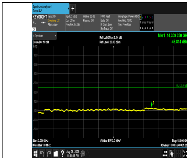
Band41(2555-2655)-20MHz-QPSK-40340-1RB#99-3000~18000-PASS
