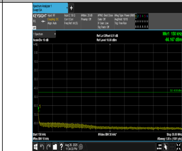
Band41(2555-2655)-20MHz-QPSK-40340-100RB#0-0.15~30-PASS
