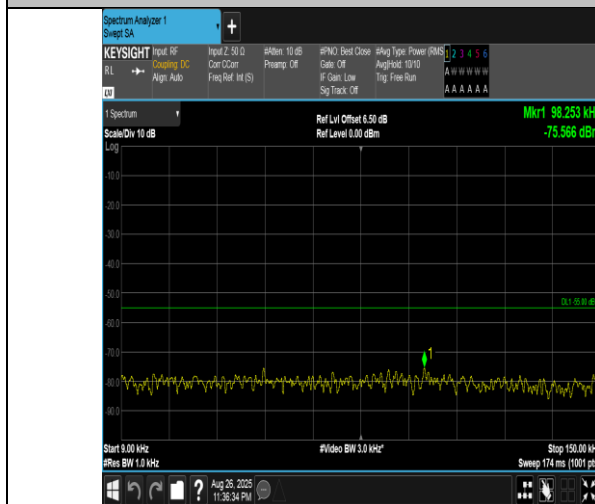
Band41(2555-2655)-20MHz-16QAM-40340-100RB#0-0.009~0.15-PASS
