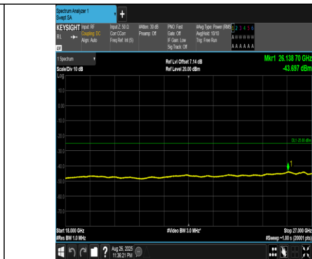
Band41(2555-2655)-20MHz-QPSK-40340-100RB#0-18000~27000-PASS
