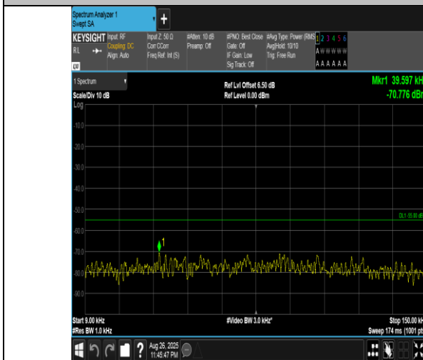
Band41(2555-2655)-20MHz-16QAM-40690-1RB#99-0.009~0.15-PASS
