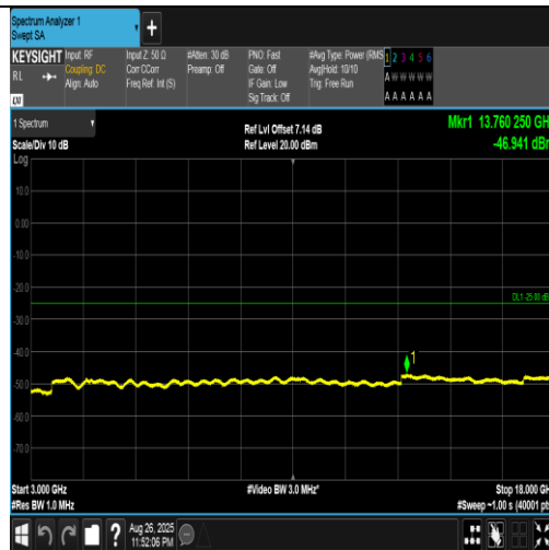
Band41(2555-2655)-20MHz-16QAM-40690-100RB#0-3000~18000-PASS
