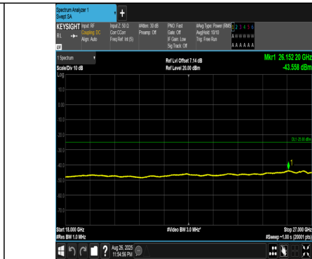
Band41(2555-2655)-20MHz-QPSK-41140-1RB#0-18000~27000-PASS
