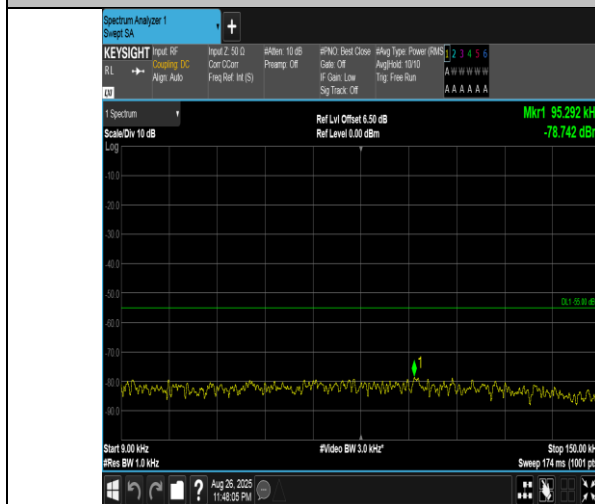
Band41(2555-2655)-20MHz-QPSK-40690-100RB#0-0.009~0.15-PASS
