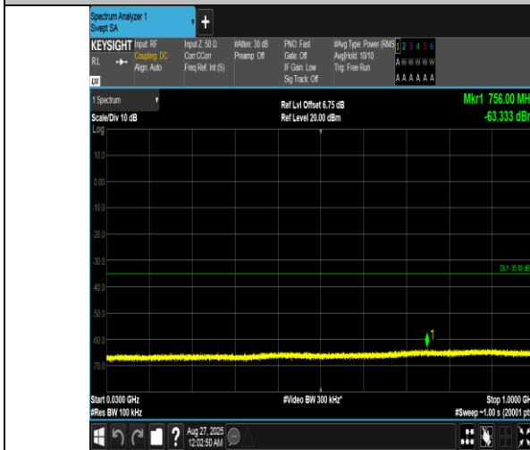
Band41(2555-2655)-20MHz-QPSK-41140-100RB#0-30~1000-PASS
