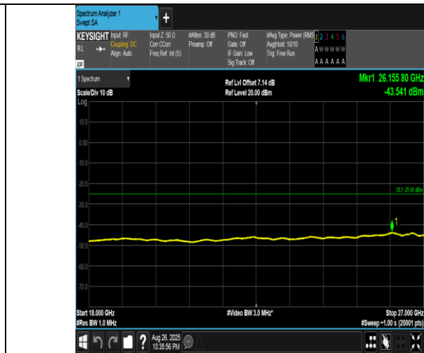
Band41(2555-2655)-15MHz-16QAM-41165-75RB#0-18000~27000-PASS
