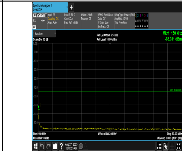
Band41(2555-2655)-20MHz-QPSK-41140-100RB#0-0.15~30-PASS
