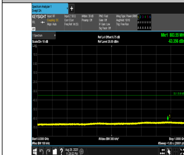
Band41(2555-2655)-20MHz-16QAM-40340-1RB#0-30~1000-PASS
