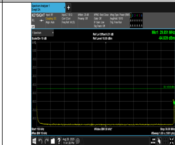
Band41(2555-2655)-20MHz-16QAM-40690-1RB#0-0.15~30-PASS
