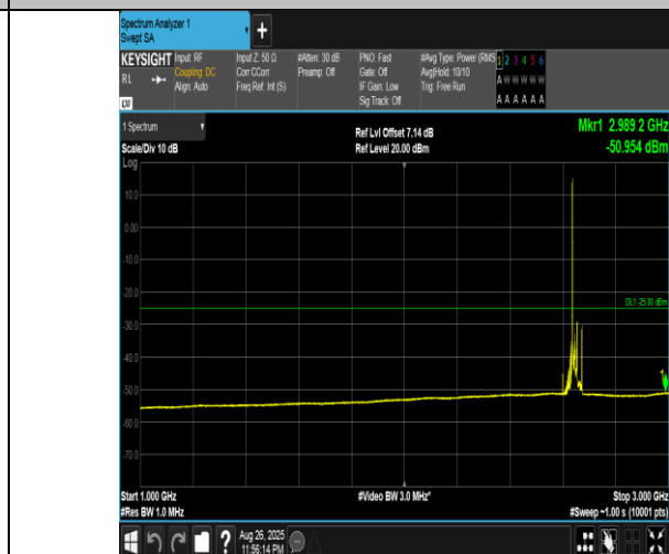
Band41(2555-2655)-20MHz-16QAM-41140-1RB#0-1000~3000-PASS
