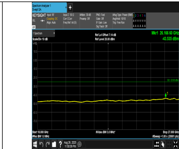
Band41(2555-2655)-20MHz-QPSK-40690-100RB#0-18000~27000-PASS
