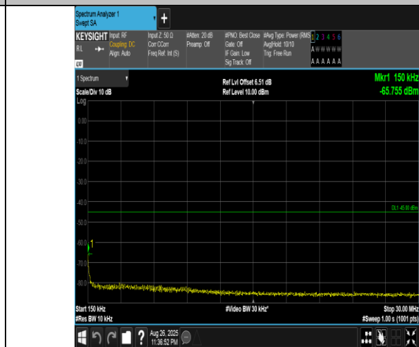
Band41(2555-2655)-20MHz-16QAM-40340-100RB#0-0.15~30-PASS
