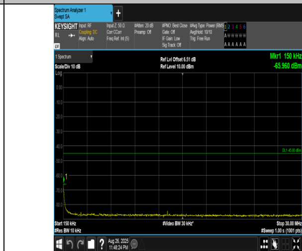
Band41(2555-2655)-20MHz-QPSK-40690-100RB#0-0.15~30-PASS
