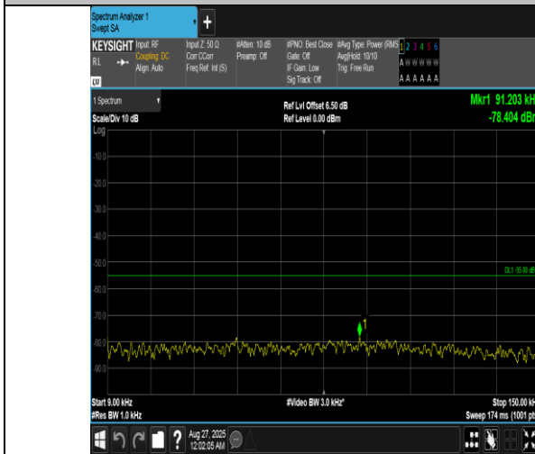
Band41(2555-2655)-20MHz-QPSK-41140-100RB#0-0.009~0.15-PASS
