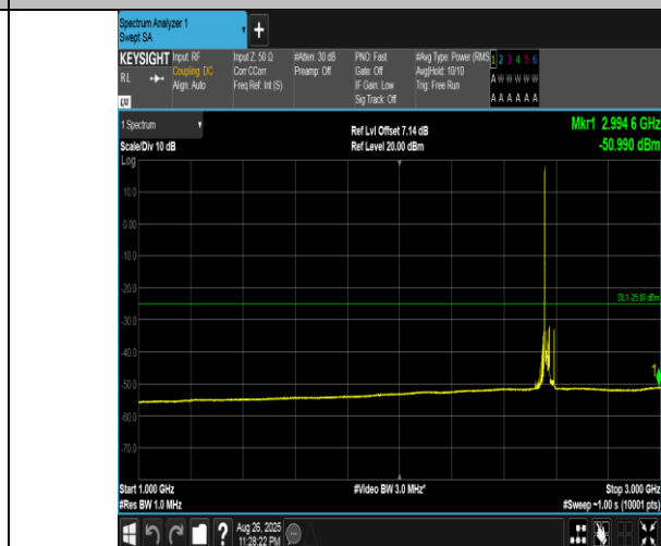
Band41(2555-2655)-20MHz-16QAM-40340-1RB#0-1000~3000-PASS
