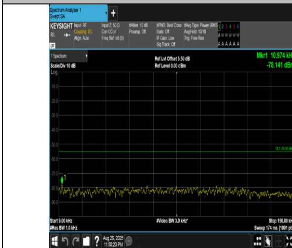
Band41(2555-2655)-20MHz-16QAM-40690-100RB#0-0.009~0.15-PASS
