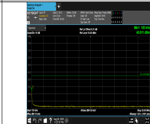
Band41(2555-2655)-20MHz-16QAM-40340-1RB#0-0.15~30-PASS
