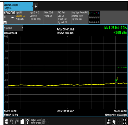
Band41(2555-2655)-20MHz-16QAM-40690-100RB#0-18000~27000-PASS
