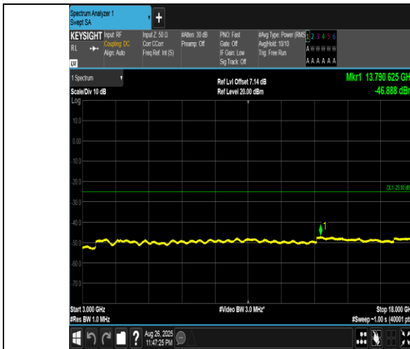
Band41(2555-2655)-20MHz-16QAM-40690-1RB#99-3000~18000-PASS
