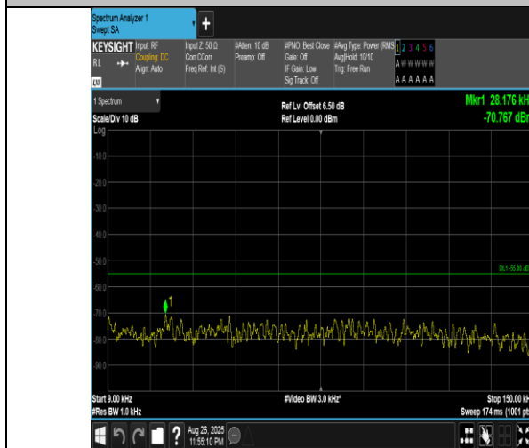
Band41(2555-2655)-20MHz-16QAM-41140-1RB#0-0.009~0.15-PASS
