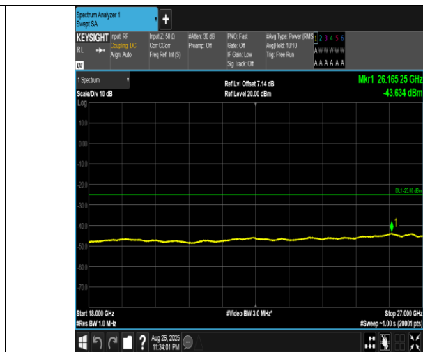
Band41(2555-2655)-20MHz-16QAM-40340-1RB#99-18000~27000-PASS
