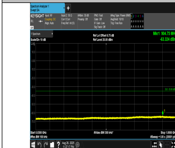
Band41(2555-2655)-20MHz-16QAM-40340-100RB#0-30~1000-PASS
