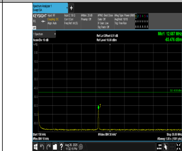
Band41(2555-2655)-20MHz-16QAM-40340-1RB#99-0.15~30-PASS
