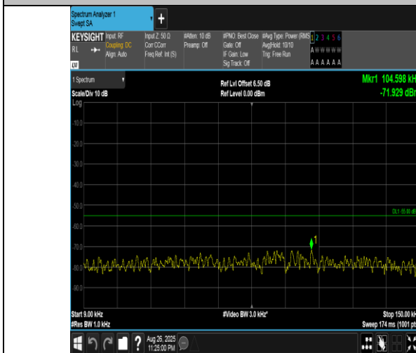
Band41(2555-2655)-20MHz-QPSK-40340-1RB#0-0.009~0.15-PASS
