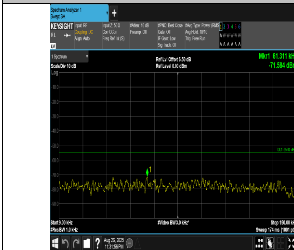
Band41(2555-2655)-20MHz-16QAM-40340-1RB#99-0.009~0.15-PASS
