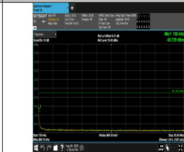
Band41(2555-2655)-20MHz-16QAM-40690-100RB#0-0.15~30-PASS
