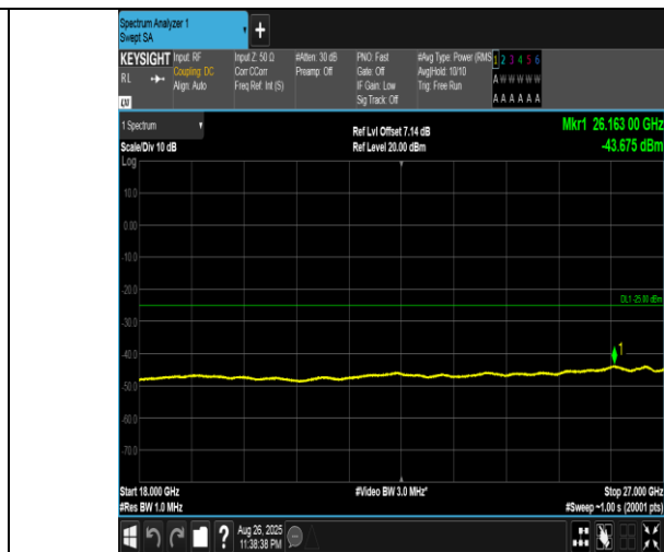
Band41(2555-2655)-20MHz-16QAM-40340-100RB#0-18000~27000-PASS
