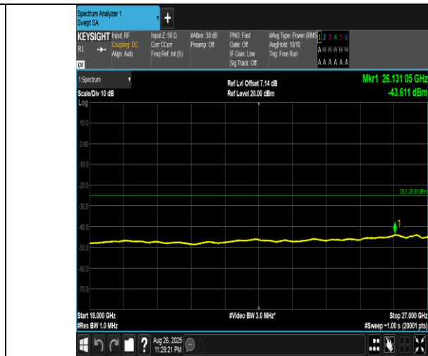
Band41(2555-2655)-20MHz-16QAM-40340-1RB#0-18000~27000-PASS
