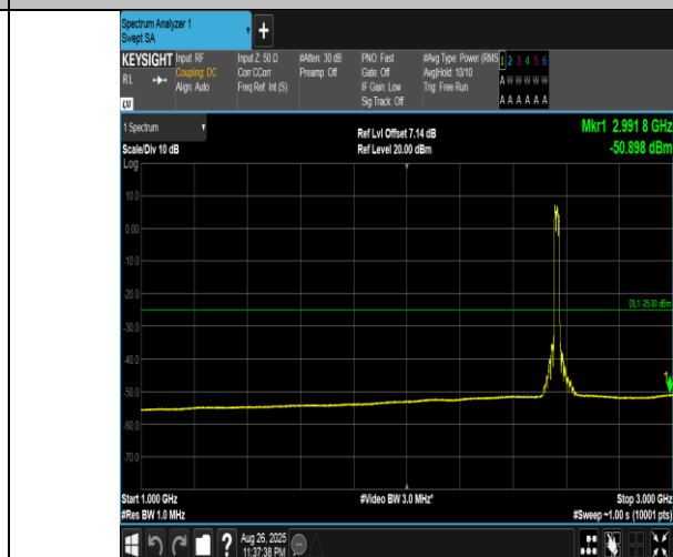
Band41(2555-2655)-20MHz-16QAM-40340-100RB#0-1000~3000-PASS
