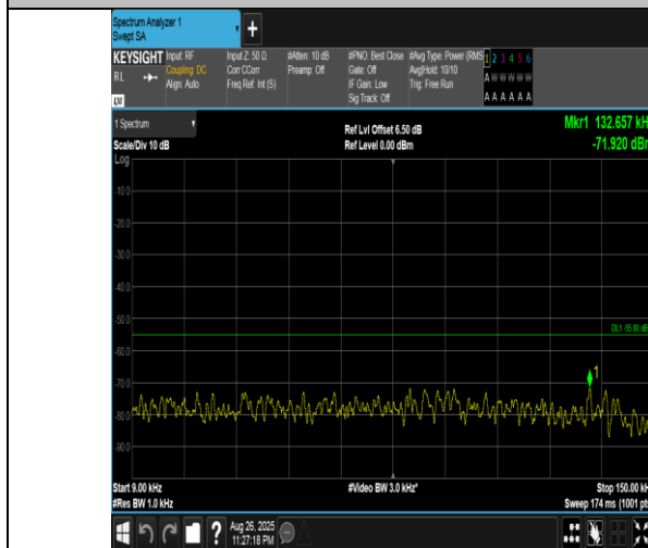
Band41(2555-2655)-20MHz-16QAM-40340-1RB#0-0.009~0.15-PASS
