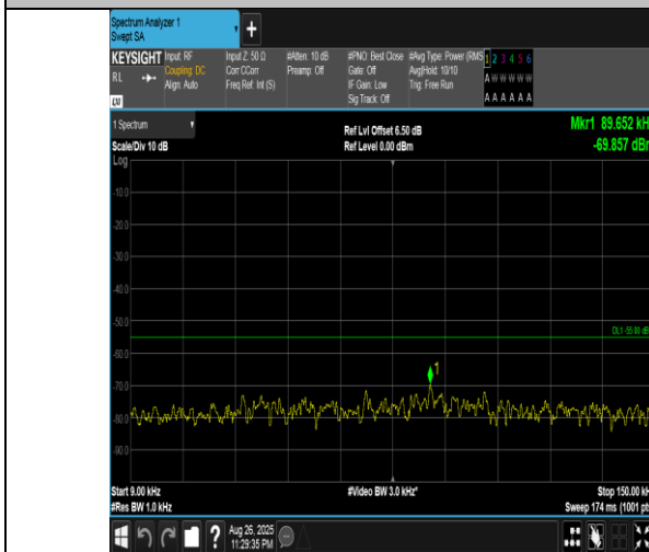
Band41(2555-2655)-20MHz-QPSK-40340-1RB#99-0.009~0.15-PASS
