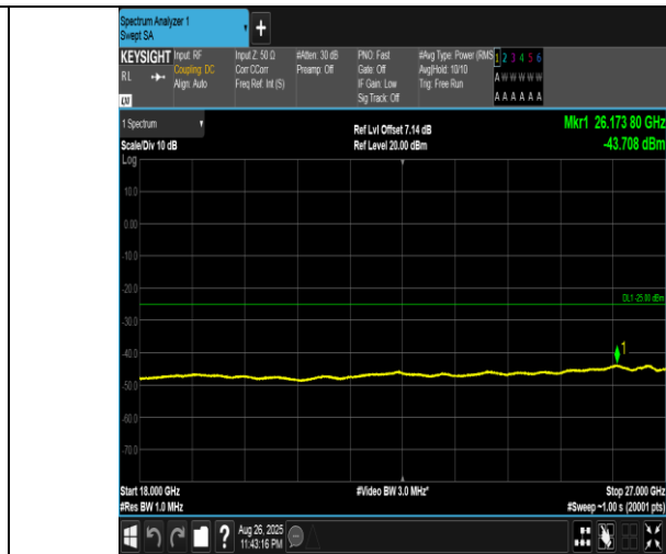
Band41(2555-2655)-20MHz-16QAM-40690-1RB#0-18000~27000-PASS
