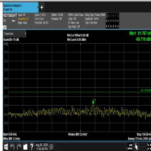
Band41(2555-2655)-20MHz-QPSK-41140-1RB#0-0.009~0.15-PASS
