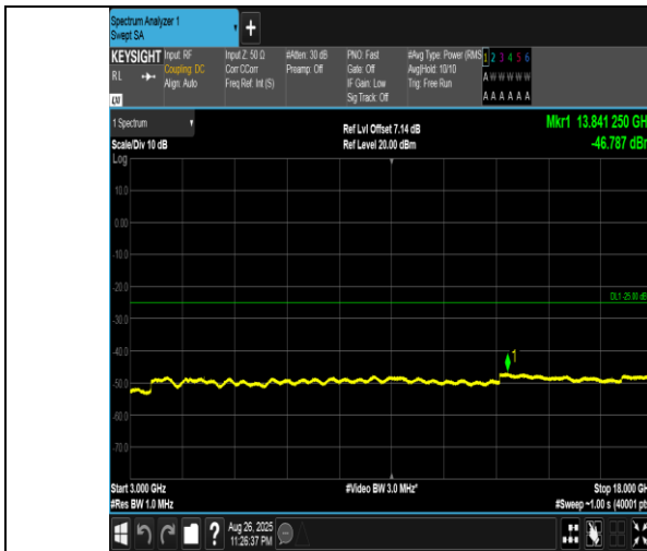
Band41(2555-2655)-20MHz-QPSK-40340-1RB#0-3000~18000-PASS
