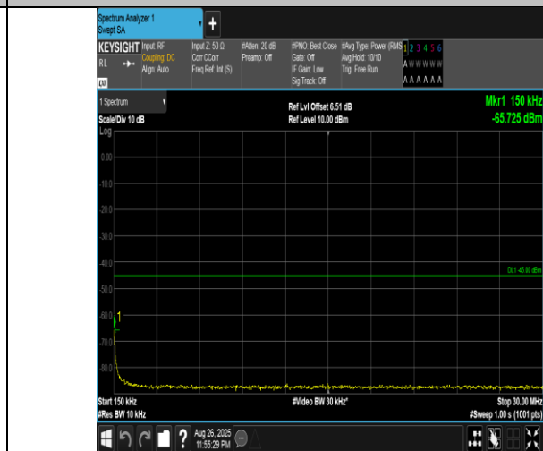
Band41(2555-2655)-20MHz-16QAM-41140-1RB#0-0.15~30-PASS
