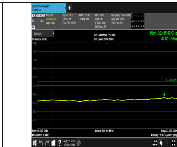
Band41(2555-2655)-20MHz-QPSK-41140-100RB#0-18000~27000-PASS
