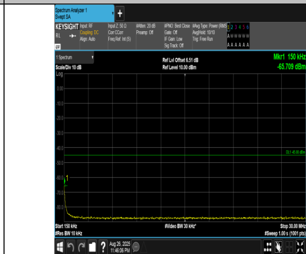
Band41(2555-2655)-20MHz-16QAM-40690-1RB#99-0.15~30-PASS
