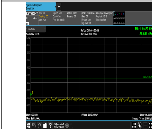
Band41(2555-2655)-20MHz-16QAM-41140-100RB#0-0.009~0.15-PASS
