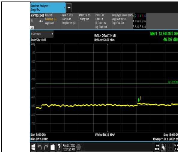
Band41(2555-2655)-20MHz-16QAM-41140-1RB#99-3000~18000-PASS
