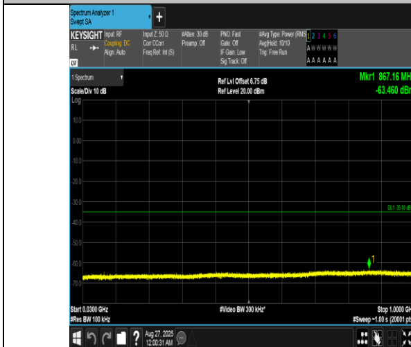
Band41(2555-2655)-20MHz-16QAM-41140-1RB#99-30~1000-PASS
