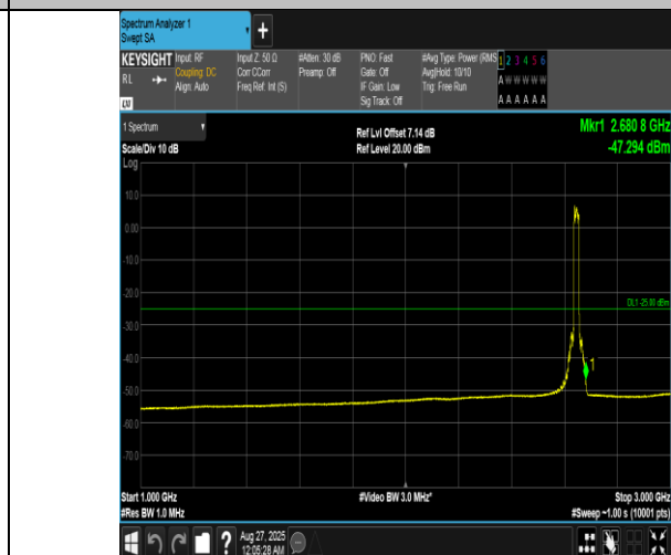
Band41(2555-2655)-20MHz-16QAM-41140-100RB#0-1000~3000-PASS
