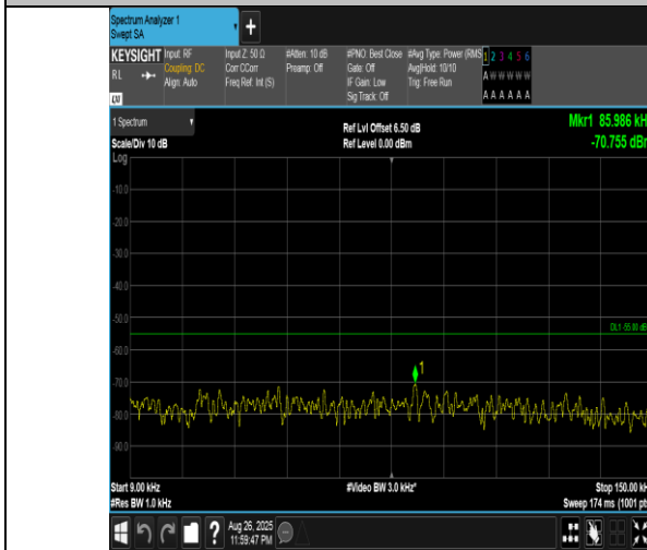
Band41(2555-2655)-20MHz-16QAM-41140-1RB#99-0.009~0.15-PASS
