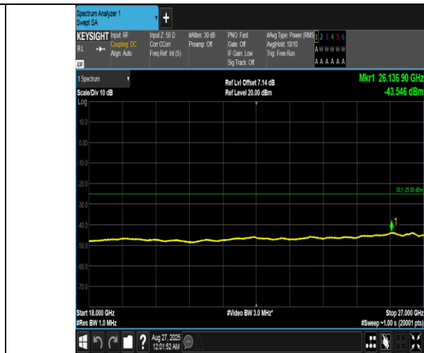
Band41(2555-2655)-20MHz-16QAM-41140-1RB#99-18000~27000-PASS
