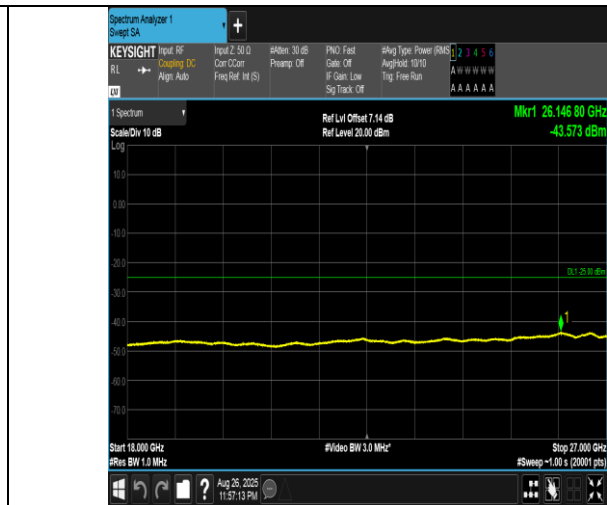
Band41(2555-2655)-20MHz-16QAM-41140-1RB#0-18000~27000-PASS
