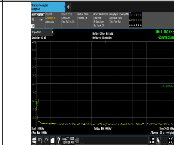
Band41(2555-2655)-20MHz-16QAM-41140-1RB#99-0.15~30-PASS
