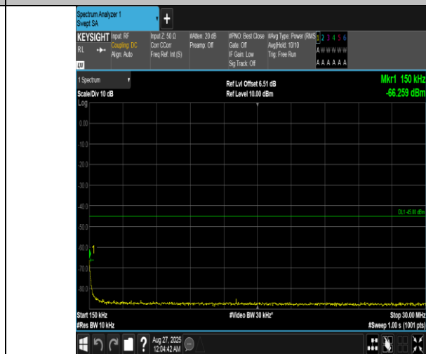
Band41(2555-2655)-20MHz-16QAM-41140-100RB#0-0.15~30-PASS
