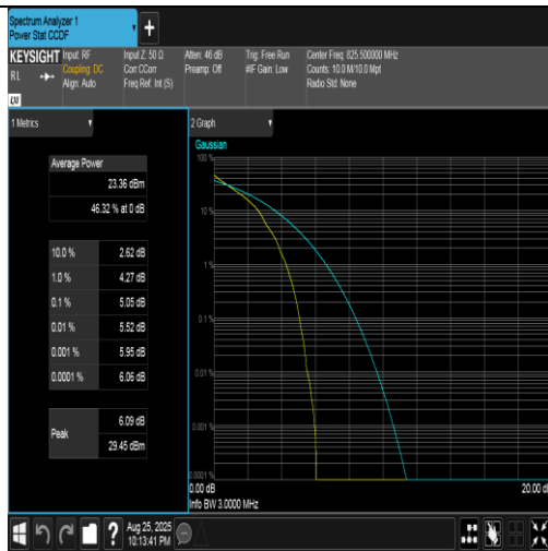
Band5-3MHz-QPSK-20415-1RB#0-PASS
