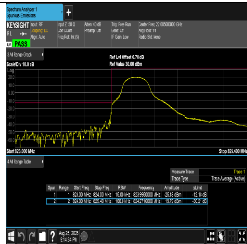
Band5-1.4MHz-16QAM-20407-1RB#0-PASS
