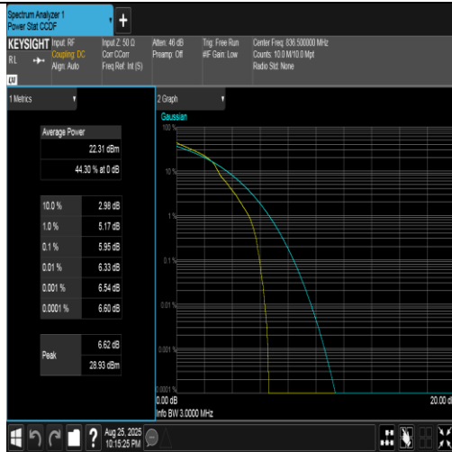
Band5-3MHz-16QAM-20525-1RB#0-PASS
