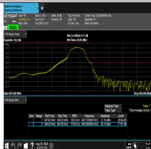
Band5-1.4MHz-QPSK-20643-1RB#5-PASS
