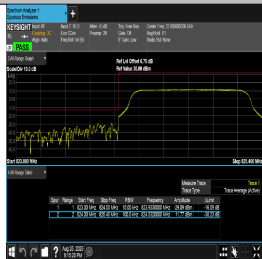
Band5-1.4MHz-16QAM-20407-6RB#0-PASS
