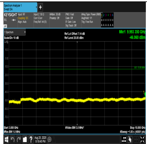
Band5-1.4MHz-QPSK-20407-1RB#5-3000~10000-PASS
