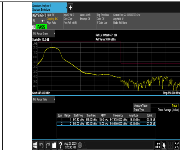
Band5-1.4MHz-16QAM-20643-1RB#0-PASS
