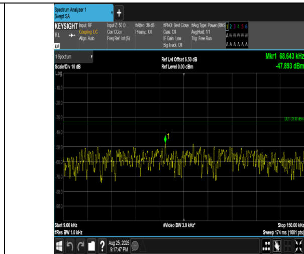
Band5-1.4MHz-16QAM-20407-1RB#0-0.009~0.15-PASS
