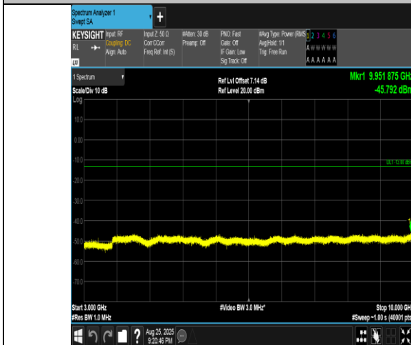
Band5-1.4MHz-16QAM-20407-1RB#5-3000~10000-PASS
