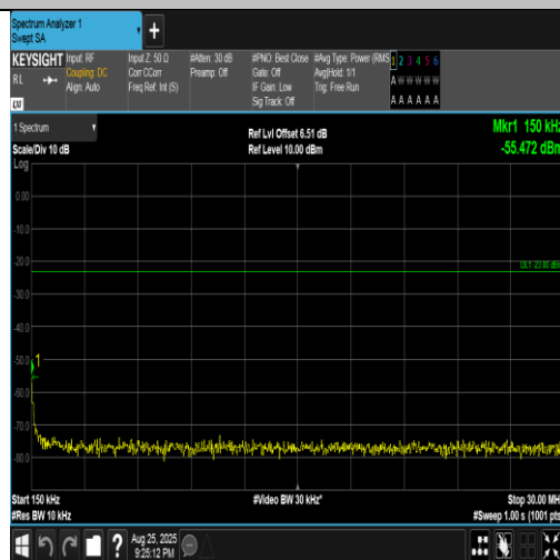
Band5-1.4MHz-QPSK-20525-1RB#5-0.15~30-PASS
