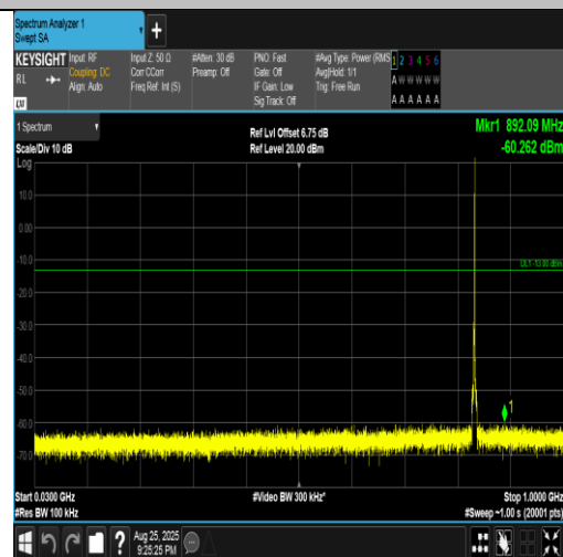
Band5-1.4MHz-QPSK-20525-1RB#5-30~1000-PASS
