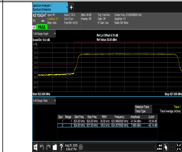
Band5-3MHz-16QAM-20415-15RB#0-PASS
