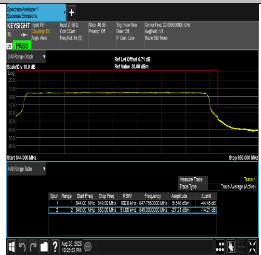
Band5-5MHz-16QAM-20625-25RB#0-PASS
