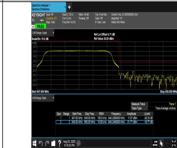
Band5-1.4MHz-16QAM-20643-6RB#0-PASS
