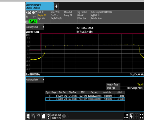
Band5-10MHz-16QAM-20450-50RB#0-PASS
