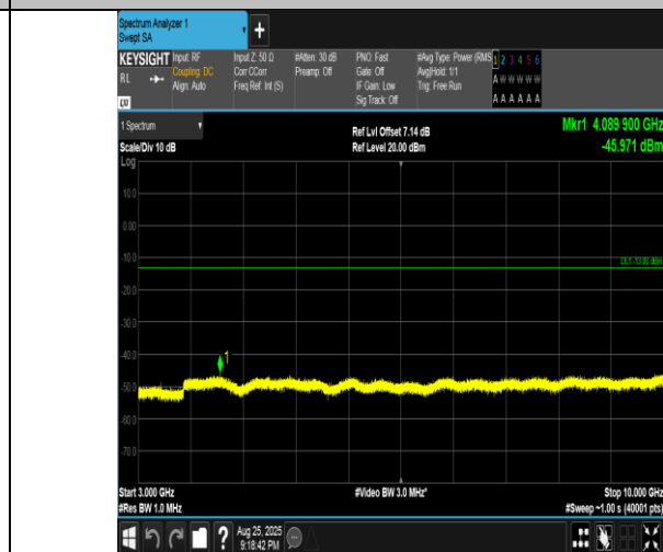
Band5-1.4MHz-16QAM-20407-1RB#0-3000~10000-PASS
