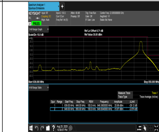
Band5-10MHz-QPSK-20600-1RB#49-PASS
