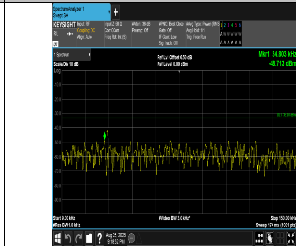
Band5-1.4MHz-QPSK-20407-1RB#5-0.009~0.15-PASS
