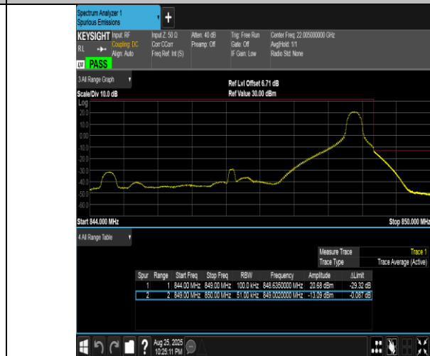
Band5-5MHz-QPSK-20625-1RB#24-PASS
