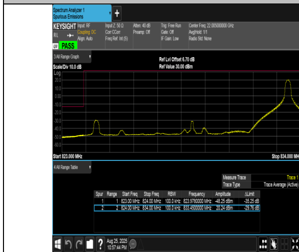
Band5-10MHz-16QAM-20450-1RB#49-PASS
