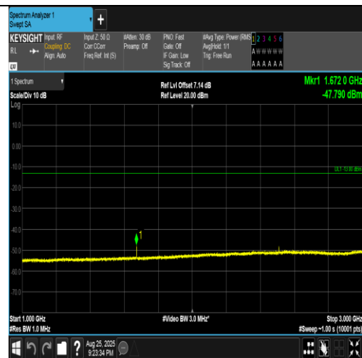
Band5-1.4MHz-QPSK-20525-1RB#0-1000~3000-PASS
