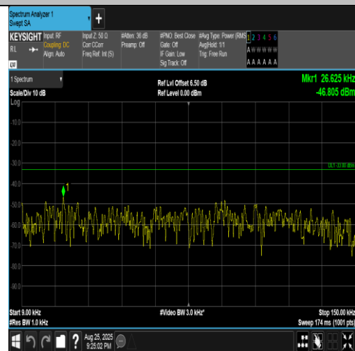
Band5-1.4MHz-QPSK-20525-1RB#5-0.009~0.15-PASS
