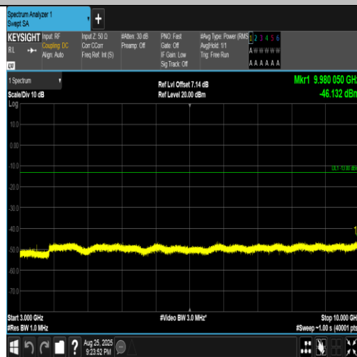
Band5-1.4MHz-QPSK-20525-1RB#0-3000~10000-PASS
