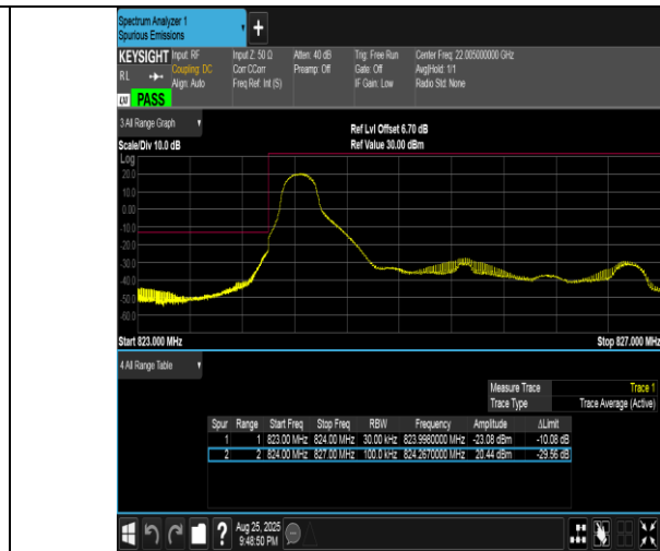
Band5-3MHz-16QAM-20415-1RB#0-PASS
