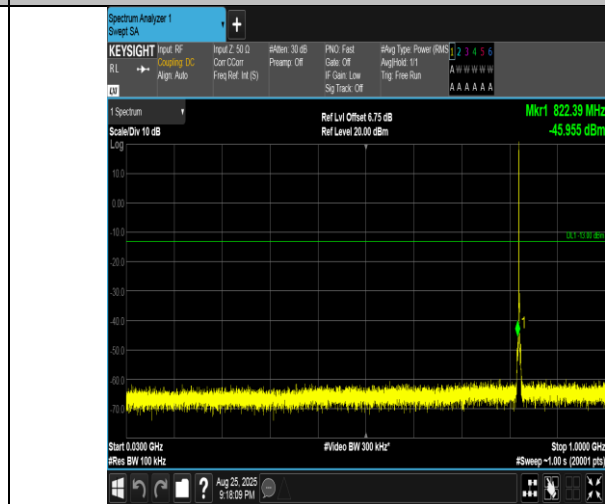
Band5-1.4MHz-16QAM-20407-1RB#0-30~1000-PASS
