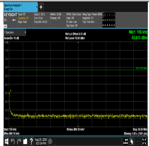
Band5-1.4MHz-QPSK-20407-6RB#0-0.15~30-PASS
