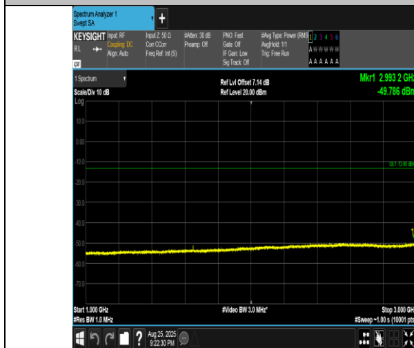
Band5-1.4MHz-16QAM-20407-6RB#0-1000~3000-PASS
