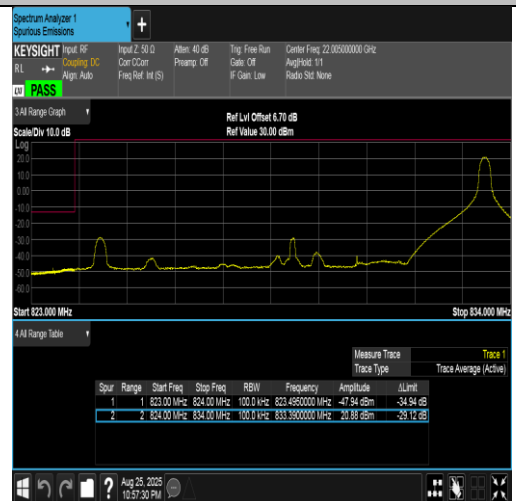
Band5-10MHz-QPSK-20450-1RB#49-PASS
