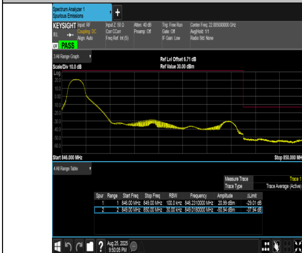
Band5-3MHz-QPSK-20635-1RB#0-PASS
