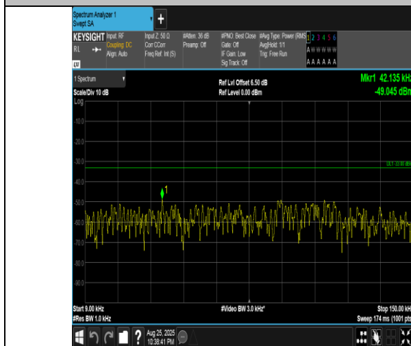
Band5-5MHz-QPSK-20625-1RB#0-0.009~0.15-PASS
