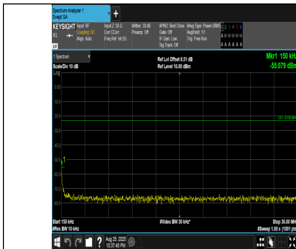
Band5-5MHz-16QAM-20525-25RB#0-0.15~30-PASS
