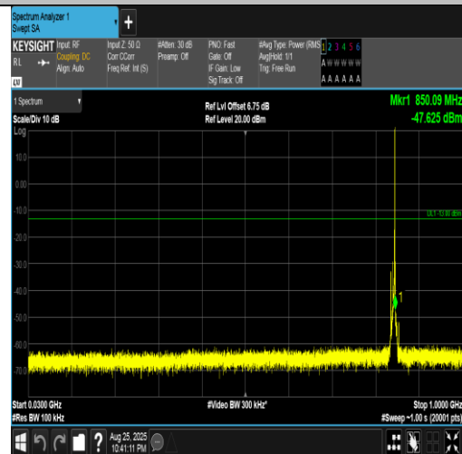
Band5-5MHz-QPSK-20625-1RB#24-30~1000-PASS
