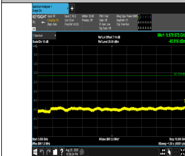
Band5-5MHz-16QAM-20525-1RB#24-3000~10000-PASS
