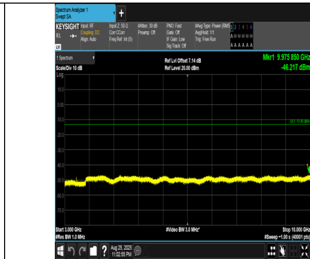
Band5-10MHz-QPSK-20450-1RB#49-3000~10000-PASS
