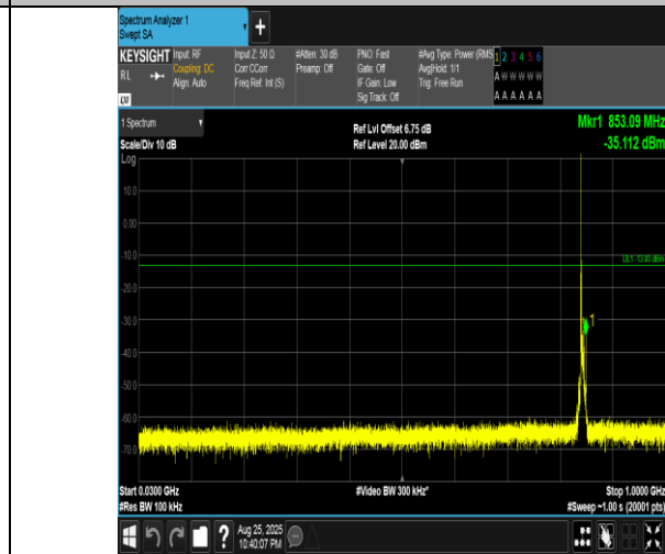
Band5-5MHz-16QAM-20625-1RB#0-30~1000-PASS
