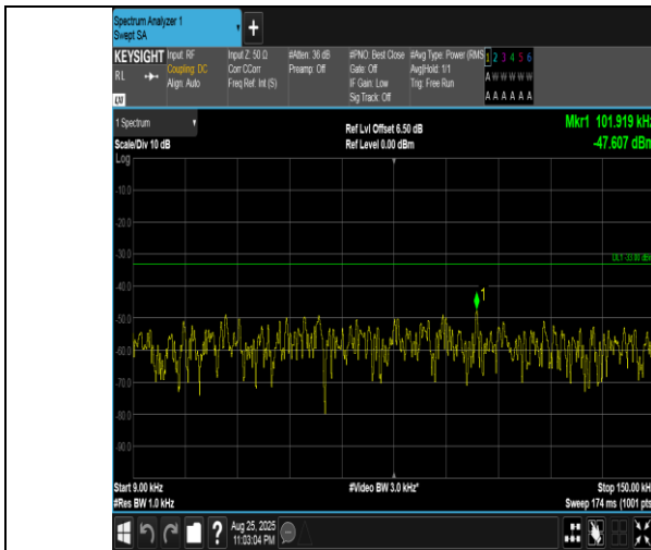
Band5-10MHz-16QAM-20450-1RB#49-0.009~0.15-PASS
