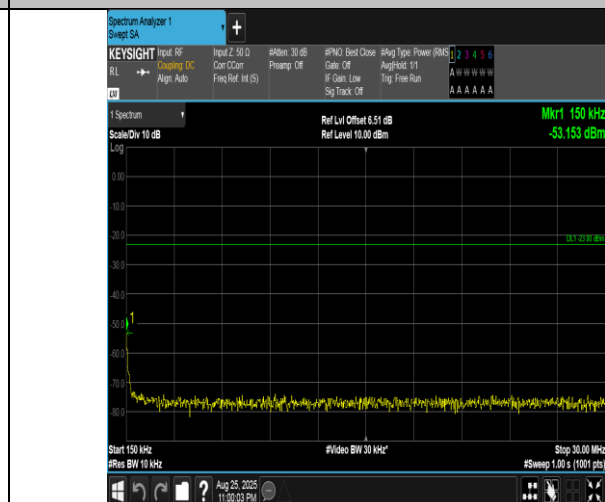
Band5-10MHz-QPSK-20450-1RB#0-0.15~30-PASS
