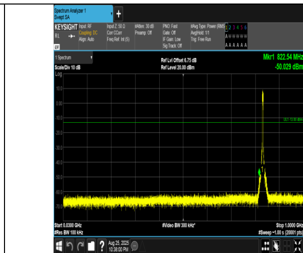
Band5-5MHz-16QAM-20525-25RB#0-30~1000-PASS
