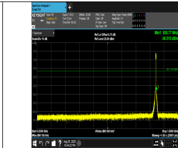
Band5-5MHz-16QAM-20625-25RB#0-30~1000-PASS
