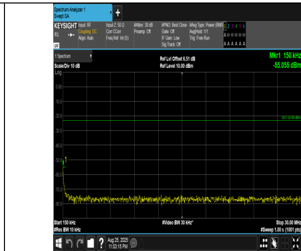
Band5-10MHz-16QAM-20450-1RB#49-0.15~30-PASS
