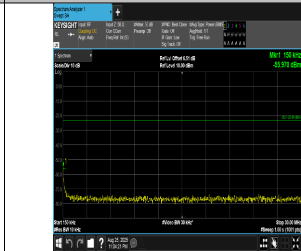
Band5-10MHz-QPSK-20450-50RB#0-0.15~30-PASS
