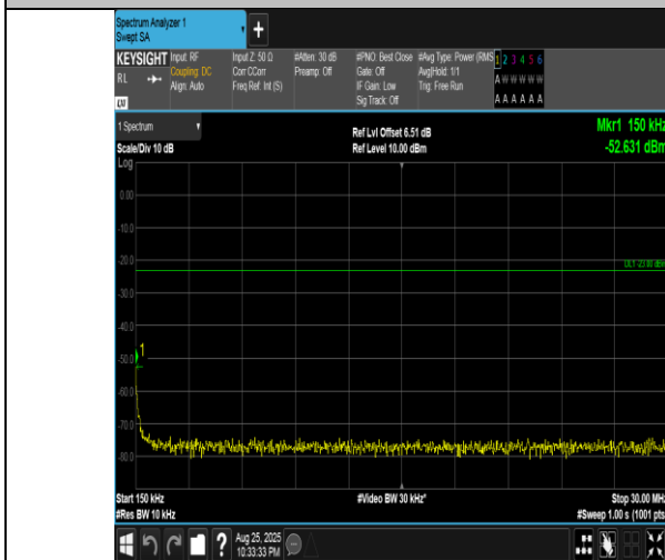
Band5-5MHz-16QAM-20525-1RB#0-0.15~30-PASS
