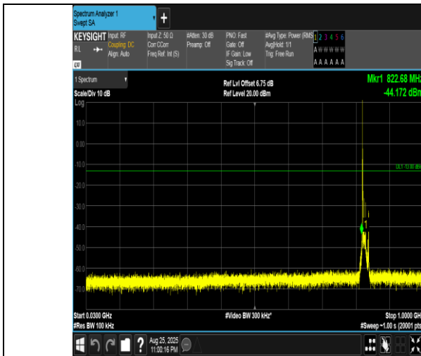
Band5-10MHz-QPSK-20450-1RB#0-30~1000-PASS
