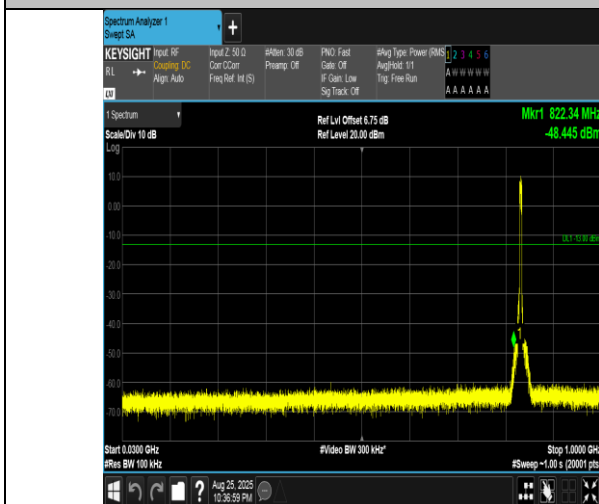
Band5-5MHz-QPSK-20525-25RB#0-30~1000-PASS
