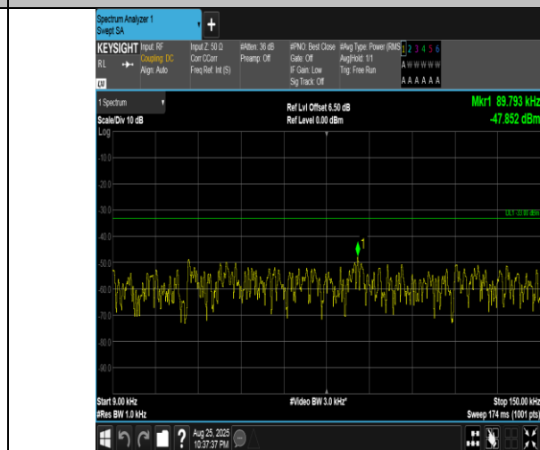
Band5-5MHz-16QAM-20525-25RB#0-0.009~0.15-PASS
