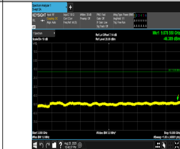
Band5-5MHz-16QAM-20625-1RB#0-3000~10000-PASS
