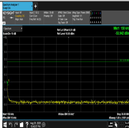
Band5-5MHz-QPSK-20625-1RB#24-0.15~30-PASS
