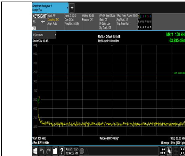
Band5-5MHz-16QAM-20625-25RB#0-0.15~30-PASS
