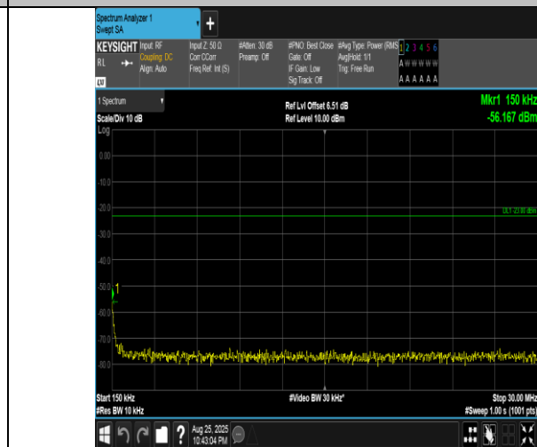
Band5-5MHz-QPSK-20625-25RB#0-0.15~30-PASS
