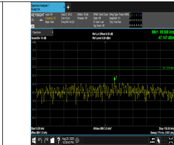
Band5-5MHz-16QAM-20625-1RB#0-0.009~0.15-PASS
