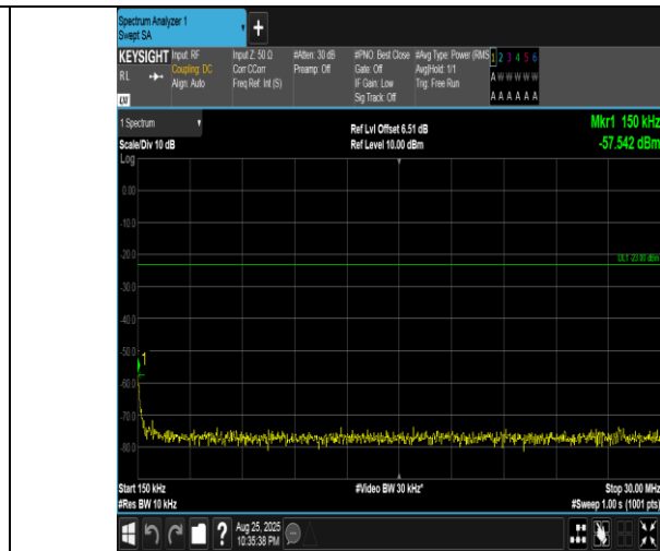
Band5-5MHz-16QAM-20525-1RB#24-0.15~30-PASS
