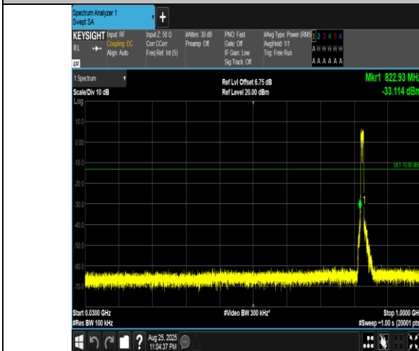
Band5-10MHz-QPSK-20450-50RB#0-30~1000-PASS
