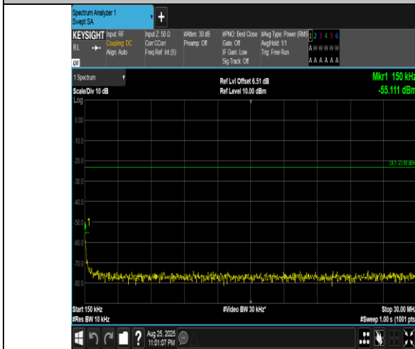
Band5-10MHz-16QAM-20450-1RB#0-0.15~30-PASS
