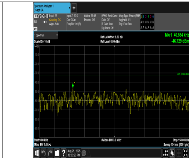
Band5-5MHz-16QAM-20525-1RB#0-0.009~0.15-PASS
