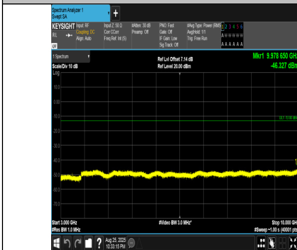
Band5-5MHz-QPSK-20525-1RB#0-3000~10000-PASS
