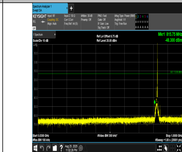
Band5-10MHz-QPSK-20450-1RB#49-30~1000-PASS
