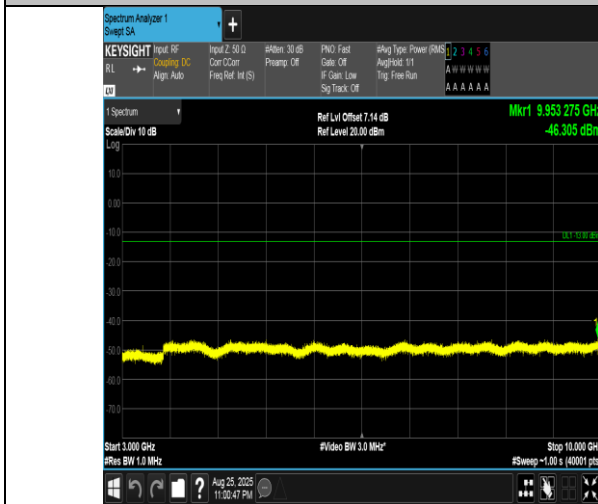
Band5-10MHz-QPSK-20450-1RB#0-3000~10000-PASS
