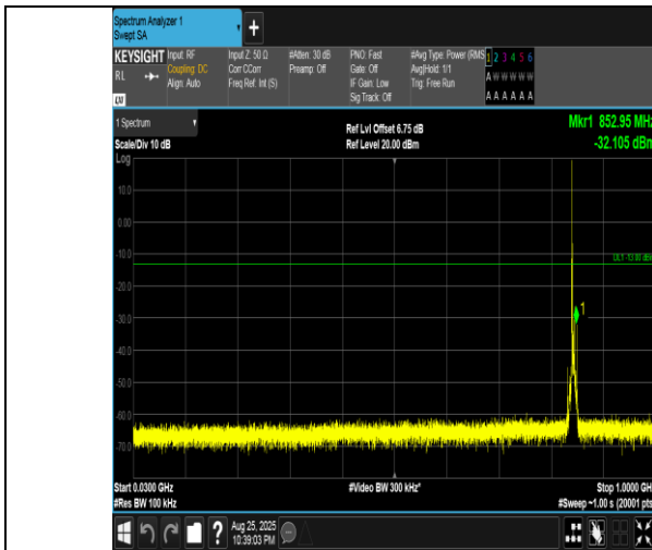
Band5-5MHz-QPSK-20625-1RB#0-30~1000-PASS
