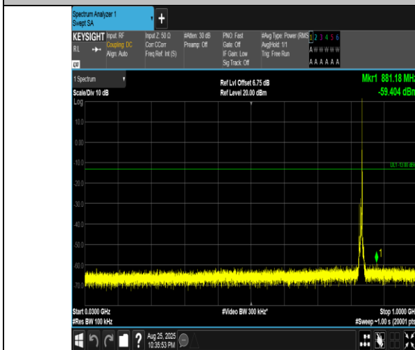
Band5-5MHz-16QAM-20525-1RB#24-30~1000-PASS
