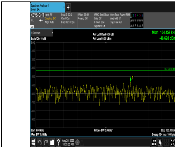
Band5-5MHz-16QAM-20525-1RB#24-0.009~0.15-PASS
