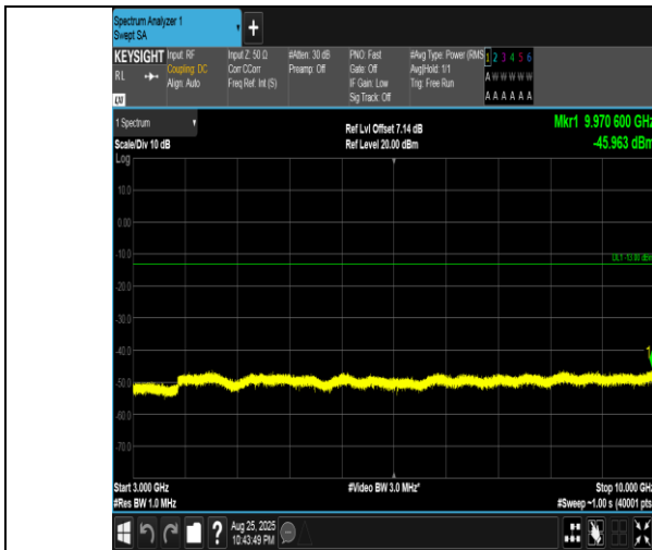
Band5-5MHz-QPSK-20625-25RB#0-3000~10000-PASS
