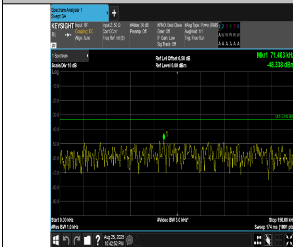
Band5-5MHz-QPSK-20625-25RB#0-0.009~0.15-PASS
