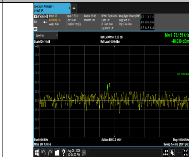
Band5-5MHz-QPSK-20525-1RB#24-0.009~0.15-PASS
