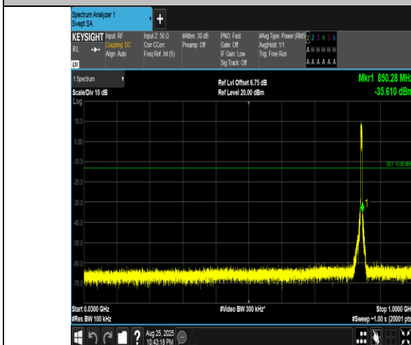
Band5-5MHz-QPSK-20625-25RB#0-30~1000-PASS
