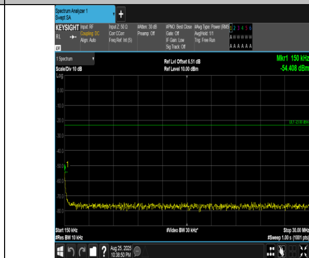
Band5-5MHz-QPSK-20625-1RB#0-0.15~30-PASS
