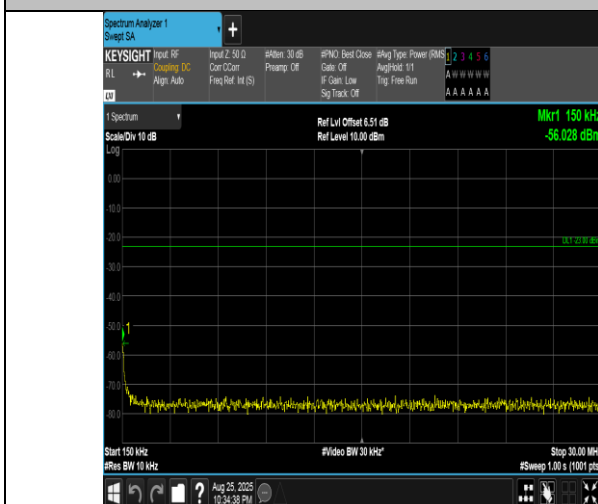
Band5-5MHz-QPSK-20525-1RB#24-0.15~30-PASS
