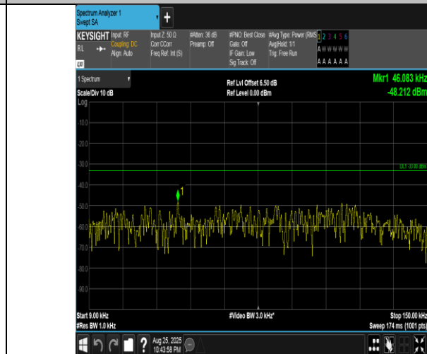
Band5-5MHz-16QAM-20625-25RB#0-0.009~0.15-PASS
