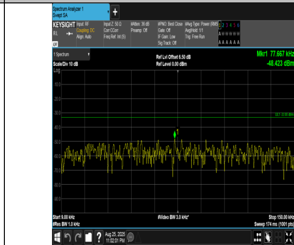
Band5-10MHz-QPSK-20450-1RB#49-0.009~0.15-PASS
