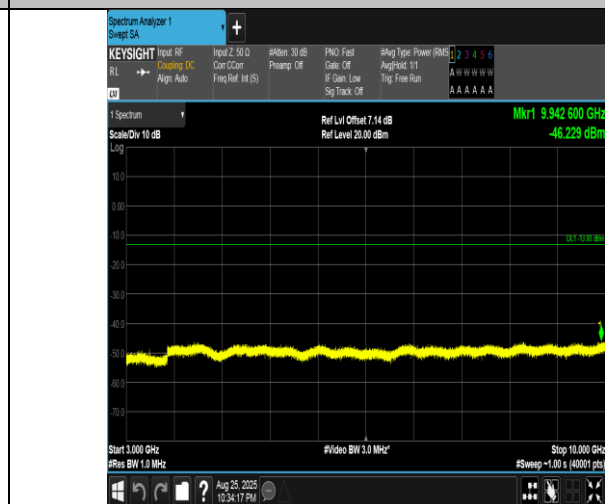
Band5-5MHz-16QAM-20525-1RB#0-3000~10000-PASS
