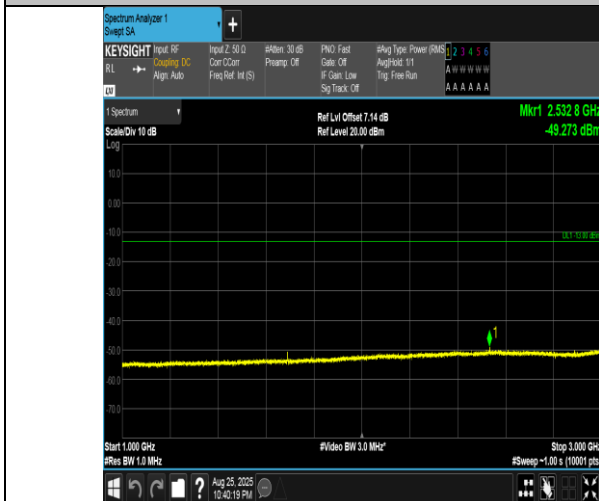
Band5-5MHz-16QAM-20625-1RB#0-1000~3000-PASS
