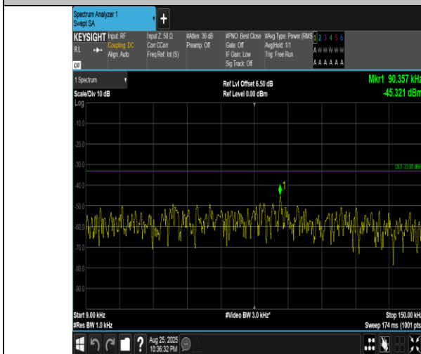
Band5-5MHz-QPSK-20525-25RB#0-0.009~0.15-PASS
