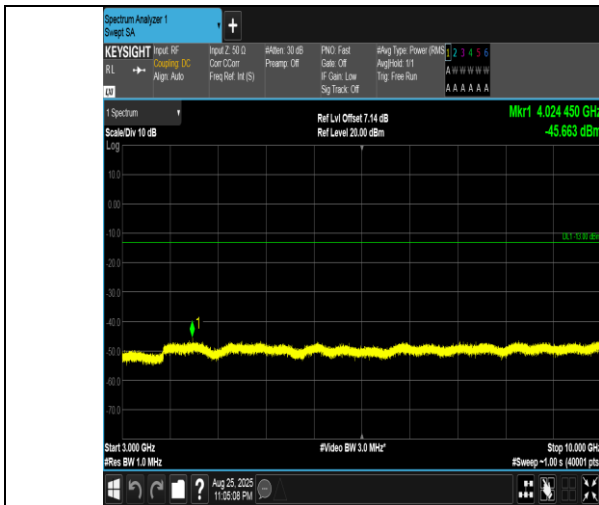
Band5-10MHz-QPSK-20450-50RB#0-3000~10000-PASS
