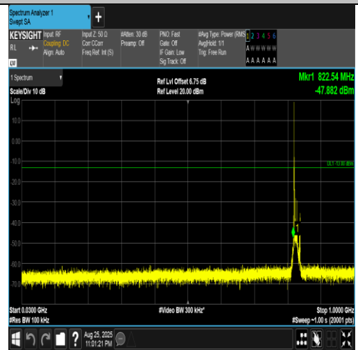
Band5-10MHz-16QAM-20450-1RB#0-30~1000-PASS
