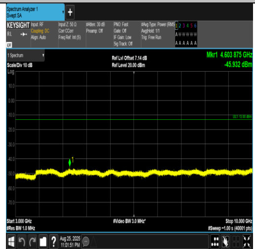
Band5-10MHz-16QAM-20450-1RB#0-3000~10000-PASS
