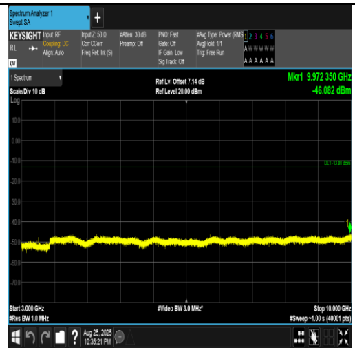
Band5-5MHz-QPSK-20525-1RB#24-3000~10000-PASS
