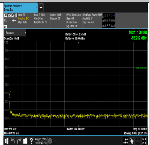
Band5-5MHz-QPSK-20525-25RB#0-0.15~30-PASS
