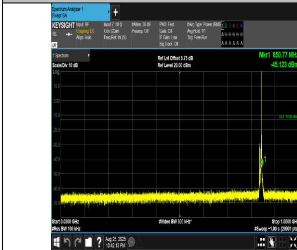
Band5-5MHz-16QAM-20625-1RB#24-30~1000-PASS
