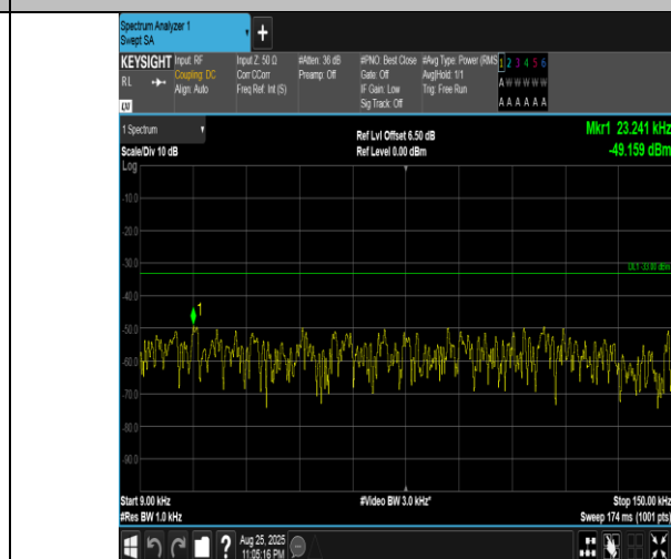
Band5-10MHz-16QAM-20450-50RB#0-0.009~0.15-PASS
