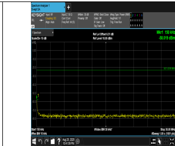
Band5-5MHz-16QAM-20625-1RB#24-0.15~30-PASS
