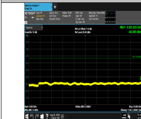
Band5-10MHz-16QAM-20450-1RB#49-3000~10000-PASS
