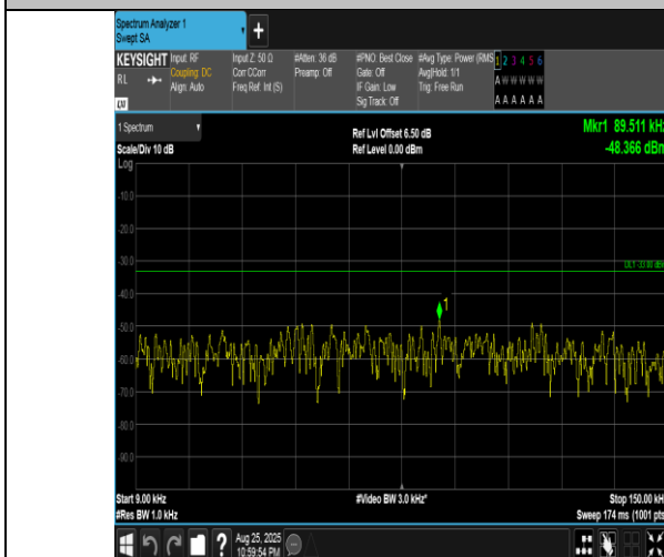
Band5-10MHz-QPSK-20450-1RB#0-0.009~0.15-PASS
