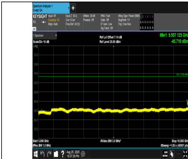
Band5-5MHz-QPSK-20525-25RB#0-3000~10000-PASS
