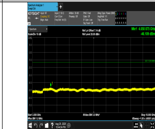
Band5-5MHz-16QAM-20625-25RB#0-3000~10000-PASS
