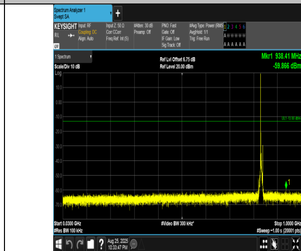
Band5-5MHz-16QAM-20525-1RB#0-30~1000-PASS
