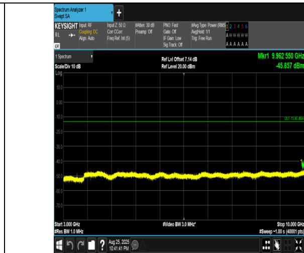
Band5-5MHz-QPSK-20625-1RB#24-3000~10000-PASS
