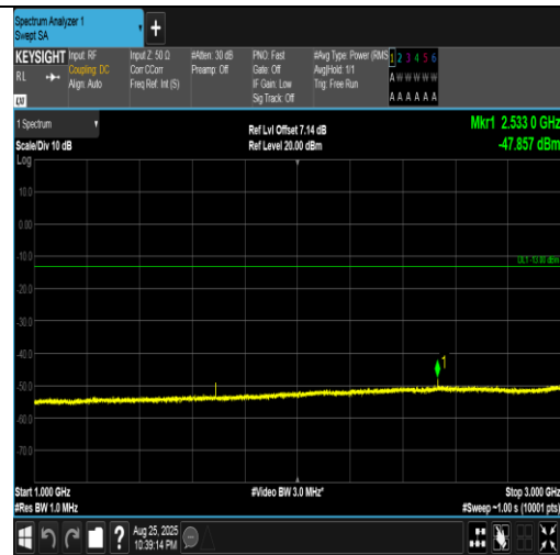
Band5-5MHz-QPSK-20625-1RB#0-1000~3000-PASS
