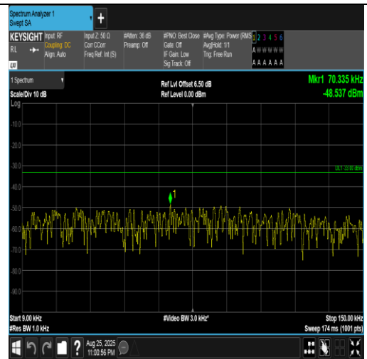
Band5-10MHz-16QAM-20450-1RB#0-0.009~0.15-PASS
