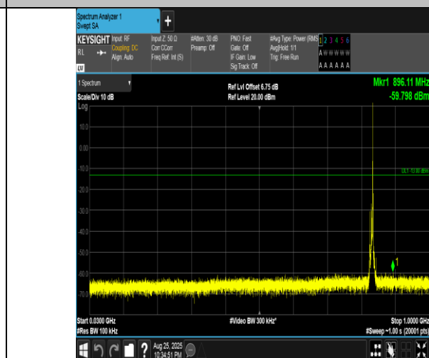
Band5-5MHz-QPSK-20525-1RB#24-30~1000-PASS
