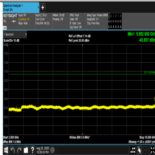
Band5-5MHz-QPSK-20625-1RB#0-3000~10000-PASS
