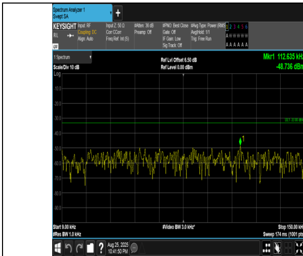
Band5-5MHz-16QAM-20625-1RB#24-0.009~0.15-PASS
