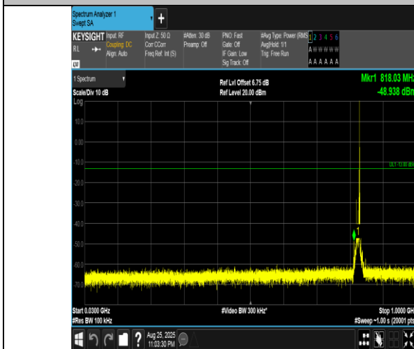
Band5-10MHz-16QAM-20450-1RB#49-30~1000-PASS
