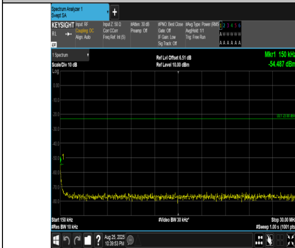
Band5-5MHz-16QAM-20625-1RB#0-0.15~30-PASS
