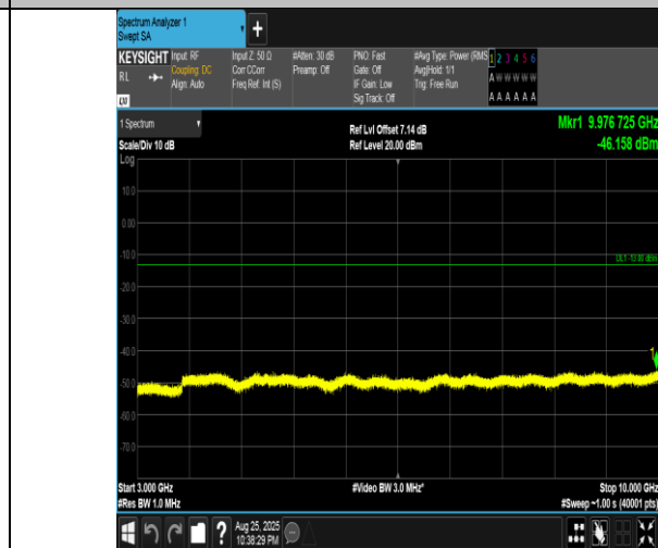
Band5-5MHz-16QAM-20525-25RB#0-3000~10000-PASS
