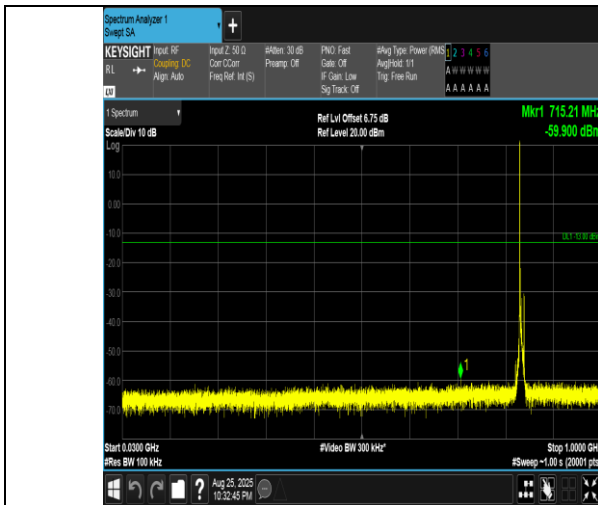
Band5-5MHz-QPSK-20525-1RB#0-30~1000-PASS
