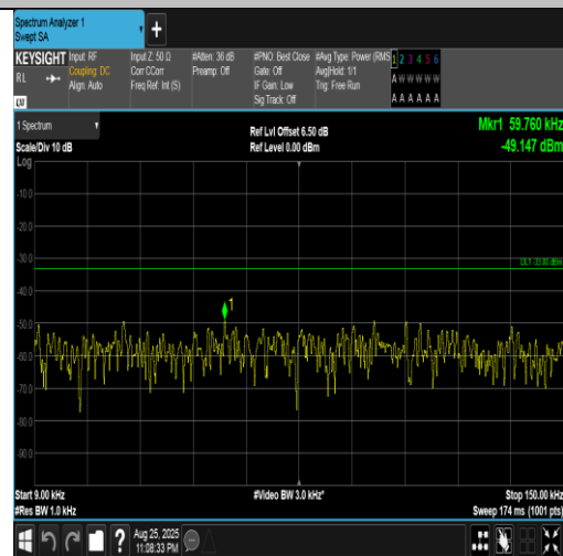
Band5-10MHz-QPSK-20525-1RB#49-0.009~0.15-PASS
