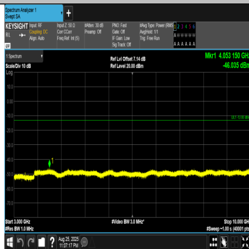
Band5-10MHz-QPSK-20525-1RB#0-3000~10000-PASS
