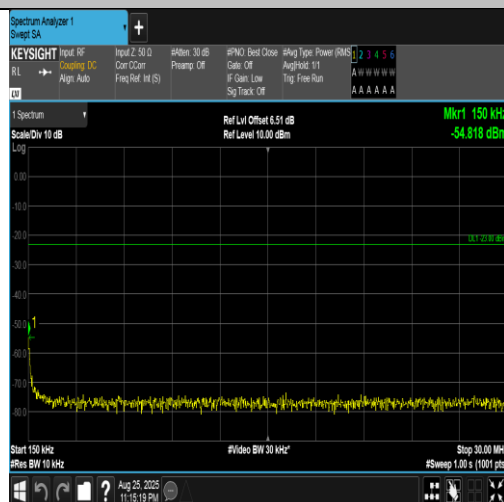
Band5-10MHz-QPSK-20600-1RB#49-0.15~30-PASS
