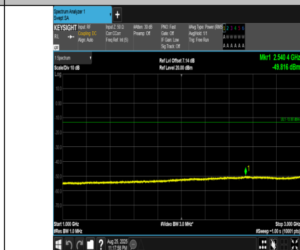
Band5-10MHz-QPSK-20600-50RB#0-1000~3000-PASS
