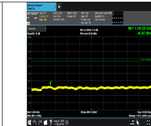
Band5-10MHz-QPSK-20525-1RB#49-3000~10000-PASS
