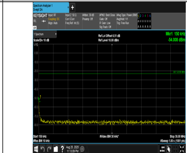
Band5-10MHz-QPSK-20600-1RB#0-0.15~30-PASS
