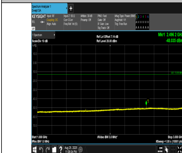
Band5-10MHz-16QAM-20525-1RB#0-1000~3000-PASS
