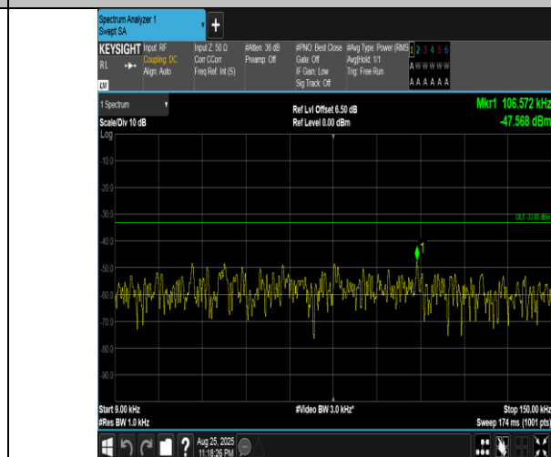
Band5-10MHz-16QAM-20600-50RB#0-0.009~0.15-PASS
