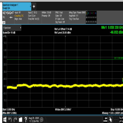
Band5-10MHz-QPSK-20600-1RB#0-3000~10000-PASS
