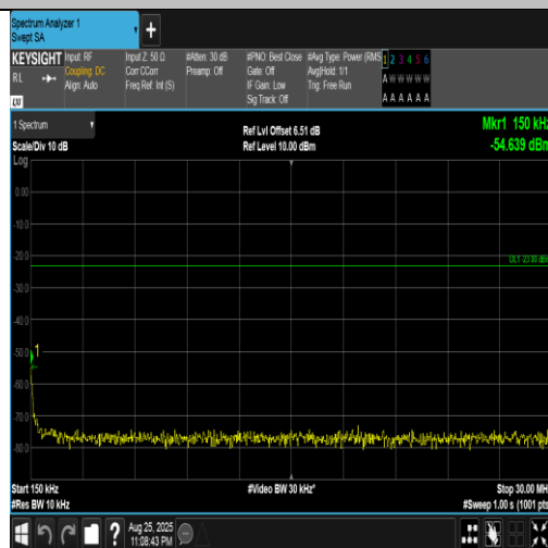
Band5-10MHz-QPSK-20525-1RB#49-0.15~30-PASS
