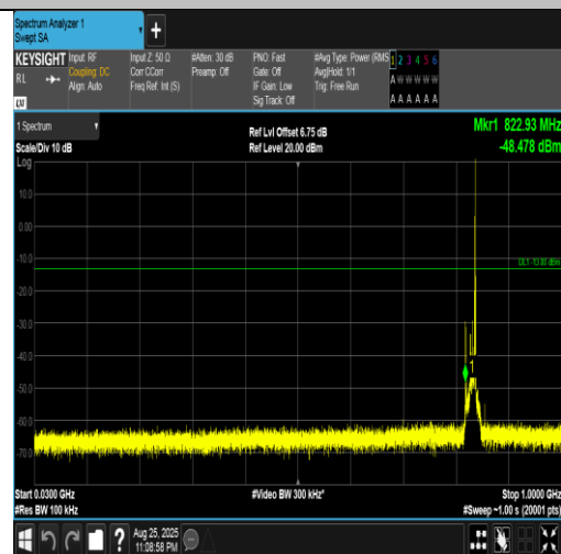
Band5-10MHz-QPSK-20525-1RB#49-30~1000-PASS
