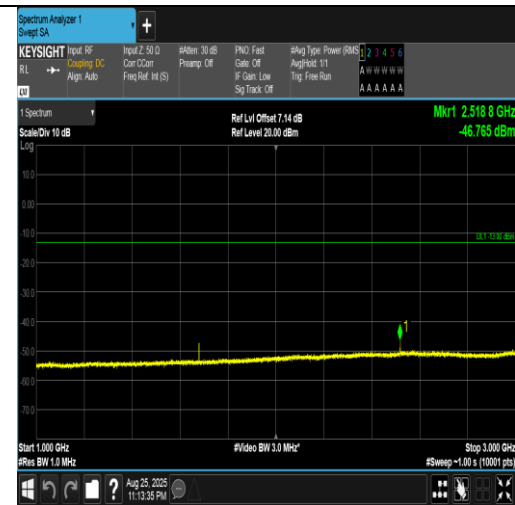
Band5-10MHz-QPSK-20600-1RB#0-1000~3000-PASS
