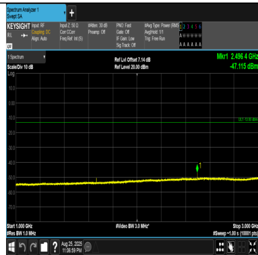
Band5-10MHz-QPSK-20525-1RB#0-1000~3000-PASS
