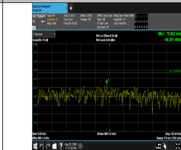
Band5-10MHz-16QAM-20525-50RB#0-0.009~0.15-PASS
