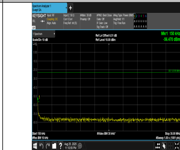
Band5-10MHz-QPSK-20525-50RB#0-0.15~30-PASS
