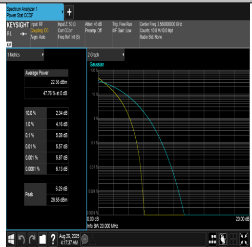
Band7-20MHz-QPSK-21350-100RB#0-PASS
