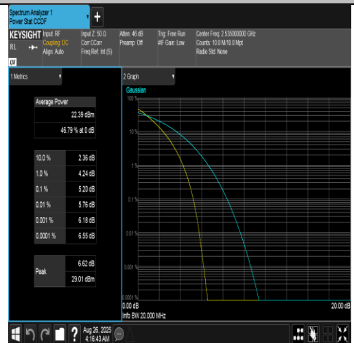
Band7-20MHz-QPSK-21100-100RB#0-PASS
