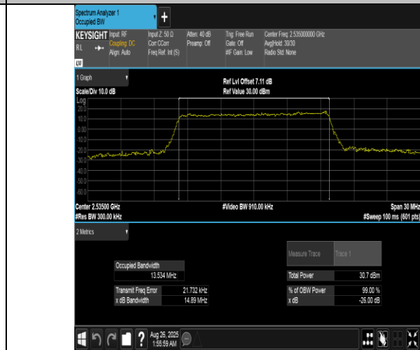
Band7-15MHz-16QAM-21100-75RB#0-PASS
