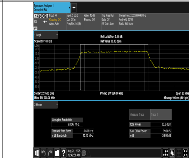
Band7-10MHz-16QAM-21100-50RB#0-PASS
