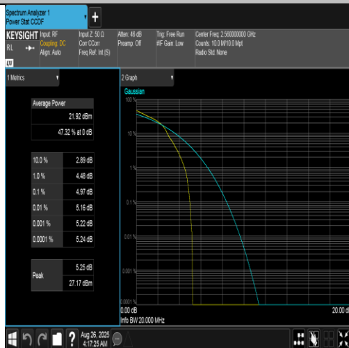
Band7-20MHz-16QAM-21350-1RB#0-PASS
