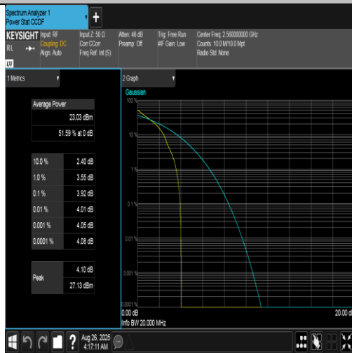
Band7-20MHz-QPSK-21350-1RB#0-PASS
