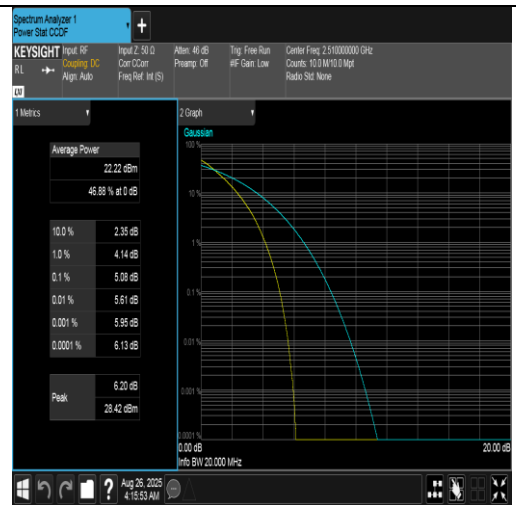
Band7-20MHz-QPSK-20850-100RB#0-PASS
