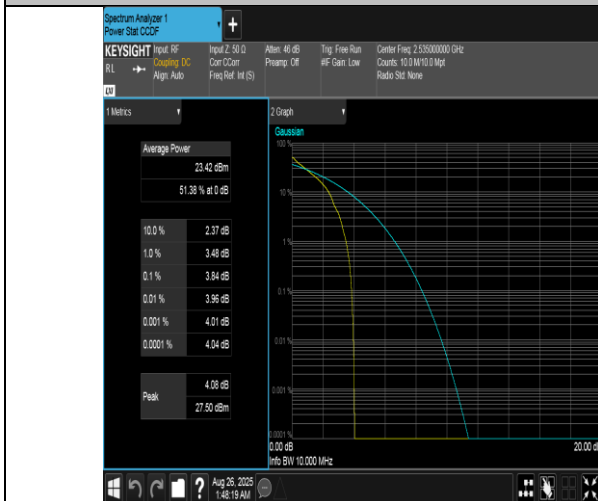
Band7-10MHz-QPSK-21100-1RB#0-PASS
