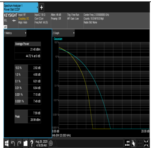
Band7-20MHz-16QAM-21100-100RB#0-PASS
