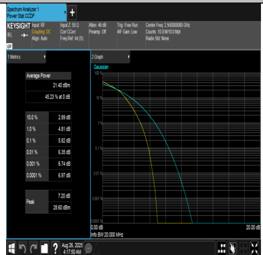
Band7-20MHz-16QAM-21350-100RB#0-PASS
