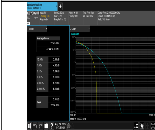
Band7-10MHz-16QAM-20800-1RB#0-PASS
