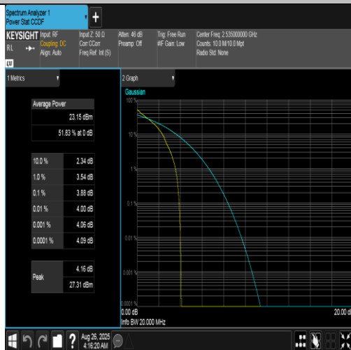
Band7-20MHz-QPSK-21100-1RB#0-PASS
