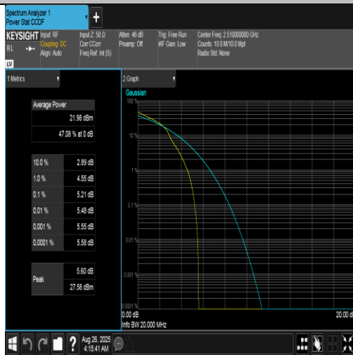
Band7-20MHz-16QAM-20850-1RB#0-PASS
