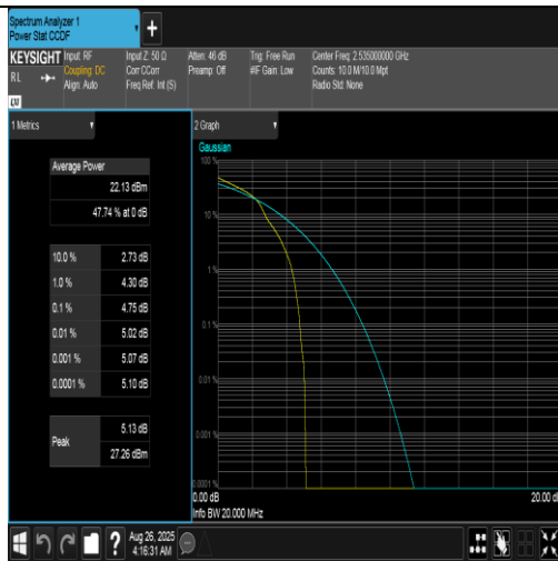
Band7-20MHz-16QAM-21100-1RB#0-PASS
