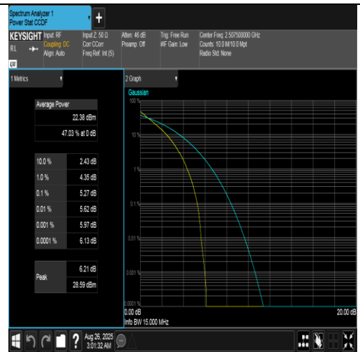
Band7-15MHz-QPSK-20825-75RB#0-PASS
