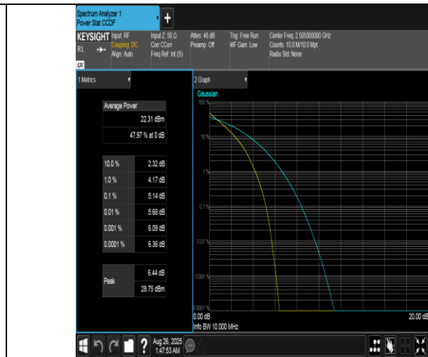
Band7-10MHz-QPSK-20800-50RB#0-PASS
