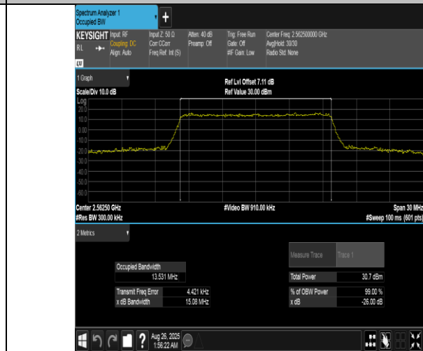
Band7-15MHz-16QAM-21375-75RB#0-PASS
