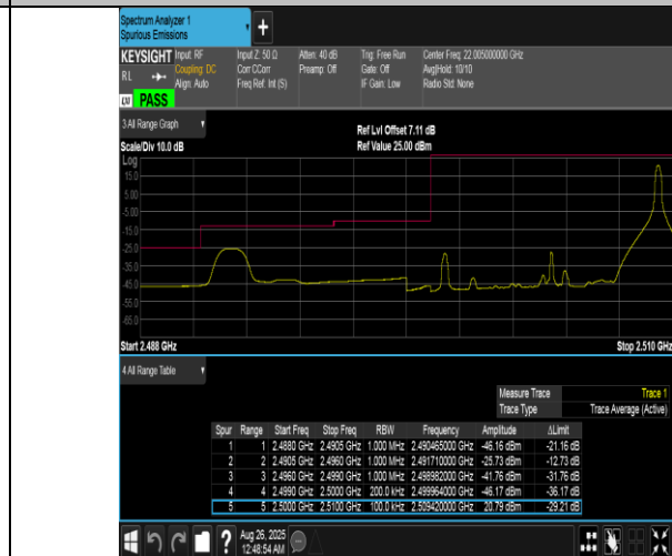
Band7-10MHz-QPSK-20800-1RB#49-PASS
