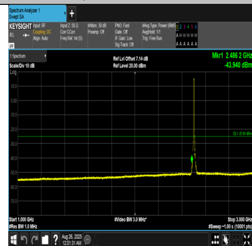
Band7-5MHz-16QAM-20775-25RB#0-1000~3000-PASS
