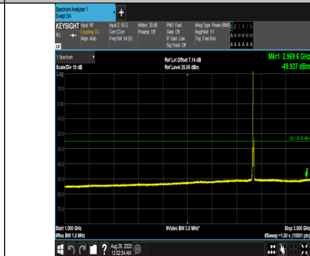
Band7-5MHz-QPSK-21100-1RB#0-1000~3000-PASS
