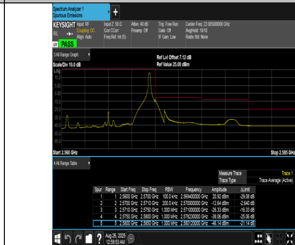
Band7-10MHz-QPSK-21400-1RB#49-PASS
