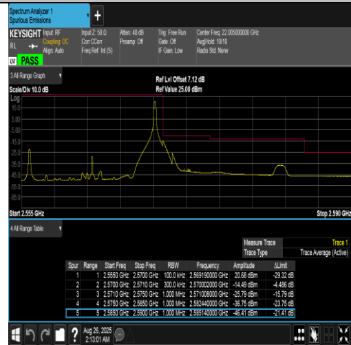
Band7-15MHz-QPSK-21375-1RB#74-PASS
