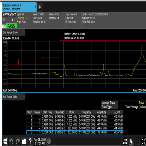
Band7-20MHz-16QAM-20850-1RB#99-PASS
