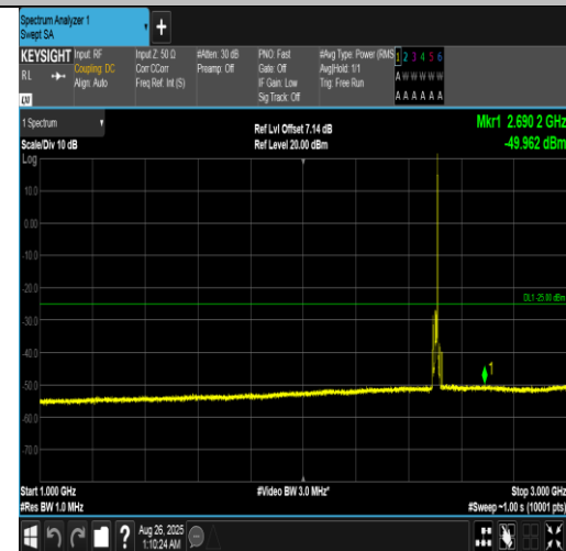
Band7-10MHz-16QAM-20800-1RB#49-1000~3000-PASS
