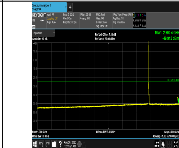
Band7-5MHz-16QAM-21425-1RB#24-1000~3000-PASS
