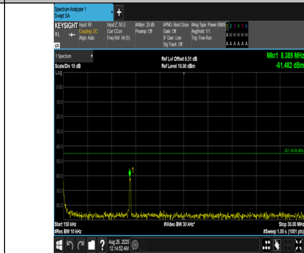
Band7-5MHz-16QAM-21425-1RB#24-0.15~30-PASS
