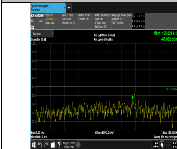
Band7-10MHz-QPSK-20800-1RB#49-0.009~0.15-PASS
