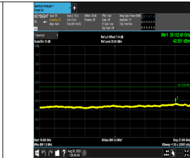
Band7-10MHz-QPSK-20800-1RB#0-18000~27000-PASS
