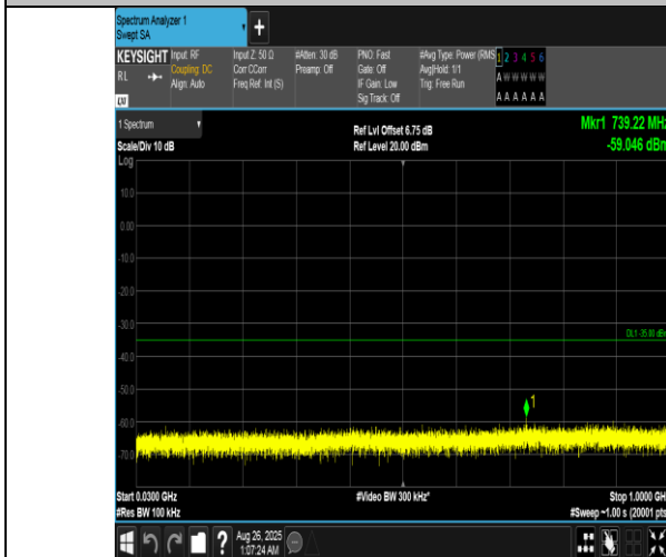
Band7-10MHz-16QAM-20800-1RB#0-30~1000-PASS
