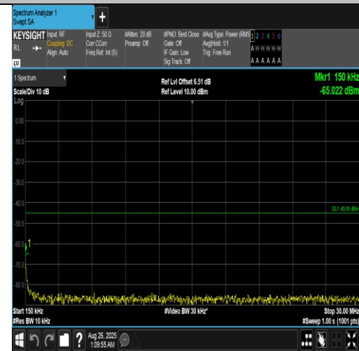
Band7-10MHz-16QAM-20800-1RB#49-0.15~30-PASS
