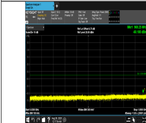
Band7-5MHz-16QAM-21425-25RB#0-30~1000-PASS
