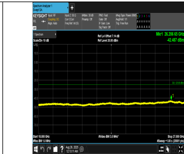
Band7-5MHz-16QAM-21425-1RB#0-18000~27000-PASS
