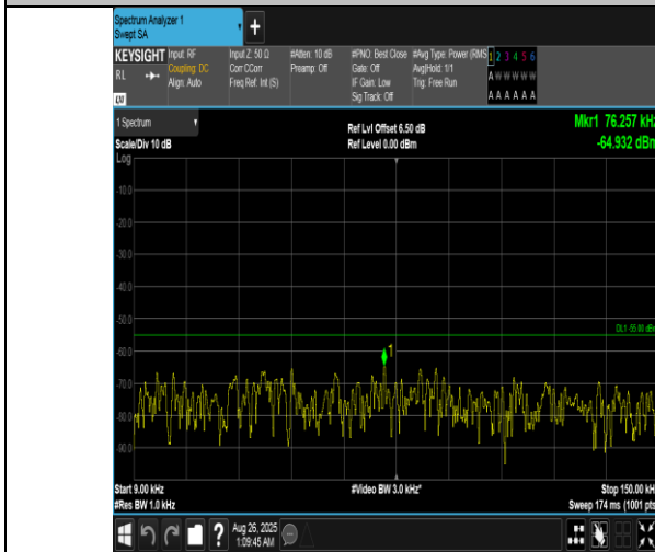
Band7-10MHz-16QAM-20800-1RB#49-0.009~0.15-PASS
