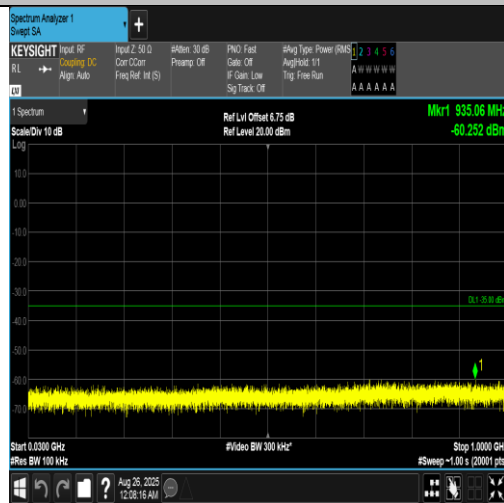
Band7-5MHz-QPSK-21100-25RB#0-30~1000-PASS
