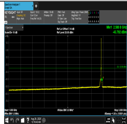
Band7-5MHz-QPSK-21425-25RB#0-1000~3000-PASS
