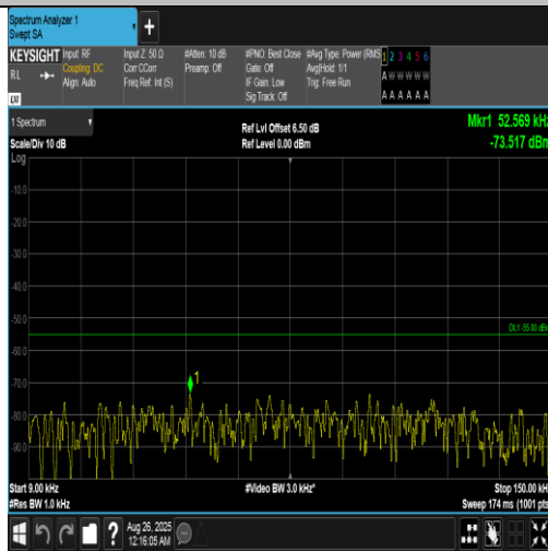
Band7-5MHz-QPSK-21425-25RB#0-0.009~0.15-PASS
