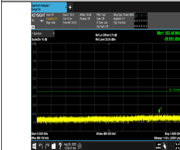
Band7-5MHz-16QAM-21100-25RB#0-30~1000-PASS
