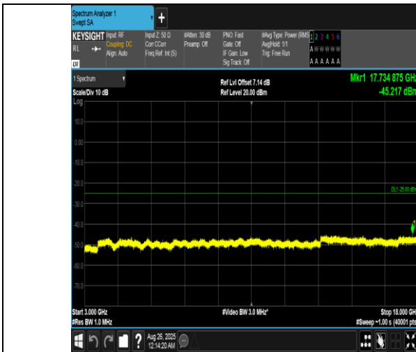
Band7-5MHz-QPSK-21425-1RB#24-3000~18000-PASS
