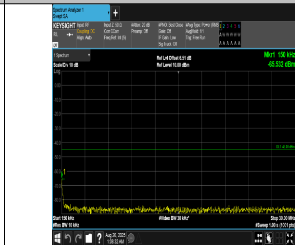
Band7-10MHz-QPSK-20800-1RB#49-0.15~30-PASS
