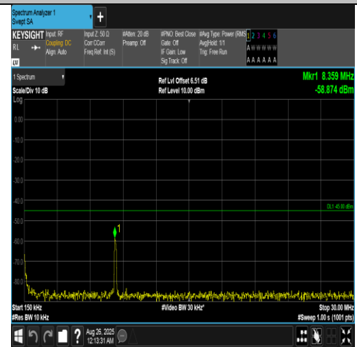
Band7-5MHz-QPSK-21425-1RB#24-0.15~30-PASS
