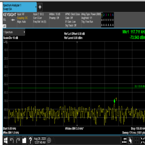
Band7-5MHz-QPSK-21100-25RB#0-0.009~0.15-PASS
