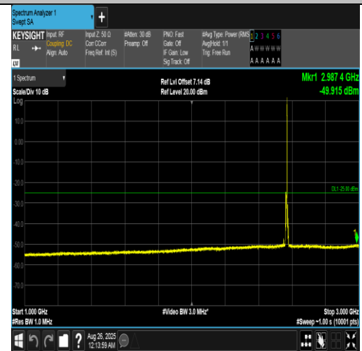
Band7-5MHz-QPSK-21425-1RB#24-1000~3000-PASS
