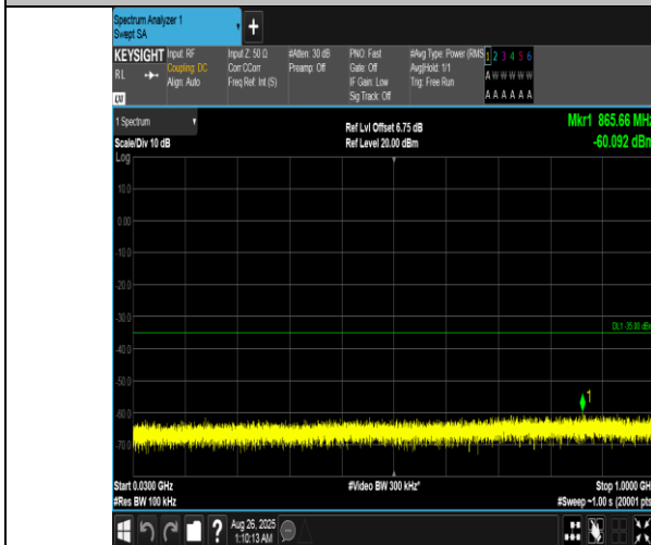
Band7-10MHz-16QAM-20800-1RB#49-30~1000-PASS
