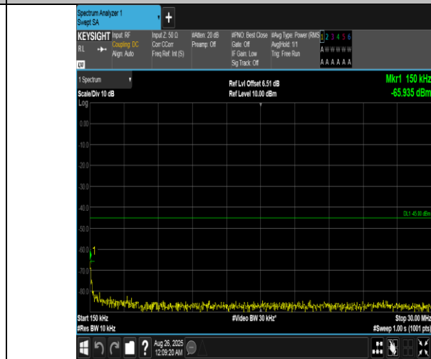
Band7-5MHz-16QAM-21100-25RB#0-0.15~30-PASS
