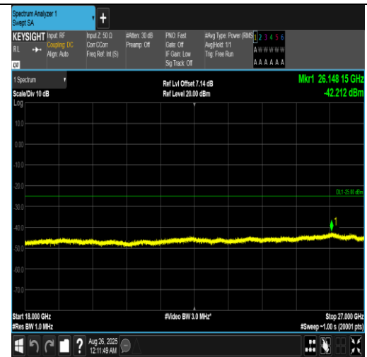
Band7-5MHz-QPSK-21425-1RB#0-18000~27000-PASS
