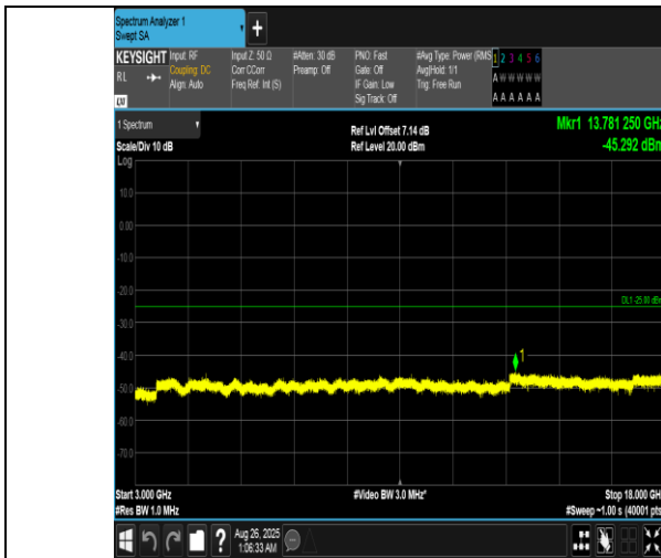
Band7-10MHz-QPSK-20800-1RB#0-3000~18000-PASS
