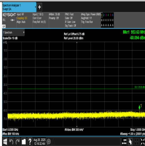
Band7-5MHz-QPSK-21425-25RB#0-30~1000-PASS
