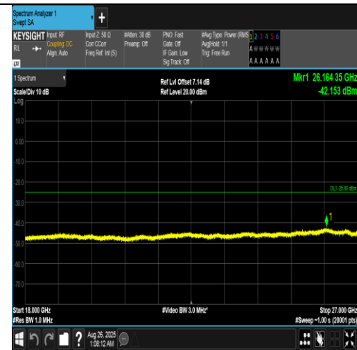
Band7-10MHz-16QAM-20800-1RB#0-18000~27000-PASS
