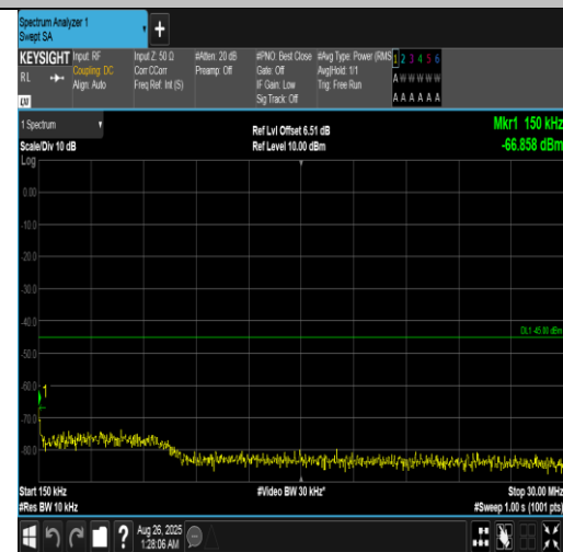
Band7-10MHz-QPSK-21400-50RB#0-0.15~30-PASS
