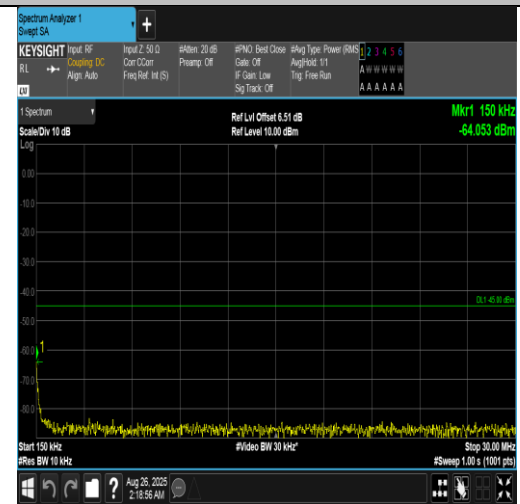
Band7-15MHz-QPSK-20825-1RB#0-0.15~30-PASS
