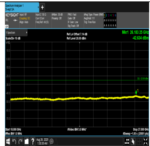
Band7-10MHz-16QAM-21400-50RB#0-18000~27000-PASS
