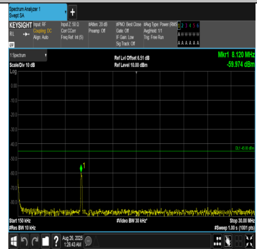
Band7-10MHz-16QAM-21400-1RB#49-0.15~30-PASS
