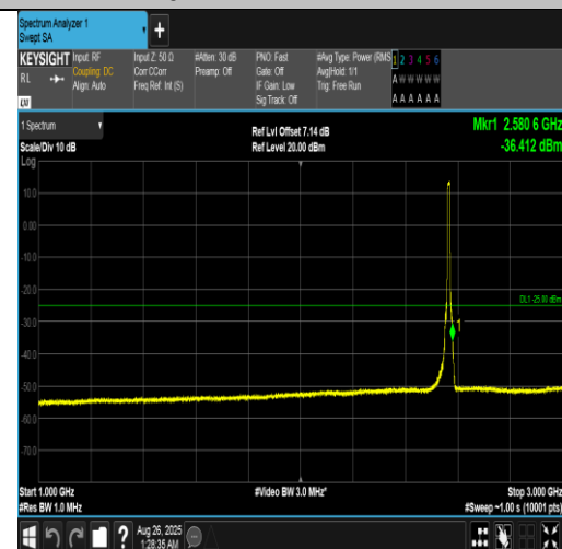
Band7-10MHz-QPSK-21400-50RB#0-1000~3000-PASS
