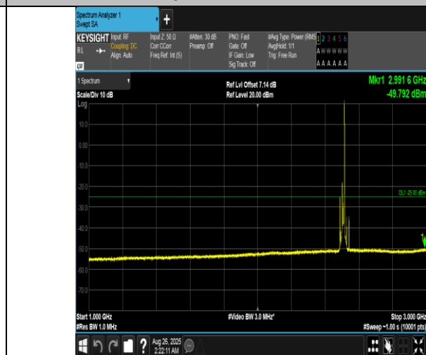
Band7-15MHz-QPSK-20825-1RB#74-1000~3000-PASS
