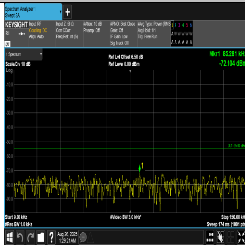
Band7-10MHz-16QAM-21400-50RB#0-0.009~0.15-PASS
