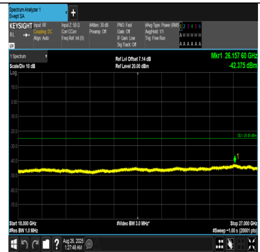
Band7-10MHz-16QAM-21400-1RB#49-18000~27000-PASS
