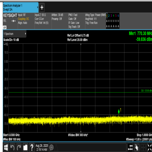
Band7-15MHz-QPSK-20825-1RB#0-30~1000-PASS
