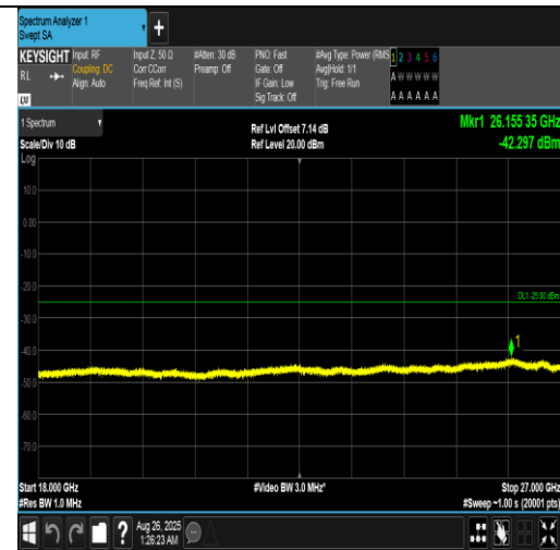
Band7-10MHz-QPSK-21400-1RB#49-18000~27000-PASS
