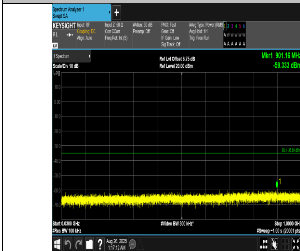
Band7-10MHz-QPSK-21100-1RB#49-30~1000-PASS
