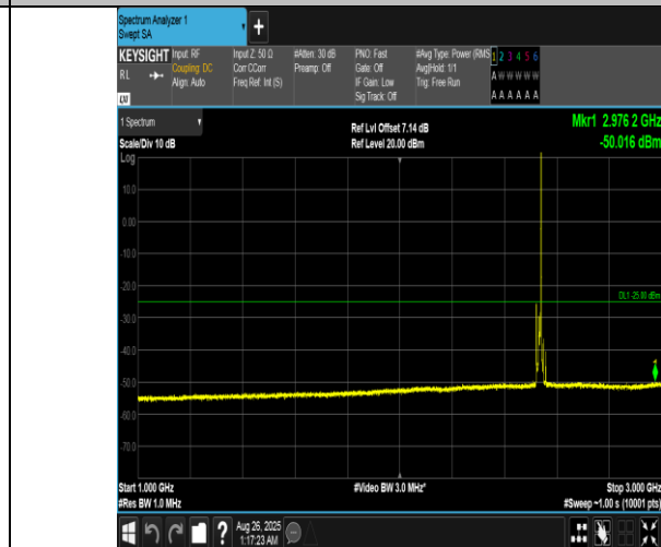
Band7-10MHz-QPSK-21100-1RB#49-1000~3000-PASS
