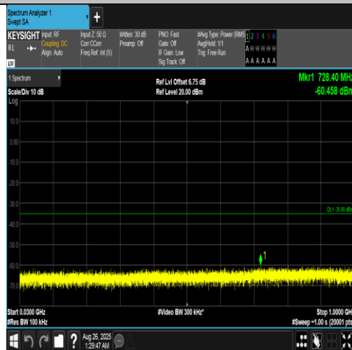
Band7-10MHz-16QAM-21400-50RB#0-30~1000-PASS
