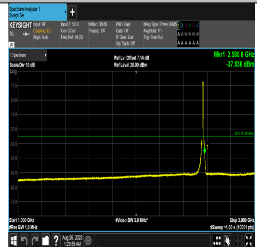
Band7-10MHz-16QAM-21400-50RB#0-1000~3000-PASS
