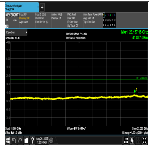
Band7-10MHz-16QAM-21400-1RB#0-18000~27000-PASS
