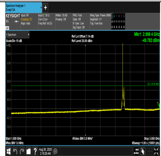
Band7-15MHz-QPSK-20825-1RB#0-1000~3000-PASS
