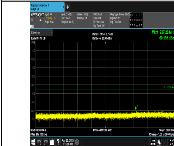
Band7-10MHz-16QAM-20800-50RB#0-30~1000-PASS
