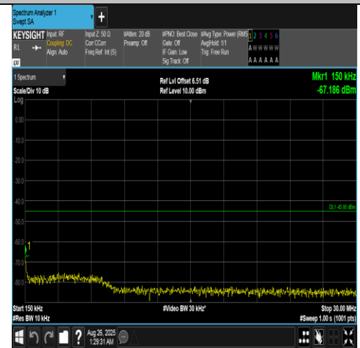
Band7-10MHz-16QAM-21400-50RB#0-0.15~30-PASS
