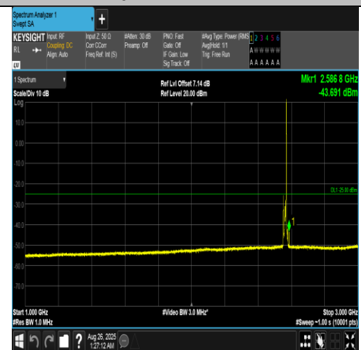
Band7-10MHz-16QAM-21400-1RB#49-1000~3000-PASS
