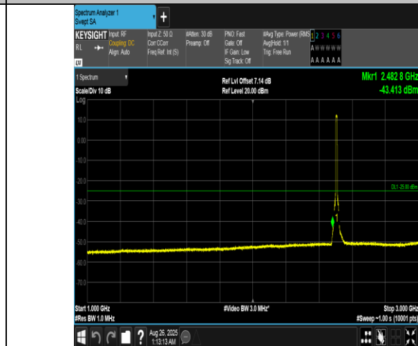
Band7-10MHz-16QAM-20800-50RB#0-1000~3000-PASS
