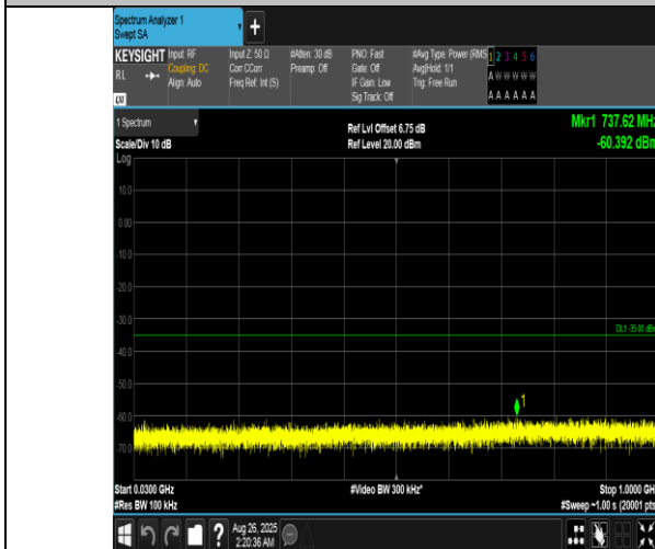
Band7-15MHz-16QAM-20825-1RB#0-30~1000-PASS
