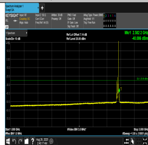
Band7-15MHz-16QAM-21375-1RB#74-1000~3000-PASS
