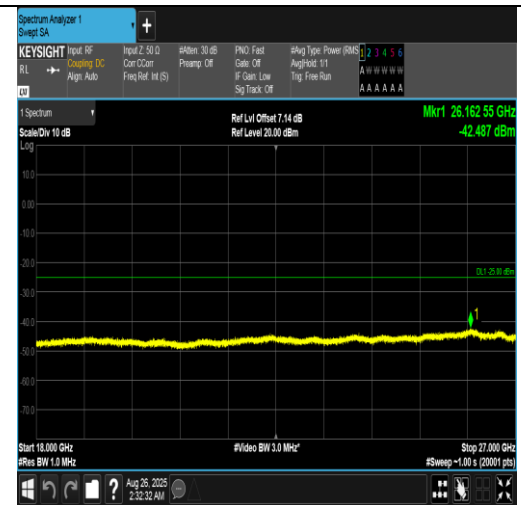
Band7-15MHz-16QAM-21100-1RB#74-18000~27000-PASS
