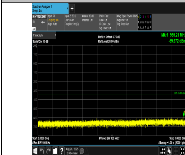
Band7-15MHz-QPSK-21375-1RB#74-30~1000-PASS
