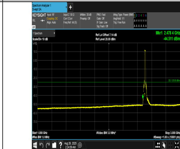
Band7-15MHz-QPSK-20825-75RB#0-1000~3000-PASS
