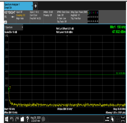
Band7-15MHz-16QAM-20825-1RB#74-0.15~30-PASS
