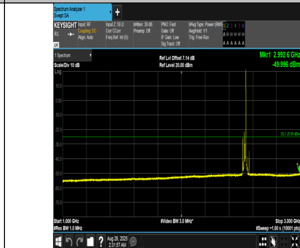
Band7-15MHz-16QAM-21100-1RB#74-1000~3000-PASS
