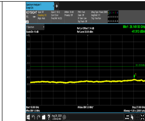
Band7-15MHz-QPSK-21375-1RB#0-18000~27000-PASS
