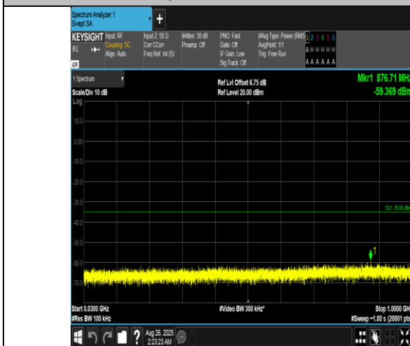
Band7-15MHz-16QAM-20825-1RB#74-30~1000-PASS
