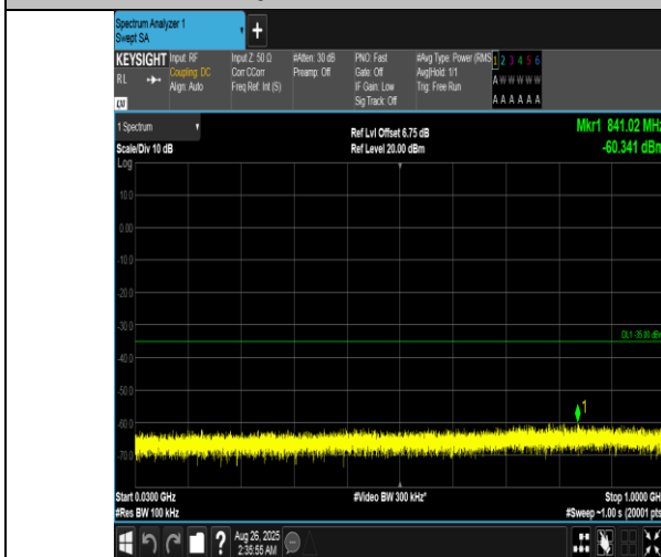
Band7-15MHz-QPSK-21375-1RB#0-30~1000-PASS
