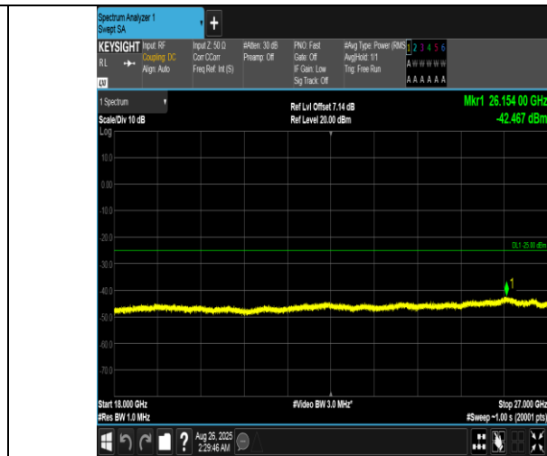
Band7-15MHz-16QAM-21100-1RB#0-18000~27000-PASS
