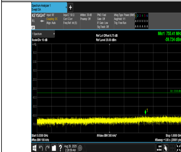
Band7-15MHz-16QAM-21100-1RB#0-30~1000-PASS
