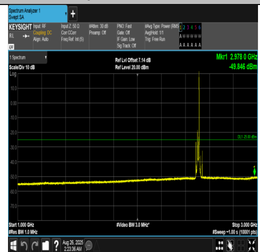
Band7-15MHz-16QAM-20825-1RB#74-1000~3000-PASS
