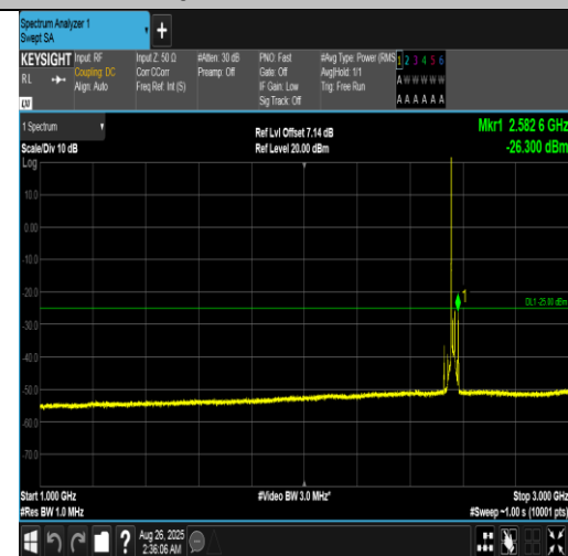
Band7-15MHz-QPSK-21375-1RB#0-1000~3000-PASS
