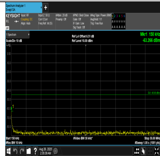
Band7-15MHz-QPSK-21375-1RB#0-0.15~30-PASS
