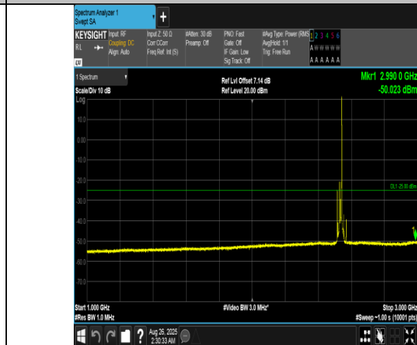
Band7-15MHz-QPSK-21100-1RB#74-1000~3000-PASS
