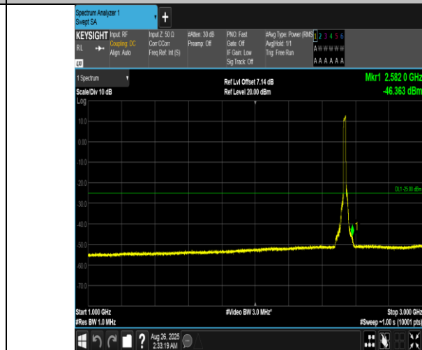
Band7-15MHz-QPSK-21100-75RB#0-1000~3000-PASS
