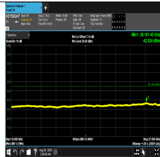
Band7-15MHz-16QAM-21375-1RB#0-18000~27000-PASS
