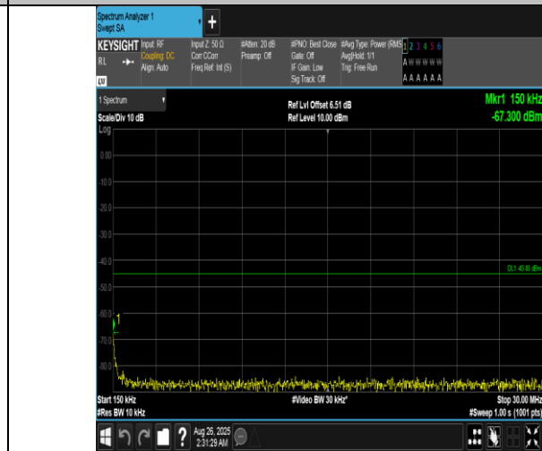
Band7-15MHz-16QAM-21100-1RB#74-0.15~30-PASS
