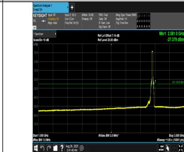
Band7-15MHz-QPSK-21375-75RB#0-1000~3000-PASS
