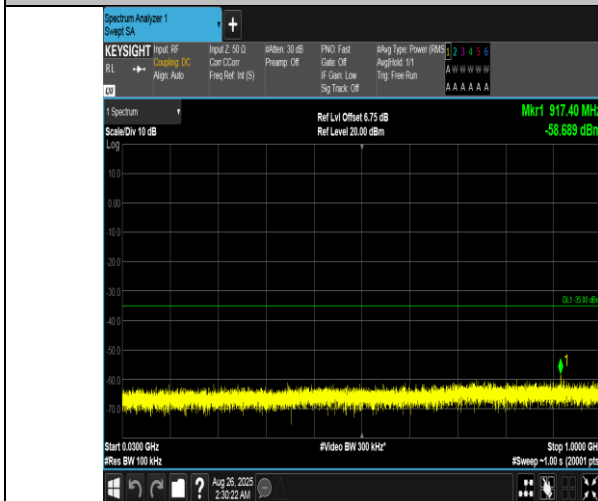
Band7-15MHz-QPSK-21100-1RB#74-30~1000-PASS
