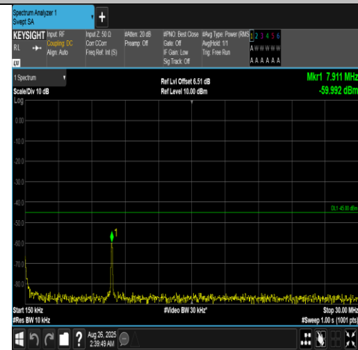
Band7-15MHz-16QAM-21375-1RB#74-0.15~30-PASS
