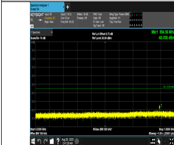
Band7-15MHz-QPSK-21375-75RB#0-30~1000-PASS
