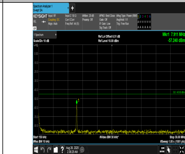
Band7-15MHz-QPSK-21375-1RB#74-0.15~30-PASS
