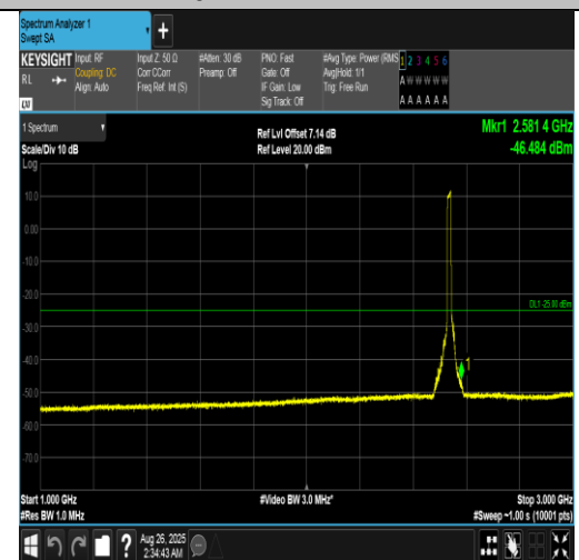
Band7-15MHz-16QAM-21100-75RB#0-1000~3000-PASS
