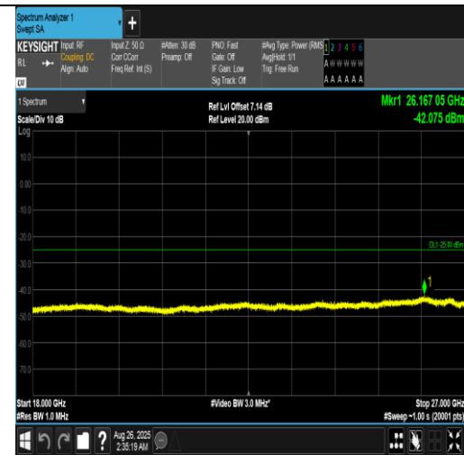
Band7-15MHz-16QAM-21100-75RB#0-18000~27000-PASS
