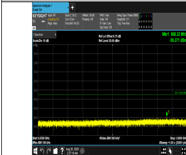
Band7-15MHz-16QAM-21375-1RB#0-30~1000-PASS
