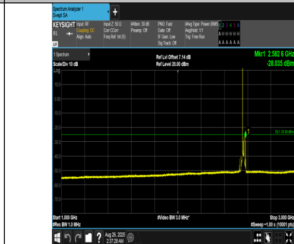
Band7-15MHz-16QAM-21375-1RB#0-1000~3000-PASS
