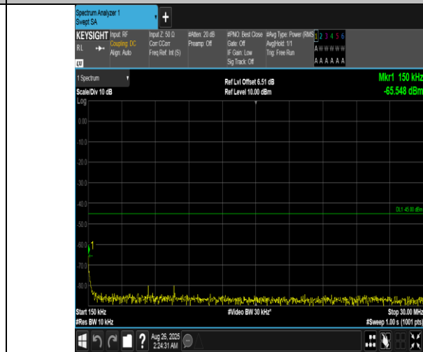
Band7-15MHz-QPSK-20825-75RB#0-0.15~30-PASS
