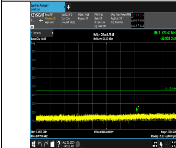
Band7-20MHz-16QAM-21100-1RB#99-30~1000-PASS
