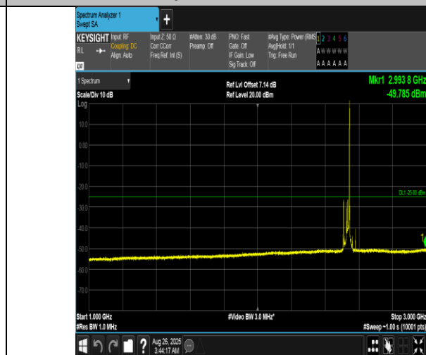
Band7-20MHz-QPSK-21100-1RB#99-1000~3000-PASS
