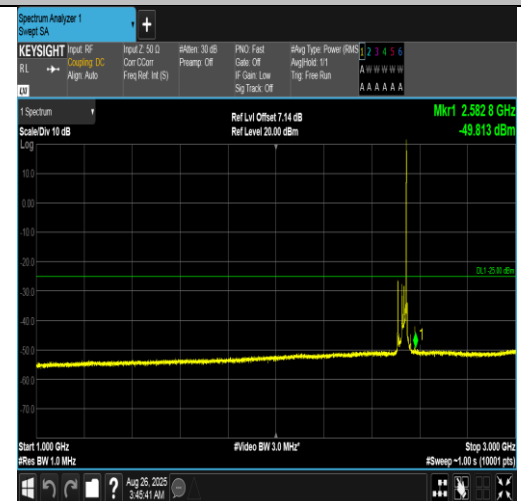
Band7-20MHz-16QAM-21100-1RB#99-1000~3000-PASS
