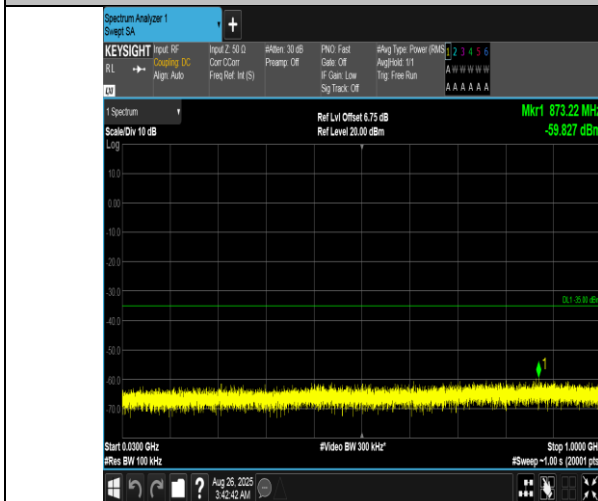
Band7-20MHz-16QAM-21100-1RB#0-30~1000-PASS
