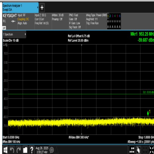
Band7-20MHz-QPSK-21350-100RB#0-30~1000-PASS
