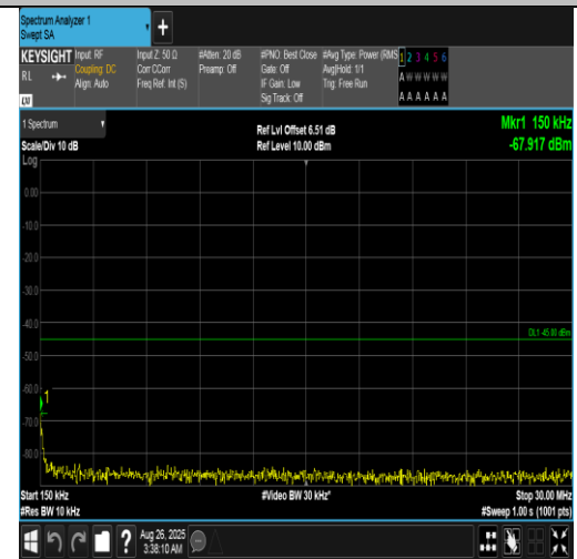
Band7-20MHz-QPSK-20850-100RB#0-0.15~30-PASS
