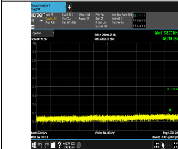
Band7-20MHz-QPSK-21350-1RB#0-30~1000-PASS
