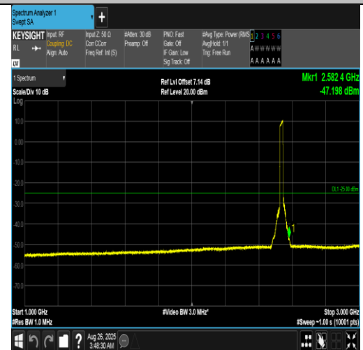
Band7-20MHz-16QAM-21100-100RB#0-1000~3000-PASS
