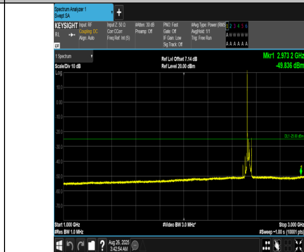
Band7-20MHz-16QAM-21100-1RB#0-1000~3000-PASS
