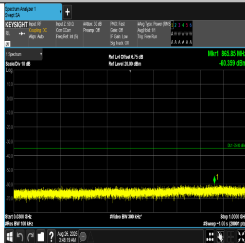
Band7-20MHz-16QAM-21100-100RB#0-30~1000-PASS
