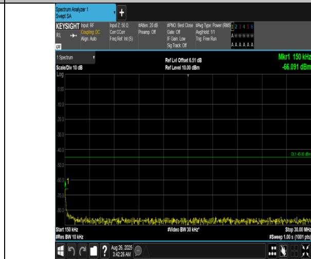
Band7-20MHz-16QAM-21100-1RB#0-0.15~30-PASS
