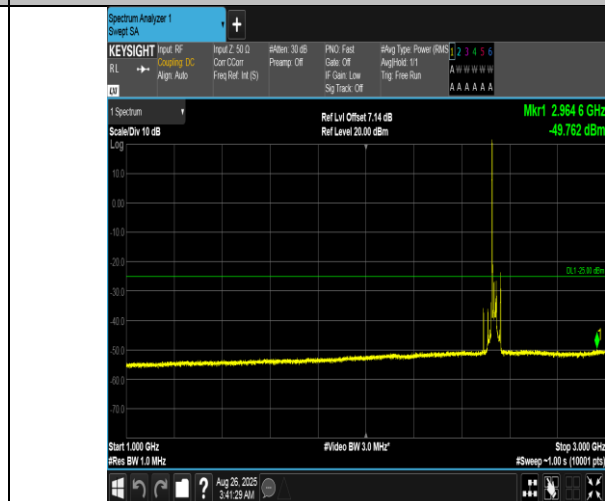
Band7-20MHz-QPSK-21100-1RB#0-1000~3000-PASS
