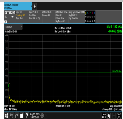
Band7-20MHz-QPSK-21100-100RB#0-0.15~30-PASS
