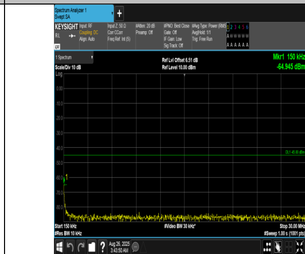
Band7-20MHz-QPSK-21100-1RB#99-0.15~30-PASS
