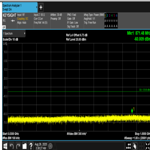
Band7-20MHz-QPSK-20850-100RB#0-30~1000-PASS
