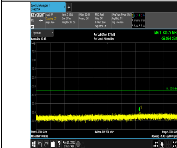
Band7-20MHz-QPSK-20850-1RB#99-30~1000-PASS
