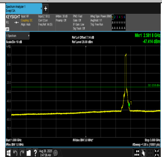
Band7-20MHz-QPSK-21100-100RB#0-1000~3000-PASS
