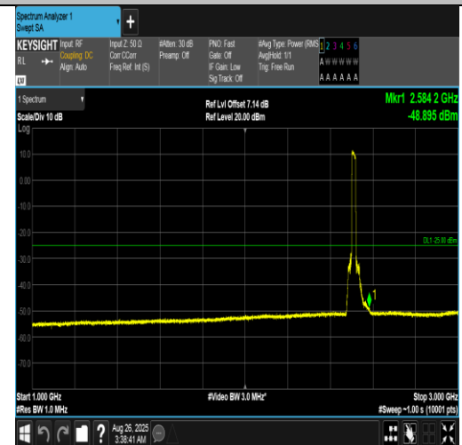
Band7-20MHz-QPSK-20850-100RB#0-1000~3000-PASS
