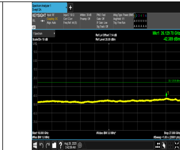
Band7-20MHz-QPSK-21100-1RB#0-18000~27000-PASS
