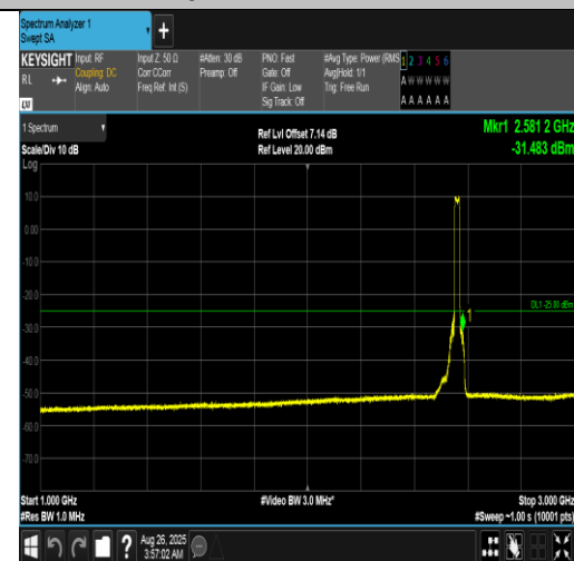
Band7-20MHz-16QAM-21350-100RB#0-1000~3000-PASS
