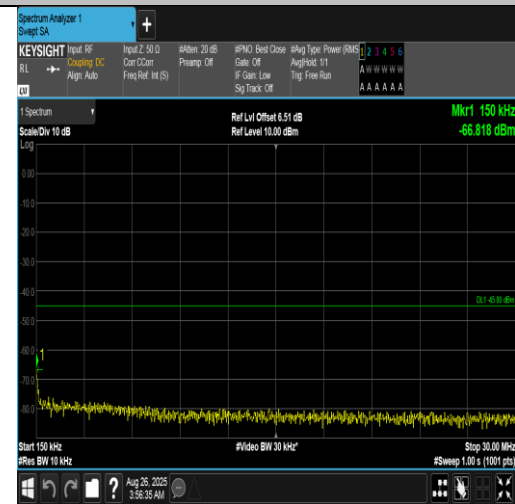
Band7-20MHz-16QAM-21350-100RB#0-0.15~30-PASS
