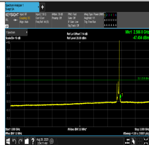
Band7-20MHz-16QAM-21350-1RB#99-1000~3000-PASS
