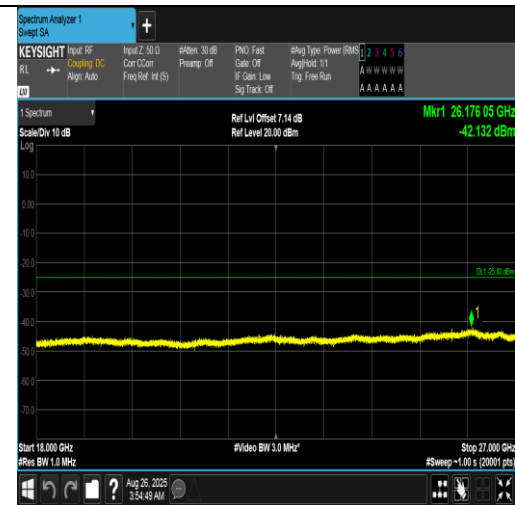
Band7-20MHz-16QAM-21350-1RB#99-18000~27000-PASS
