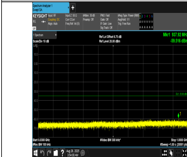
Band7-20MHz-16QAM-21350-1RB#99-30~1000-PASS
