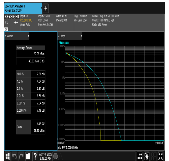
Band12-5MHz-QPSK-23035-25RB#0-PASS
