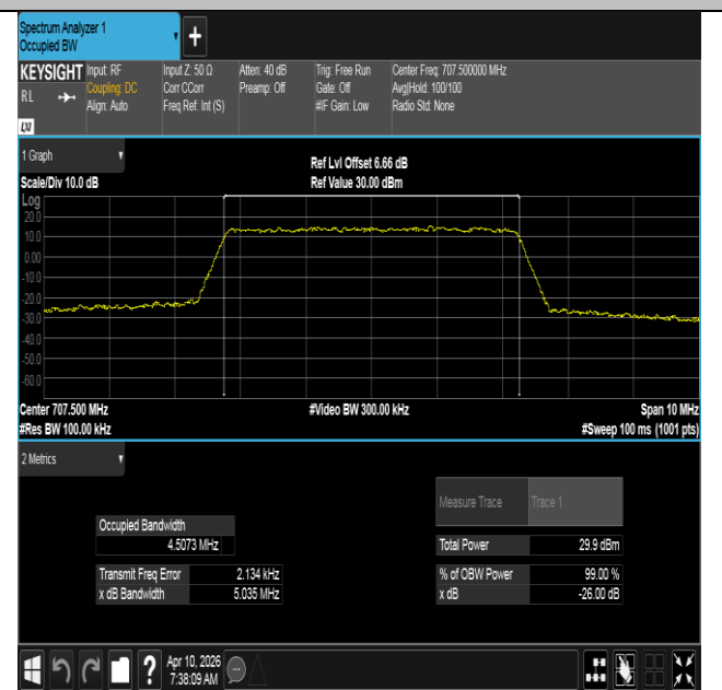
Band12-5MHz-16QAM-23095-25RB#0-PASS
