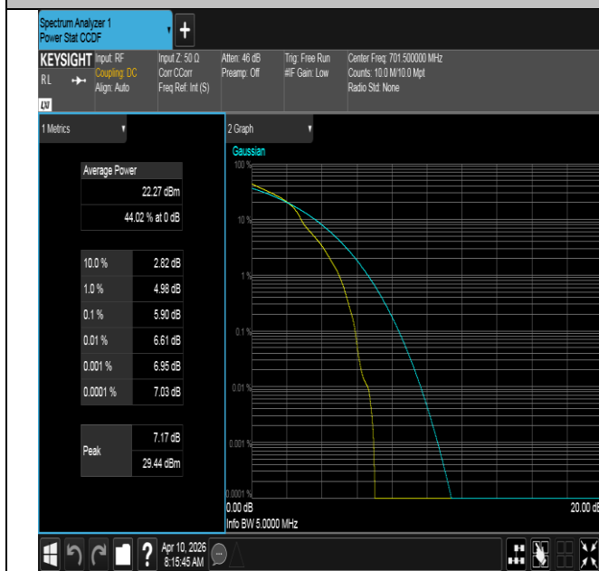
Band12-5MHz-16QAM-23035-1RB#0-PASS
