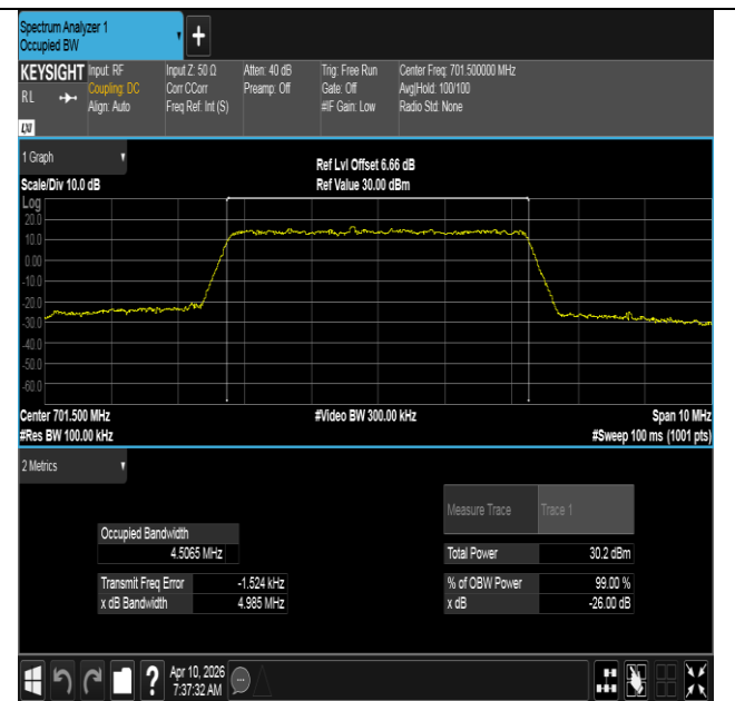
Band12-5MHz-16QAM-23035-25RB#0-PASS
