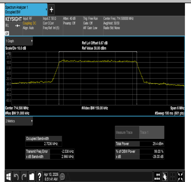
Band12-3MHz-16QAM-23165-15RB#0-PASS
