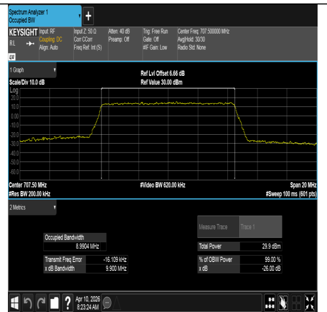
Band12-10MHz-16QAM-23095-50RB#0-PASS
