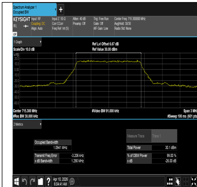
Band12-1.4MHz-QPSK-23173-6RB#0-PASS
