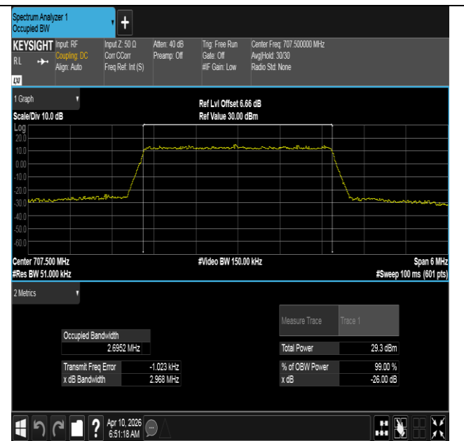
Band12-3MHz-16QAM-23095-15RB#0-PASS
