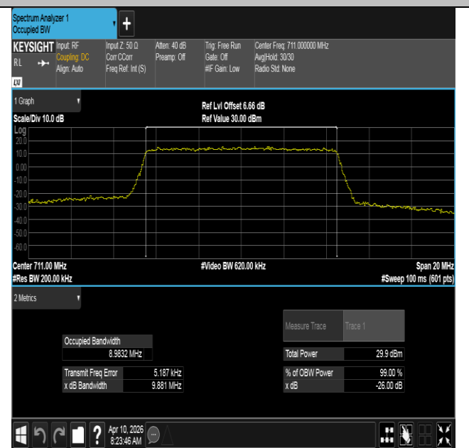
Band12-10MHz-16QAM-23130-50RB#0-PASS
