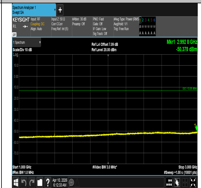
Band12-1.4MHz-QPSK-23017-6RB#0-1000~3000-PASS
