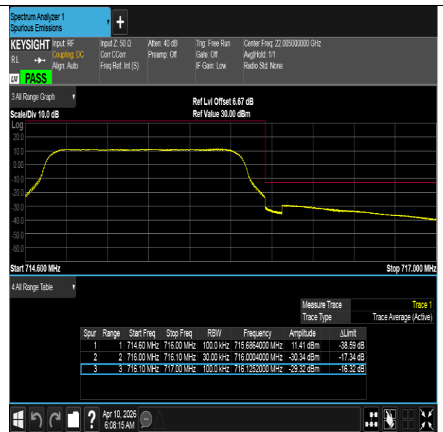
Band12-1.4MHz-16QAM-23173-6RB#0-PASS
