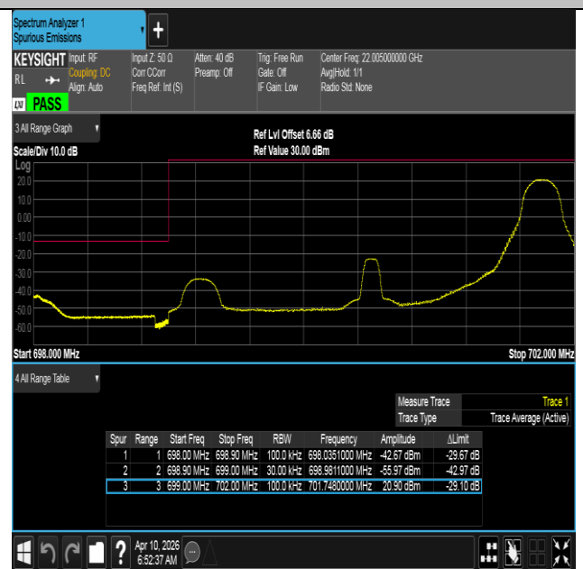
Band12-3MHz-QPSK-23025-1RB#14-PASS
