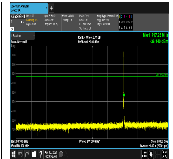
Band12-1.4MHz-16QAM-23173-6RB#0-30~1000-PASS
