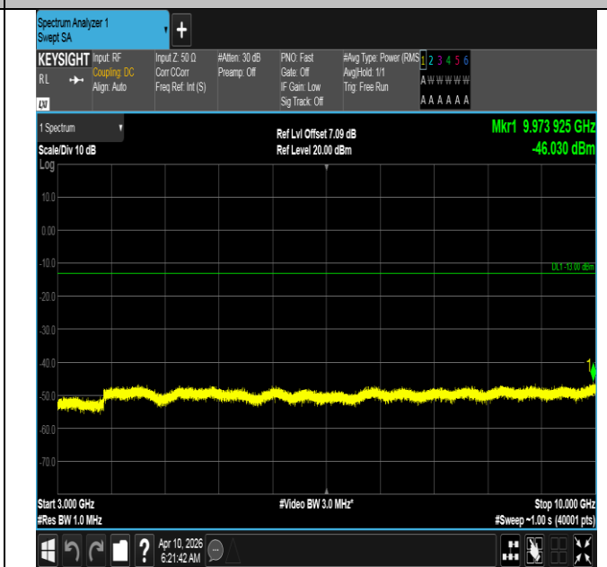
Band12-1.4MHz-QPSK-23173-1RB#5-3000~10000-PASS
