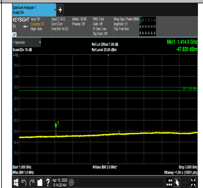
Band12-1.4MHz-QPSK-23095-1RB#0-1000~3000-PASS
