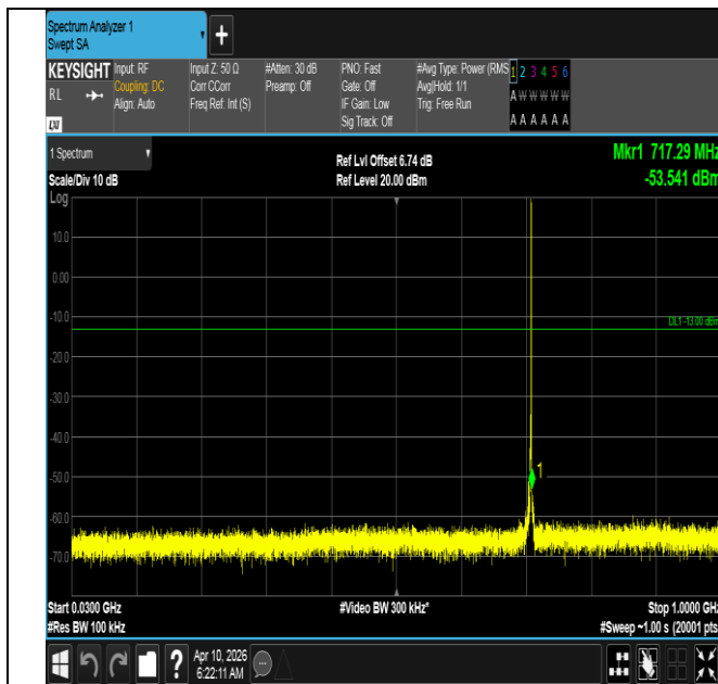
Band12-1.4MHz-16QAM-23173-1RB#5-30~1000-PASS
