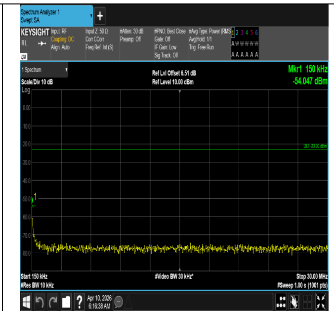
Band12-1.4MHz-16QAM-23095-1RB#5-0.15~30-PASS
