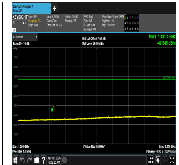
Band12-1.4MHz-16QAM-23173-1RB#5-1000~3000-PASS
