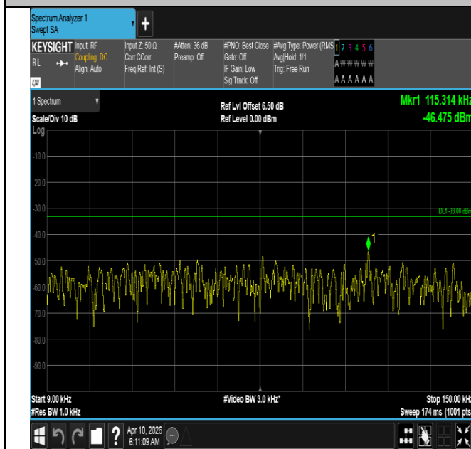
Band12-1.4MHz-16QAM-23017-1RB#5-0.009~0.15-PASS
