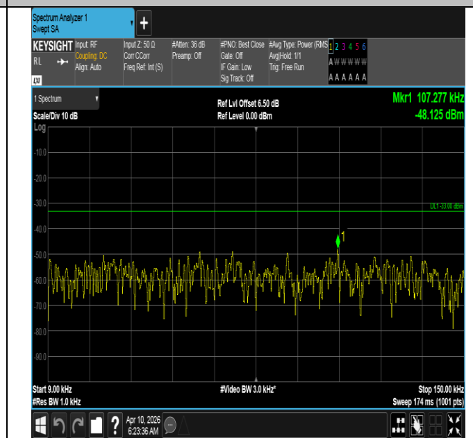
Band12-1.4MHz-16QAM-23173-6RB#0-0.009~0.15-PASS
