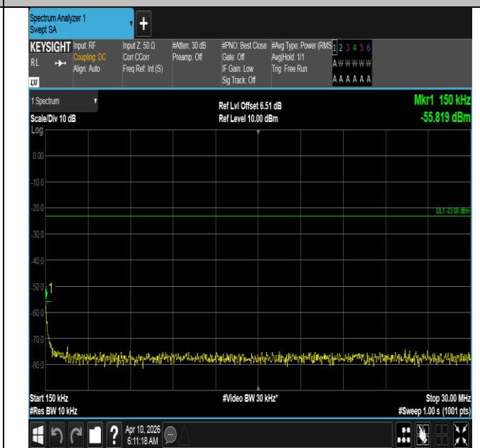
Band12-1.4MHz-16QAM-23017-1RB#5-0.15~30-PASS
