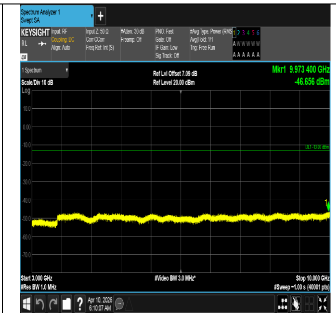
Band12-1.4MHz-16QAM-23017-1RB#0-3000~10000-PASS
