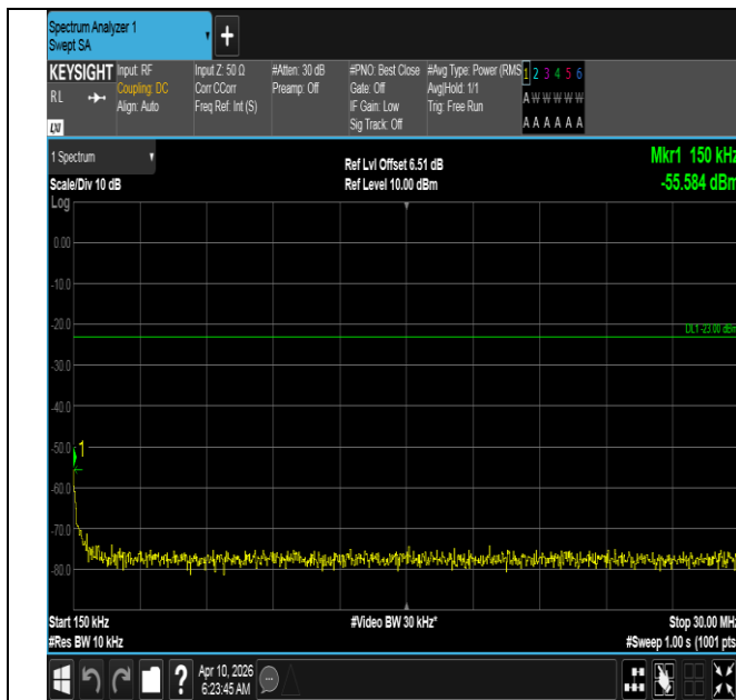
Band12-1.4MHz-16QAM-23173-6RB#0-0.15~30-PASS
