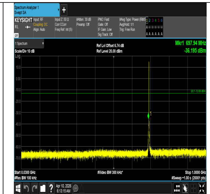
Band12-1.4MHz-16QAM-23017-6RB#0-30~1000-PASS
