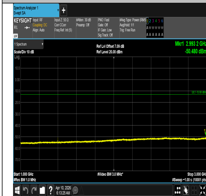
Band12-1.4MHz-16QAM-23017-6RB#0-1000~3000-PASS
