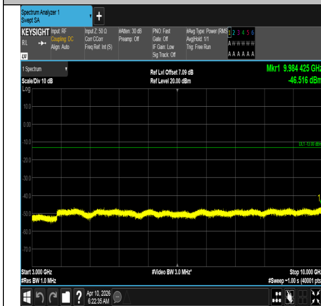
Band12-1.4MHz-16QAM-23173-1RB#5-3000~10000-PASS
