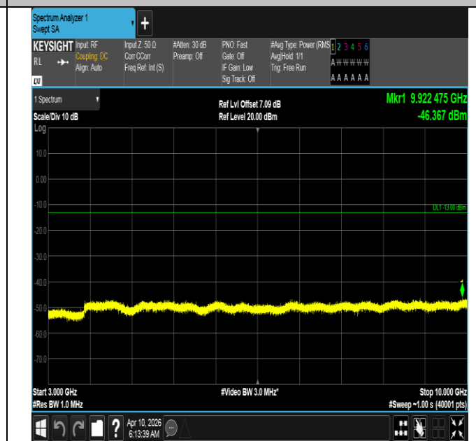
Band12-1.4MHz-16QAM-23017-6RB#0-3000~10000-PASS
