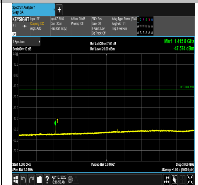
Band12-1.4MHz-16QAM-23095-1RB#5-1000~3000-PASS
