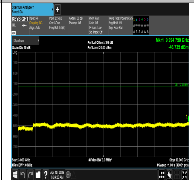
Band12-1.4MHz-16QAM-23173-6RB#0-3000~10000-PASS
