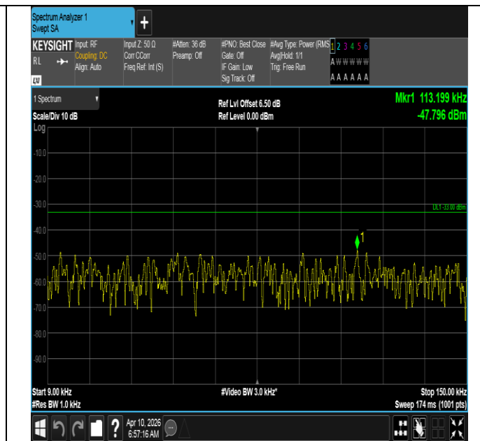
Band12-3MHz-QPSK-23025-1RB#14-0.009~0.15-PASS
