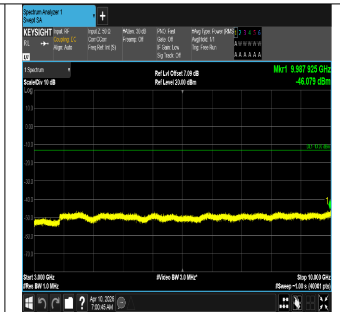
Band12-3MHz-16QAM-23025-15RB#0-3000~10000-PASS
