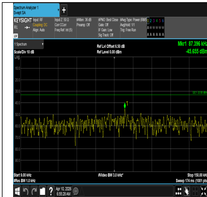
Band12-3MHz-QPSK-23025-1RB#0-0.009~0.15-PASS
