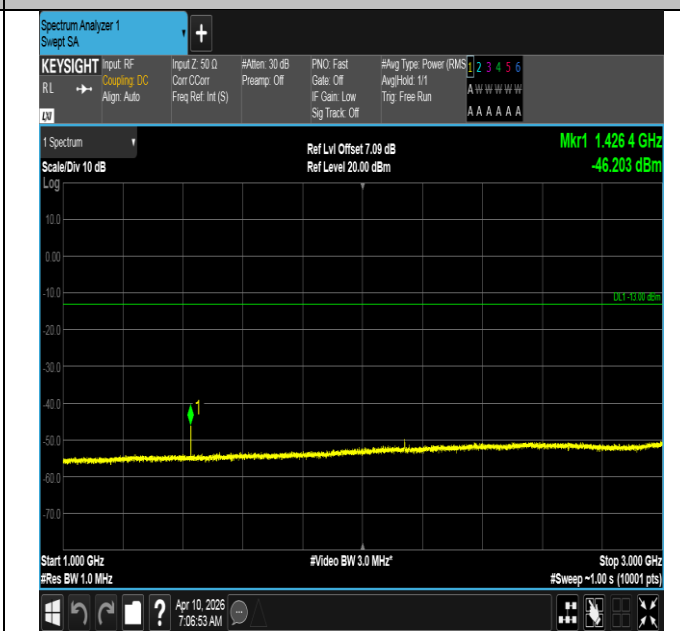
Band12-3MHz-QPSK-23165-1RB#0-1000~3000-PASS
