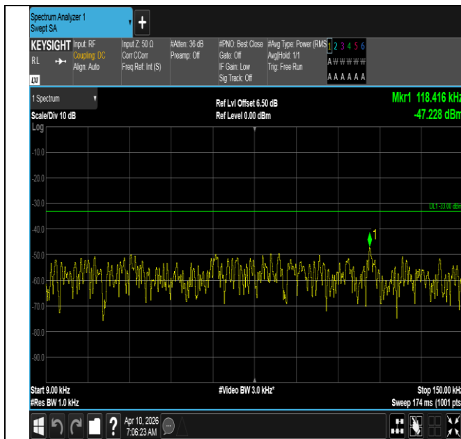
Band12-3MHz-QPSK-23165-1RB#0-0.009~0.15-PASS
