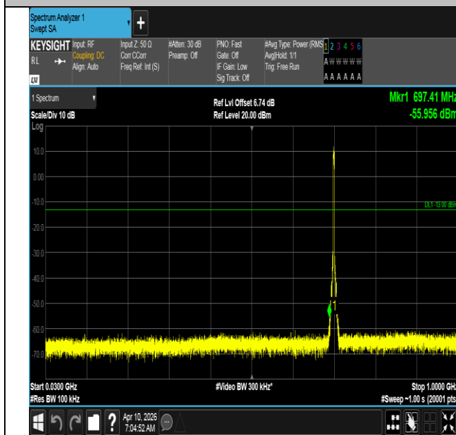
Band12-3MHz-QPSK-23095-15RB#0-30~1000-PASS
