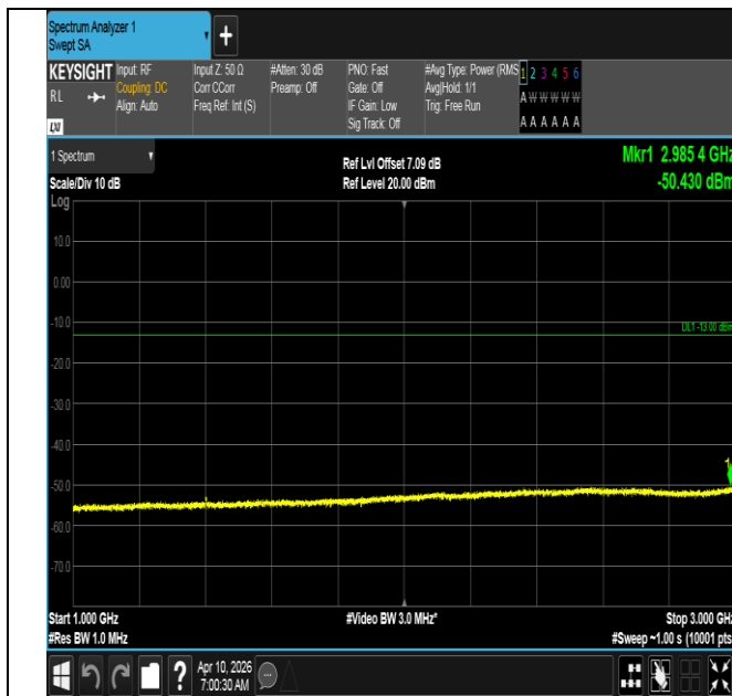
Band12-3MHz-16QAM-23025-15RB#0-1000~3000-PASS
