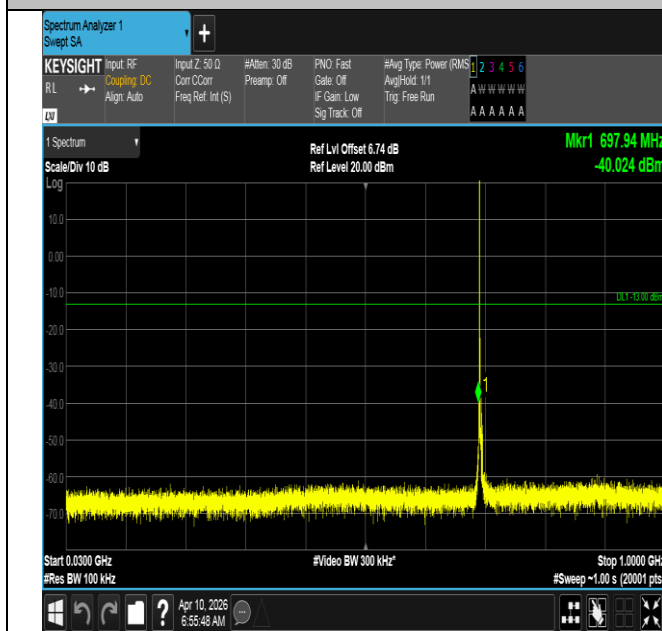
Band12-3MHz-QPSK-23025-1RB#0-30~1000-PASS
