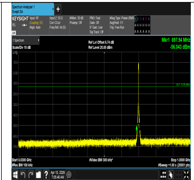
Band12-3MHz-16QAM-23095-15RB#0-30~1000-PASS
