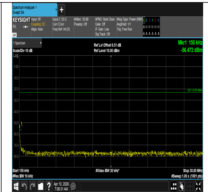
Band12-3MHz-QPSK-23165-1RB#0-0.15~30-PASS
