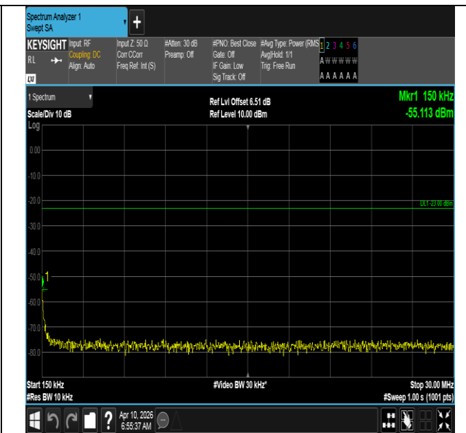
Band12-3MHz-QPSK-23025-1RB#0-0.15~30-PASS
