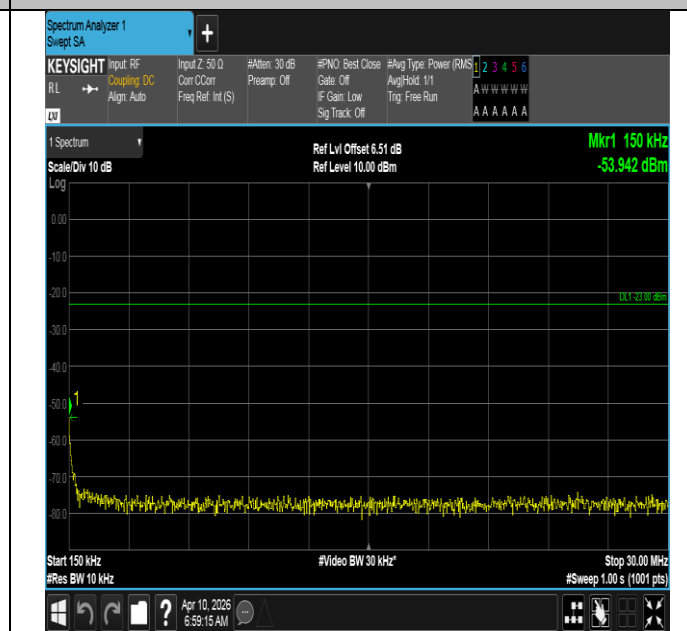
Band12-3MHz-QPSK-23025-15RB#0-0.15~30-PASS
