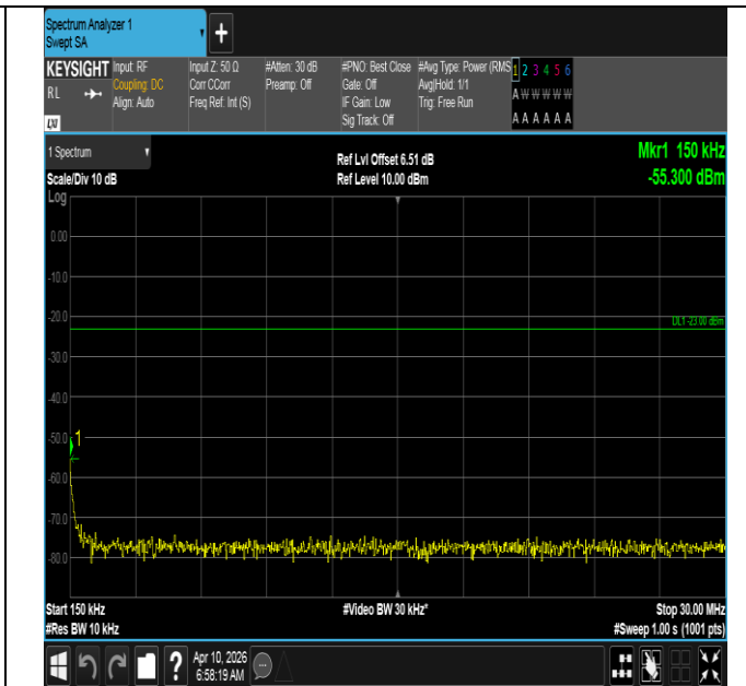
Band12-3MHz-16QAM-23025-1RB#14-0.15~30-PASS
