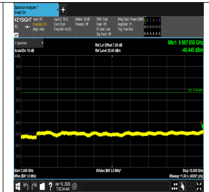
Band12-3MHz-16QAM-23095-1RB#0-3000~10000-PASS
