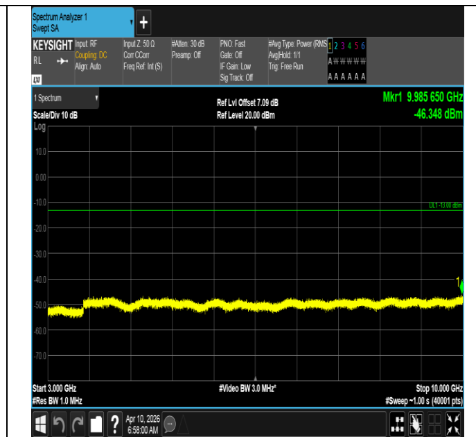
Band12-3MHz-QPSK-23025-1RB#14-3000~10000-PASS
