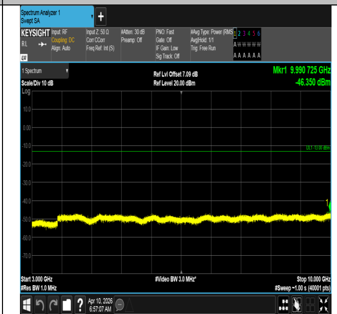
Band12-3MHz-16QAM-23025-1RB#0-3000~10000-PASS
