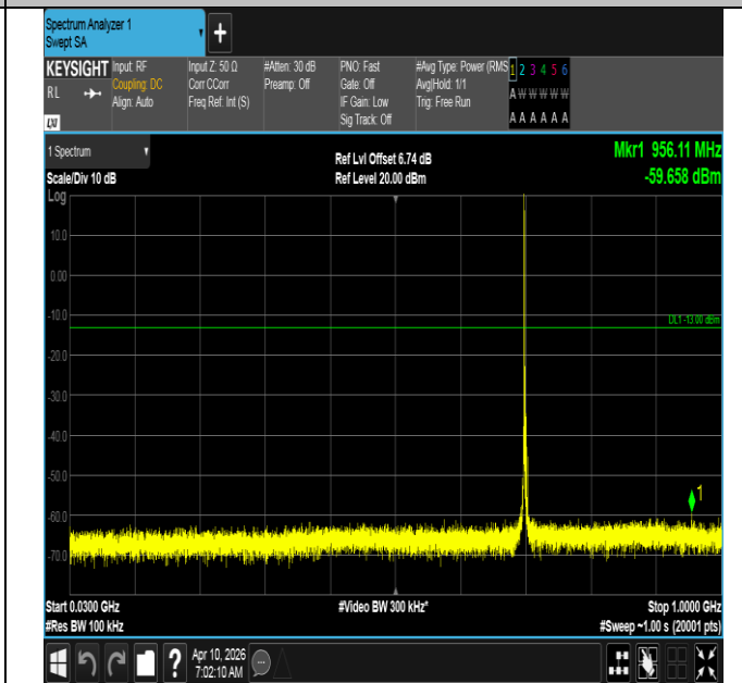
Band12-3MHz-16QAM-23095-1RB#0-30~1000-PASS
