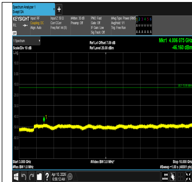
Band12-3MHz-QPSK-23025-1RB#0-3000~10000-PASS
