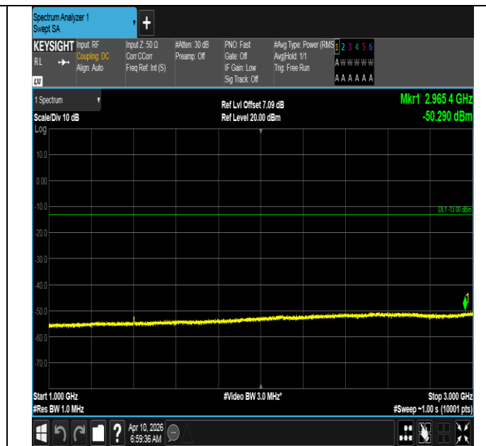
Band12-3MHz-QPSK-23025-15RB#0-1000~3000-PASS
