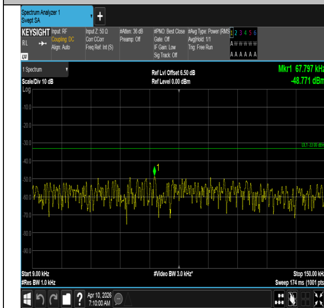
Band12-3MHz-QPSK-23165-15RB#0-0.009~0.15-PASS
