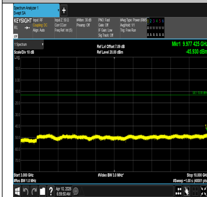
Band12-3MHz-QPSK-23025-15RB#0-3000~10000-PASS
