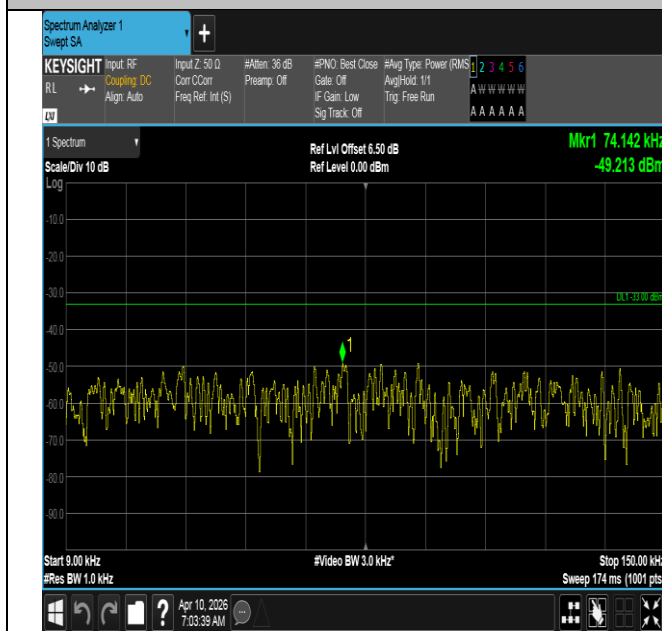
Band12-3MHz-16QAM-23095-1RB#14-0.009~0.15-PASS
