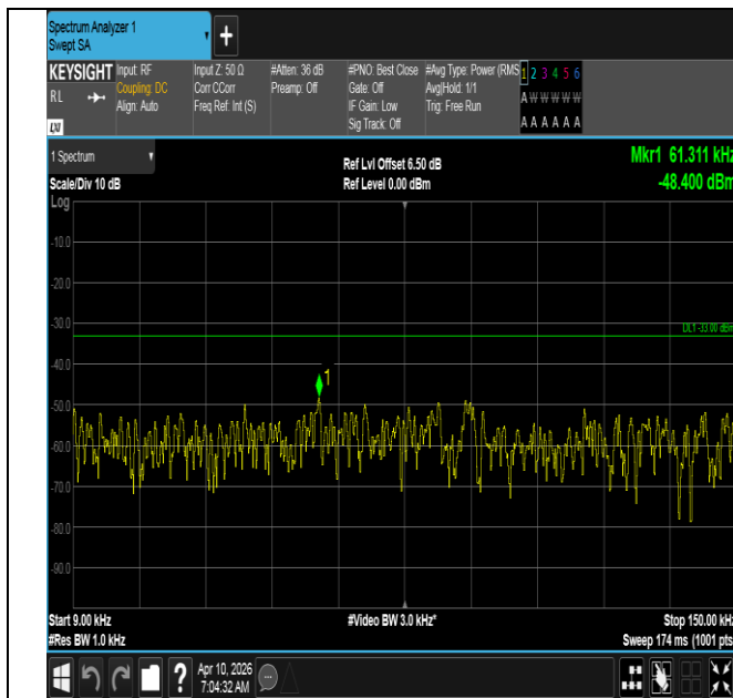
Band12-3MHz-QPSK-23095-15RB#0-0.009~0.15-PASS
