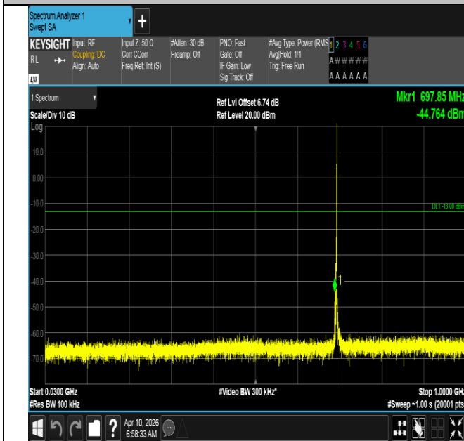
Band12-3MHz-16QAM-23025-1RB#14-30~1000-PASS
