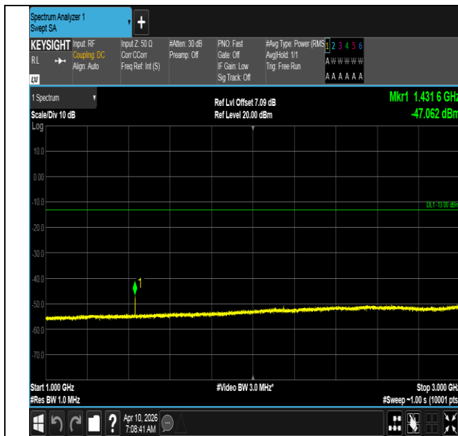
Band12-3MHz-QPSK-23165-1RB#14-1000~3000-PASS
