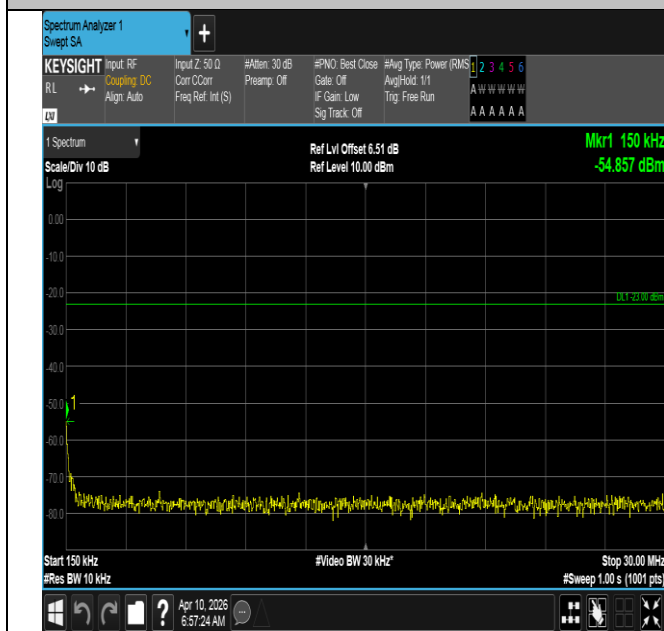
Band12-3MHz-QPSK-23025-1RB#14-0.15~30-PASS
