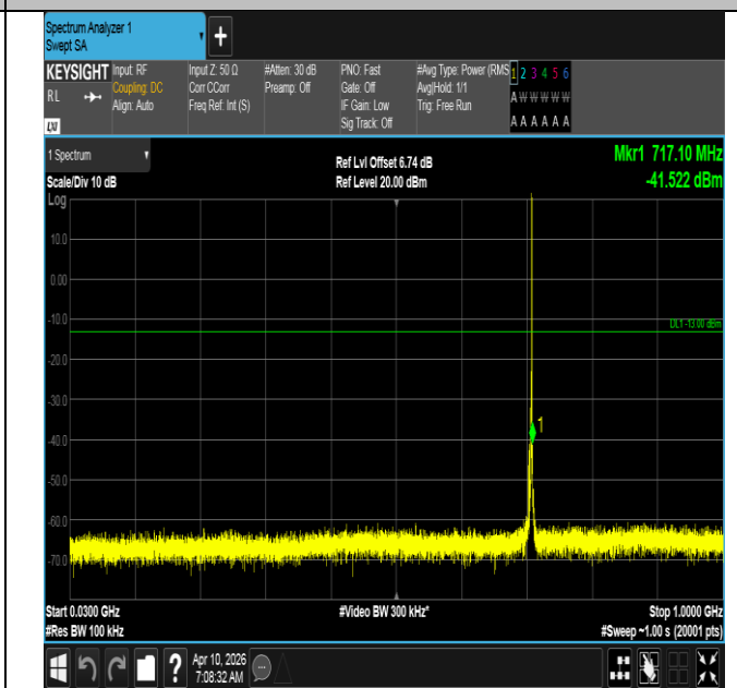
Band12-3MHz-QPSK-23165-1RB#14-30~1000-PASS
