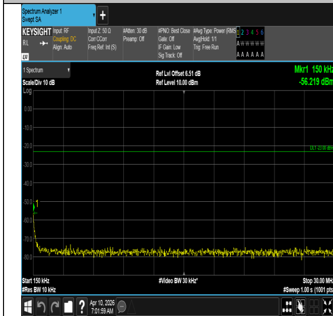
Band12-3MHz-16QAM-23095-1RB#0-0.15~30-PASS
