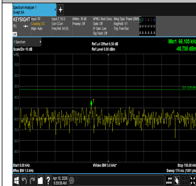
Band12-3MHz-QPSK-23025-15RB#0-0.009~0.15-PASS
