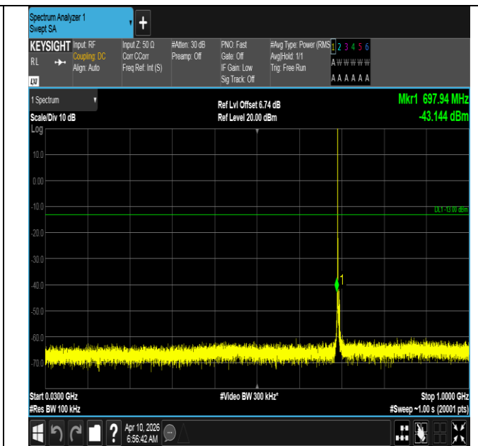
Band12-3MHz-16QAM-23025-1RB#0-30~1000-PASS
