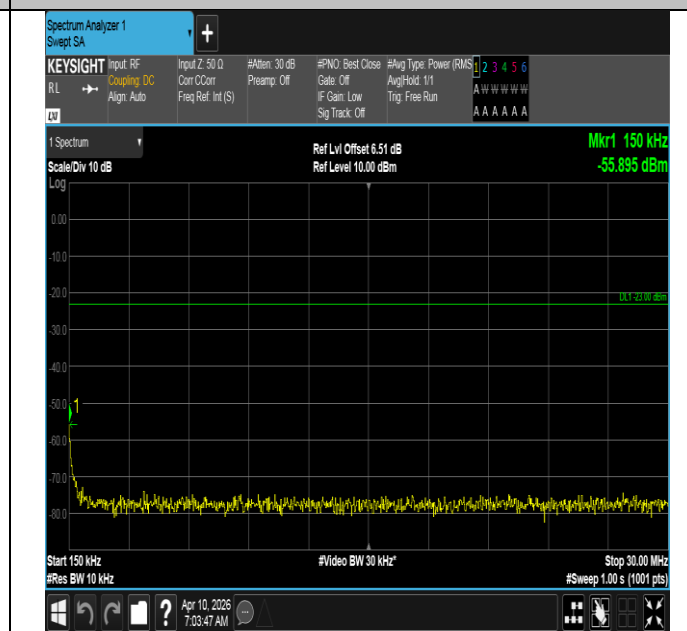
Band12-3MHz-16QAM-23095-1RB#14-0.15~30-PASS
