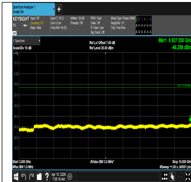
Band12-3MHz-QPSK-23095-15RB#0-3000~10000-PASS
