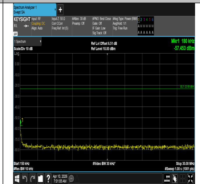
Band12-3MHz-QPSK-23095-1RB#0-0.15~30-PASS
