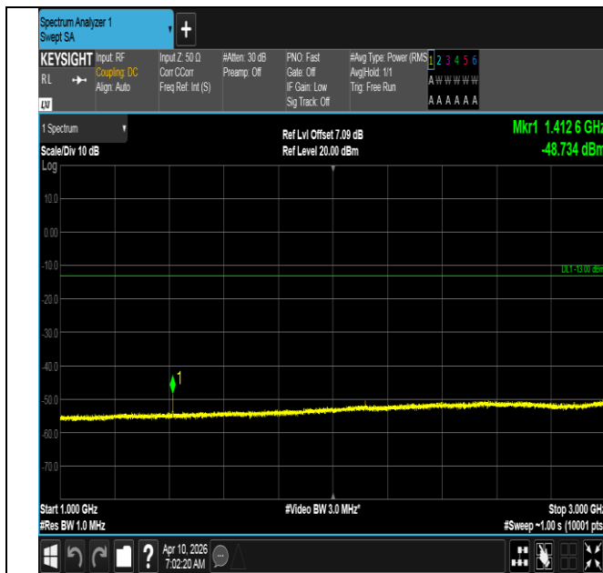
Band12-3MHz-16QAM-23095-1RB#0-1000~3000-PASS
