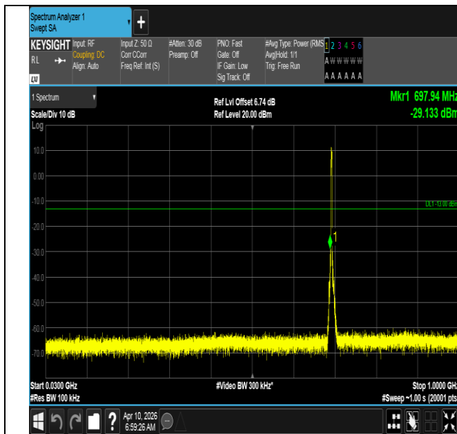
Band12-3MHz-QPSK-23025-15RB#0-30~1000-PASS
