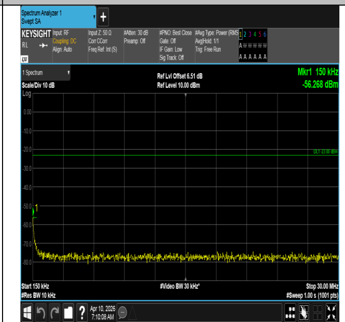
Band12-3MHz-QPSK-23165-15RB#0-0.15~30-PASS
