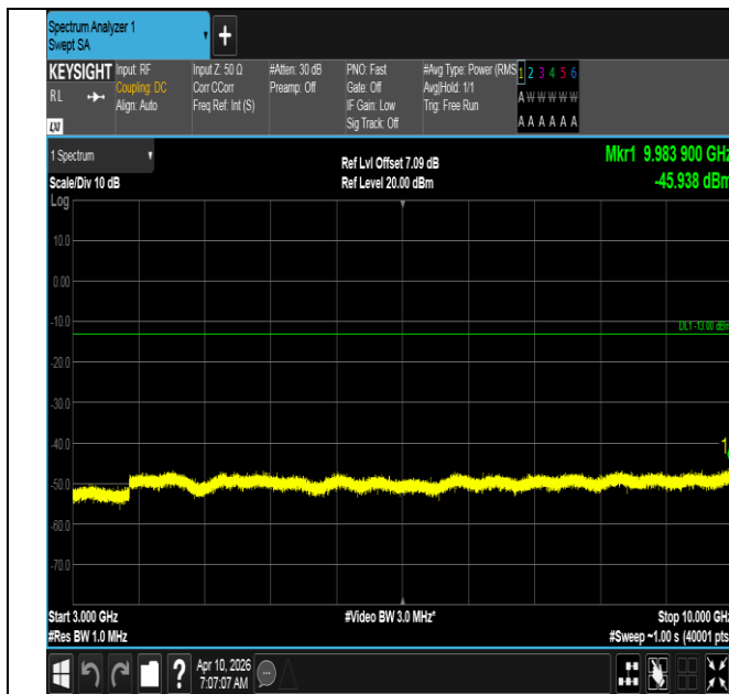
Band12-3MHz-QPSK-23165-1RB#0-3000~10000-PASS
