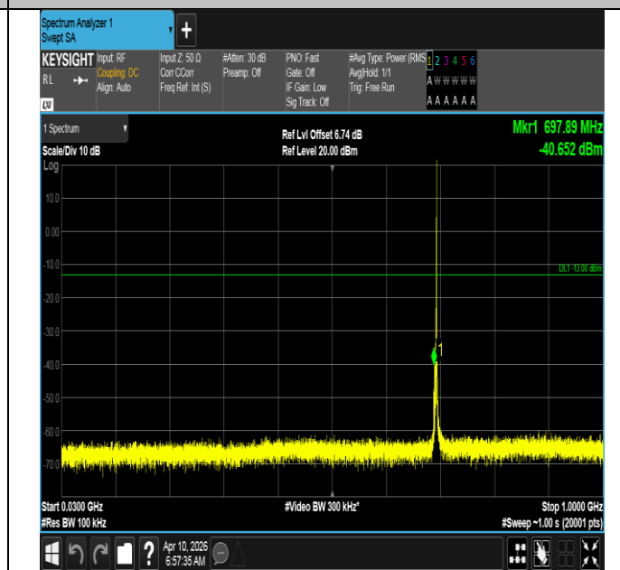
Band12-3MHz-QPSK-23025-1RB#14-30~1000-PASS
