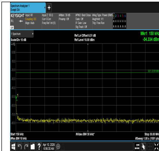
Band12-3MHz-16QAM-23025-1RB#0-0.15~30-PASS
