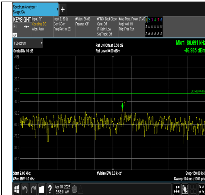
Band12-3MHz-16QAM-23025-1RB#14-0.009~0.15-PASS
