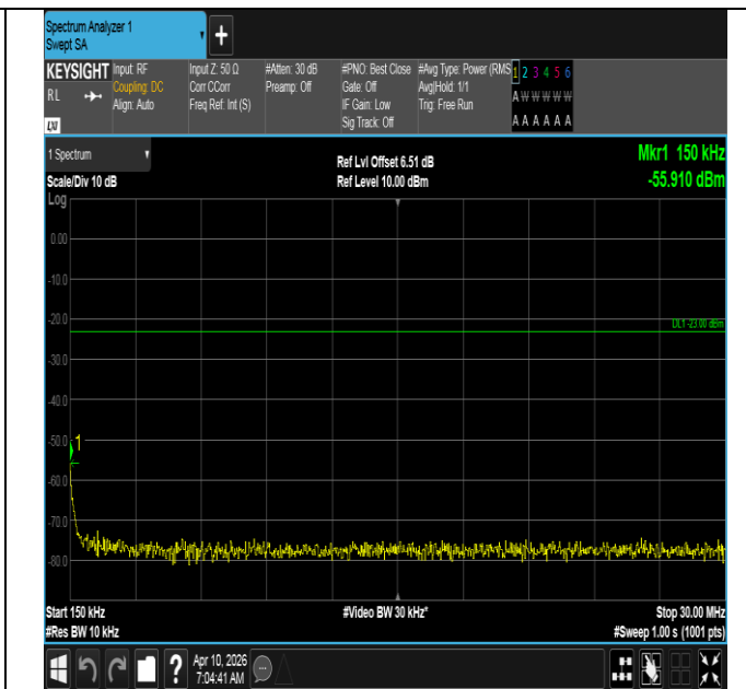
Band12-3MHz-QPSK-23095-15RB#0-0.15~30-PASS
