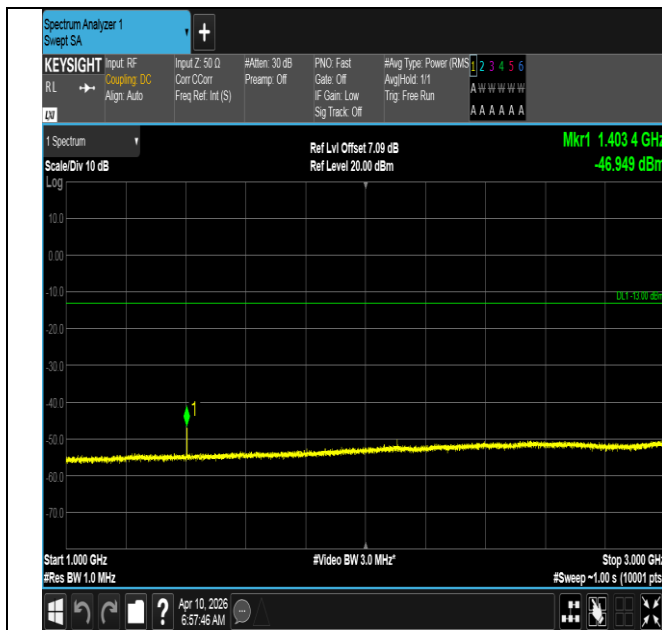
Band12-3MHz-QPSK-23025-1RB#14-1000~3000-PASS
