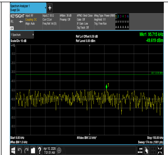
Band12-3MHz-16QAM-23095-1RB#0-0.009~0.15-PASS
