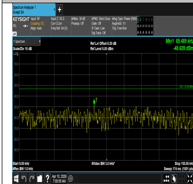
Band12-3MHz-QPSK-23095-1RB#0-0.009~0.15-PASS
