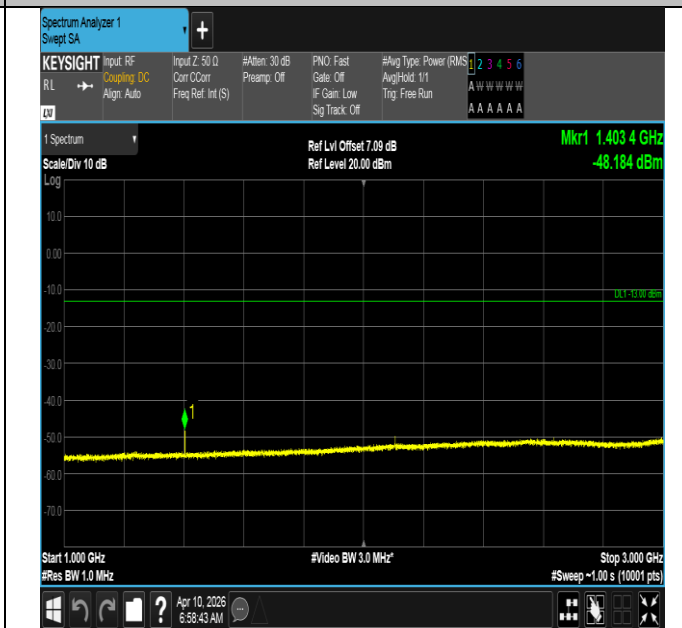
Band12-3MHz-16QAM-23025-1RB#14-1000~3000-PASS
