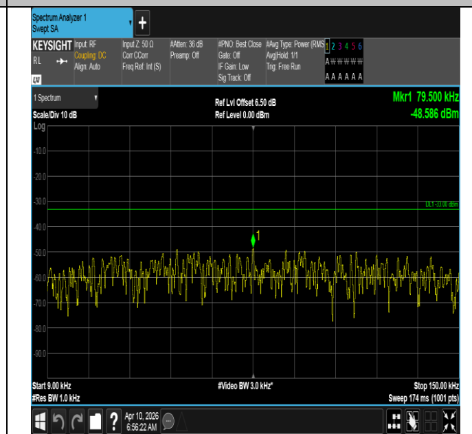
Band12-3MHz-16QAM-23025-1RB#0-0.009~0.15-PASS
