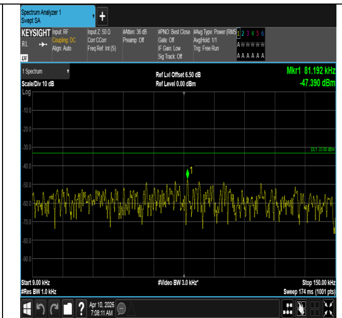
Band12-3MHz-QPSK-23165-1RB#14-0.009~0.15-PASS
