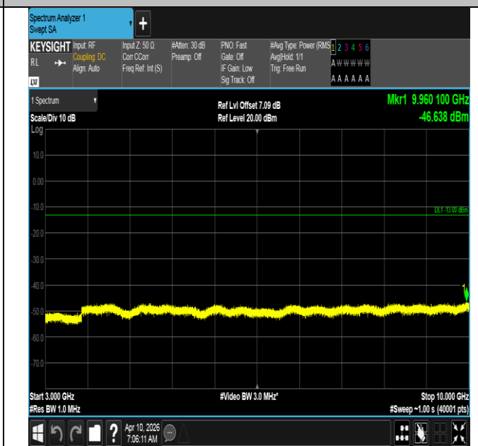
Band12-3MHz-16QAM-23095-15RB#0-3000~10000-PASS
