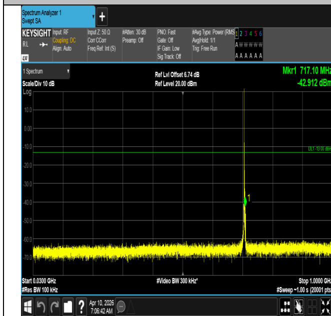
Band12-3MHz-QPSK-23165-1RB#0-30~1000-PASS
