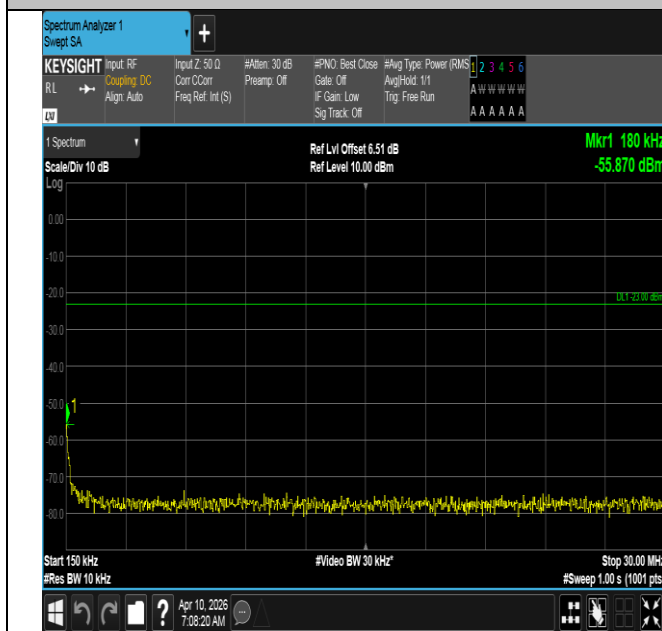
Band12-3MHz-QPSK-23165-1RB#14-0.15~30-PASS
