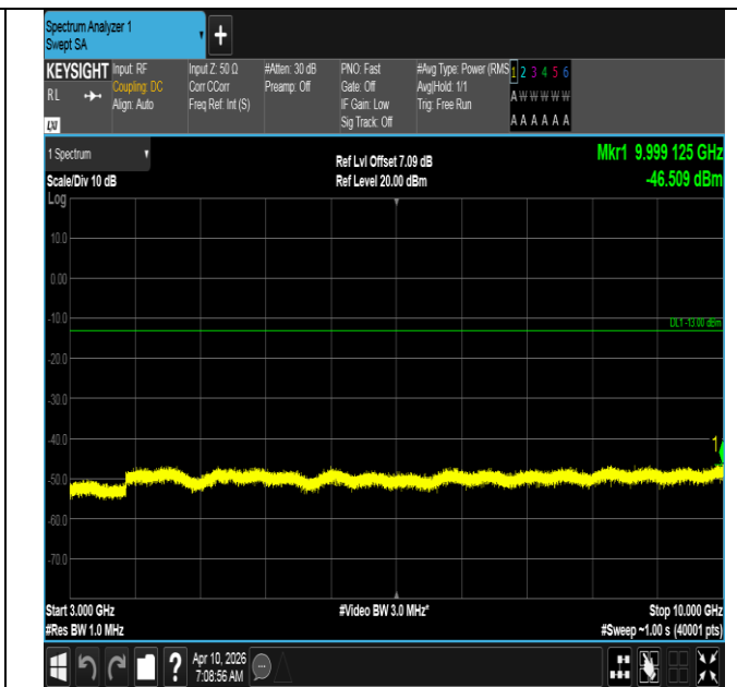
Band12-3MHz-QPSK-23165-1RB#14-3000~10000-PASS
