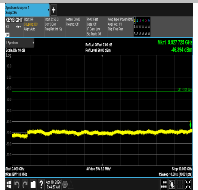
Band12-5MHz-QPSK-23035-1RB#24-3000~10000-PASS
