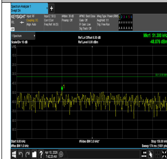
Band12-5MHz-QPSK-23035-1RB#0-0.009~0.15-PASS
