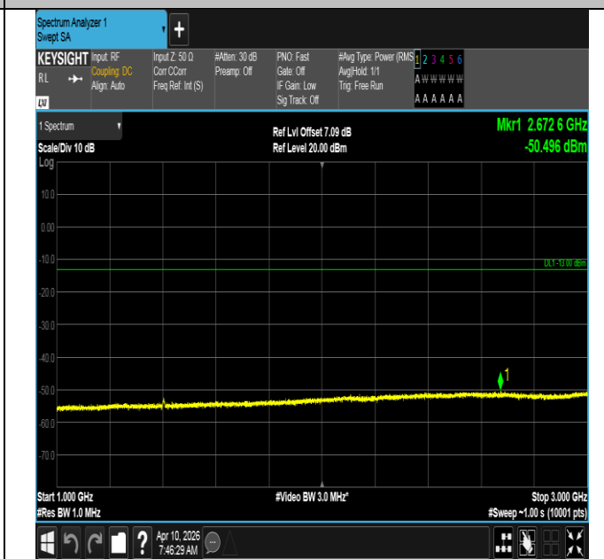
Band12-5MHz-QPSK-23035-25RB#0-1000~3000-PASS
