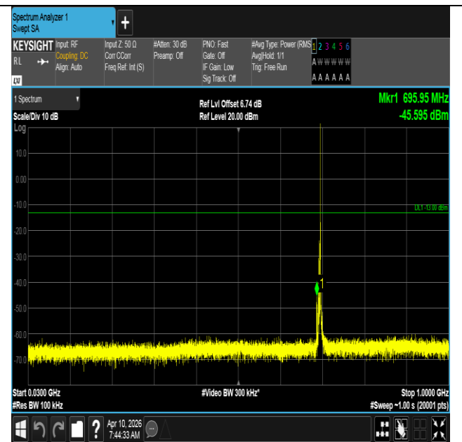
Band12-5MHz-QPSK-23035-1RB#24-30~1000-PASS
