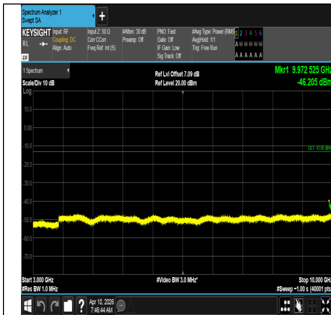
Band12-5MHz-QPSK-23035-25RB#0-3000~10000-PASS
