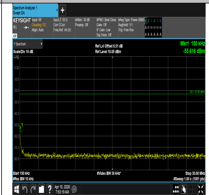
Band12-5MHz-QPSK-23155-1RB#0-0.15~30-PASS
