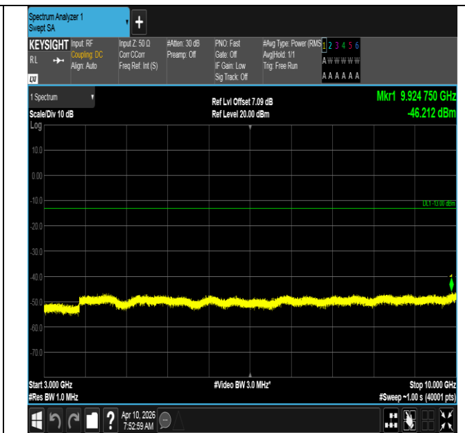
Band12-5MHz-16QAM-23095-25RB#0-3000~10000-PASS
