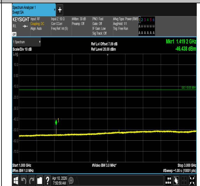
Band12-5MHz-16QAM-23095-1RB#24-1000~3000-PASS
