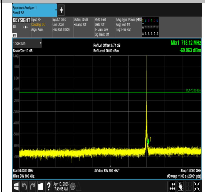
Band12-5MHz-QPSK-23095-1RB#24-30~1000-PASS
