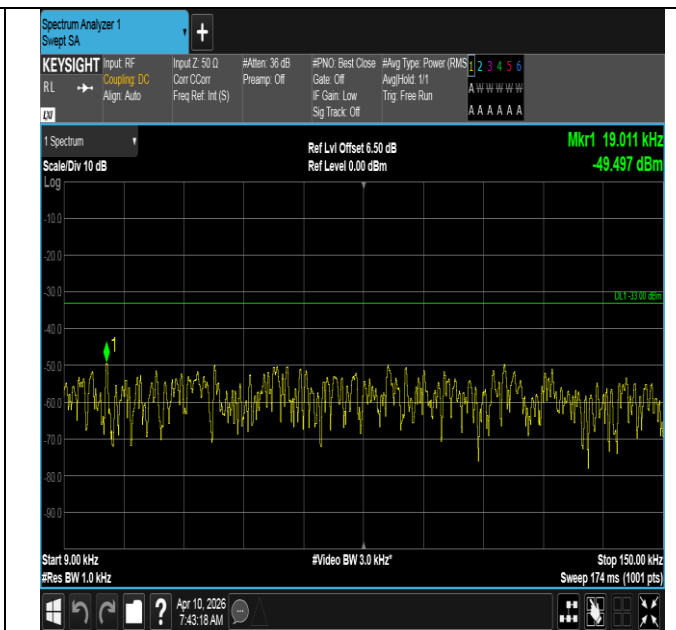
Band12-5MHz-16QAM-23035-1RB#0-0.009~0.15-PASS
