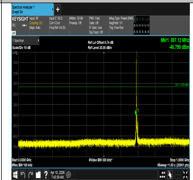
Band12-5MHz-16QAM-23035-1RB#0-30~1000-PASS
