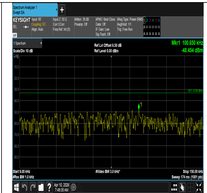
Band12-5MHz-QPSK-23095-1RB#24-0.009~0.15-PASS
