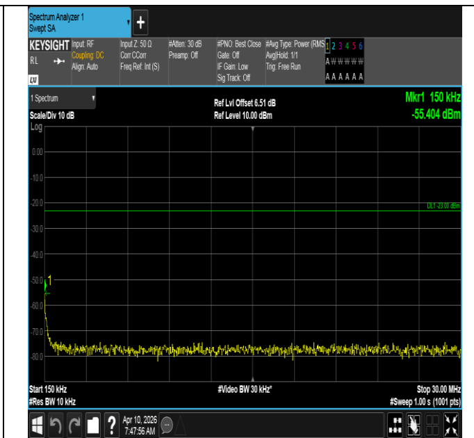
Band12-5MHz-QPSK-23095-1RB#0-0.15~30-PASS
