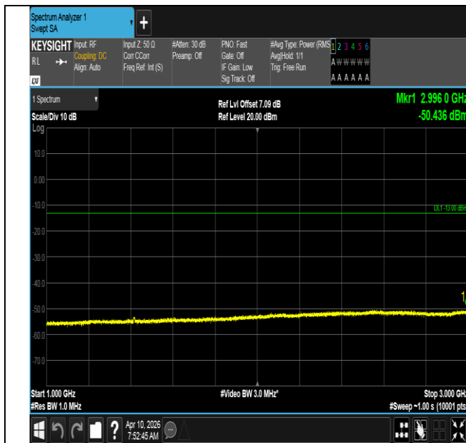
Band12-5MHz-16QAM-23095-25RB#0-1000~3000-PASS
