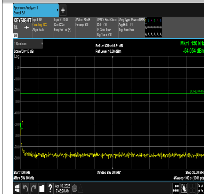
Band12-5MHz-16QAM-23035-1RB#0-0.15~30-PASS
