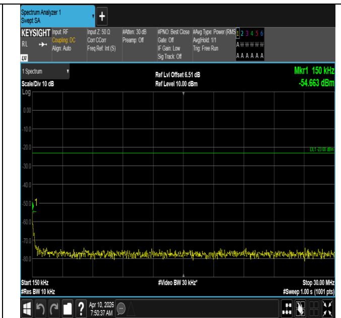
Band12-5MHz-16QAM-23095-1RB#24-0.15~30-PASS
