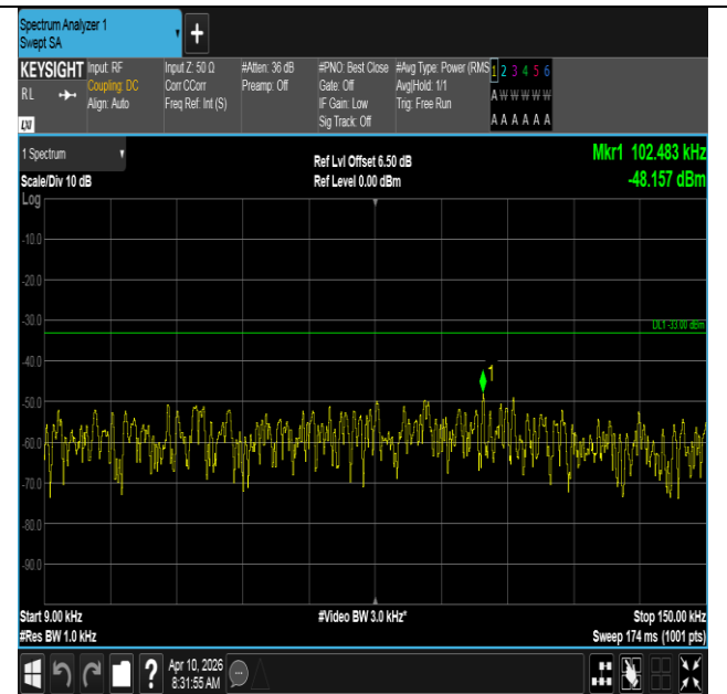
Band12-10MHz-16QAM-23060-50RB#0-0.009~0.15-PASS
