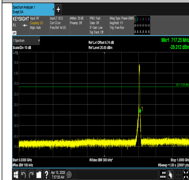
Band12-5MHz-QPSK-23155-25RB#0-30~1000-PASS
