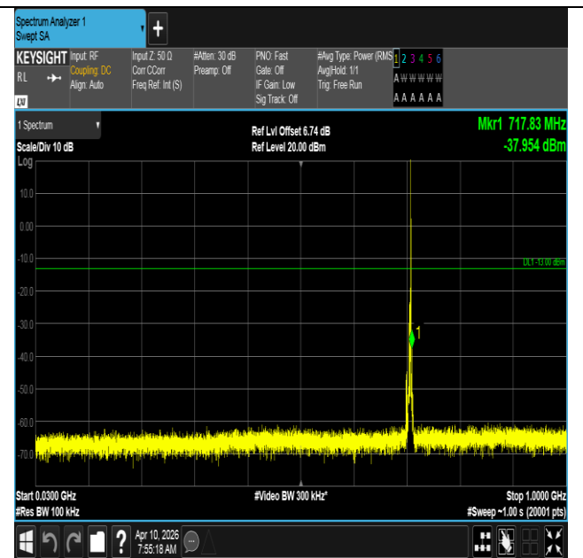
Band12-5MHz-QPSK-23155-1RB#24-30~1000-PASS
