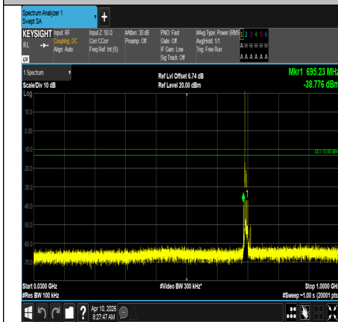
Band12-10MHz-QPSK-23060-1RB#0-30~1000-PASS
