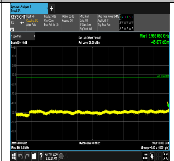
Band12-10MHz-QPSK-23095-1RB#49-3000~10000-PASS
