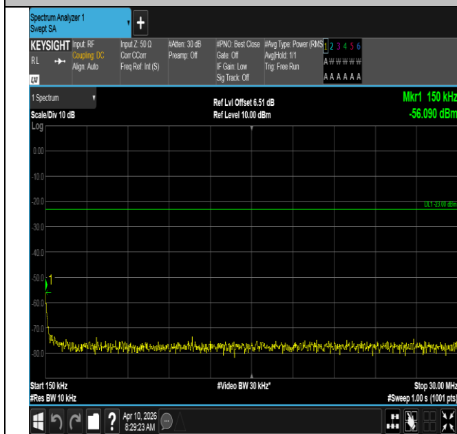
Band12-10MHz-QPSK-23060-1RB#49-0.15~30-PASS
