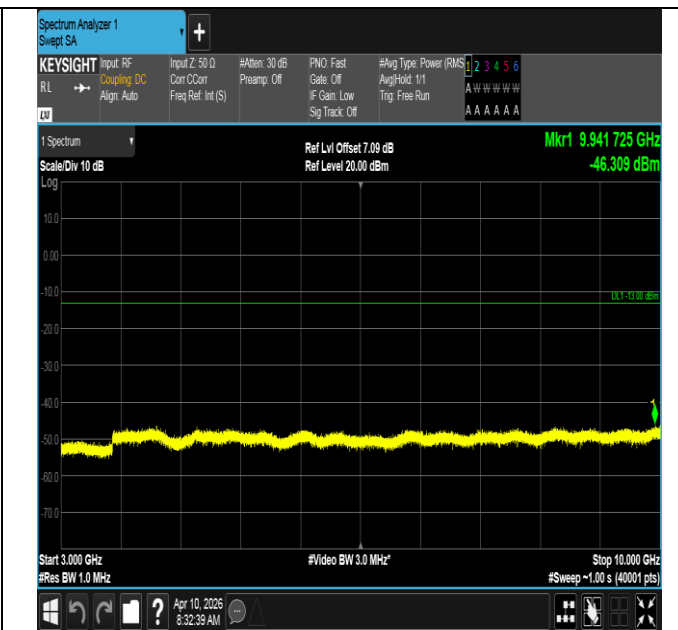
Band12-10MHz-16QAM-23060-50RB#0-3000~10000-PASS
