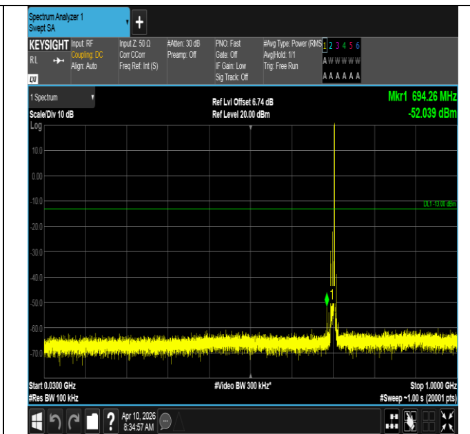
Band12-10MHz-QPSK-23095-1RB#49-30~1000-PASS
