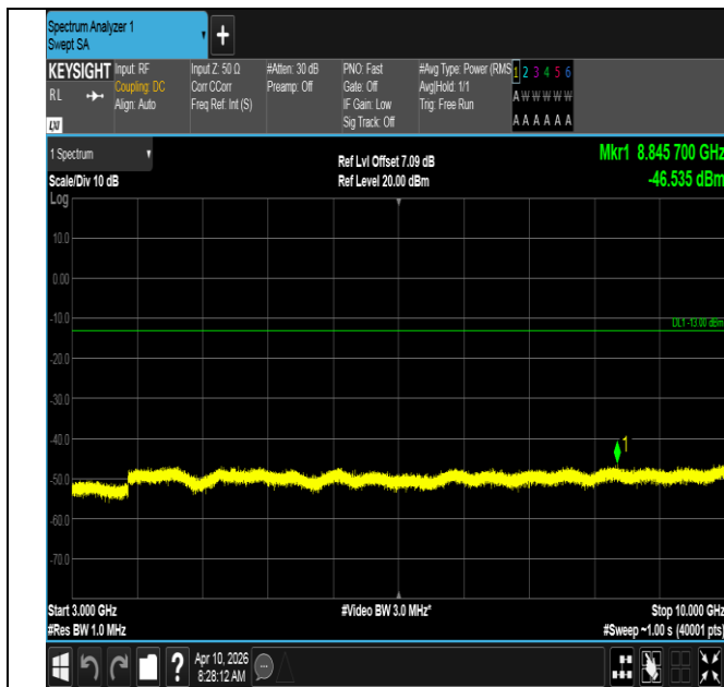
Band12-10MHz-QPSK-23060-1RB#0-3000~10000-PASS
