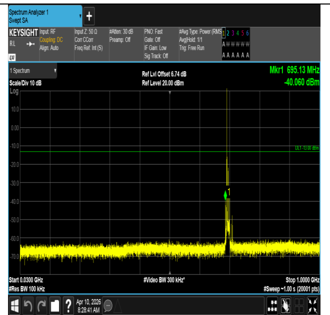
Band12-10MHz-16QAM-23060-1RB#0-30~1000-PASS
