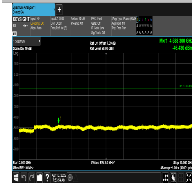
Band12-5MHz-QPSK-23155-1RB#0-3000~10000-PASS
