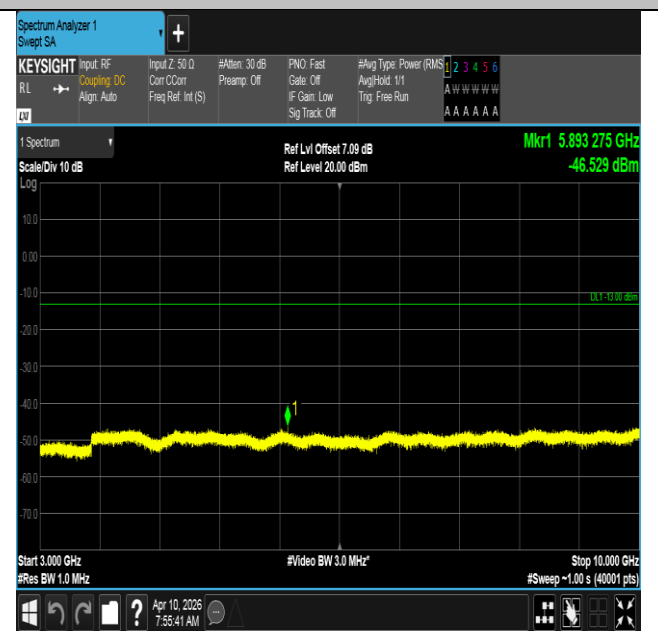
Band12-5MHz-QPSK-23155-1RB#24-3000~10000-PASS
