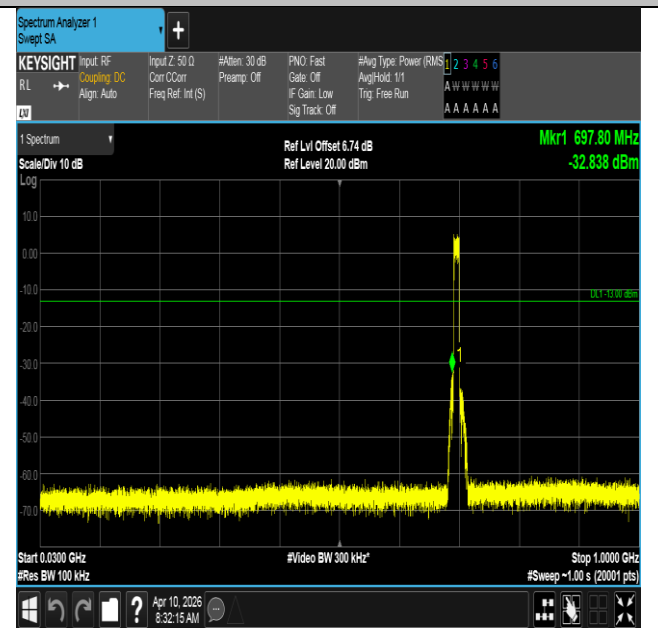
Band12-10MHz-16QAM-23060-50RB#0-30~1000-PASS
