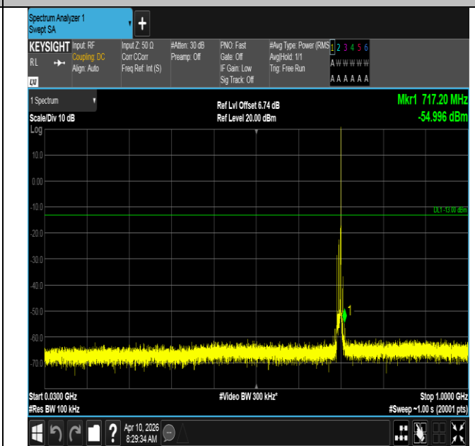
Band12-10MHz-QPSK-23060-1RB#49-30~1000-PASS
