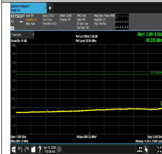
Band12-5MHz-16QAM-23155-25RB#0-1000~3000-PASS
