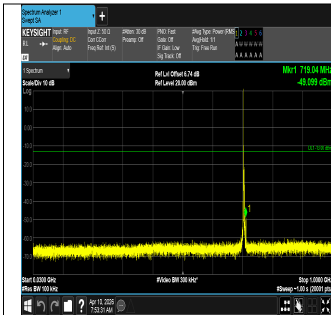
Band12-5MHz-QPSK-23155-1RB#0-30~1000-PASS
