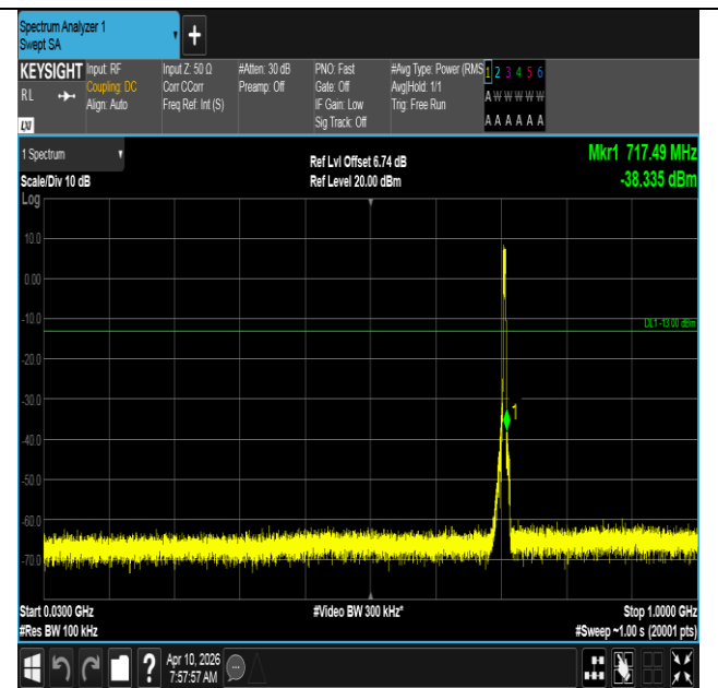
Band12-5MHz-16QAM-23155-25RB#0-30~1000-PASS
