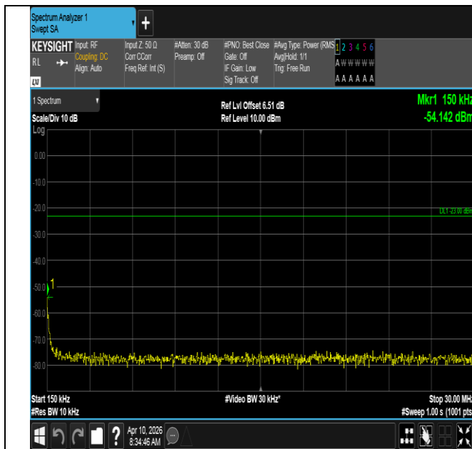
Band12-10MHz-QPSK-23095-1RB#49-0.15~30-PASS
