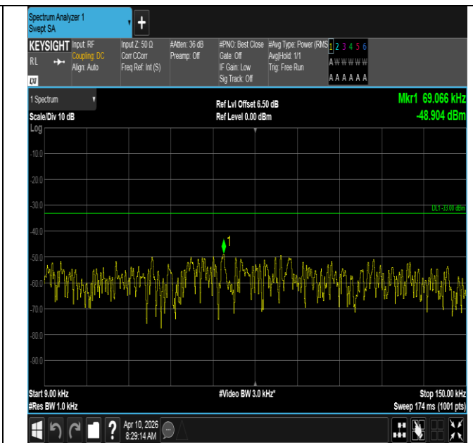
Band12-10MHz-QPSK-23060-1RB#49-0.009~0.15-PASS
