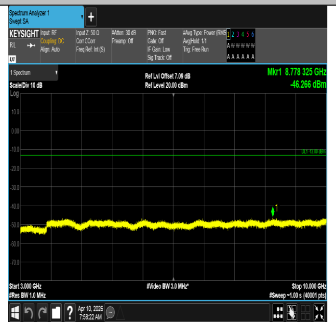
Band12-5MHz-16QAM-23155-25RB#0-3000~10000-PASS
