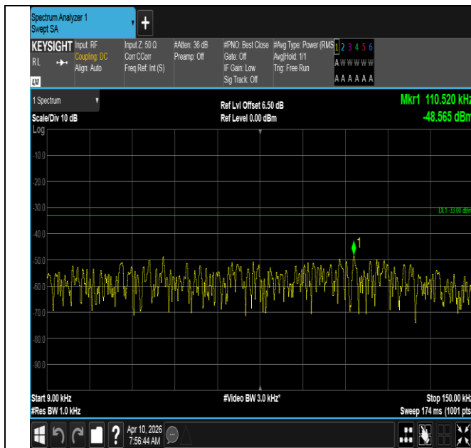
Band12-5MHz-QPSK-23155-25RB#0-0.009~0.15-PASS
