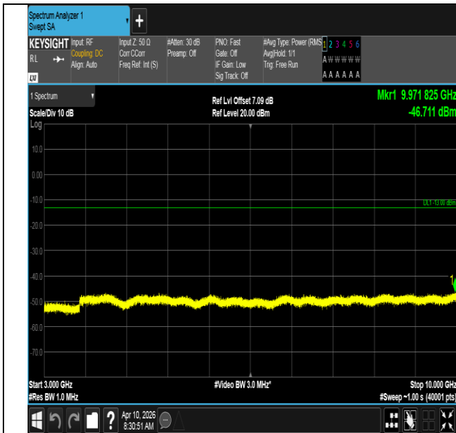
Band12-10MHz-16QAM-23060-1RB#49-3000~10000-PASS
