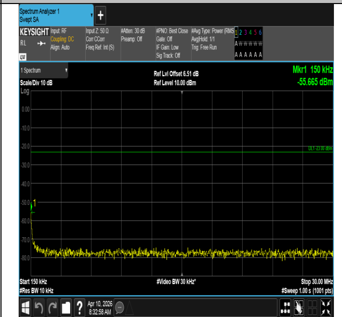
Band12-10MHz-QPSK-23095-1RB#0-0.15~30-PASS
