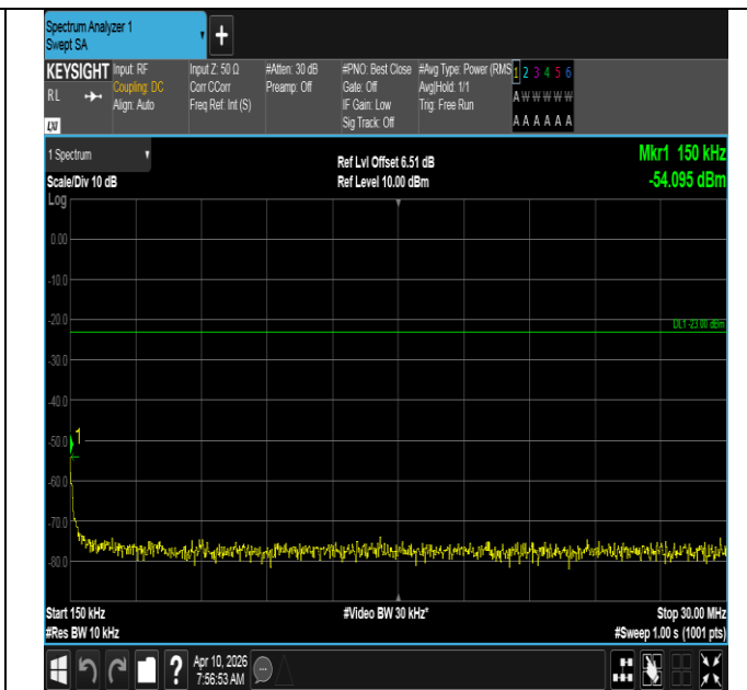
Band12-5MHz-QPSK-23155-25RB#0-0.15~30-PASS
