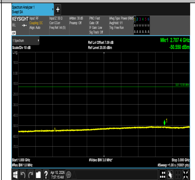
Band12-5MHz-QPSK-23155-25RB#0-1000~3000-PASS
