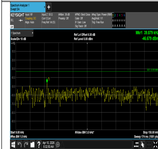
Band12-10MHz-QPSK-23095-1RB#0-0.009~0.15-PASS
