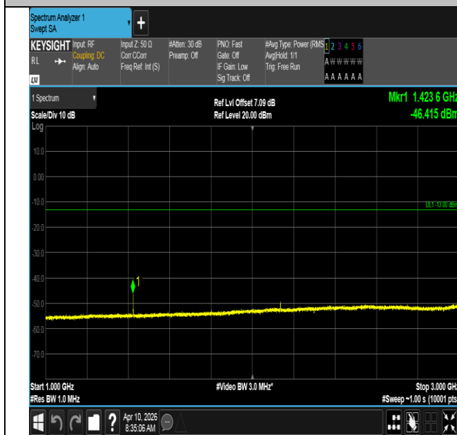
Band12-10MHz-QPSK-23095-1RB#49-1000~3000-PASS
