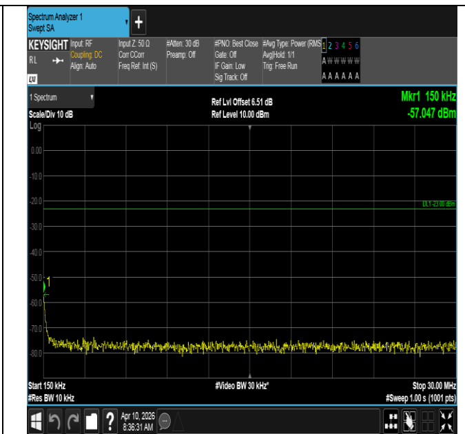
Band12-10MHz-QPSK-23095-50RB#0-0.15~30-PASS
