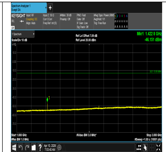
Band12-5MHz-QPSK-23155-1RB#0-1000~3000-PASS
