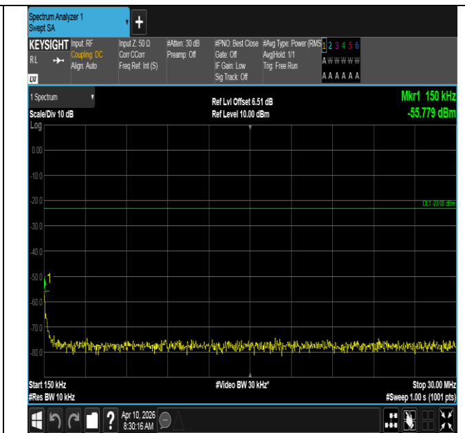
Band12-10MHz-16QAM-23060-1RB#49-0.15~30-PASS
