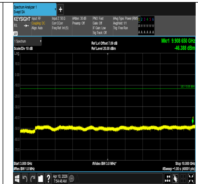
Band12-5MHz-16QAM-23155-1RB#0-3000~10000-PASS
