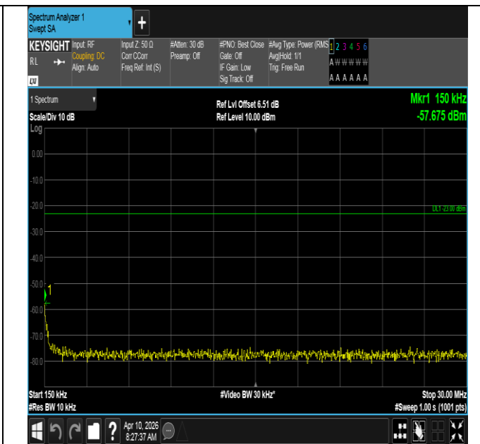
Band12-10MHz-QPSK-23060-1RB#0-0.15~30-PASS
