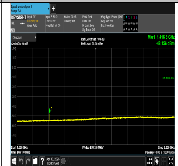
Band12-10MHz-16QAM-23060-1RB#49-1000~3000-PASS
