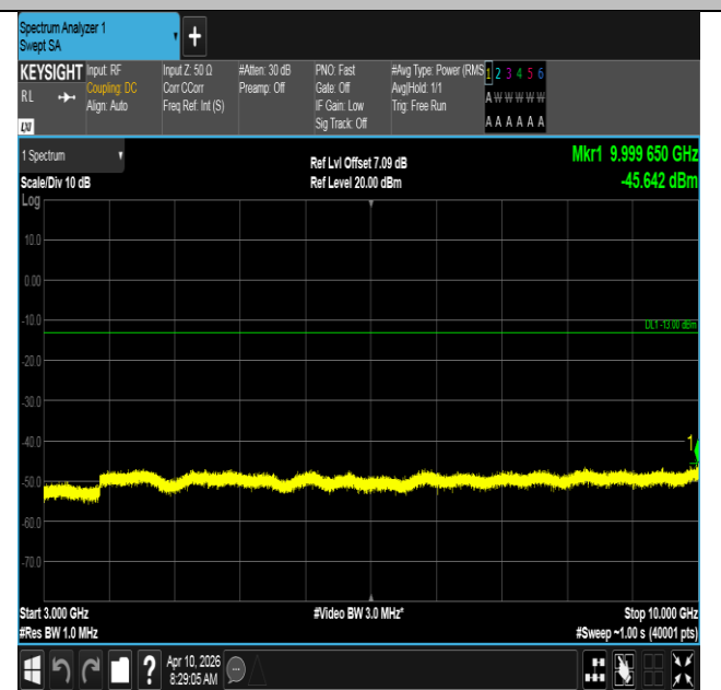
Band12-10MHz-16QAM-23060-1RB#0-3000~10000-PASS
