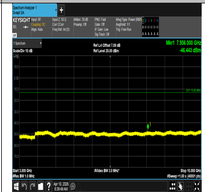
Band12-10MHz-16QAM-23130-1RB#0-3000~10000-PASS
