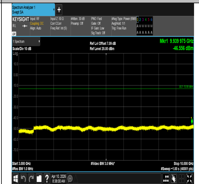
Band12-10MHz-16QAM-23095-50RB#0-3000~10000-PASS
