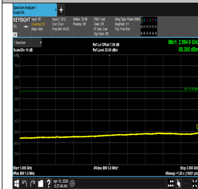
Band12-10MHz-16QAM-23095-50RB#0-1000~3000-PASS
