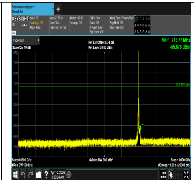
Band12-10MHz-16QAM-23130-1RB#0-30~1000-PASS
