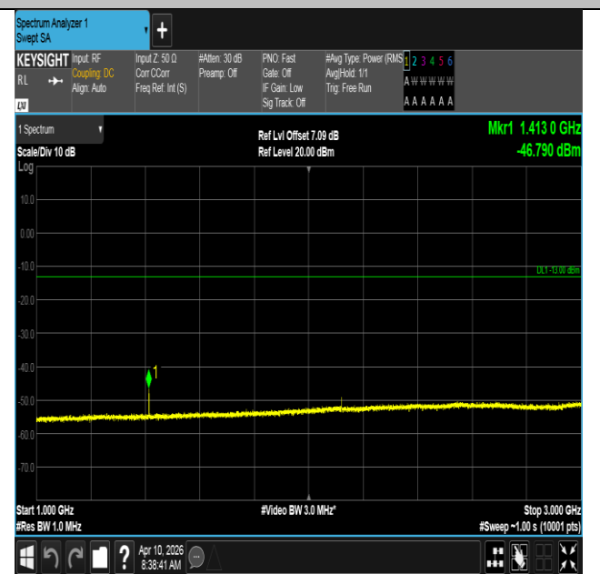
Band12-10MHz-QPSK-23130-1RB#0-1000~3000-PASS
