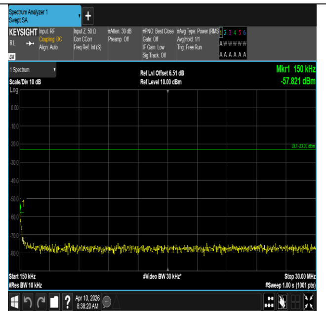
Band12-10MHz-QPSK-23130-1RB#0-0.15~30-PASS
