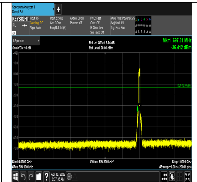
Band12-10MHz-16QAM-23095-50RB#0-30~1000-PASS
