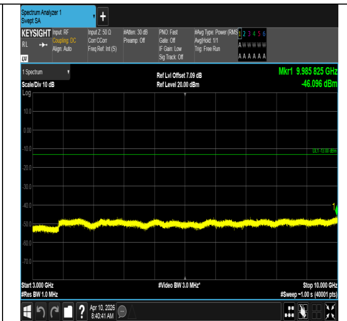
Band12-10MHz-QPSK-23130-1RB#49-3000~10000-PASS
