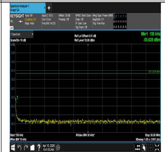
Band12-10MHz-QPSK-23130-50RB#0-0.15~30-PASS
