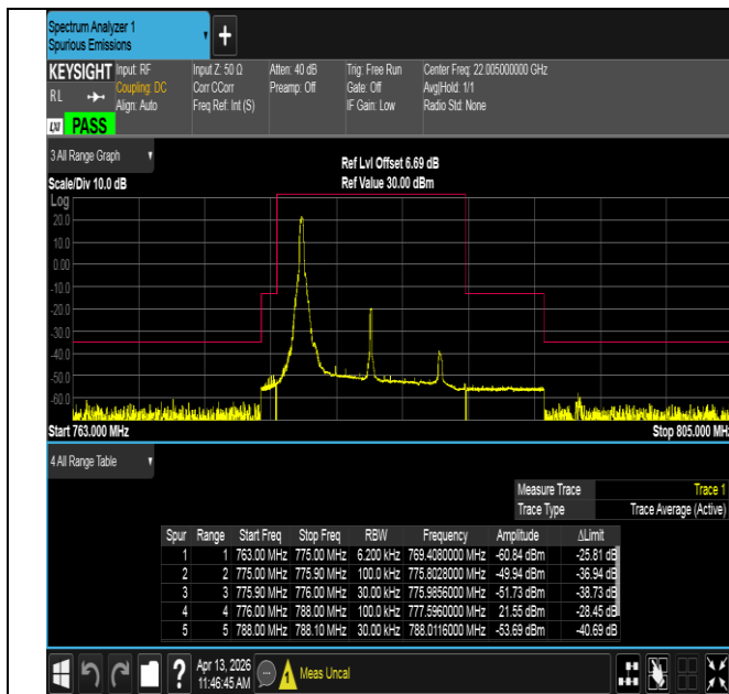
Band13-10MHz-QPSK-23230-1RB#0-PASS
