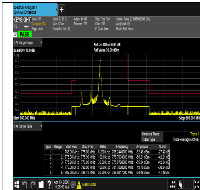
Band13-5MHz-16QAM-23205-1RB#24-PASS
