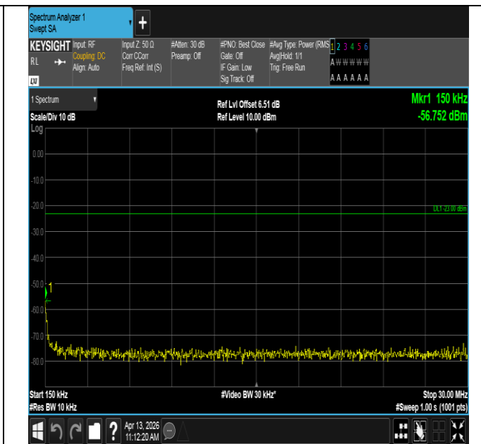
Band13-5MHz-QPSK-23205-25RB#0-0.15~30-PASS
