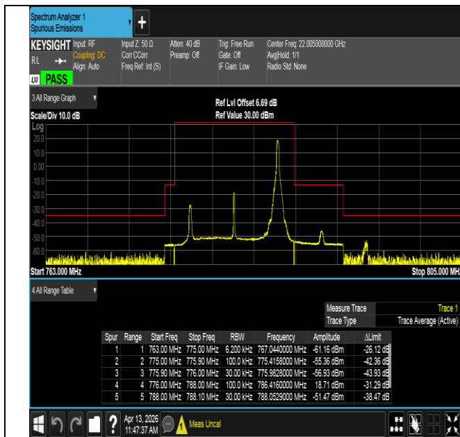
Band13-10MHz-16QAM-23230-1RB#49-PASS
