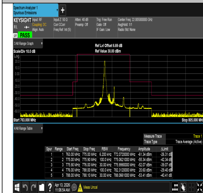
Band13-5MHz-QPSK-23255-1RB#0-PASS
