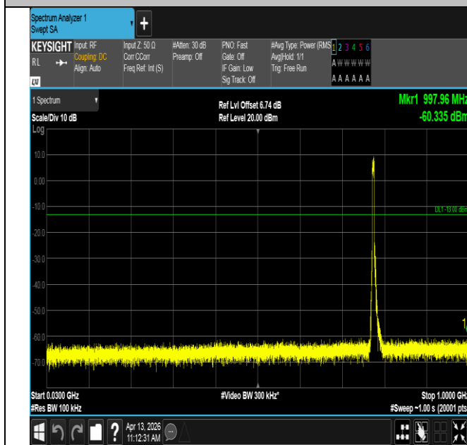
Band13-5MHz-QPSK-23205-25RB#0-30~1000-PASS
