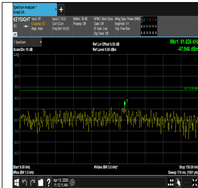
Band13-5MHz-QPSK-23205-25RB#0-0.009~0.15-PASS
