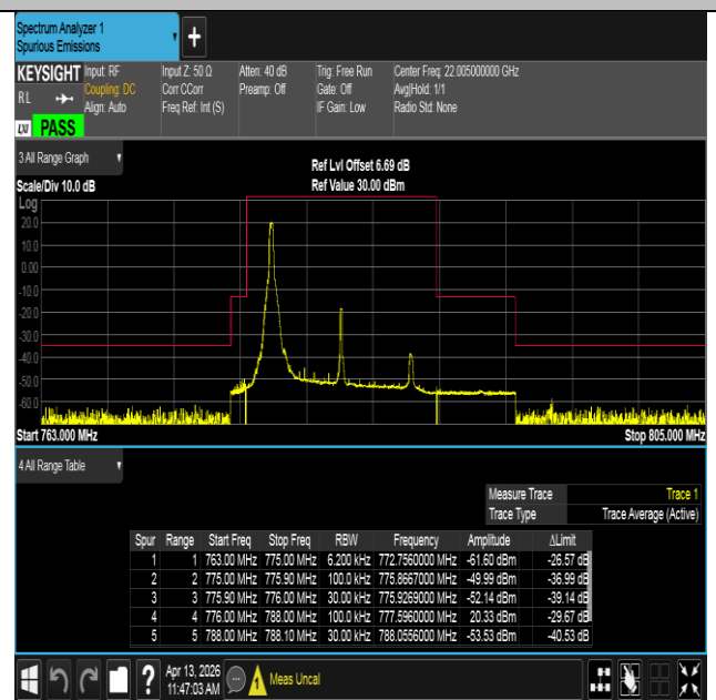
Band13-10MHz-16QAM-23230-1RB#0-PASS
