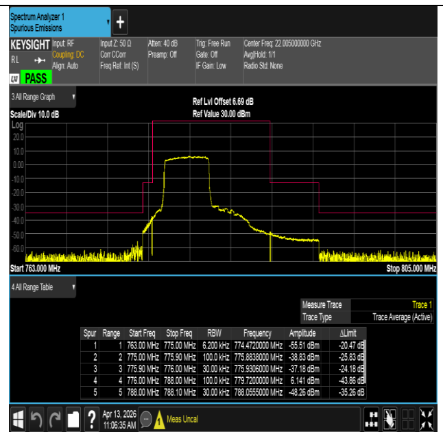
Band13-5MHz-16QAM-23205-25RB#0-PASS
