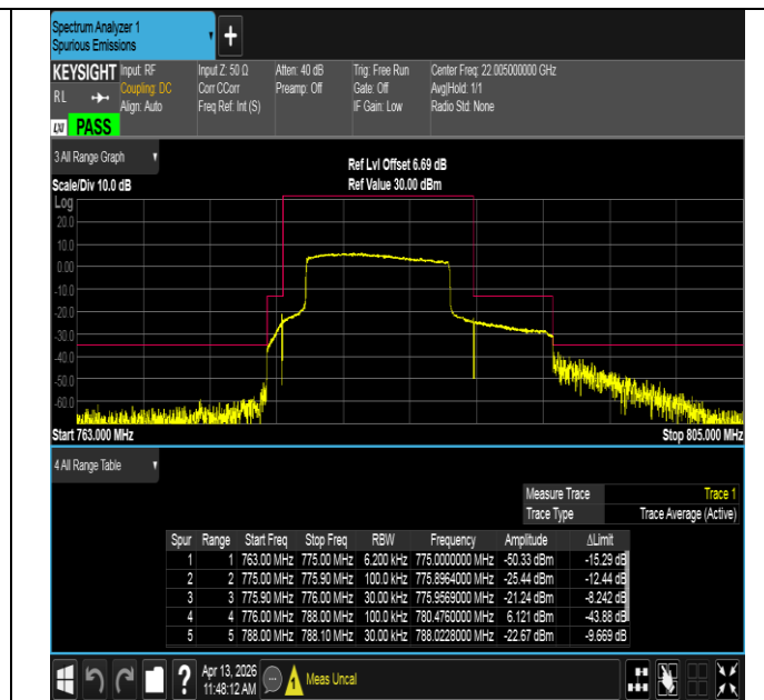
Band13-10MHz-16QAM-23230-50RB#0-PASS
