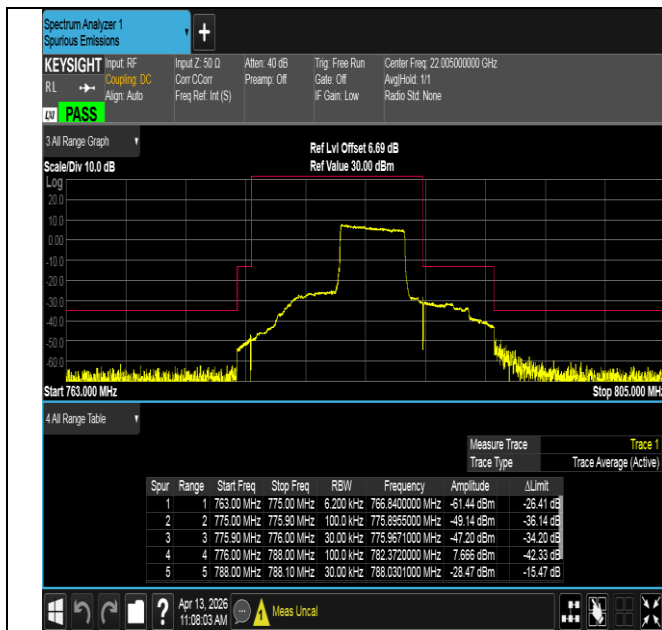
Band13-5MHz-QPSK-23255-25RB#0-PASS
