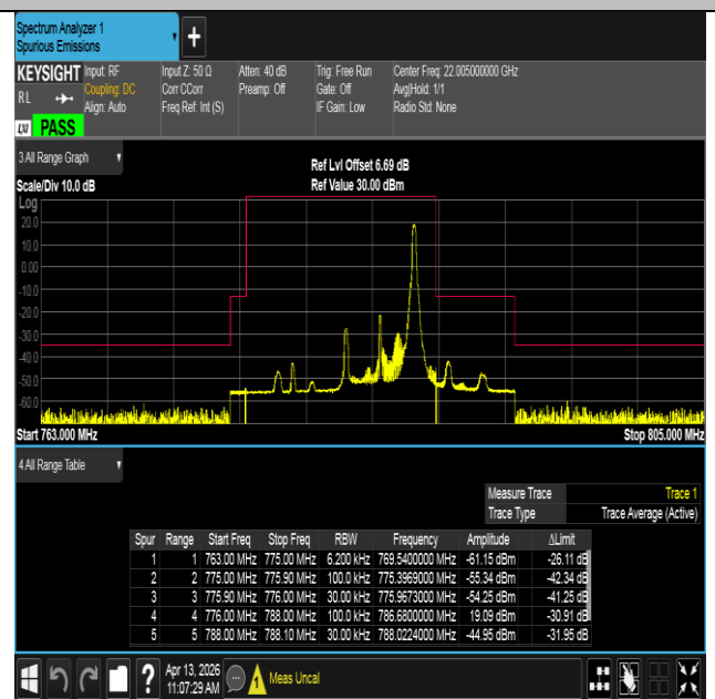
Band13-5MHz-QPSK-23255-1RB#24-PASS
