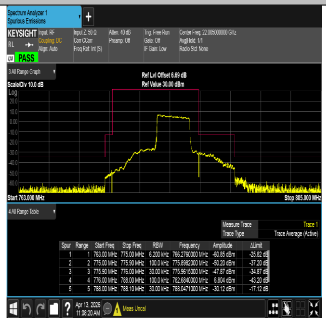
Band13-5MHz-16QAM-23255-25RB#0-PASS
