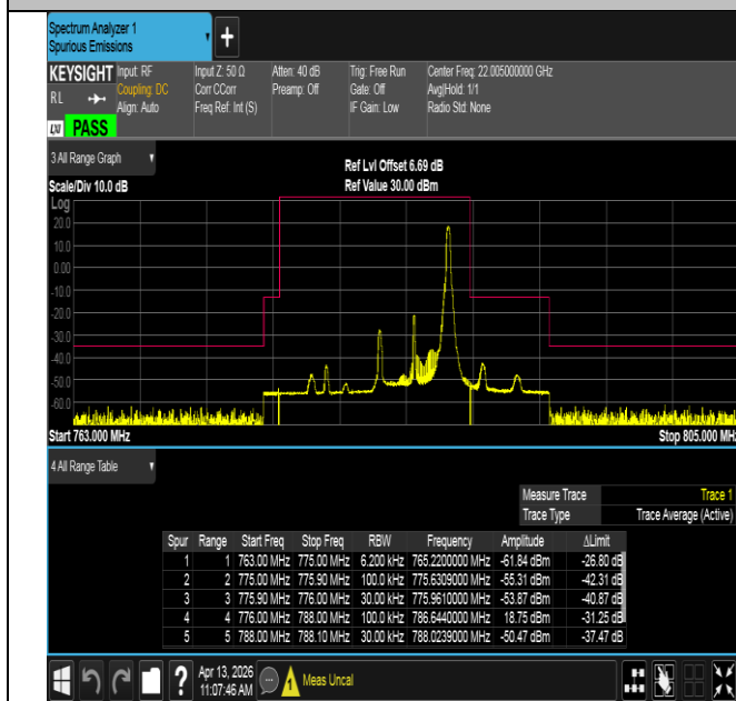
Band13-5MHz-16QAM-23255-1RB#24-PASS
