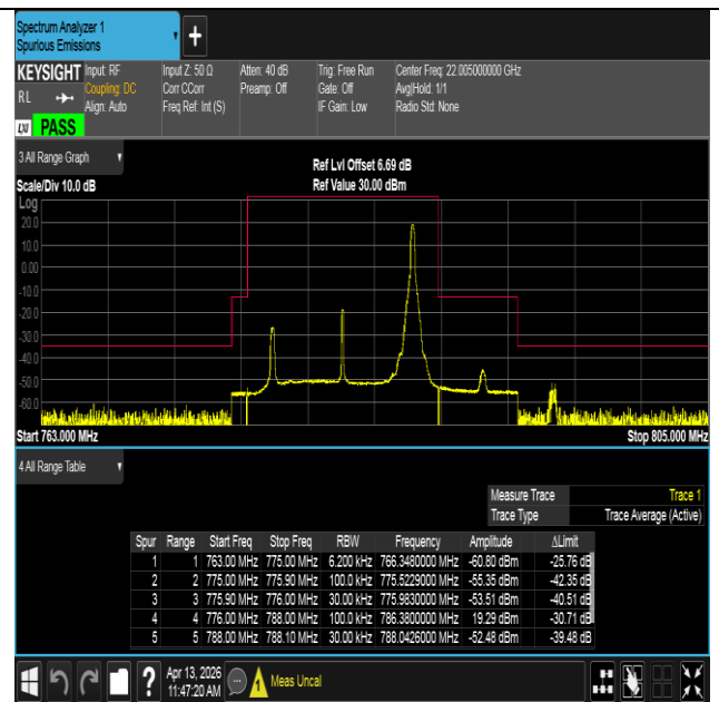
Band13-10MHz-QPSK-23230-1RB#49-PASS
