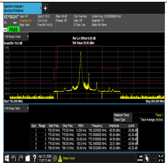
Band13-5MHz-16QAM-23255-1RB#0-PASS
