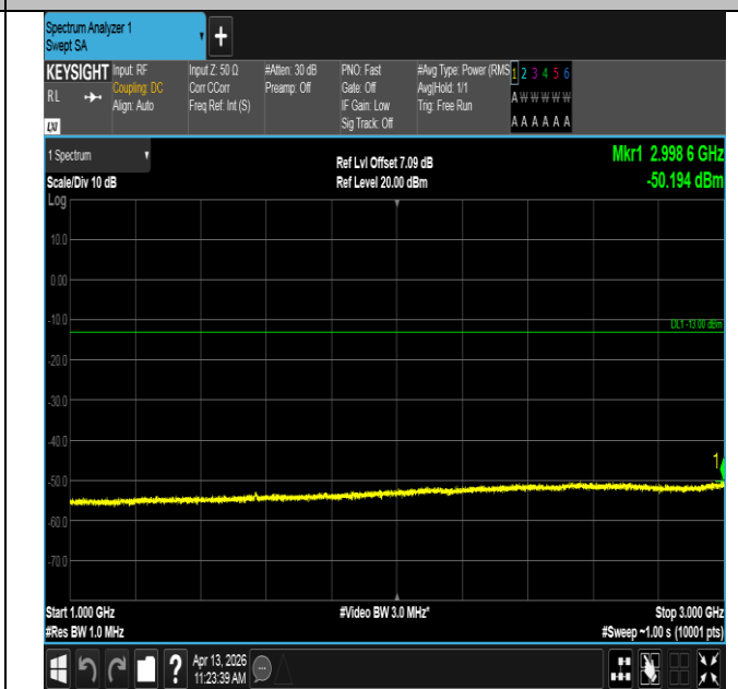
Band13-5MHz-QPSK-23255-25RB#0-1000~3000-PASS
