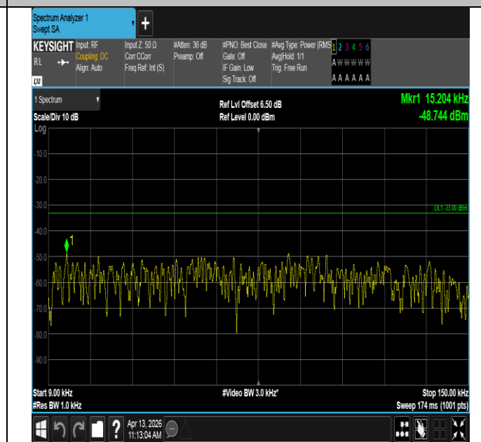
Band13-5MHz-16QAM-23205-25RB#0-0.009~0.15-PASS
