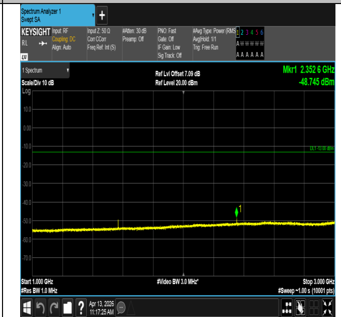
Band13-5MHz-16QAM-23230-1RB#24-1000~3000-PASS
