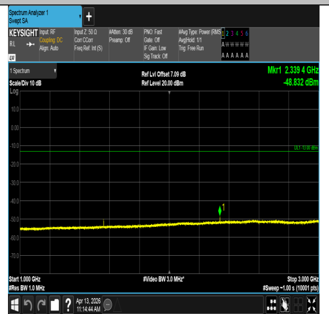
Band13-5MHz-QPSK-23230-1RB#0-1000~3000-PASS
