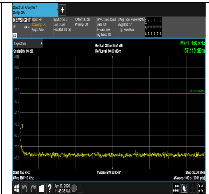
Band13-10MHz-QPSK-23230-1RB#0-0.15~30-PASS
