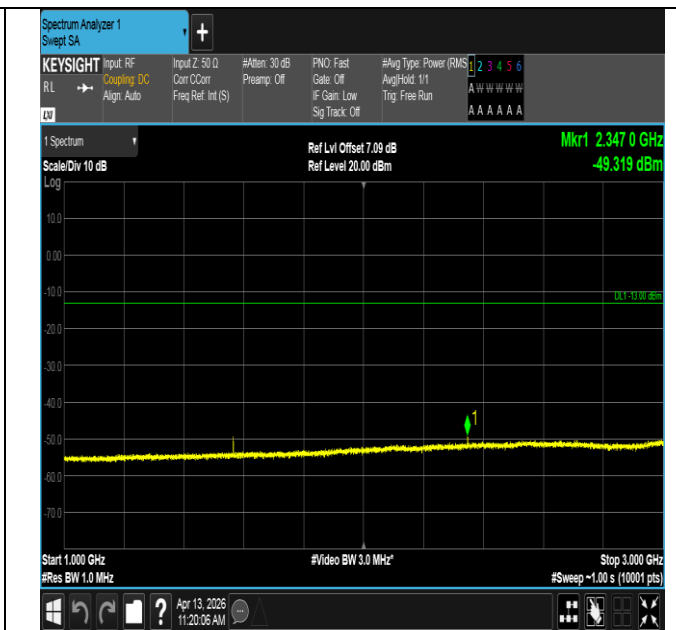
Band13-5MHz-QPSK-23255-1RB#0-1000~3000-PASS
