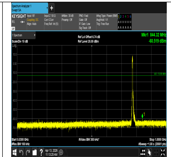
Band13-5MHz-16QAM-23205-25RB#0-30~1000-PASS
