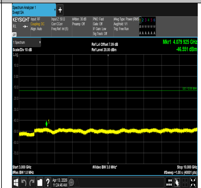
Band13-5MHz-16QAM-23255-25RB#0-3000~10000-PASS
