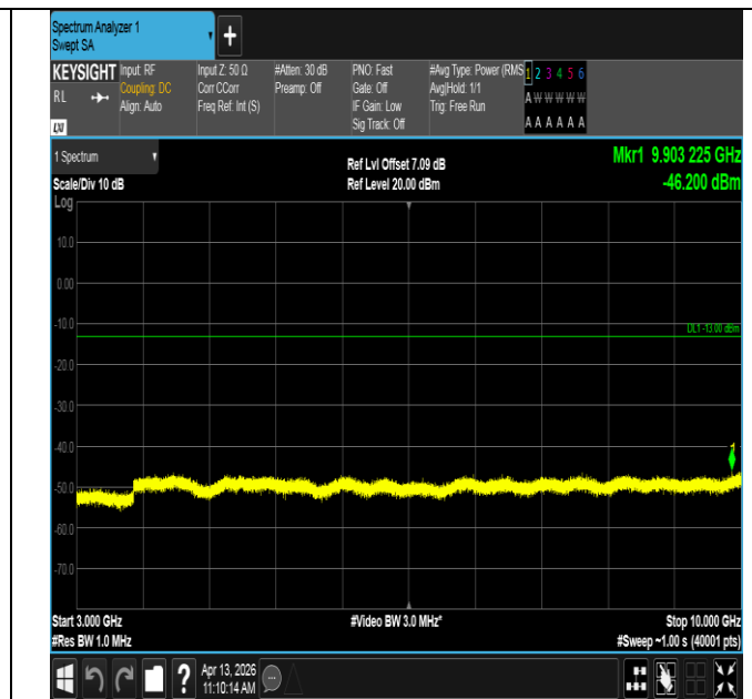
Band13-5MHz-16QAM-23205-1RB#0-3000~10000-PASS
