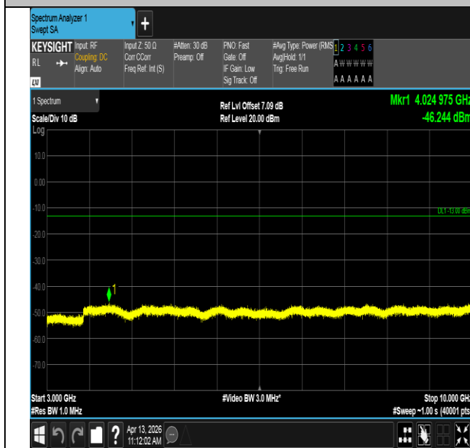
Band13-5MHz-16QAM-23205-1RB#24-3000~10000-PASS
