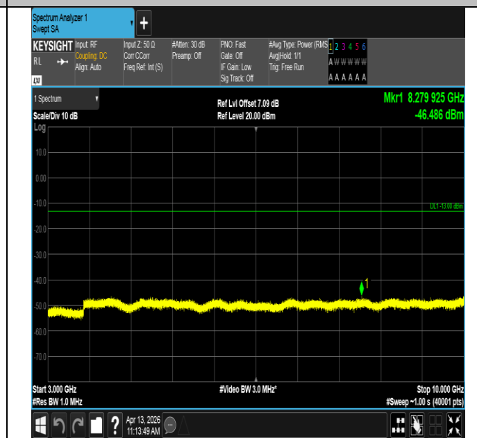
Band13-5MHz-16QAM-23205-25RB#0-3000~10000-PASS
