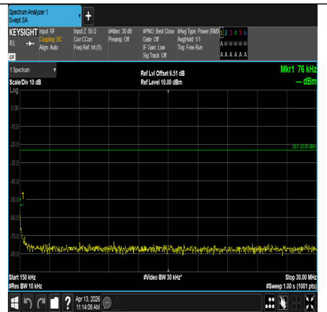
Band13-5MHz-QPSK-23230-1RB#0-0.15~30-PASS
