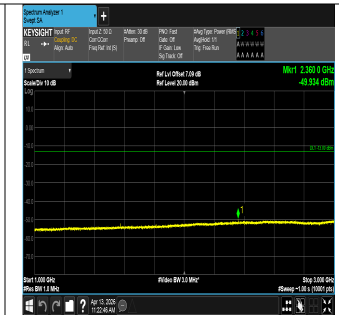
Band13-5MHz-16QAM-23255-1RB#24-1000~3000-PASS
