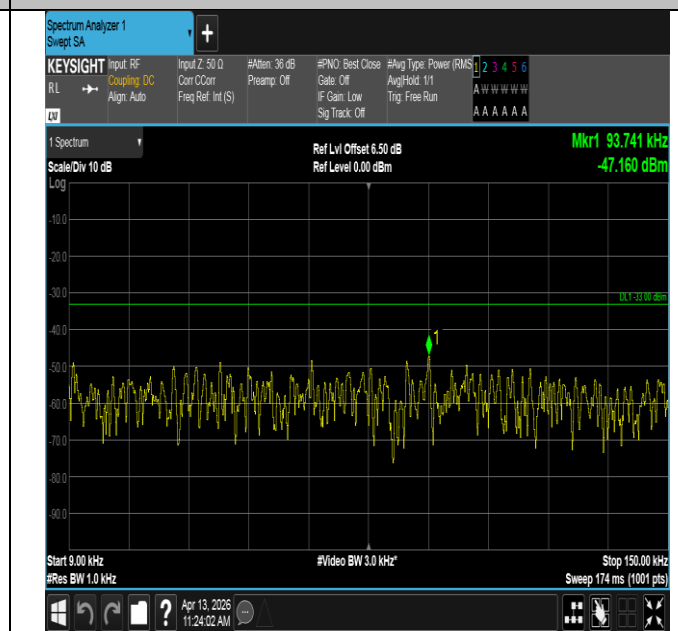
Band13-5MHz-16QAM-23255-25RB#0-0.009~0.15-PASS
