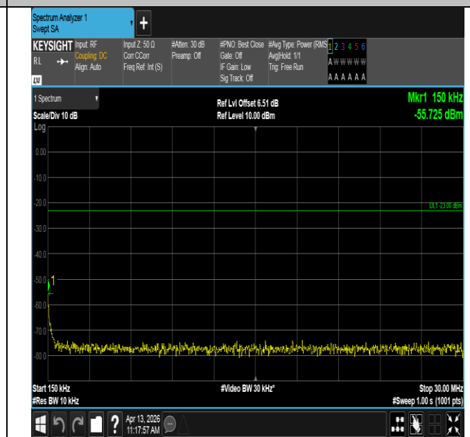
Band13-5MHz-QPSK-23230-25RB#0-0.15~30-PASS
