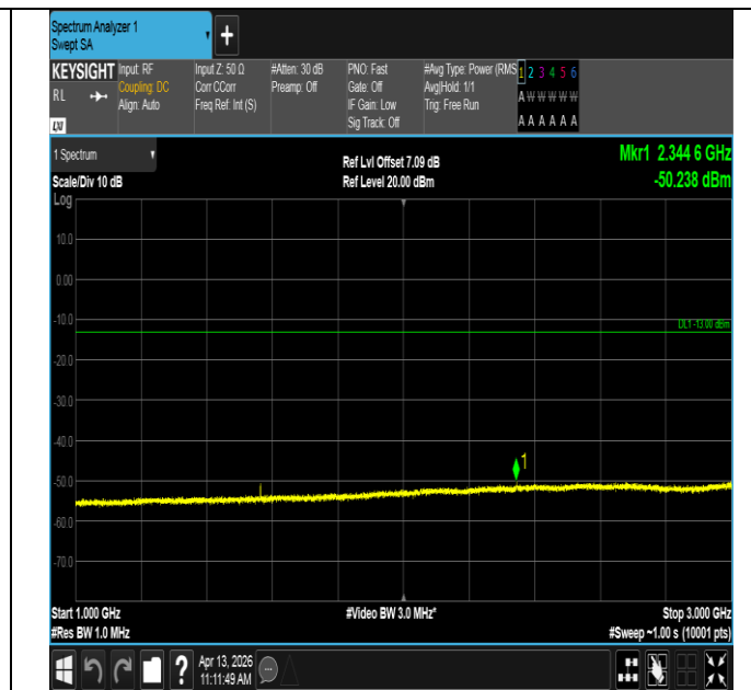
Band13-5MHz-16QAM-23205-1RB#24-1000~3000-PASS
