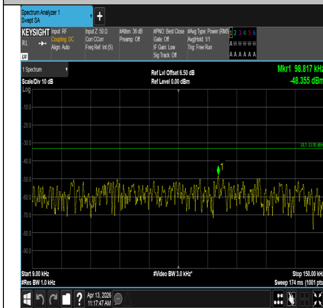
Band13-5MHz-QPSK-23230-25RB#0-0.009~0.15-PASS
