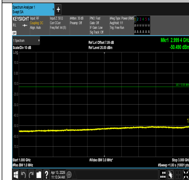
Band13-5MHz-16QAM-23205-25RB#0-1000~3000-PASS
