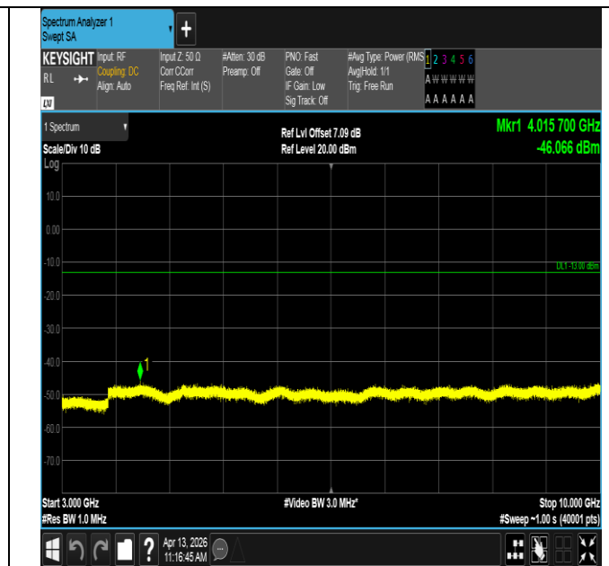
Band13-5MHz-QPSK-23230-1RB#24-3000~10000-PASS
