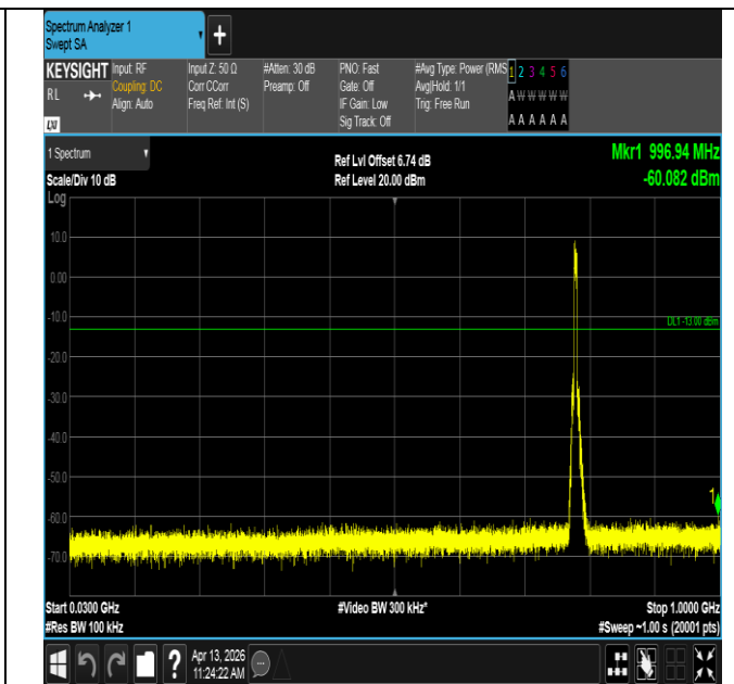
Band13-5MHz-16QAM-23255-25RB#0-30~1000-PASS
