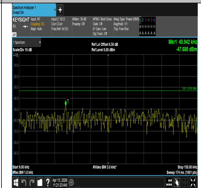
Band13-5MHz-QPSK-23255-1RB#24-0.009~0.15-PASS
