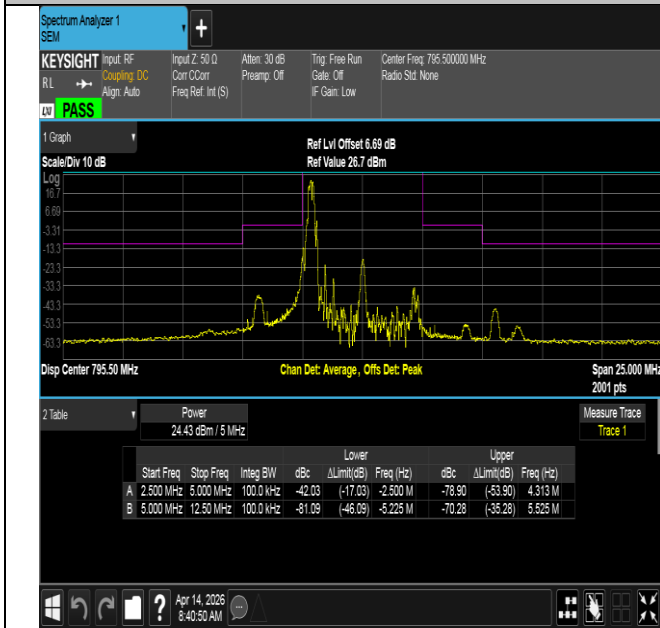
NTNV-Band14-5MHz-16QAM-23355-1RB#0-2.50-5.00-PASS
