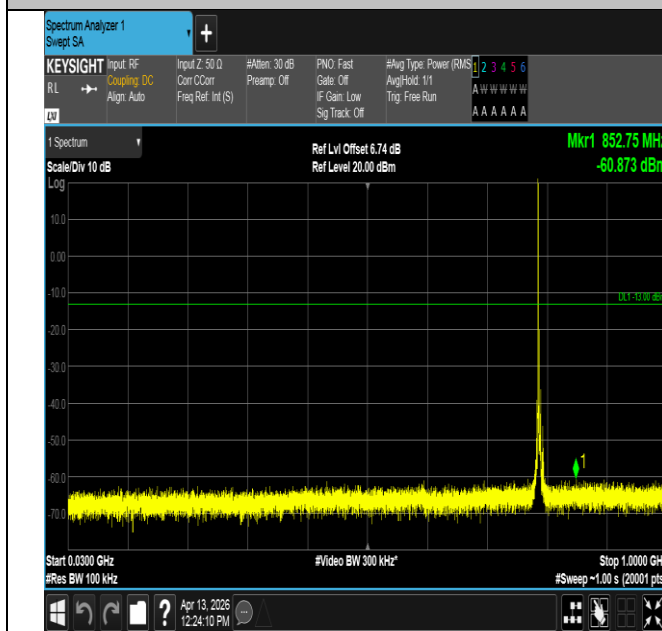
Band14-5MHz-QPSK-23330-1RB#0-30~1000-PASS
