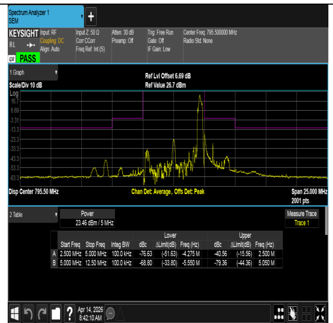
NTNV-Band14-5MHz-16QAM-23355-1RB#24--5.00--2.50-PASS
