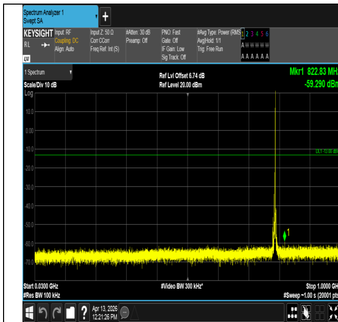
Band14-5MHz-16QAM-23305-1RB#24-30~1000-PASS
