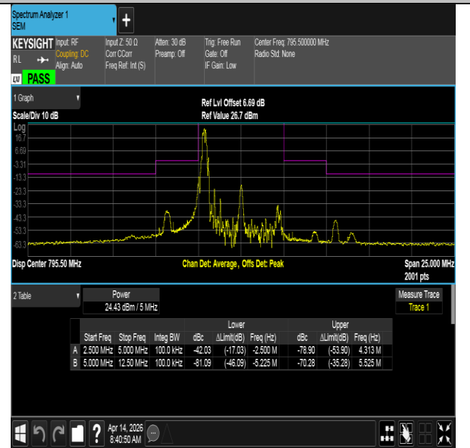
NTNV-Band14-5MHz-16QAM-23355-1RB#0-5.00-12.50-PASS
