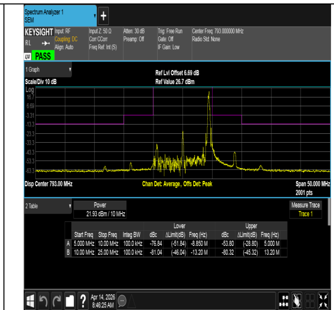
NTVN-Band14-10MHz-16QAM-23330-1RB#49--25.00--10.00-PASS
