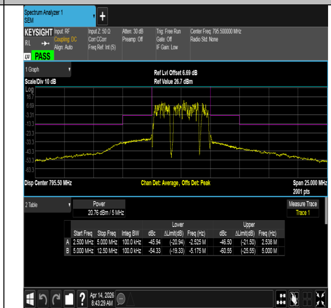
NTNV-Band14-5MHz-16QAM-23355-25RB#0-2.50-5.00-PASS
