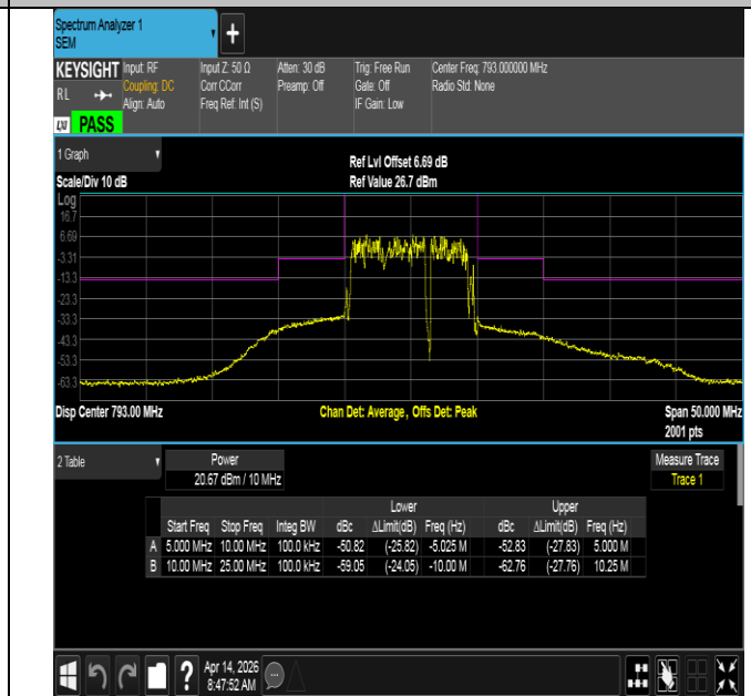
NTNV-Band14-10MHz-16QAM-23330-50RB#0--5.00-5.00-PASS
