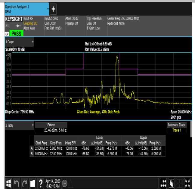
NTNV-Band14-5MHz-16QAM-23355-1RB#24-5.00-12.50-PASS
