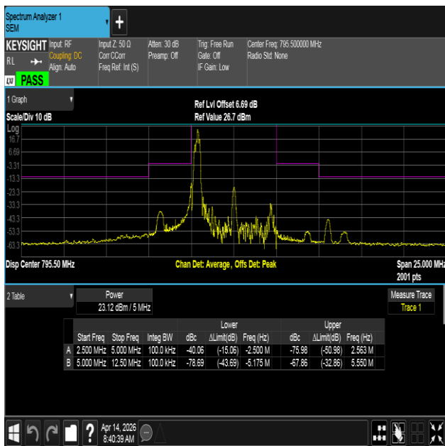
NTNV-Band14-5MHz-QPSK-23355-1RB#0-5.00-12.50-PASS
