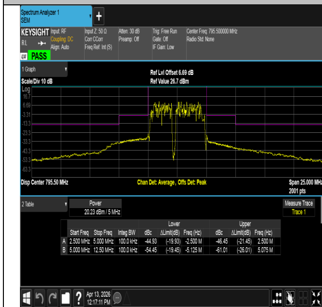
NTNV-Band14-5MHz-16QAM-23355-25RB#0--2.50-2.50-PASS
