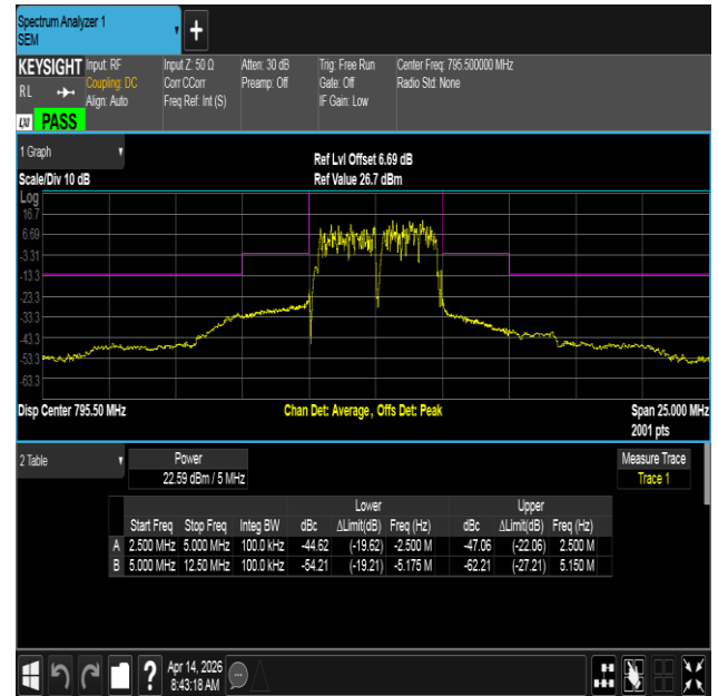
NTNV-Band14-5MHz-QPSK-23355-25RB#0--5.00--2.50-PASS
