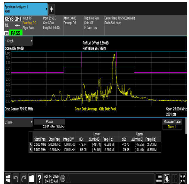
NTNV-Band14-5MHz-QPSK-23355-1RB#24--12.50--5.00-PASS
