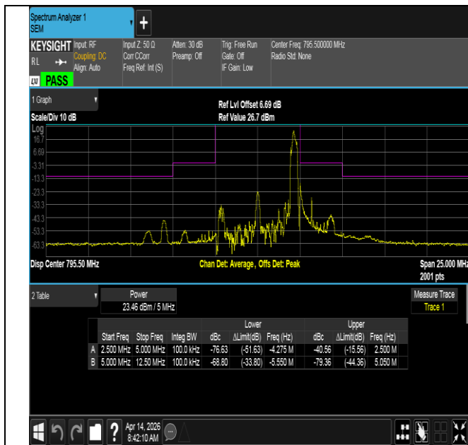
NTNV-Band14-5MHz-16QAM-23355-1RB#24--12.50--5.00-PASS
