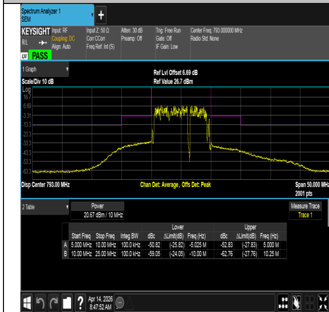
NTNV-Band14-10MHz-16QAM-23330-50RB#0--10.00--5.00-PASS
