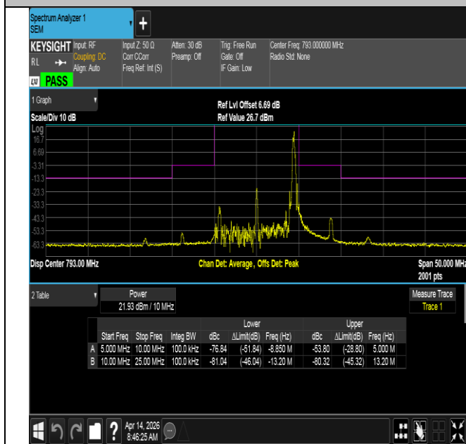
NTVN-Band14-10MHz-16QAM-23330-1RB#49--10.00--5.00-PASS
