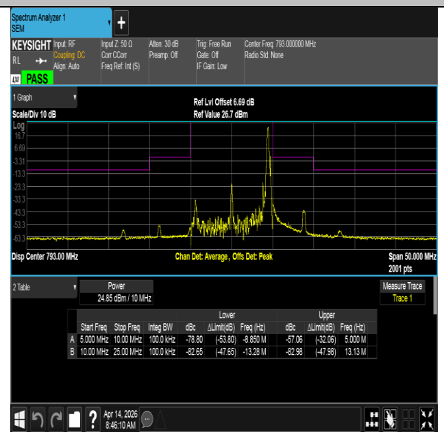
NTNV-Band14-10MHz-QPSK-23330-1RB#49-5.00-5.00-PASS
