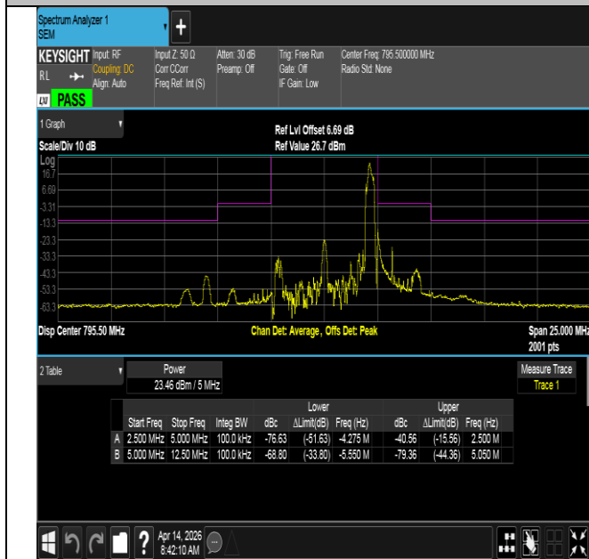
NTNV-Band14-5MHz-16QAM-23355-1RB#24--2.50-2.50-PASS
