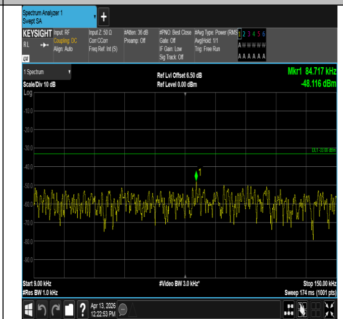
Band14-5MHz-16QAM-23305-25RB#0-0.009~0.15-PASS
