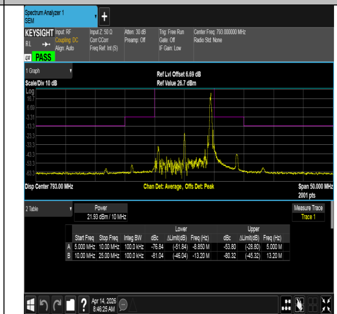
NTVN-Band14-10MHz-16QAM-23330-1RB#49--5.00-5.00-PASS
