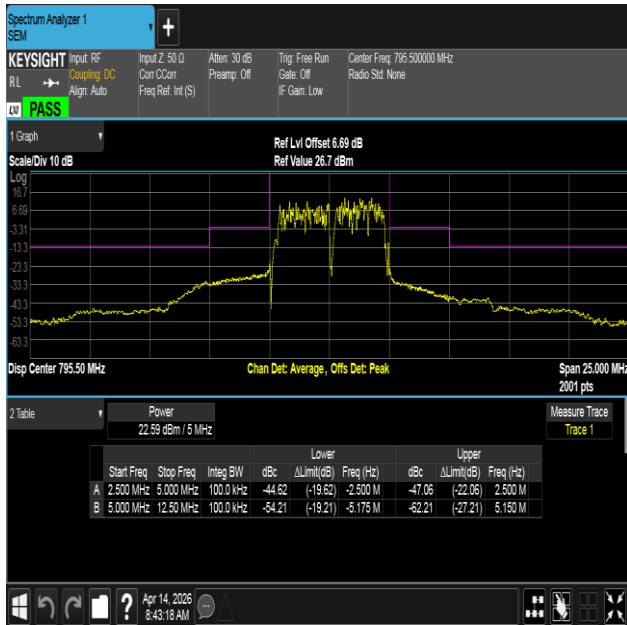
NTNV-Band14-5MHz-QPSK-23355-25RB#0--12.50--5.00-PASS
