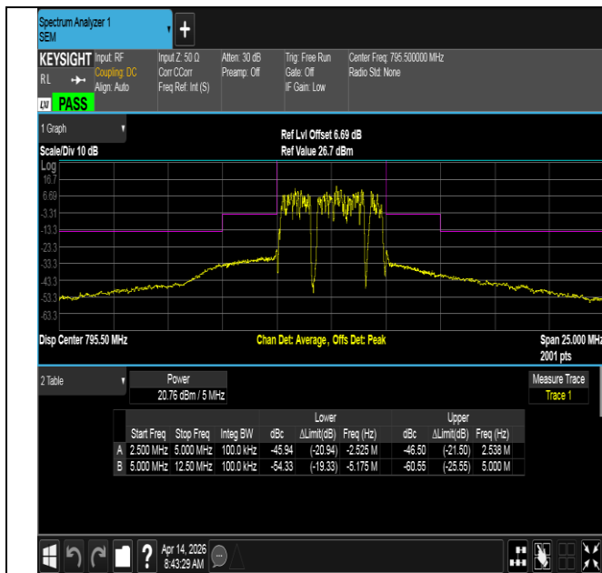
NTNV-Band14-5MHz-16QAM-23355-25RB#0--12.50--5.00-PASS
