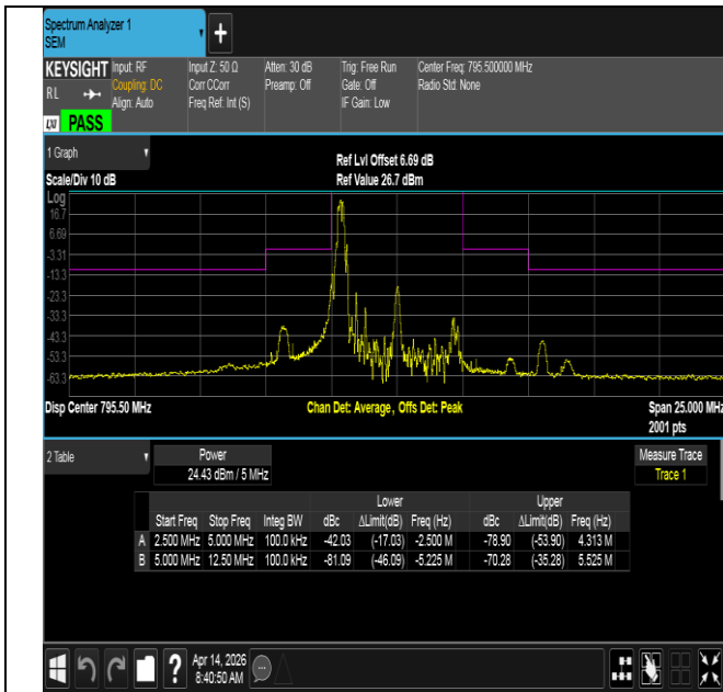
NTNV-Band14-5MHz-16QAM-23355-1RB#0--12.50--5.00-PASS
