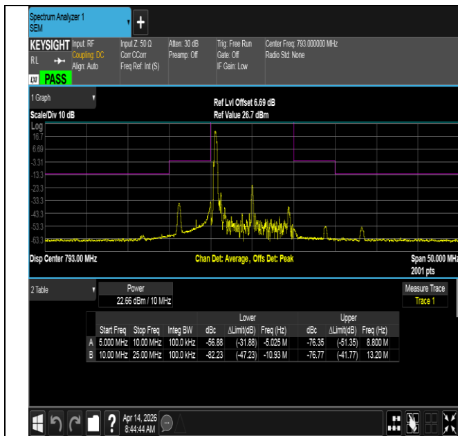
NTNV-Band14-10MHz-QPSK-23330-1RB#0-10.00-25.00-PASS
