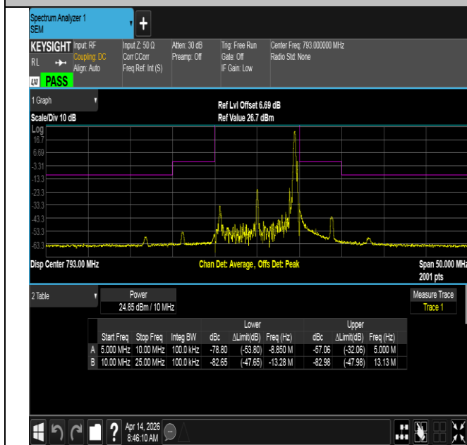
NTNV-Band14-10MHz-QPSK-23330-1RB#49-10.00-5.00-PASS
