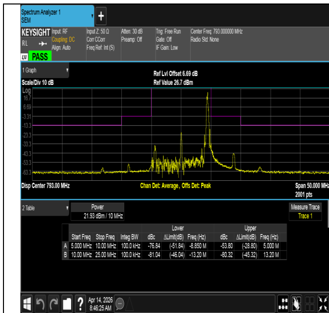
NTNV-Band14-10MHz-16QAM-23330-1RB#49-10.00-25.00-PASS
