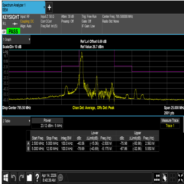
NTNV-Band14-5MHz-QPSK-23355-1RB#0--5.00--2.50-PASS
