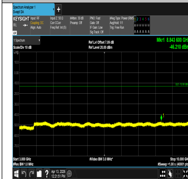
Band14-5MHz-16QAM-23305-1RB#24-3000~10000-PASS
