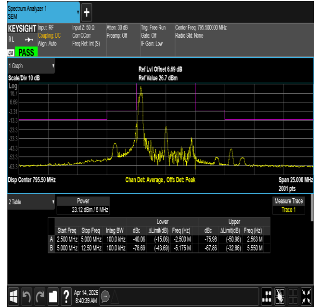
NTNV-Band14-5MHz-QPSK-23355-1RB#0-2.50-5.00-PASS
