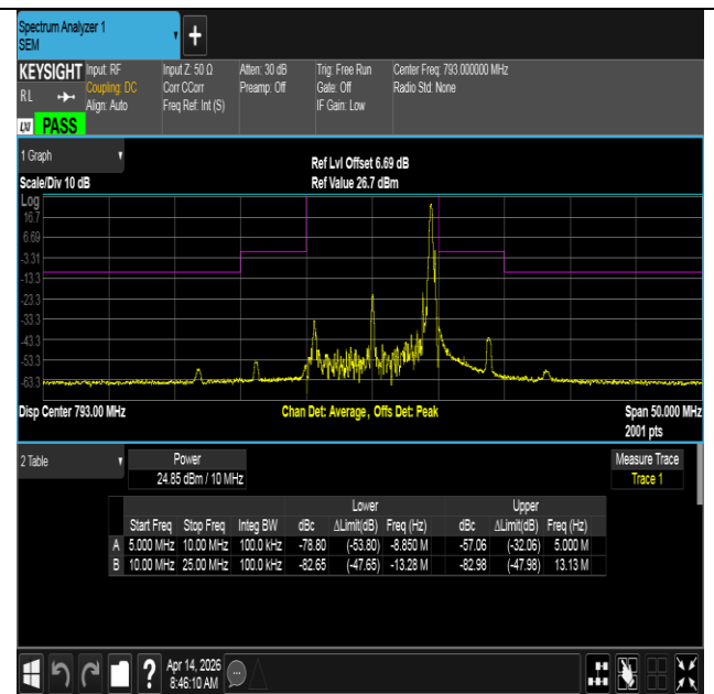
NTNV-Band14-10MHz-QPSK-23330-1RB#49-25.00-10.00-PASS
