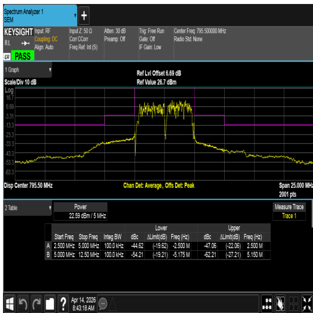
NTNV-Band14-5MHz-QPSK-23355-25RB#0--2.50-2.50-PASS
