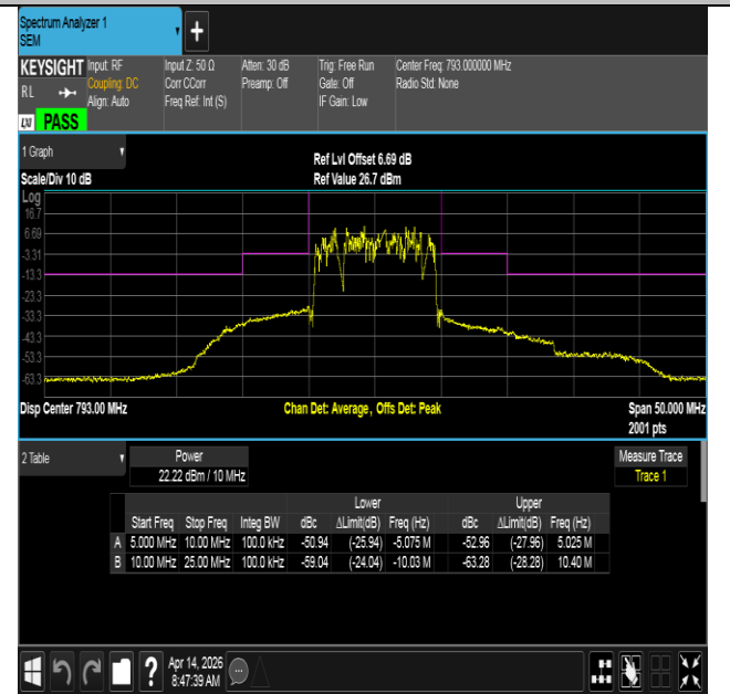
NTVN-Band14-10MHz-QPSK-23330-50RB#0-5.00-10.00-PASS
