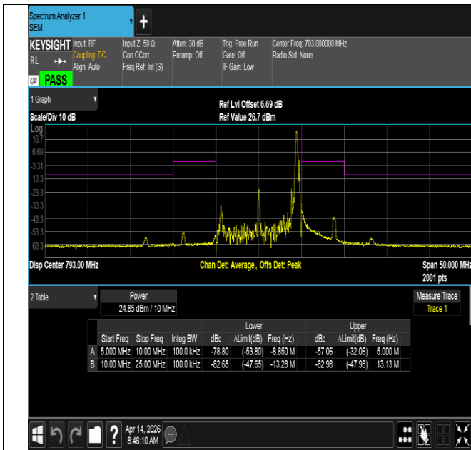
NTVN-Band14-10MHz-QPSK-23330-1RB#49-10.00-25.00-PASS
