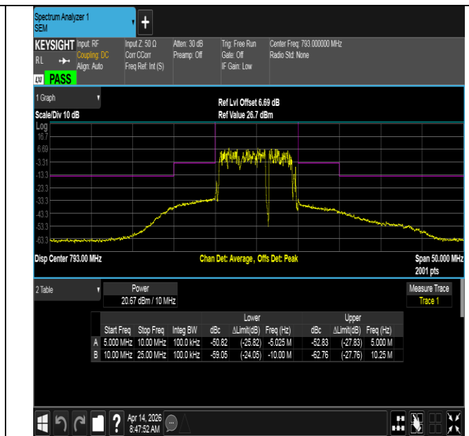
NTNV-Band14-10MHz-16QAM-23330-50RB#0--25.00--10.00-PASS
