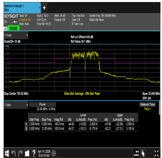
NTNV-Band14-5MHz-QPSK-23355-25RB#0-5.00-12.50-PASS
