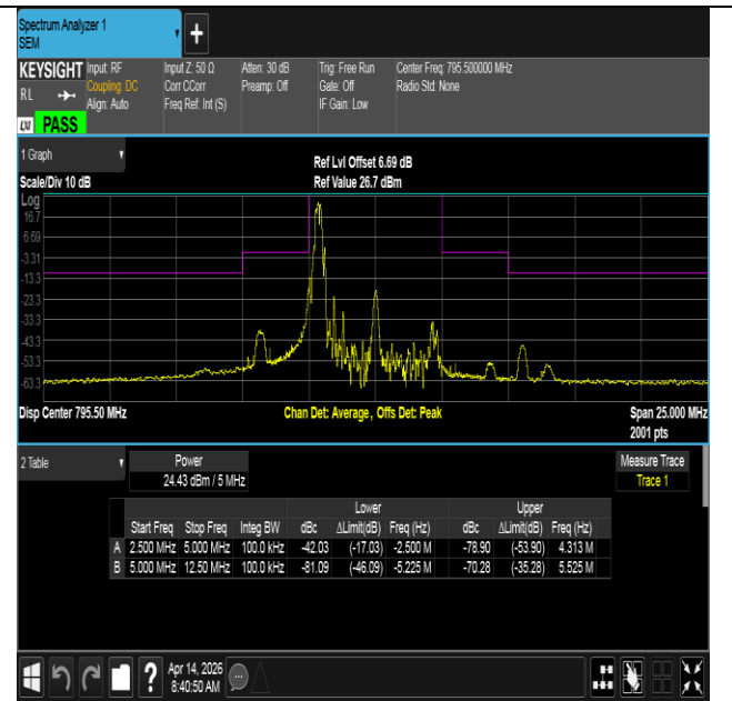
NTNV-Band14-5MHz-16QAM-23355-1RB#0--5.00--2.50-PASS
