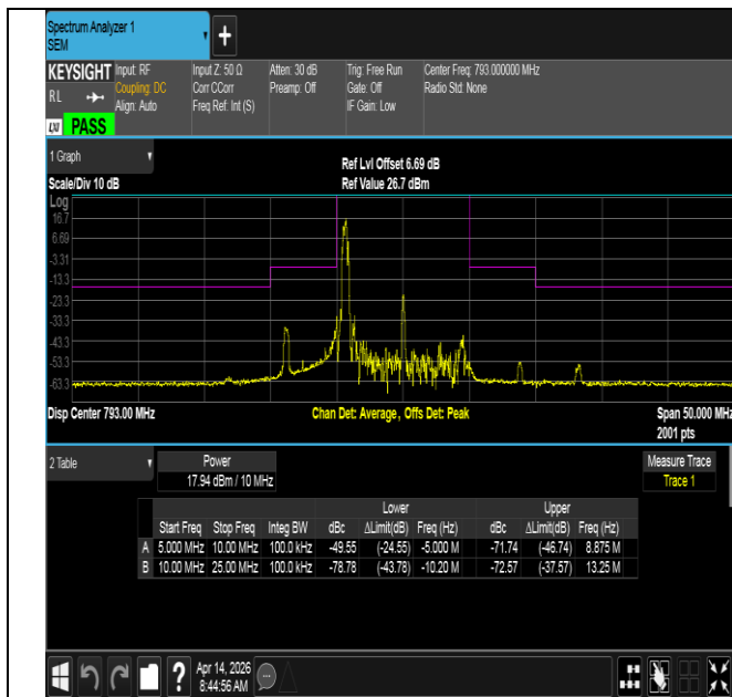
NTVN-Band14-10MHz-16QAM-23330-1RB#0-10.00-25.00-PASS
