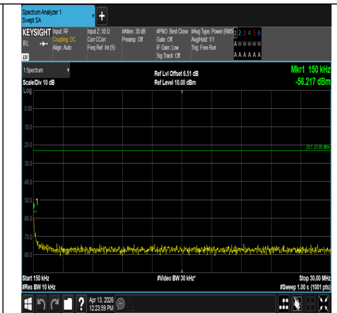
Band14-5MHz-QPSK-23330-1RB#0-0.15~30-PASS
