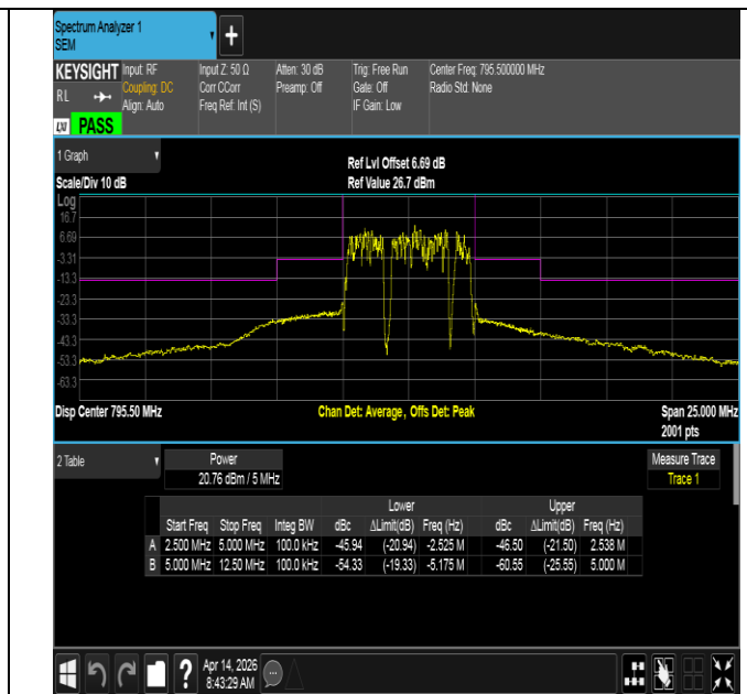
NTNV-Band14-5MHz-16QAM-23355-25RB#0--5.00--2.50-PASS
