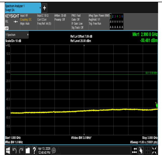
Band14-10MHz-QPSK-23330-50RB#0-1000~3000-PASS
