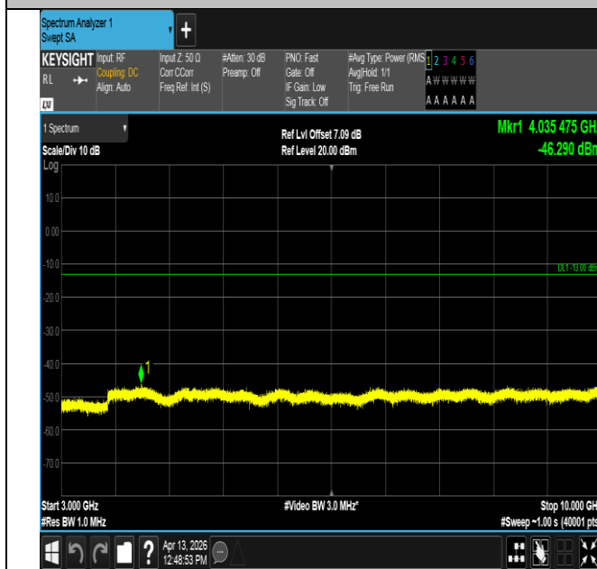
Band14-10MHz-QPSK-23330-50RB#0-3000~10000-PASS
