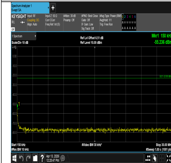
Band14-5MHz-QPSK-23330-1RB#24-0.15~30-PASS
