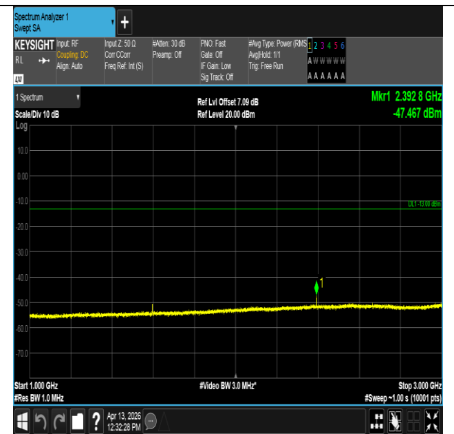
Band14-5MHz-16QAM-23355-1RB#24-1000~3000-PASS
