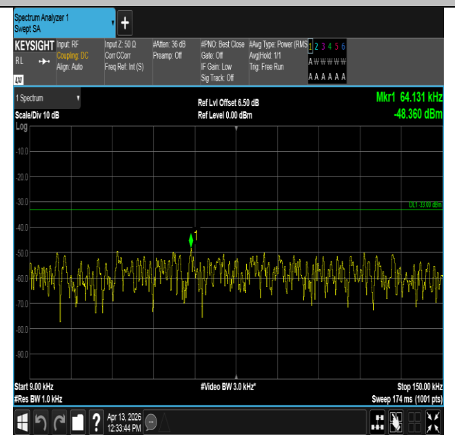
Band14-5MHz-16QAM-23355-25RB#0-0.009~0.15-PASS
