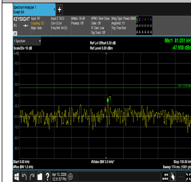
Band14-5MHz-16QAM-23355-1RB#24-0.009~0.15-PASS
