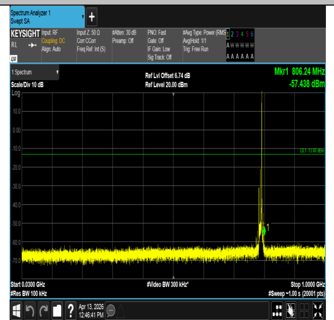
Band14-10MHz-QPSK-23330-1RB#49-30~1000-PASS
