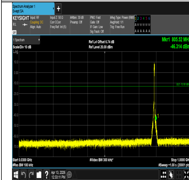
Band14-5MHz-QPSK-23355-25RB#0-30~1000-PASS
