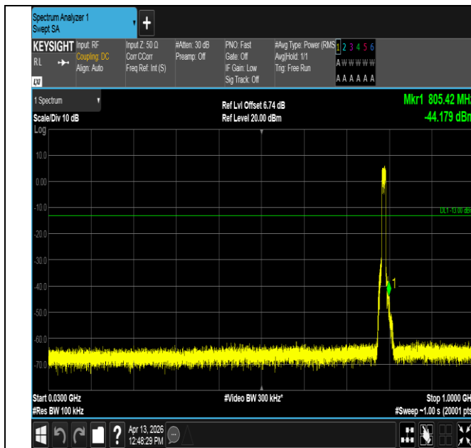
Band14-10MHz-QPSK-23330-50RB#0-30~1000-PASS
