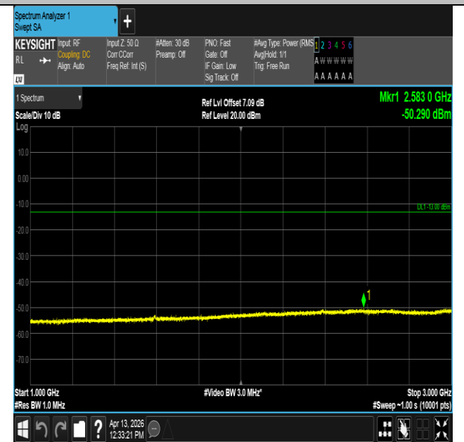
Band14-5MHz-QPSK-23355-25RB#0-1000~3000-PASS
