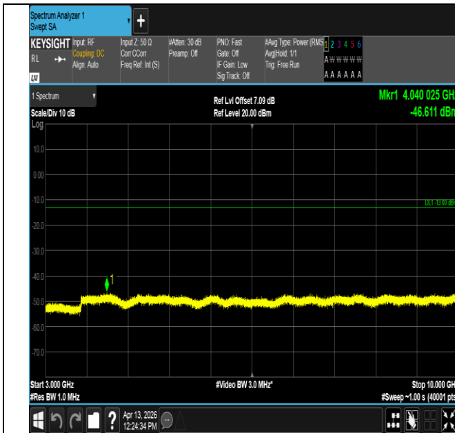
Band14-5MHz-QPSK-23330-1RB#0-3000~10000-PASS
