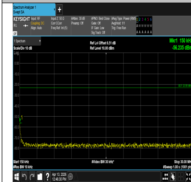
Band14-10MHz-QPSK-23330-1RB#49-0.15~30-PASS
