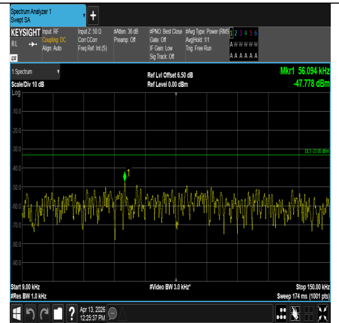
Band14-5MHz-QPSK-23330-1RB#24-0.009~0.15-PASS
