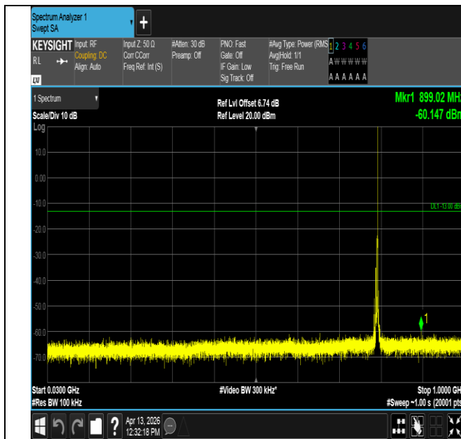
Band14-5MHz-16QAM-23355-1RB#24-30~1000-PASS
