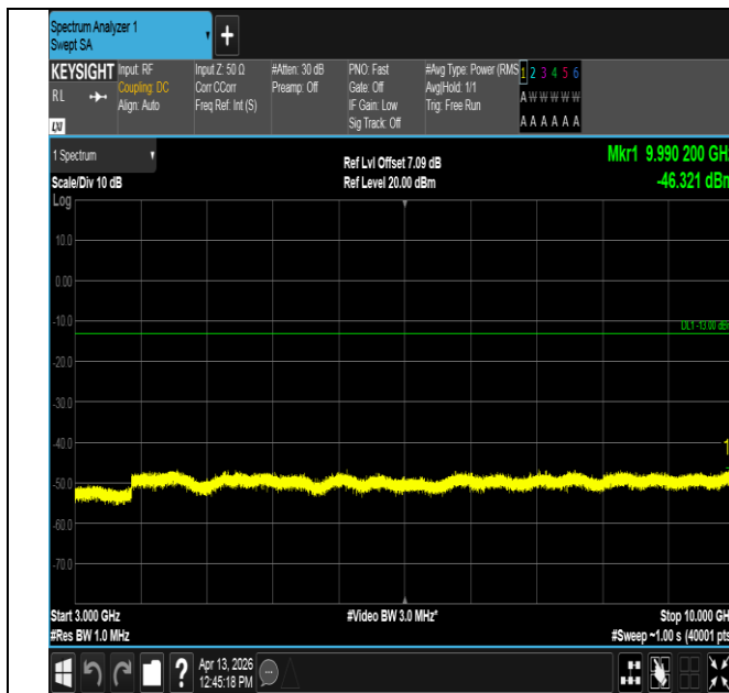
Band14-10MHz-QPSK-23330-1RB#0-3000~10000-PASS
