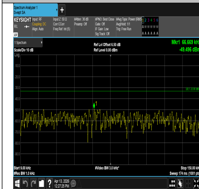
Band14-5MHz-QPSK-23330-25RB#0-0.009~0.15-PASS
