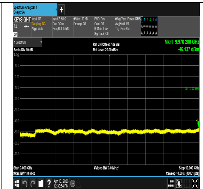
Band14-5MHz-16QAM-23355-1RB#0-3000~10000-PASS
