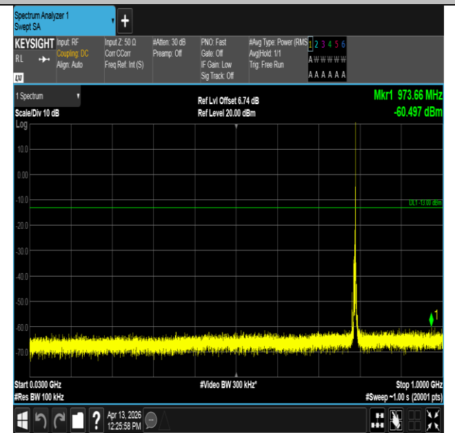
Band14-5MHz-QPSK-23330-1RB#24-30~1000-PASS
