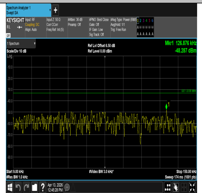
Band14-10MHz-16QAM-23330-1RB#0-0.009~0.15-PASS
