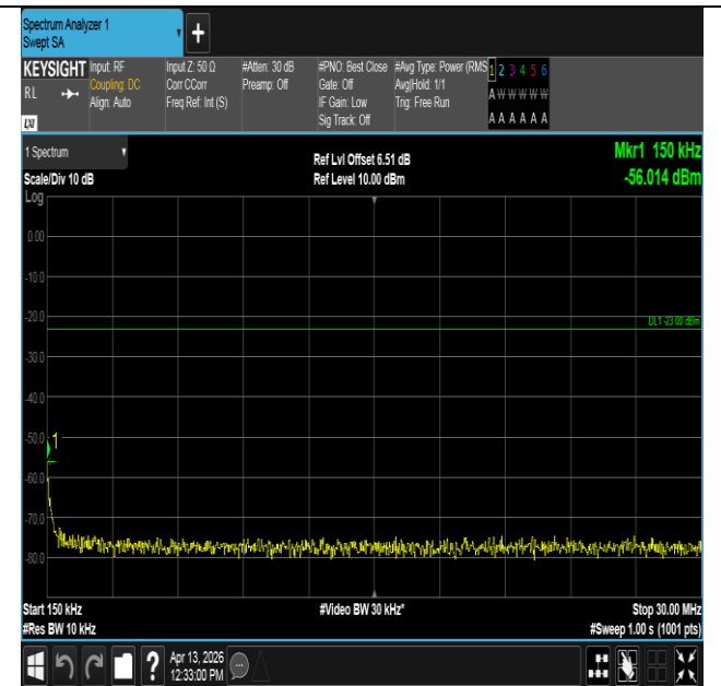
Band14-5MHz-QPSK-23355-25RB#0-0.15~30-PASS
