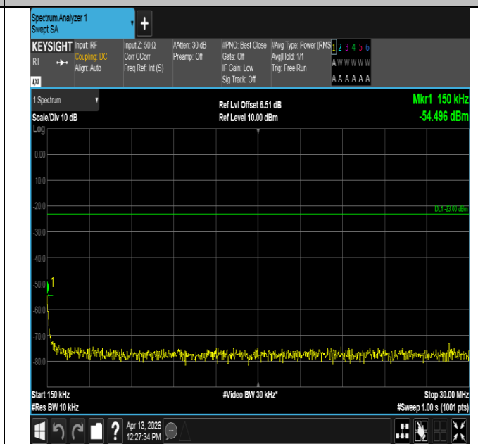
Band14-5MHz-QPSK-23330-25RB#0-0.15~30-PASS
