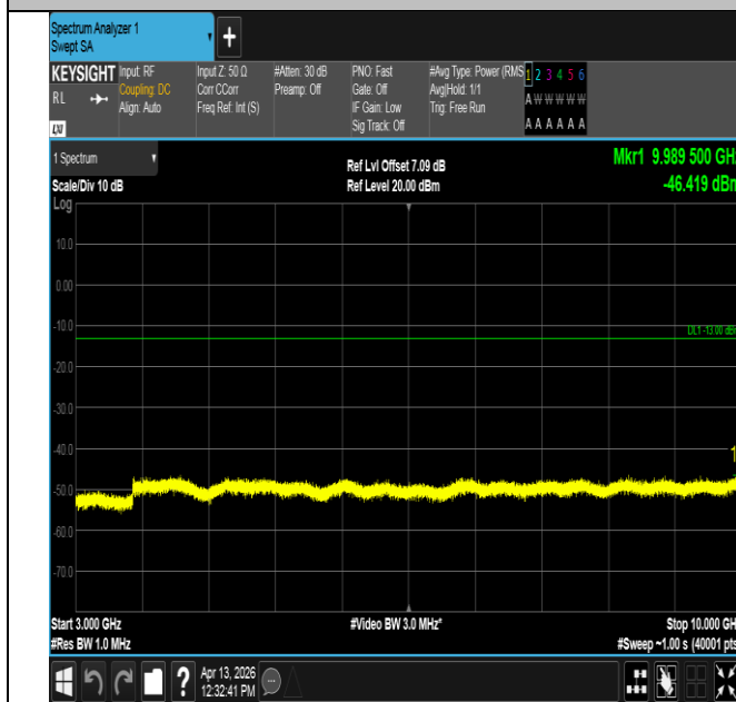
Band14-5MHz-16QAM-23355-1RB#24-3000~10000-PASS
