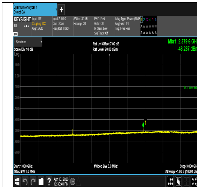
Band14-5MHz-16QAM-23355-1RB#0-1000~3000-PASS
