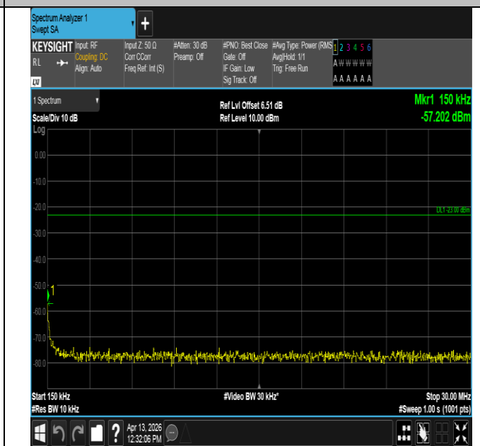
Band14-5MHz-16QAM-23355-1RB#24-0.15~30-PASS
