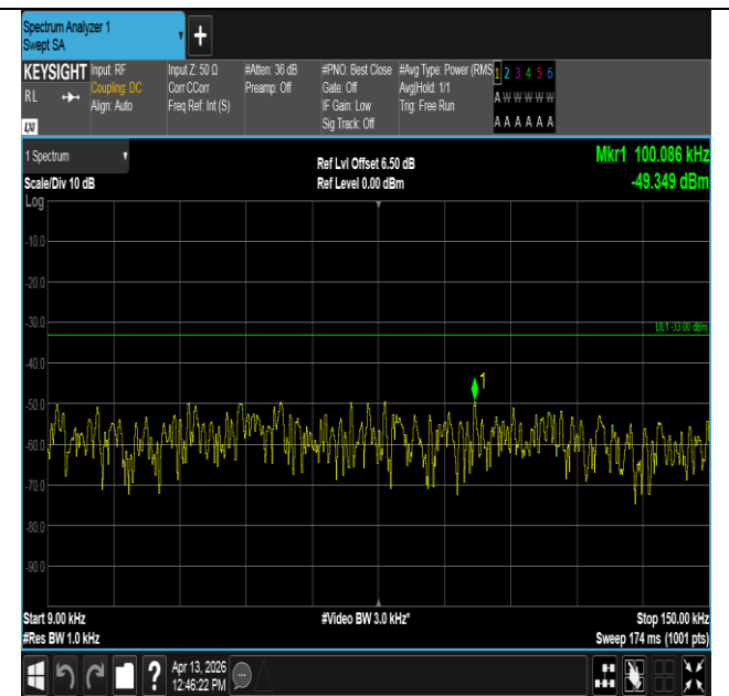
Band14-10MHz-QPSK-23330-1RB#49-0.009~0.15-PASS
