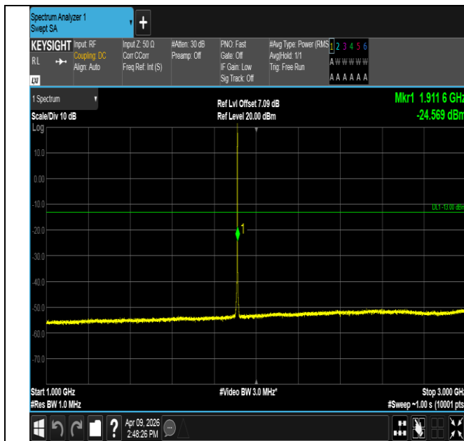
Band2-1.4MHz-QPSK-19193-1RB#5-1000~3000-PASS
