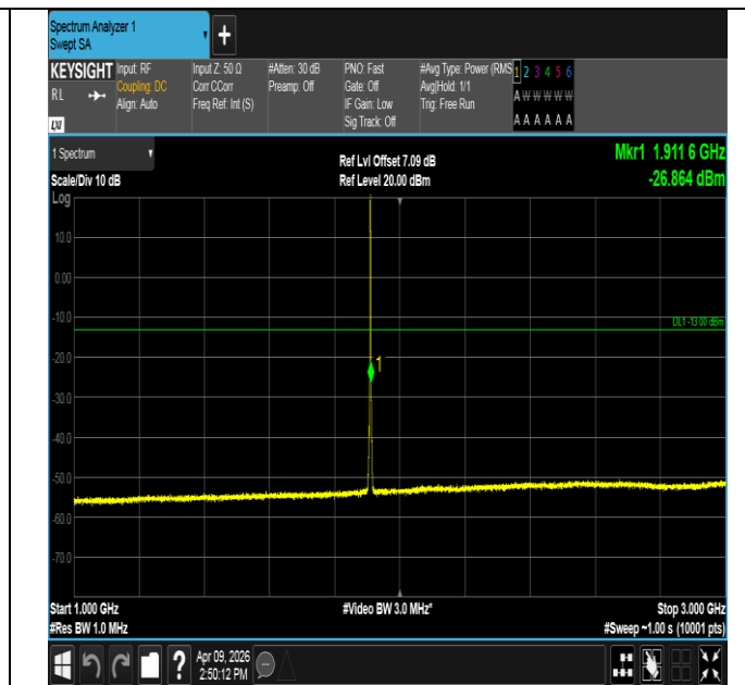
Band2-1.4MHz-QPSK-19193-6RB#0-1000~3000-PASS
