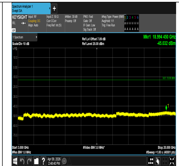
Band2-1.4MHz-QPSK-19193-1RB#5-3000~20000-PASS
