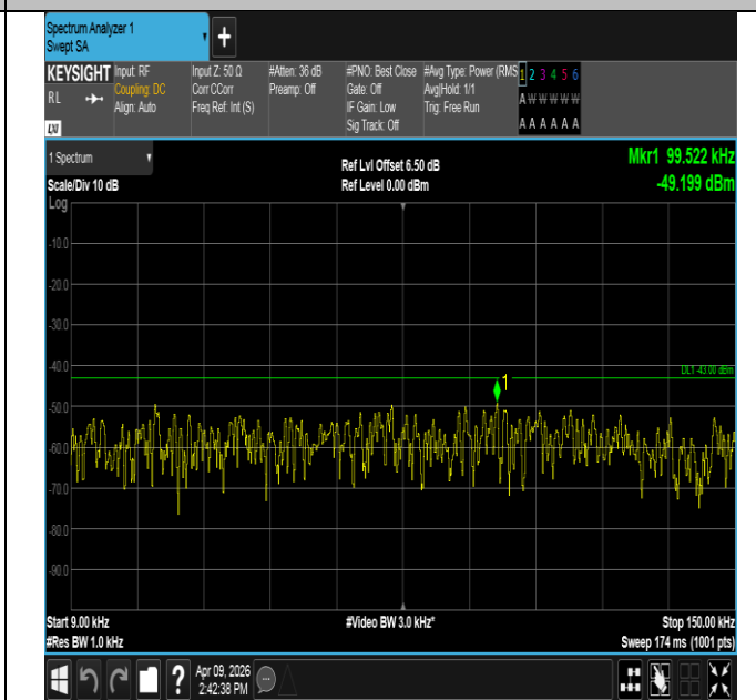
Band2-1.4MHz-QPSK-18900-1RB#5-0.009~0.15-PASS
