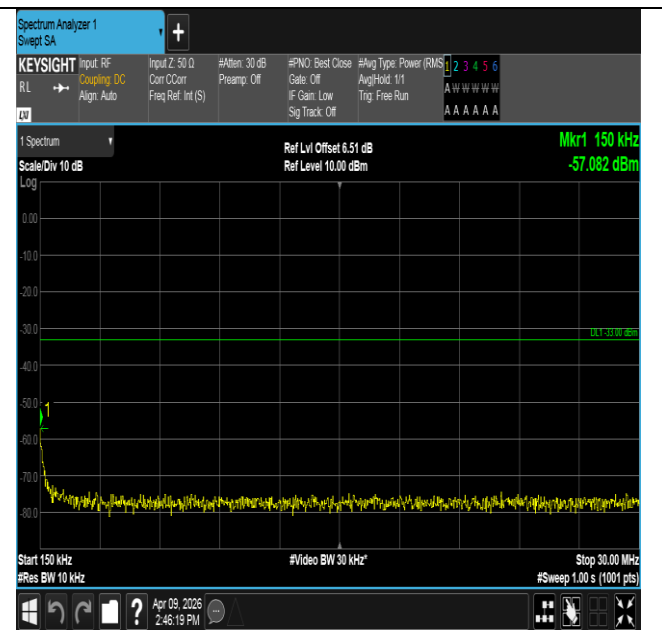
Band2-1.4MHz-QPSK-19193-1RB#0-0.15~30-PASS
