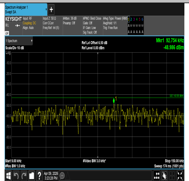
Band2-3MHz-QPSK-18615-1RB#14-0.009~0.15-PASS
