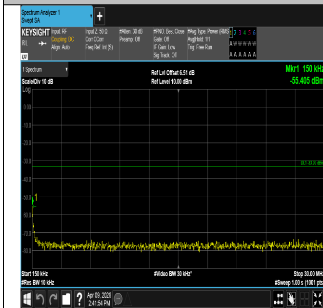
Band2-1.4MHz-16QAM-18900-1RB#0-0.15~30-PASS
