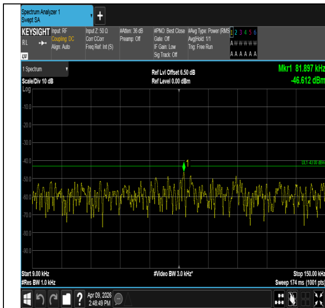
Band2-1.4MHz-16QAM-19193-1RB#5-0.009~0.15-PASS
