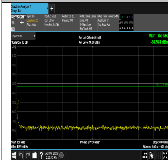
Band2-1.4MHz-16QAM-19193-6RB#0-0.15~30-PASS
