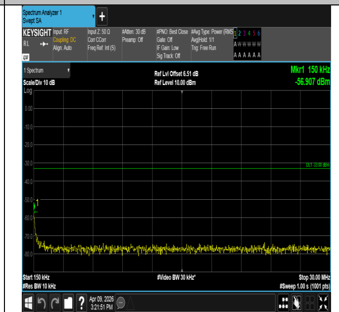
Band2-3MHz-QPSK-18615-1RB#0-0.15~30-PASS
