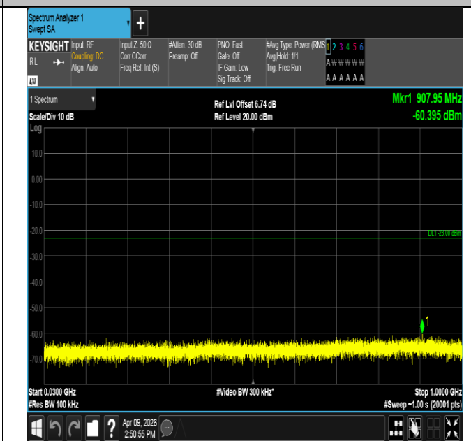
Band2-1.4MHz-16QAM-19193-6RB#0-30~1000-PASS
