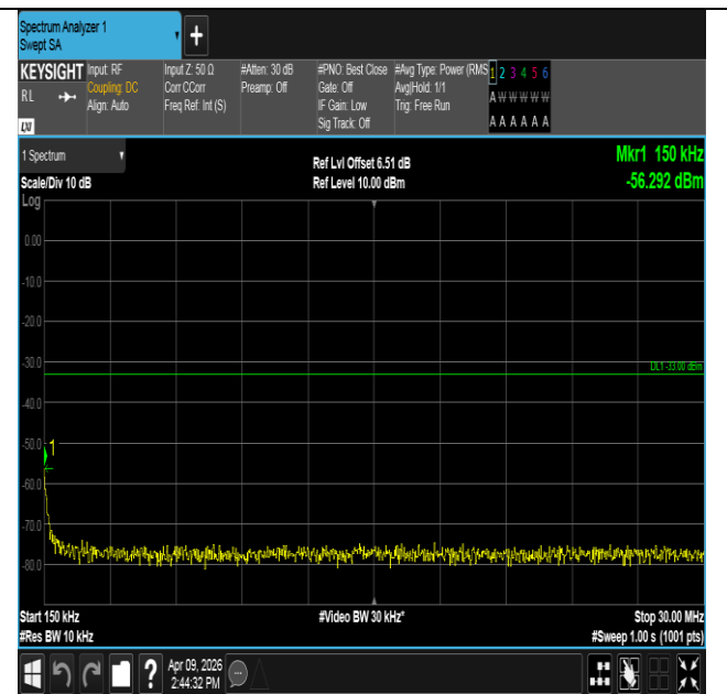
Band2-1.4MHz-QPSK-18900-6RB#0-0.15~30-PASS
