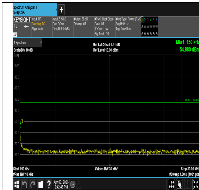
Band2-1.4MHz-QPSK-18900-1RB#5-0.15~30-PASS
