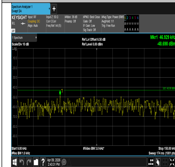
Band2-1.4MHz-16QAM-18900-1RB#5-0.009~0.15-PASS
