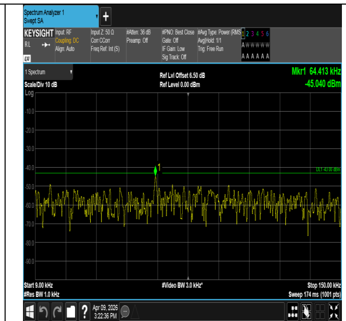
Band2-3MHz-16QAM-18615-1RB#0-0.009~0.15-PASS
