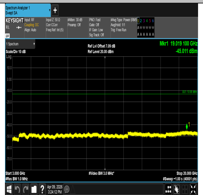
Band2-3MHz-QPSK-18615-1RB#14-3000~20000-PASS
