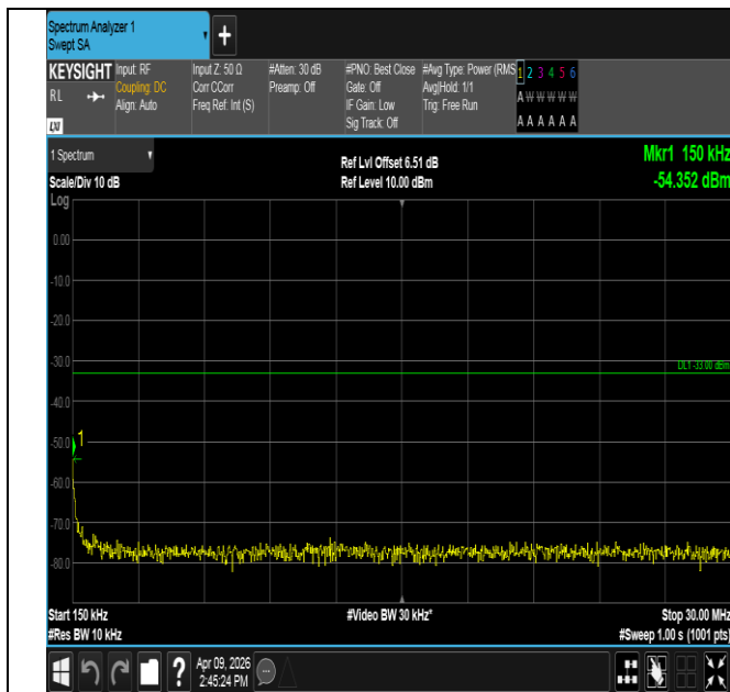
Band2-1.4MHz-16QAM-18900-6RB#0-0.15~30-PASS
