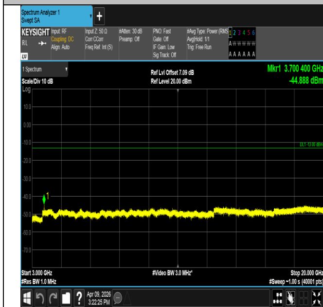
Band2-3MHz-QPSK-18615-1RB#0-3000~20000-PASS
