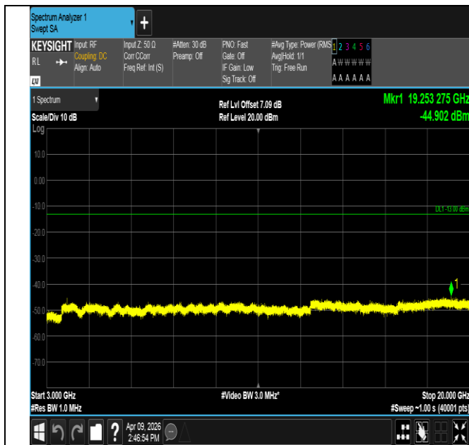
Band2-1.4MHz-QPSK-19193-1RB#0-3000~20000-PASS
