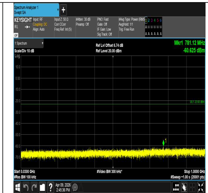
Band2-1.4MHz-16QAM-18900-6RB#0-30~1000-PASS
