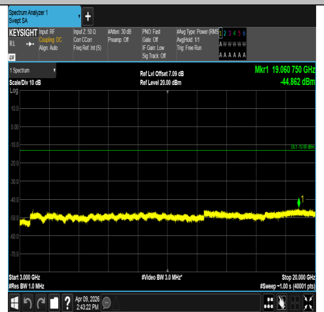
Band2-1.4MHz-QPSK-18900-1RB#5-3000~20000-PASS
