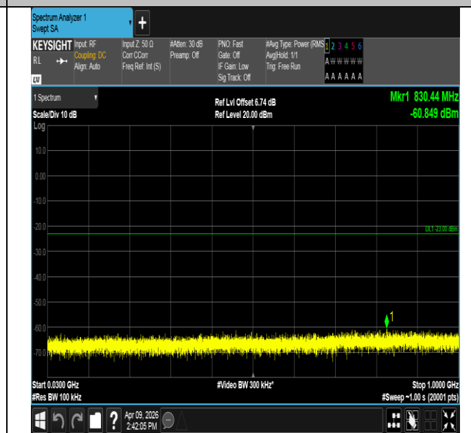
Band2-1.4MHz-16QAM-18900-1RB#0-30~1000-PASS
