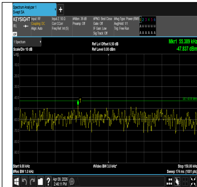
Band2-1.4MHz-QPSK-19193-1RB#0-0.009~0.15-PASS
