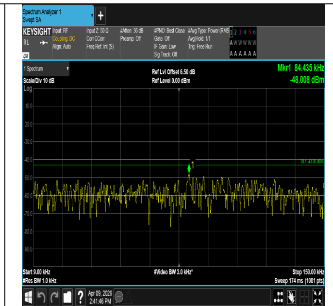
Band2-1.4MHz-16QAM-18900-1RB#0-0.009~0.15-PASS
