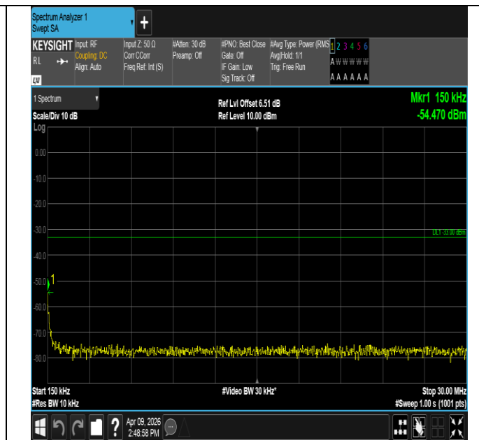
Band2-1.4MHz-16QAM-19193-1RB#5-0.15~30-PASS
