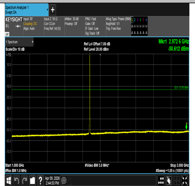
Band2-1.4MHz-QPSK-18900-6RB#0-1000~3000-PASS
