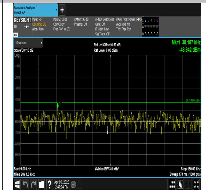
Band2-1.4MHz-16QAM-19193-1RB#0-0.009~0.15-PASS
