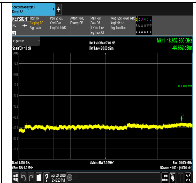
Band2-1.4MHz-16QAM-18900-1RB#0-3000~20000-PASS
