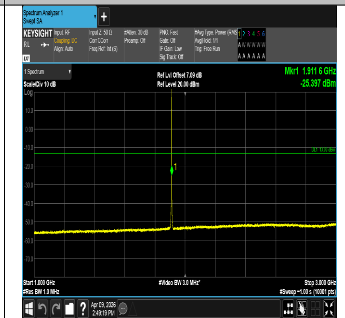
Band2-1.4MHz-16QAM-19193-1RB#5-1000~3000-PASS
