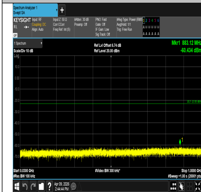
Band2-1.4MHz-QPSK-18900-6RB#0-30~1000-PASS
