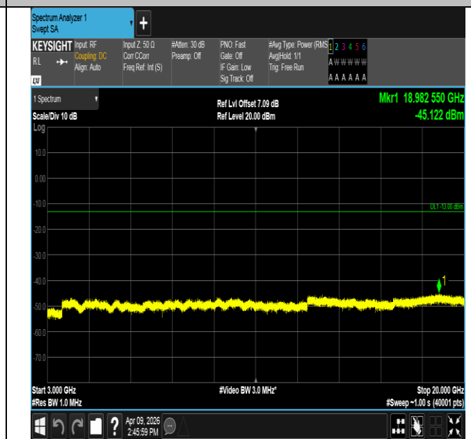
Band2-1.4MHz-16QAM-18900-6RB#0-3000~20000-PASS
