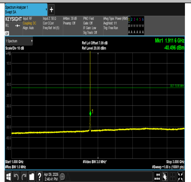
Band2-1.4MHz-QPSK-19193-1RB#0-1000~3000-PASS
