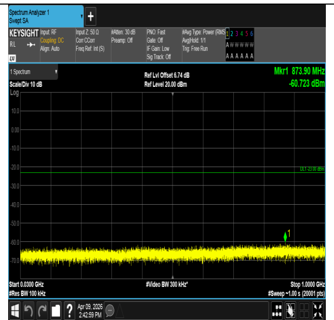
Band2-1.4MHz-QPSK-18900-1RB#5-30~1000-PASS
