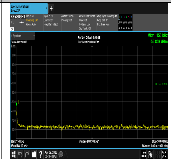
Band2-1.4MHz-16QAM-18900-1RB#5-0.15~30-PASS
