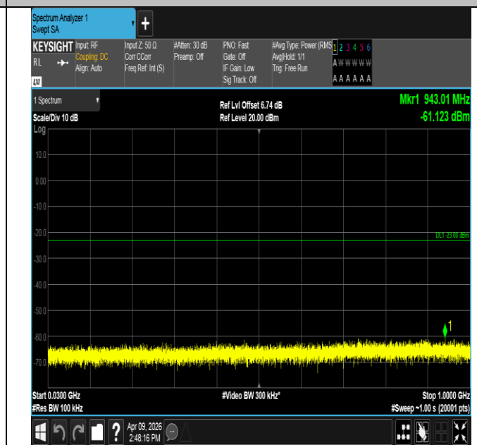
Band2-1.4MHz-QPSK-19193-1RB#5-30~1000-PASS
