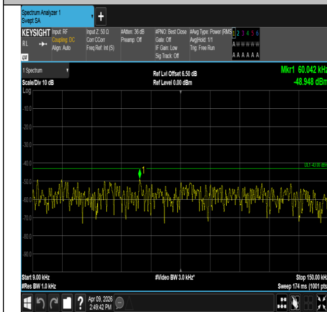
Band2-1.4MHz-QPSK-19193-6RB#0-0.009~0.15-PASS
