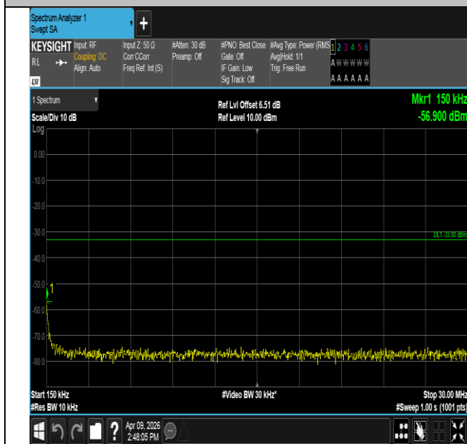
Band2-1.4MHz-QPSK-19193-1RB#5-0.15~30-PASS
