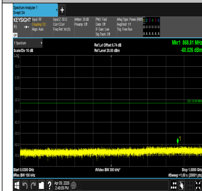
Band2-1.4MHz-16QAM-19193-1RB#5-30~1000-PASS
