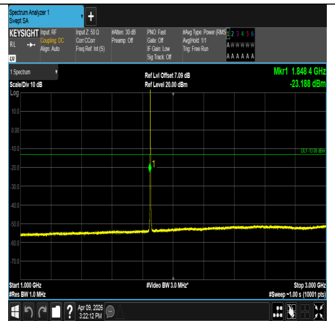
Band2-3MHz-QPSK-18615-1RB#0-1000~3000-PASS
