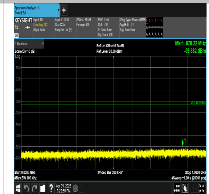
Band2-3MHz-16QAM-18615-1RB#0-30~1000-PASS
