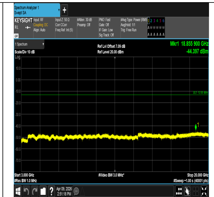
Band2-1.4MHz-16QAM-19193-6RB#0-3000~20000-PASS
