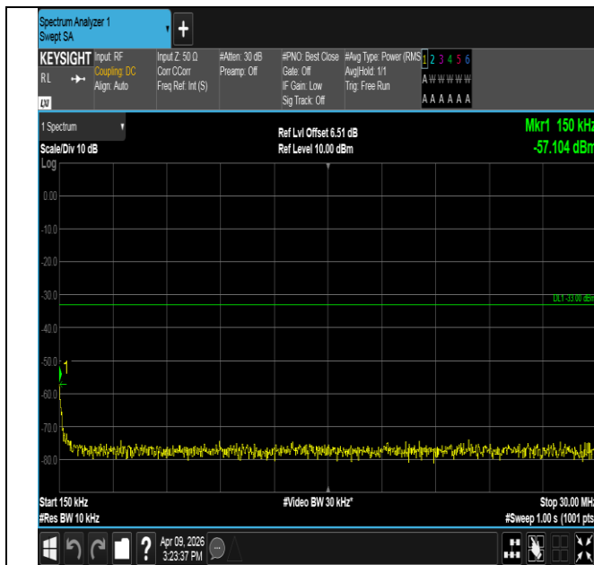
Band2-3MHz-QPSK-18615-1RB#14-0.15~30-PASS
