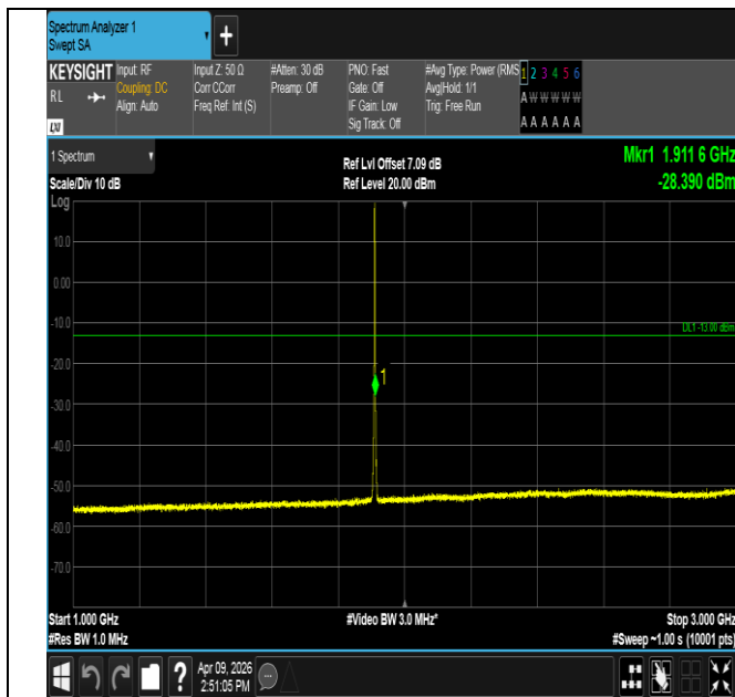
Band2-1.4MHz-16QAM-19193-6RB#0-1000~3000-PASS
