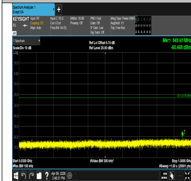
Band2-1.4MHz-QPSK-19193-1RB#0-30~1000-PASS
