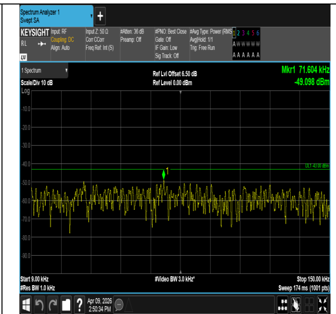
Band2-1.4MHz-16QAM-19193-6RB#0-0.009~0.15-PASS
