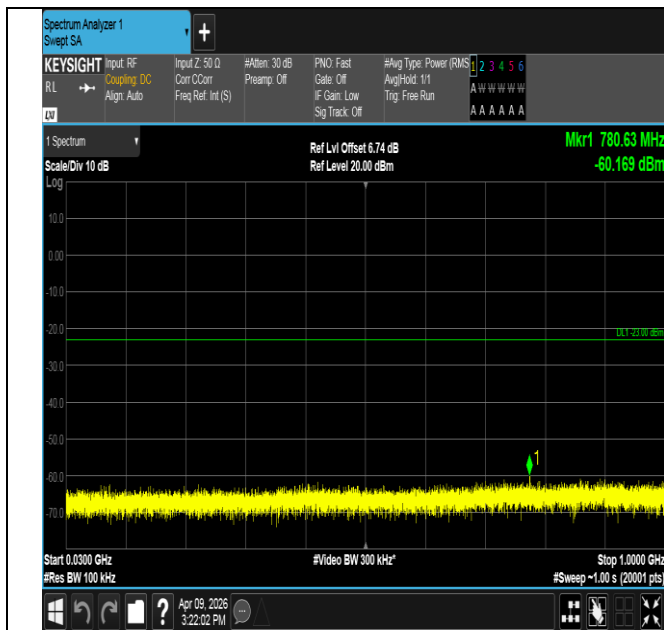
Band2-3MHz-QPSK-18615-1RB#0-30~1000-PASS
