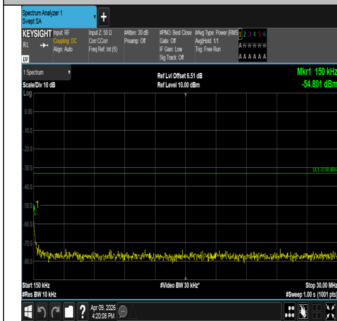
Band2-5MHz-QPSK-19175-1RB#24-0.15~30-PASS
