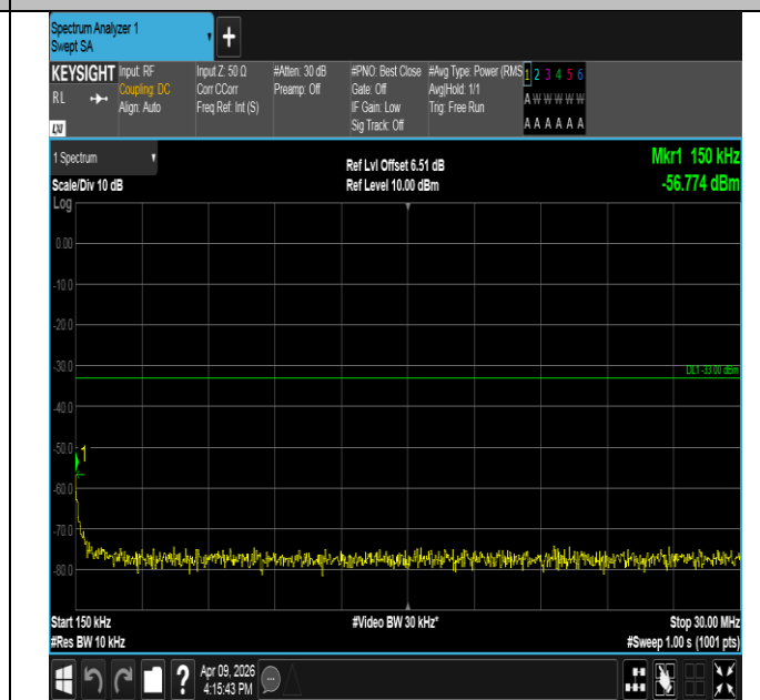
Band2-5MHz-16QAM-18900-1RB#24-0.15~30-PASS
