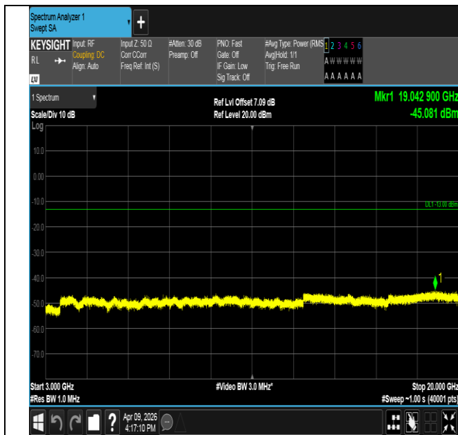
Band2-5MHz-QPSK-18900-25RB#0-3000~20000-PASS
