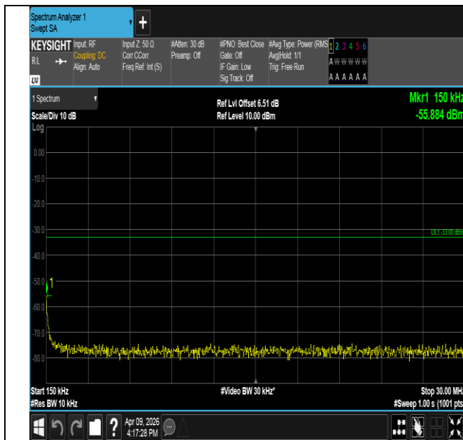
Band2-5MHz-16QAM-18900-25RB#0-0.15~30-PASS
