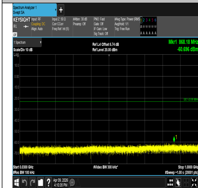
Band2-5MHz-16QAM-18625-1RB#24-30~1000-PASS
