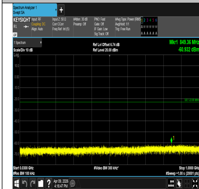
Band2-5MHz-QPSK-18900-25RB#0-30~1000-PASS
