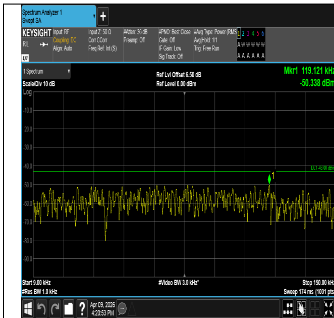
Band2-5MHz-16QAM-19175-1RB#24-0.009~0.15-PASS
