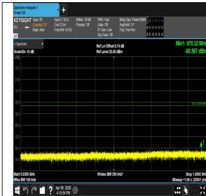
Band2-5MHz-16QAM-18900-1RB#24-30~1000-PASS
