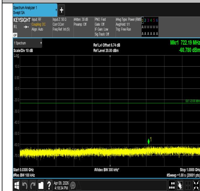
Band2-5MHz-QPSK-19175-1RB#0-30~1000-PASS
