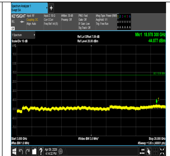
Band2-5MHz-16QAM-18900-1RB#0-3000~20000-PASS
