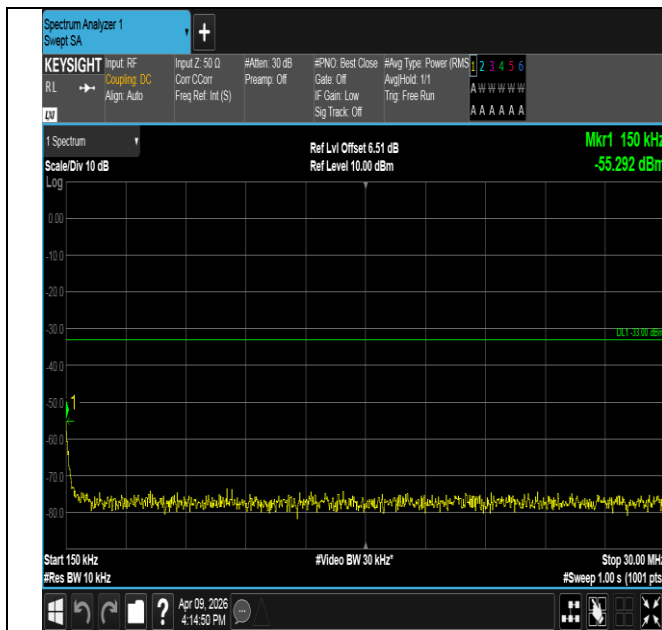
Band2-5MHz-QPSK-18900-1RB#24-0.15~30-PASS
