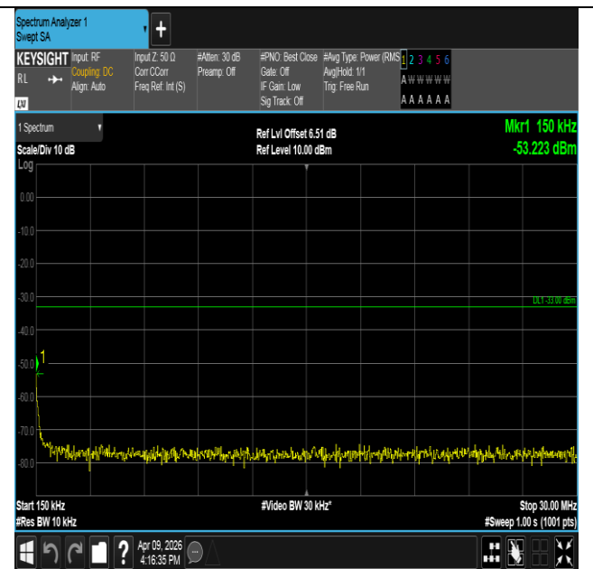
Band2-5MHz-QPSK-18900-25RB#0-0.15~30-PASS
