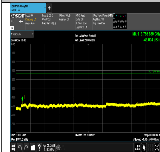
Band2-5MHz-QPSK-18900-1RB#0-3000~20000-PASS
