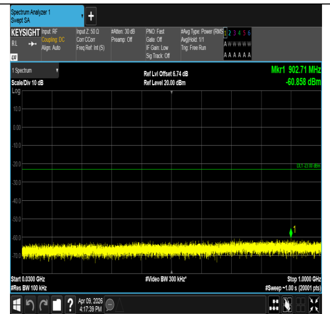
Band2-5MHz-16QAM-18900-25RB#0-30~1000-PASS
