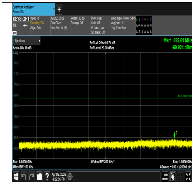
Band2-5MHz-QPSK-19175-25RB#0-30~1000-PASS
