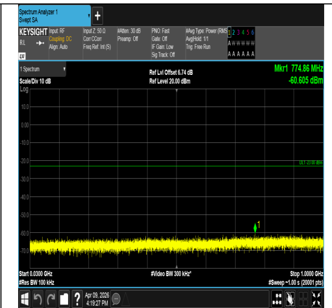
Band2-5MHz-16QAM-19175-1RB#0-30~1000-PASS
