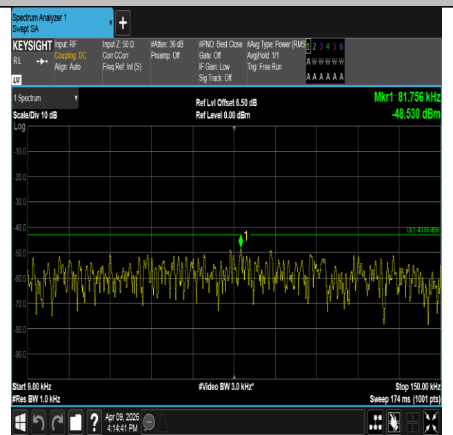
Band2-5MHz-QPSK-18900-1RB#24-0.009~0.15-PASS
