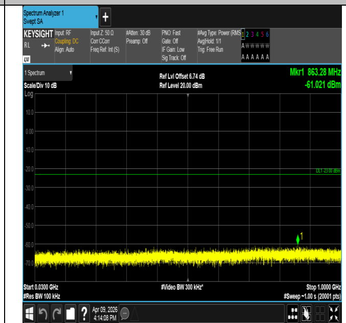
Band2-5MHz-16QAM-18900-1RB#0-30~1000-PASS
