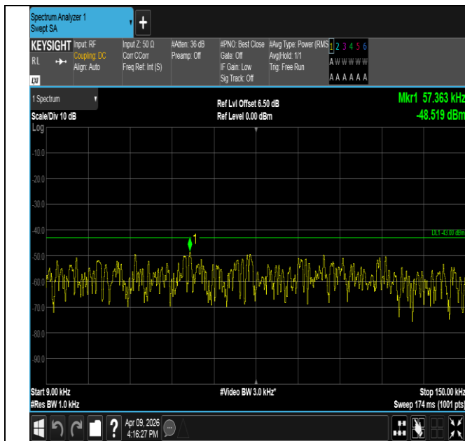
Band2-5MHz-QPSK-18900-25RB#0-0.009~0.15-PASS
