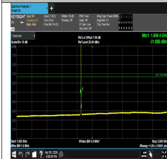
Band2-5MHz-16QAM-18625-1RB#0-1000~3000-PASS
