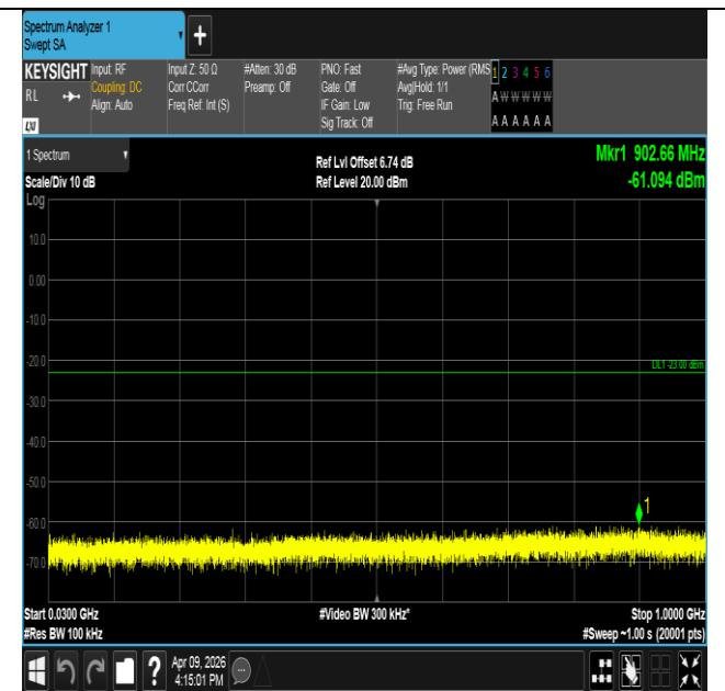
Band2-5MHz-QPSK-18900-1RB#24-30~1000-PASS
