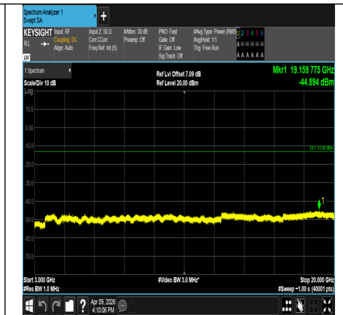
Band2-5MHz-QPSK-18625-1RB#24-3000~20000-PASS
