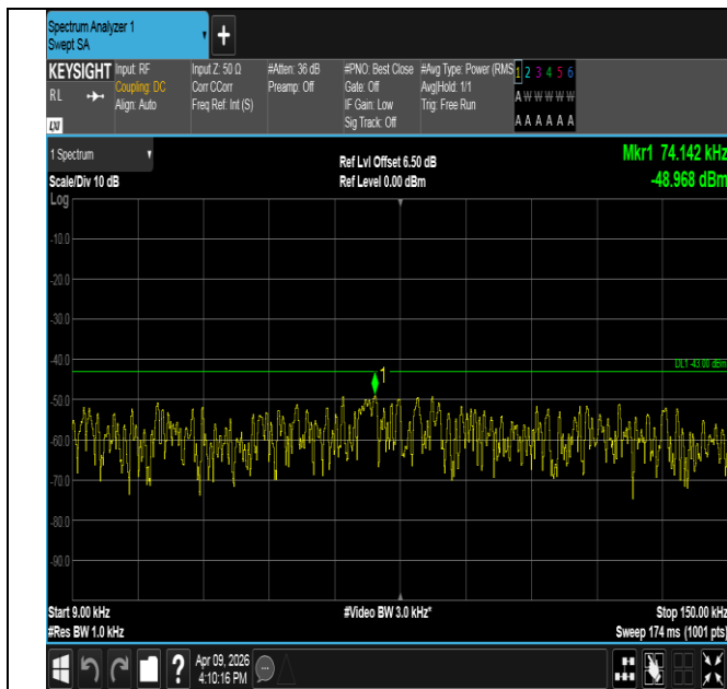
Band2-5MHz-16QAM-18625-1RB#24-0.009~0.15-PASS
