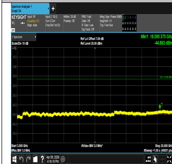
Band2-5MHz-16QAM-18900-1RB#24-3000~20000-PASS
