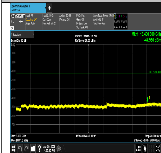
Band2-5MHz-QPSK-19175-25RB#0-3000~20000-PASS
