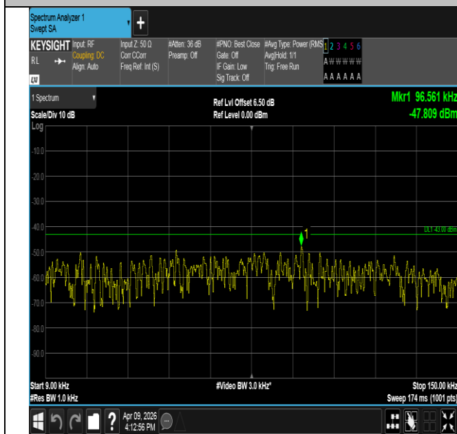
Band2-5MHz-QPSK-18900-1RB#0-0.009~0.15-PASS
