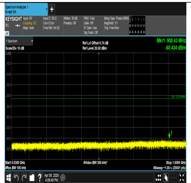
Band2-5MHz-16QAM-18625-1RB#0-30~1000-PASS
