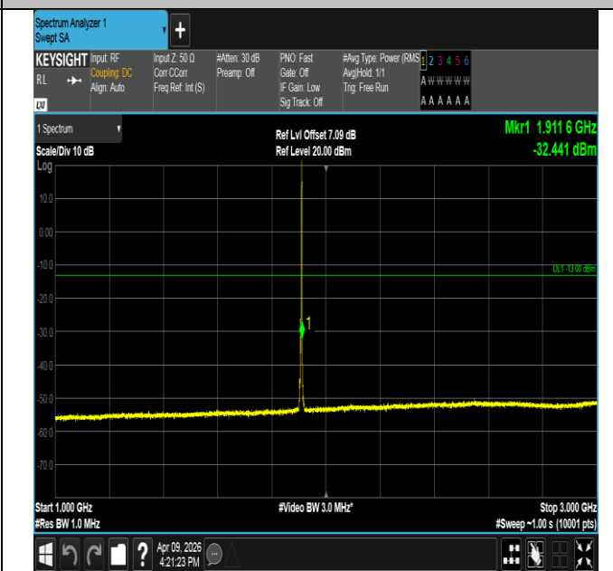
Band2-5MHz-16QAM-19175-1RB#24-1000~3000-PASS
