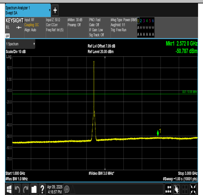
Band2-5MHz-QPSK-18900-25RB#0-1000~3000-PASS
