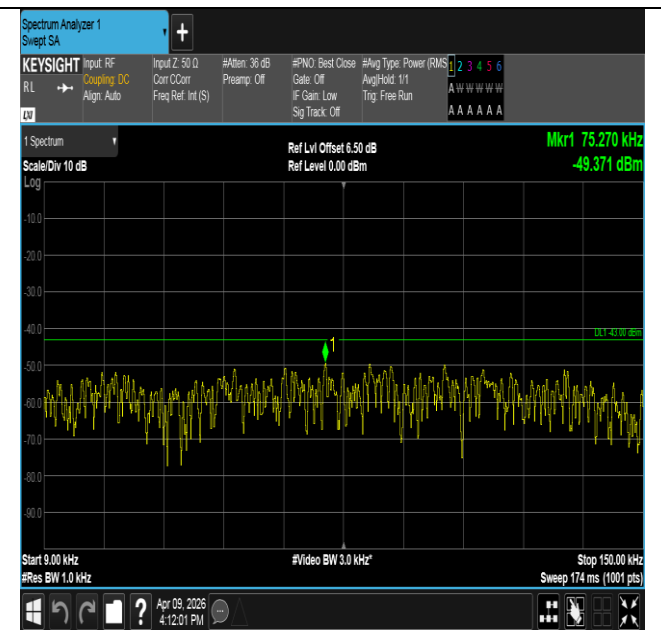
Band2-5MHz-16QAM-18625-25RB#0-0.009~0.15-PASS
