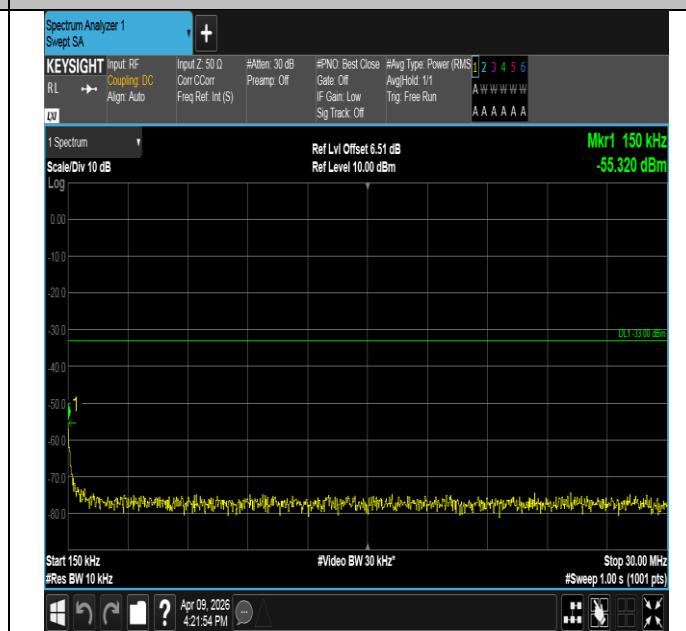
Band2-5MHz-QPSK-19175-25RB#0-0.15~30-PASS
