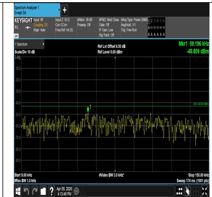
Band2-5MHz-16QAM-18900-1RB#0-0.009~0.15-PASS
