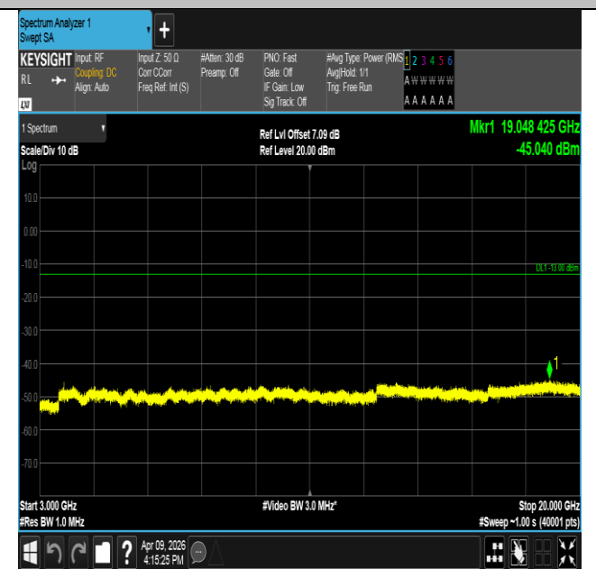
Band2-5MHz-QPSK-18900-1RB#24-3000~20000-PASS
