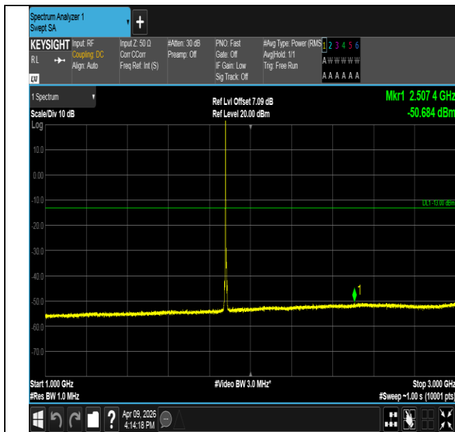
Band2-5MHz-16QAM-18900-1RB#0-1000~3000-PASS
