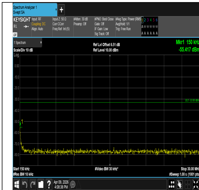
Band2-5MHz-16QAM-18625-1RB#0-0.15~30-PASS
