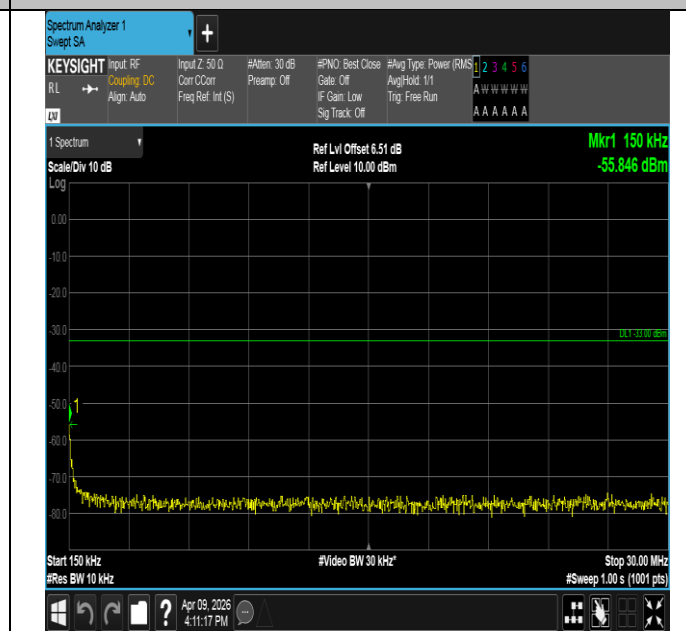
Band2-5MHz-QPSK-18625-25RB#0-0.15~30-PASS
