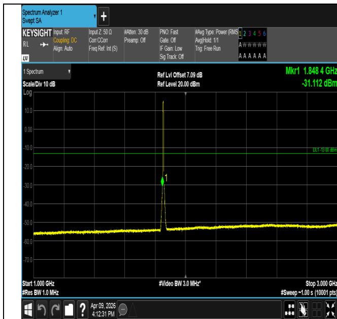
Band2-5MHz-16QAM-18625-25RB#0-1000~3000-PASS
