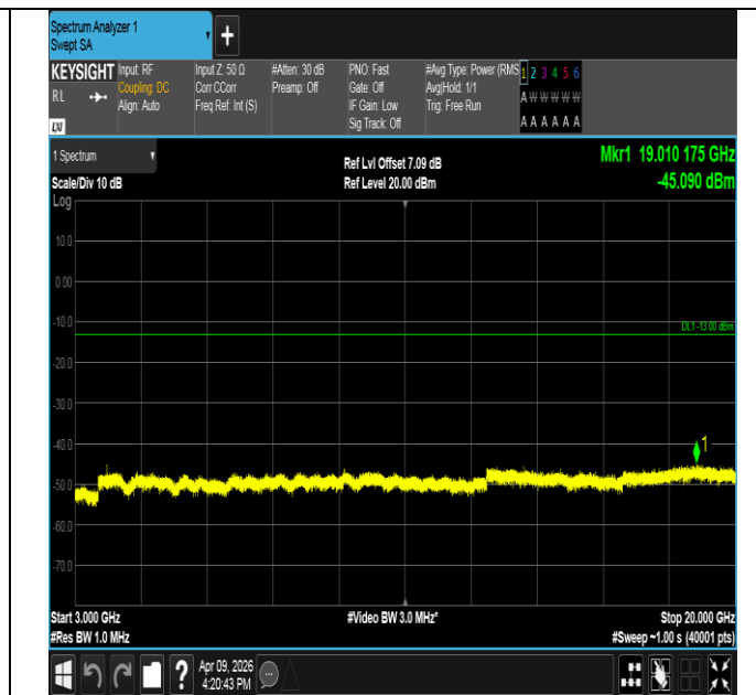
Band2-5MHz-QPSK-19175-1RB#24-3000~20000-PASS
