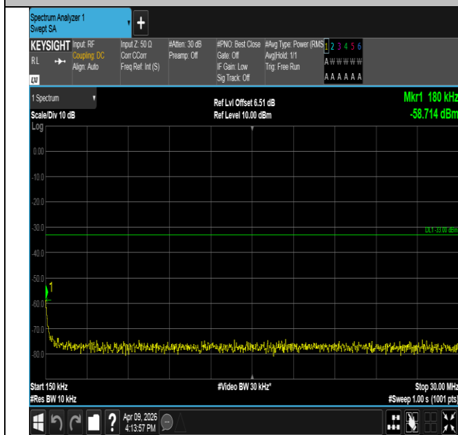
Band2-5MHz-16QAM-18900-1RB#0-0.15~30-PASS
