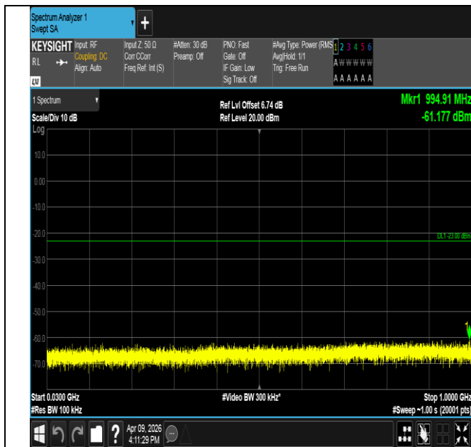
Band2-5MHz-QPSK-18625-25RB#0-30~1000-PASS
