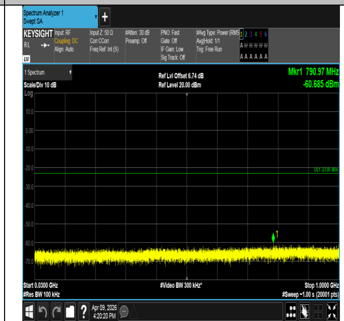
Band2-5MHz-QPSK-19175-1RB#24-30~1000-PASS
