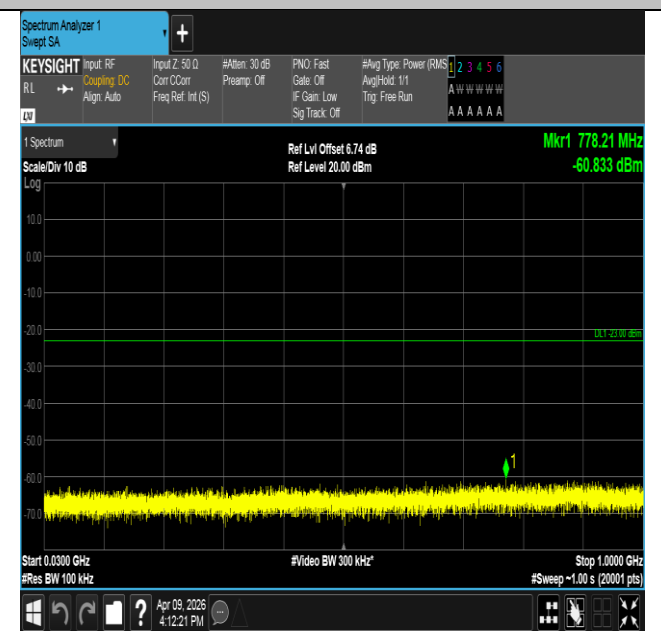
Band2-5MHz-16QAM-18625-25RB#0-30~1000-PASS
