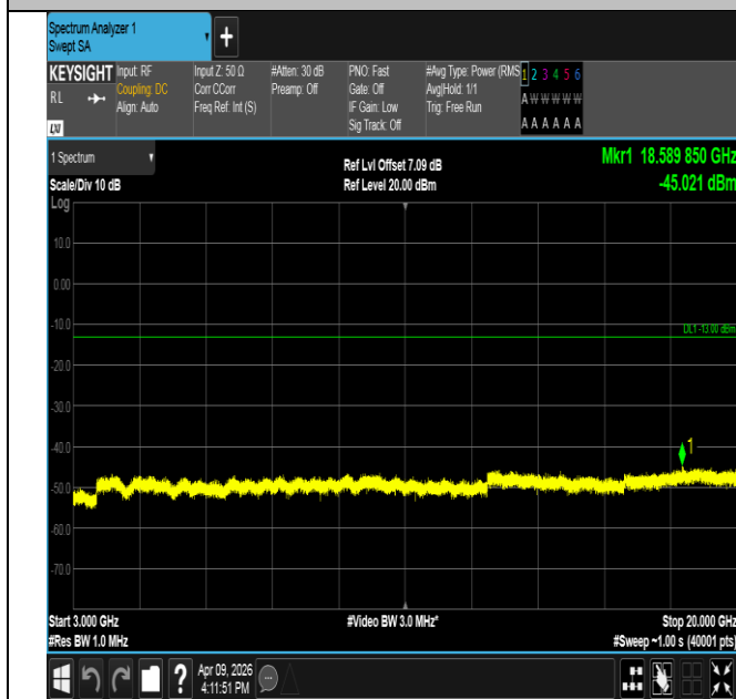
Band2-5MHz-QPSK-18625-25RB#0-3000~20000-PASS
