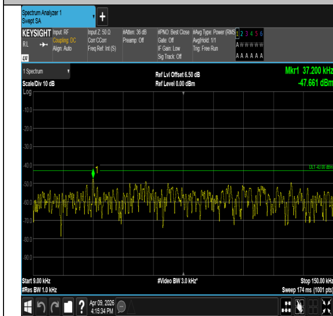
Band2-5MHz-16QAM-18900-1RB#24-0.009~0.15-PASS
