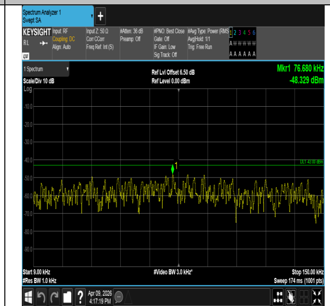
Band2-5MHz-16QAM-18900-25RB#0-0.009~0.15-PASS
