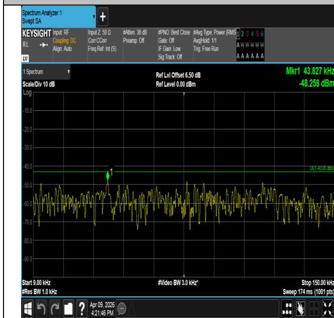
Band2-5MHz-QPSK-19175-25RB#0-0.009~0.15-PASS
