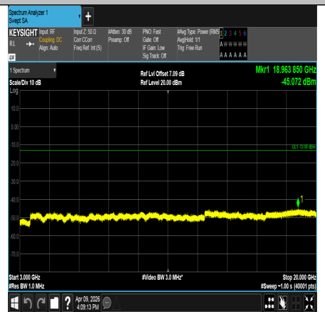
Band2-5MHz-16QAM-18625-1RB#0-3000~20000-PASS
