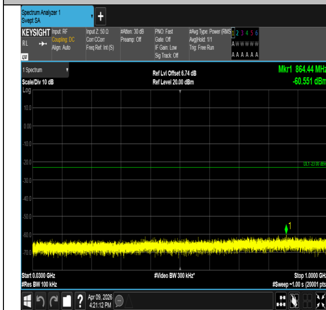
Band2-5MHz-16QAM-19175-1RB#24-30~1000-PASS
