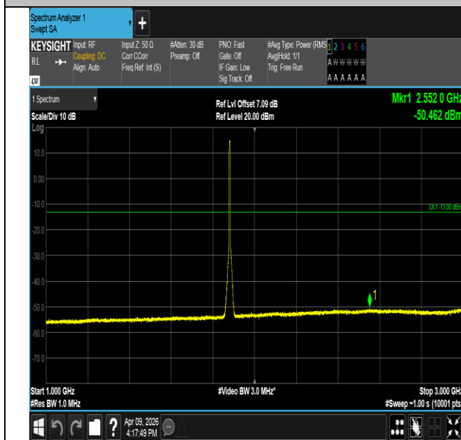
Band2-5MHz-16QAM-18900-25RB#0-1000~3000-PASS
