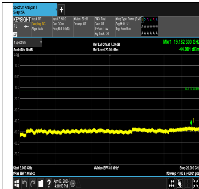
Band2-5MHz-16QAM-18625-1RB#24-3000~20000-PASS
