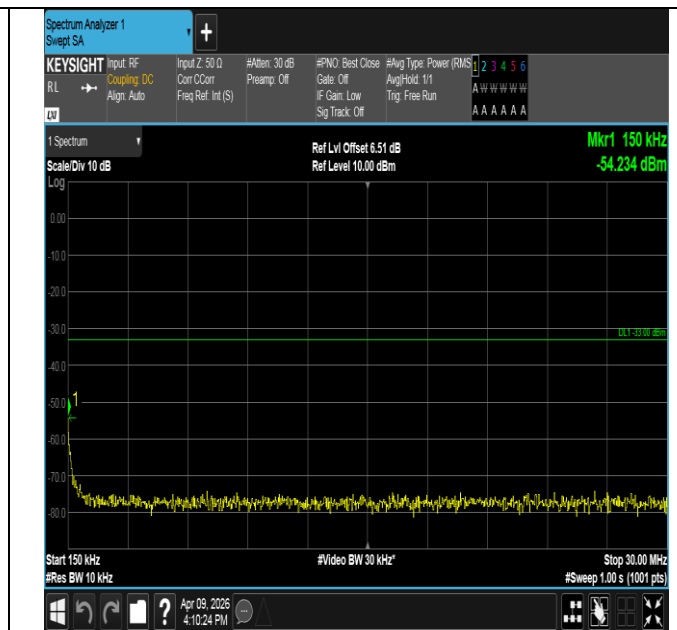
Band2-5MHz-16QAM-18625-1RB#24-0.15~30-PASS
