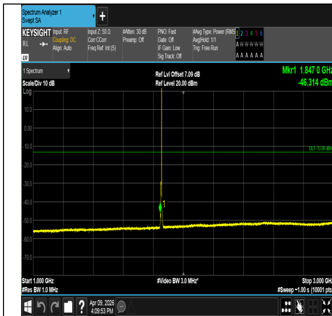
Band2-5MHz-QPSK-18625-1RB#24-1000~3000-PASS
