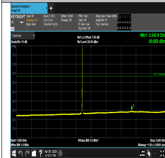
Band2-5MHz-QPSK-18900-1RB#24-1000~3000-PASS
