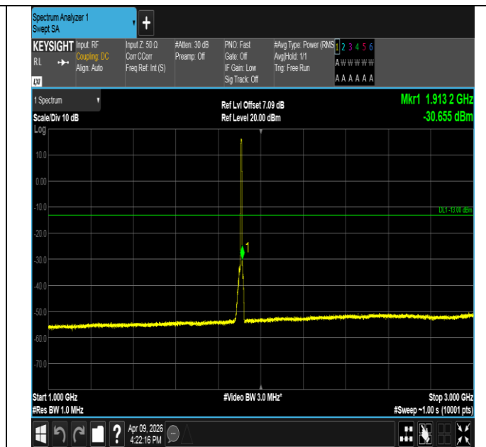
Band2-5MHz-QPSK-19175-25RB#0-1000~3000-PASS
