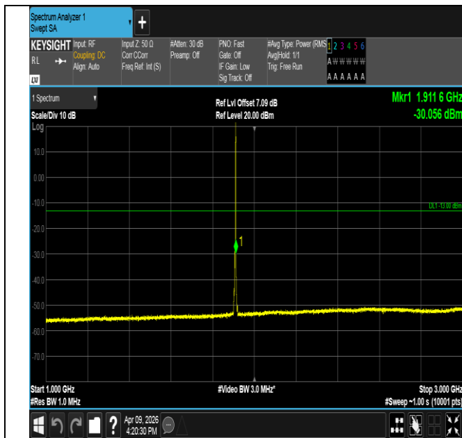
Band2-5MHz-QPSK-19175-1RB#24-1000~3000-PASS
