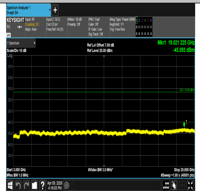
Band2-5MHz-16QAM-18900-25RB#0-3000~20000-PASS
