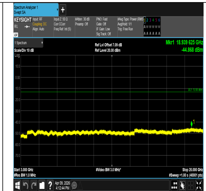
Band2-5MHz-16QAM-18625-25RB#0-3000~20000-PASS
