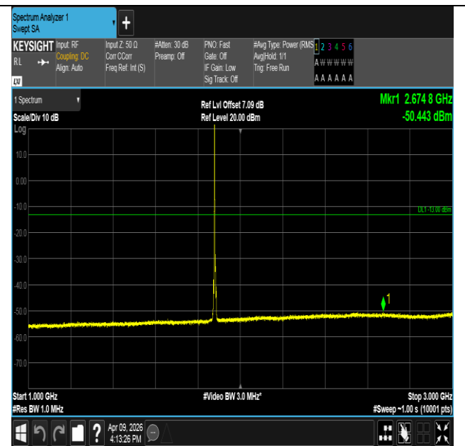
Band2-5MHz-QPSK-18900-1RB#0-1000~3000-PASS
