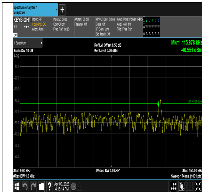
Band2-5MHz-QPSK-19175-1RB#0-0.009~0.15-PASS
