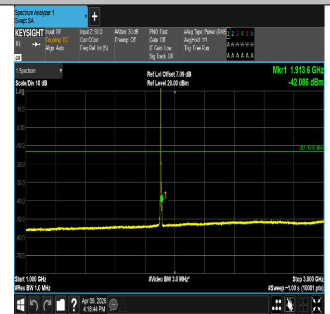
Band2-5MHz-QPSK-19175-1RB#0-1000~3000-PASS
