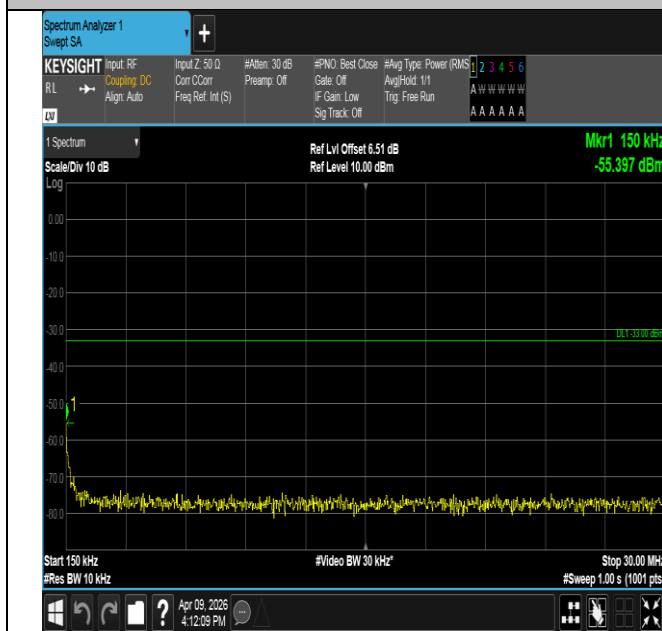
Band2-5MHz-16QAM-18625-25RB#0-0.15~30-PASS
