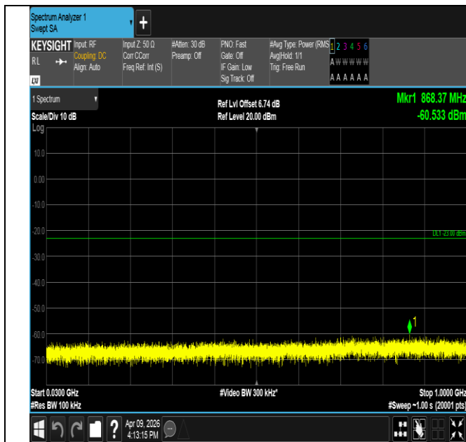
Band2-5MHz-QPSK-18900-1RB#0-30~1000-PASS
