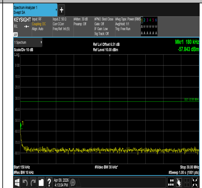
Band2-5MHz-QPSK-18900-1RB#0-0.15~30-PASS
