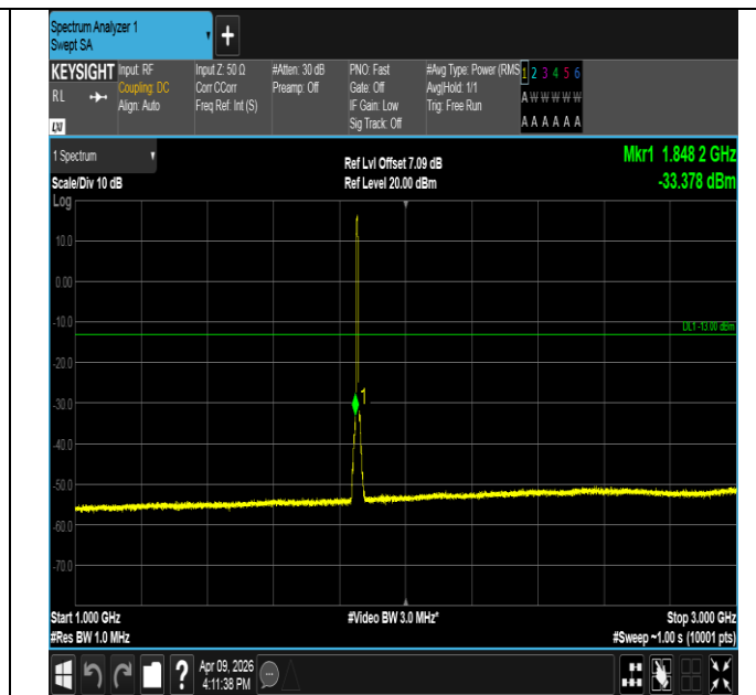
Band2-5MHz-QPSK-18625-25RB#0-1000~3000-PASS
