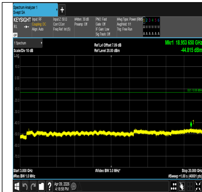
Band2-5MHz-QPSK-19175-1RB#0-3000~20000-PASS
