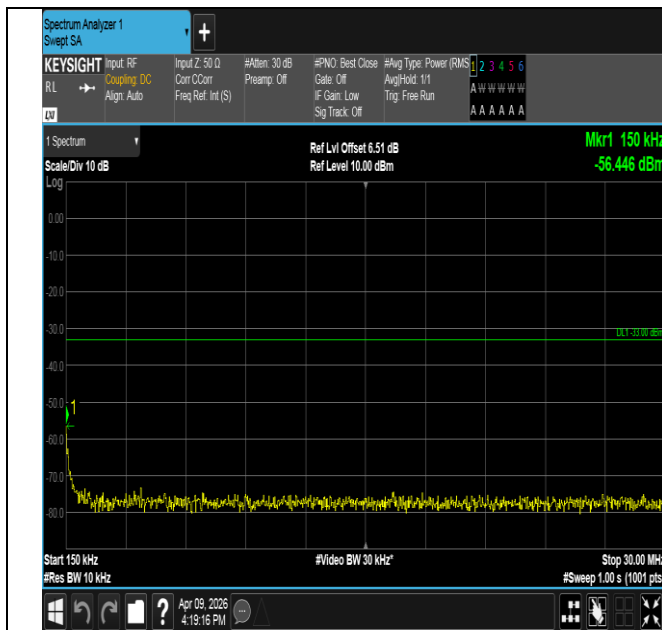
Band2-5MHz-16QAM-19175-1RB#0-0.15~30-PASS
