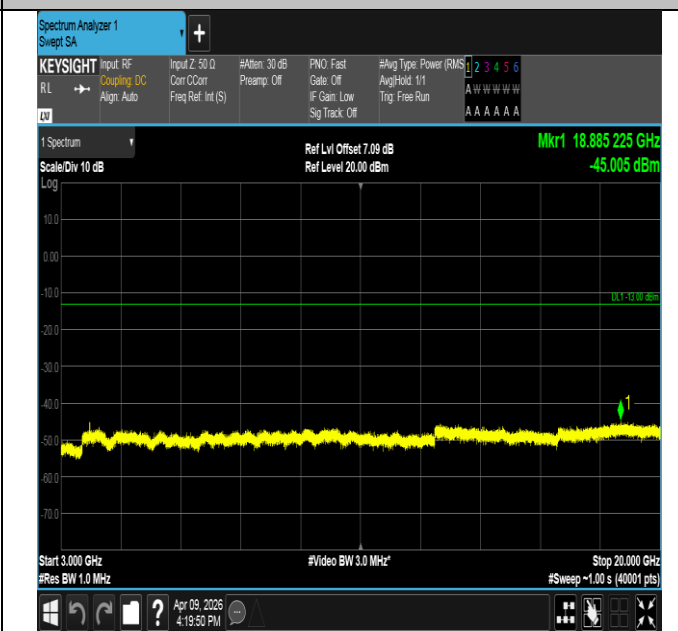
Band2-5MHz-16QAM-19175-1RB#0-3000~20000-PASS
