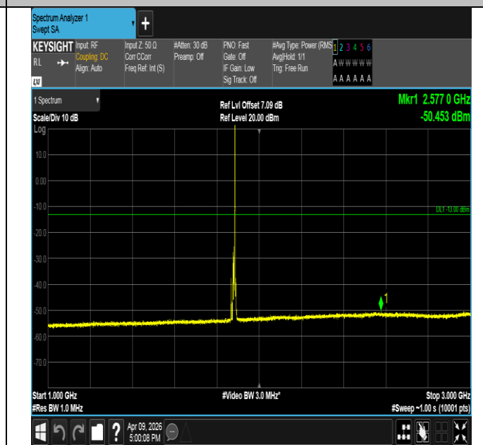
Band2-10MHz-16QAM-18900-1RB#49-1000~3000-PASS
