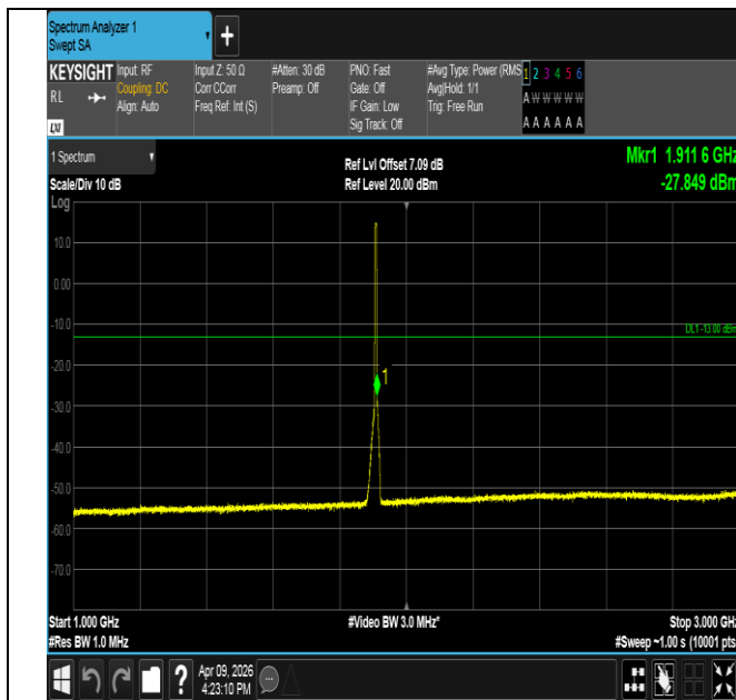
Band2-5MHz-16QAM-19175-25RB#0-1000~3000-PASS
