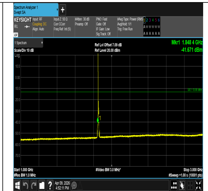
Band2-10MHz-QPSK-18650-1RB#0-1000~3000-PASS
