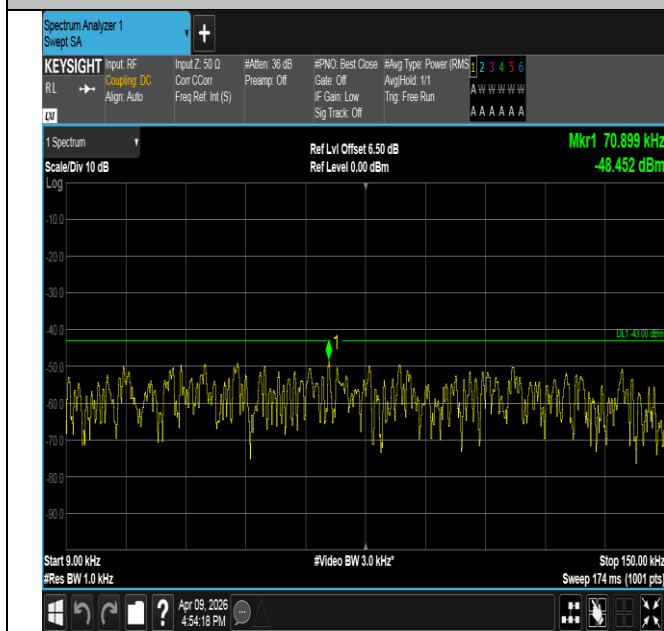
Band2-10MHz-16QAM-18650-1RB#49-0.009~0.15-PASS
