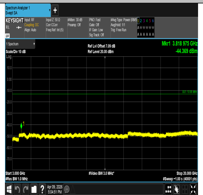
Band2-10MHz-QPSK-19150-1RB#49-3000~20000-PASS
