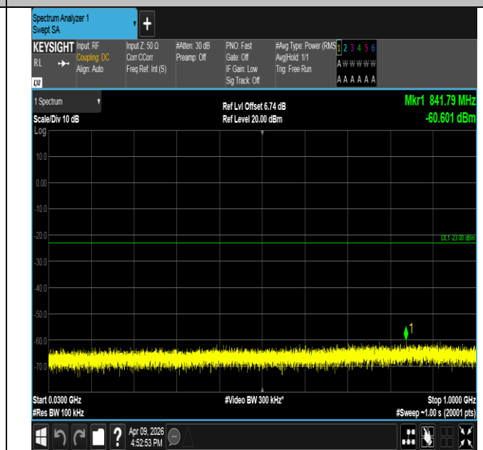
Band2-10MHz-16QAM-18650-1RB#0-30~1000-PASS
