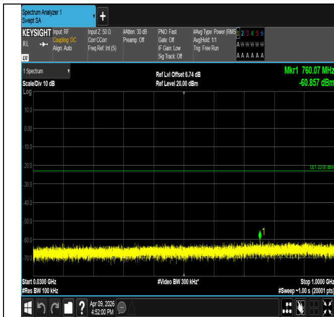
Band2-10MHz-QPSK-18650-1RB#0-30~1000-PASS
