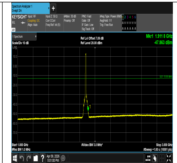
Band2-10MHz-QPSK-18900-50RB#0-1000~3000-PASS
