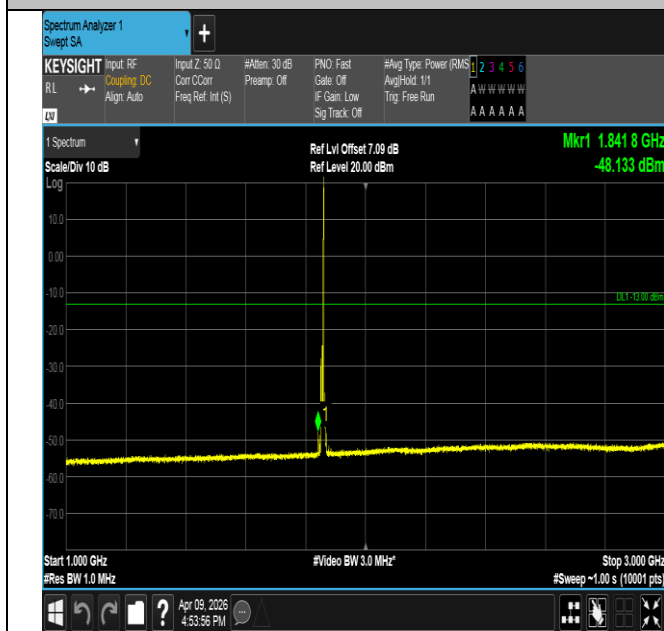
Band2-10MHz-QPSK-18650-1RB#49-1000~3000-PASS
