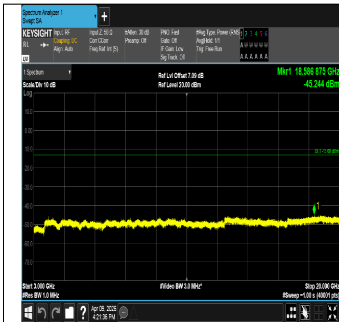
Band2-5MHz-16QAM-19175-1RB#24-3000~20000-PASS
