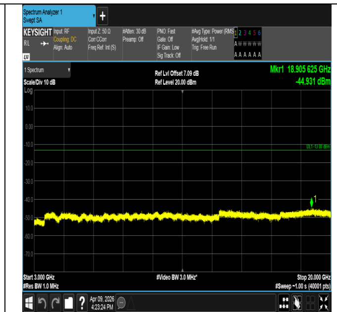
Band2-5MHz-16QAM-19175-25RB#0-3000~20000-PASS
