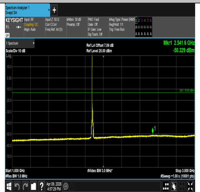
Band2-10MHz-QPSK-18900-1RB#0-1000~3000-PASS
