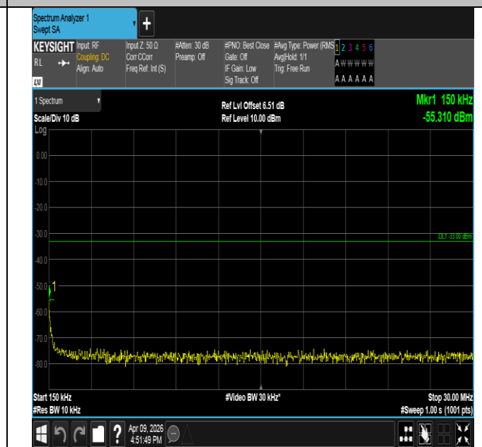
Band2-10MHz-QPSK-18650-1RB#0-0.15~30-PASS
