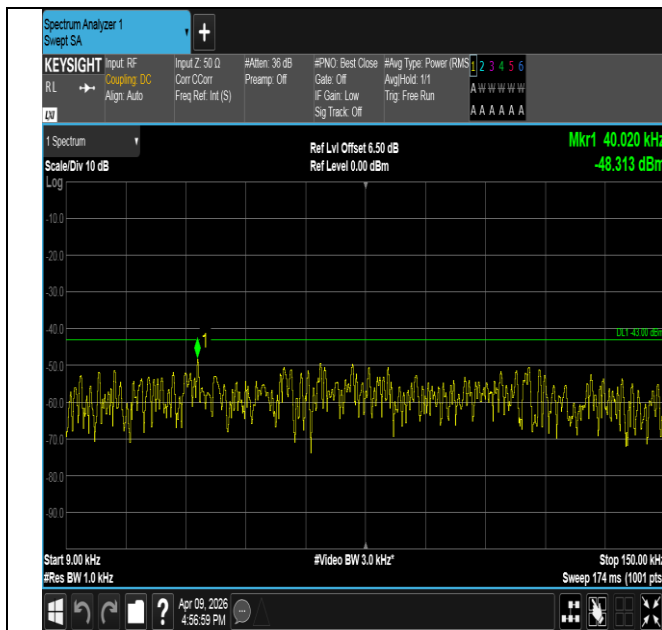
Band2-10MHz-QPSK-18900-1RB#0-0.009~0.15-PASS
