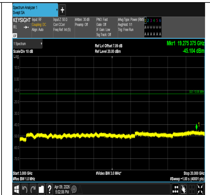
Band2-10MHz-16QAM-18900-50RB#0-3000~20000-PASS
