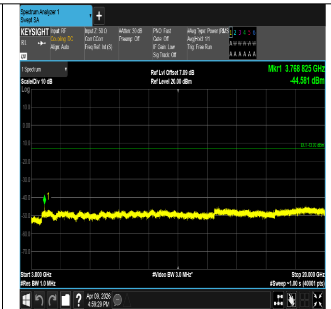
Band2-10MHz-QPSK-18900-1RB#49-3000~20000-PASS
