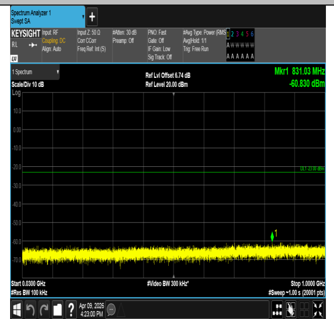
Band2-5MHz-16QAM-19175-25RB#0-30~1000-PASS
