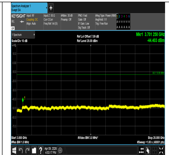
Band2-10MHz-16QAM-18650-1RB#0-3000~20000-PASS
