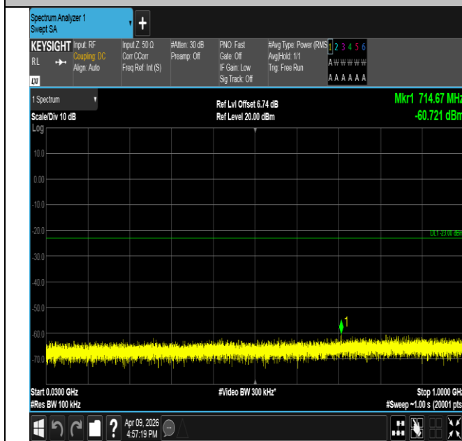
Band2-10MHz-QPSK-18900-1RB#0-30~1000-PASS
