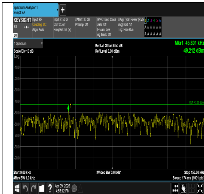
Band2-10MHz-QPSK-18650-50RB#0-0.009~0.15-PASS
