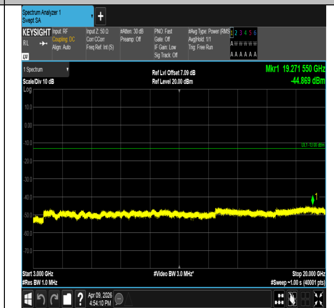
Band2-10MHz-QPSK-18650-1RB#49-3000~20000-PASS
