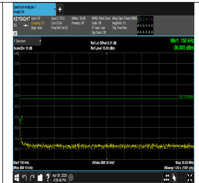
Band2-10MHz-16QAM-18900-1RB#49-0.15~30-PASS
