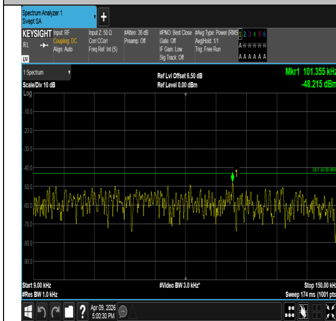
Band2-10MHz-QPSK-18900-50RB#0-0.009~0.15-PASS
