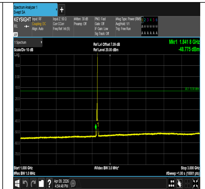
Band2-10MHz-16QAM-18650-1RB#49-1000~3000-PASS
