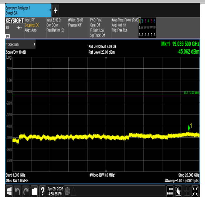
Band2-10MHz-16QAM-18900-1RB#0-3000~20000-PASS
