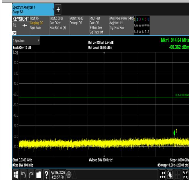
Band2-10MHz-16QAM-18900-1RB#49-30~1000-PASS
