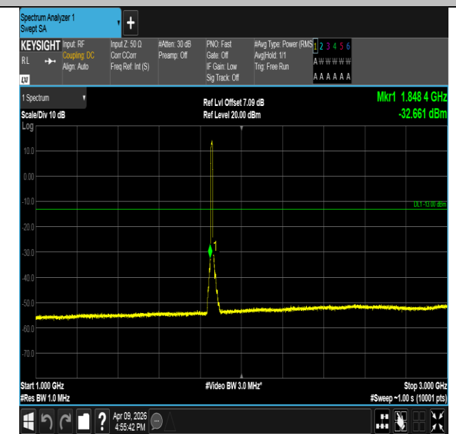
Band2-10MHz-QPSK-18650-50RB#0-1000~3000-PASS
