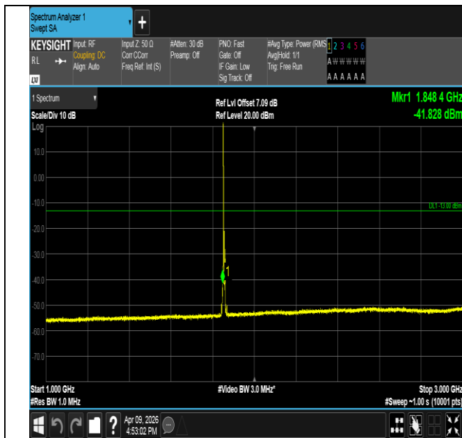
Band2-10MHz-16QAM-18650-1RB#0-1000~3000-PASS
