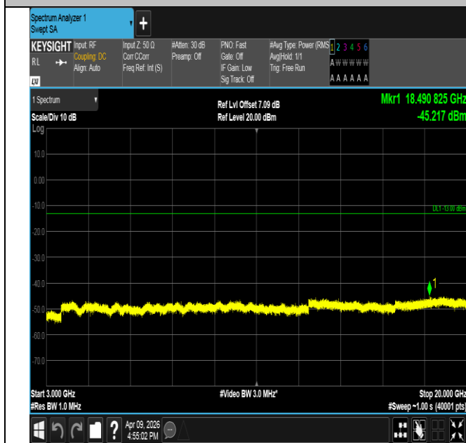
Band2-10MHz-16QAM-18650-1RB#49-3000~20000-PASS
