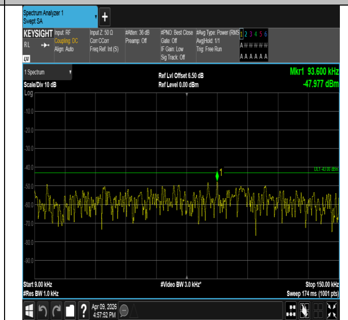
Band2-10MHz-16QAM-18900-1RB#0-0.009~0.15-PASS
