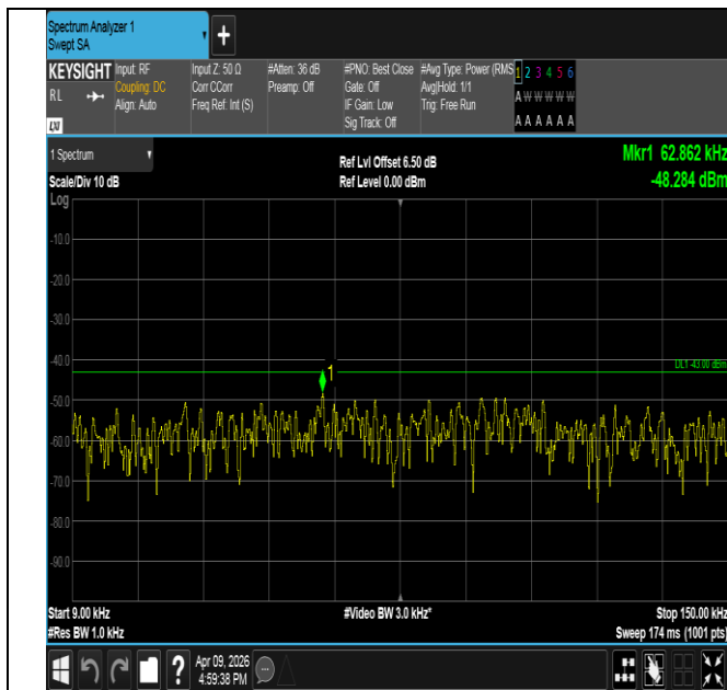
Band2-10MHz-16QAM-18900-1RB#49-0.009~0.15-PASS
