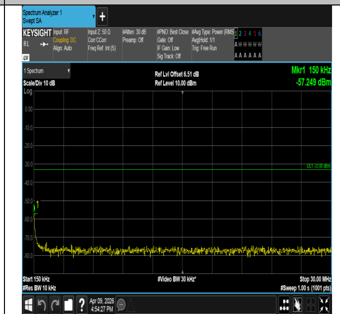
Band2-10MHz-16QAM-18650-1RB#49-0.15~30-PASS
