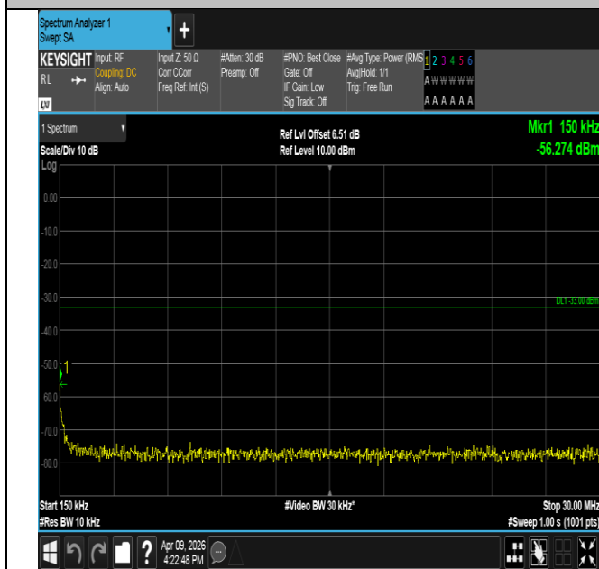
Band2-5MHz-16QAM-19175-25RB#0-0.15~30-PASS
