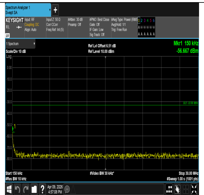
Band2-10MHz-QPSK-18900-1RB#0-0.15~30-PASS
