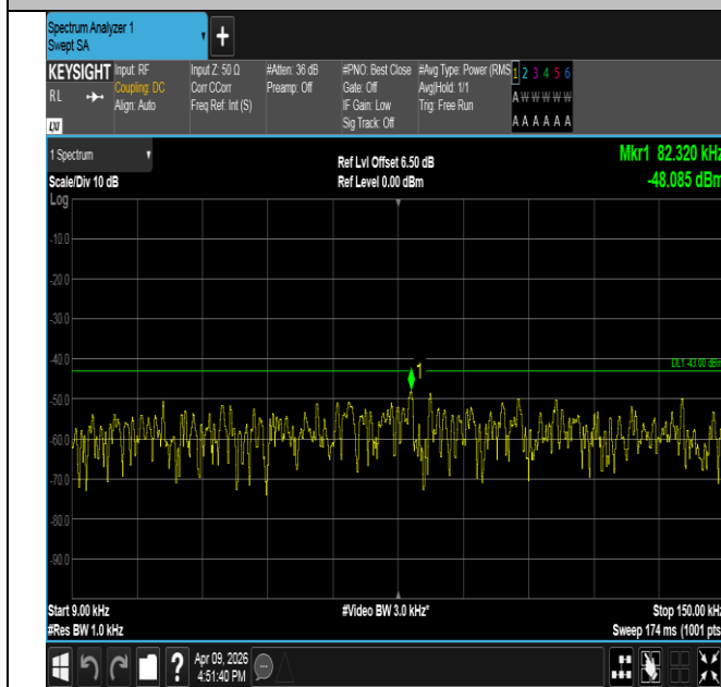
Band2-10MHz-QPSK-18650-1RB#0-0.009~0.15-PASS
