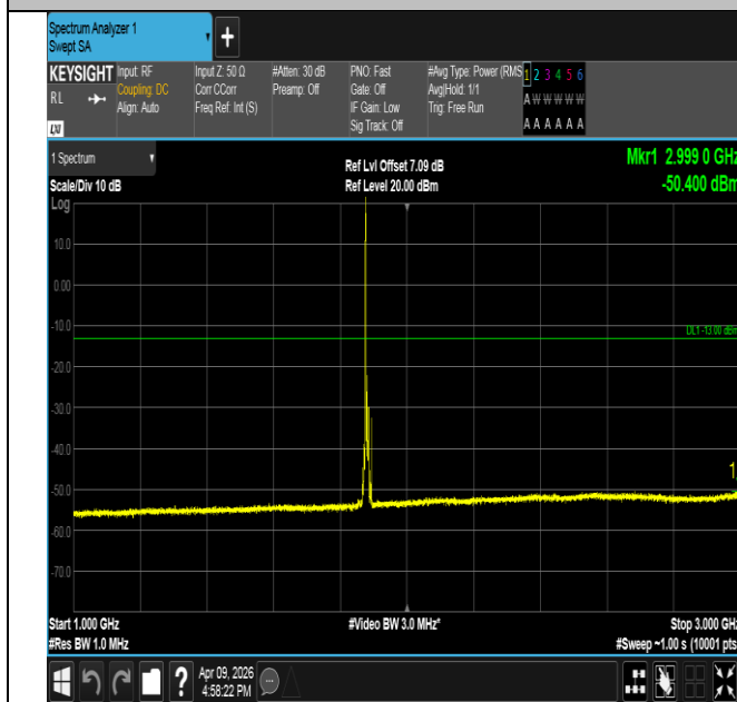
Band2-10MHz-16QAM-18900-1RB#0-1000~3000-PASS
