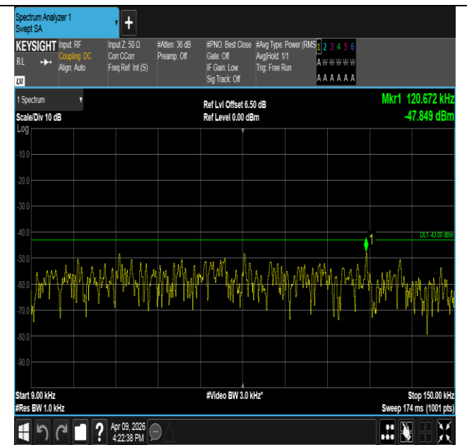
Band2-5MHz-16QAM-19175-25RB#0-0.009~0.15-PASS
