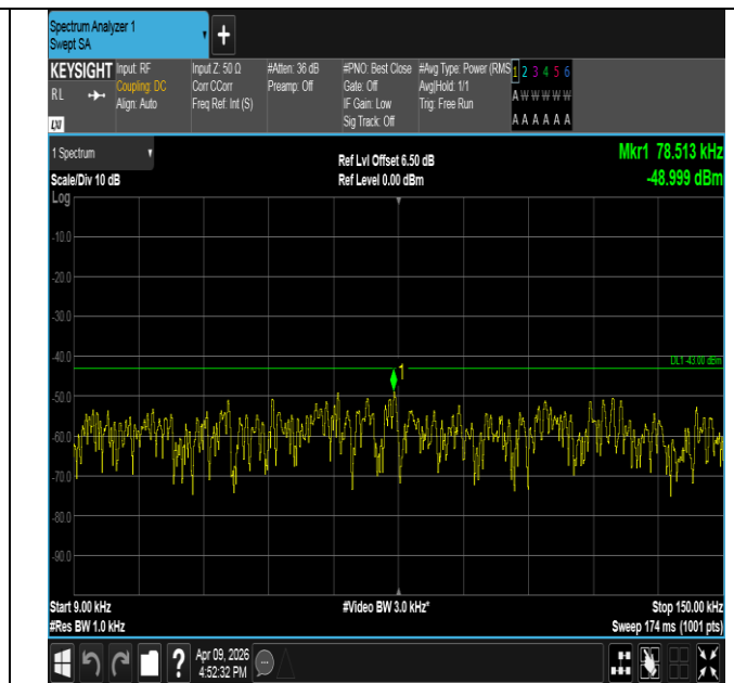
Band2-10MHz-16QAM-18650-1RB#0-0.009~0.15-PASS
