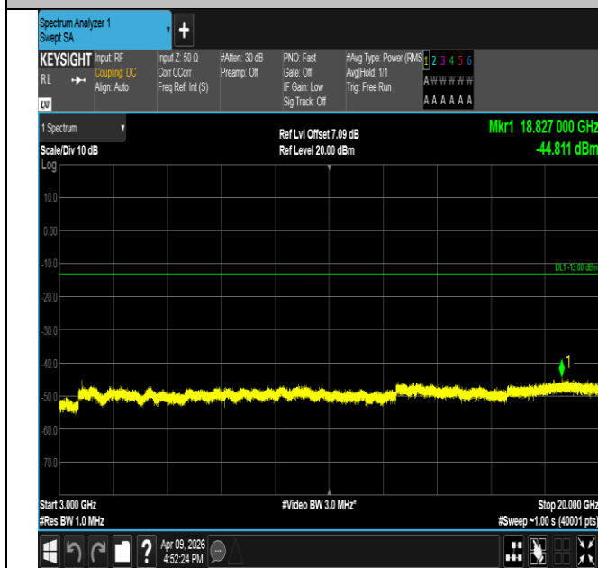
Band2-10MHz-QPSK-18650-1RB#0-3000~20000-PASS
