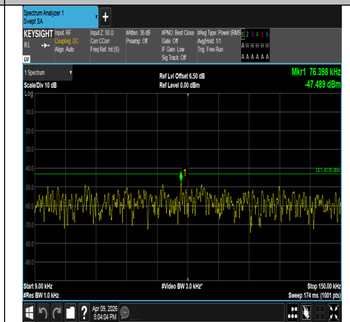
Band2-10MHz-QPSK-19150-1RB#49-0.009~0.15-PASS
