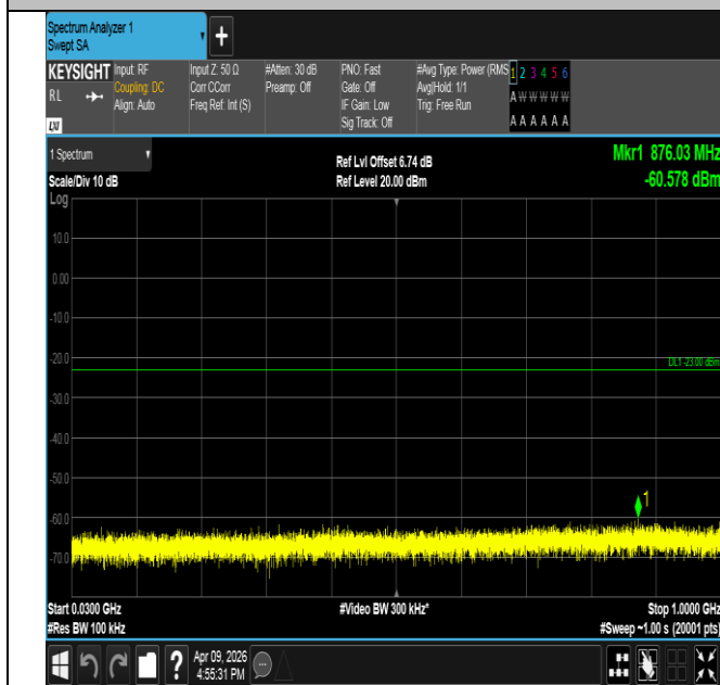
Band2-10MHz-QPSK-18650-50RB#0-30~1000-PASS
