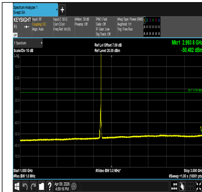
Band2-10MHz-QPSK-18900-1RB#49-1000~3000-PASS
