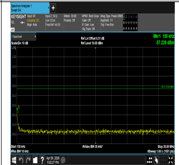
Band2-10MHz-QPSK-19150-1RB#0-0.15~30-PASS
