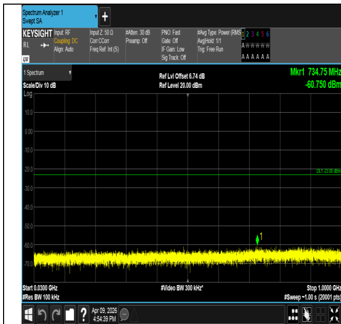
Band2-10MHz-16QAM-18650-1RB#49-30~1000-PASS
