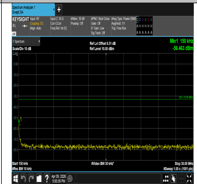
Band2-10MHz-QPSK-18900-50RB#0-0.15~30-PASS
