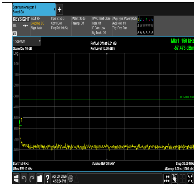
Band2-10MHz-QPSK-18650-1RB#49-0.15~30-PASS
