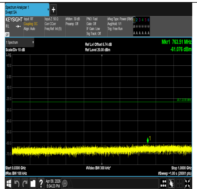
Band2-10MHz-QPSK-19150-1RB#49-30~1000-PASS
