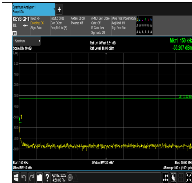
Band2-10MHz-16QAM-18900-1RB#0-0.15~30-PASS
