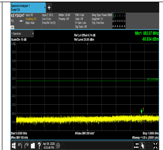
Band2-10MHz-QPSK-18650-1RB#49-30~1000-PASS
