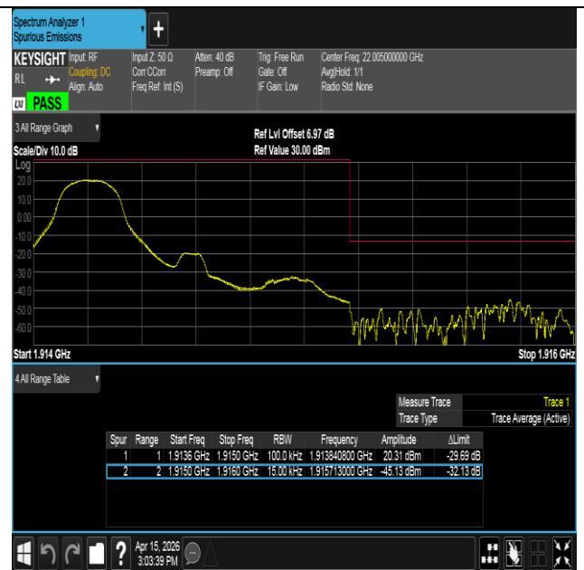
Band25-1.4MHz-16QAM-26683-1RB#0-PASS
