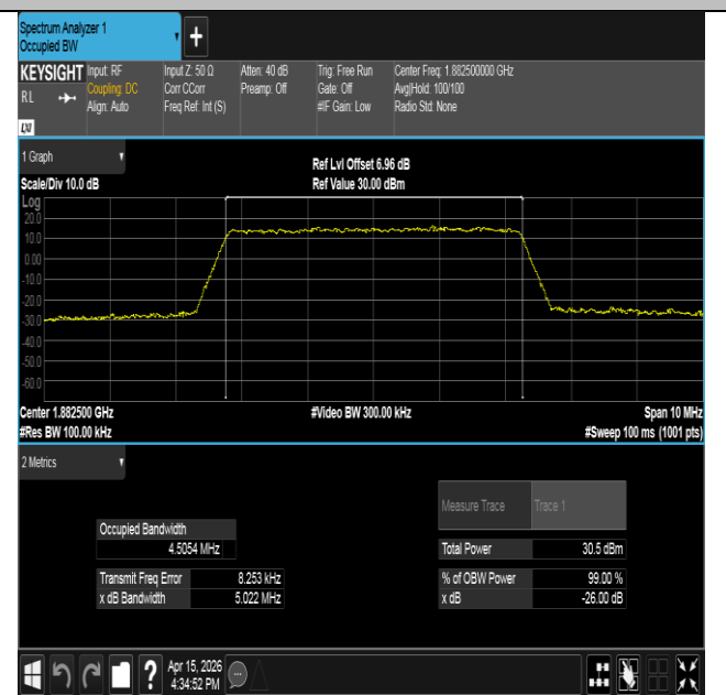
Band25-5MHz-16QAM-26365-25RB#0-PASS
