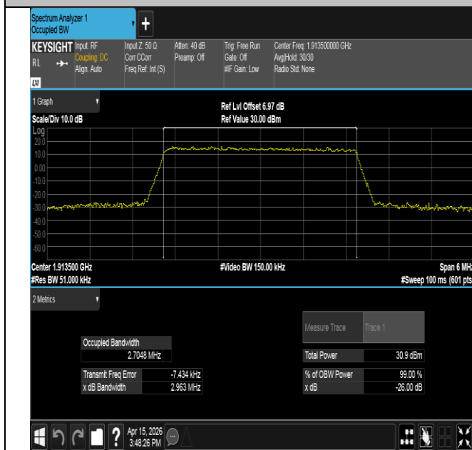
Band25-3MHz-QPSK-26675-15RB#0-PASS
