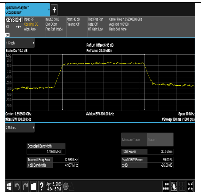
Band25-5MHz-16QAM-26065-25RB#0-PASS
