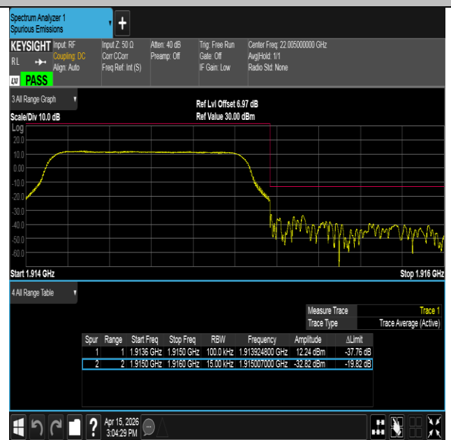
Band25-1.4MHz-16QAM-26683-6RB#0-PASS
