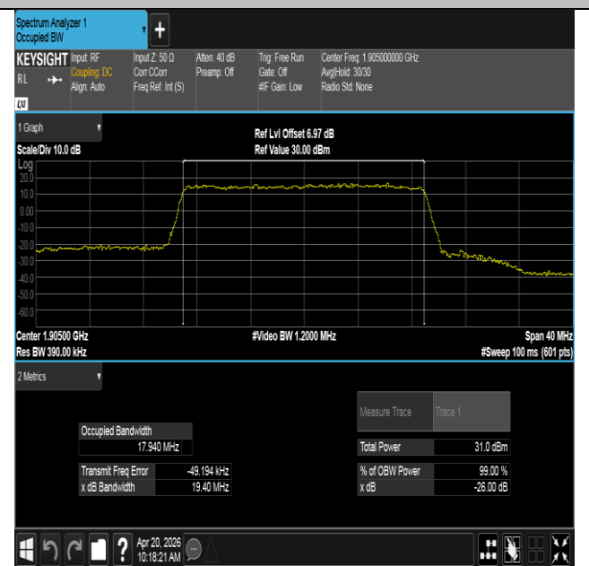
Band25-20MHz-16QAM-26590-100RB#0-PASS
