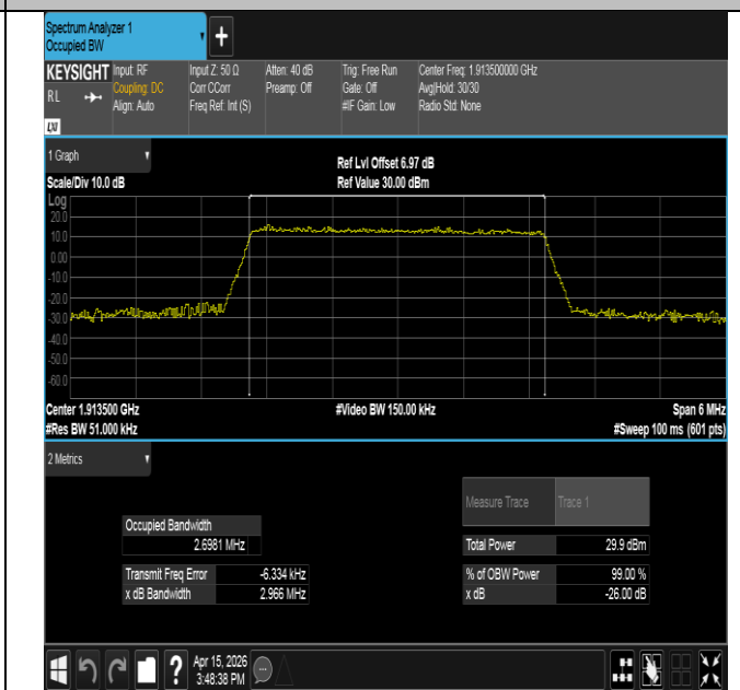
Band25-3MHz-16QAM-26675-15RB#0-PASS
