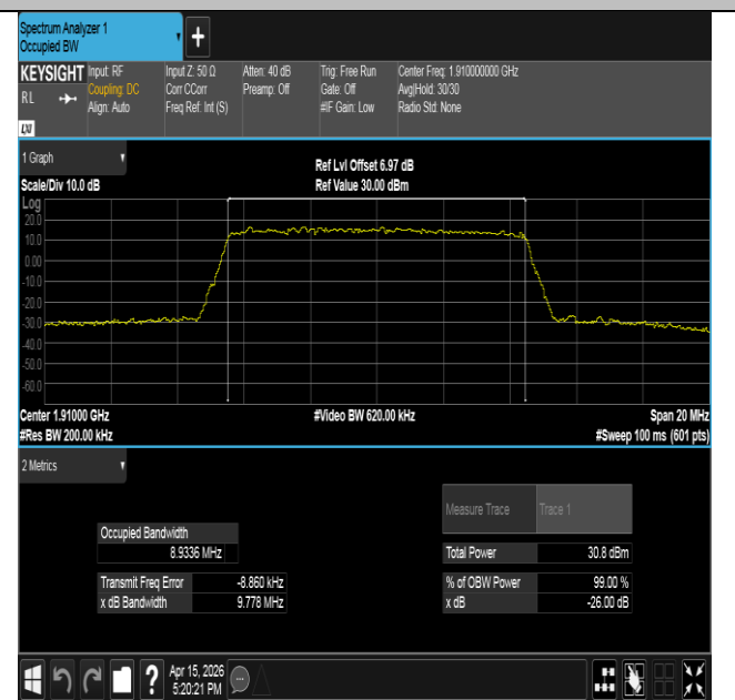
Band25-10MHz-16QAM-26640-50RB#0-PASS
