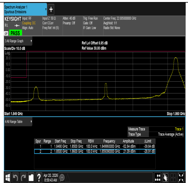
Band25-10MHz-QPSK-26090-1RB#49-PASS
