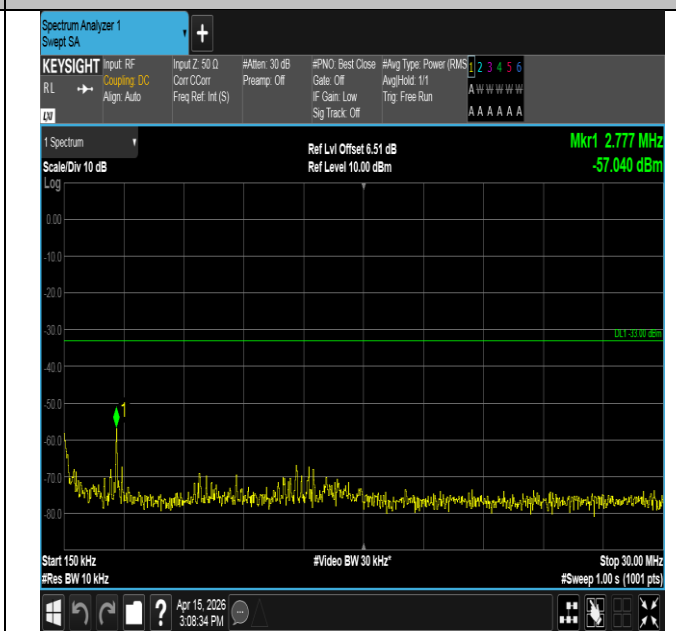
Band25-1.4MHz-QPSK-26047-6RB#0-0.15~30-PASS
