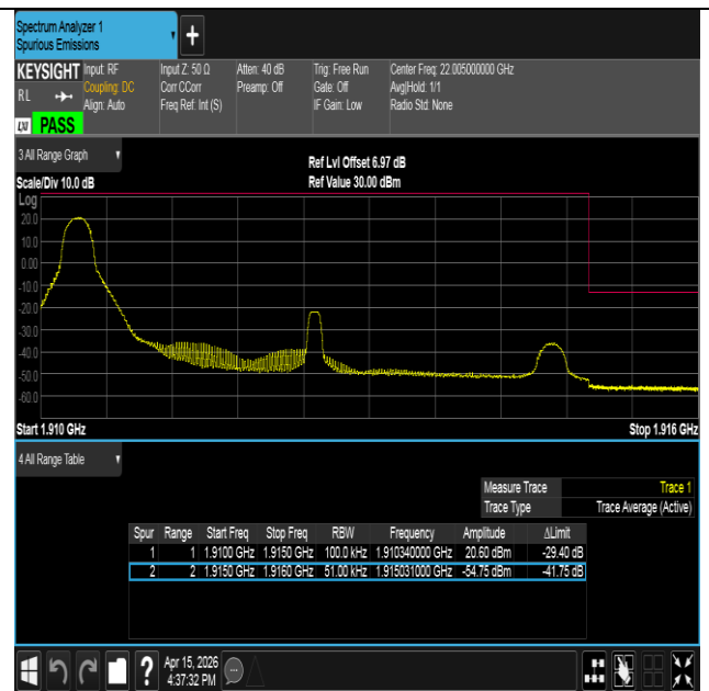
Band25-5MHz-16QAM-26665-1RB#0-PASS
