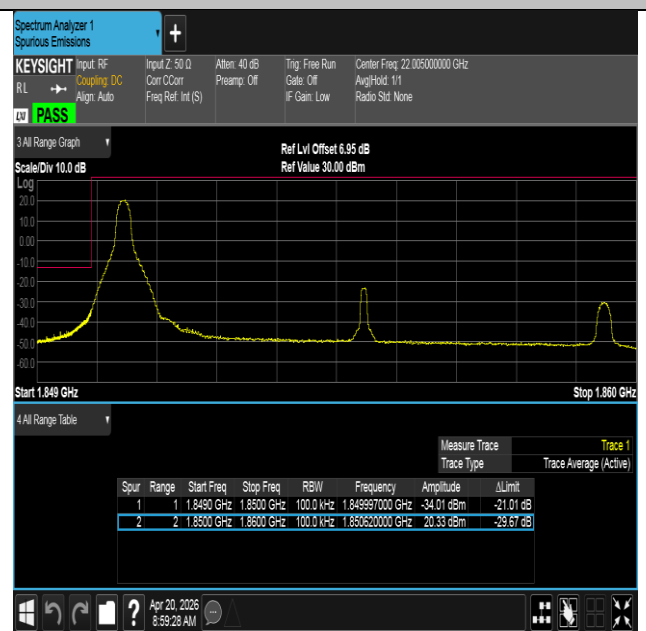
Band25-10MHz-16QAM-26090-1RB#0-PASS
