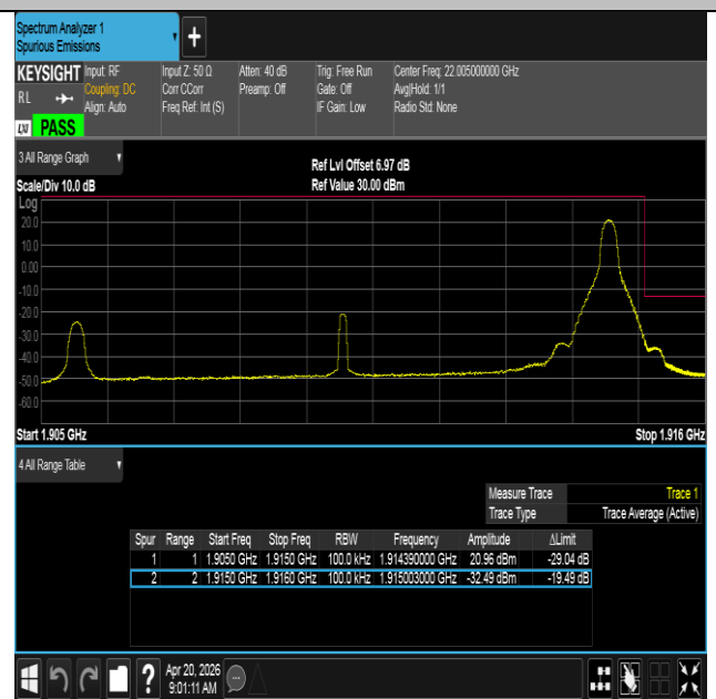
Band25-10MHz-QPSK-26640-1RB#49-PASS
