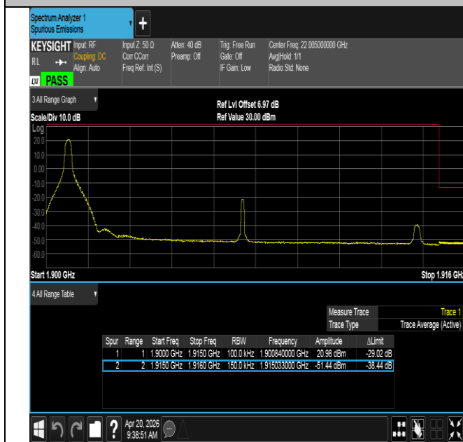
Band25-15MHz-QPSK-26615-1RB#0-PASS
