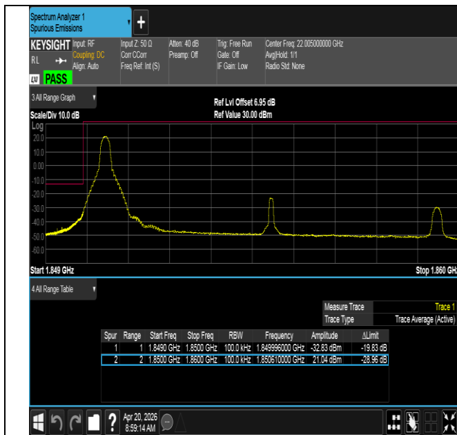
Band25-10MHz-QPSK-26090-1RB#0-PASS
