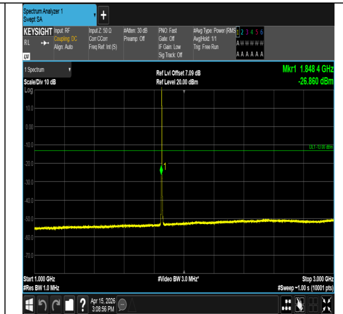
Band25-1.4MHz-QPSK-26047-6RB#0-1000~3000-PASS
