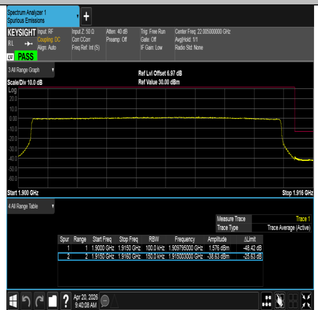
Band25-15MHz-16QAM-26615-75RB#0-PASS
