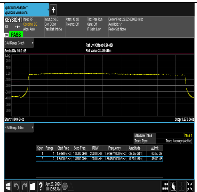
Band25-20MHz-16QAM-26140-100RB#0-PASS
