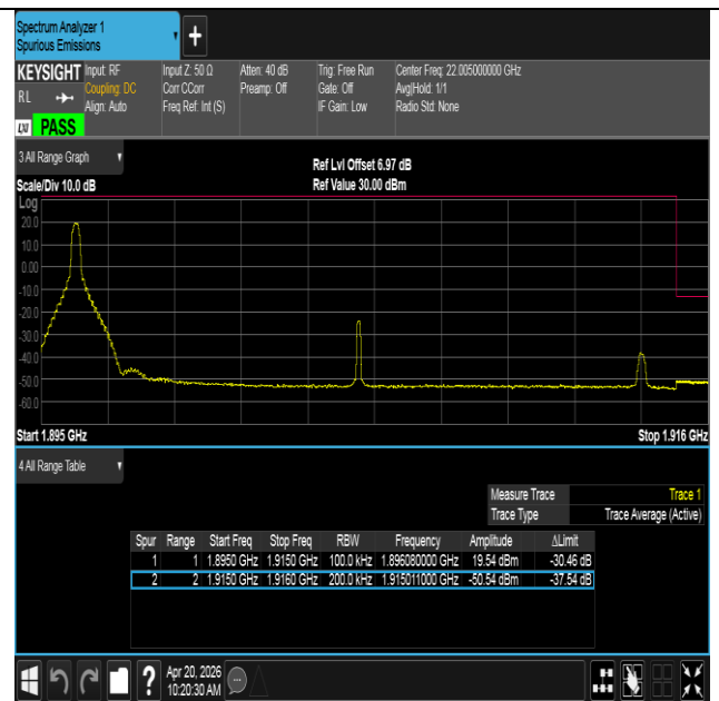
Band25-20MHz-16QAM-26590-1RB#0-PASS
