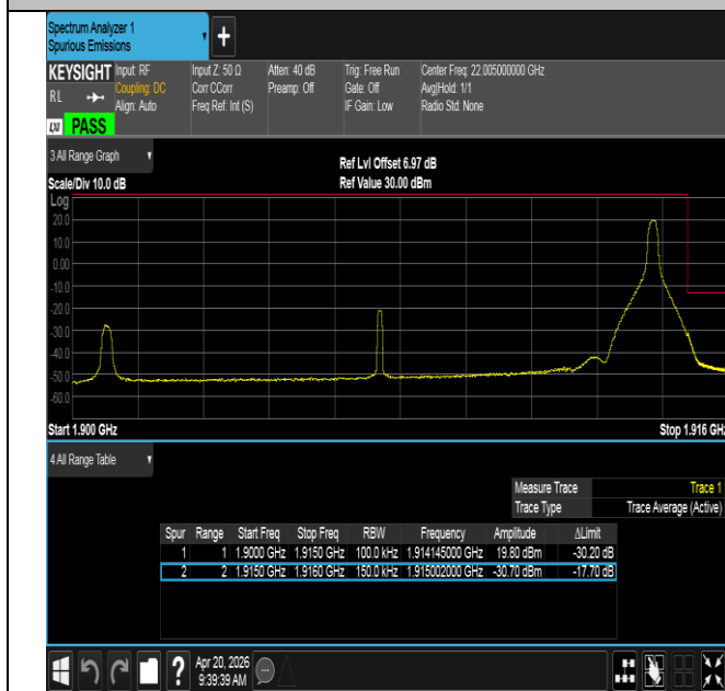
Band25-15MHz-16QAM-26615-1RB#74-PASS
