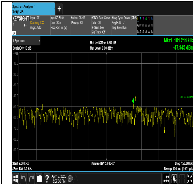
Band25-1.4MHz-16QAM-26047-1RB#5-0.009~0.15-PASS
