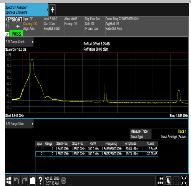
Band25-15MHz-16QAM-26115-1RB#0-PASS
