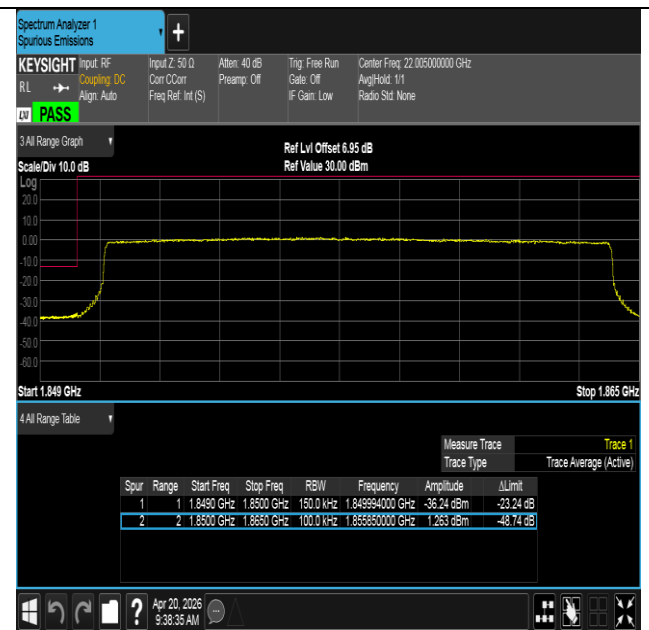
Band25-15MHz-16QAM-26115-75RB#0-PASS
