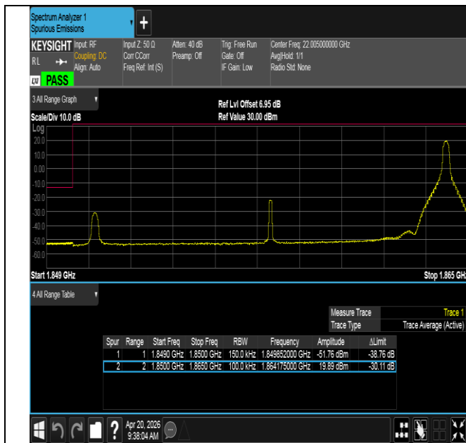
Band25-15MHz-16QAM-26115-1RB#74-PASS
