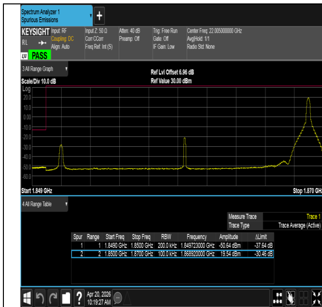
Band25-20MHz-16QAM-26140-1RB#99-PASS
