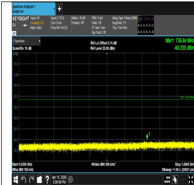
Band25-1.4MHz-QPSK-26047-6RB#0-30~1000-PASS
