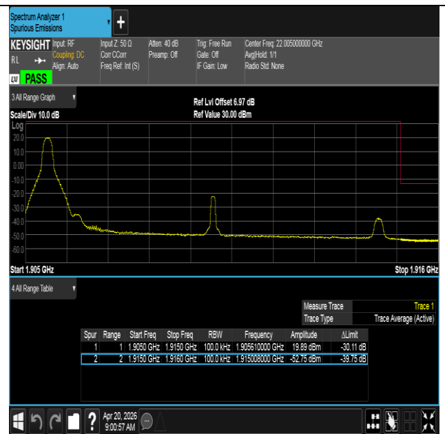
Band25-10MHz-16QAM-26640-1RB#0-PASS
