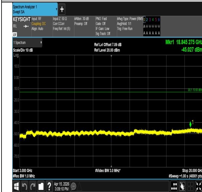
Band25-1.4MHz-QPSK-26047-6RB#0-3000~20000-PASS
