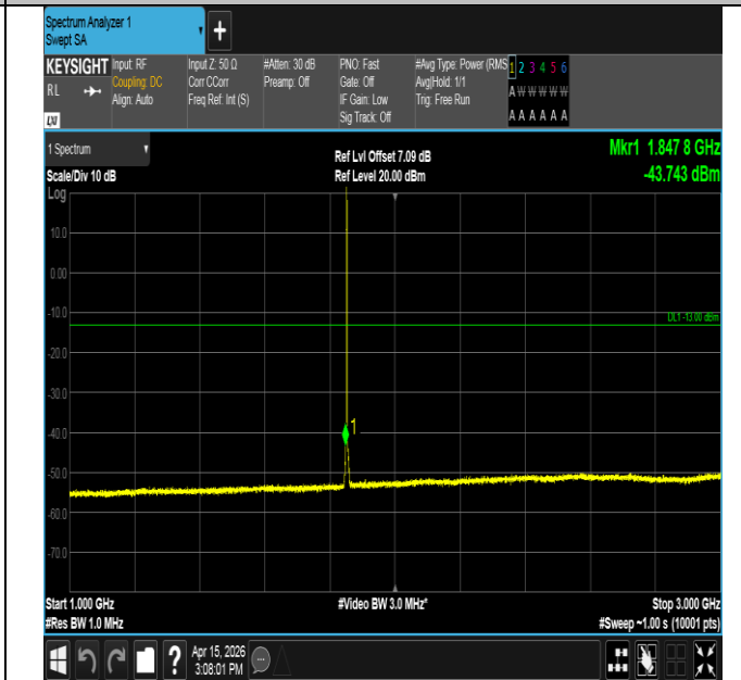
Band25-1.4MHz-16QAM-26047-1RB#5-1000~3000-PASS
