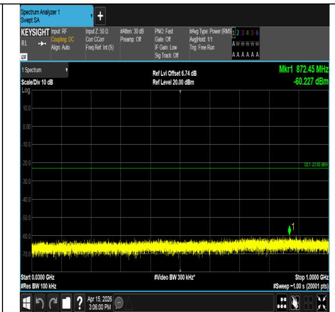
Band25-1.4MHz-16QAM-26047-1RB#0-30~1000-PASS
