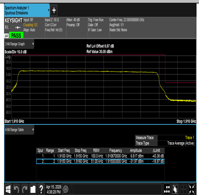
Band25-5MHz-16QAM-26665-25RB#0-PASS
