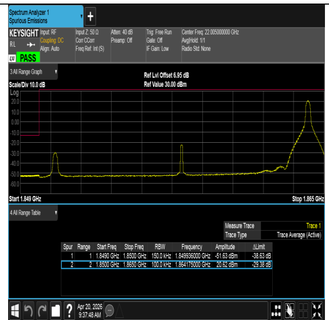
Band25-15MHz-QPSK-26115-1RB#74-PASS
