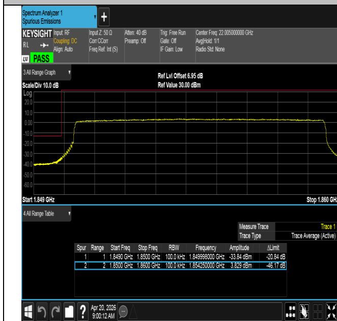
Band25-10MHz-QPSK-26090-50RB#0-PASS
