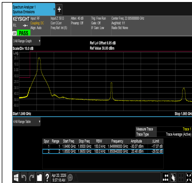
Band25-15MHz-QPSK-26115-1RB#0-PASS
