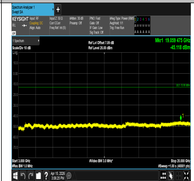
Band25-1.4MHz-16QAM-26047-1RB#0-3000~20000-PASS
