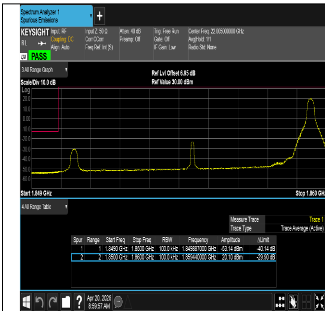
Band25-10MHz-16QAM-26090-1RB#49-PASS
