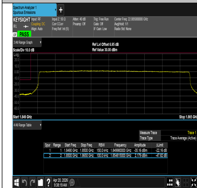
Band25-15MHz-QPSK-26115-75RB#0-PASS
