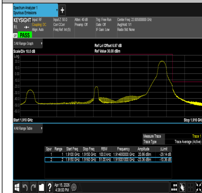
Band25-5MHz-16QAM-26665-1RB#24-PASS
