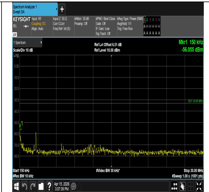
Band25-1.4MHz-16QAM-26047-1RB#5-0.15~30-PASS
