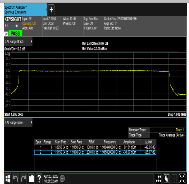
Band25-20MHz-16QAM-26590-100RB#0-PASS
