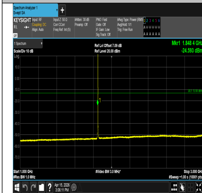
Band25-1.4MHz-16QAM-26047-1RB#0-1000~3000-PASS
