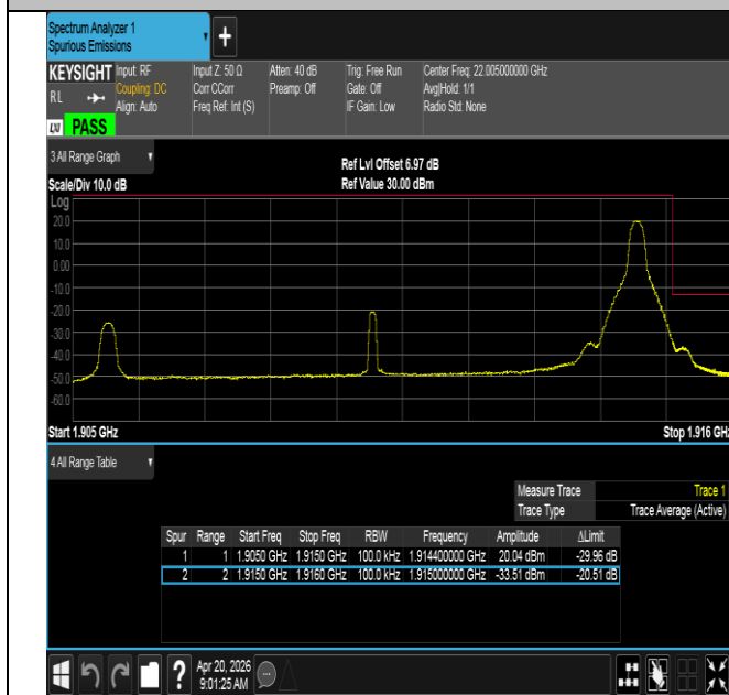
Band25-10MHz-16QAM-26640-1RB#49-PASS
