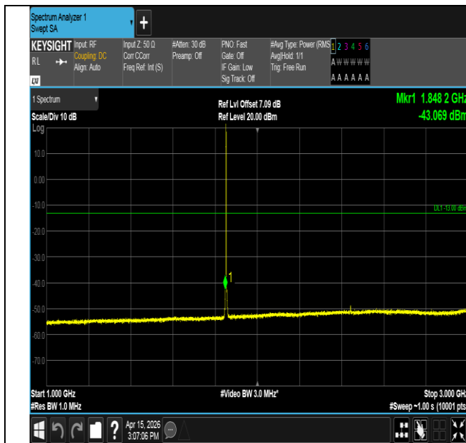
Band25-1.4MHz-QPSK-26047-1RB#5-1000~3000-PASS
