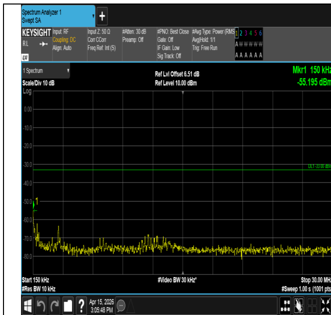
Band25-1.4MHz-16QAM-26047-1RB#0-0.15~30-PASS
