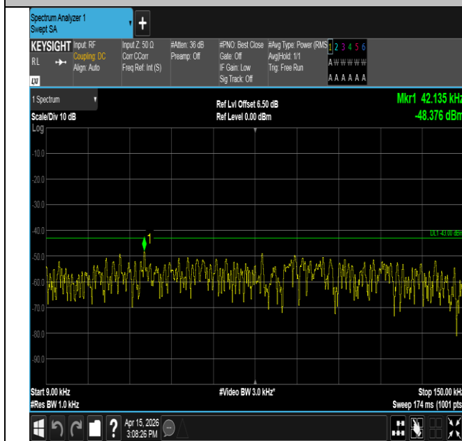
Band25-1.4MHz-QPSK-26047-6RB#0-0.009~0.15-PASS
