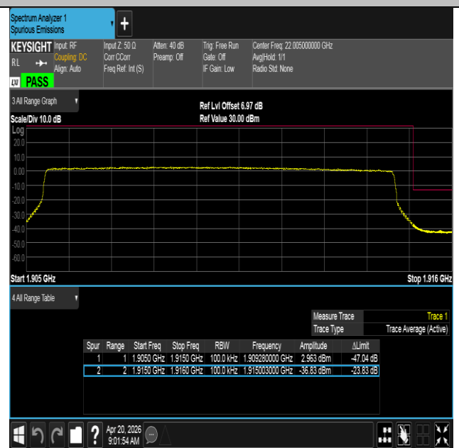
Band25-10MHz-16QAM-26640-50RB#0-PASS
