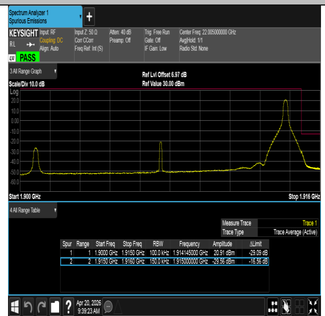
Band25-15MHz-QPSK-26615-1RB#74-PASS
