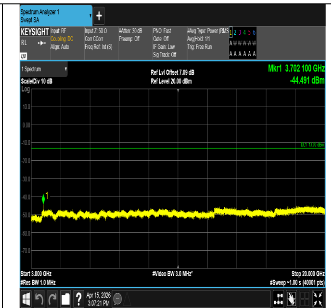
Band25-1.4MHz-QPSK-26047-1RB#5-3000~20000-PASS
