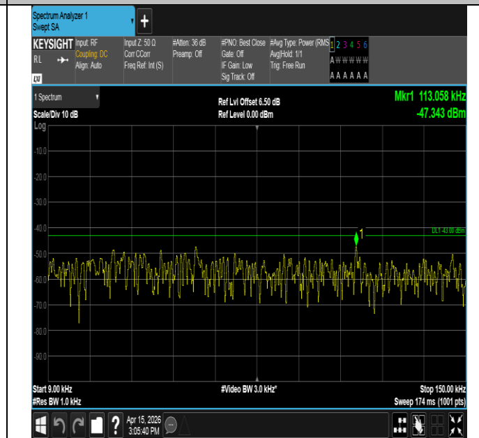
Band25-1.4MHz-16QAM-26047-1RB#0-0.009~0.15-PASS
