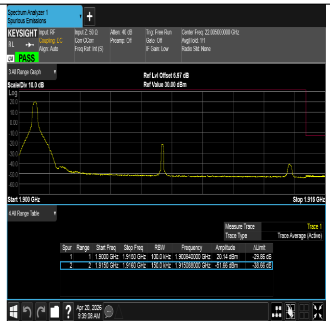
Band25-15MHz-16QAM-26615-1RB#0-PASS
