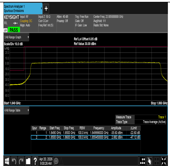
Band25-10MHz-16QAM-26090-50RB#0-PASS
