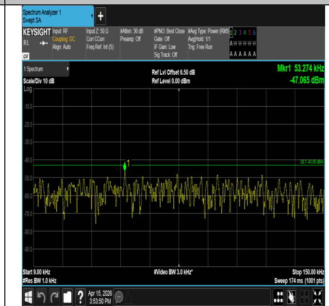
Band25-3MHz-QPSK-26055-1RB#14-0.009~0.15-PASS
