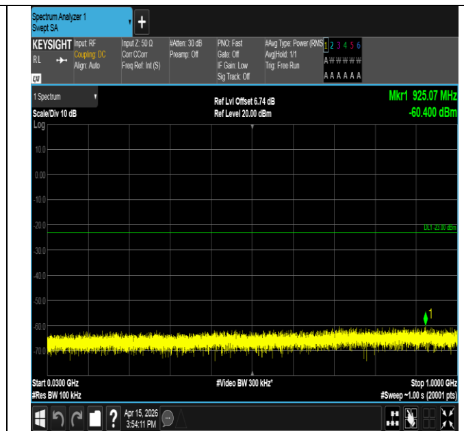
Band25-3MHz-QPSK-26055-1RB#14-30~1000-PASS
