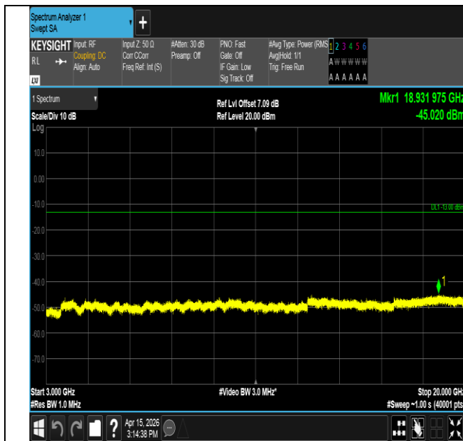
Band25-1.4MHz-QPSK-26365-6RB#0-3000~20000-PASS
