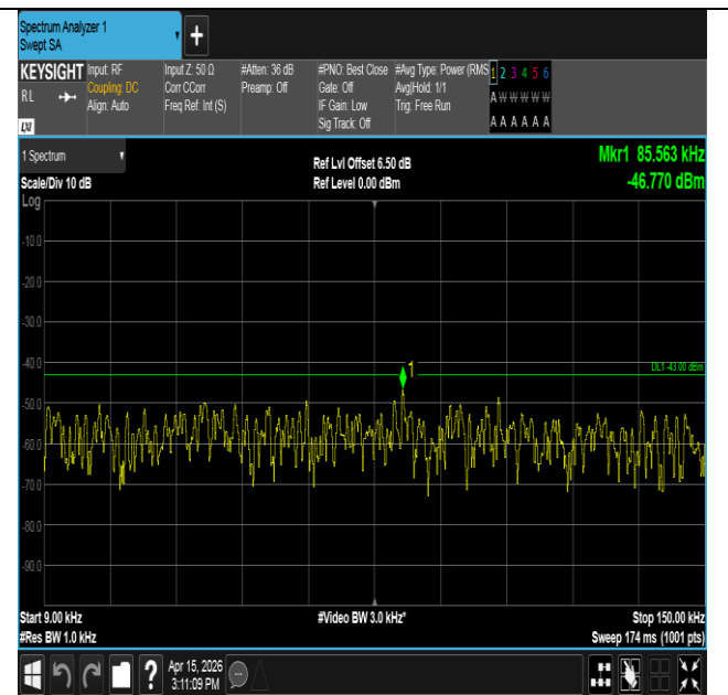
Band25-1.4MHz-16QAM-26365-1RB#0-0.009~0.15-PASS
