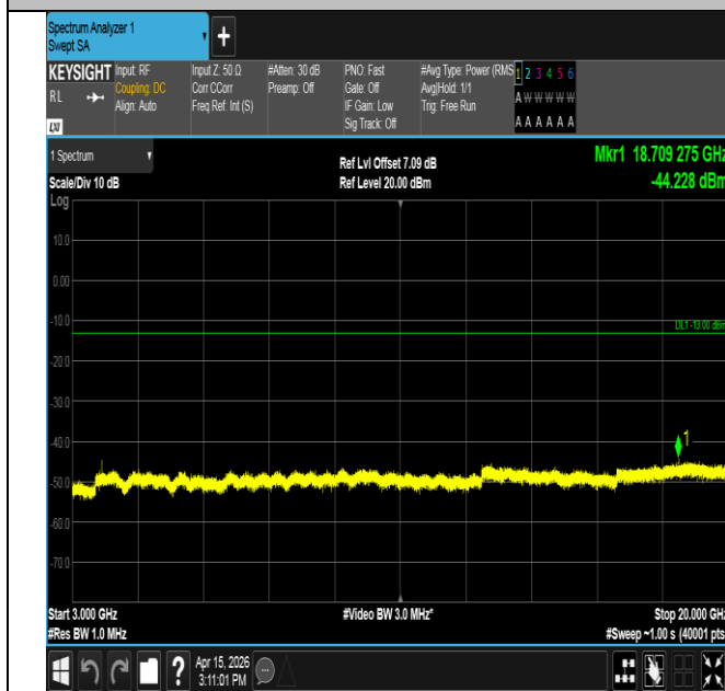
Band25-1.4MHz-QPSK-26365-1RB#0-3000~20000-PASS
