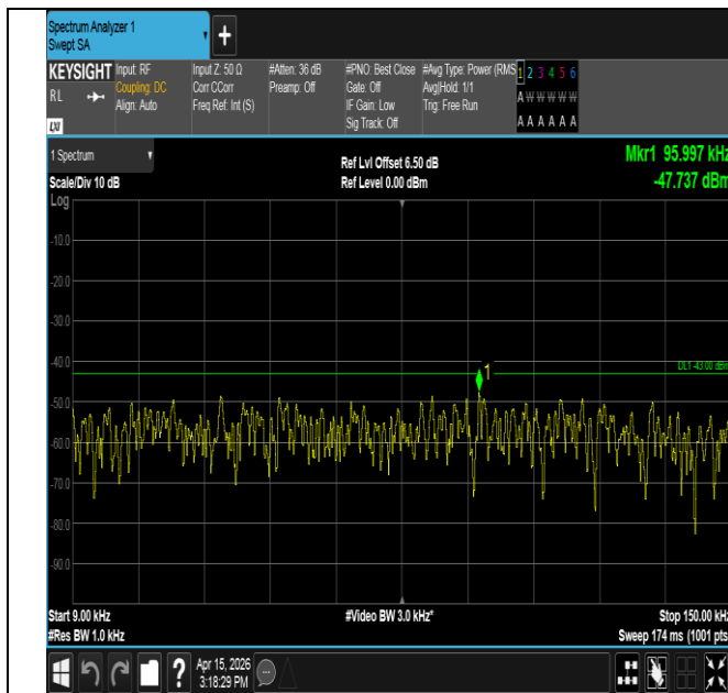
Band25-1.4MHz-16QAM-26683-1RB#5-0.009~0.15-PASS
