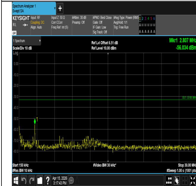
Band25-1.4MHz-QPSK-26683-1RB#5-0.15~30-PASS
