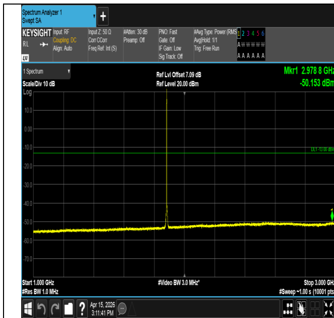
Band25-1.4MHz-16QAM-26365-1RB#0-1000~3000-PASS
