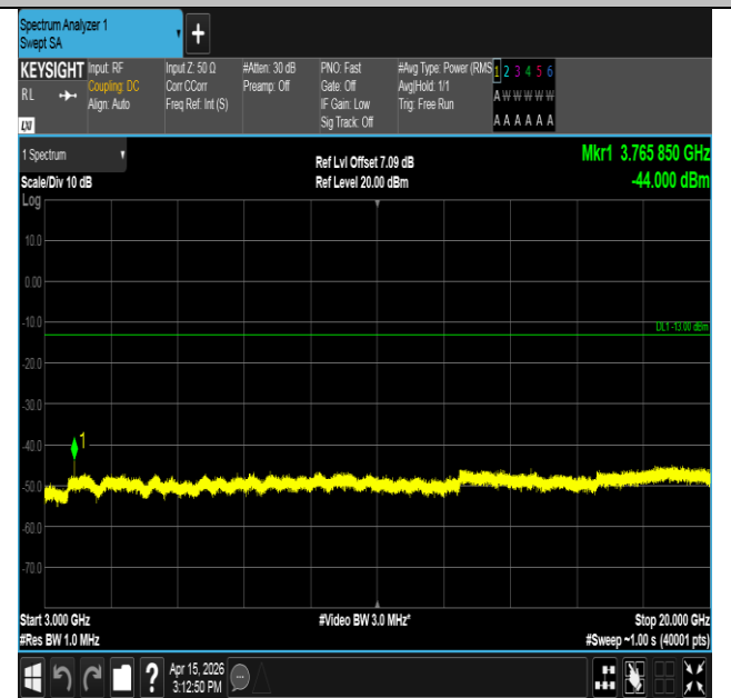
Band25-1.4MHz-QPSK-26365-1RB#5-3000~20000-PASS
