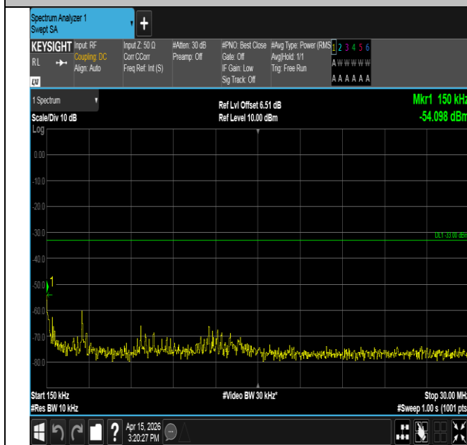
Band25-1.4MHz-16QAM-26683-6RB#0-0.15~30-PASS
