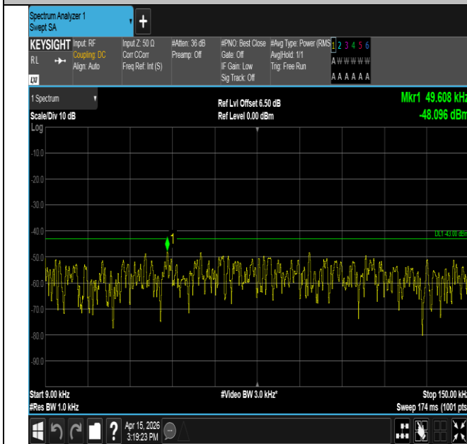
Band25-1.4MHz-QPSK-26683-6RB#0-0.009~0.15-PASS
