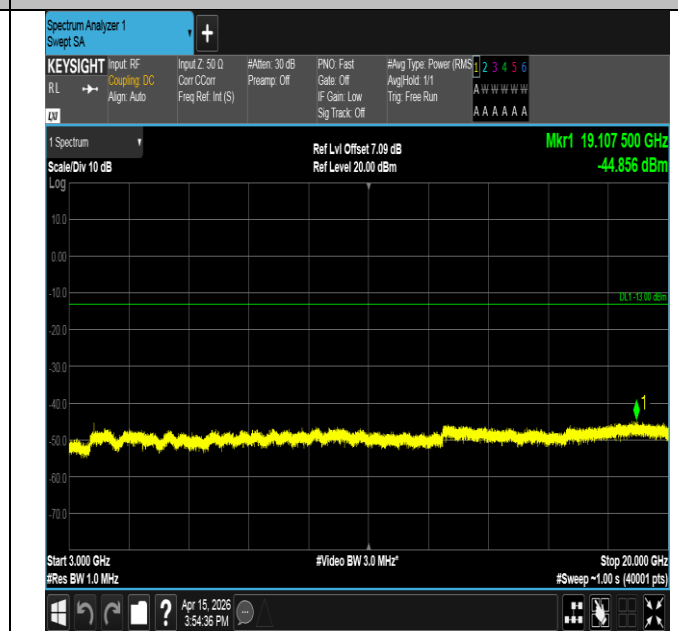
Band25-3MHz-QPSK-26055-1RB#14-3000~20000-PASS
