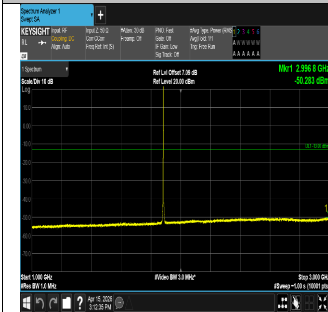
Band25-1.4MHz-QPSK-26365-1RB#5-1000~3000-PASS
