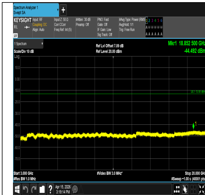
Band25-1.4MHz-16QAM-26683-1RB#5-3000~20000-PASS
