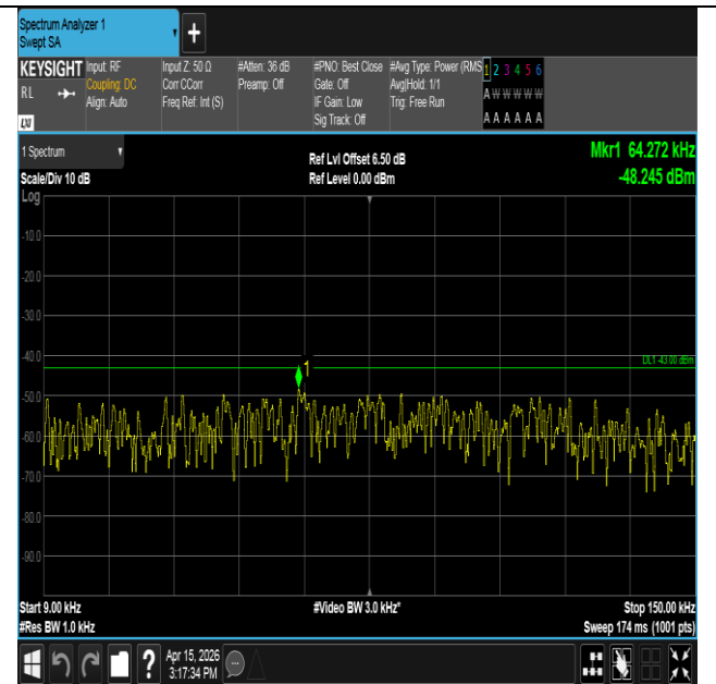
Band25-1.4MHz-QPSK-26683-1RB#5-0.009~0.15-PASS
