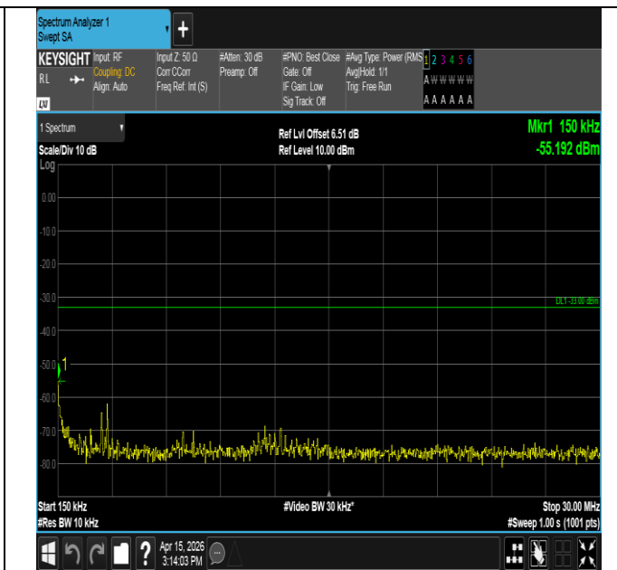
Band25-1.4MHz-QPSK-26365-6RB#0-0.15~30-PASS
