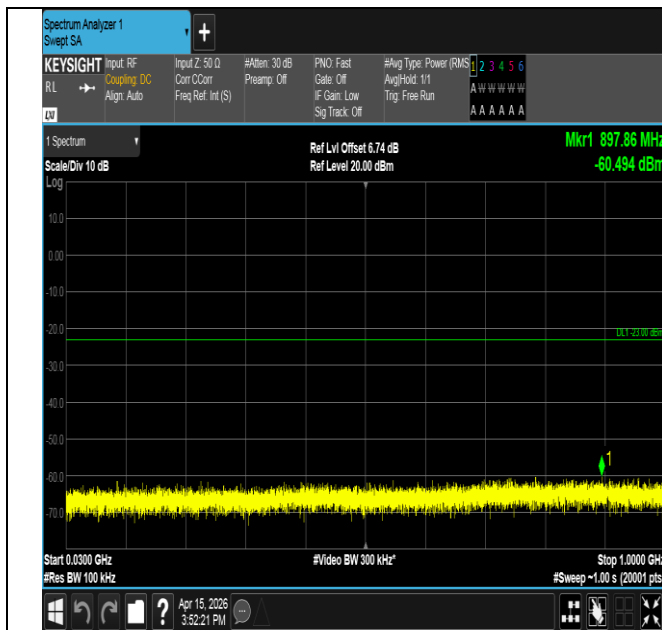
Band25-3MHz-QPSK-26055-1RB#0-30~1000-PASS
