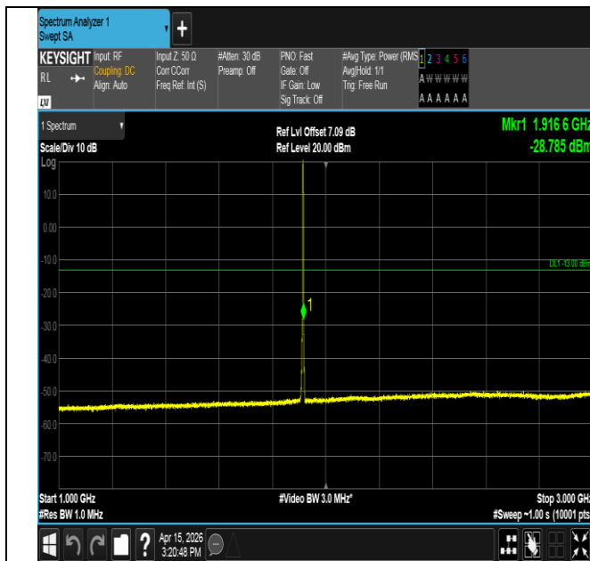
Band25-1.4MHz-16QAM-26683-6RB#0-1000~3000-PASS
