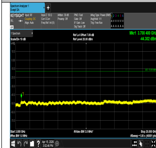
Band25-3MHz-QPSK-26055-1RB#0-3000~20000-PASS
