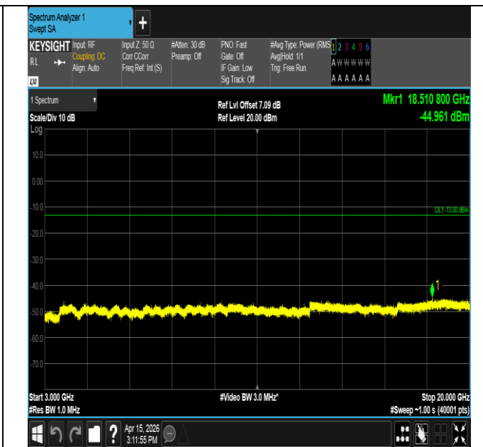
Band25-1.4MHz-16QAM-26365-1RB#0-3000~20000-PASS
