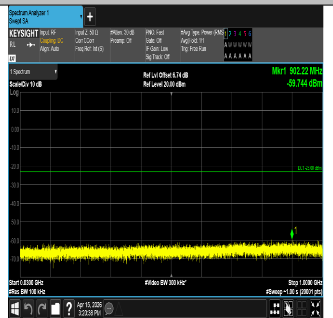
Band25-1.4MHz-16QAM-26683-6RB#0-30~1000-PASS
