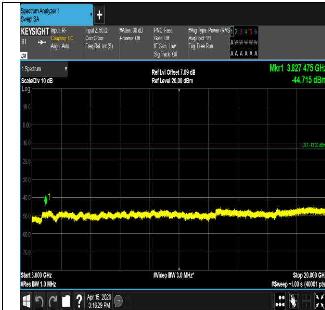
Band25-1.4MHz-QPSK-26683-1RB#0-3000~20000-PASS
