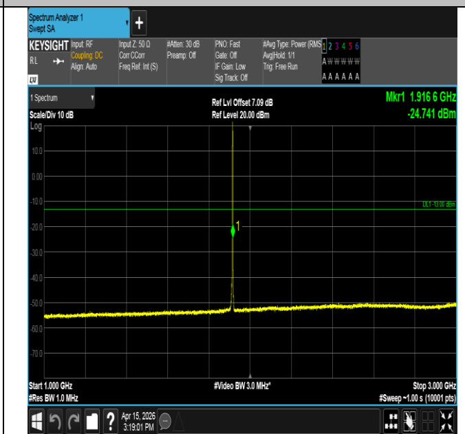
Band25-1.4MHz-16QAM-26683-1RB#5-1000~3000-PASS
