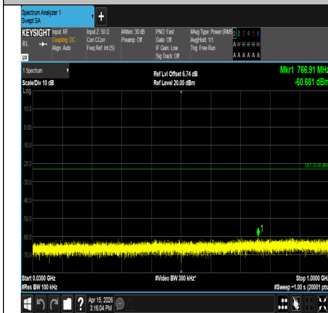
Band25-1.4MHz-QPSK-26683-1RB#0-30~1000-PASS
