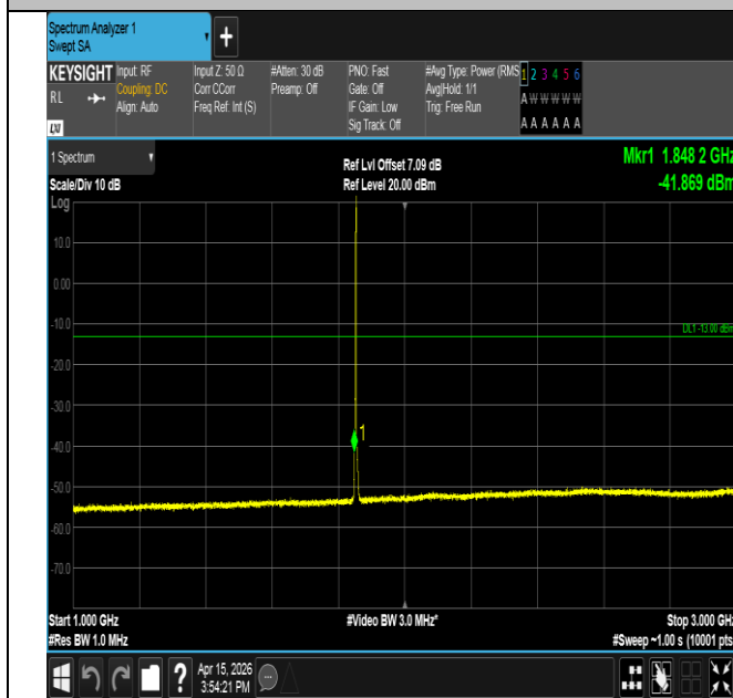
Band25-3MHz-QPSK-26055-1RB#14-1000~3000-PASS
