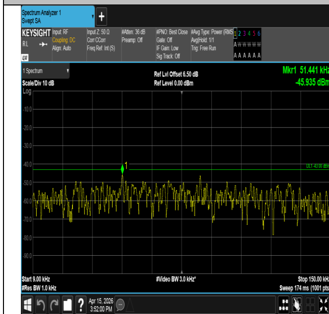
Band25-3MHz-QPSK-26055-1RB#0-0.009~0.15-PASS
