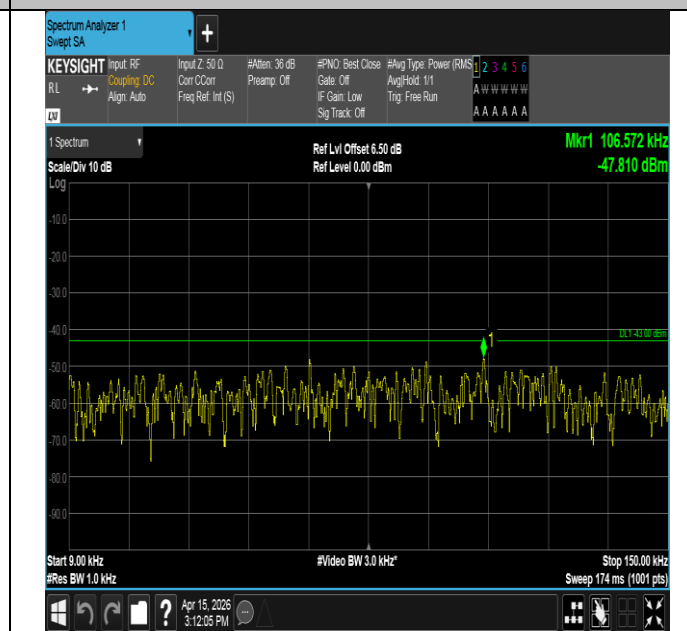
Band25-1.4MHz-QPSK-26365-1RB#5-0.009~0.15-PASS
