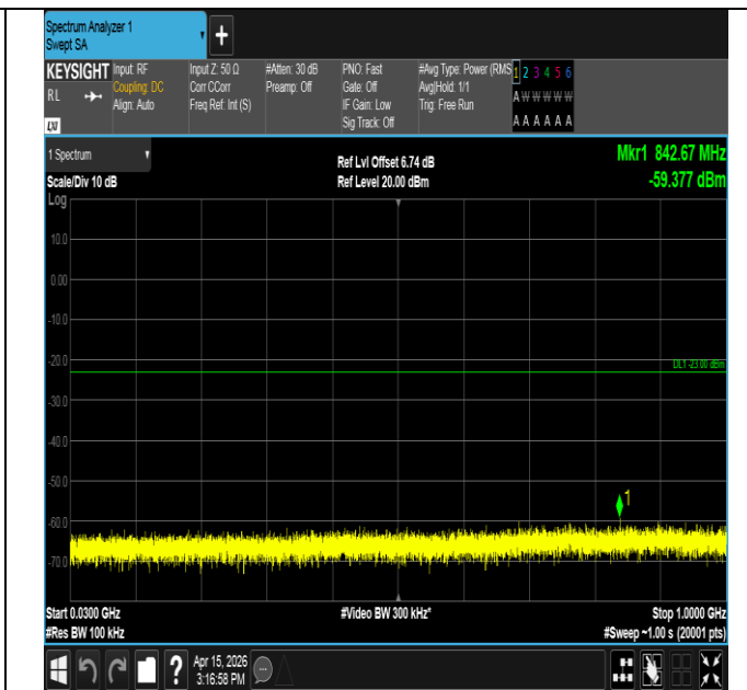
Band25-1.4MHz-16QAM-26683-1RB#0-30~1000-PASS
