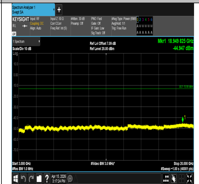
Band25-1.4MHz-16QAM-26683-1RB#0-3000~20000-PASS
