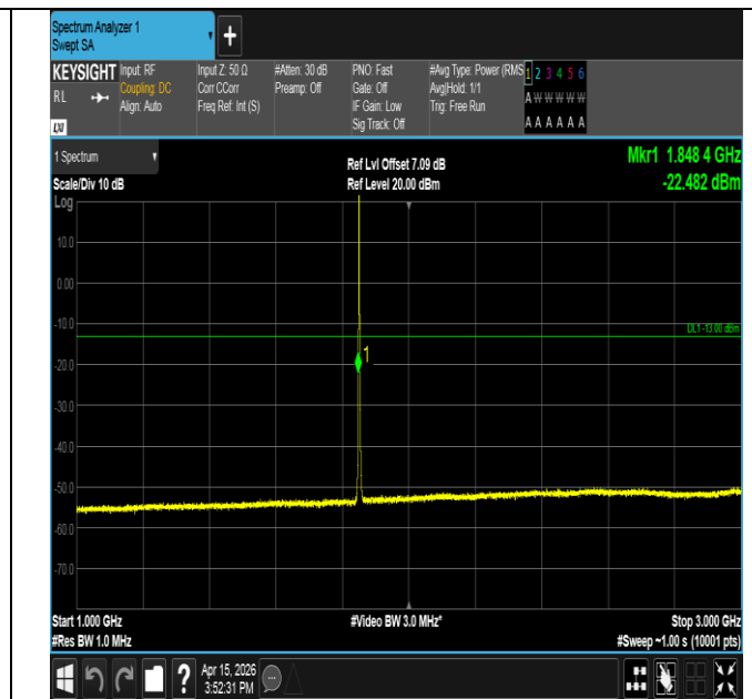
Band25-3MHz-QPSK-26055-1RB#0-1000~3000-PASS
