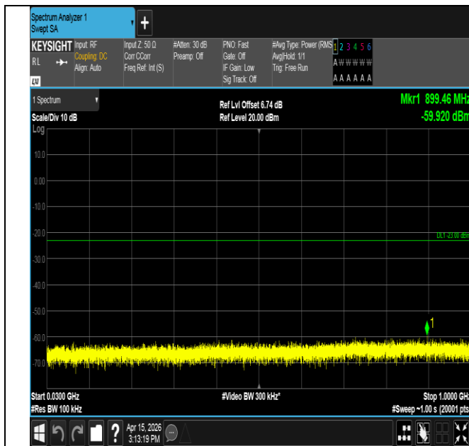
Band25-1.4MHz-16QAM-26365-1RB#5-30~1000-PASS
