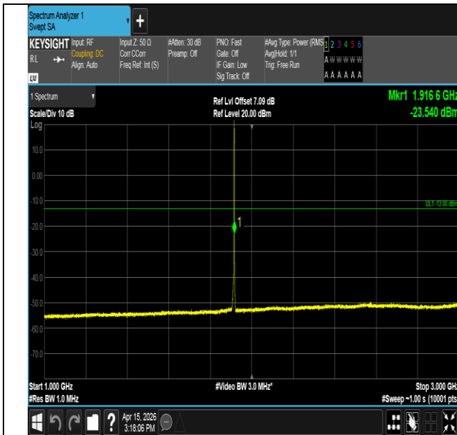
Band25-1.4MHz-QPSK-26683-1RB#5-1000~3000-PASS
