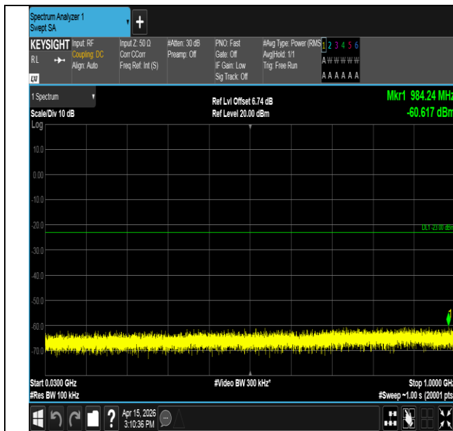
Band25-1.4MHz-QPSK-26365-1RB#0-30~1000-PASS
