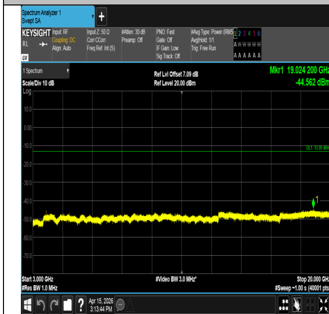
Band25-1.4MHz-16QAM-26365-1RB#5-3000~20000-PASS
