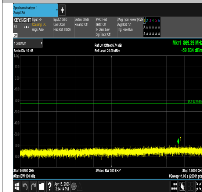
Band25-1.4MHz-QPSK-26365-6RB#0-30~1000-PASS
