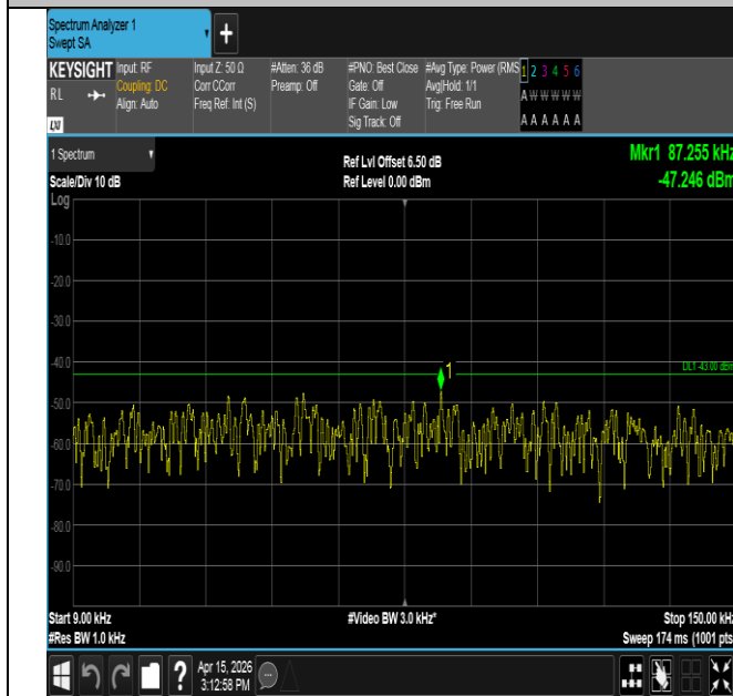
Band25-1.4MHz-16QAM-26365-1RB#5-0.009~0.15-PASS
