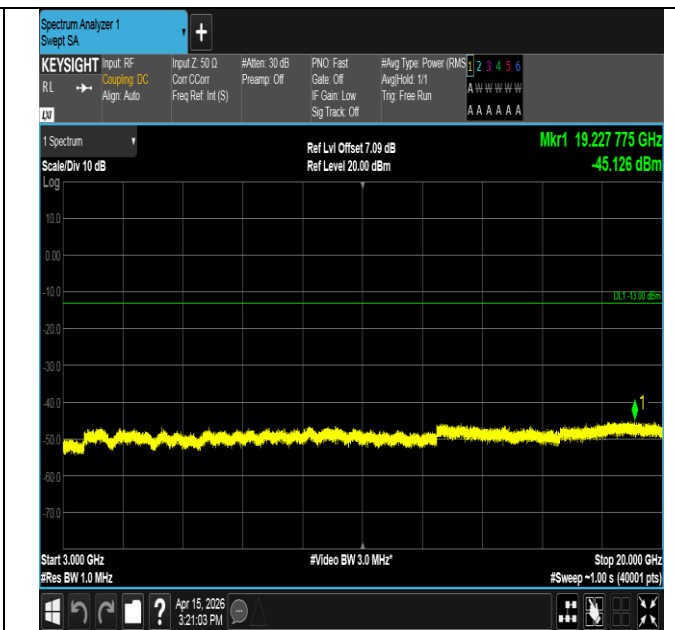
Band25-1.4MHz-16QAM-26683-6RB#0-3000~20000-PASS
