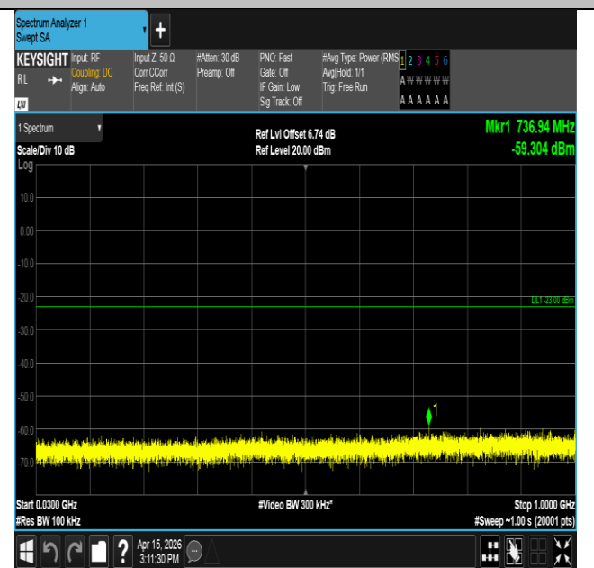
Band25-1.4MHz-16QAM-26365-1RB#0-30~1000-PASS
