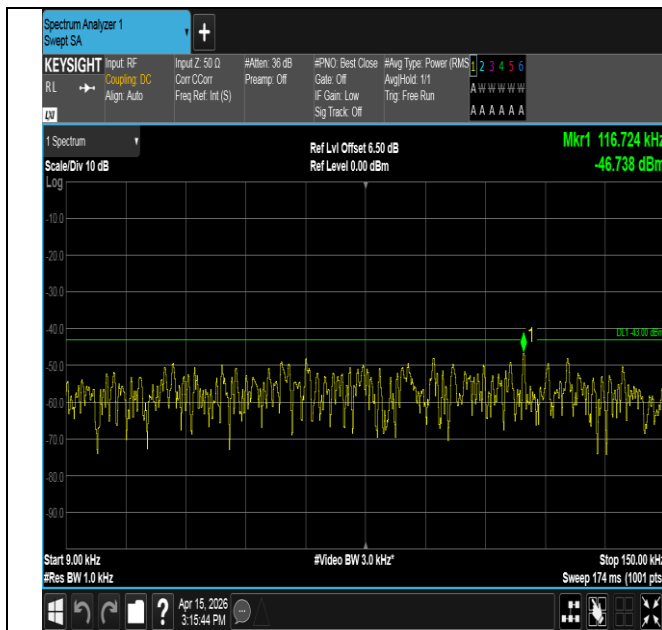
Band25-1.4MHz-QPSK-26683-1RB#0-0.009~0.15-PASS
