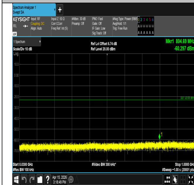
Band25-1.4MHz-16QAM-26683-1RB#5-30~1000-PASS
