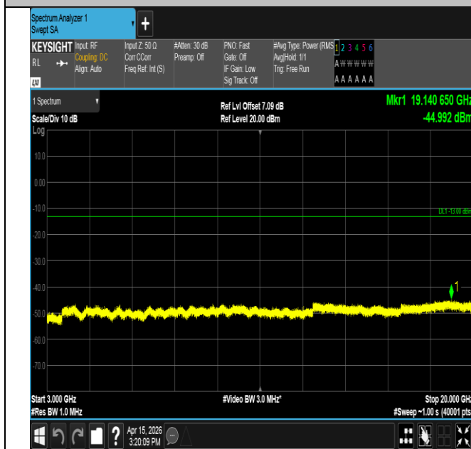
Band25-1.4MHz-QPSK-26683-6RB#0-3000~20000-PASS
