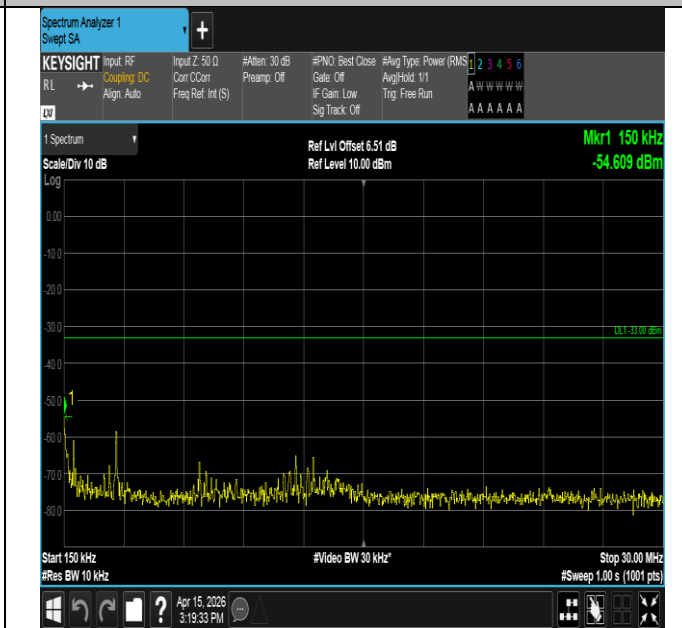
Band25-1.4MHz-QPSK-26683-6RB#0-0.15~30-PASS
