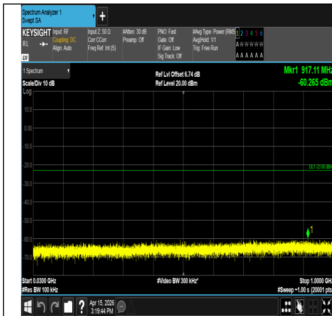
Band25-1.4MHz-QPSK-26683-6RB#0-30~1000-PASS
