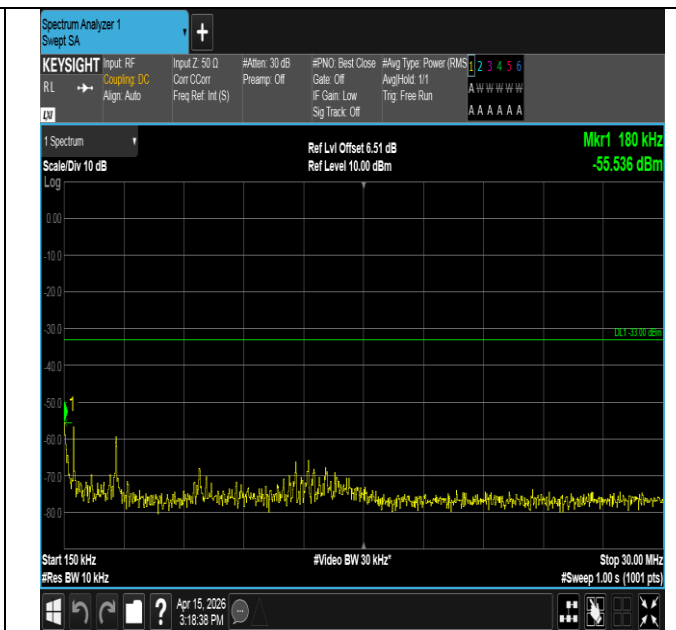
Band25-1.4MHz-16QAM-26683-1RB#5-0.15~30-PASS
