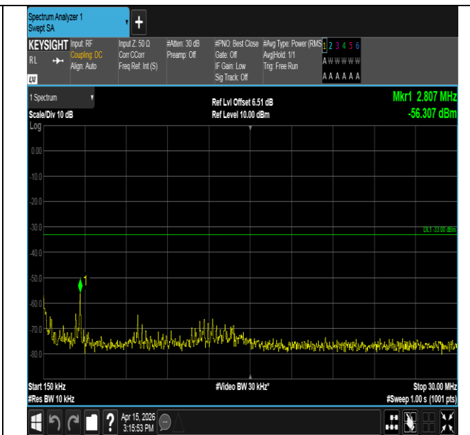
Band25-1.4MHz-QPSK-26683-1RB#0-0.15~30-PASS
