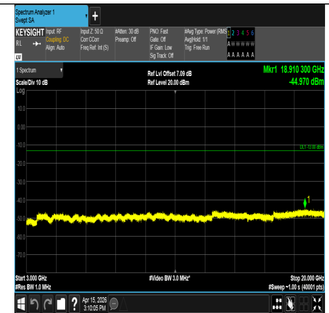
Band25-1.4MHz-16QAM-26047-6RB#0-3000~20000-PASS
