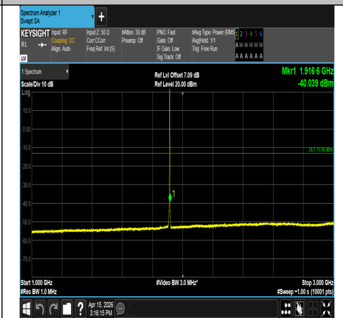
Band25-1.4MHz-QPSK-26683-1RB#0-1000~3000-PASS
