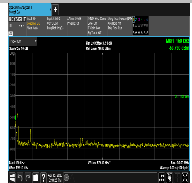
Band25-1.4MHz-QPSK-26365-1RB#0-0.15~30-PASS
