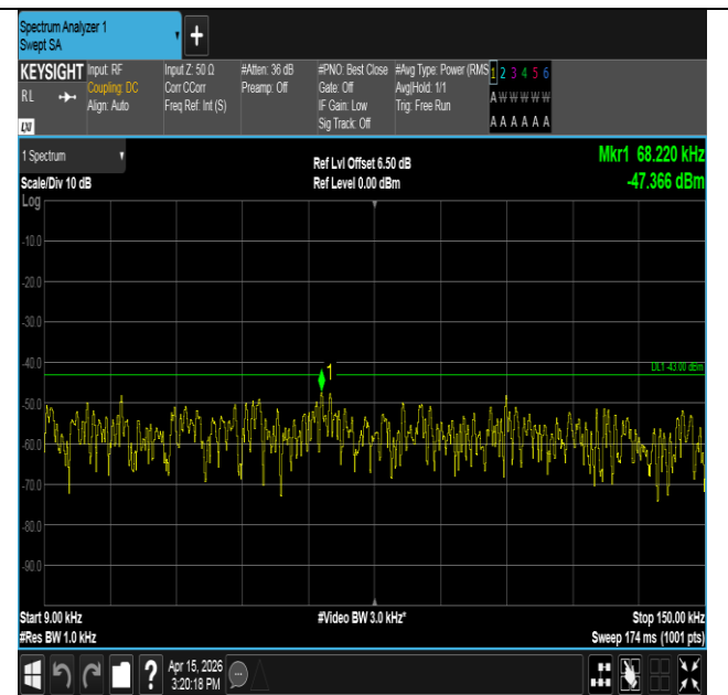
Band25-1.4MHz-16QAM-26683-6RB#0-0.009~0.15-PASS
