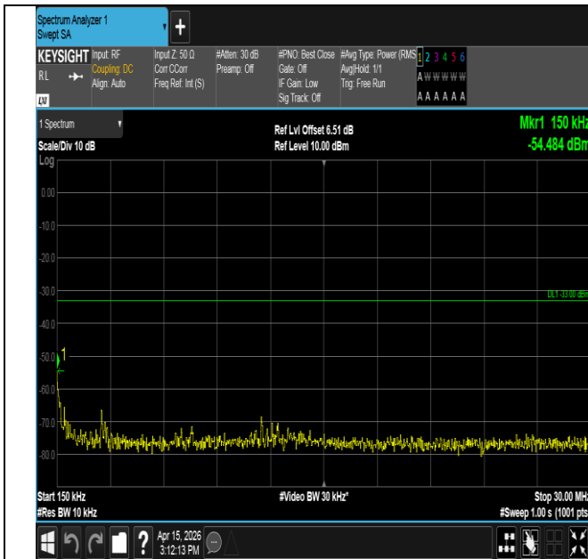
Band25-1.4MHz-QPSK-26365-1RB#5-0.15~30-PASS
