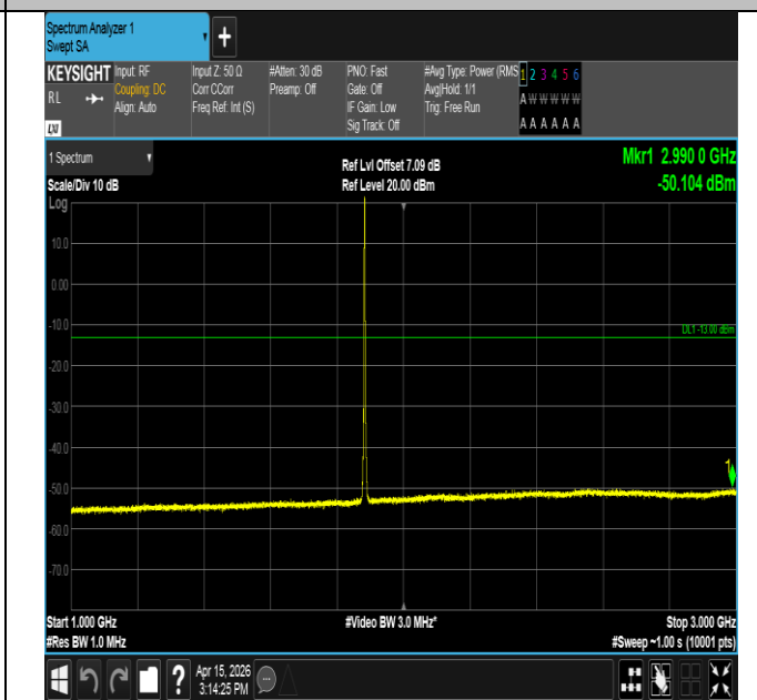
Band25-1.4MHz-QPSK-26365-6RB#0-1000~3000-PASS
