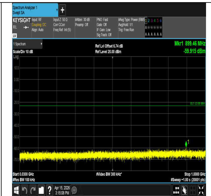
Band25-1.4MHz-16QAM-26365-6RB#0-30~1000-PASS
