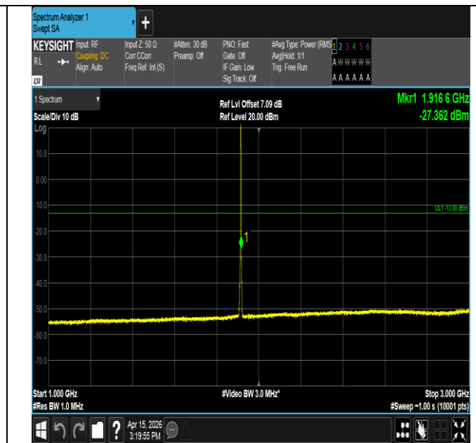
Band25-1.4MHz-QPSK-26683-6RB#0-1000~3000-PASS
