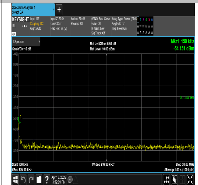
Band25-3MHz-QPSK-26055-1RB#0-0.15~30-PASS
