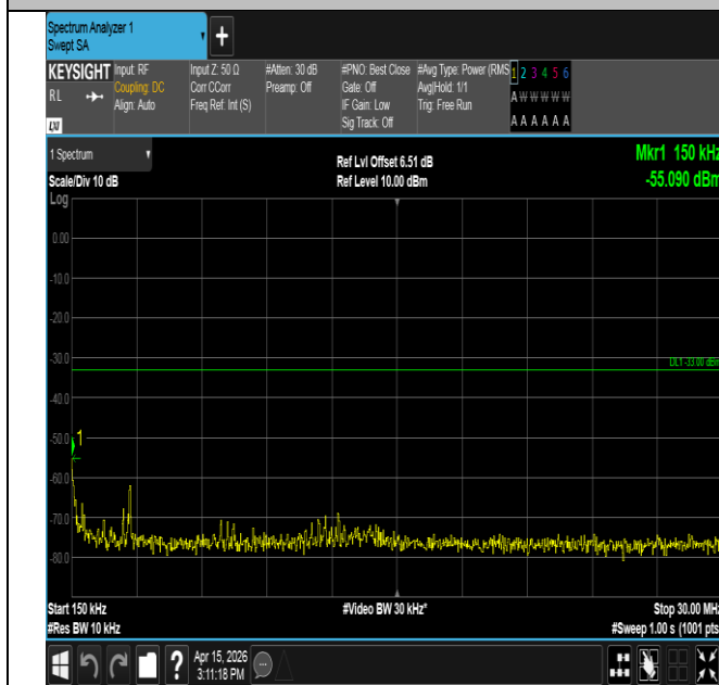
Band25-1.4MHz-16QAM-26365-1RB#0-0.15~30-PASS
