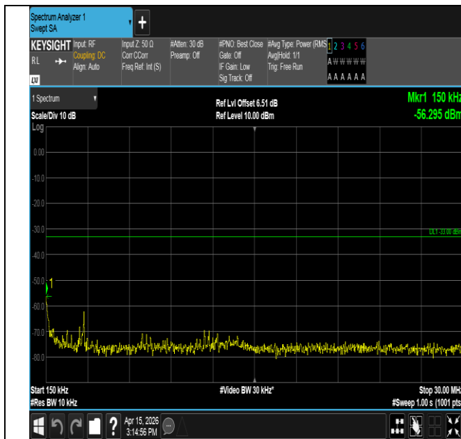
Band25-1.4MHz-16QAM-26365-6RB#0-0.15~30-PASS
