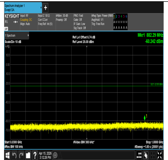
Band25-1.4MHz-QPSK-26365-1RB#5-30~1000-PASS
