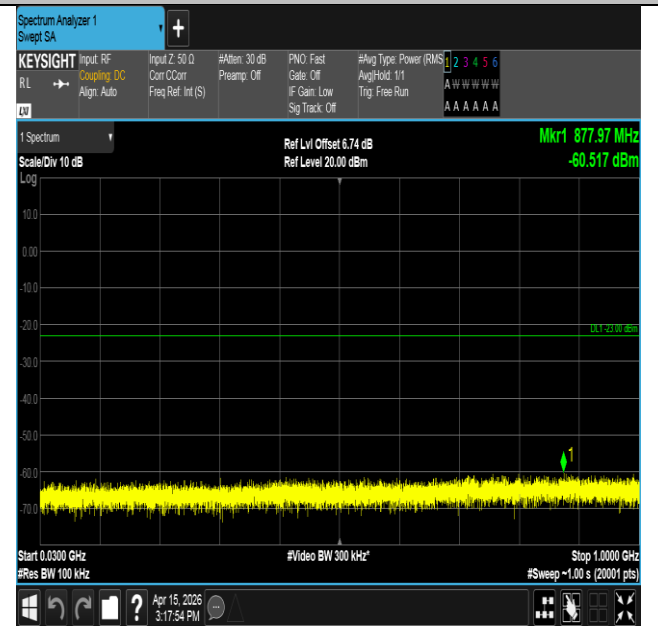
Band25-1.4MHz-QPSK-26683-1RB#5-30~1000-PASS
