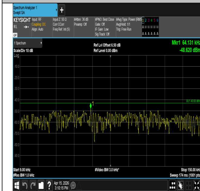
Band25-1.4MHz-QPSK-26365-1RB#0-0.009~0.15-PASS
