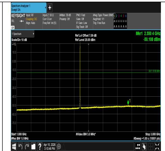
Band25-1.4MHz-QPSK-26365-1RB#0-1000~3000-PASS
