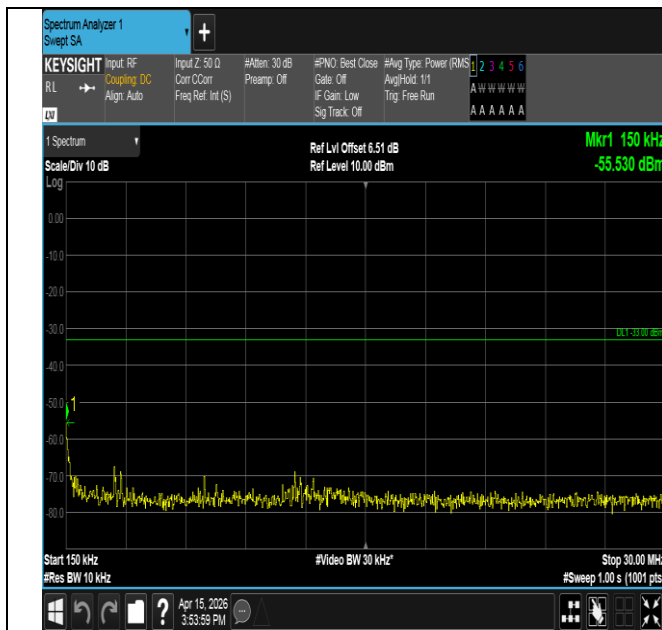
Band25-3MHz-QPSK-26055-1RB#14-0.15~30-PASS
