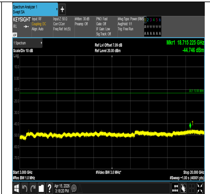
Band25-1.4MHz-QPSK-26683-1RB#5-3000~20000-PASS
