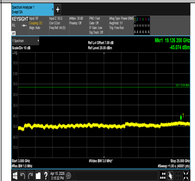
Band25-1.4MHz-16QAM-26365-6RB#0-3000~20000-PASS
