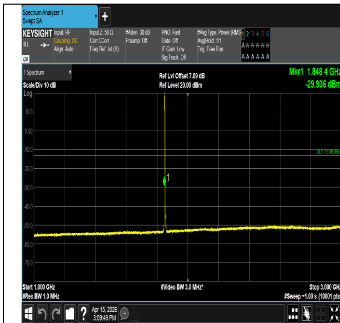
Band25-1.4MHz-16QAM-26047-6RB#0-1000~3000-PASS
