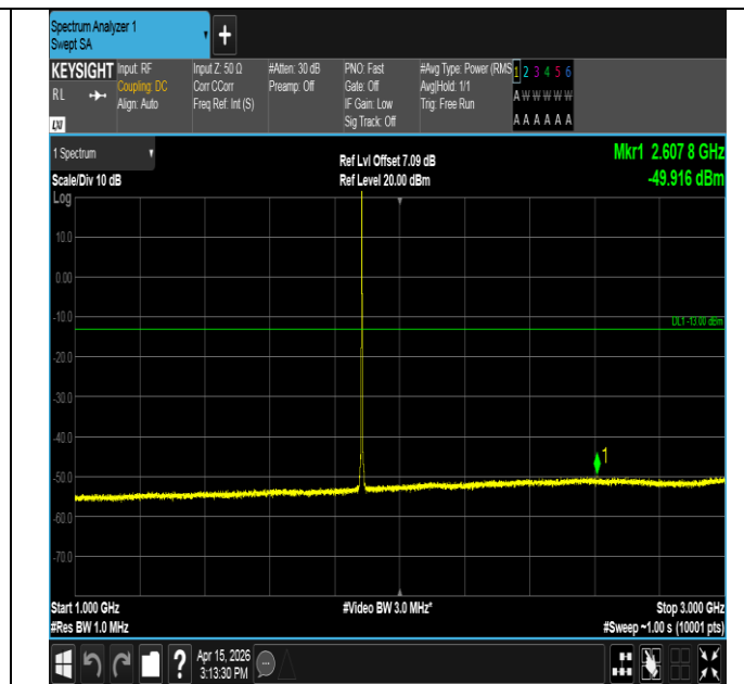
Band25-1.4MHz-16QAM-26365-1RB#5-1000~3000-PASS
