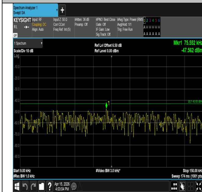
Band25-3MHz-QPSK-26675-1RB#0-0.009~0.15-PASS
