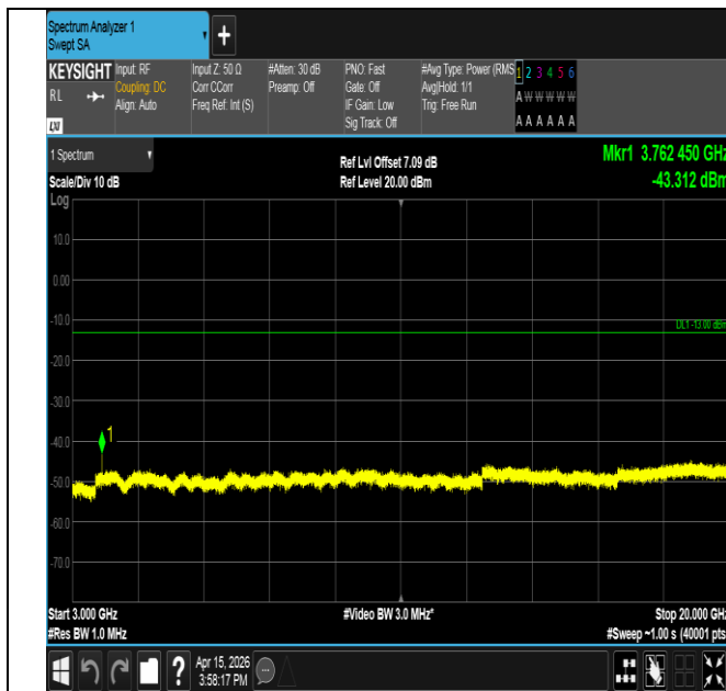
Band25-3MHz-QPSK-26365-1RB#0-3000~20000-PASS
