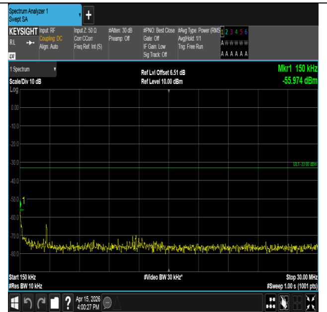
Band25-3MHz-16QAM-26365-1RB#14-0.15~30-PASS
