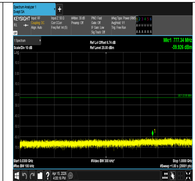
Band25-3MHz-QPSK-26675-1RB#14-30~1000-PASS
