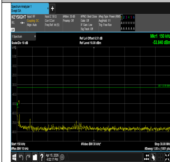
Band25-3MHz-16QAM-26365-15RB#0-0.15~30-PASS
