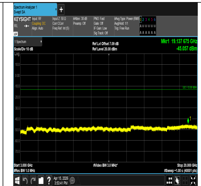
Band25-3MHz-16QAM-26055-1RB#0-3000~20000-PASS
