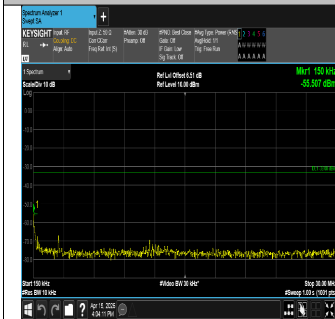
Band25-3MHz-16QAM-26675-1RB#0-0.15~30-PASS
