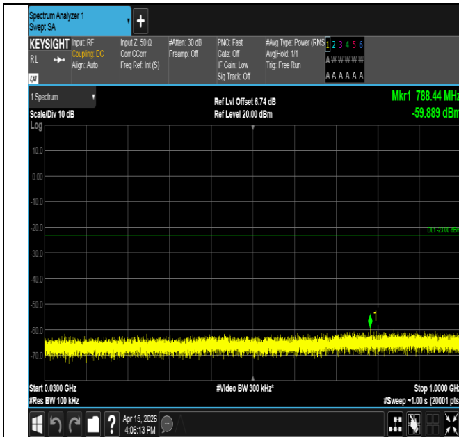
Band25-3MHz-16QAM-26675-1RB#14-30~1000-PASS
