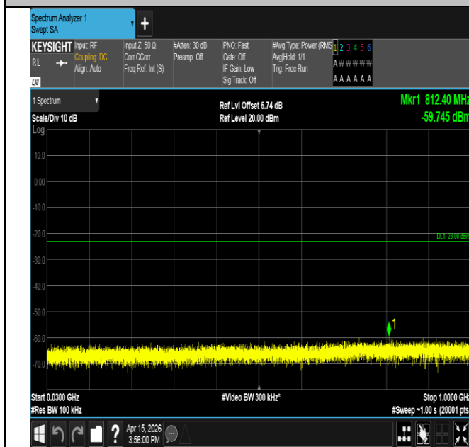
Band25-3MHz-QPSK-26055-15RB#0-30~1000-PASS
