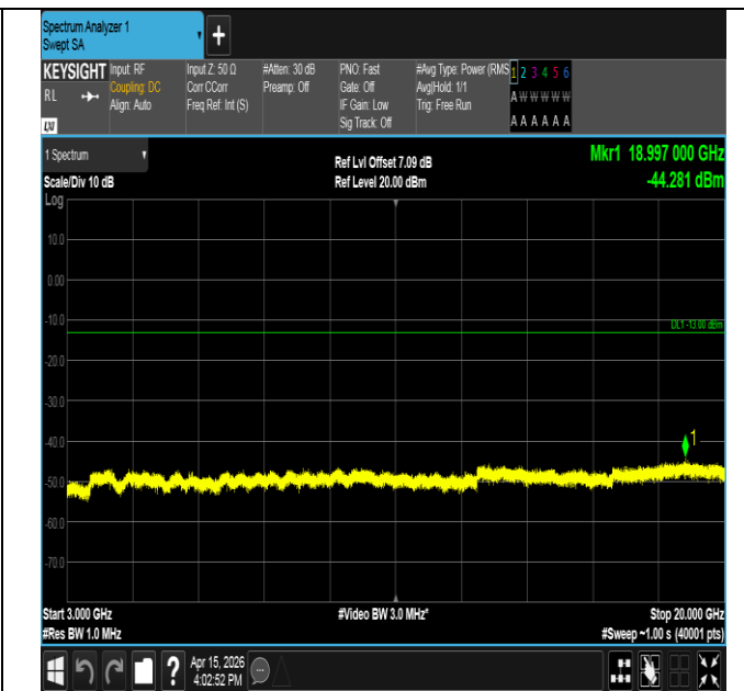
Band25-3MHz-16QAM-26365-15RB#0-3000~20000-PASS
