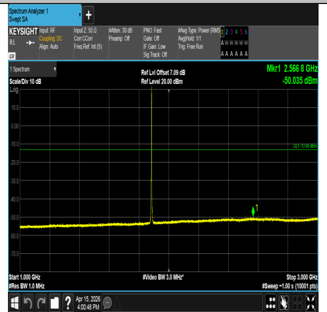
Band25-3MHz-16QAM-26365-1RB#14-1000~3000-PASS
