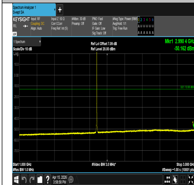
Band25-3MHz-16QAM-26365-1RB#0-1000~3000-PASS
