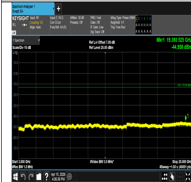
Band25-3MHz-16QAM-26675-1RB#14-3000~20000-PASS
