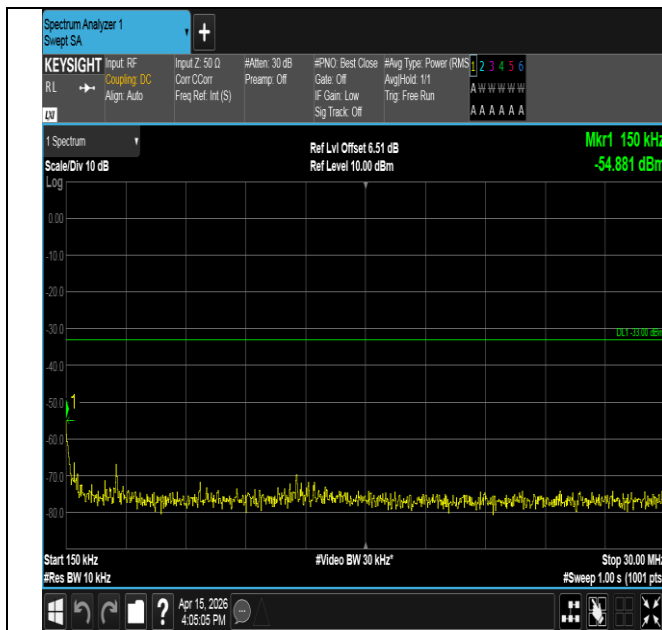
Band25-3MHz-QPSK-26675-1RB#14-0.15~30-PASS
