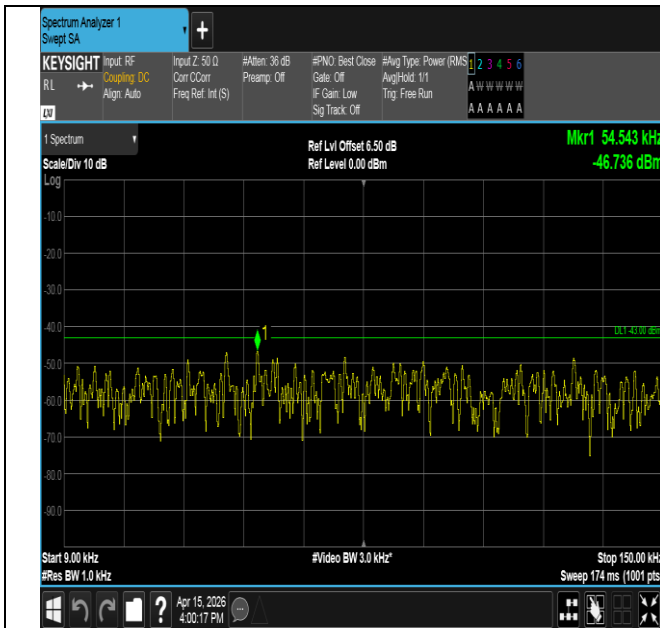
Band25-3MHz-16QAM-26365-1RB#14-0.009~0.15-PASS
