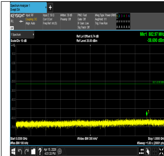
Band25-3MHz-QPSK-26365-15RB#0-30~1000-PASS
