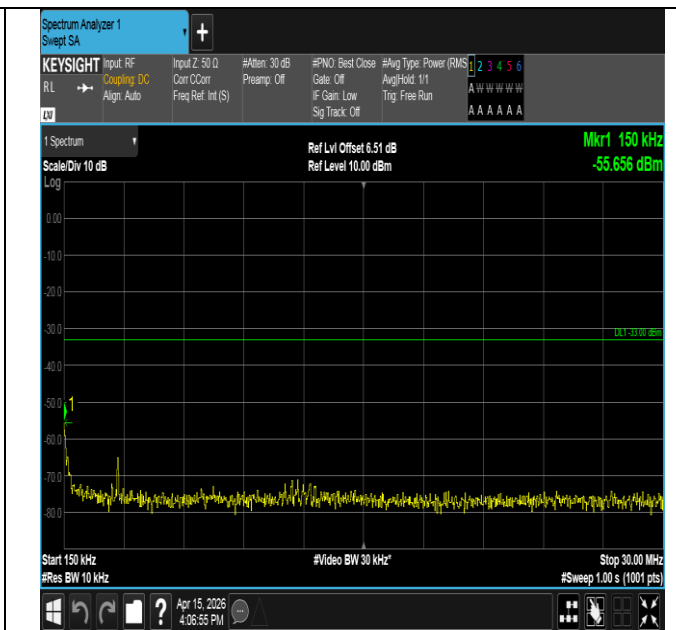
Band25-3MHz-QPSK-26675-15RB#0-0.15~30-PASS
