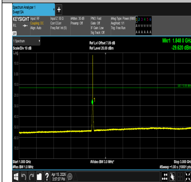
Band25-3MHz-16QAM-26055-15RB#0-1000~3000-PASS
