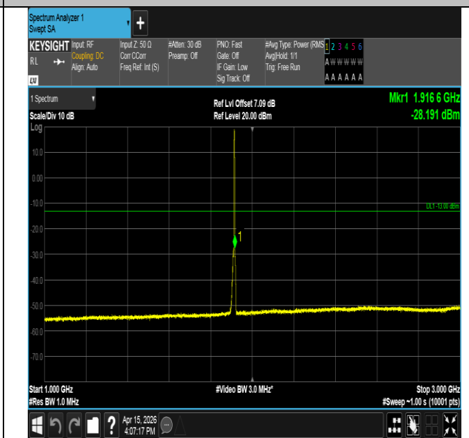
Band25-3MHz-QPSK-26675-15RB#0-1000~3000-PASS
