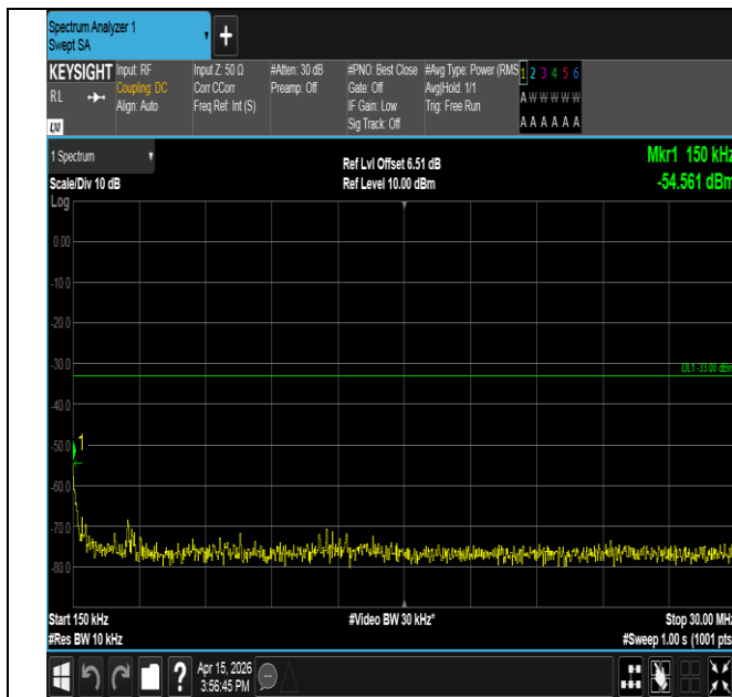
Band25-3MHz-16QAM-26055-15RB#0-0.15~30-PASS
