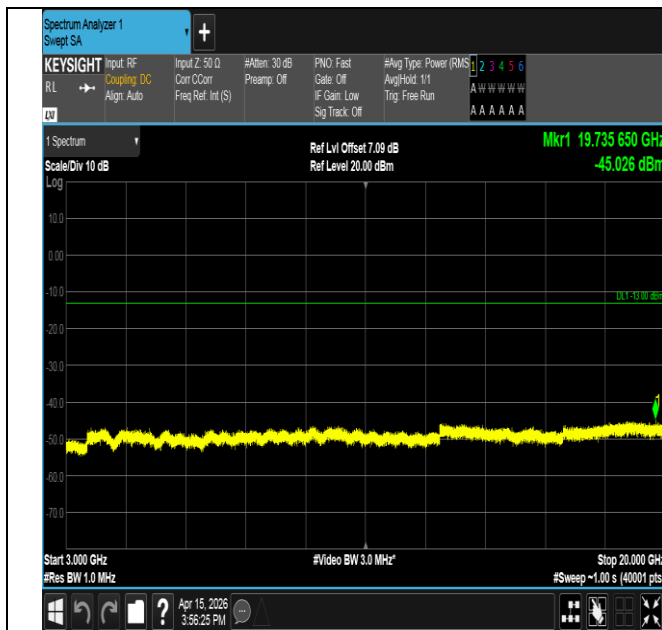
Band25-3MHz-QPSK-26055-15RB#0-3000~20000-PASS
