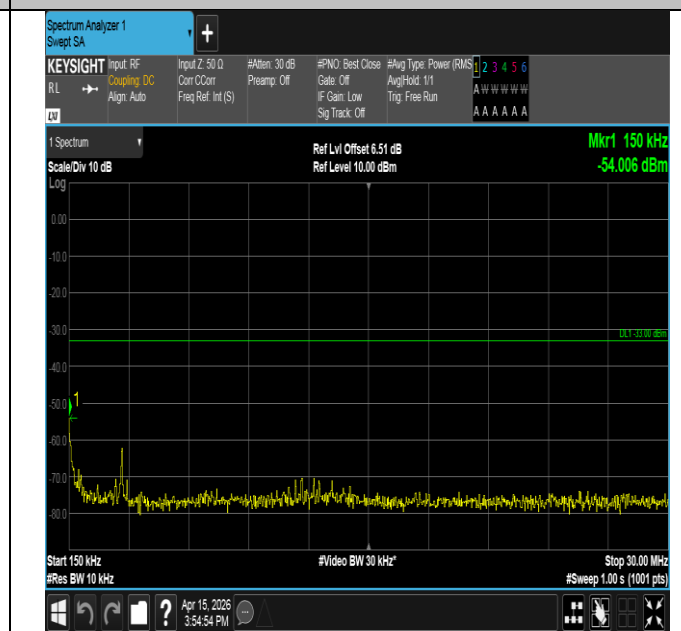
Band25-3MHz-16QAM-26055-1RB#14-0.15~30-PASS
