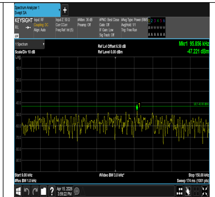
Band25-3MHz-QPSK-26365-1RB#14-0.009~0.15-PASS
