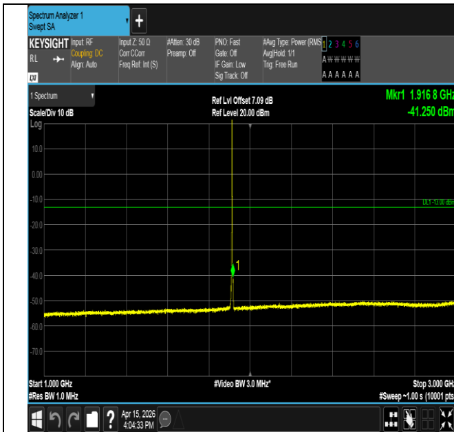
Band25-3MHz-16QAM-26675-1RB#0-1000~3000-PASS
