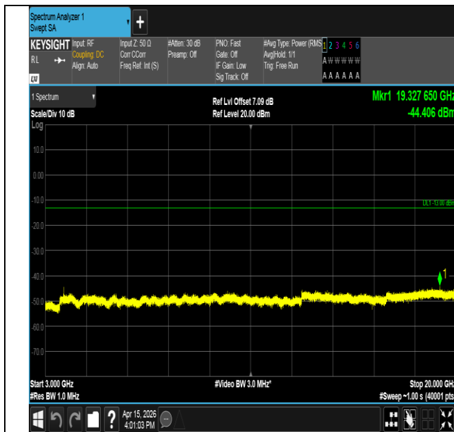
Band25-3MHz-16QAM-26365-1RB#14-3000~20000-PASS
