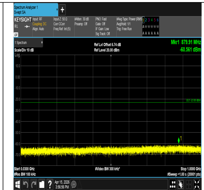
Band25-3MHz-16QAM-26055-15RB#0-30~1000-PASS
