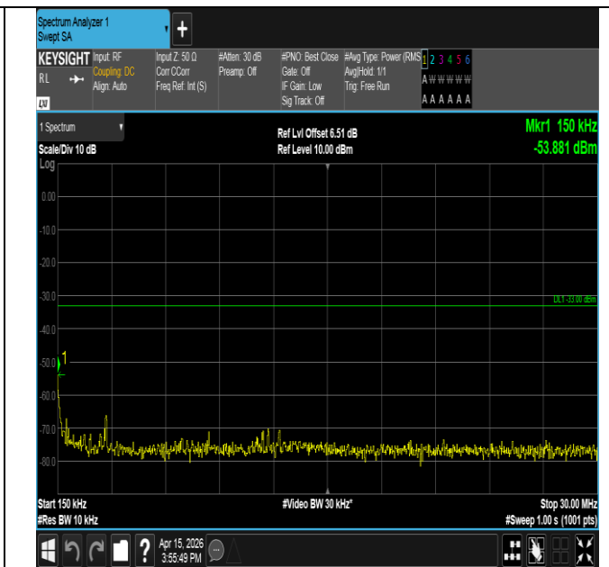
Band25-3MHz-QPSK-26055-15RB#0-0.15~30-PASS
