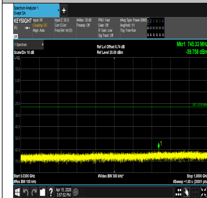
Band25-3MHz-QPSK-26365-1RB#0-30~1000-PASS
