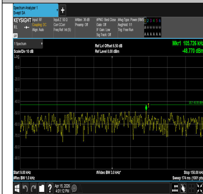
Band25-3MHz-QPSK-26365-15RB#0-0.009~0.15-PASS
