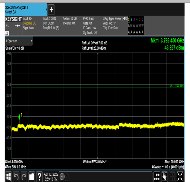
Band25-3MHz-16QAM-26365-1RB#0-3000~20000-PASS
