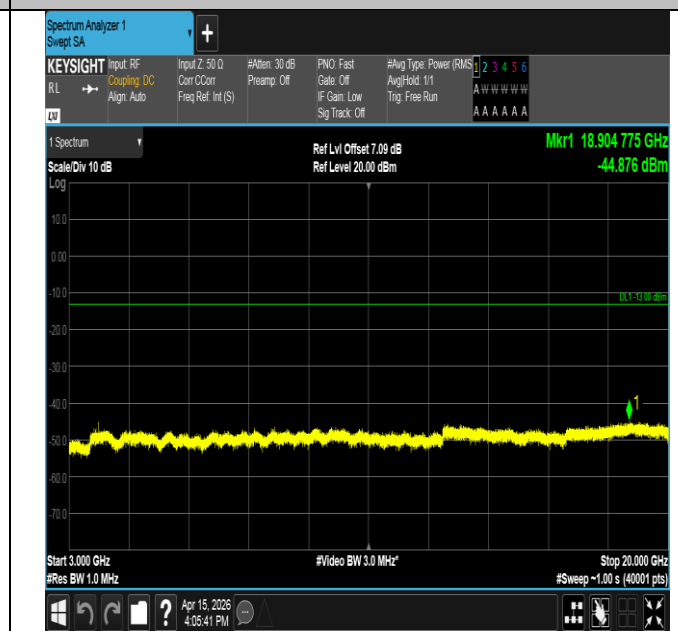
Band25-3MHz-QPSK-26675-1RB#14-3000~20000-PASS
