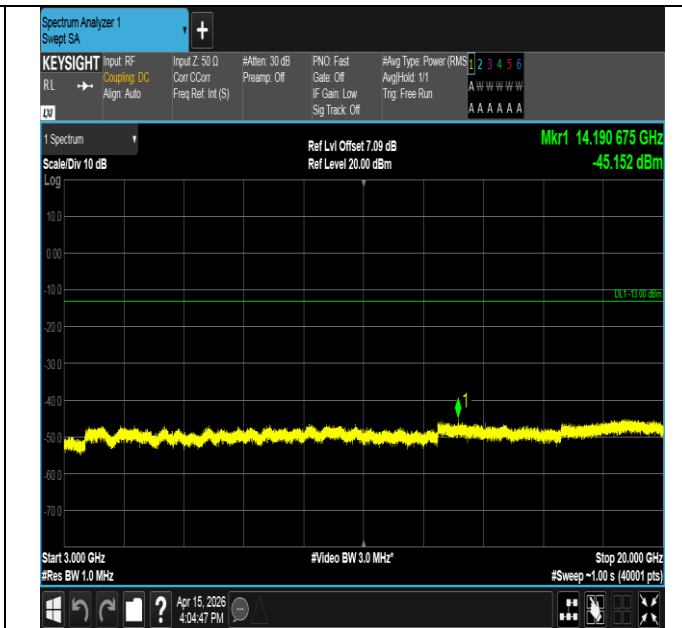
Band25-3MHz-16QAM-26675-1RB#0-3000~20000-PASS
