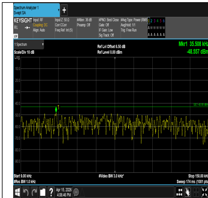
Band25-3MHz-QPSK-26675-15RB#0-0.009~0.15-PASS
