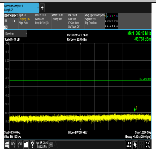
Band25-3MHz-16QAM-26365-15RB#0-30~1000-PASS
