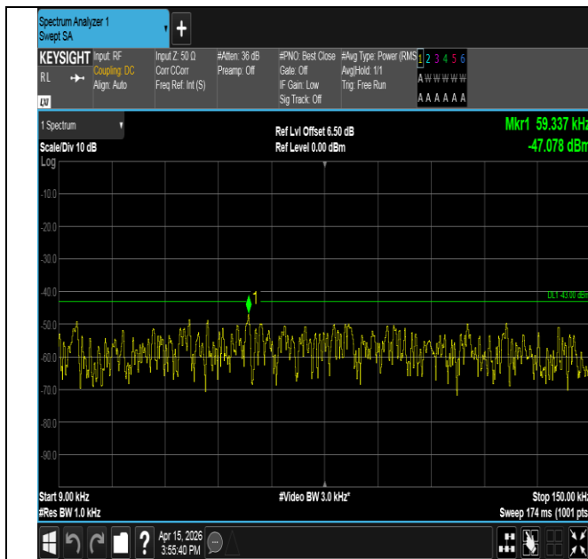
Band25-3MHz-QPSK-26055-15RB#0-0.009~0.15-PASS
