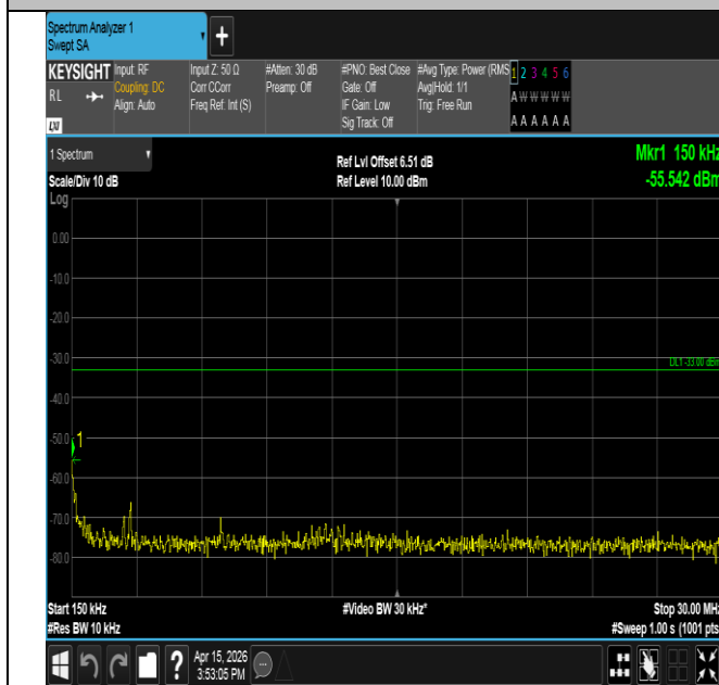
Band25-3MHz-16QAM-26055-1RB#0-0.15~30-PASS
