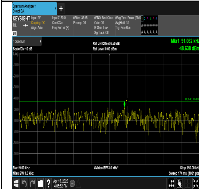
Band25-3MHz-16QAM-26675-1RB#14-0.009~0.15-PASS
