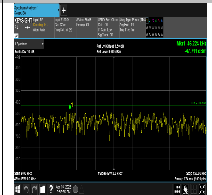
Band25-3MHz-16QAM-26055-15RB#0-0.009~0.15-PASS
