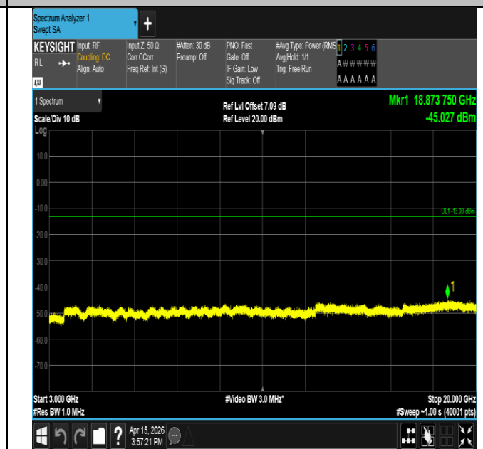
Band25-3MHz-16QAM-26055-15RB#0-3000~20000-PASS
