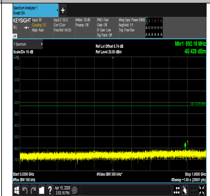
Band25-3MHz-16QAM-26055-1RB#0-30~1000-PASS
