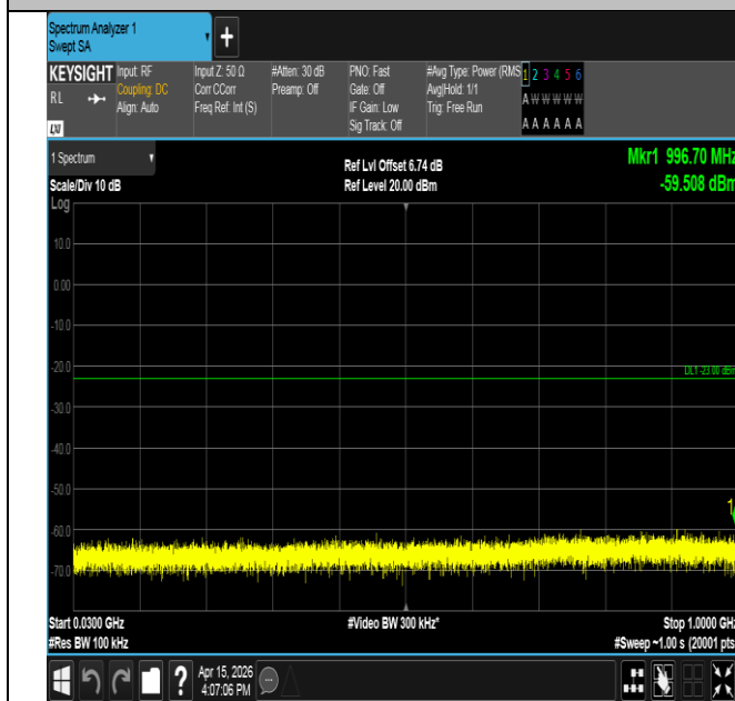
Band25-3MHz-QPSK-26675-15RB#0-30~1000-PASS
