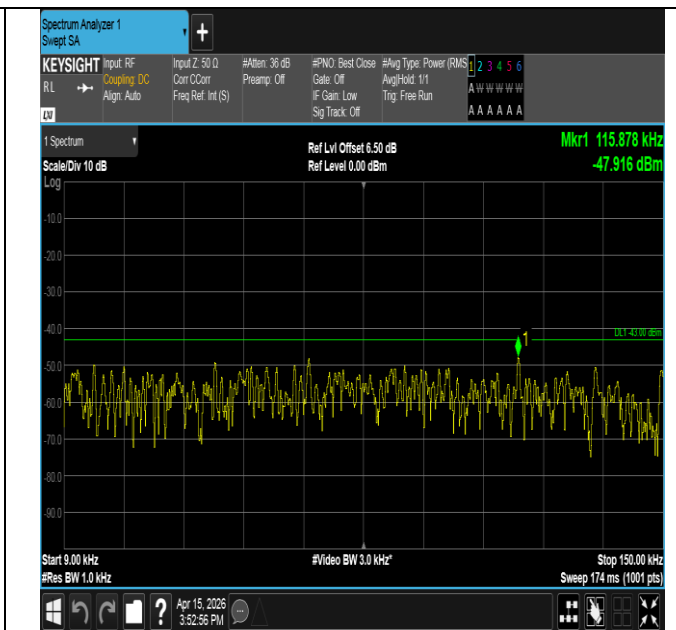
Band25-3MHz-16QAM-26055-1RB#0-0.009~0.15-PASS
