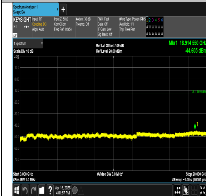
Band25-3MHz-QPSK-26365-15RB#0-3000~20000-PASS
