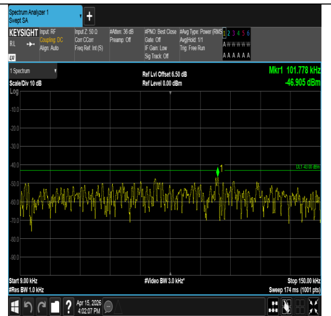
Band25-3MHz-16QAM-26365-15RB#0-0.009~0.15-PASS
