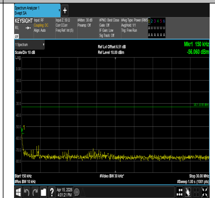
Band25-3MHz-QPSK-26365-15RB#0-0.15~30-PASS
