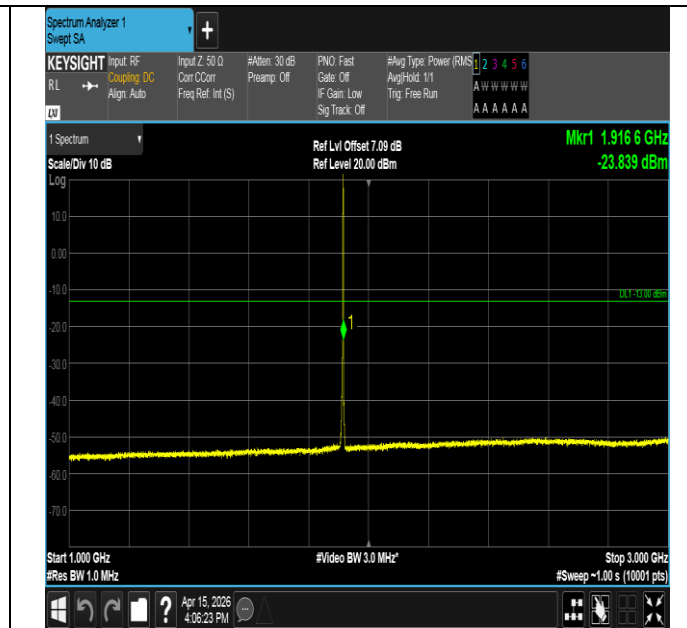
Band25-3MHz-16QAM-26675-1RB#14-1000~3000-PASS
