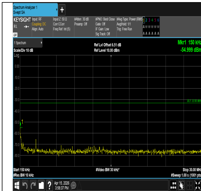
Band25-3MHz-16QAM-26365-1RB#0-0.15~30-PASS
