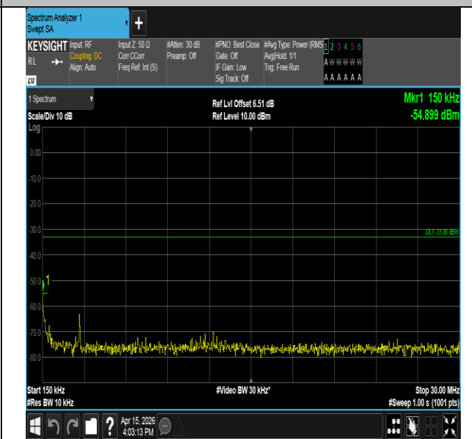
Band25-3MHz-QPSK-26675-1RB#0-0.15~30-PASS
