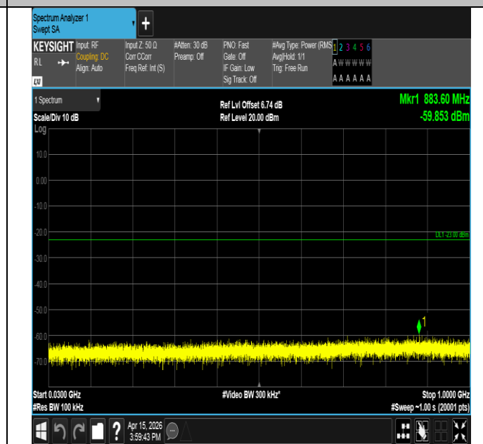
Band25-3MHz-QPSK-26365-1RB#14-30~1000-PASS
