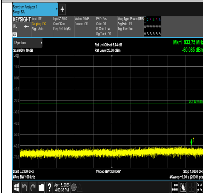
Band25-3MHz-16QAM-26365-1RB#14-30~1000-PASS
