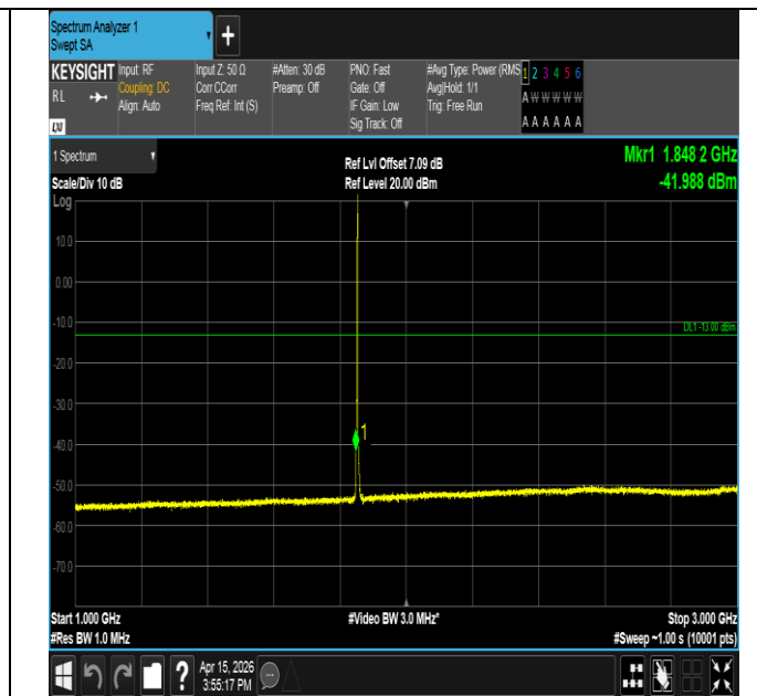
Band25-3MHz-16QAM-26055-1RB#14-1000~3000-PASS
