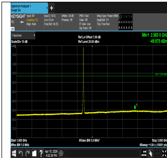
Band25-3MHz-16QAM-26365-15RB#0-1000~3000-PASS
