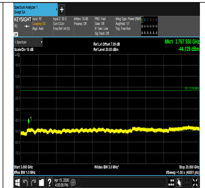
Band25-3MHz-QPSK-26365-1RB#14-3000~20000-PASS
