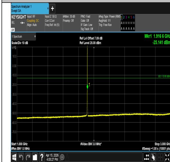
Band25-3MHz-QPSK-26675-1RB#14-1000~3000-PASS
