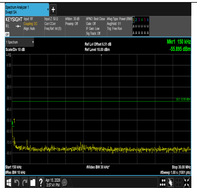
Band25-3MHz-QPSK-26365-1RB#0-0.15~30-PASS
