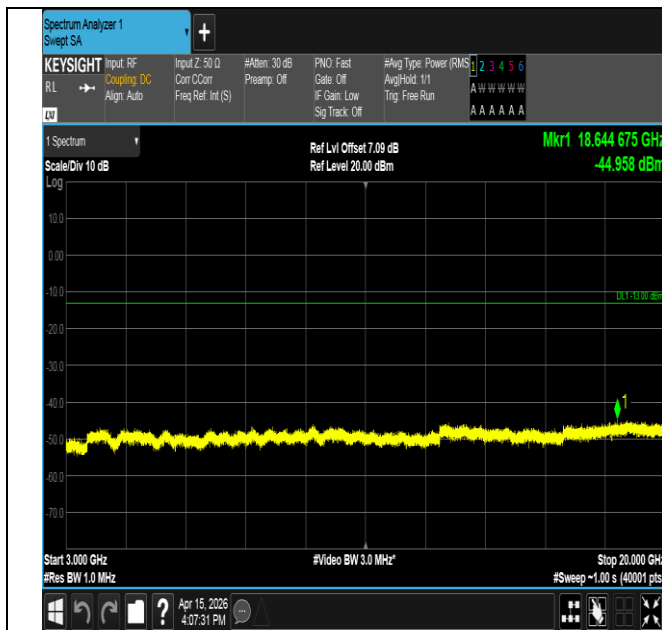
Band25-3MHz-QPSK-26675-15RB#0-3000~20000-PASS
