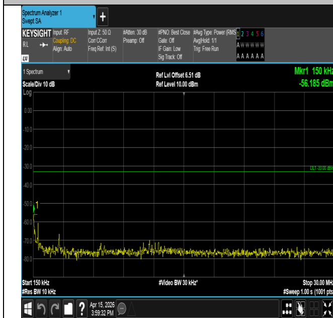
Band25-3MHz-QPSK-26365-1RB#14-0.15~30-PASS
