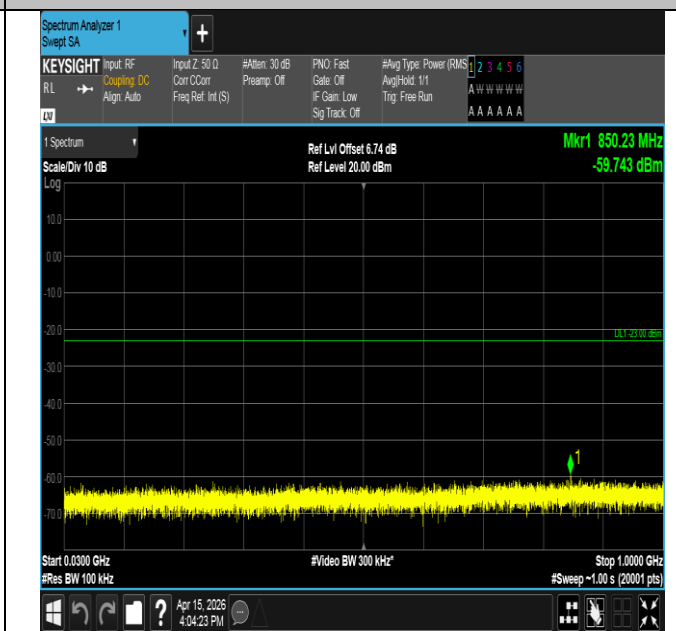
Band25-3MHz-16QAM-26675-1RB#0-30~1000-PASS
