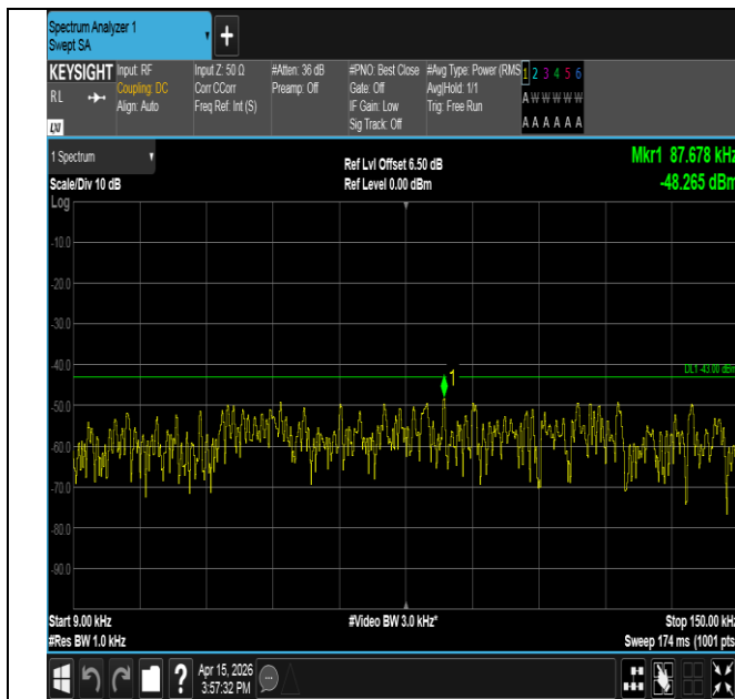
Band25-3MHz-QPSK-26365-1RB#0-0.009~0.15-PASS
