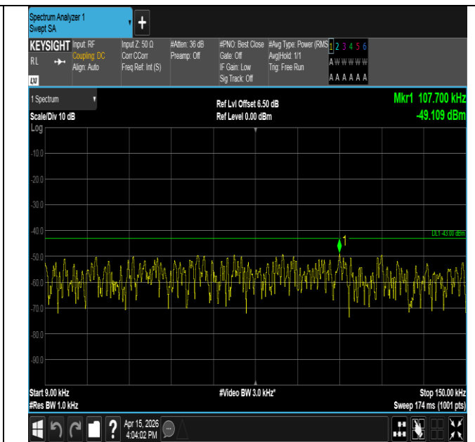
Band25-3MHz-16QAM-26675-1RB#0-0.009~0.15-PASS
