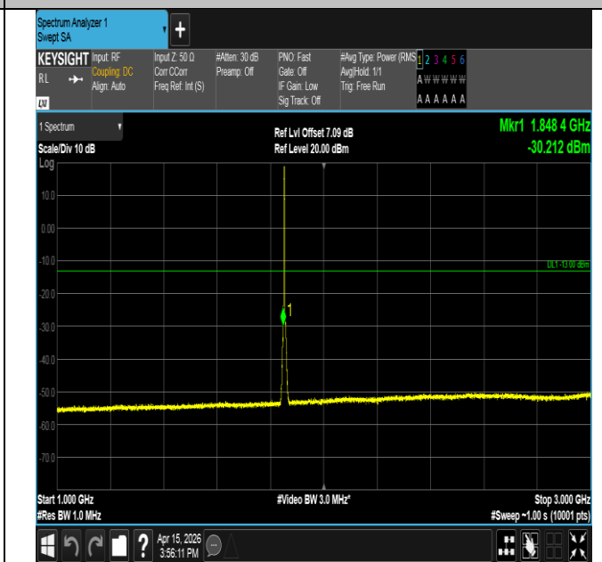
Band25-3MHz-QPSK-26055-15RB#0-1000~3000-PASS
