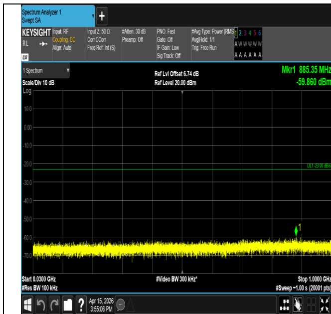
Band25-3MHz-16QAM-26055-1RB#14-30~1000-PASS
