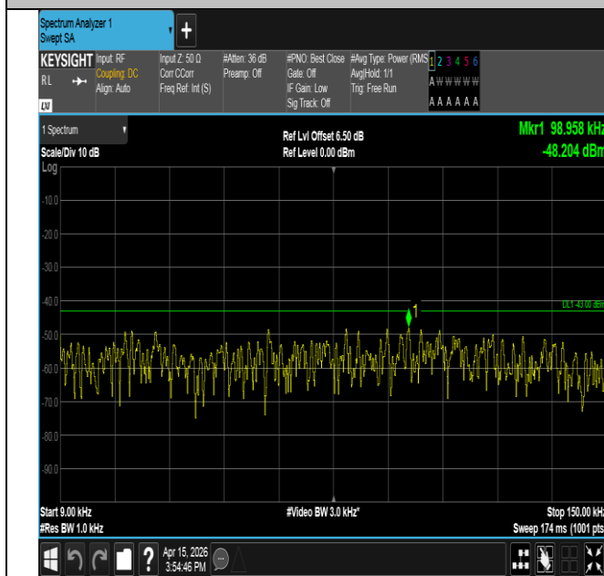
Band25-3MHz-16QAM-26055-1RB#14-0.009~0.15-PASS
