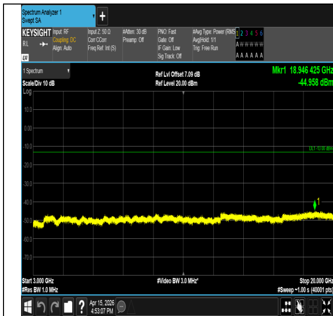
Band25-5MHz-16QAM-26665-1RB#24-3000~20000-PASS
