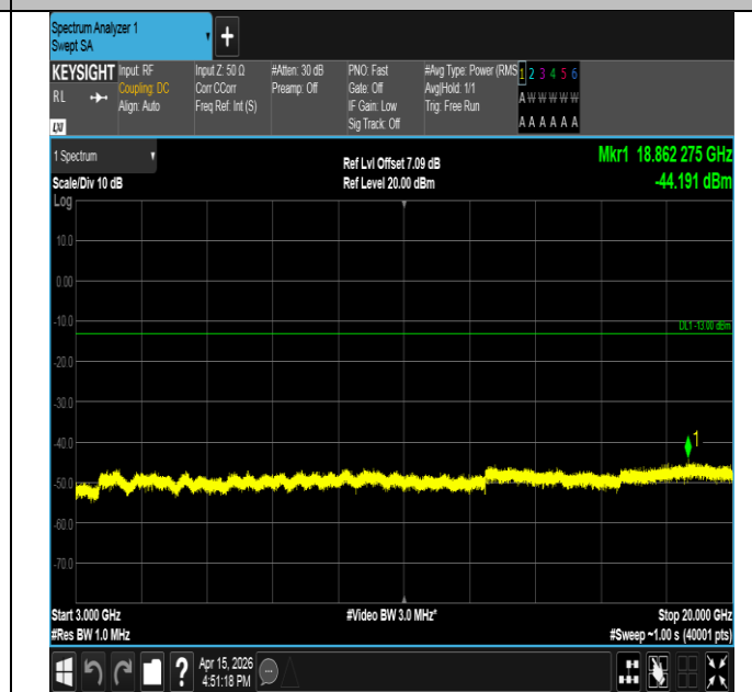
Band25-5MHz-16QAM-26665-1RB#0-3000~20000-PASS
