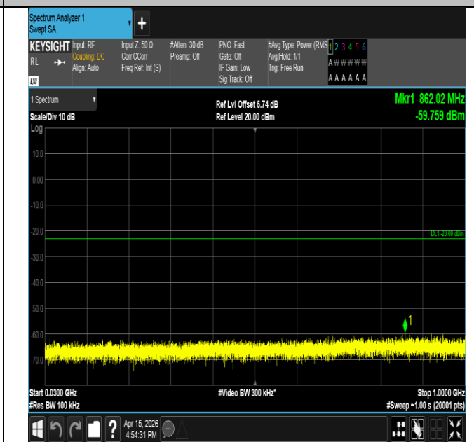
Band25-5MHz-16QAM-26665-25RB#0-30~1000-PASS
