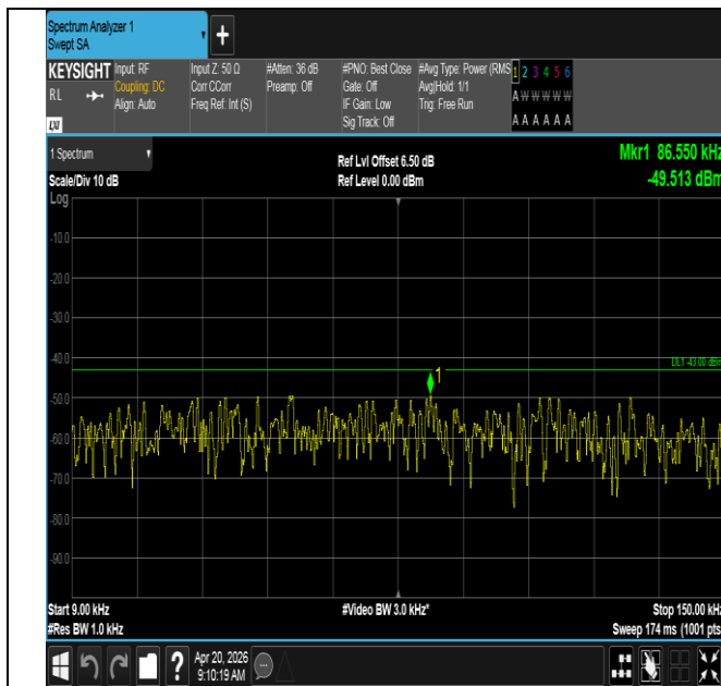
Band25-10MHz-16QAM-26365-1RB#49-0.009~0.15-PASS
