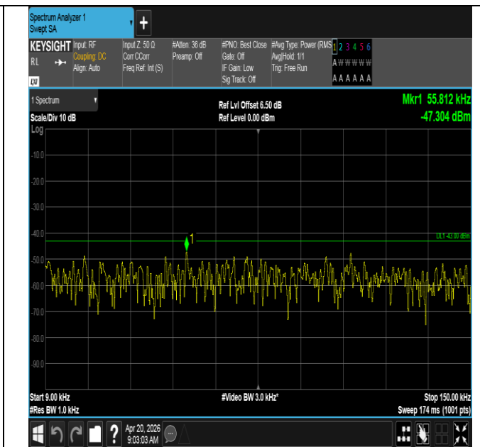
Band25-10MHz-16QAM-26090-1RB#0-0.009~0.15-PASS
