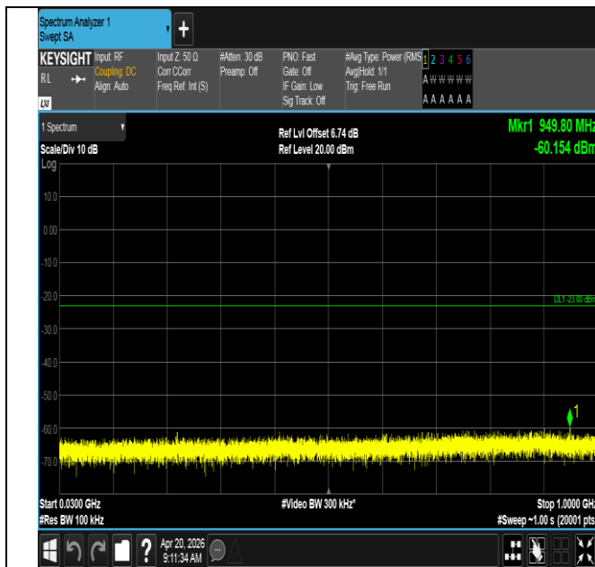
Band25-10MHz-QPSK-26365-50RB#0-30~1000-PASS
