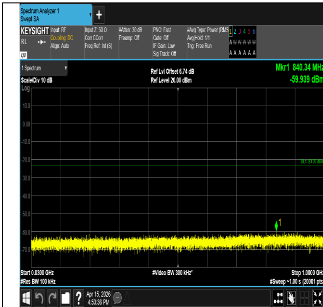
Band25-5MHz-QPSK-26665-25RB#0-30~1000-PASS
