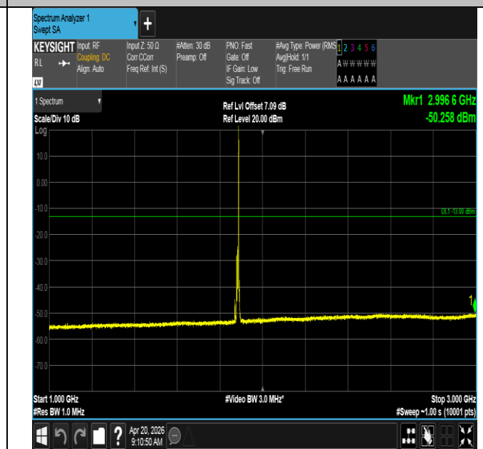
Band25-10MHz-16QAM-26365-1RB#49-1000~3000-PASS
