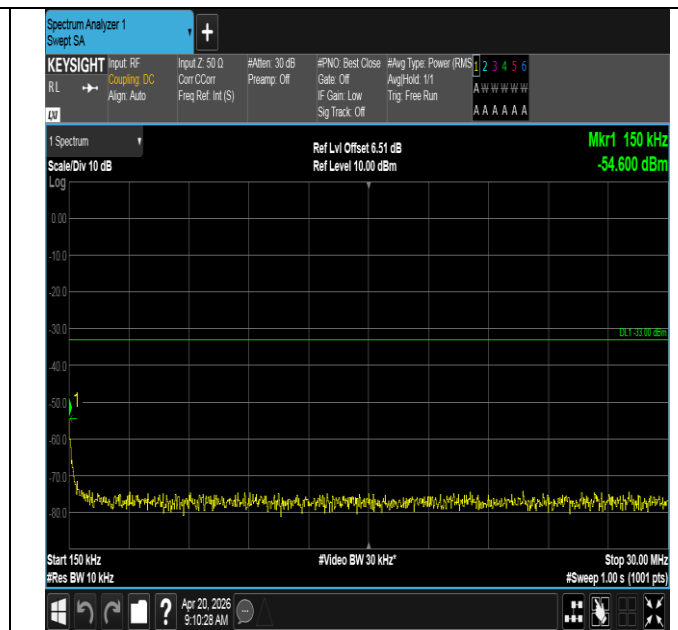
Band25-10MHz-16QAM-26365-1RB#49-0.15~30-PASS
