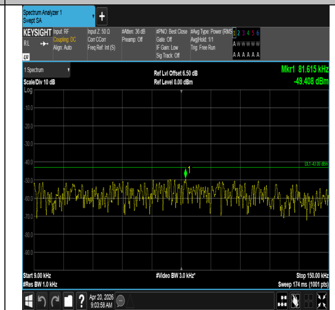
Band25-10MHz-QPSK-26090-1RB#49-0.009~0.15-PASS
