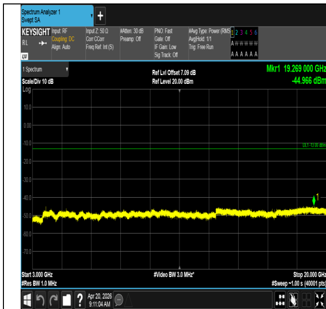
Band25-10MHz-16QAM-26365-1RB#49-3000~20000-PASS
