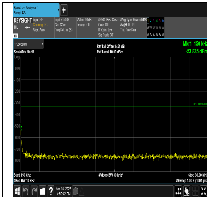
Band25-5MHz-16QAM-26665-1RB#0-0.15~30-PASS
