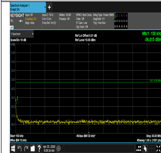
Band25-10MHz-QPSK-26365-1RB#49-0.15~30-PASS
