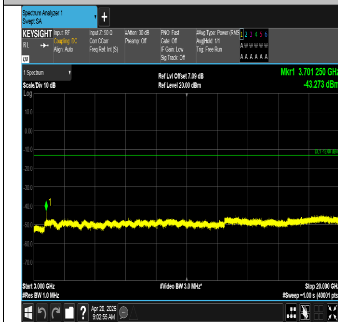
Band25-10MHz-QPSK-26090-1RB#0-3000~20000-PASS
