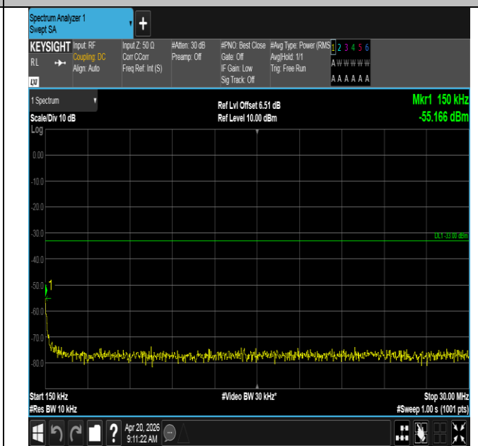
Band25-10MHz-QPSK-26365-50RB#0-0.15~30-PASS
