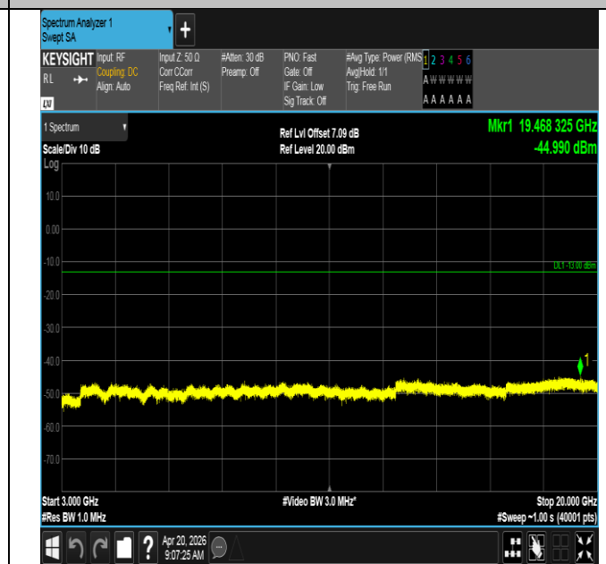
Band25-10MHz-16QAM-26090-50RB#0-3000~20000-PASS
