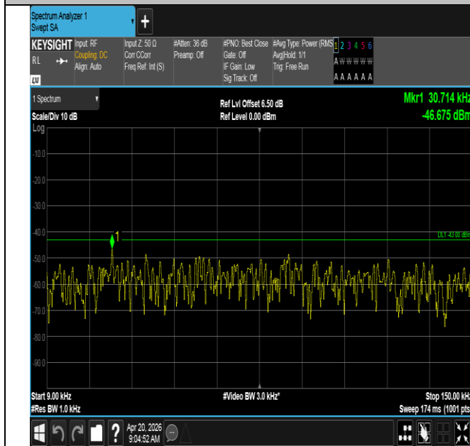
Band25-10MHz-16QAM-26090-1RB#49-0.009~0.15-PASS
