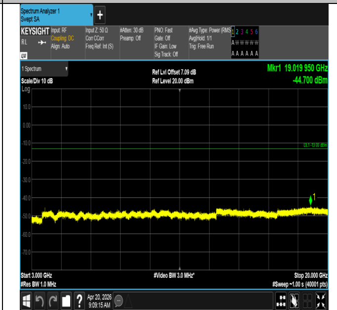
Band25-10MHz-16QAM-26365-1RB#0-3000~20000-PASS
