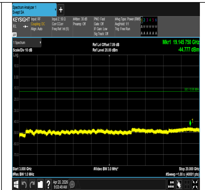
Band25-10MHz-16QAM-26090-1RB#0-3000~20000-PASS
