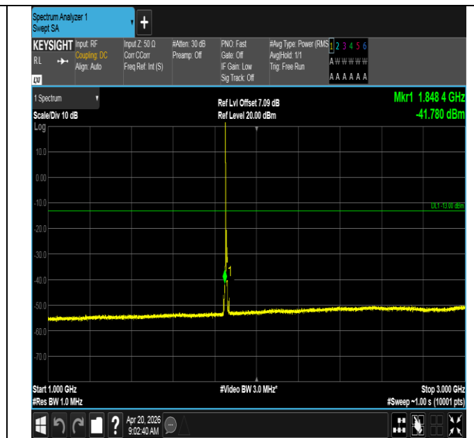
Band25-10MHz-QPSK-26090-1RB#0-1000~3000-PASS
