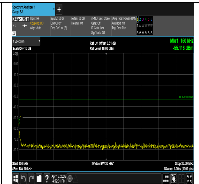
Band25-5MHz-16QAM-26665-1RB#24-0.15~30-PASS
