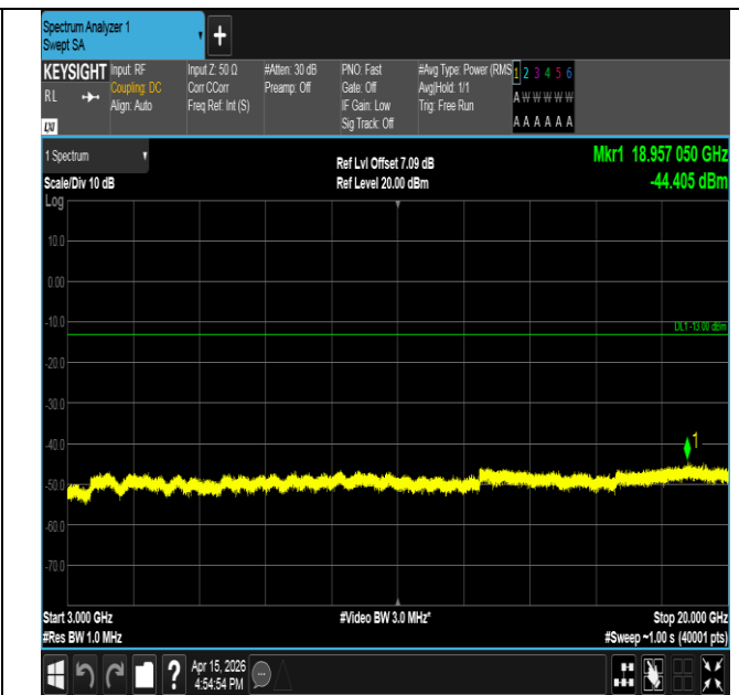
Band25-5MHz-16QAM-26665-25RB#0-3000~20000-PASS
