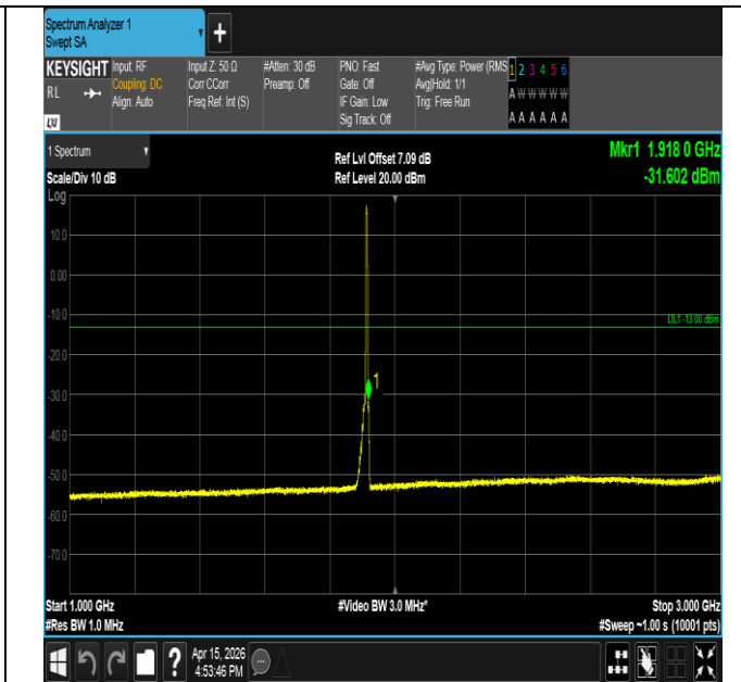
Band25-5MHz-QPSK-26665-25RB#0-1000~3000-PASS
