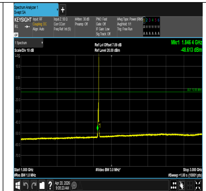
Band25-10MHz-16QAM-26090-1RB#49-1000~3000-PASS
