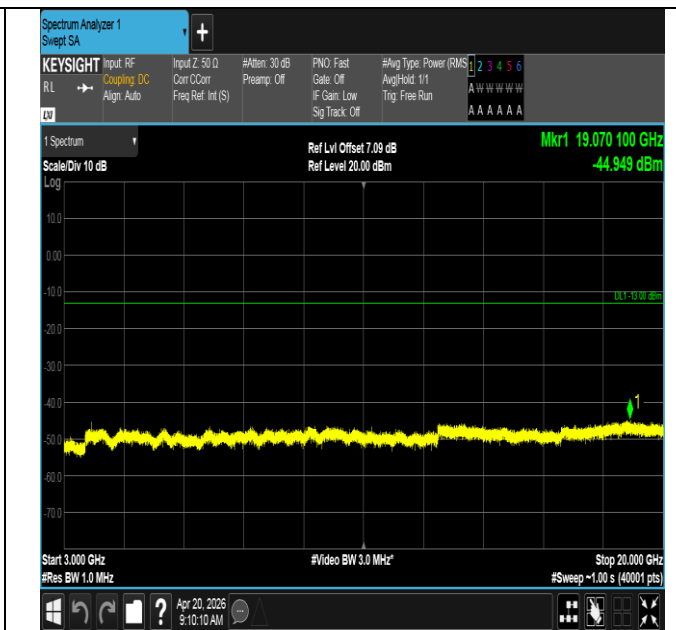
Band25-10MHz-QPSK-26365-1RB#49-3000~20000-PASS
