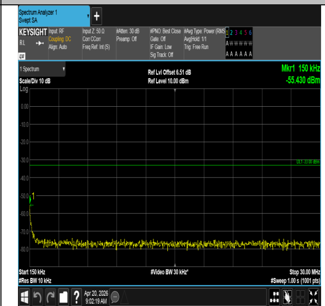
Band25-10MHz-QPSK-26090-1RB#0-0.15~30-PASS
