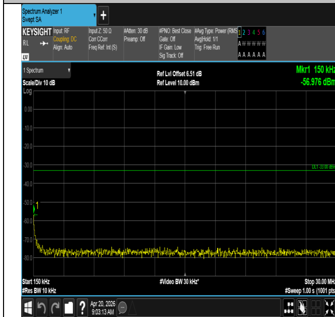
Band25-10MHz-16QAM-26090-1RB#0-0.15~30-PASS
