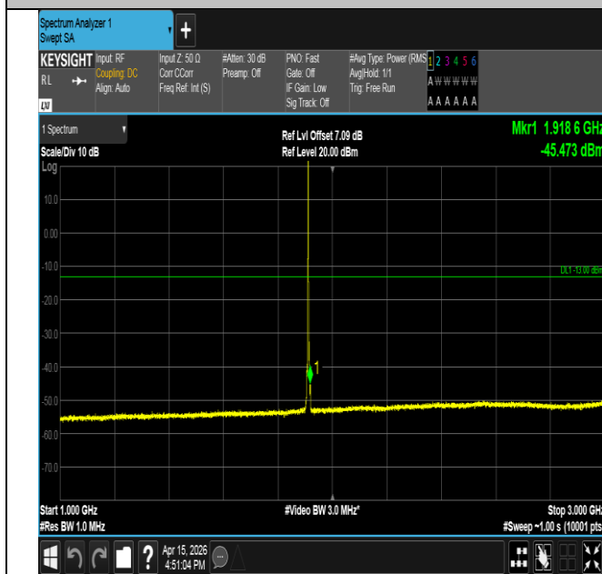
Band25-5MHz-16QAM-26665-1RB#0-1000~3000-PASS
