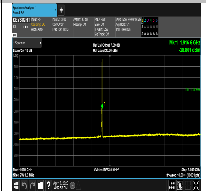
Band25-5MHz-16QAM-26665-1RB#24-1000~3000-PASS
