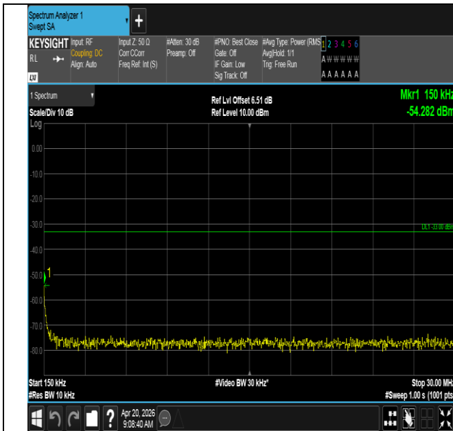
Band25-10MHz-16QAM-26365-1RB#0-0.15~30-PASS
