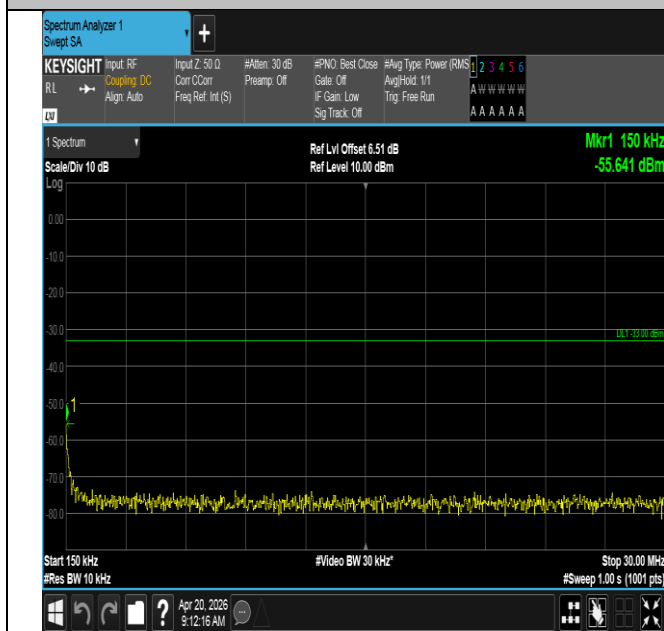
Band25-10MHz-16QAM-26365-50RB#0-0.15~30-PASS
