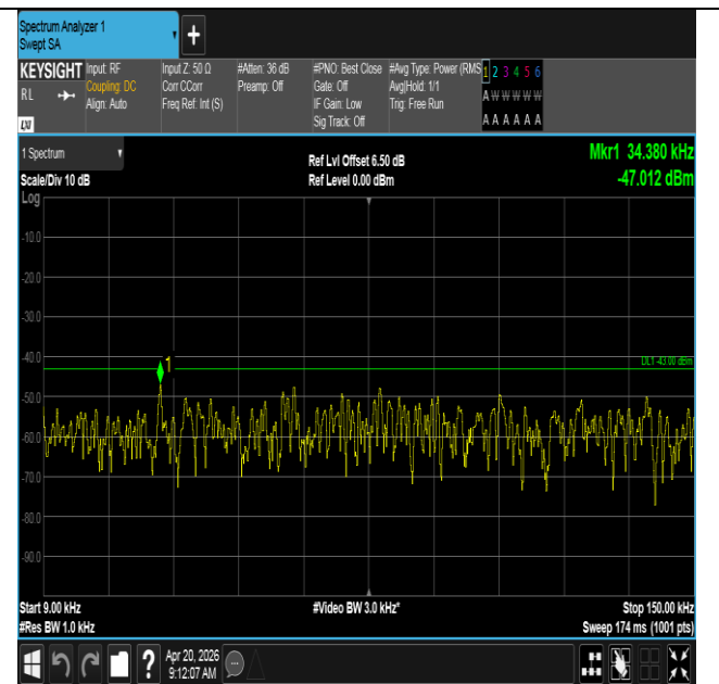
Band25-10MHz-16QAM-26365-50RB#0-0.009~0.15-PASS
