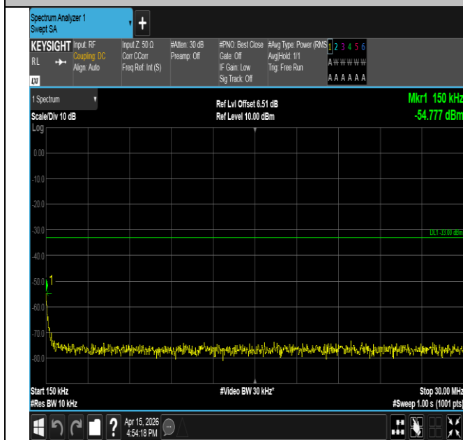
Band25-5MHz-16QAM-26665-25RB#0-0.15~30-PASS
