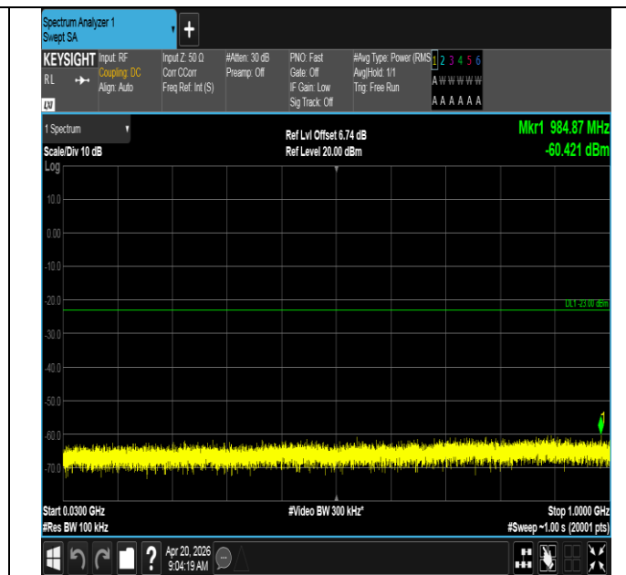
Band25-10MHz-QPSK-26090-1RB#49-30~1000-PASS
