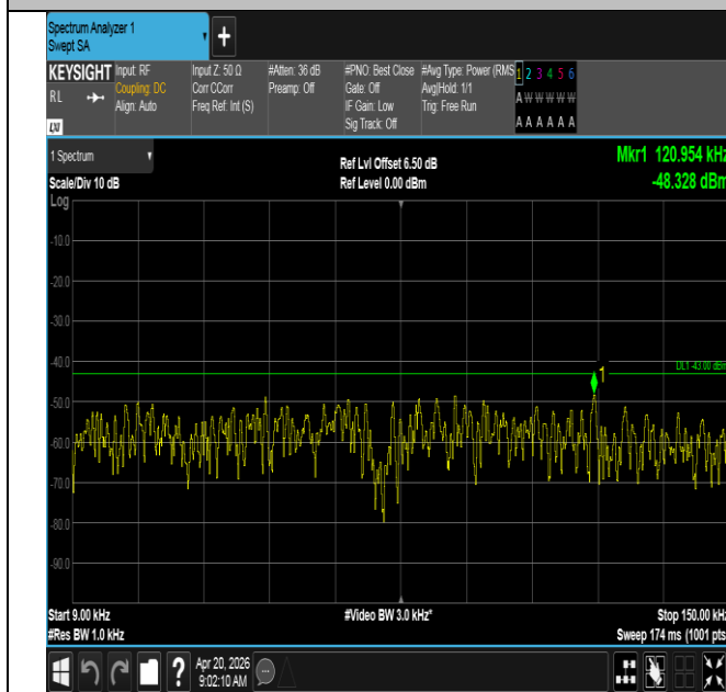
Band25-10MHz-QPSK-26090-1RB#0-0.009~0.15-PASS
