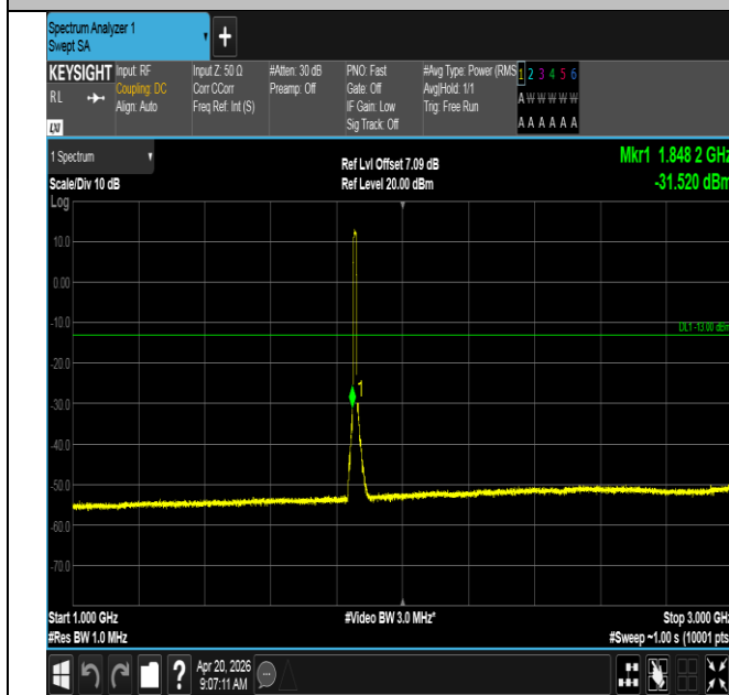
Band25-10MHz-16QAM-26090-50RB#0-1000~3000-PASS
