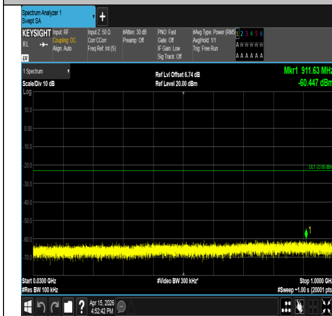
Band25-5MHz-16QAM-26665-1RB#24-30~1000-PASS
