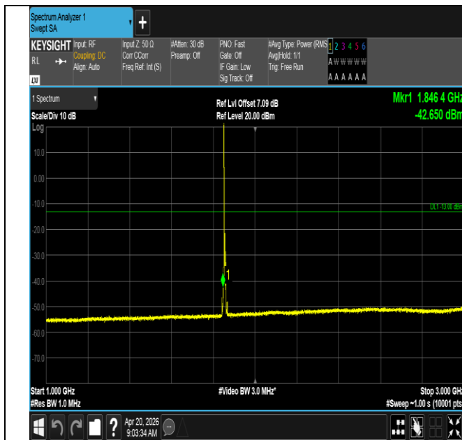
Band25-10MHz-16QAM-26090-1RB#0-1000~3000-PASS
