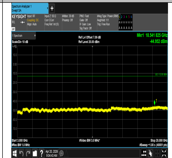
Band25-10MHz-QPSK-26090-1RB#49-3000~20000-PASS
