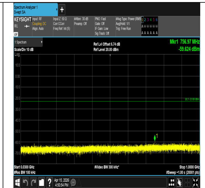
Band25-5MHz-16QAM-26665-1RB#0-30~1000-PASS
