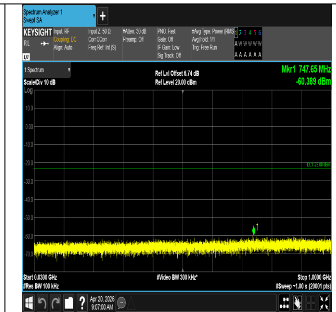
Band25-10MHz-16QAM-26090-50RB#0-30~1000-PASS
