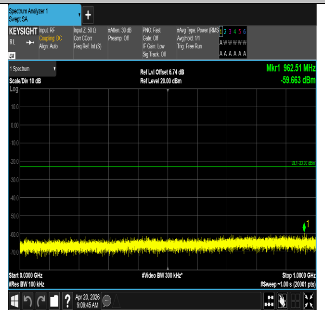
Band25-10MHz-QPSK-26365-1RB#49-30~1000-PASS
