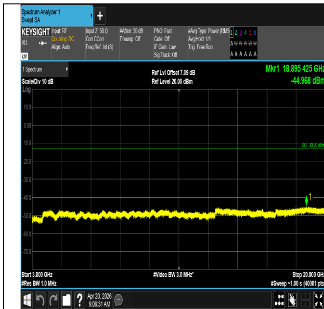
Band25-10MHz-QPSK-26090-50RB#0-3000~20000-PASS
