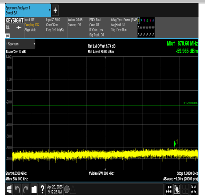
Band25-10MHz-16QAM-26365-50RB#0-30~1000-PASS
