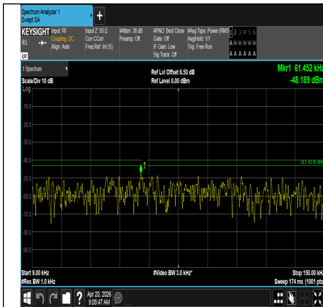
Band25-10MHz-QPSK-26090-50RB#0-0.009~0.15-PASS
