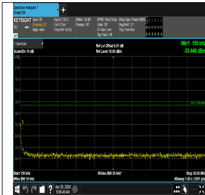
Band25-10MHz-16QAM-26090-50RB#0-0.15~30-PASS
