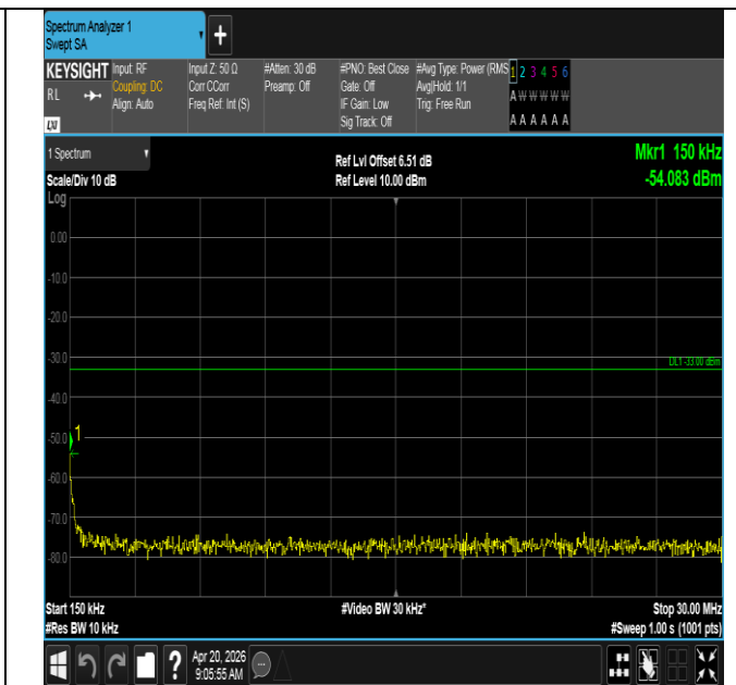
Band25-10MHz-QPSK-26090-50RB#0-0.15~30-PASS
