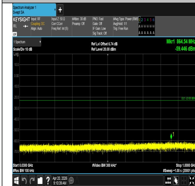
Band25-10MHz-16QAM-26365-1RB#49-30~1000-PASS
