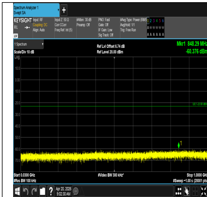
Band25-10MHz-QPSK-26090-1RB#0-30~1000-PASS
