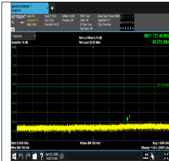
Band25-10MHz-16QAM-26090-1RB#49-30~1000-PASS
