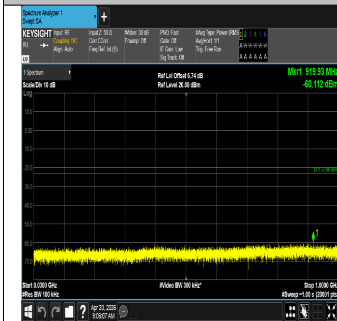
Band25-10MHz-QPSK-26090-50RB#0-30~1000-PASS
