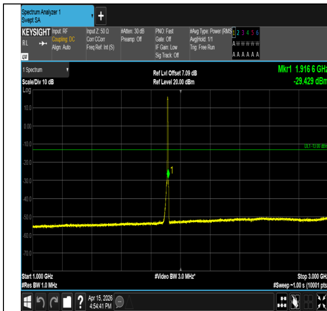
Band25-5MHz-16QAM-26665-25RB#0-1000~3000-PASS
