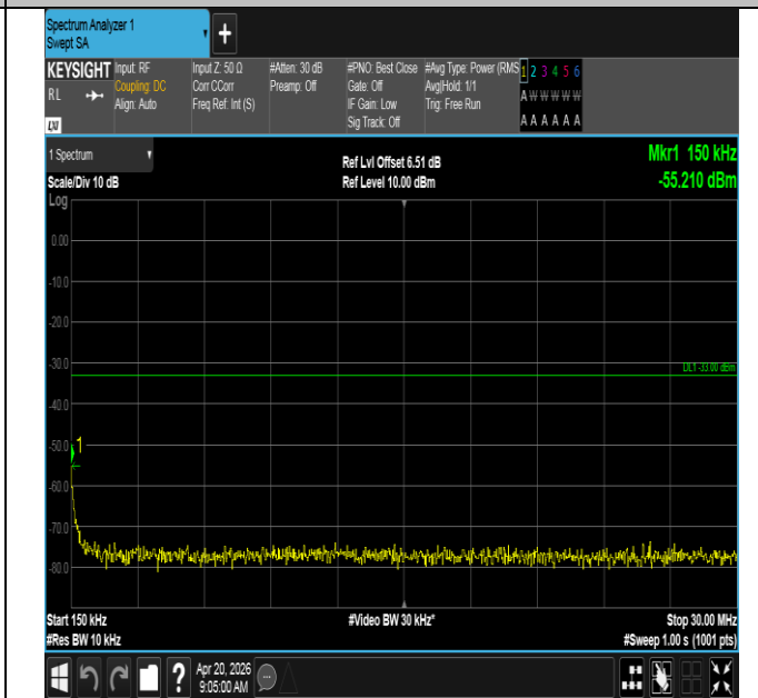
Band25-10MHz-16QAM-26090-1RB#49-0.15~30-PASS
