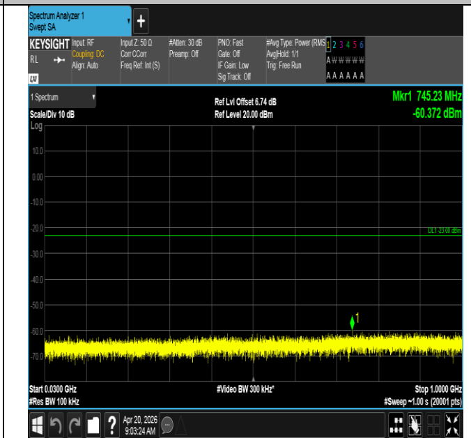
Band25-10MHz-16QAM-26090-1RB#0-30~1000-PASS
