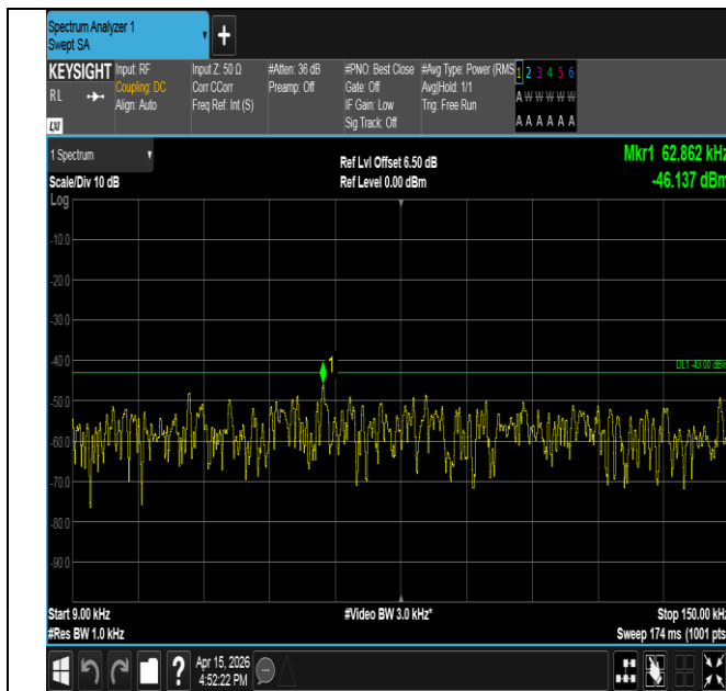
Band25-5MHz-16QAM-26665-1RB#24-0.009~0.15-PASS
