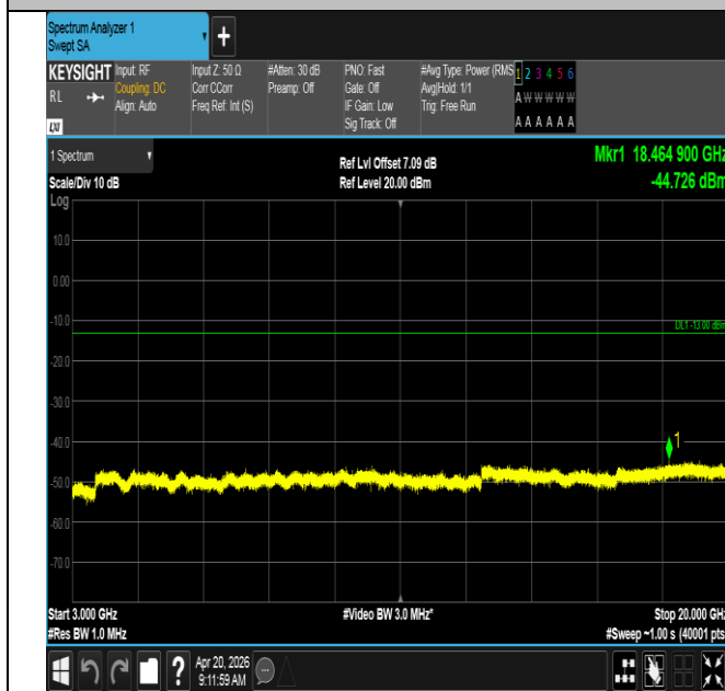
Band25-10MHz-QPSK-26365-50RB#0-3000~20000-PASS
