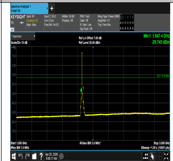
Band25-10MHz-QPSK-26090-50RB#0-1000~3000-PASS
