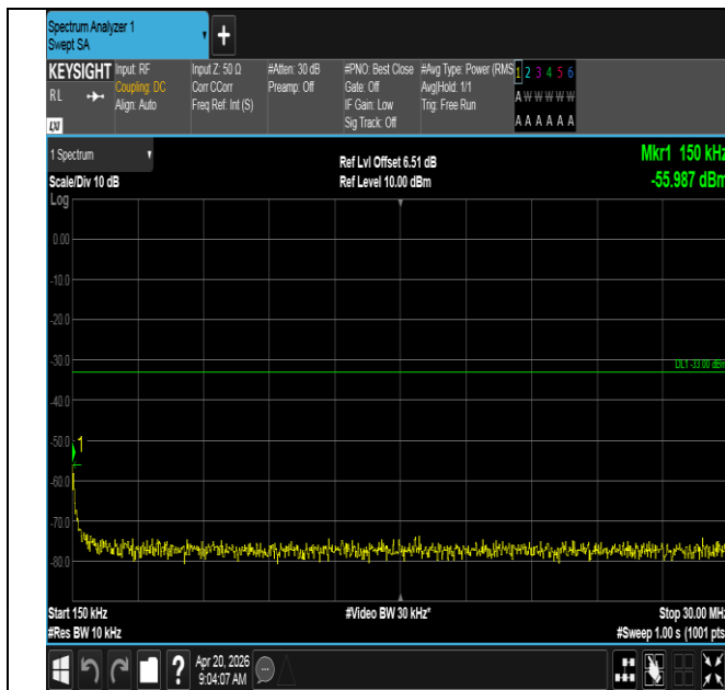
Band25-10MHz-QPSK-26090-1RB#49-0.15~30-PASS
