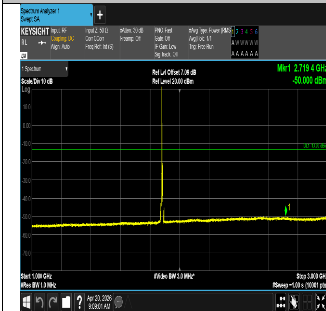
Band25-10MHz-16QAM-26365-1RB#0-1000~3000-PASS
