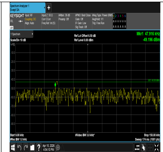
Band25-5MHz-16QAM-26665-25RB#0-0.009~0.15-PASS
