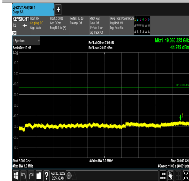
Band25-10MHz-16QAM-26090-1RB#49-3000~20000-PASS
