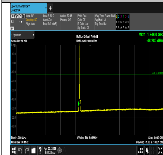
Band25-10MHz-QPSK-26090-1RB#49-1000~3000-PASS
