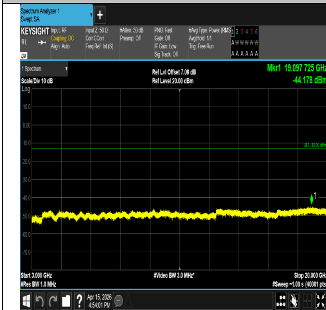
Band25-5MHz-QPSK-26665-25RB#0-3000~20000-PASS
