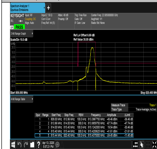
Band26(814-824)-1.4MHz-16QAM-26697-1RB#5-PASS
