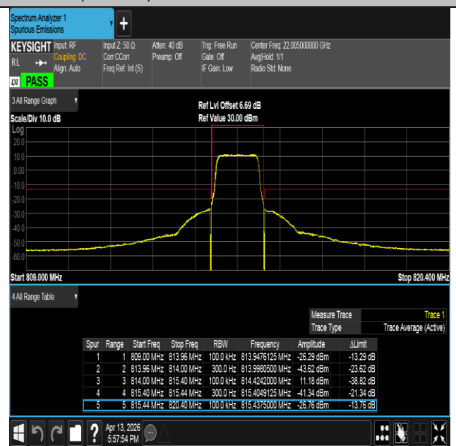
Band26(814-824)-1.4MHz-16QAM-26697-6RB#0-PASS
