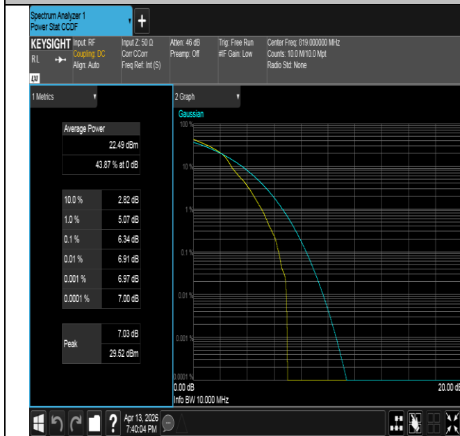
Band26(814-824)-10MHz-16QAM-26740-1RB#0-PASS
