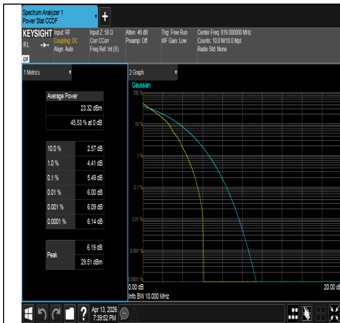
Band26(814-824)-10MHz-QPSK-26740-1RB#0-PASS
