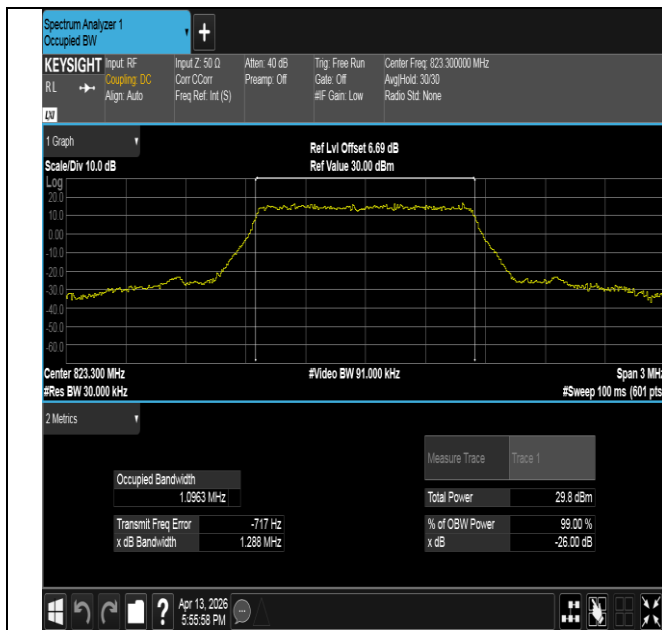
Band26(814-824)-1.4MHz-QPSK-26783-6RB#0-PASS
