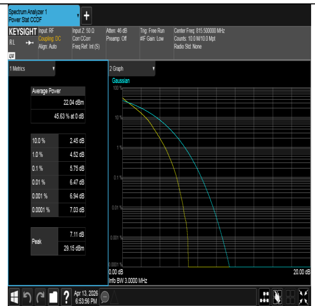
Band26(814-824)-3MHz-QPSK-26705-15RB#0-PASS
