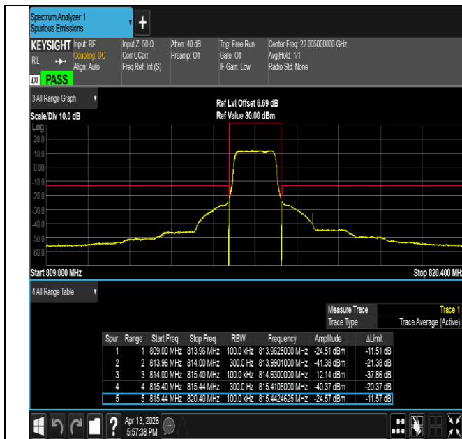
Band26(814-824)-1.4MHz-QPSK-26697-6RB#0-PASS
