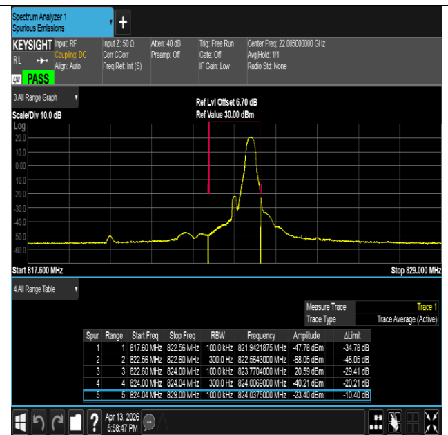
Band26(814-824)-1.4MHz-QPSK-26783-1RB#5-PASS
