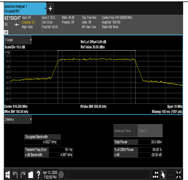
Band26(814-824)-5MHz-16QAM-26715-25RB#0-PASS
