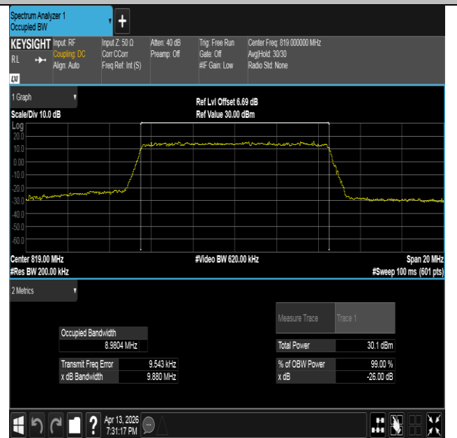
Band26(814-824)-10MHz-16QAM-26740-50RB#0-PASS
