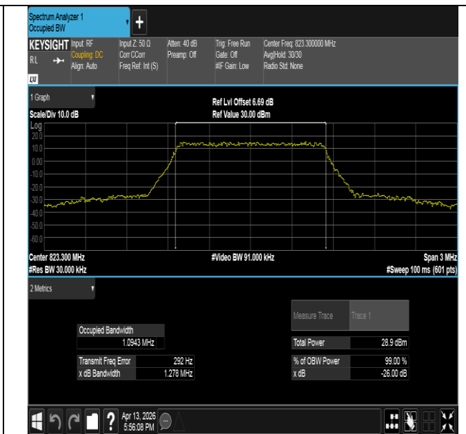
Band26(814-824)-1.4MHz-16QAM-26783-6RB#0-PASS
