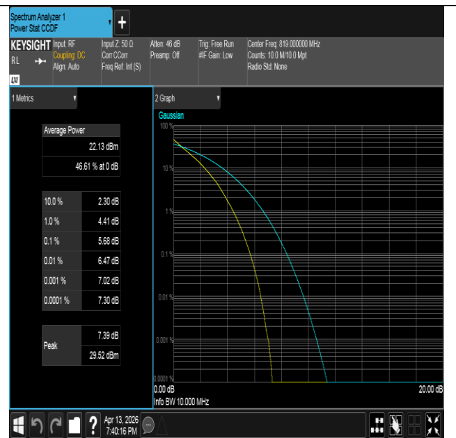
Band26(814-824)-10MHz-QPSK-26740-50RB#0-PASS
