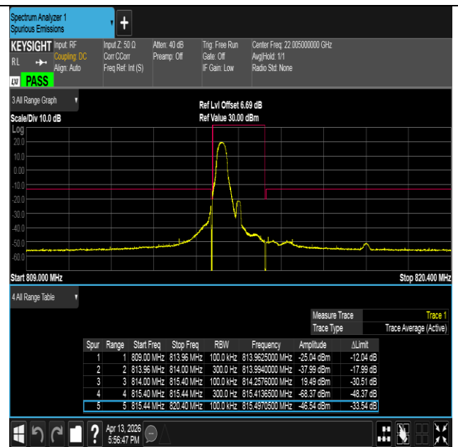
Band26(814-824)-1.4MHz-16QAM-26697-1RB#0-PASS
