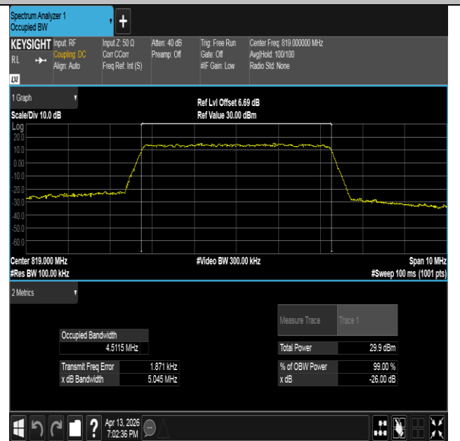
Band26(814-824)-5MHz-16QAM-26740-25RB#0-PASS
