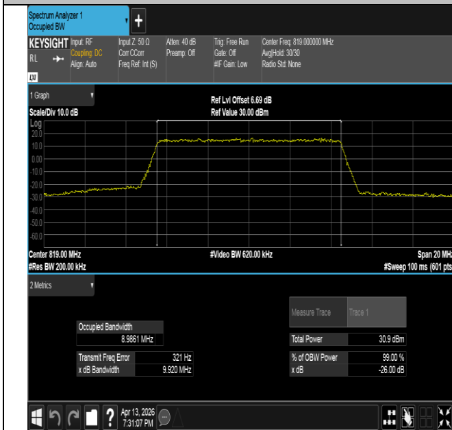
Band26(814-824)-10MHz-QPSK-26740-50RB#0-PASS
