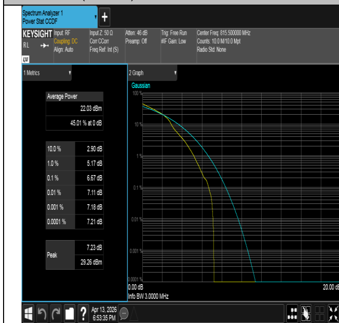
Band26(814-824)-3MHz-16QAM-26705-1RB#0-PASS
