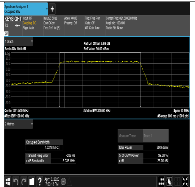
Band26(814-824)-5MHz-16QAM-26765-25RB#0-PASS
