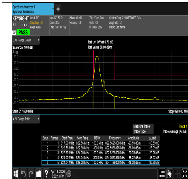
Band26(814-824)-1.4MHz-QPSK-26783-1RB#0-PASS
