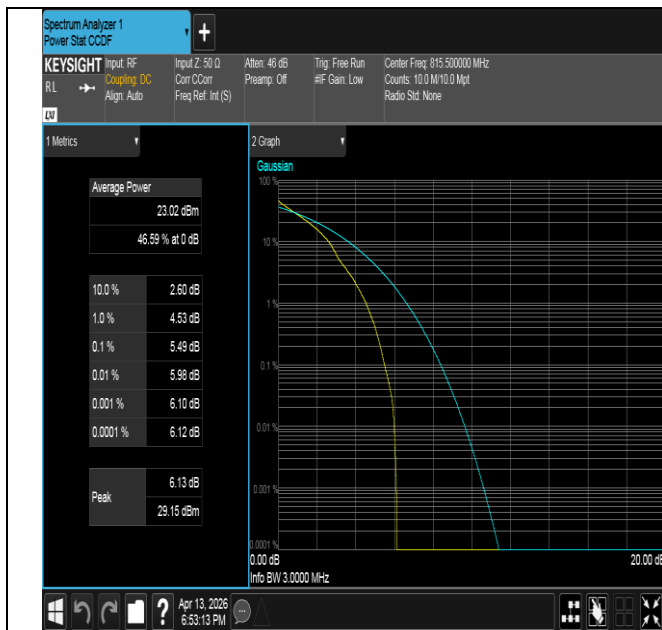
Band26(814-824)-3MHz-QPSK-26705-1RB#0-PASS
