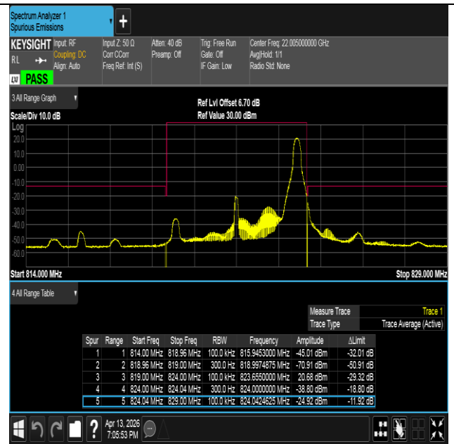
Band26(814-824)-5MHz-QPSK-26765-1RB#24-PASS
