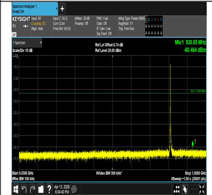
Band26(814-824)-1.4MHz-16QAM-26697-6RB#0-30~1000-PA SS
