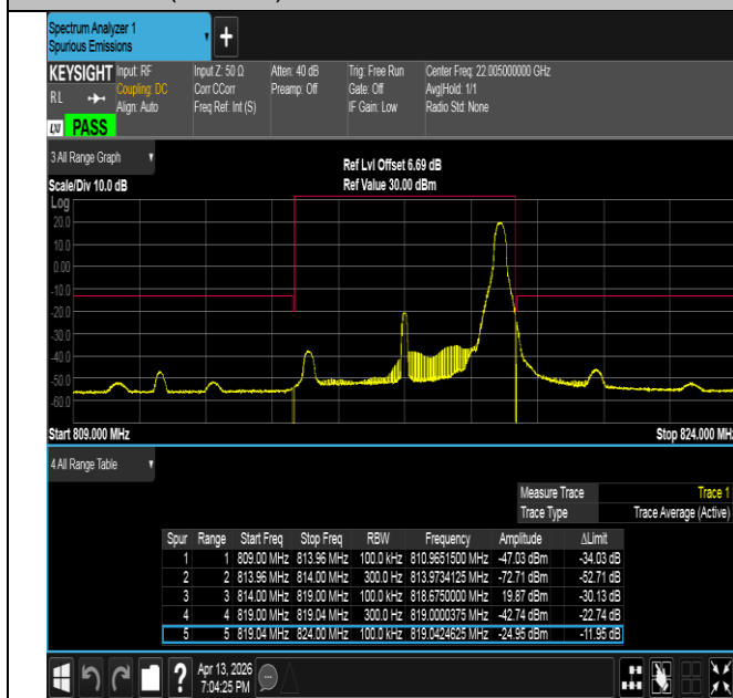
Band26(814-824)-5MHz-16QAM-26715-1RB#24-PASS
