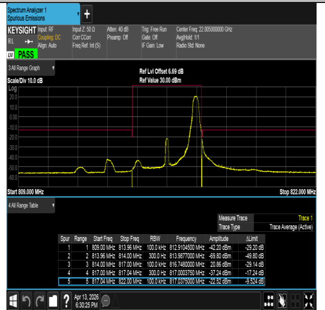
Band26(814-824)-3MHz-QPSK-26705-1RB#14-PASS
