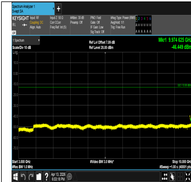
Band26(814-824)-1.4MHz-16QAM-26697-1RB#5-3000~10000 -PASS
