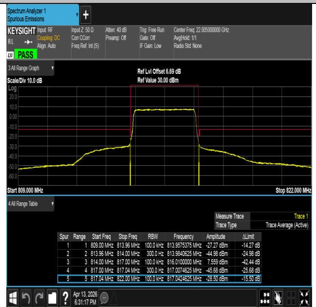
Band26(814-824)-3MHz-16QAM-26705-15RB#0-PASS
