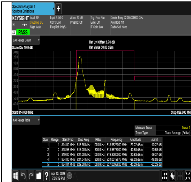
Band26(814-824)-5MHz-QPSK-26765-1RB#0-PASS
