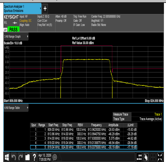
Band26(814-824)-5MHz-16QAM-26715-25RB#0-PASS
