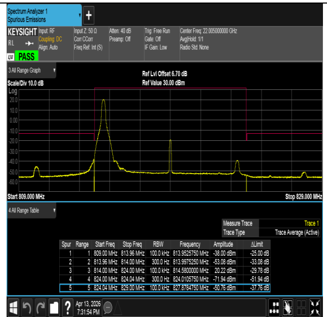
Band26(814-824)-10MHz-16QAM-26740-1RB#0-PASS
