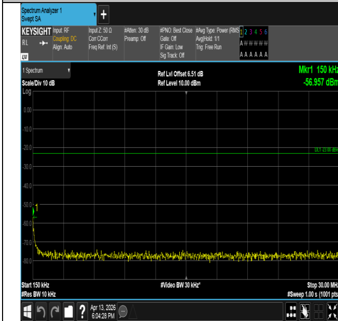
Band26(814-824)-1.4MHz-16QAM-26697-6RB#0-0.15~30-PA SS
