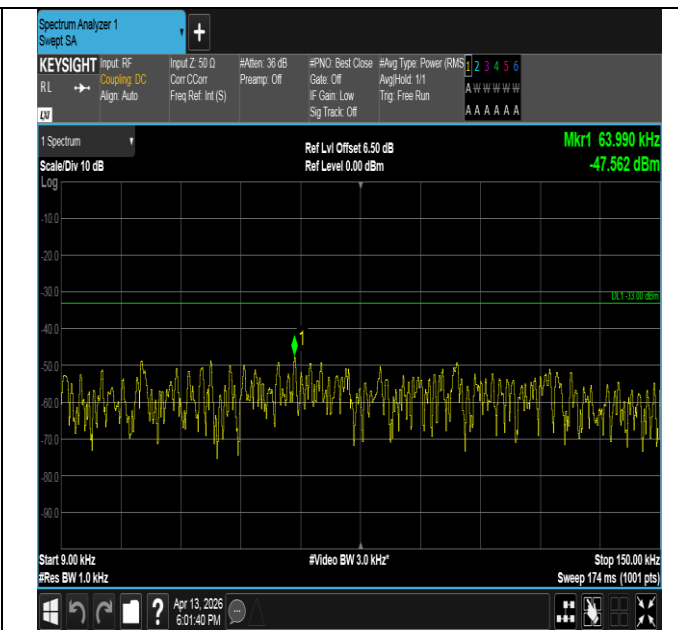
Band26(814-824)-1.4MHz-QPSK-26697-1RB#5-0.009~0.15-P ASS
