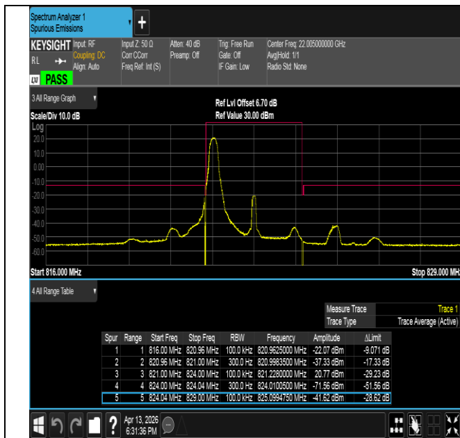
Band26(814-824)-3MHz-QPSK-26775-1RB#0-PASS
