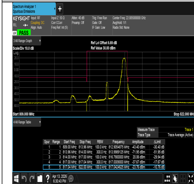
Band26(814-824)-3MHz-16QAM-26705-1RB#14-PASS
