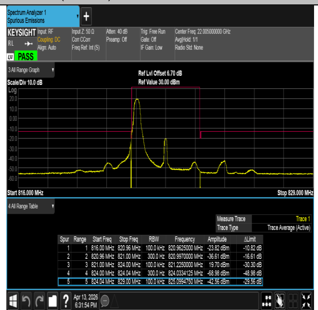
Band26(814-824)-3MHz-QPSK-26775-1RB#0-PASS
