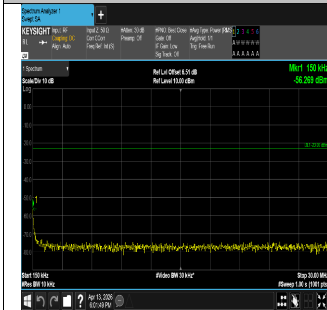
Band26(814-824)-1.4MHz-QPSK-26697-1RB#5-0.15~30-PAS S
