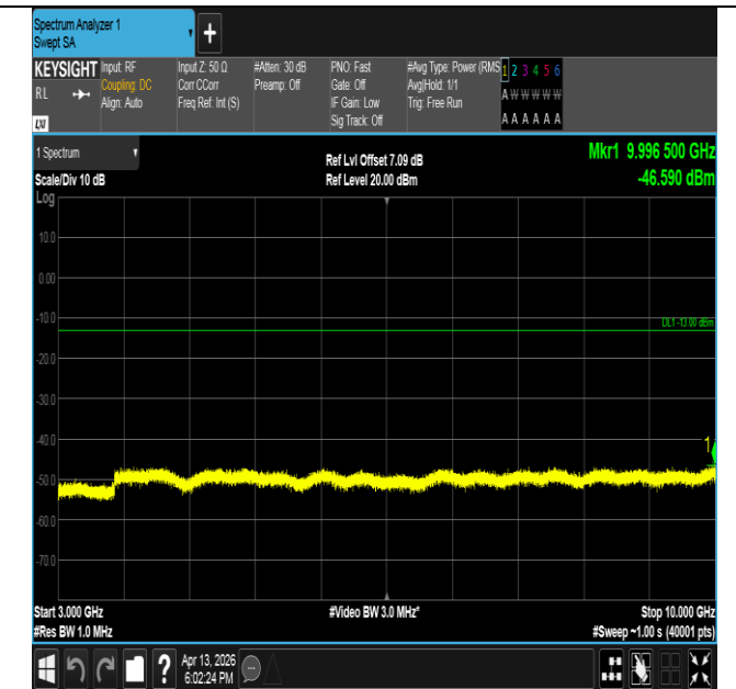
Band26(814-824)-1.4MHz-QPSK-26697-1RB#5-3000~10000- PASS
