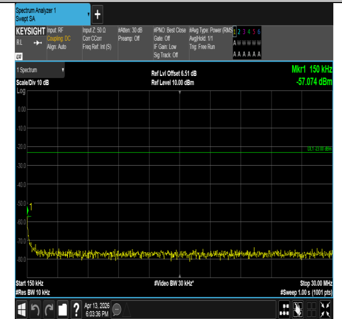
Band26(814-824)-1.4MHz-QPSK-26697-6RB#0-0.15~30-PAS S
