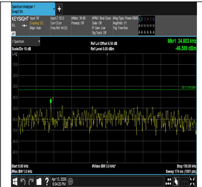
Band26(814-824)-1.4MHz-16QAM-26697-6RB#0-0.009~0.15- PASS
