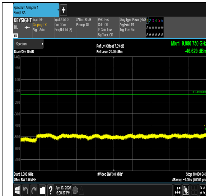
Band26(814-824)-1.4MHz-QPSK-26697-1RB#0-3000~10000- PASS
