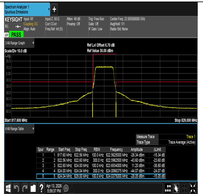
Band26(814-824)-1.4MHz-16QAM-26783-6RB#0-PASS
