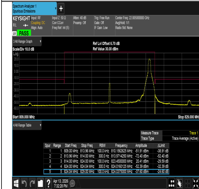
Band26(814-824)-10MHz-16QAM-26740-1RB#49-PASS
