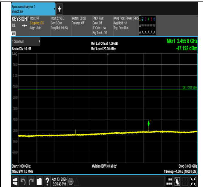
Band26(814-824)-1.4MHz-QPSK-26740-1RB#0-1000~3000-P ASS
