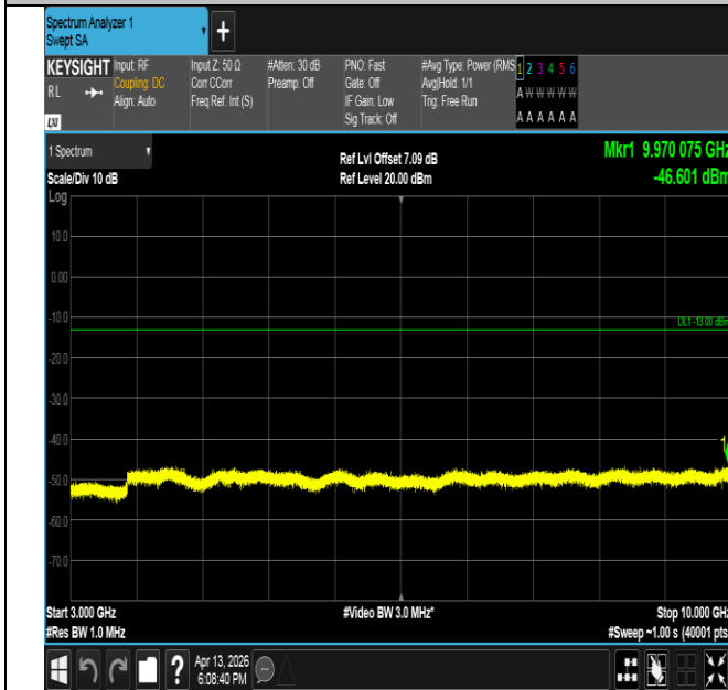
Band26(814-824)-1.4MHz-16QAM-26740-1RB#5-3000~10000 -PASS
