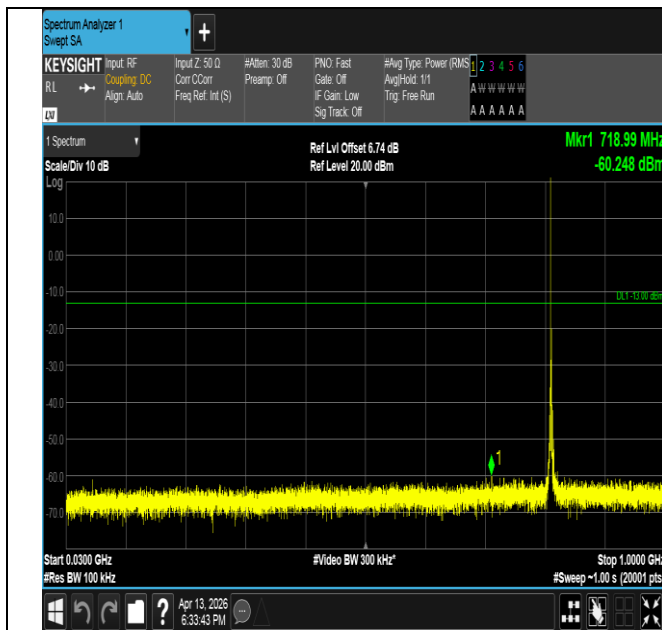
Band26(814-824)-3MHz-QPSK-26705-1RB#0-30~1000-PASS
