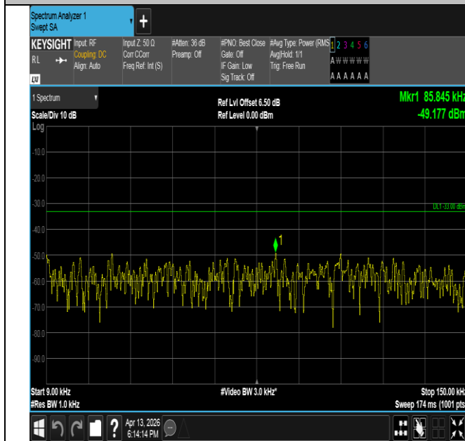
Band26(814-824)-1.4MHz-QPSK-26783-6RB#0-0.009~0.15-P ASS
