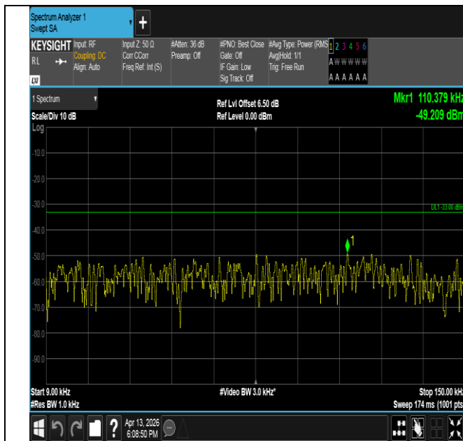
Band26(814-824)-1.4MHz-QPSK-26740-6RB#0-0.009~0.15-P
