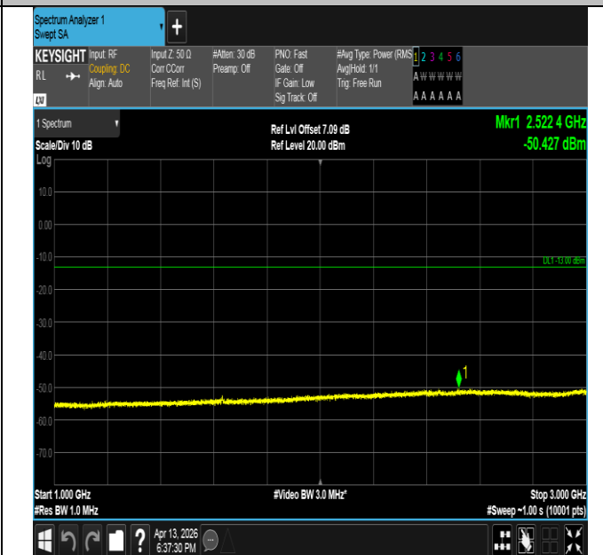
Band26(814-824)-3MHz-QPSK-26705-15RB#0-1000~3000-P
