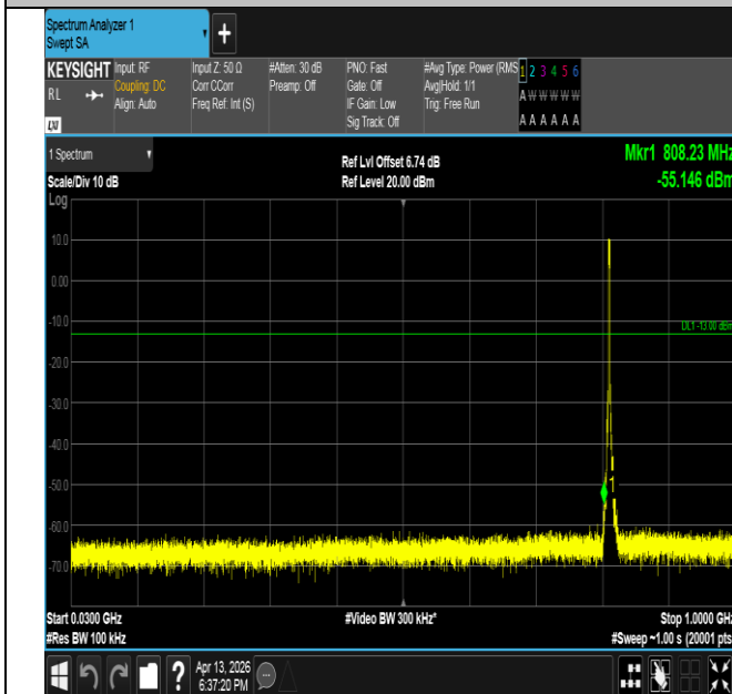
Band26(814-824)-3MHz-QPSK-26705-15RB#0-30~1000-PAS
