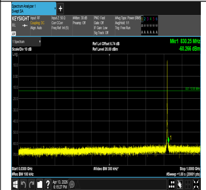
Band26(814-824)-1.4MHz-16QAM-26783-6RB#0-30~1000-PA SS
