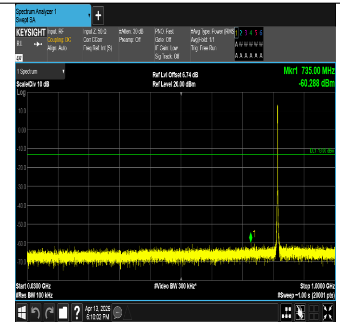
Band26(814-824)-1.4MHz-16QAM-26740-6RB#0-30~1000-PA
