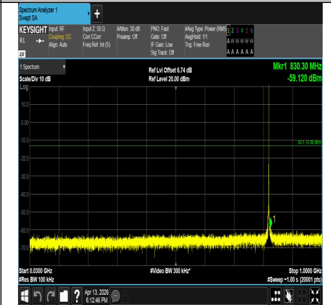
Band26(814-824)-1.4MHz-QPSK-26783-1RB#5-30~1000-PAS S
