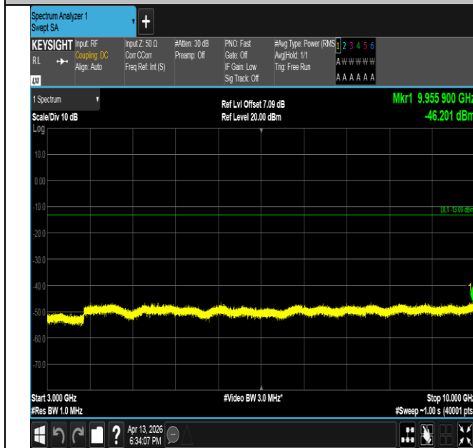
Band26(814-824)-3MHz-QPSK-26705-1RB#0-3000~10000-P ASS
