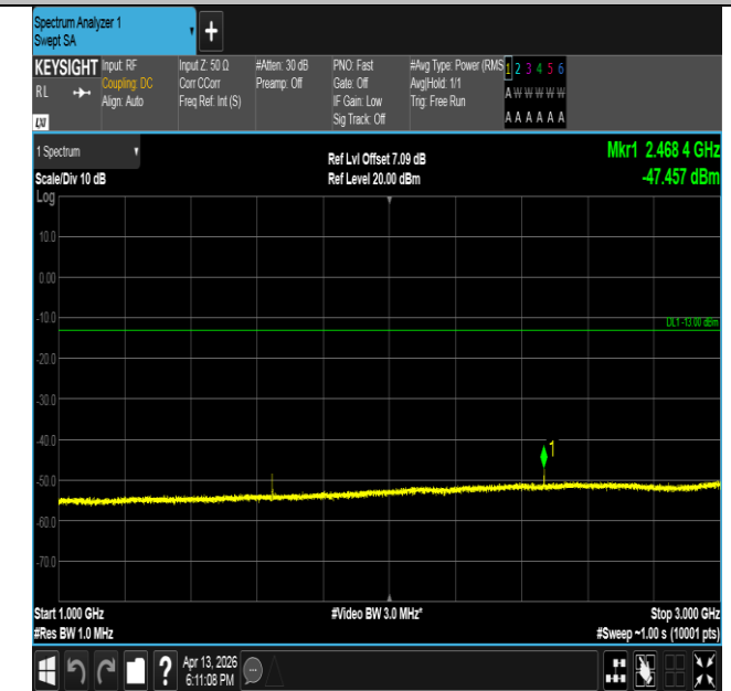
Band26(814-824)-1.4MHz-QPSK-26783-1RB#0-1000~3000-P ASS
