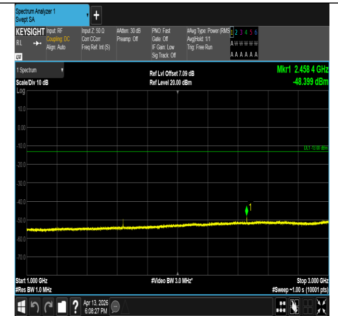
Band26(814-824)-1.4MHz-16QAM-26740-1RB#5-1000~3000- PASS
