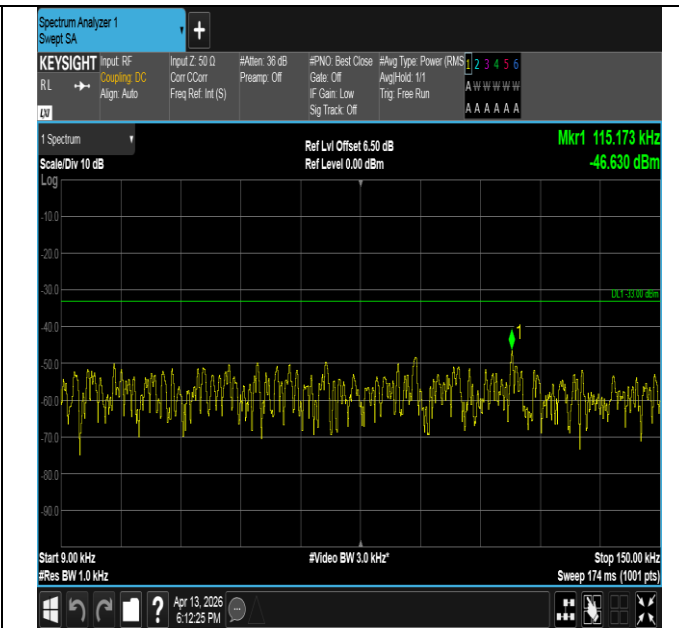
Band26(814-824)-1.4MHz-QPSK-26783-1RB#5-0.009~0.15-P ASS
