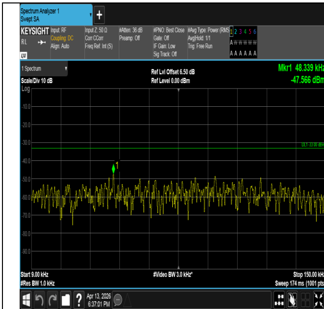
Band26(814-824)-3MHz-QPSK-26705-15RB#0-0.009~0.15-P
