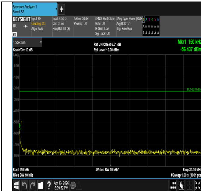
Band26(814-824)-1.4MHz-16QAM-26740-6RB#0-0.15~30-PA
