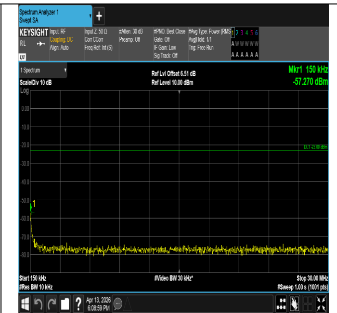
Band26(814-824)-1.4MHz-QPSK-26740-6RB#0-0.15~30-PAS
