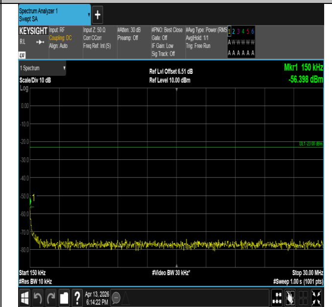
Band26(814-824)-1.4MHz-QPSK-26783-6RB#0-0.15~30-PAS S
