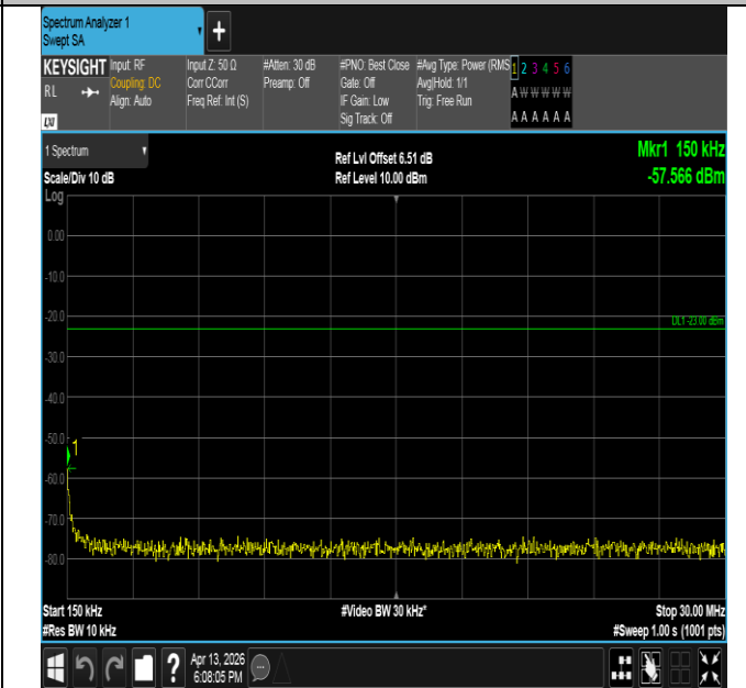
Band26(814-824)-1.4MHz-16QAM-26740-1RB#5-0.15~30-PA SS
