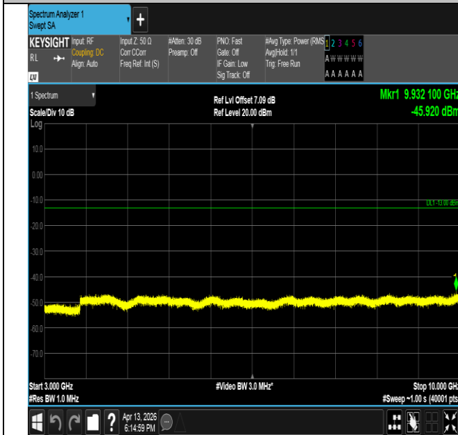
Band26(814-824)-1.4MHz-QPSK-26783-6RB#0-3000~10000-
