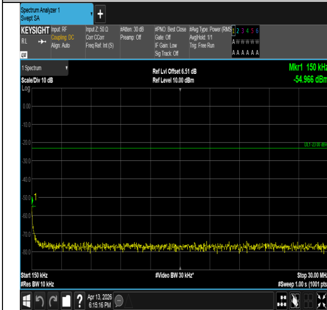
Band26(814-824)-1.4MHz-16QAM-26783-6RB#0-0.15~30-PA SS
