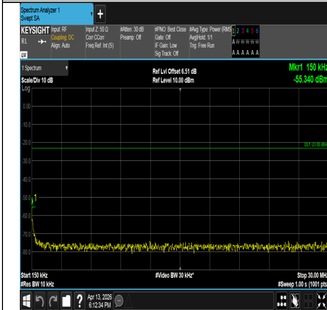
Band26(814-824)-1.4MHz-QPSK-26783-1RB#5-0.15~30-PAS S
