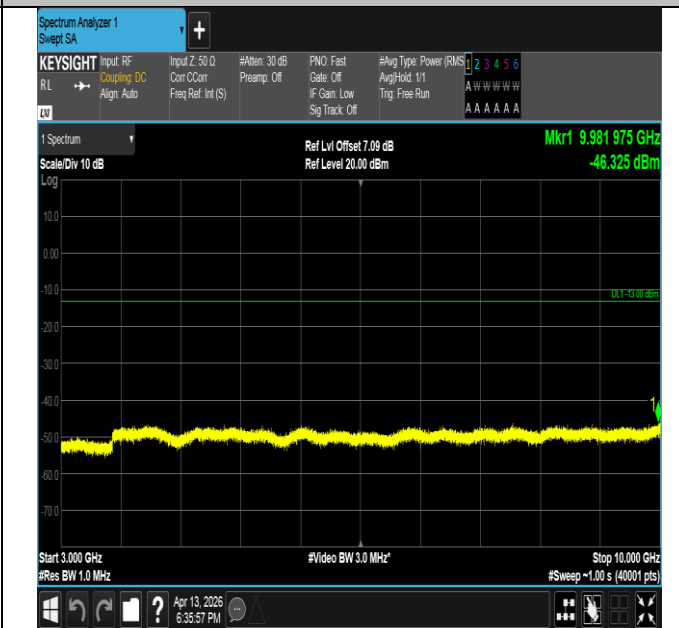
Band26(814-824)-3MHz-QPSK-26705-1RB#14-3000~10000-P
