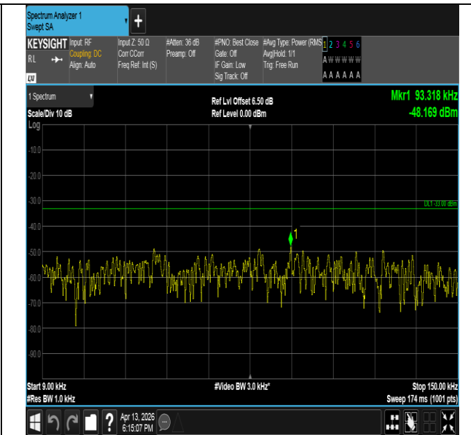
Band26(814-824)-1.4MHz-16QAM-26783-6RB#0-0.009~0.15- PASS
