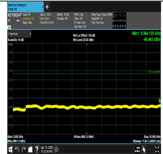
Band26(814-824)-1.4MHz-16QAM-26783-1RB#0-3000~10000
