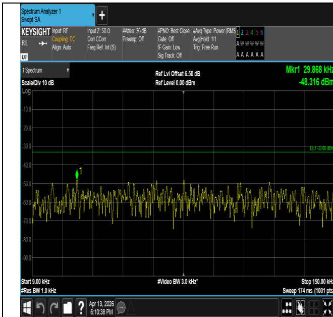
Band26(814-824)-1.4MHz-QPSK-26783-1RB#0-0.009~0.15-P ASS
