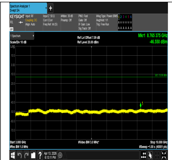
Band26(814-824)-1.4MHz-QPSK-26783-1RB#5-3000~10000- PASS
