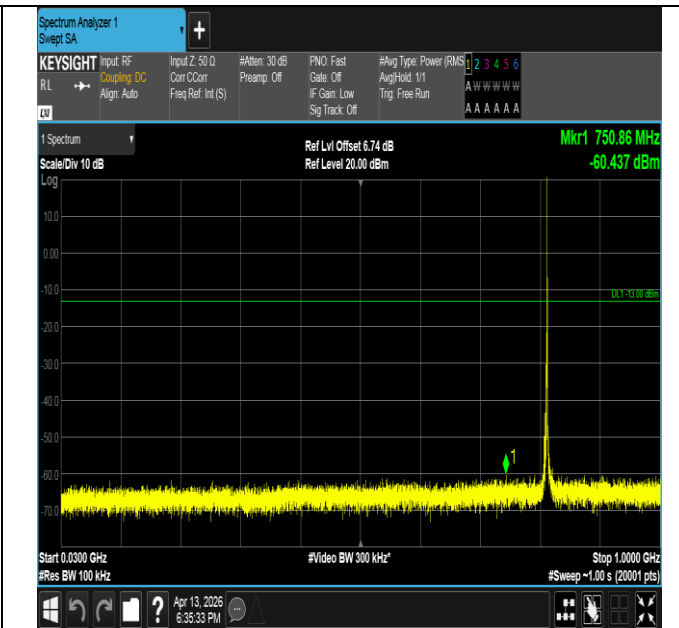
Band26(814-824)-3MHz-QPSK-26705-1RB#14-30~1000-PAS
