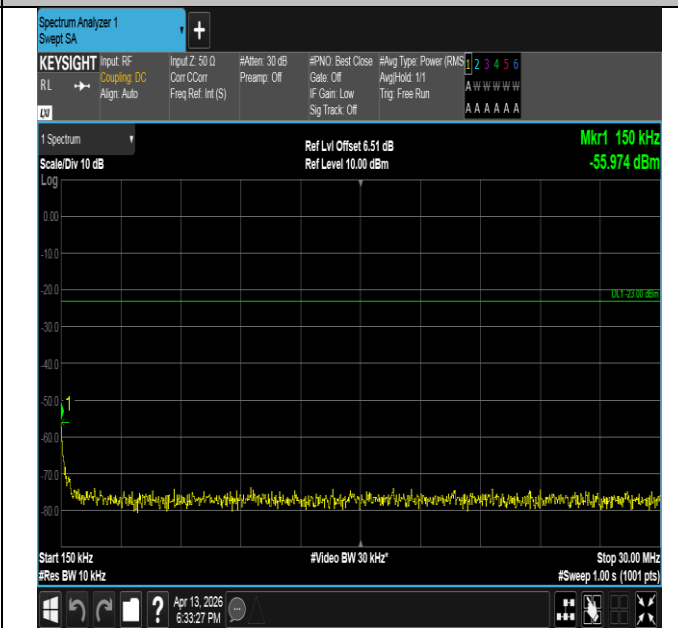
Band26(814-824)-3MHz-QPSK-26705-1RB#0-0.15~30-PASS
