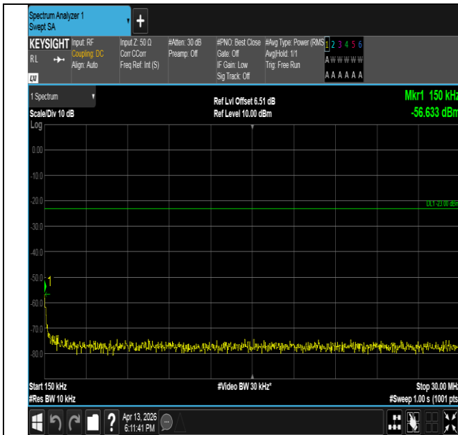
Band26(814-824)-1.4MHz-16QAM-26783-1RB#0-0.15~30-PA
