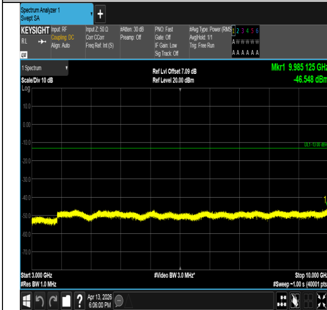
Band26(814-824)-1.4MHz-QPSK-26740-1RB#0-3000~10000- PASS
