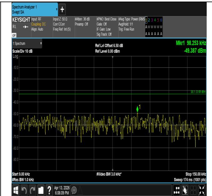
Band26(814-824)-1.4MHz-16QAM-26740-1RB#0-0.009~0.15- PASS
