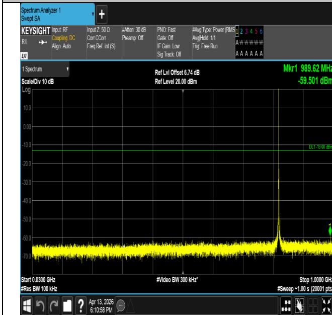
Band26(814-824)-1.4MHz-QPSK-26783-1RB#0-30~1000-PAS S
