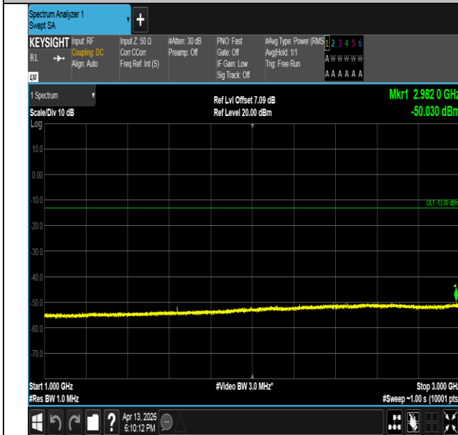
Band26(814-824)-1.4MHz-16QAM-26740-6RB#0-1000~3000-
