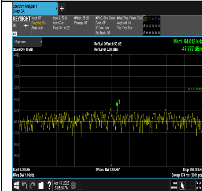
Band26(814-824)-1.4MHz-QPSK-26740-1RB#0-0.009~0.15-P ASS
