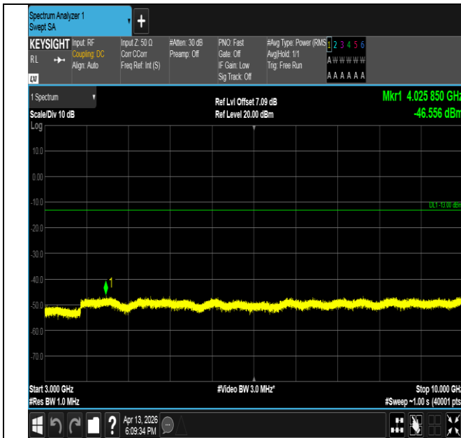
Band26(814-824)-1.4MHz-QPSK-26740-6RB#0-3000~10000- PASS
