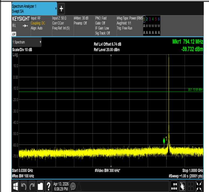
Band26(814-824)-1.4MHz-16QAM-26740-1RB#0-30~1000-PA SS
