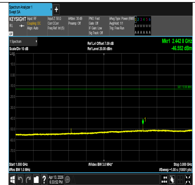
Band26(814-824)-3MHz-QPSK-26705-1RB#0-1000~3000-PA SS
