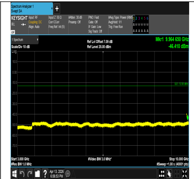
Band26(814-824)-1.4MHz-16QAM-26740-1RB#0-3000~10000 -PASS
