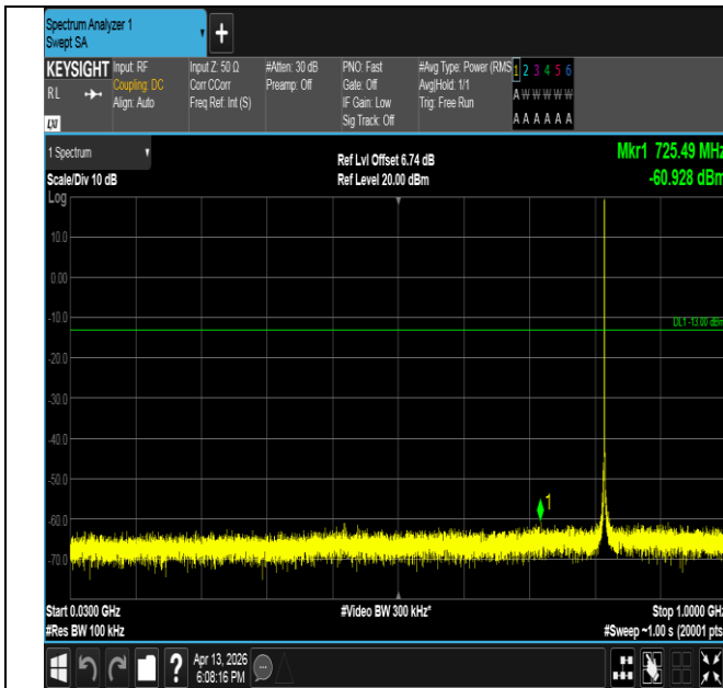
Band26(814-824)-1.4MHz-16QAM-26740-1RB#5-30~1000-PA SS
