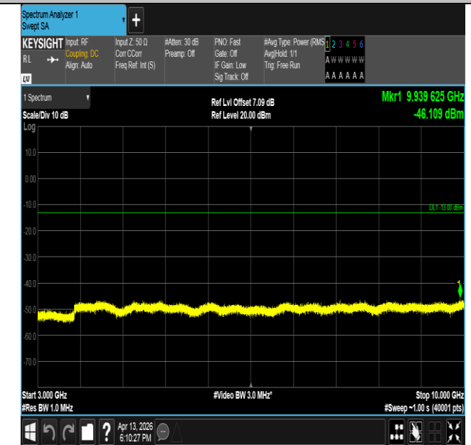
Band26(814-824)-1.4MHz-16QAM-26740-6RB#0-3000~10000
