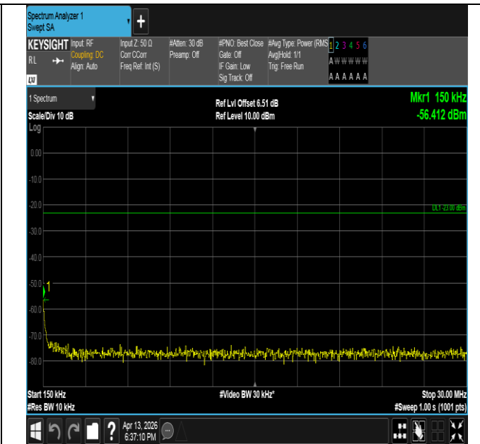
Band26(814-824)-3MHz-QPSK-26705-15RB#0-0.15~30-PAS
