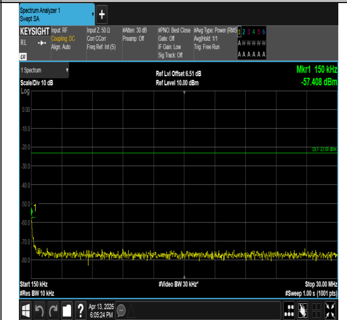
Band26(814-824)-1.4MHz-QPSK-26740-1RB#0-0.15~30-PAS S
