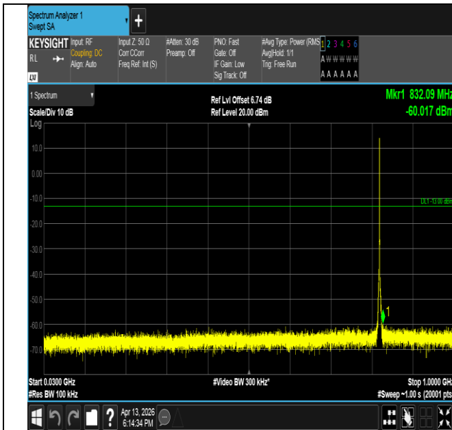
Band26(814-824)-1.4MHz-QPSK-26783-6RB#0-30~1000-PAS
