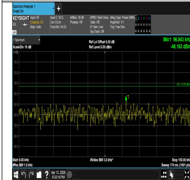
Band26(814-824)-3MHz-QPSK-26705-1RB#0-0.009~0.15-PA SS
