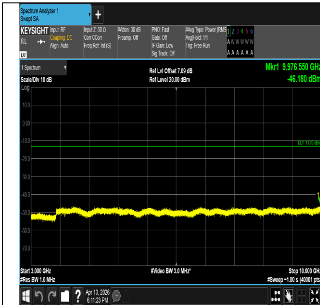
Band26(814-824)-1.4MHz-QPSK-26783-1RB#0-3000~10000- PASS
