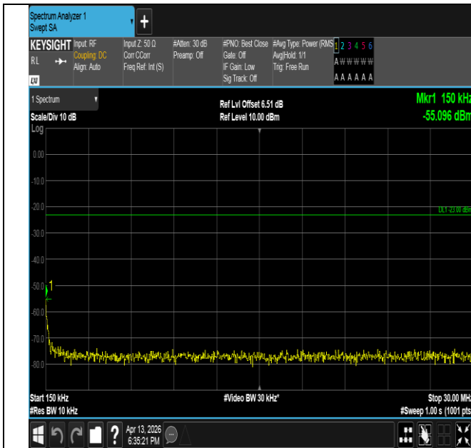
Band26(814-824)-3MHz-QPSK-26705-1RB#14-0.15~30-PAS
