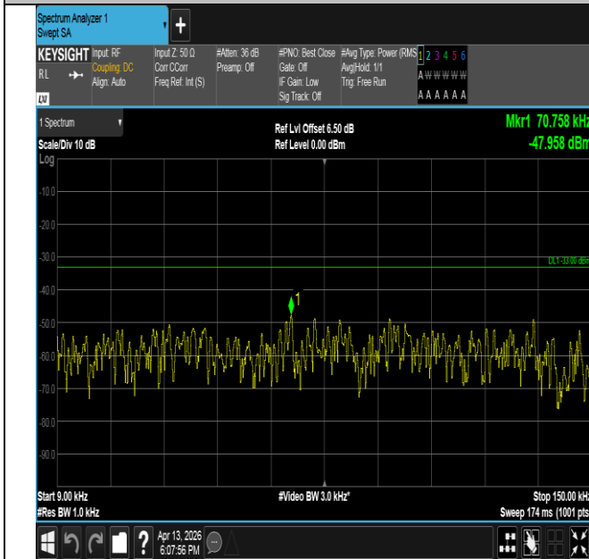
Band26(814-824)-1.4MHz-16QAM-26740-1RB#5-0.009~0.15- PASS
