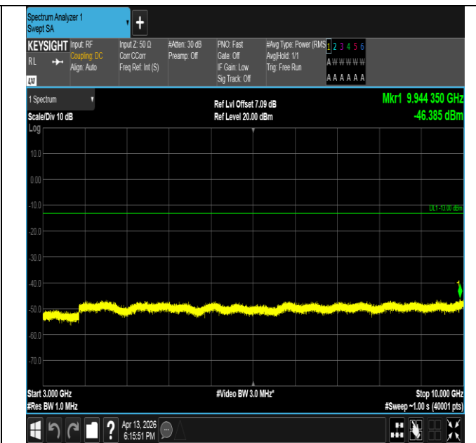
Band26(814-824)-1.4MHz-16QAM-26783-6RB#0-3000~10000 -PASS
