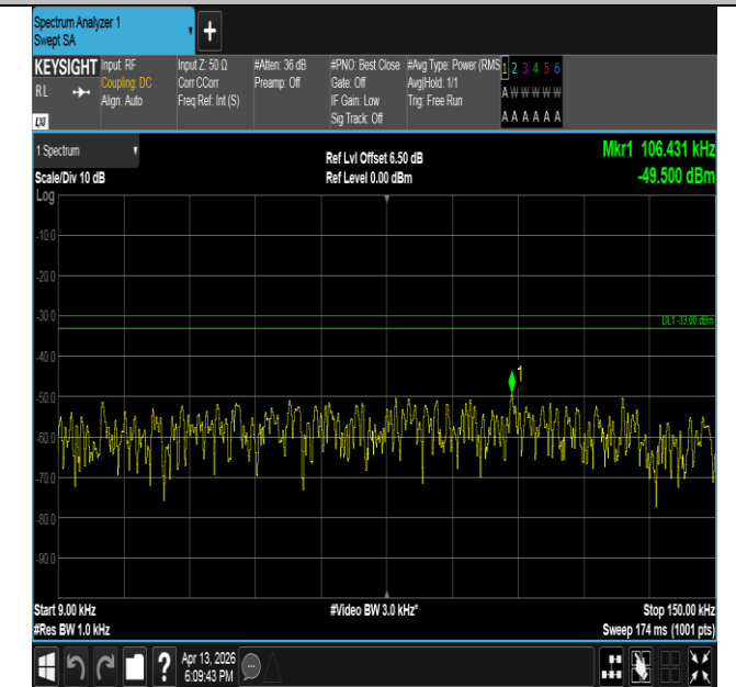
Band26(814-824)-1.4MHz-16QAM-26740-6RB#0-0.009~0.15- PASS
