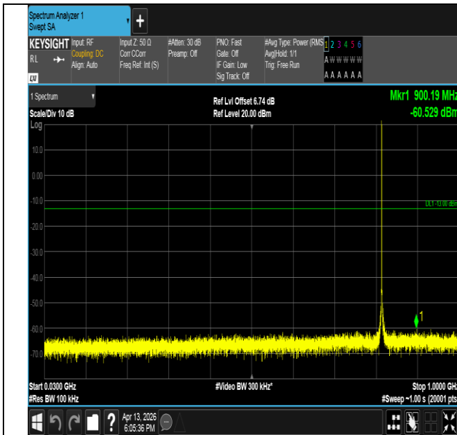
Band26(814-824)-1.4MHz-QPSK-26740-1RB#0-30~1000-PAS S
