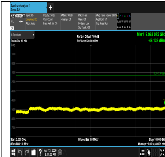
Band26(814-824)-1.4MHz-16QAM-26783-1RB#5-3000~10000 -PASS
