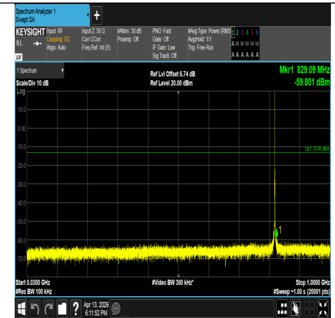
Band26(814-824)-1.4MHz-16QAM-26783-1RB#0-30~1000-PA
