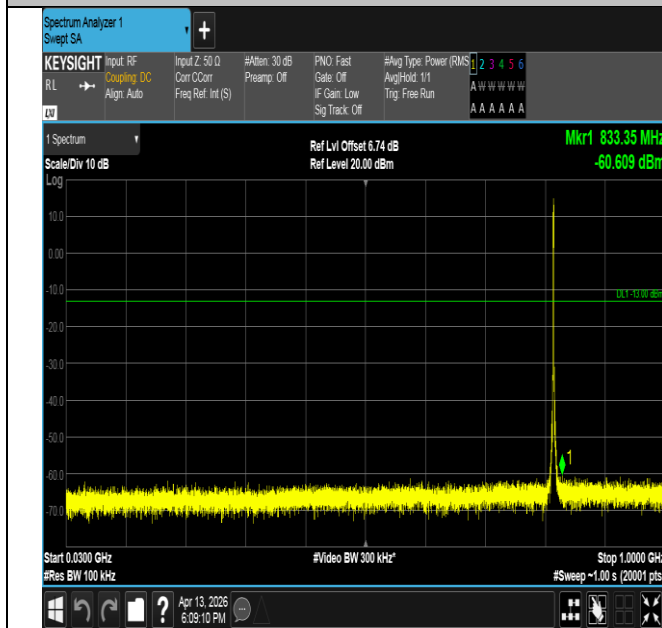
Band26(814-824)-1.4MHz-QPSK-26740-6RB#0-30~1000-PAS
