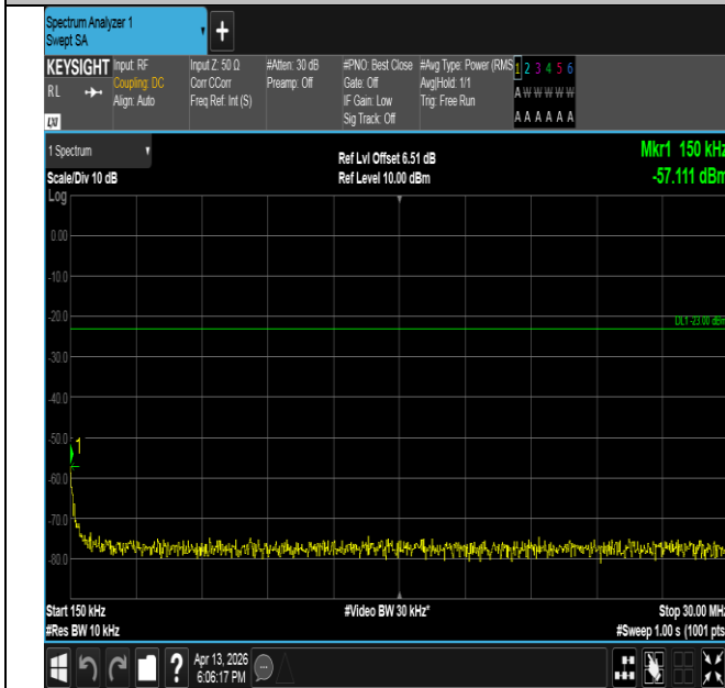
Band26(814-824)-1.4MHz-16QAM-26740-1RB#0-0.15~30-PA SS
