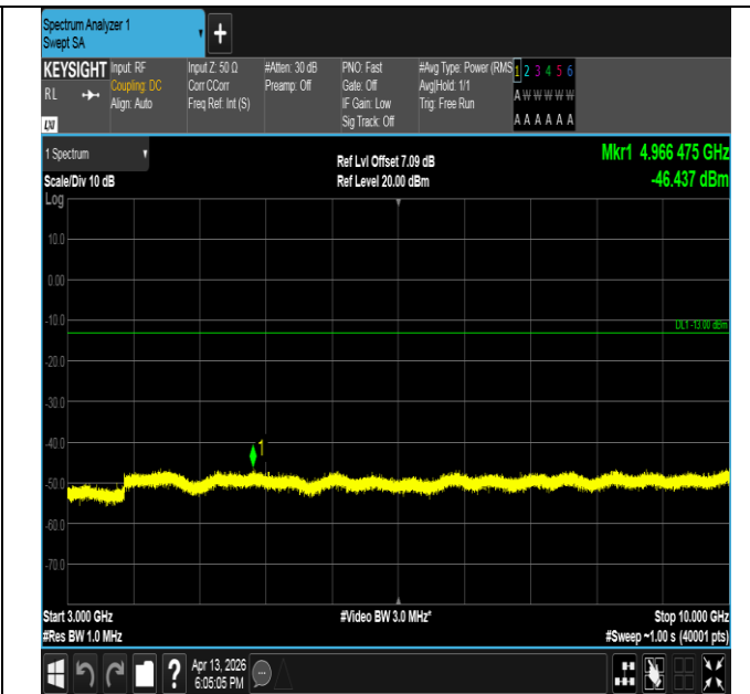
Band26(814-824)-1.4MHz-16QAM-26697-6RB#0-3000~10000 -PASS
