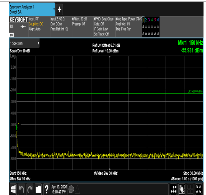
Band26(814-824)-1.4MHz-QPSK-26783-1RB#0-0.15~30-PAS S
