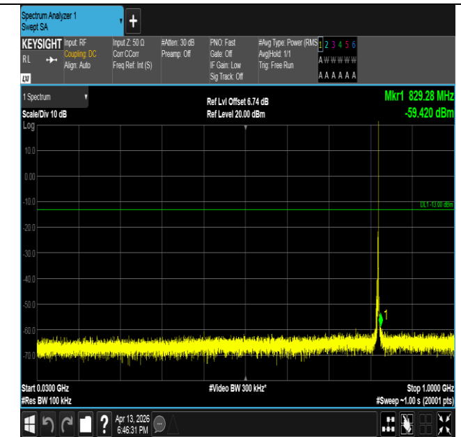
Band26(814-824)-3MHz-QPSK-26775-1RB#14-30~1000-PAS
