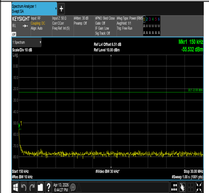
Band26(814-824)-3MHz-QPSK-26775-1RB#0-0.15~30-PASS
