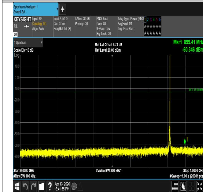
Band26(814-824)-3MHz-16QAM-26740-1RB#14-30~1000-PA SS
