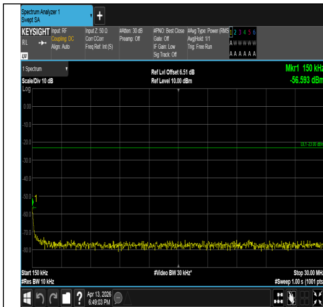
Band26(814-824)-3MHz-16QAM-26775-15RB#0-0.15~30-PA
