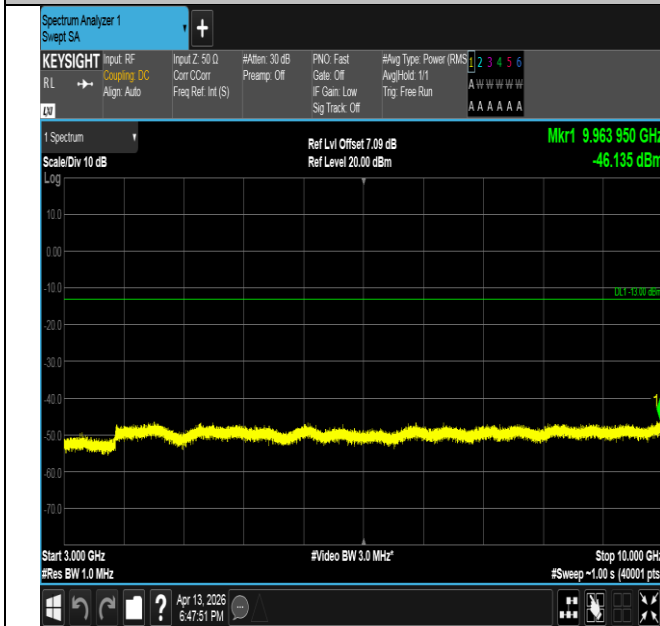
Band26(814-824)-3MHz-16QAM-26775-1RB#14-3000~10000 -PASS
