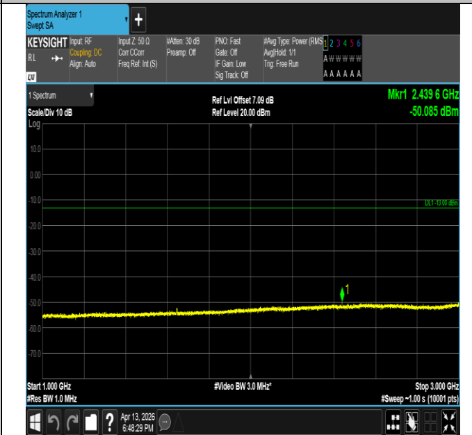
Band26(814-824)-3MHz-QPSK-26775-15RB#0-1000~3000-P ASS
