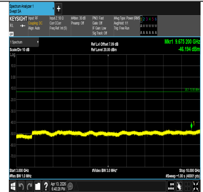
Band26(814-824)-3MHz-16QAM-26740-1RB#0-3000~10000-PASS
