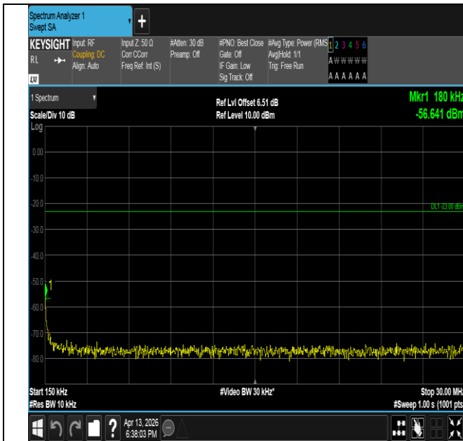
Band26(814-824)-3MHz-16QAM-26705-15RB#0-0.15~30-PA
