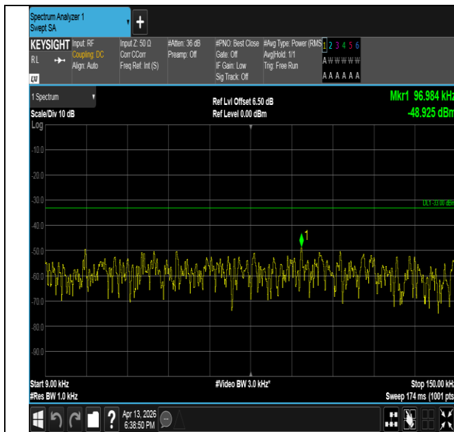
Band26(814-824)-3MHz-QPSK-26740-1RB#0-0.009~0.15-PA SS
