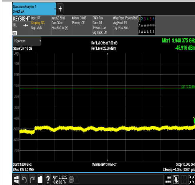
Band26(814-824)-3MHz-QPSK-26775-1RB#0-3000~10000-P ASS
