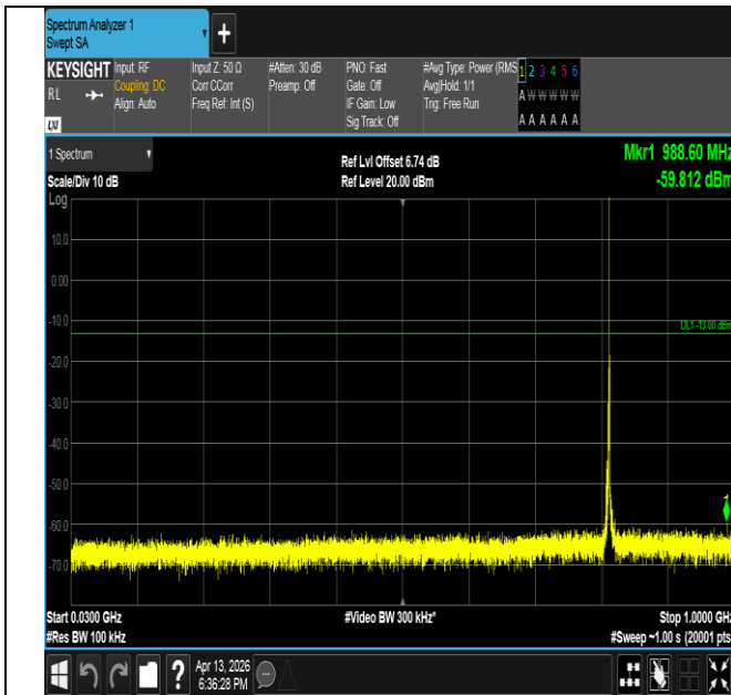
Band26(814-824)-3MHz-16QAM-26705-1RB#14-30~1000-PA SS
