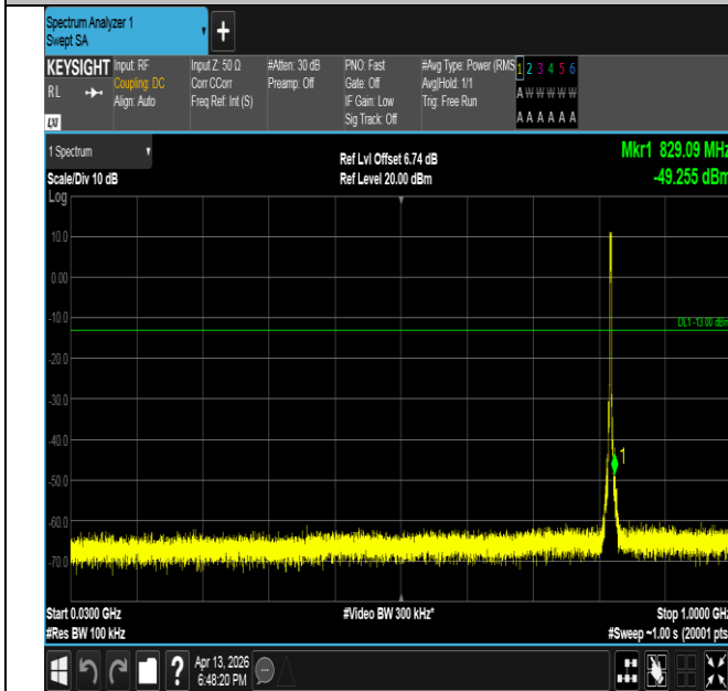
Band26(814-824)-3MHz-QPSK-26775-15RB#0-30~1000-PAS S
