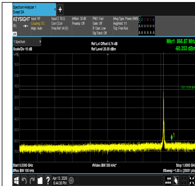
Band26(814-824)-3MHz-QPSK-26775-1RB#0-30~1000-PASS
