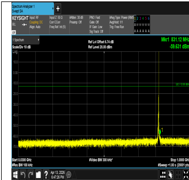
Band26(814-824)-3MHz-16QAM-26775-1RB#14-30~1000-PA SS
