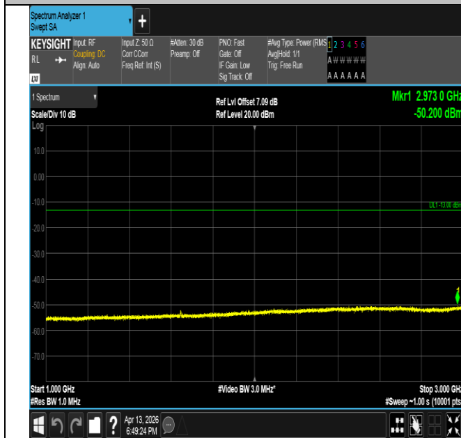
Band26(814-824)-3MHz-16QAM-26775-15RB#0-1000~3000-
