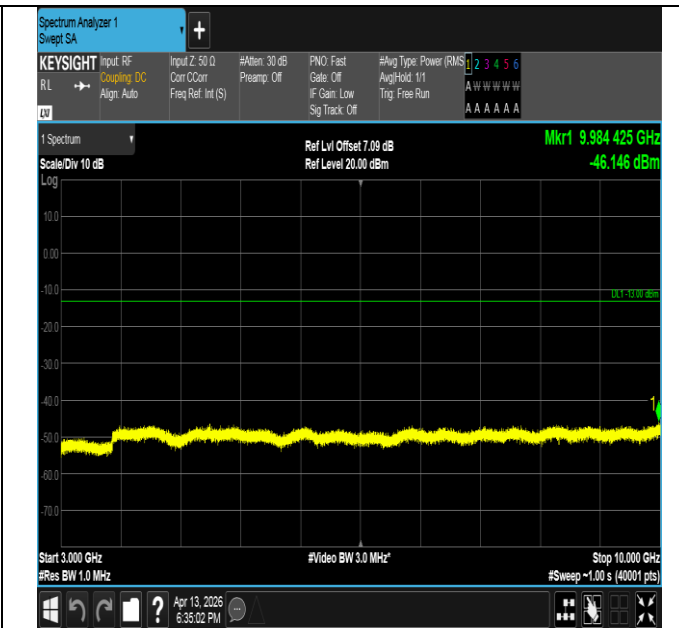
Band26(814-824)-3MHz-16QAM-26705-1RB#0-3000~10000- PASS
