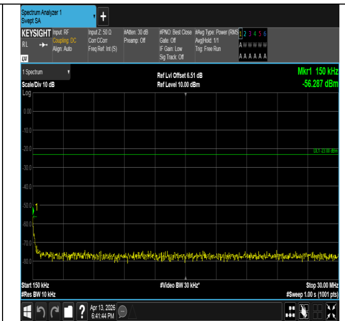
Band26(814-824)-3MHz-16QAM-26740-1RB#14-0.15~30-PAS S
