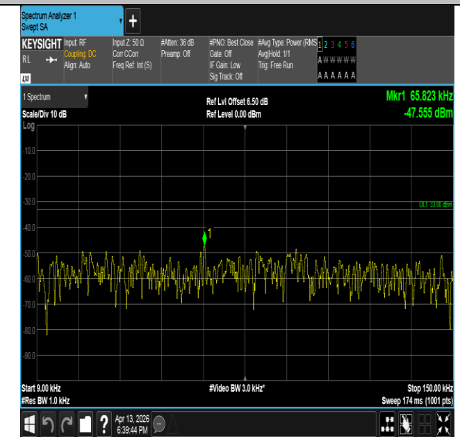
Band26(814-824)-3MHz-16QAM-26740-1RB#0-0.009~0.15-P
