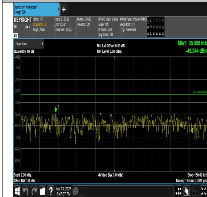
Band26(814-824)-3MHz-16QAM-26775-1RB#14-0.009~0.15- PASS
