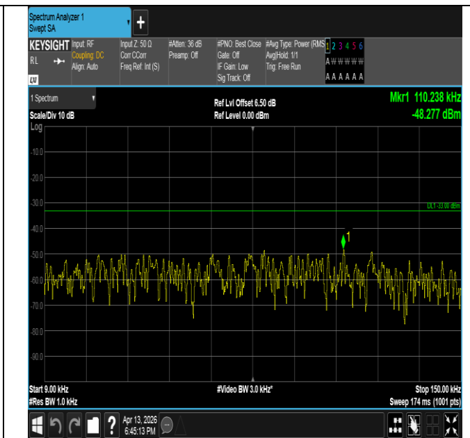
Band26(814-824)-3MHz-16QAM-26775-1RB#0-0.009~0.15-P ASS
