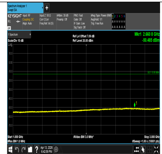
Band26(814-824)-3MHz-QPSK-26740-15RB#0-1000~3000-P
