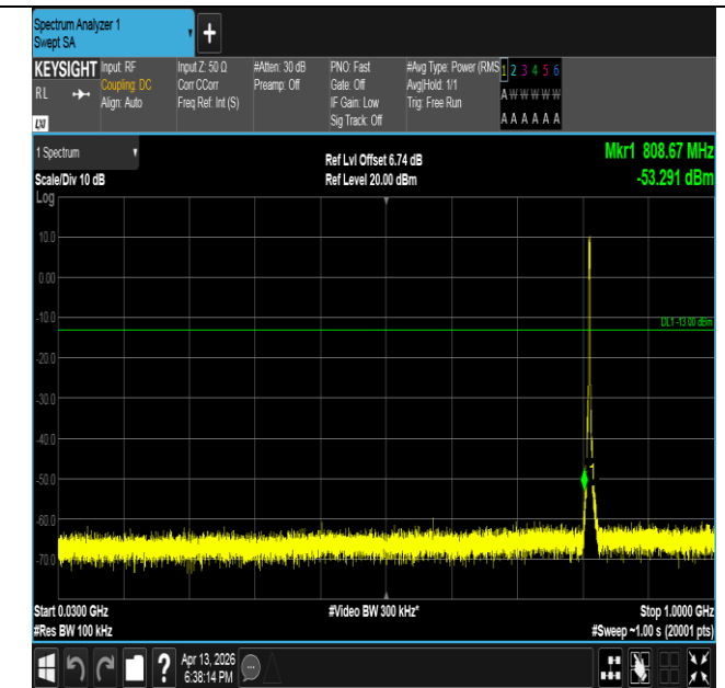
Band26(814-824)-3MHz-16QAM-26705-15RB#0-30~1000-PA
