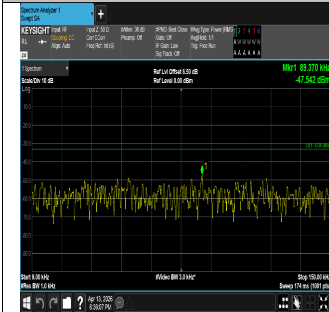
Band26(814-824)-3MHz-16QAM-26705-1RB#14-0.009~0.15- PASS
