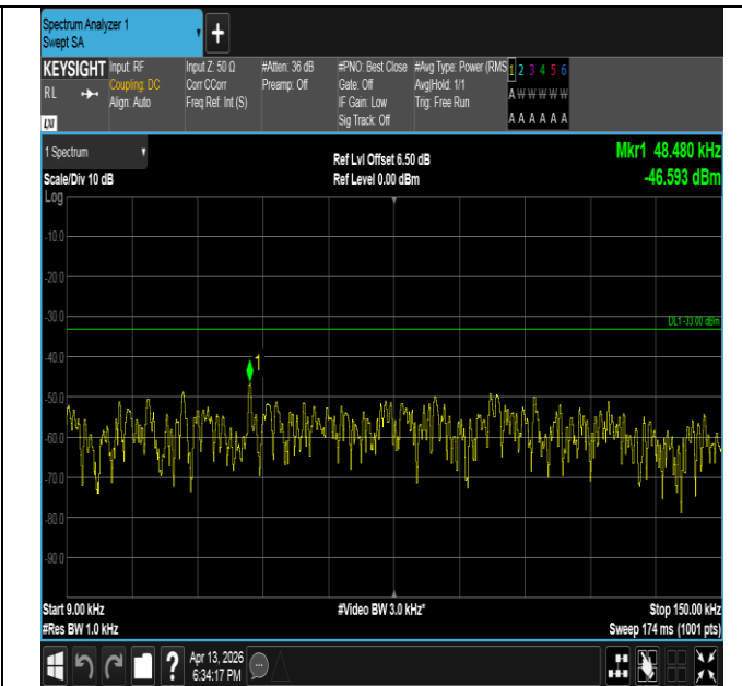
Band26(814-824)-3MHz-16QAM-26705-1RB#0-0.009~0.15-P ASS
