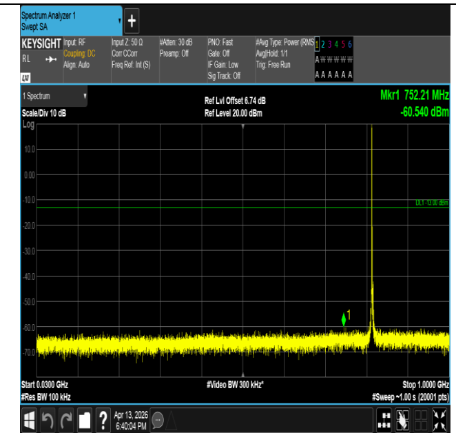
Band26(814-824)-3MHz-16QAM-26740-1RB#0-30~1000-PAS
