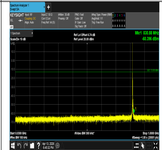
Band26(814-824)-3MHz-16QAM-26775-1RB#0-30~1000-PAS S
