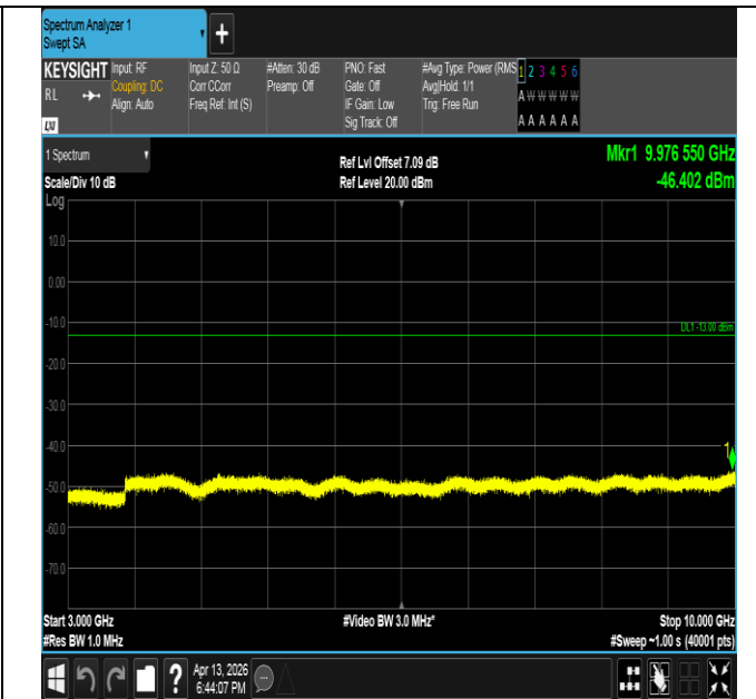
Band26(814-824)-3MHz-16QAM-26740-15RB#0-3000~10000 -PASS
