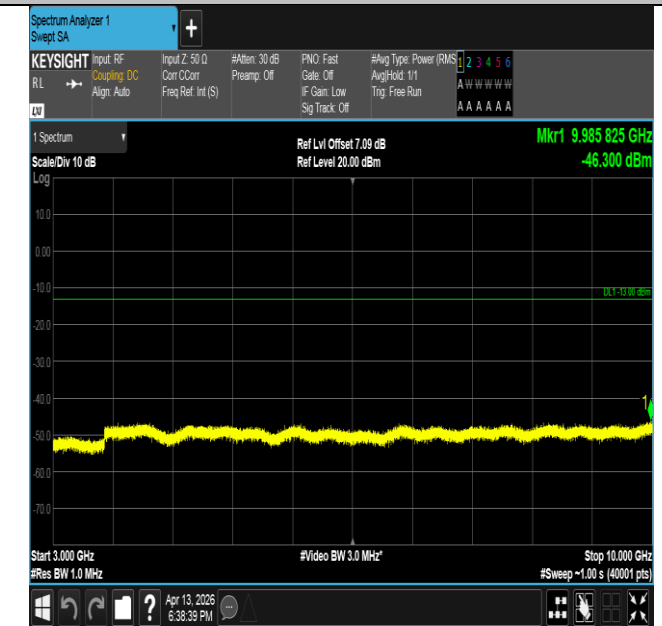
Band26(814-824)-3MHz-16QAM-26705-15RB#0-3000~10000
