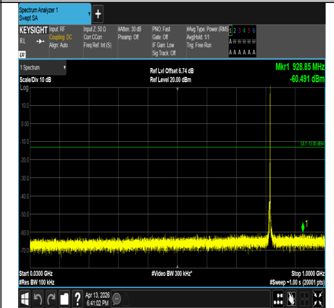
Band26(814-824)-3MHz-QPSK-26740-1RB#14-30~1000-PAS S
