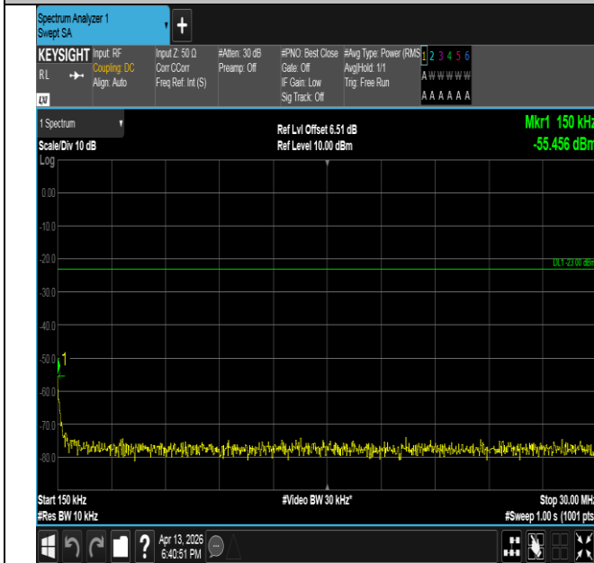
Band26(814-824)-3MHz-QPSK-26740-1RB#14-0.15~30-PAS S
