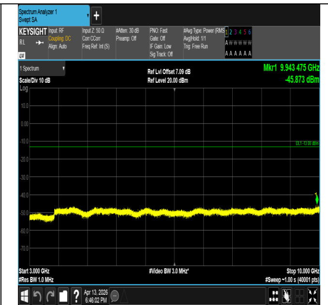
Band26(814-824)-3MHz-16QAM-26775-1RB#0-3000~10000- PASS
