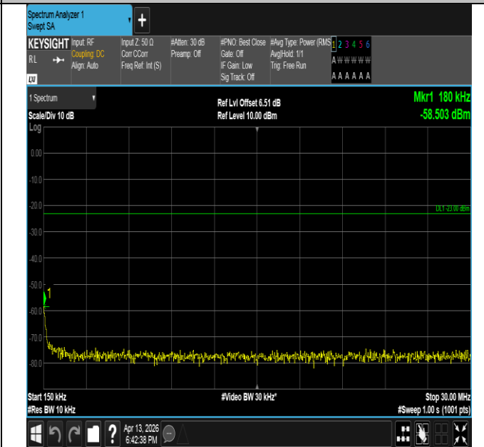
Band26(814-824)-3MHz-QPSK-26740-15RB#0-0.15~30-PAS S
