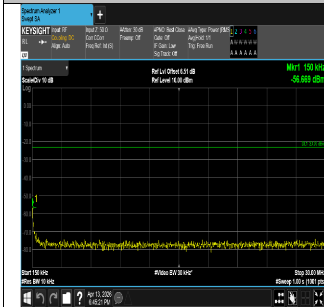
Band26(814-824)-3MHz-16QAM-26775-1RB#0-0.15~30-PAS S
