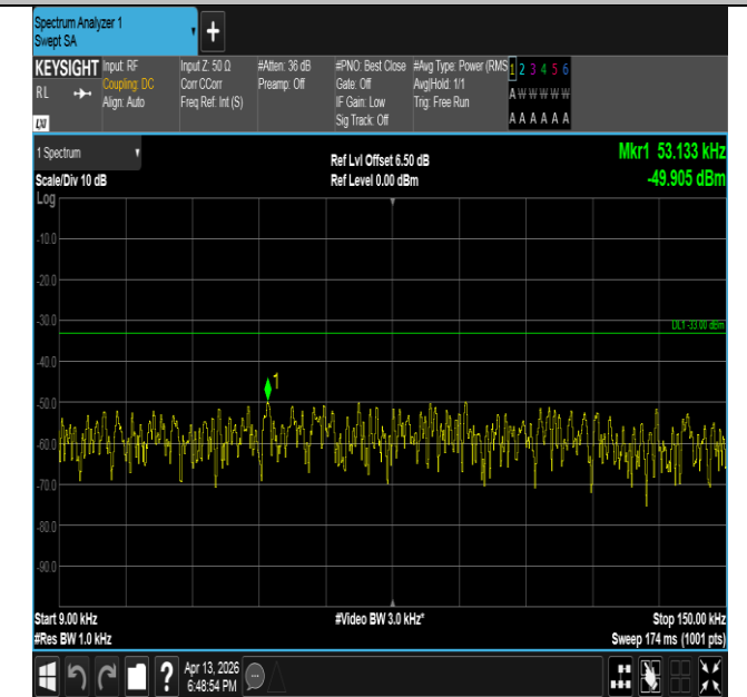
Band26(814-824)-3MHz-16QAM-26775-15RB#0-0.009~0.15- PASS
