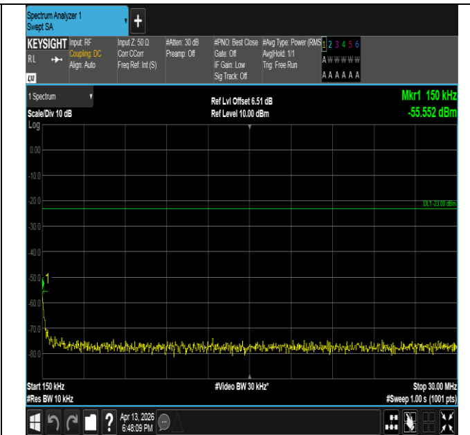
Band26(814-824)-3MHz-QPSK-26775-15RB#0-0.15~30-PAS S
