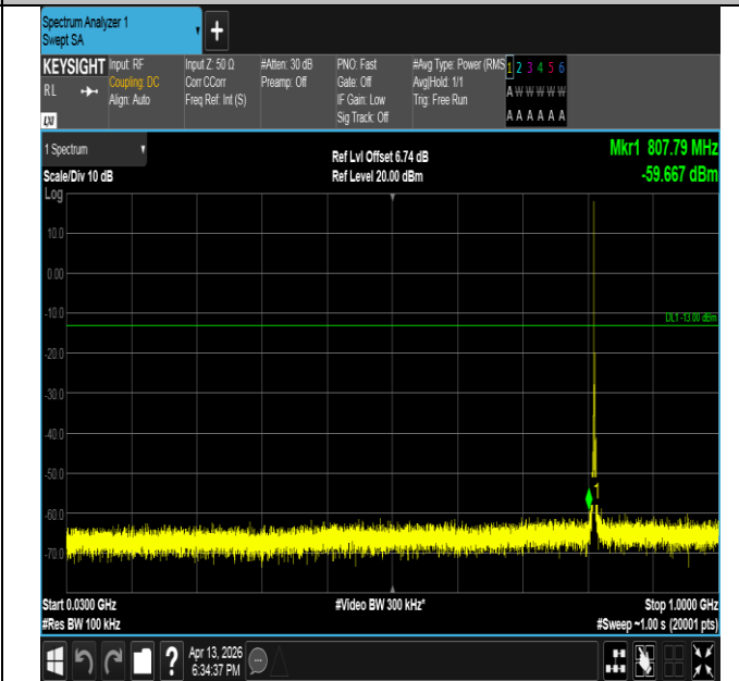
Band26(814-824)-3MHz-16QAM-26705-1RB#0-30~1000-PAS S
