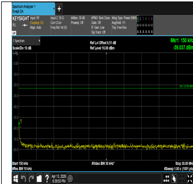
Band26(814-824)-3MHz-16QAM-26740-1RB#0-0.15~30-PAS
