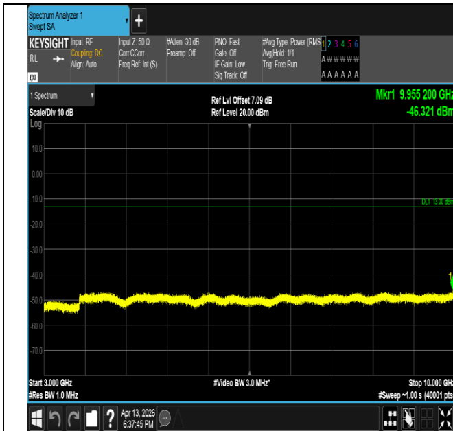
Band26(814-824)-3MHz-QPSK-26705-15RB#0-3000~10000- PASS
