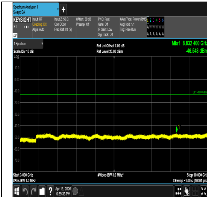
Band26(814-824)-3MHz-QPSK-26740-1RB#0-3000~10000-P ASS
