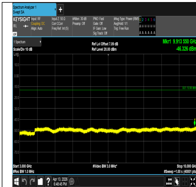
Band26(814-824)-3MHz-QPSK-26775-15RB#0-3000~10000- PASS
