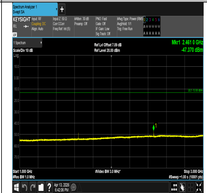
Band26(814-824)-3MHz-16QAM-26740-1RB#14-1000~3000- PASS
