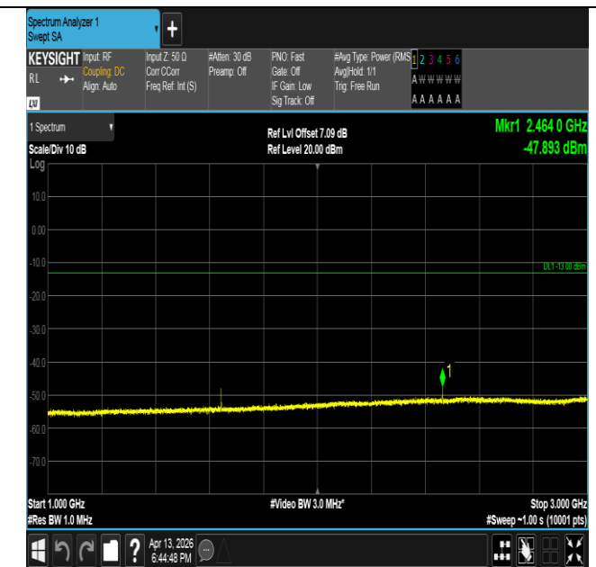
Band26(814-824)-3MHz-QPSK-26775-1RB#0-1000~3000-PA SS
