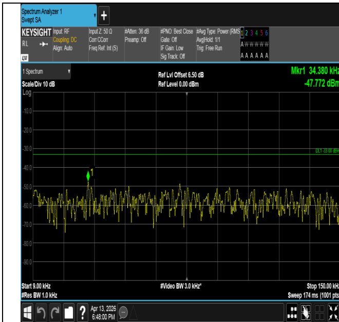
Band26(814-824)-3MHz-QPSK-26775-15RB#0-0.009~0.15-P ASS
