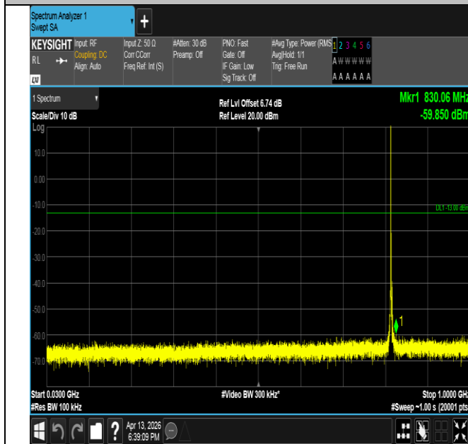
Band26(814-824)-3MHz-QPSK-26740-1RB#0-30~1000-PASS
