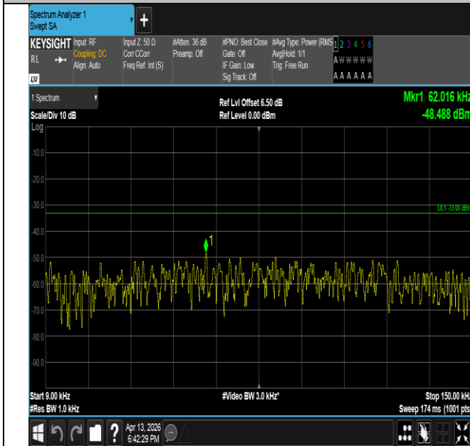
Band26(814-824)-3MHz-QPSK-26740-15RB#0-0.009~0.15-P ASS
