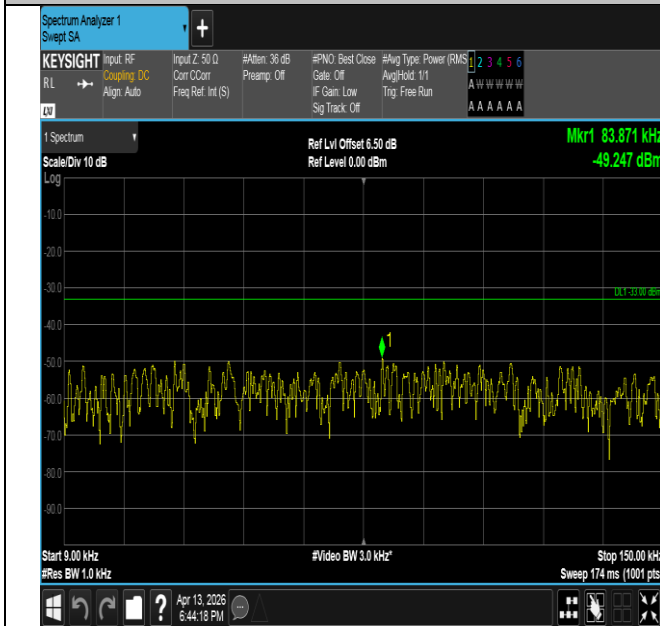
Band26(814-824)-3MHz-QPSK-26775-1RB#0-0.009~0.15-PA SS
