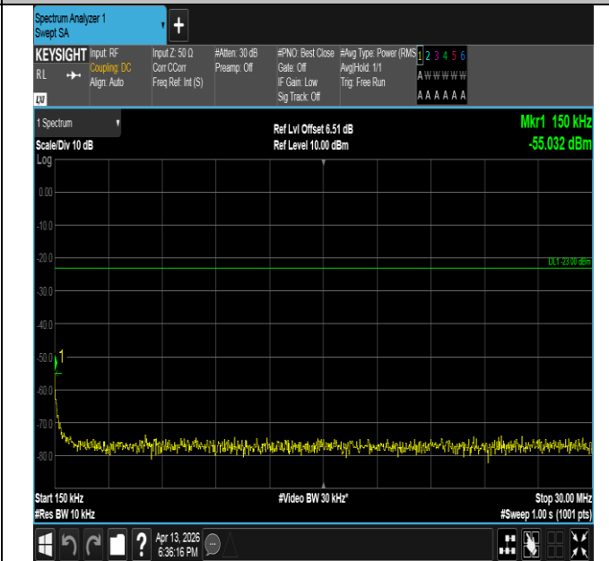
Band26(814-824)-3MHz-16QAM-26705-1RB#14-0.15~30-PAS S
