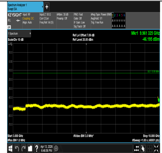
Band26(814-824)-3MHz-QPSK-26775-1RB#14-3000~10000-P
