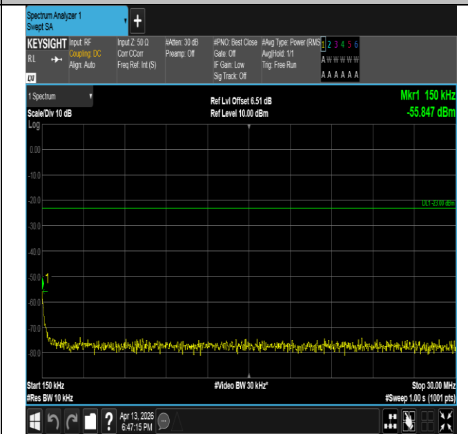
Band26(814-824)-3MHz-16QAM-26775-1RB#14-0.15~30-PAS S
