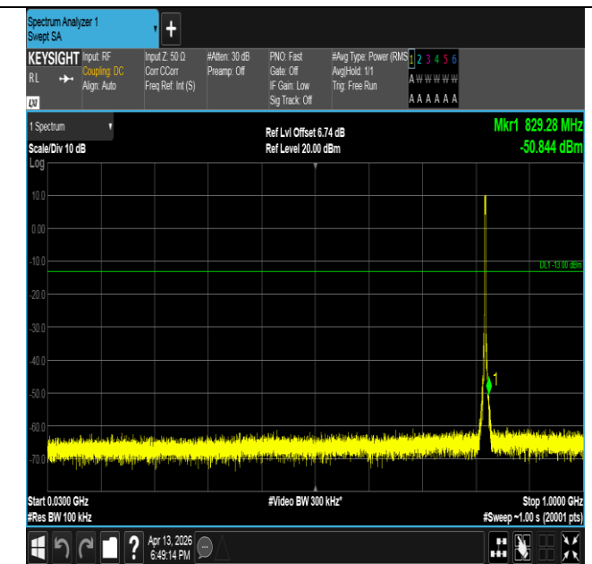
Band26(814-824)-3MHz-16QAM-26775-15RB#0-30~1000-PA
