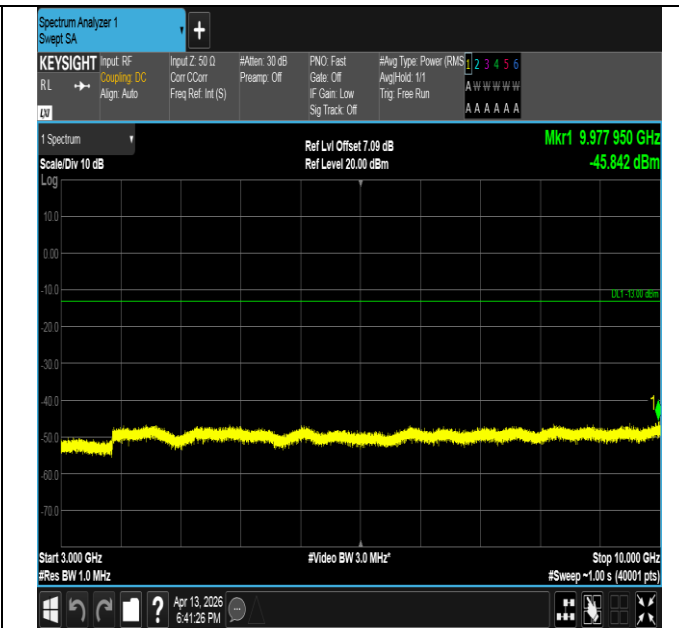
Band26(814-824)-3MHz-QPSK-26740-1RB#14-3000~10000-P ASS
