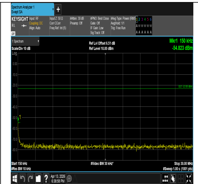
Band26(814-824)-3MHz-QPSK-26740-1RB#0-0.15~30-PASS
