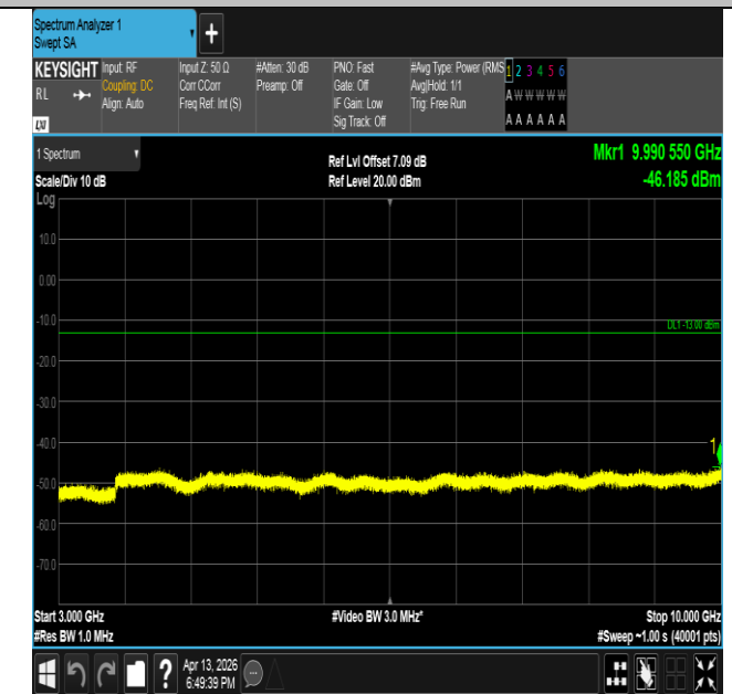
Band26(814-824)-3MHz-16QAM-26775-15RB#0-3000~10000
