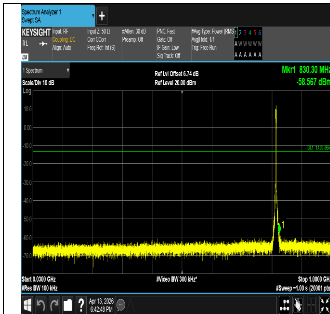
Band26(814-824)-3MHz-QPSK-26740-15RB#0-30~1000-PAS
