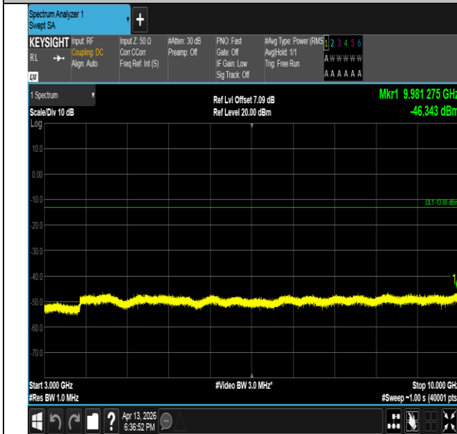
Band26(814-824)-3MHz-16QAM-26705-1RB#14-3000~10000 -PASS
