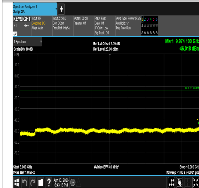
Band26(814-824)-3MHz-QPSK-26740-15RB#0-3000~10000-
