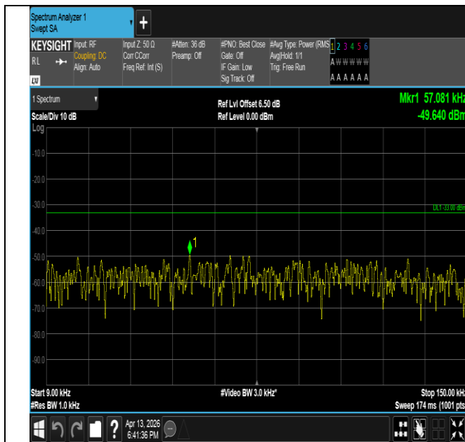
Band26(814-824)-3MHz-16QAM-26740-1RB#14-0.009~0.15- PASS
