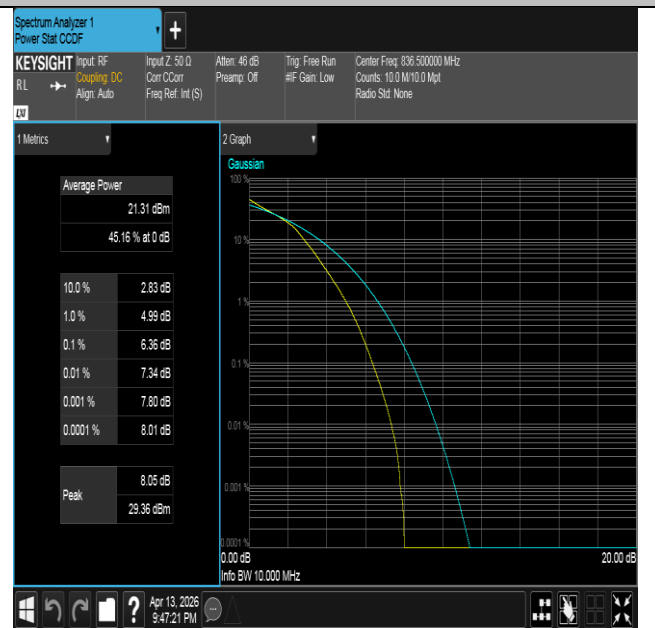
Band26(824-849)-10MHz-16QAM-26915-50RB#0-PASS
