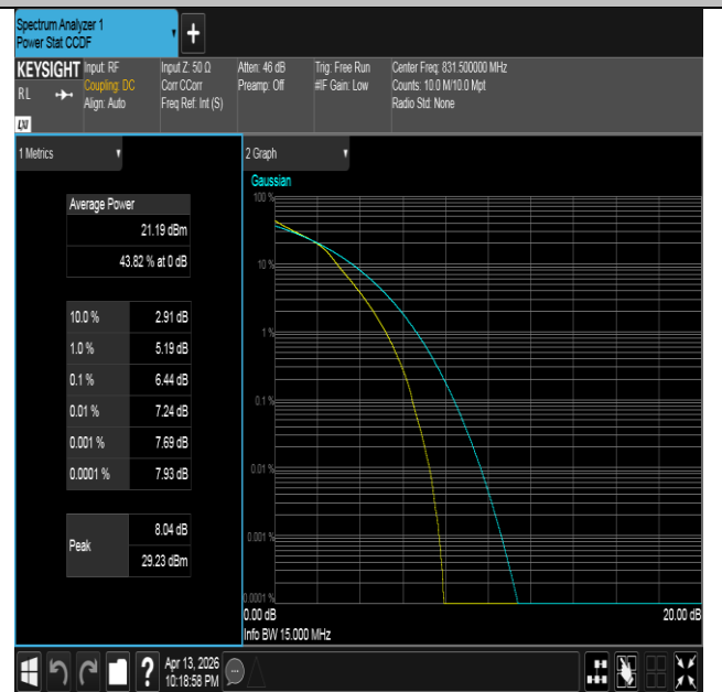
Band26(824-849)-15MHz-16QAM-26865-75RB#0-PASS
