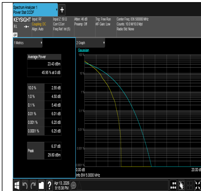
Band26(824-849)-5MHz-QPSK-26915-1RB#0-PASS
