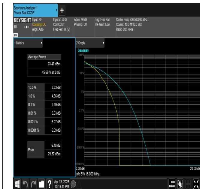
Band26(824-849)-15MHz-QPSK-26915-1RB#0-PASS
