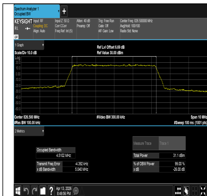
Band26(824-849)-5MHz-QPSK-26815-25RB#0-PASS
