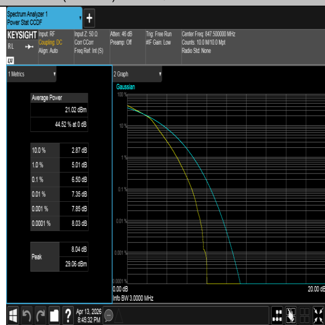
Band26(824-849)-3MHz-16QAM-27025-15RB#0-PASS
