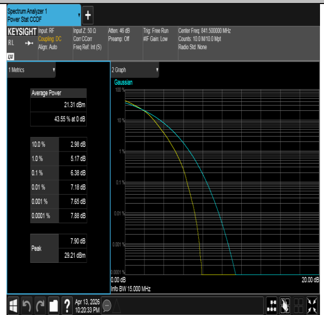
Band26(824-849)-15MHz-16QAM-26965-75RB#0-PASS
