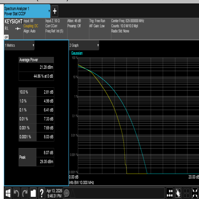
Band26(824-849)-10MHz-16QAM-26840-50RB#0-PASS
