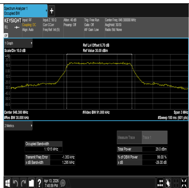
Band26(824-849)-1.4MHz-16QAM-27033-6RB#0-PASS
