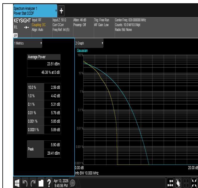
Band26(824-849)-10MHz-QPSK-26840-1RB#0-PASS
