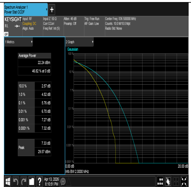
Band26(824-849)-1.4MHz-QPSK-26915-6RB#0-PASS
