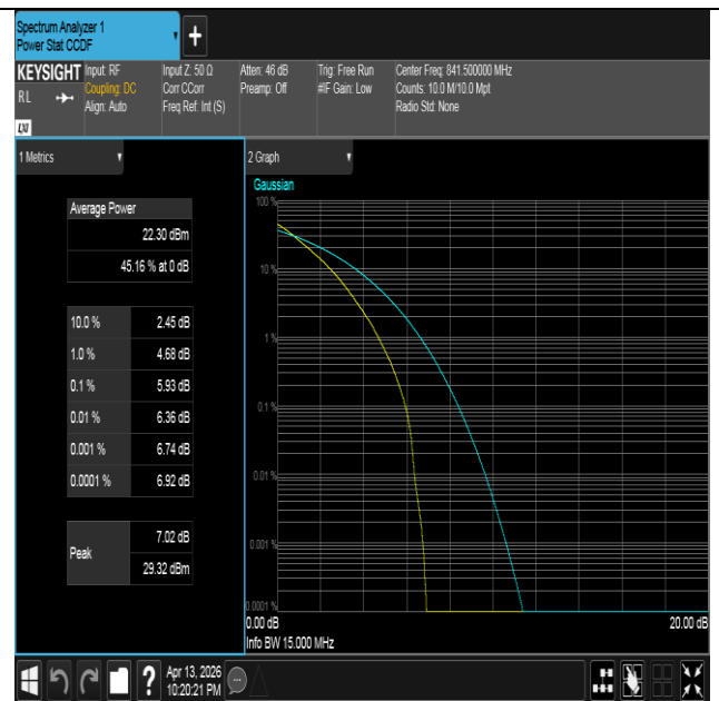
Band26(824-849)-15MHz-QPSK-26965-75RB#0-PASS
