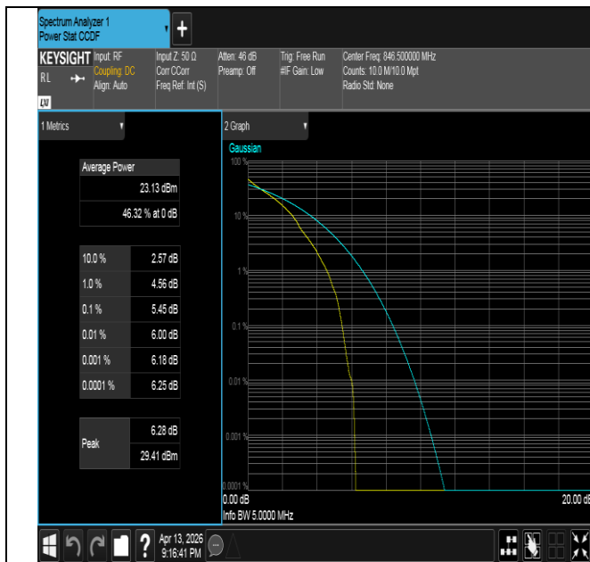
Band26(824-849)-5MHz-QPSK-27015-1RB#0-PASS
