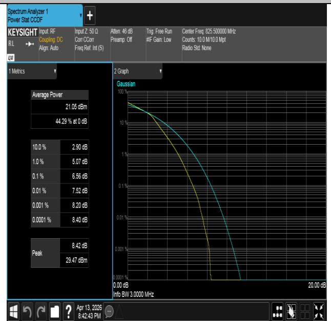
Band26(824-849)-3MHz-16QAM-26805-15RB#0-PASS
