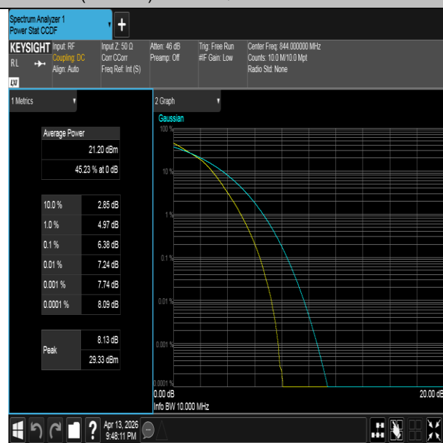
Band26(824-849)-10MHz-16QAM-26990-50RB#0-PASS
