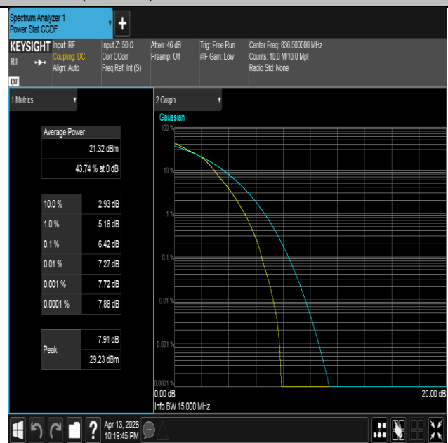
Band26(824-849)-15MHz-16QAM-26915-75RB#0-PASS
