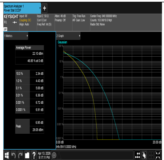
Band26(824-849)-5MHz-QPSK-27015-25RB#0-PASS
