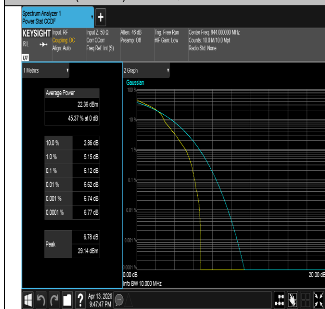
Band26(824-849)-10MHz-16QAM-26990-1RB#0-PASS
