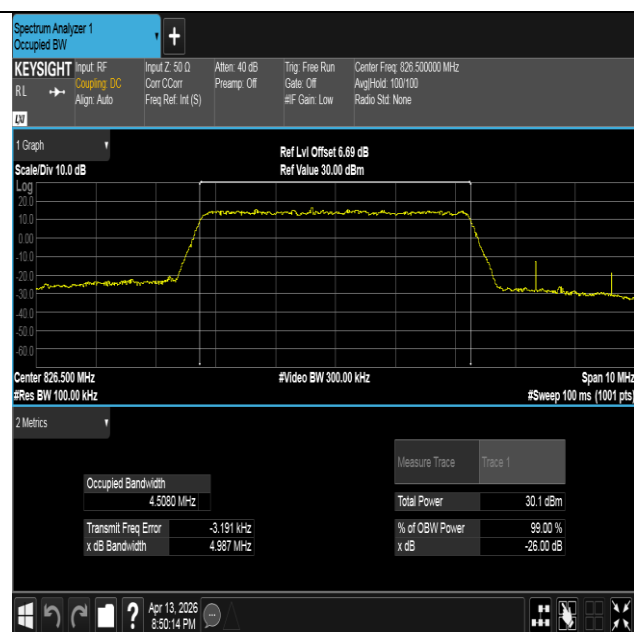
Band26(824-849)-5MHz-16QAM-26815-25RB#0-PASS
