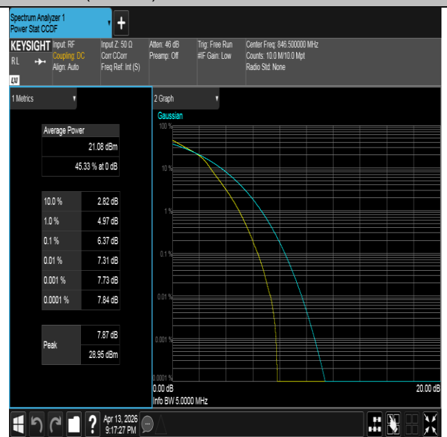
Band26(824-849)-5MHz-16QAM-27015-25RB#0-PASS
