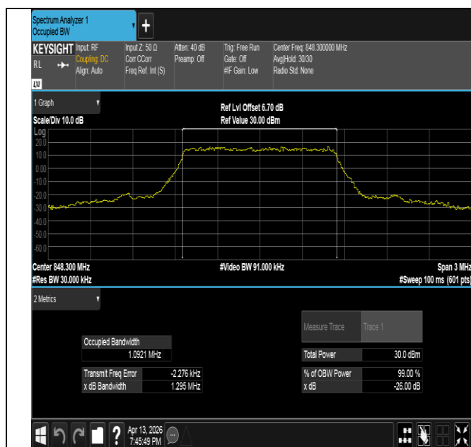
Band26(824-849)-1.4MHz-QPSK-27033-6RB#0-PASS
