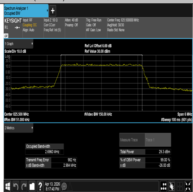
Band26(824-849)-3MHz-16QAM-26805-15RB#0-PASS
