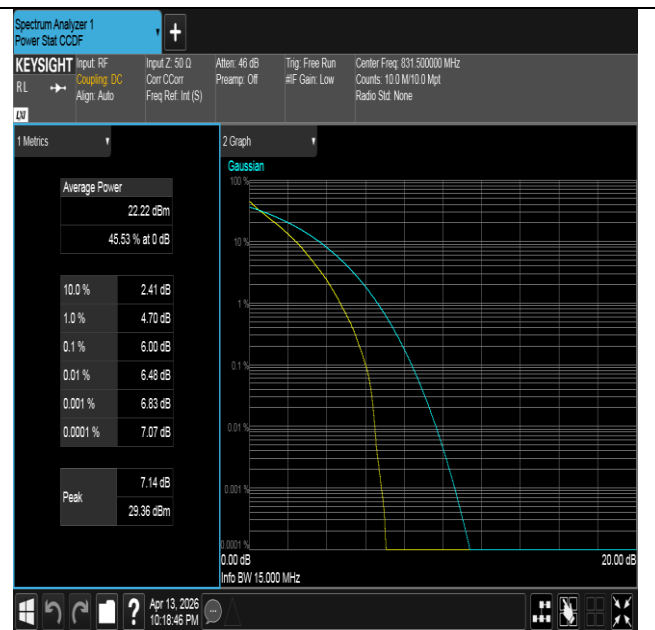
Band26(824-849)-15MHz-QPSK-26865-75RB#0-PASS
