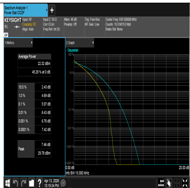
Band26(824-849)-15MHz-QPSK-26915-75RB#0-PASS
