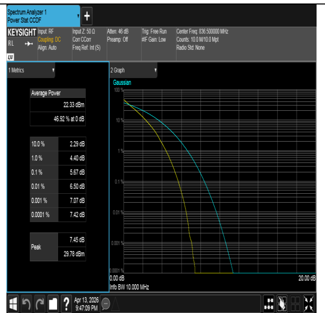
Band26(824-849)-10MHz-QPSK-26915-50RB#0-PASS
