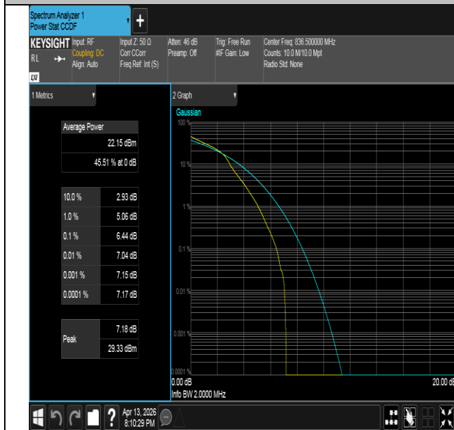
Band26(824-849)-1.4MHz-16QAM-26915-1RB#0-PASS
