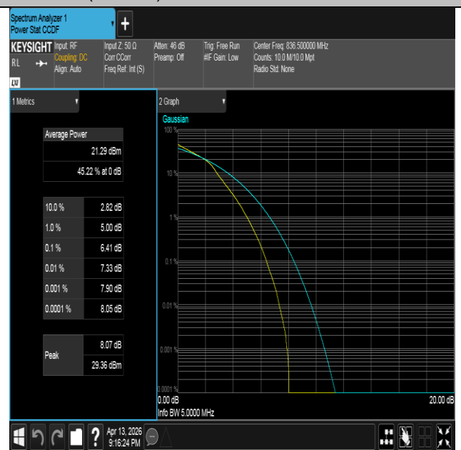
Band26(824-849)-5MHz-16QAM-26915-25RB#0-PASS
