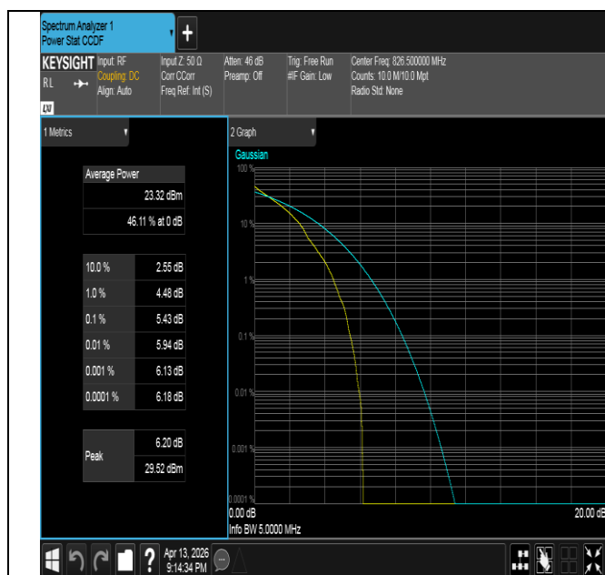
Band26(824-849)-5MHz-QPSK-26815-1RB#0-PASS
