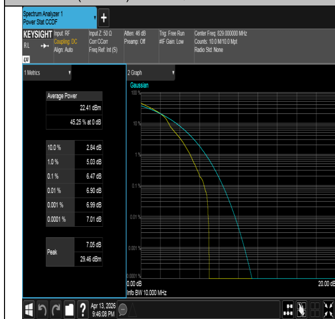
Band26(824-849)-10MHz-16QAM-26840-1RB#0-PASS
