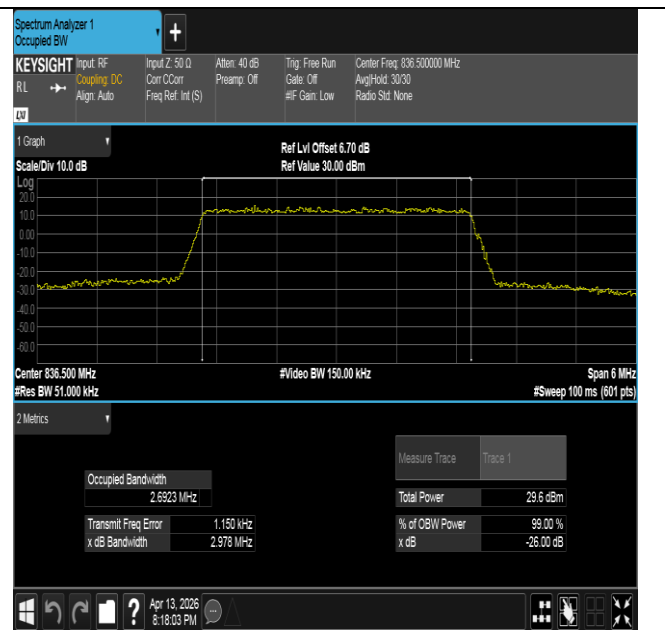
Band26(824-849)-3MHz-16QAM-26915-15RB#0-PASS
