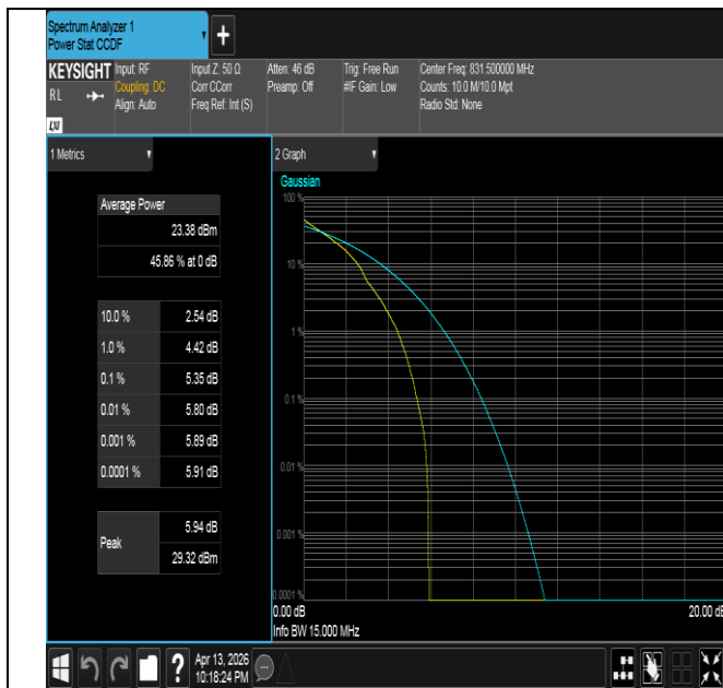
Band26(824-849)-15MHz-QPSK-26865-1RB#0-PASS
