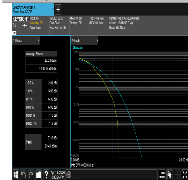
Band26(824-849)-3MHz-16QAM-26915-1RB#0-PASS
