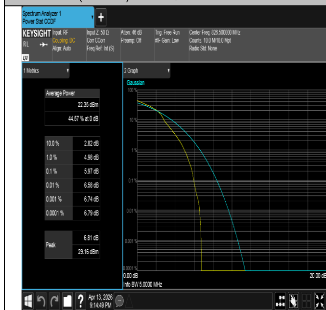
Band26(824-849)-5MHz-16QAM-26815-1RB#0-PASS
