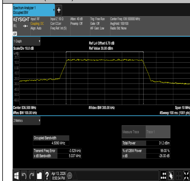
Band26(824-849)-5MHz-QPSK-26915-25RB#0-PASS
