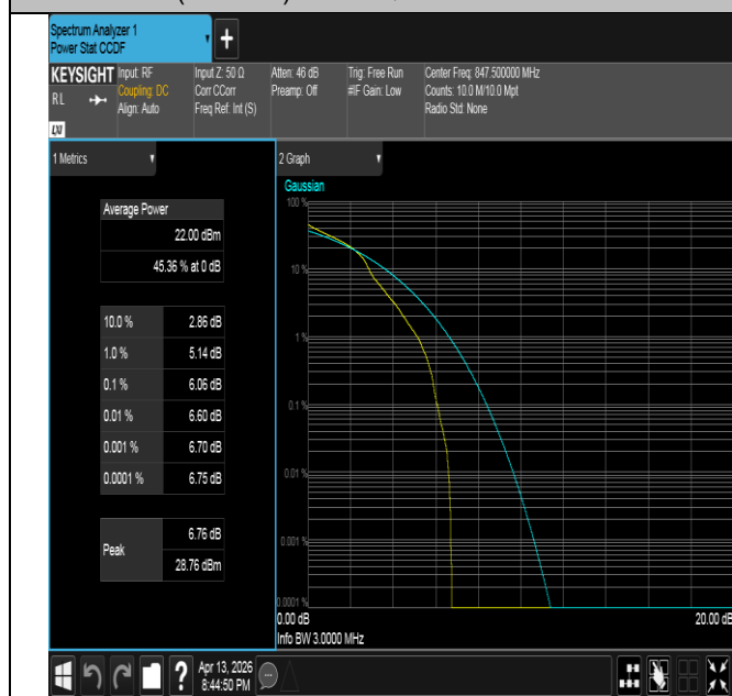
Band26(824-849)-3MHz-16QAM-27025-1RB#0-PASS
