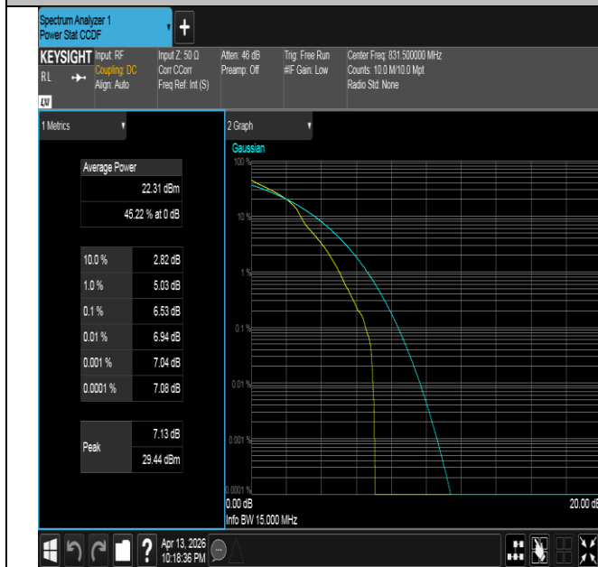
Band26(824-849)-15MHz-16QAM-26865-1RB#0-PASS
