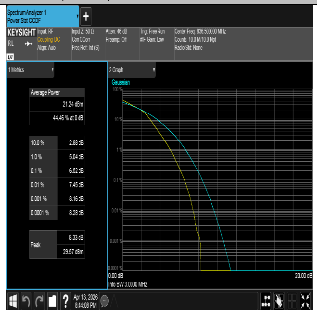
Band26(824-849)-3MHz-16QAM-26915-15RB#0-PASS
