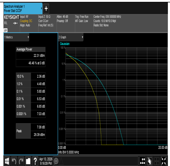
Band26(824-849)-5MHz-QPSK-26915-25RB#0-PASS
