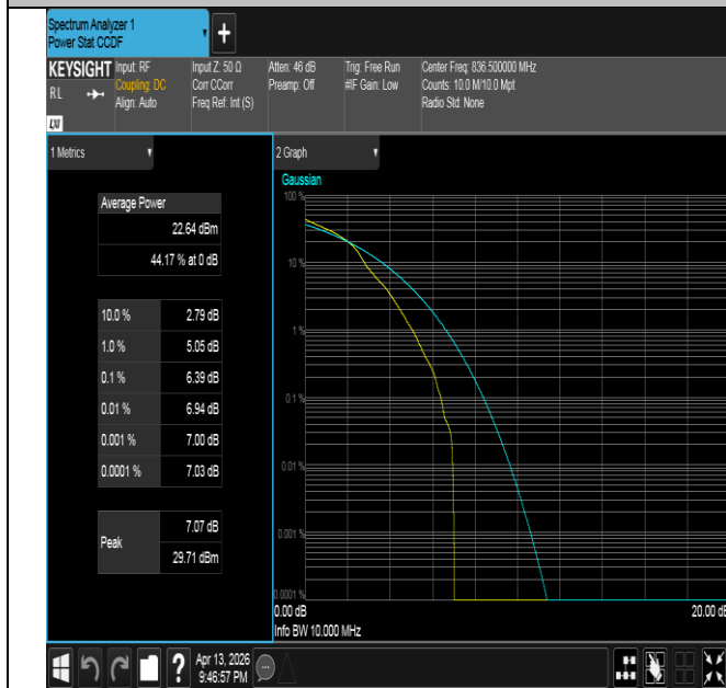
Band26(824-849)-10MHz-16QAM-26915-1RB#0-PASS
