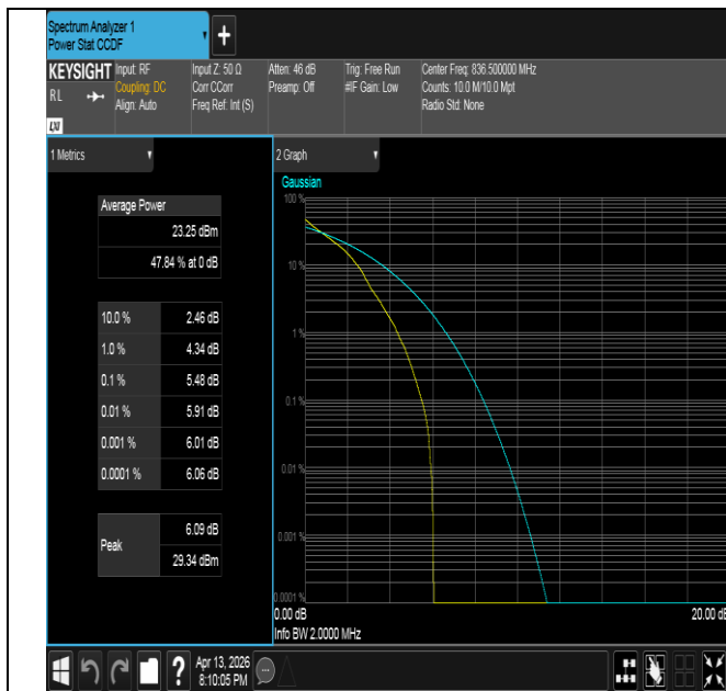
Band26(824-849)-1.4MHz-QPSK-26915-1RB#0-PASS
