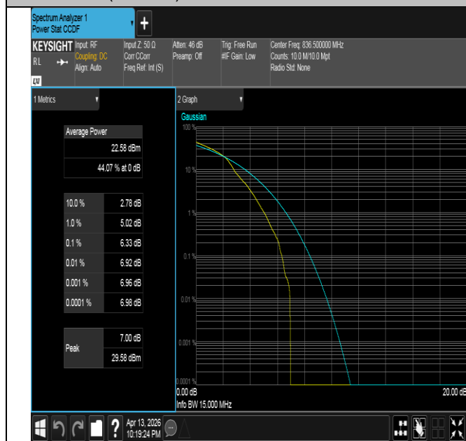
Band26(824-849)-15MHz-16QAM-26915-1RB#0-PASS
