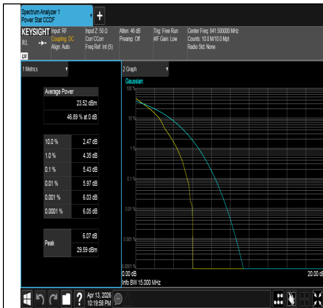
Band26(824-849)-15MHz-QPSK-26965-1RB#0-PASS
