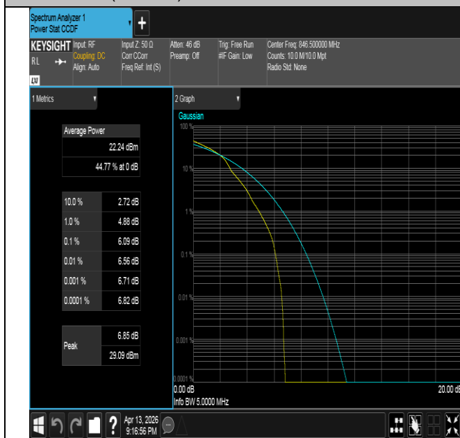
Band26(824-849)-5MHz-16QAM-27015-1RB#0-PASS
