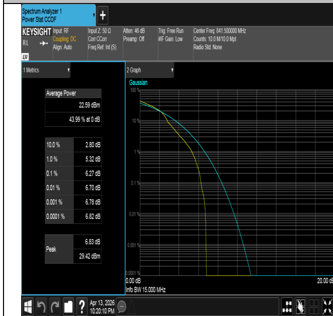
Band26(824-849)-15MHz-16QAM-26965-1RB#0-PASS
