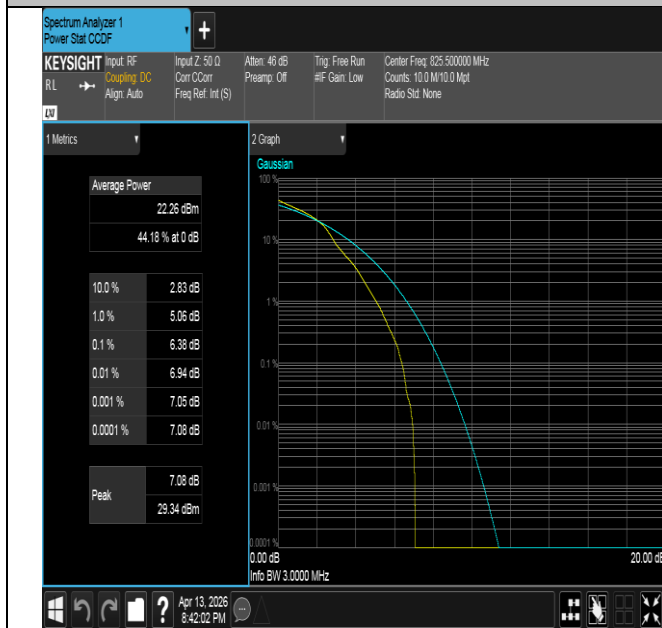
Band26(824-849)-3MHz-16QAM-26805-1RB#0-PASS
