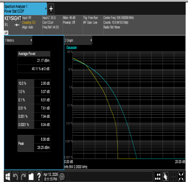
Band26(824-849)-1.4MHz-16QAM-26915-6RB#0-PASS
