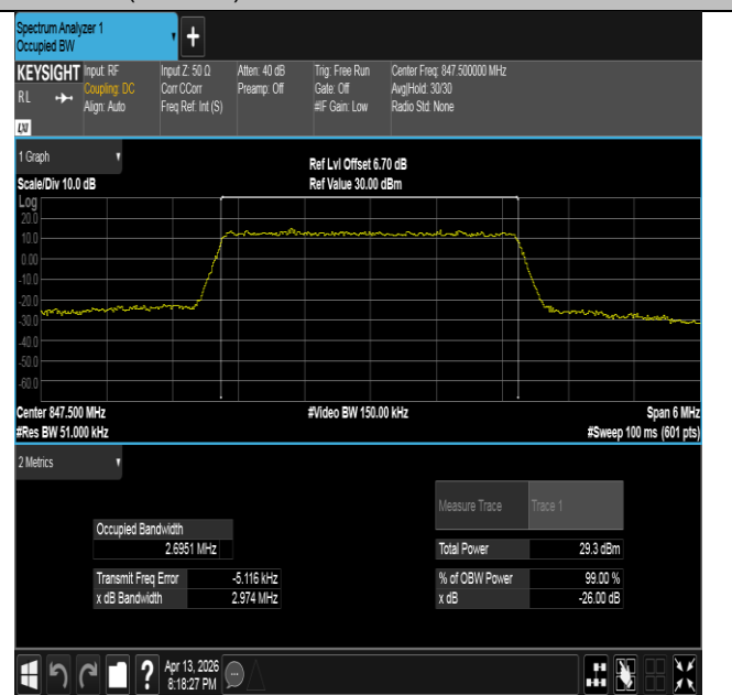
Band26(824-849)-3MHz-16QAM-27025-15RB#0-PASS
