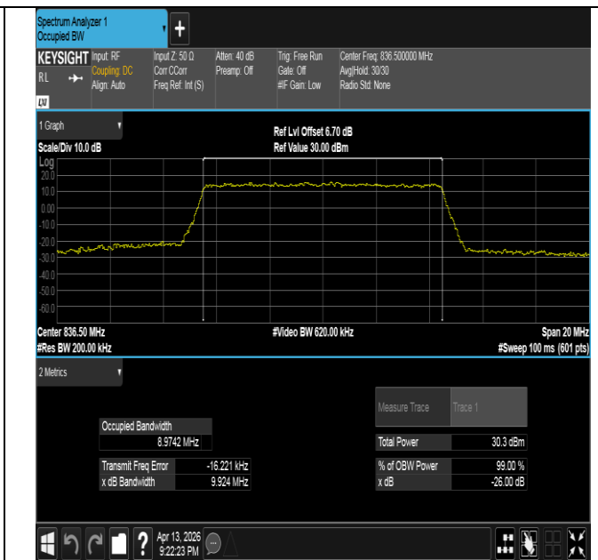
Band26(824-849)-10MHz-16QAM-26915-50RB#0-PASS
