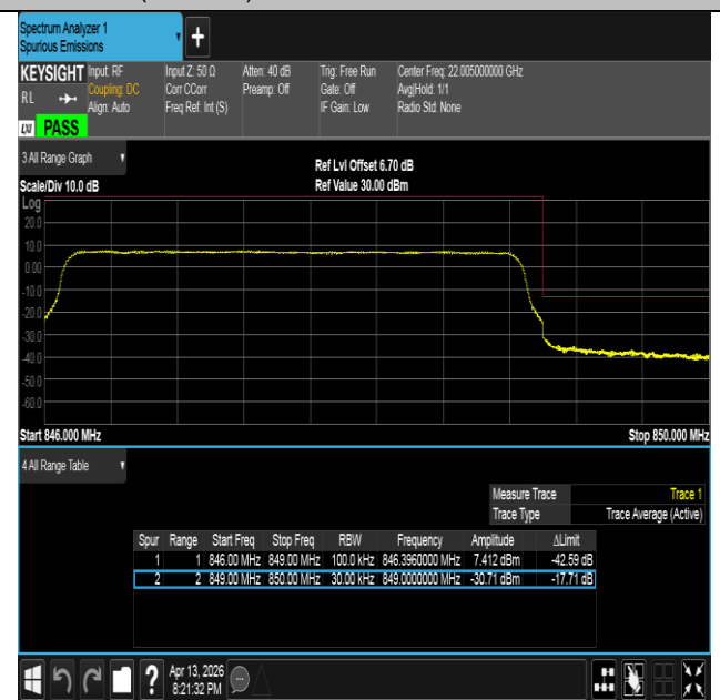
Band26(824-849)-3MHz-16QAM-27025-15RB#0-PASS
