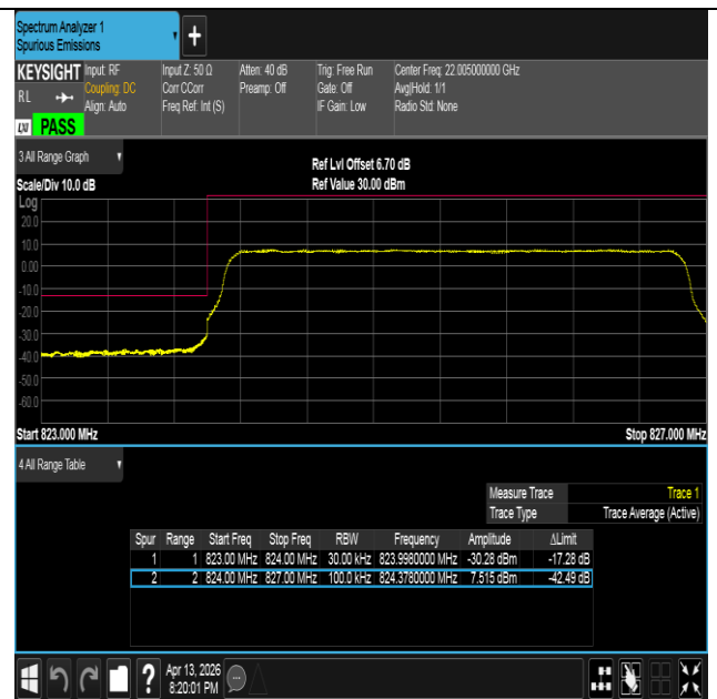
Band26(824-849)-3MHz-16QAM-26805-15RB#0-PASS
