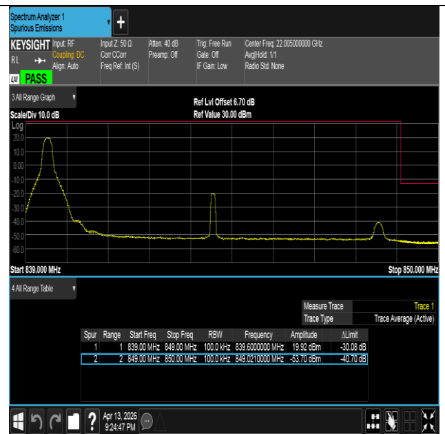
Band26(824-849)-10MHz-16QAM-26990-1RB#0-PASS
