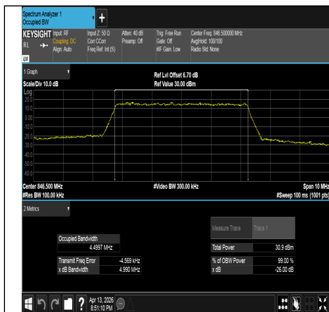
Band26(824-849)-5MHz-QPSK-27015-25RB#0-PASS
