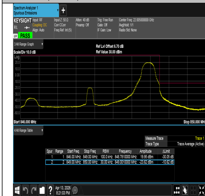
Band26(824-849)-3MHz-16QAM-27025-1RB#14-PASS
