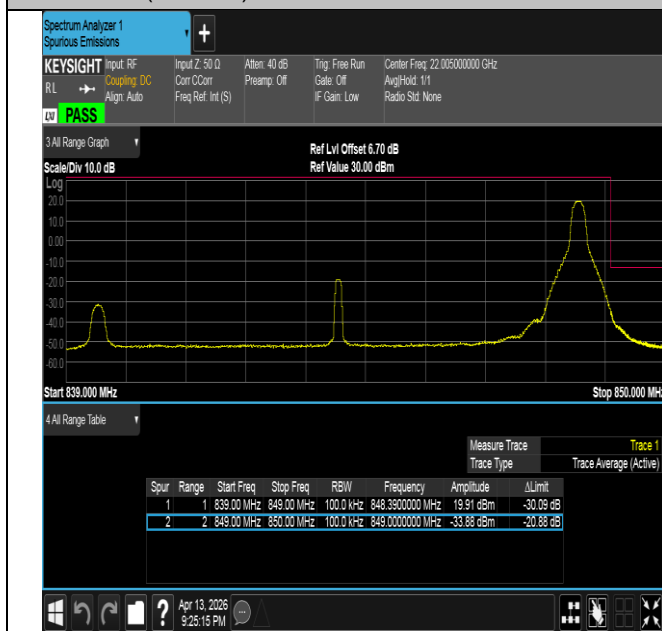
Band26(824-849)-10MHz-16QAM-26990-1RB#49-PASS
