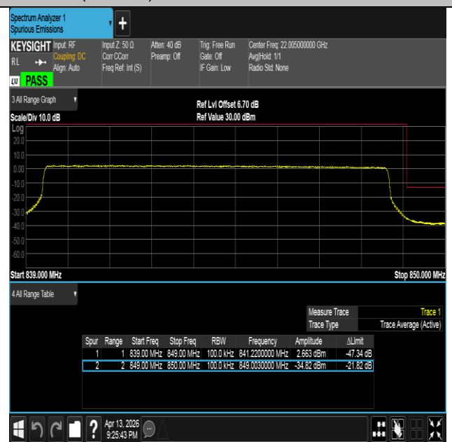
Band26(824-849)-10MHz-16QAM-26990-50RB#0-PASS
