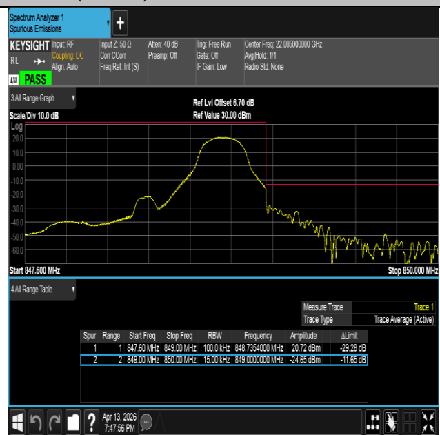
Band26(824-849)-1.4MHz-QPSK-27033-1RB#5-PASS
