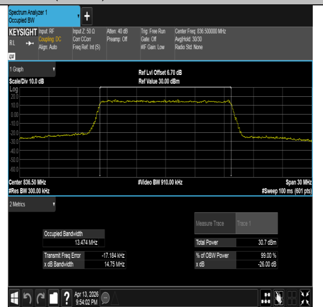
Band26(824-849)-15MHz-16QAM-26915-75RB#0-PASS
