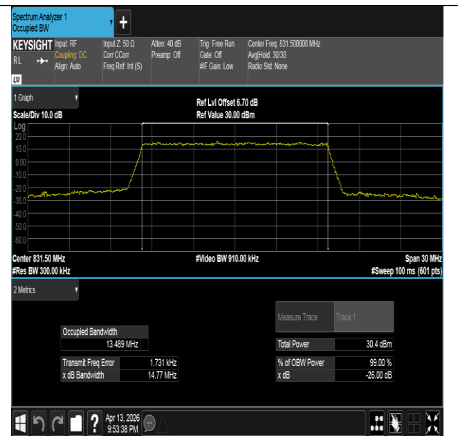
Band26(824-849)-15MHz-16QAM-26865-75RB#0-PASS
