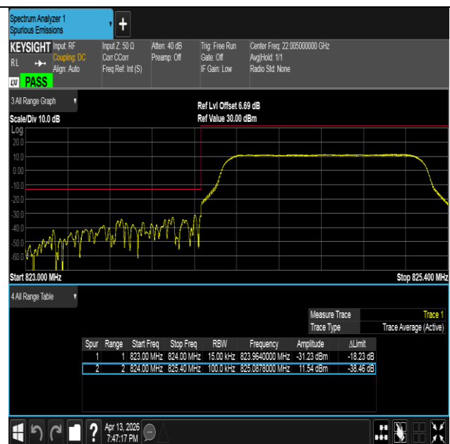
Band26(824-849)-1.4MHz-16QAM-26797-6RB#0-PASS
