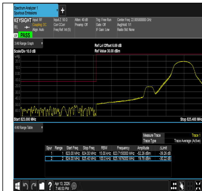
Band26(824-849)-1.4MHz-16QAM-26797-1RB#5-PASS
