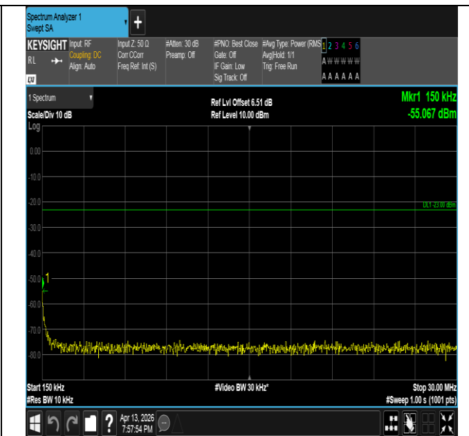
Band26(824-849)-1.4MHz-QPSK-26915-6RB#0-0.15~30-PAS S
