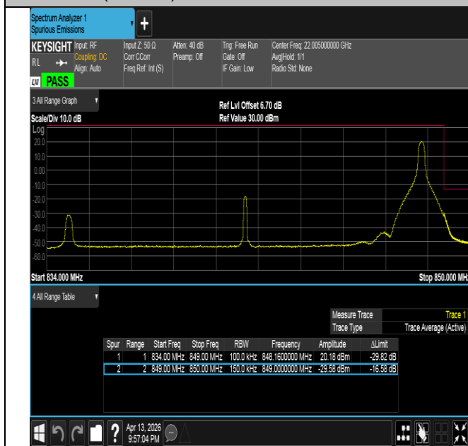
Band26(824-849)-15MHz-16QAM-26965-1RB#74-PASS
