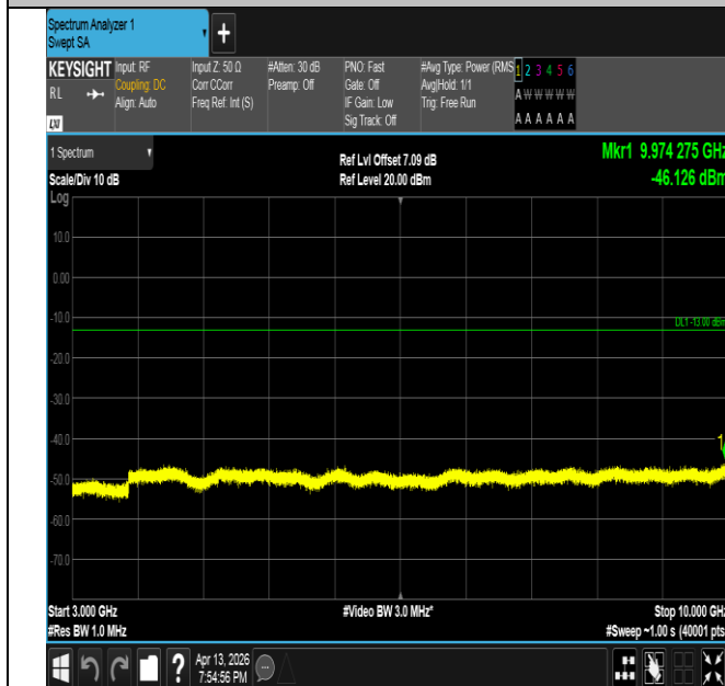
Band26(824-849)-1.4MHz-QPSK-26915-1RB#0-3000~10000-
