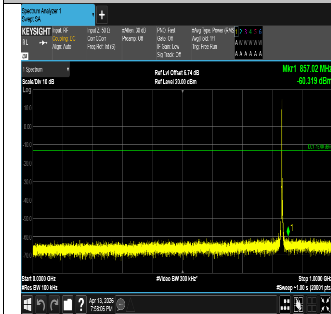
Band26(824-849)-1.4MHz-QPSK-26915-6RB#0-30~1000-PAS S
