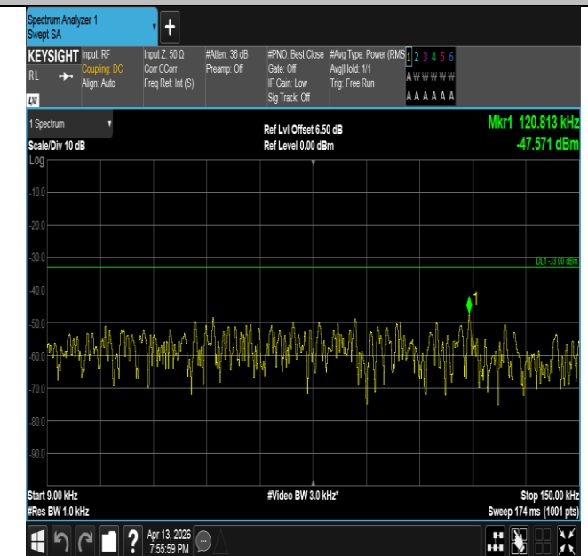
Band26(824-849)-1.4MHz-QPSK-26915-1RB#5-0.009~0.15-P
