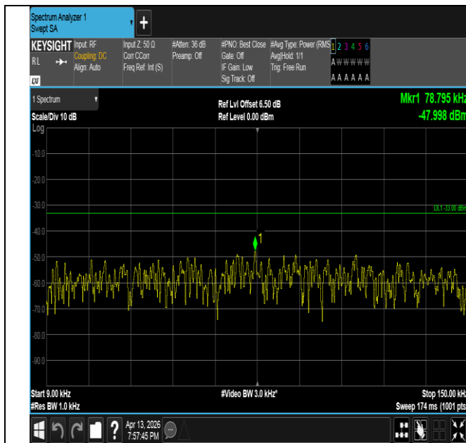
Band26(824-849)-1.4MHz-QPSK-26915-6RB#0-0.009~0.15-P ASS
