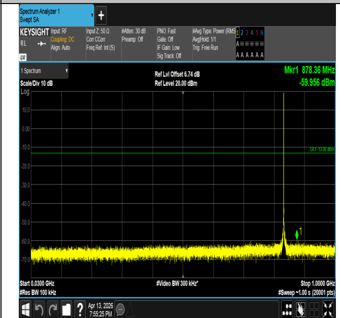
Band26(824-849)-1.4MHz-16QAM-26915-1RB#0-30~1000-PA SS
