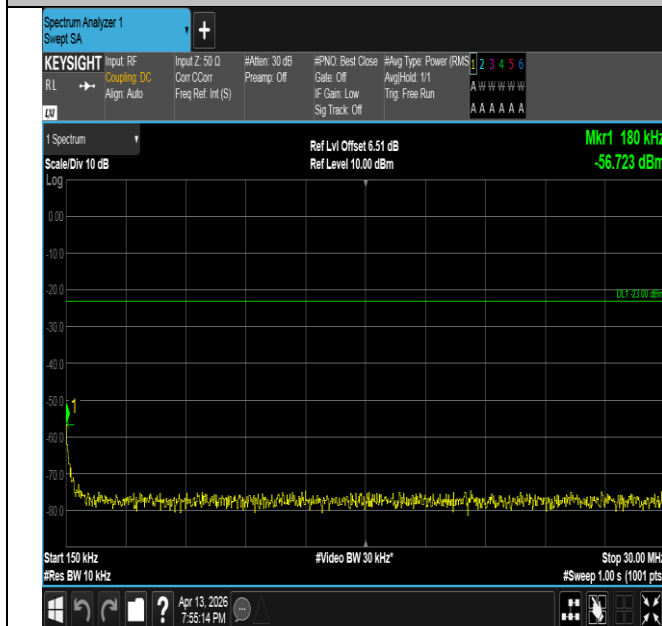
Band26(824-849)-1.4MHz-16QAM-26915-1RB#0-0.15~30-PA SS
