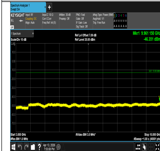
Band26(824-849)-1.4MHz-QPSK-26797-6RB#0-3000~10000-
