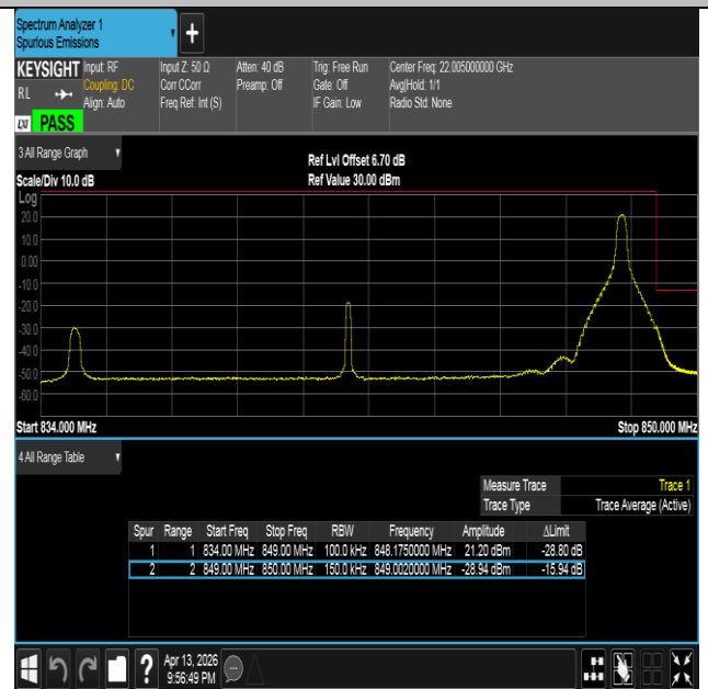
Band26(824-849)-15MHz-QPSK-26965-1RB#74-PASS
