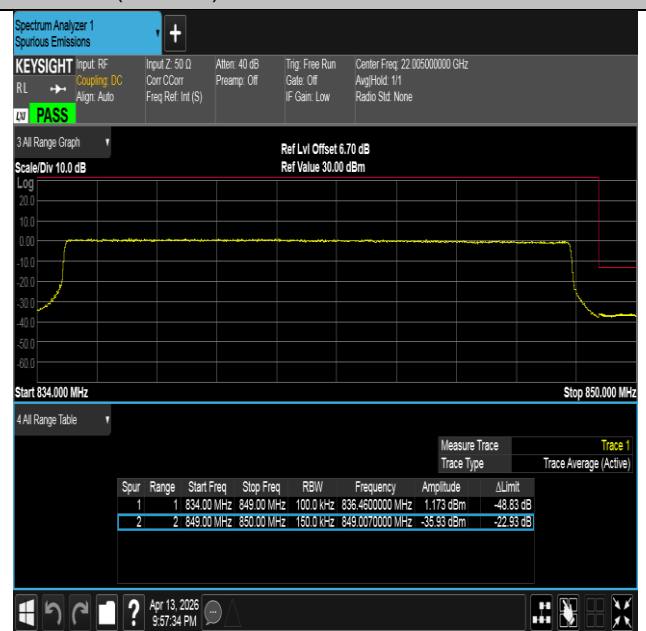
Band26(824-849)-15MHz-16QAM-26965-75RB#0-PASS
