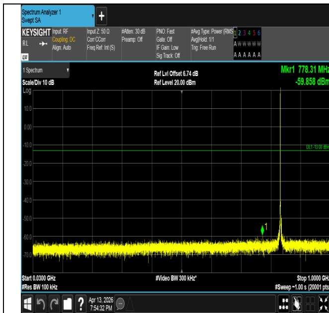
Band26(824-849)-1.4MHz-QPSK-26915-1RB#0-30~1000-PAS
