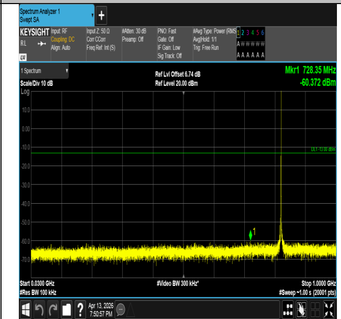
Band26(824-849)-1.4MHz-QPSK-26797-1RB#5-30~1000-PAS S
