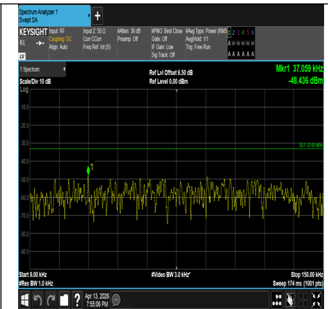
Band26(824-849)-1.4MHz-16QAM-26915-1RB#0-0.009~0.15- PASS
