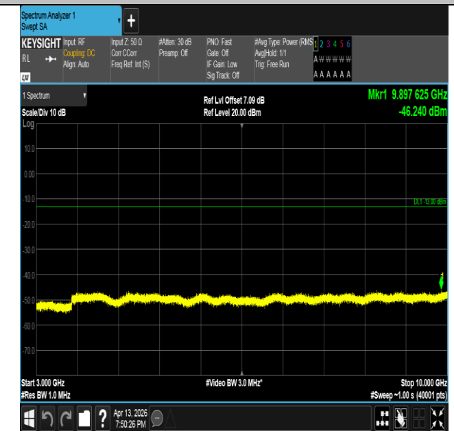
Band26(824-849)-1.4MHz-16QAM-26797-1RB#0-3000~10000
