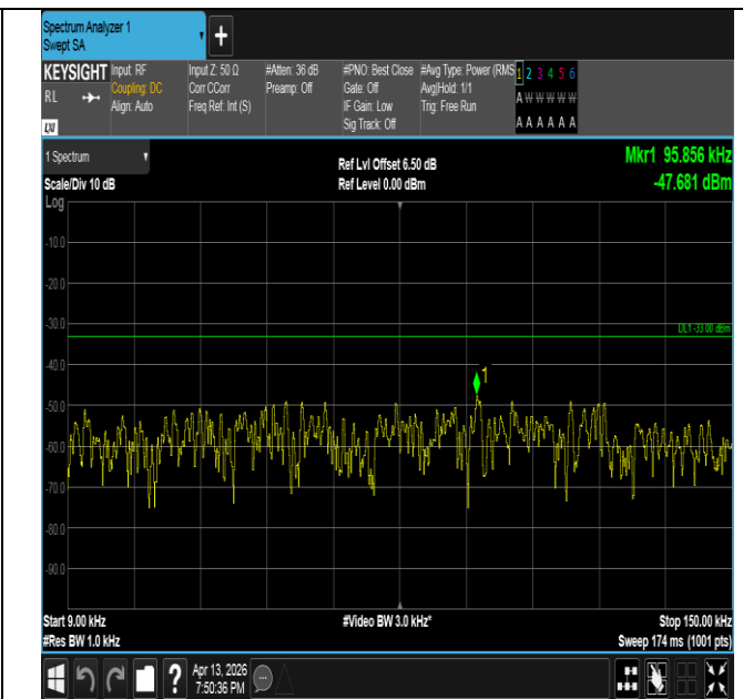
Band26(824-849)-1.4MHz-QPSK-26797-1RB#5-0.009~0.15-P ASS
