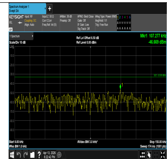
Band26(824-849)-3MHz-16QAM-26805-1RB#0-0.009~0.15-P ASS
