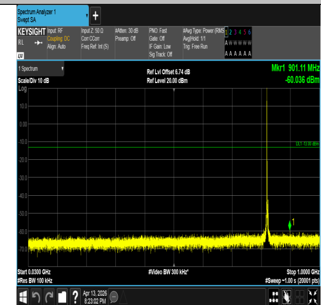
Band26(824-849)-3MHz-16QAM-26805-1RB#0-30~1000-PAS S
