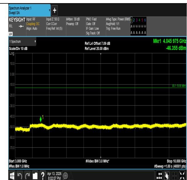
Band26(824-849)-1.4MHz-QPSK-27033-1RB#5-3000~10000- PASS
