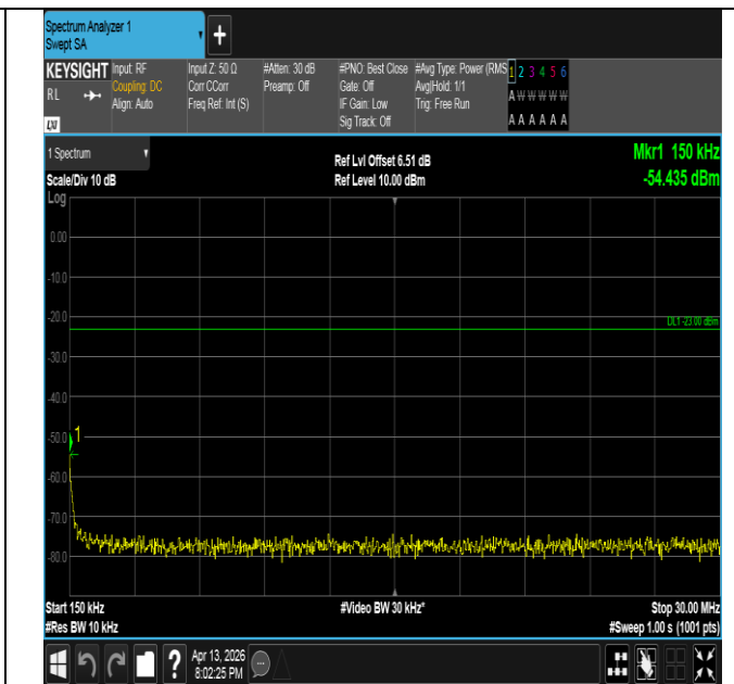
Band26(824-849)-1.4MHz-16QAM-27033-1RB#5-0.15~30-PA SS
