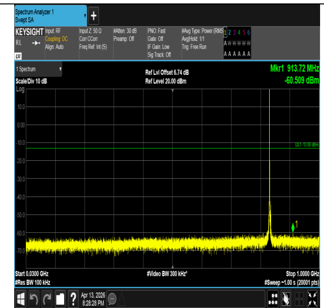
Band26(824-849)-3MHz-16QAM-26915-1RB#0-30~1000-PAS
