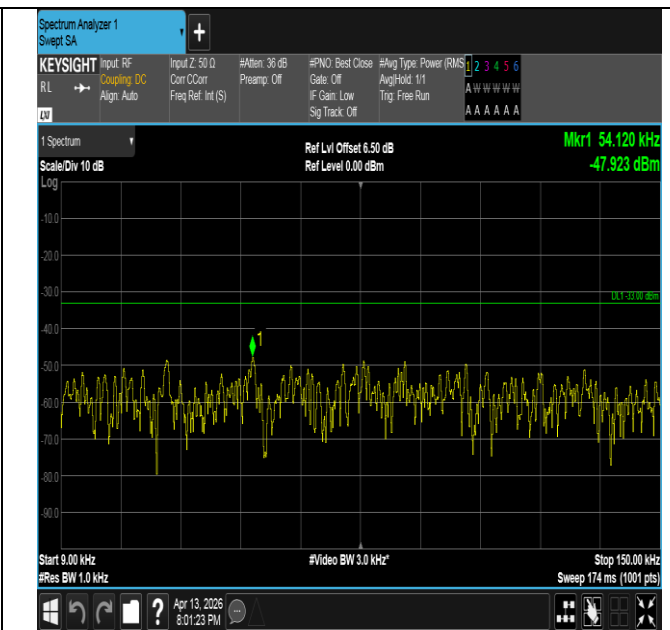
Band26(824-849)-1.4MHz-QPSK-27033-1RB#5-0.009~0.15-P ASS
