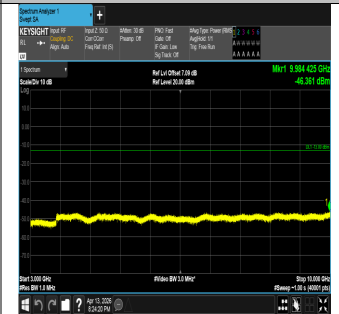
Band26(824-849)-3MHz-QPSK-26805-1RB#14-3000~10000-P
