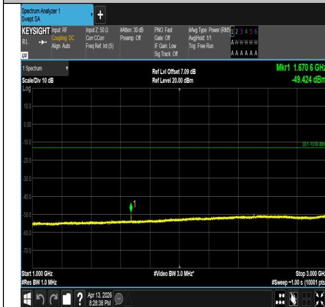
Band26(824-849)-3MHz-16QAM-26915-1RB#0-1000~3000-P
