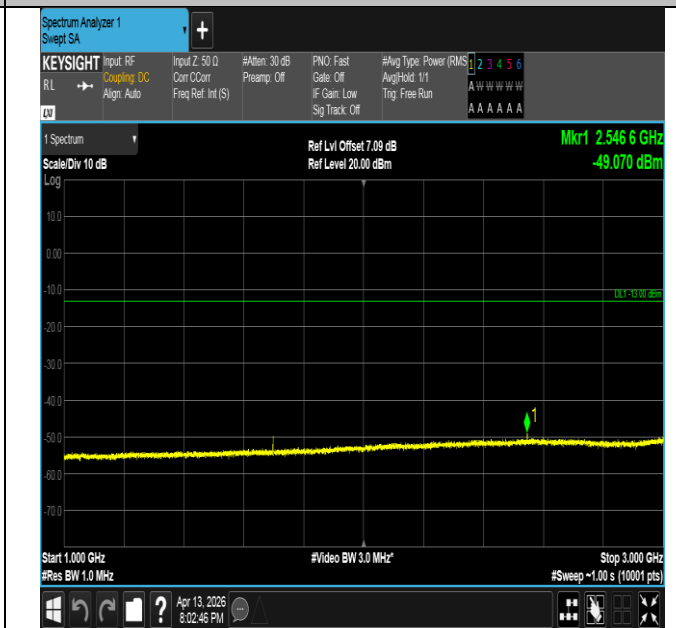
Band26(824-849)-1.4MHz-16QAM-27033-1RB#5-1000~3000- PASS
