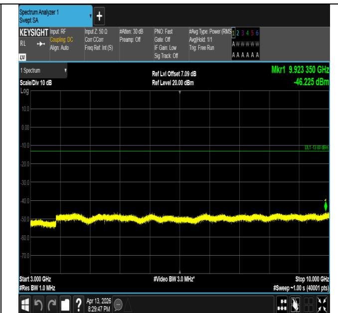
Band26(824-849)-3MHz-QPSK-26915-1RB#14-3000~10000-P
