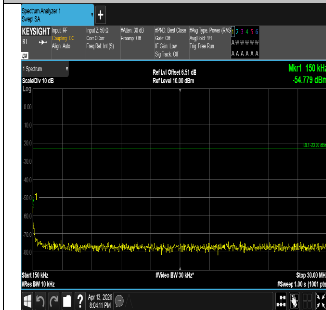
Band26(824-849)-1.4MHz-16QAM-27033-6RB#0-0.15~30-PA SS
