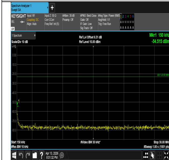
Band26(824-849)-1.4MHz-QPSK-27033-1RB#5-0.15~30-PAS S
