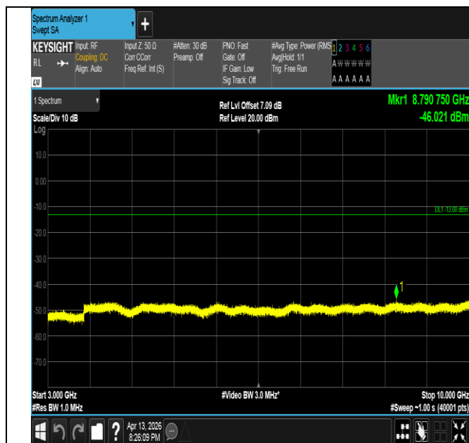
Band26(824-849)-3MHz-QPSK-26805-15RB#0-3000~10000- PASS
