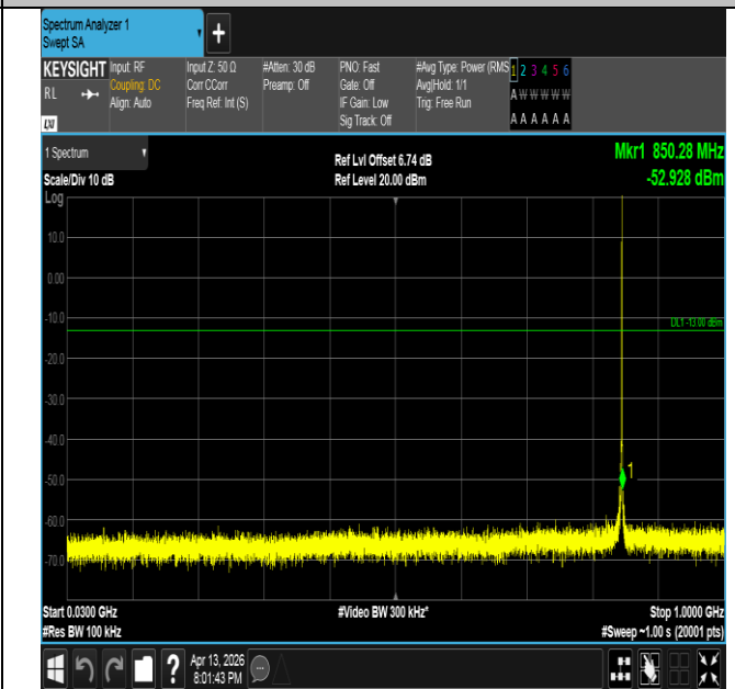
Band26(824-849)-1.4MHz-QPSK-27033-1RB#5-30~1000-PAS S
