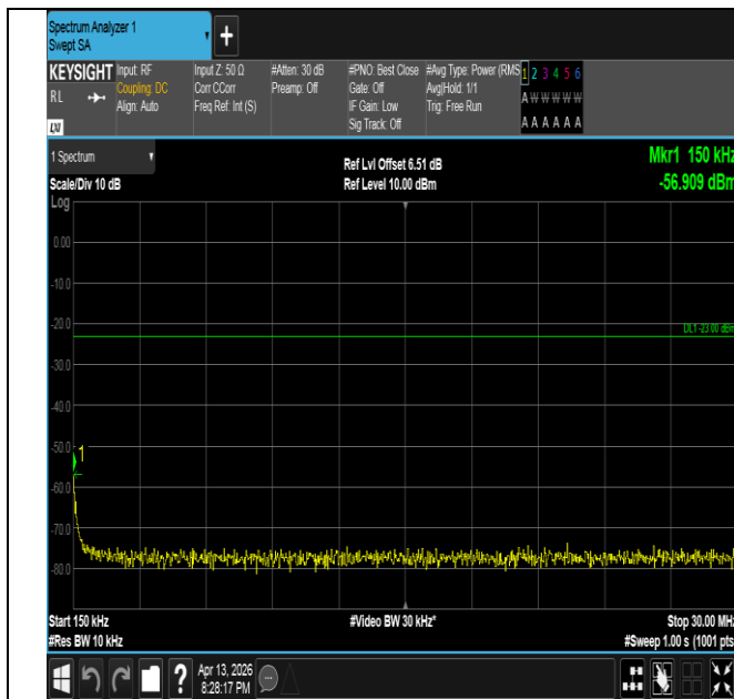
Band26(824-849)-3MHz-16QAM-26915-1RB#0-0.15~30-PAS
