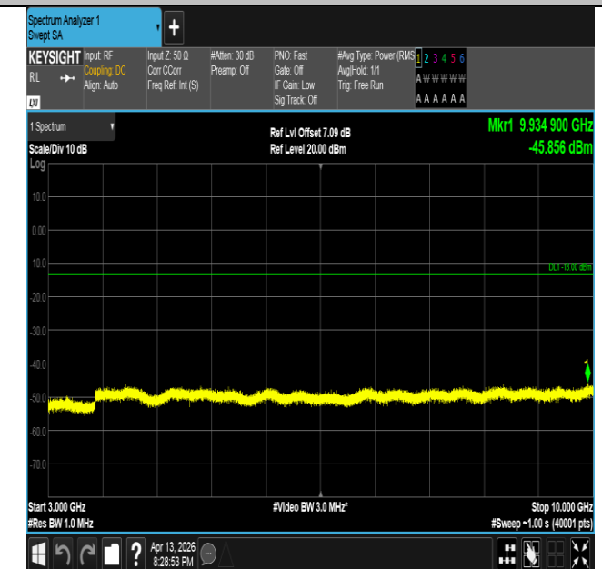
Band26(824-849)-3MHz-16QAM-26915-1RB#0-3000~10000-PASS
