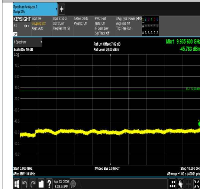
Band26(824-849)-1.4MHz-QPSK-27033-6RB#0-3000~10000-
