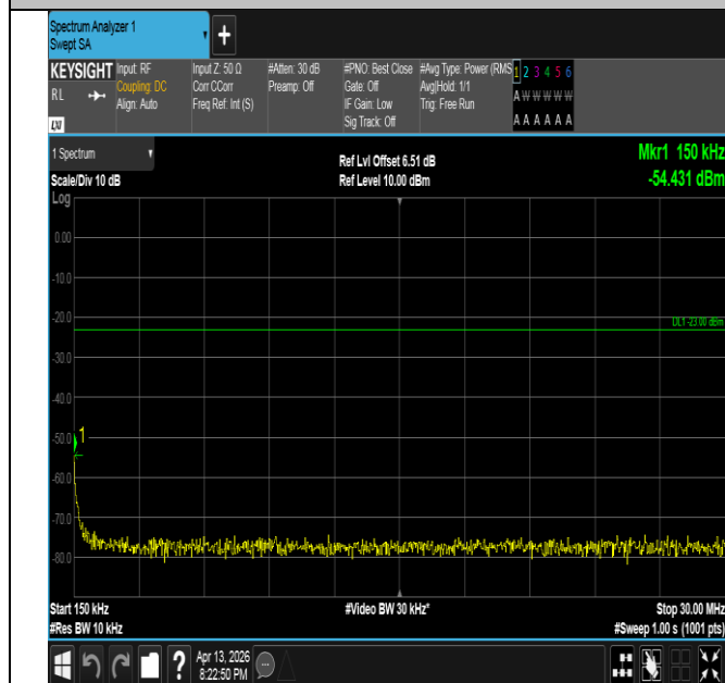
Band26(824-849)-3MHz-16QAM-26805-1RB#0-0.15~30-PAS S
