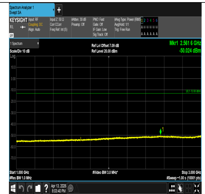
Band26(824-849)-1.4MHz-QPSK-27033-6RB#0-1000~3000-P
