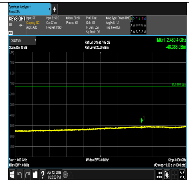
Band26(824-849)-3MHz-16QAM-26805-1RB#14-1000~3000- PASS
