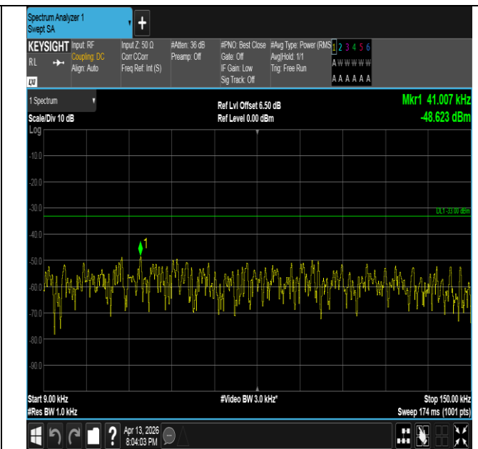
Band26(824-849)-1.4MHz-16QAM-27033-6RB#0-0.009~0.15- PASS
