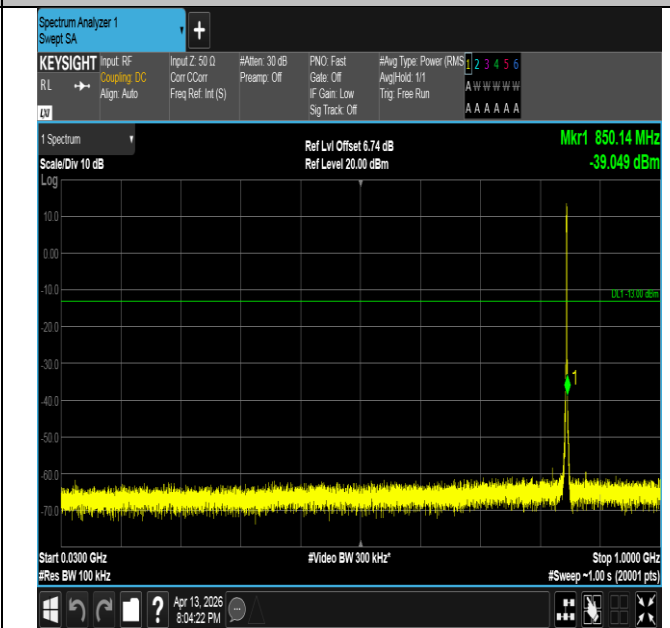
Band26(824-849)-1.4MHz-16QAM-27033-6RB#0-30~1000-PA SS
