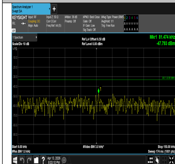
Band26(824-849)-1.4MHz-QPSK-27033-6RB#0-0.009~0.15-P ASS
