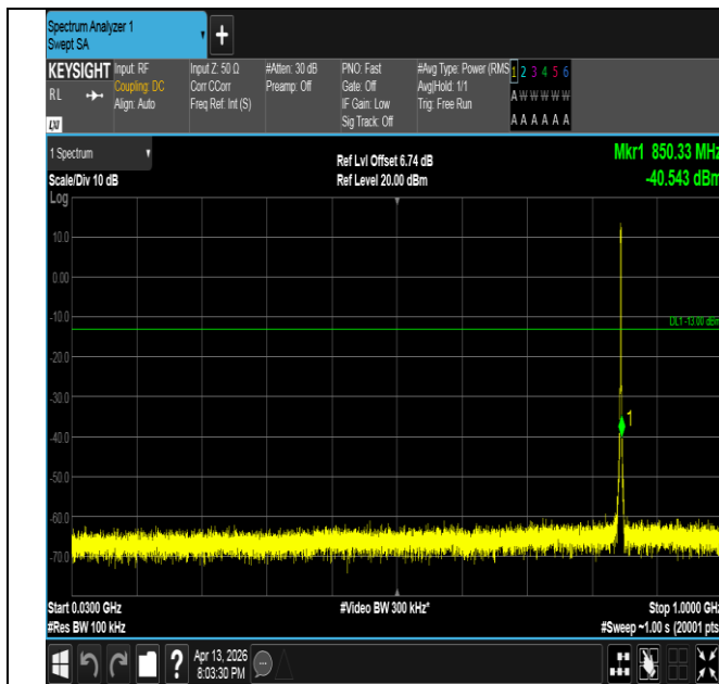
Band26(824-849)-1.4MHz-QPSK-27033-6RB#0-30~1000-PAS
