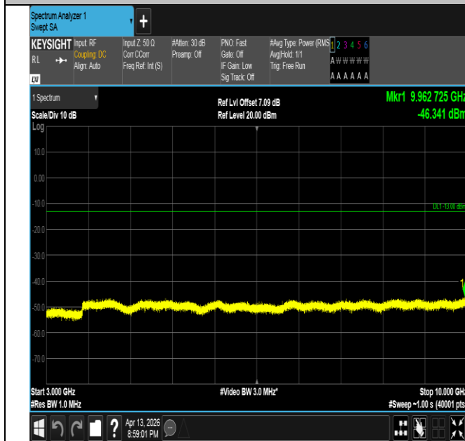
Band26(824-849)-5MHz-QPSK-26815-25RB#0-3000~10000-
