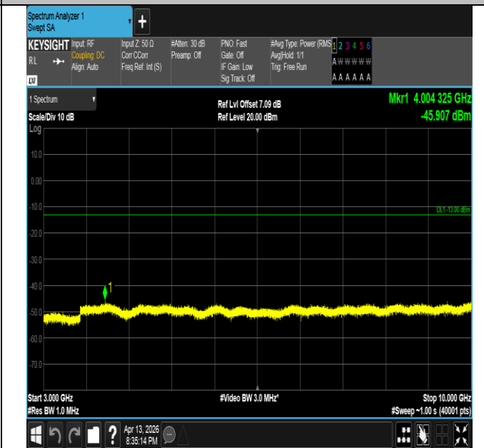
Band26(824-849)-3MHz-QPSK-27025-1RB#14-3000~10000-P
