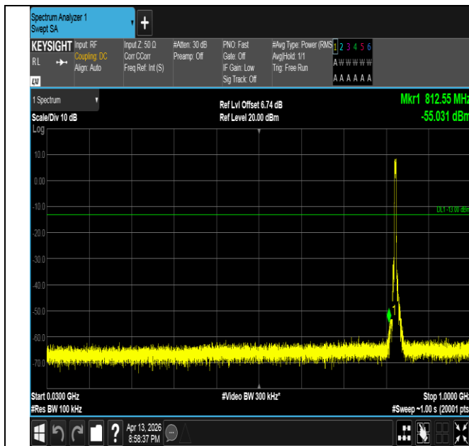
Band26(824-849)-5MHz-QPSK-26815-25RB#0-30~1000-PAS
