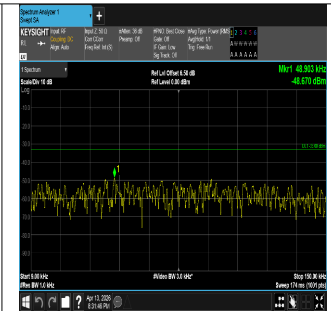
Band26(824-849)-3MHz-16QAM-26915-15RB#0-0.009~0.15- PASS
