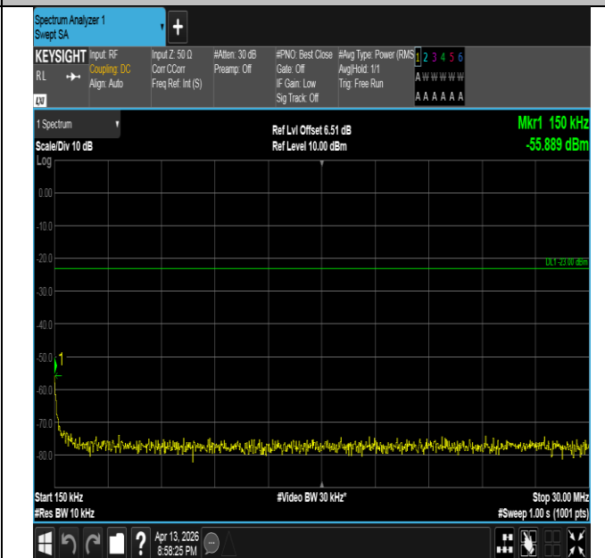
Band26(824-849)-5MHz-QPSK-26815-25RB#0-0.15~30-PAS
