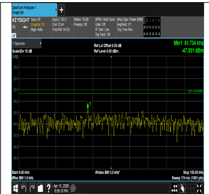
Band26(824-849)-5MHz-16QAM-26815-25RB#0-0.009~0.15- PASS
