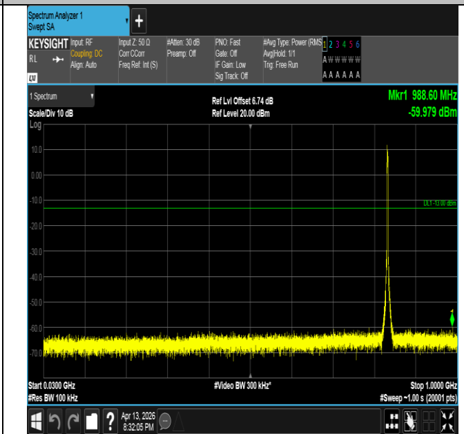
Band26(824-849)-3MHz-16QAM-26915-15RB#0-30~1000-PA SS
