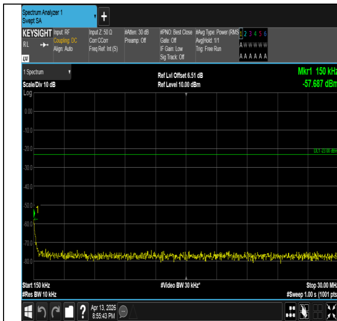
Band26(824-849)-5MHz-16QAM-26815-1RB#0-0.15~30-PAS
