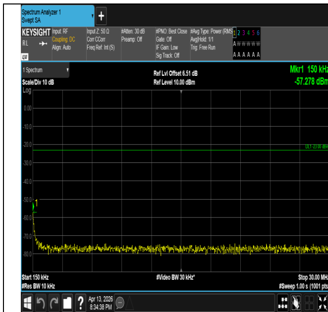
Band26(824-849)-3MHz-QPSK-27025-1RB#14-0.15~30-PAS
