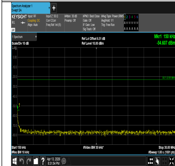
Band26(824-849)-3MHz-16QAM-26915-15RB#0-0.15~30-PA SS
