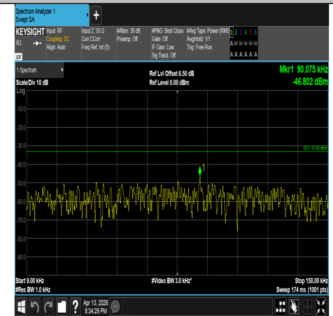
Band26(824-849)-3MHz-QPSK-27025-1RB#14-0.009~0.15-P ASS
