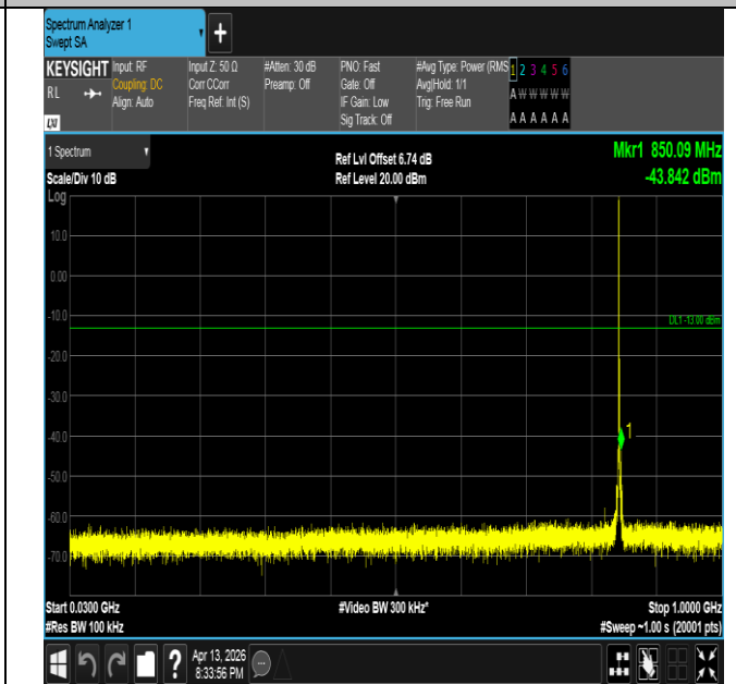
Band26(824-849)-3MHz-16QAM-27025-1RB#0-30~1000-PAS S
