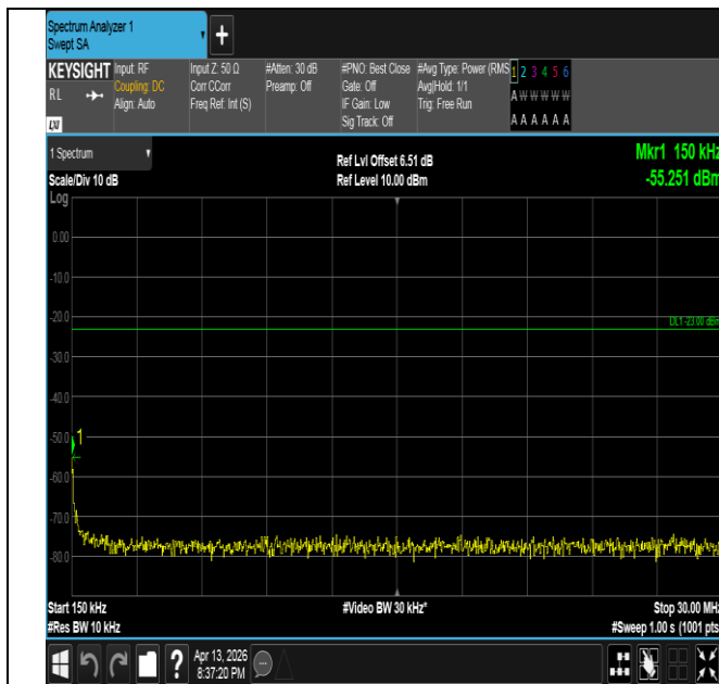
Band26(824-849)-3MHz-16QAM-27025-15RB#0-0.15~30-PA
