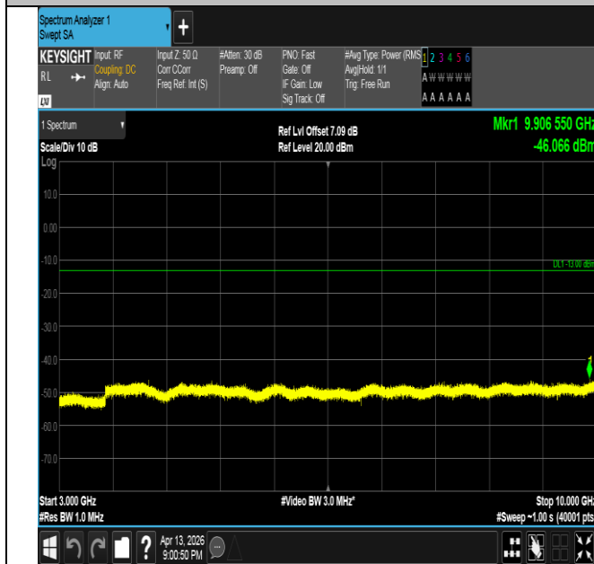
Band26(824-849)-5MHz-QPSK-26915-1RB#0-3000~10000-P ASS
