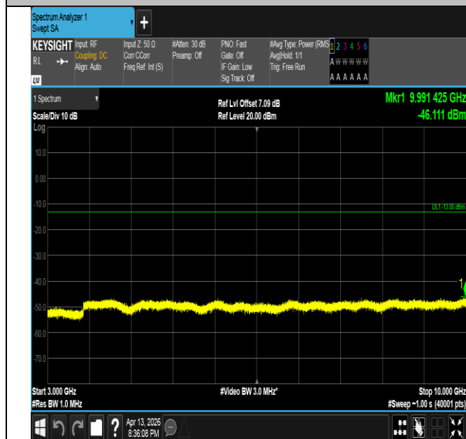
Band26(824-849)-3MHz-16QAM-27025-1RB#14-3000~10000
