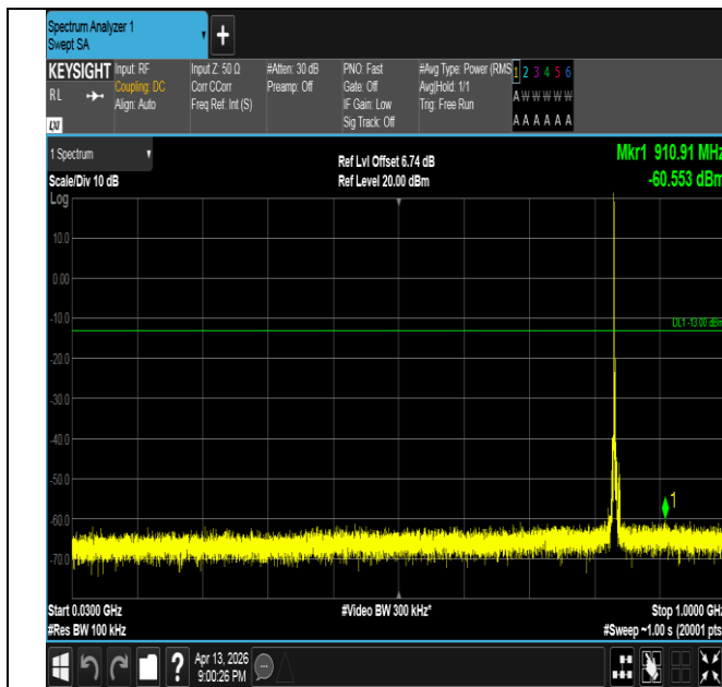
Band26(824-849)-5MHz-QPSK-26915-1RB#0-30~1000-PASS
