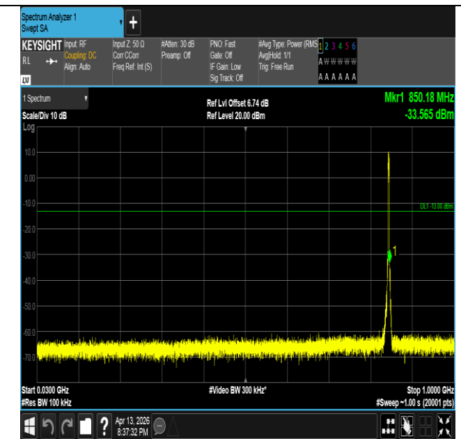
Band26(824-849)-3MHz-16QAM-27025-15RB#0-30~1000-PA
