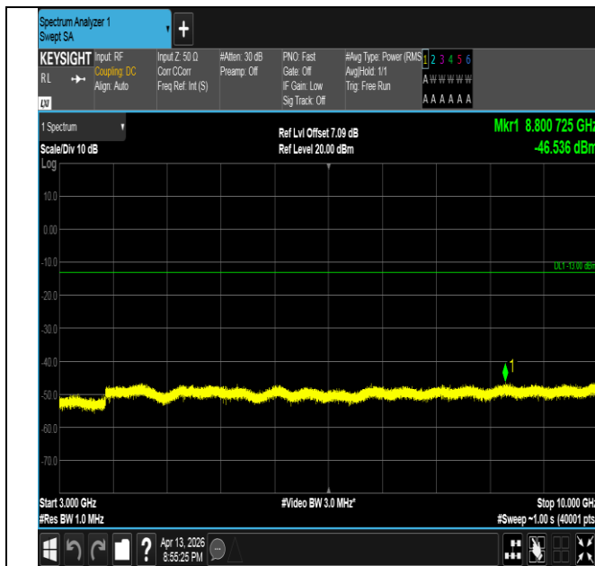
Band26(824-849)-5MHz-QPSK-26815-1RB#0-3000~10000-P
