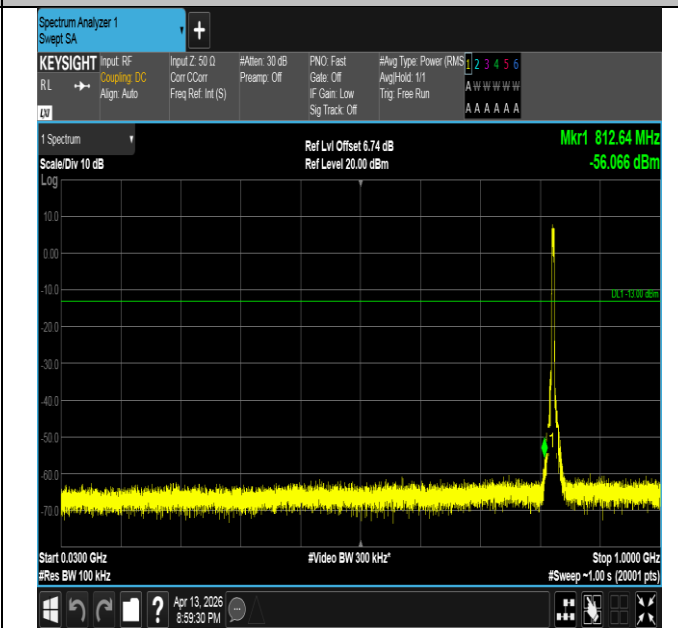
Band26(824-849)-5MHz-16QAM-26815-25RB#0-30~1000-PA SS
