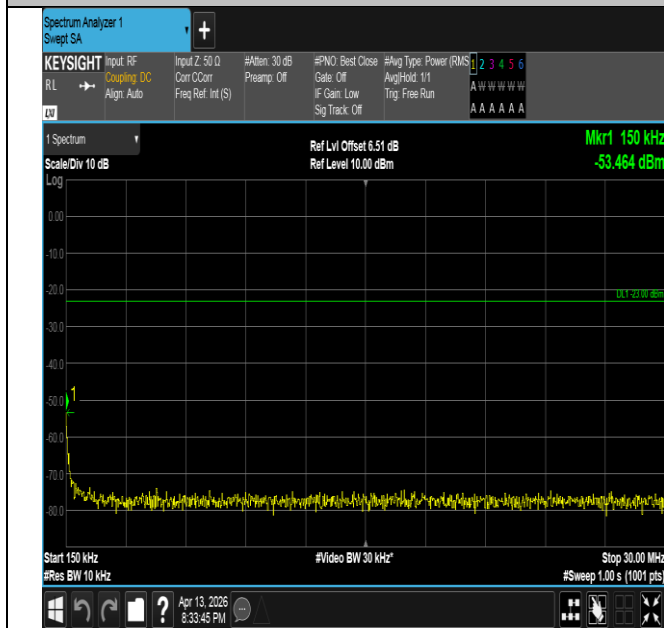
Band26(824-849)-3MHz-16QAM-27025-1RB#0-0.15~30-PAS S
