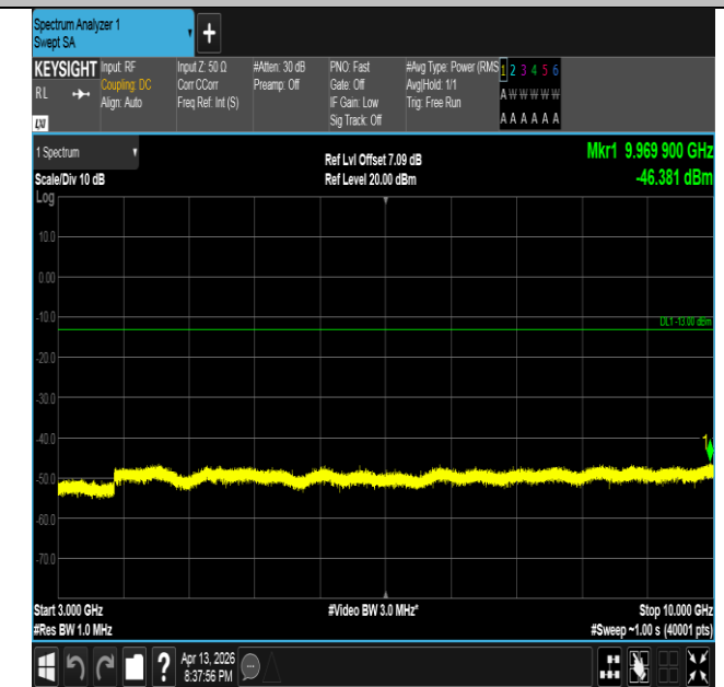
Band26(824-849)-3MHz-16QAM-27025-15RB#0-3000~10000
