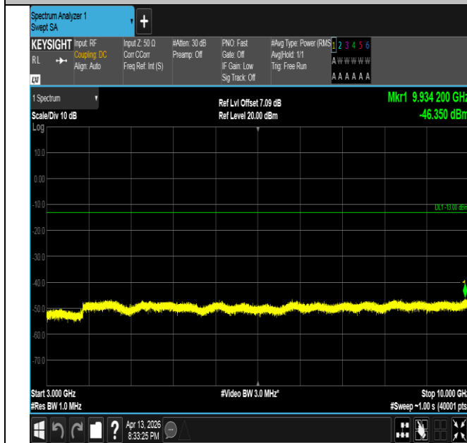
Band26(824-849)-3MHz-QPSK-27025-1RB#0-3000~10000-P ASS
