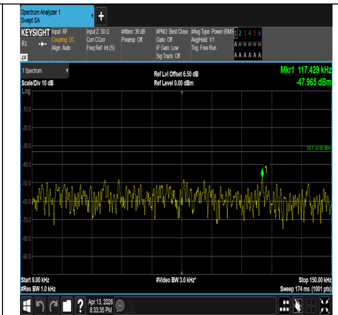
Band26(824-849)-3MHz-16QAM-27025-1RB#0-0.009~0.15-P ASS
