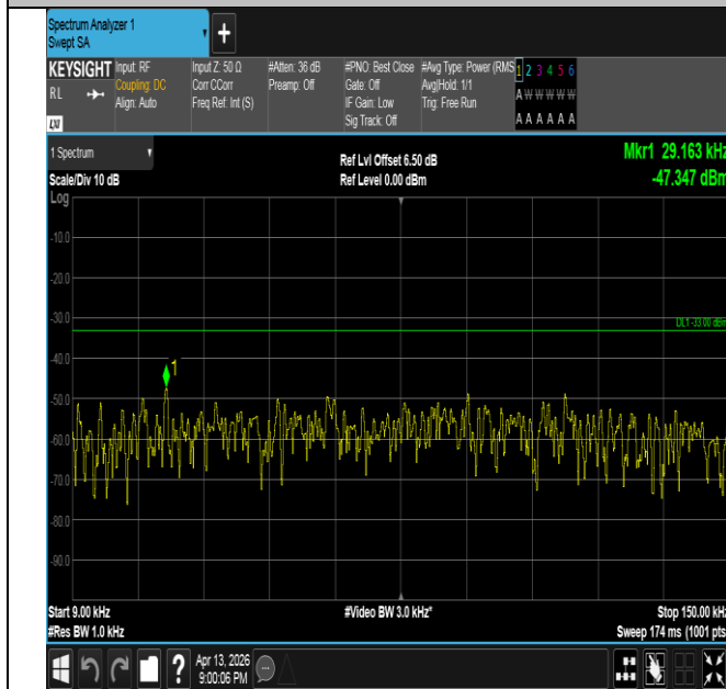
Band26(824-849)-5MHz-QPSK-26915-1RB#0-0.009~0.15-PA SS
