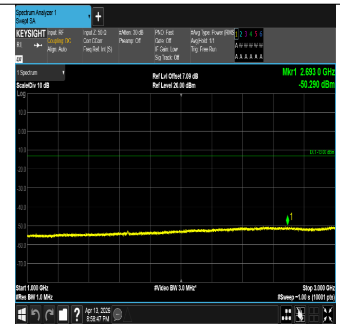
Band26(824-849)-5MHz-QPSK-26815-25RB#0-1000~3000-P
