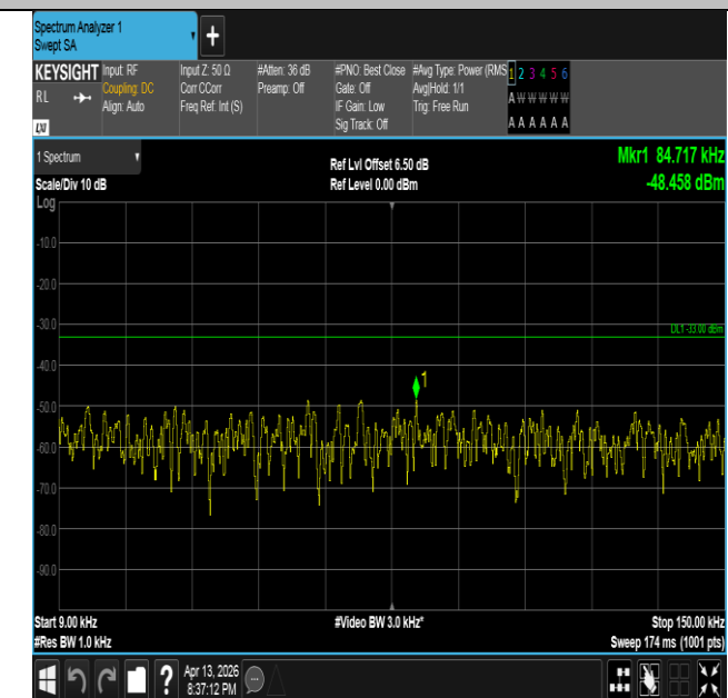
Band26(824-849)-3MHz-16QAM-27025-15RB#0-0.009~0.15-
