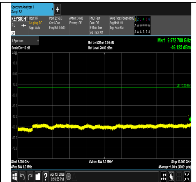
Band26(824-849)-5MHz-16QAM-26815-25RB#0-3000~10000 -PASS
