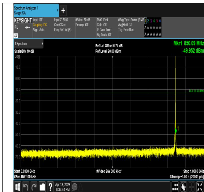
Band26(824-849)-3MHz-16QAM-27025-1RB#14-30~1000-PA
