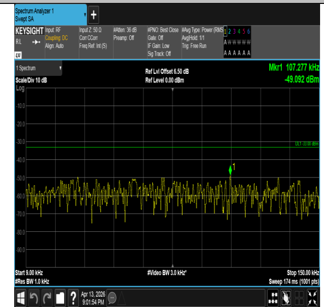
Band26(824-849)-5MHz-QPSK-26915-1RB#24-0.009~0.15-P ASS
