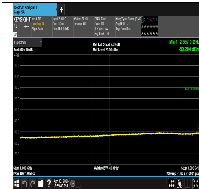
Band26(824-849)-5MHz-16QAM-26815-25RB#0-1000~3000- PASS
