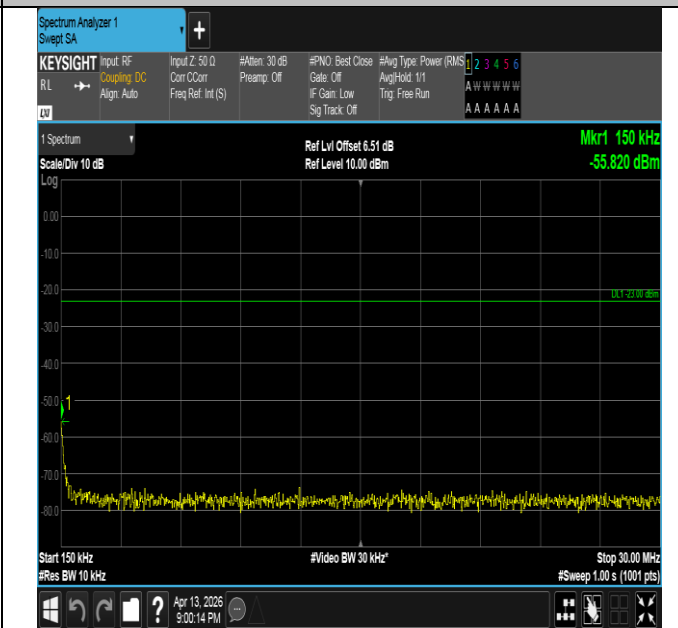
Band26(824-849)-5MHz-QPSK-26915-1RB#0-0.15~30-PASS
