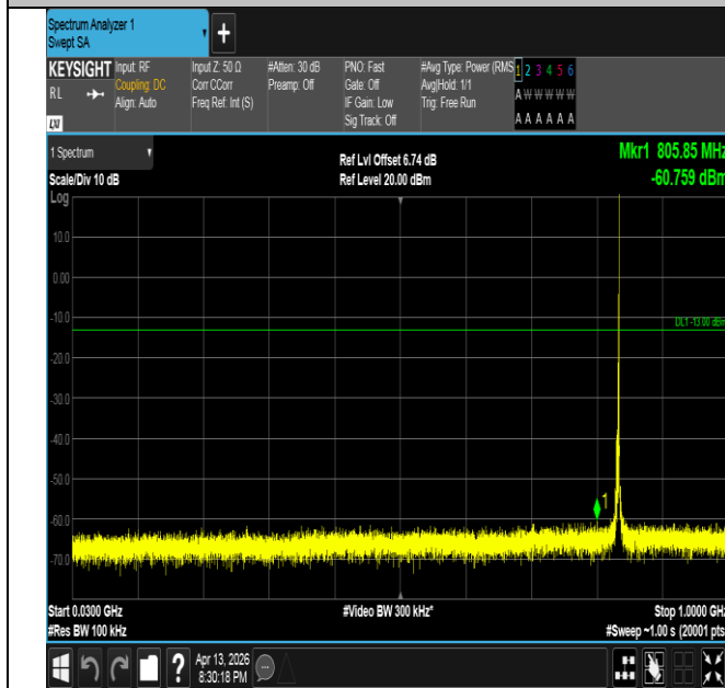
Band26(824-849)-3MHz-16QAM-26915-1RB#14-30~1000-PA SS
