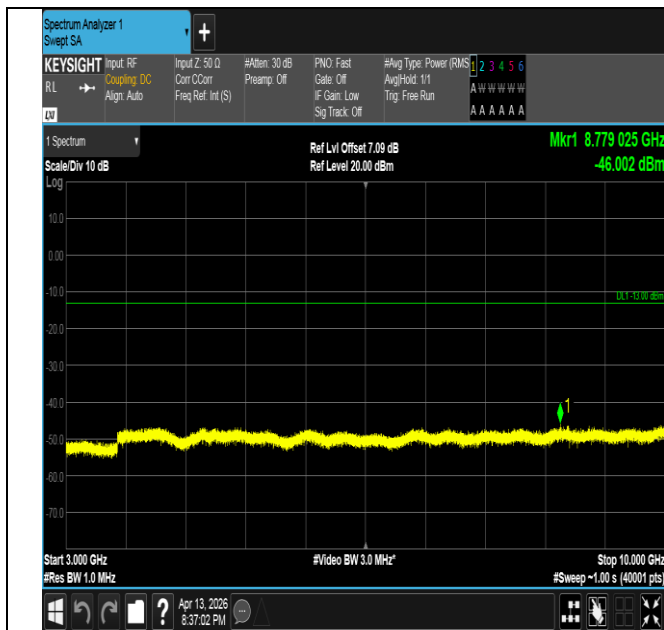
Band26(824-849)-3MHz-QPSK-27025-15RB#0-3000~10000- PASS
