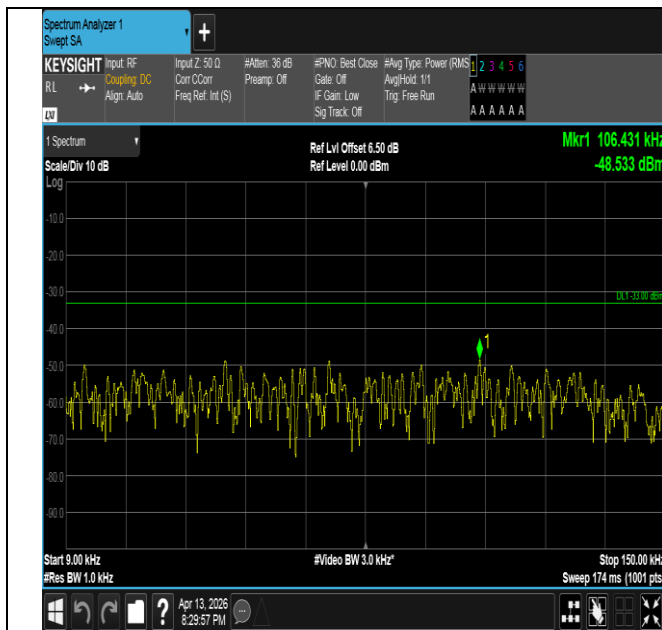
Band26(824-849)-3MHz-16QAM-26915-1RB#14-0.009~0.15- PASS
