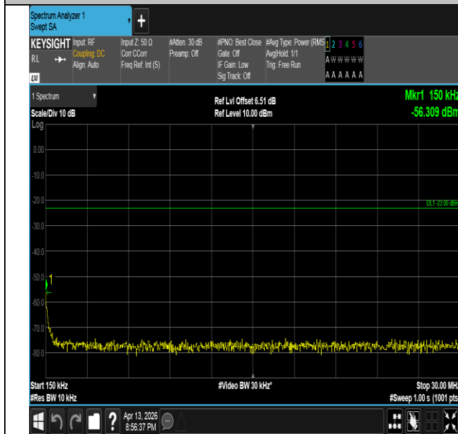
Band26(824-849)-5MHz-QPSK-26815-1RB#24-0.15~30-PAS
