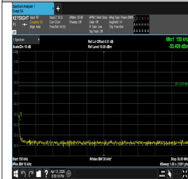
Band26(824-849)-5MHz-16QAM-26815-25RB#0-0.15~30-PA SS
