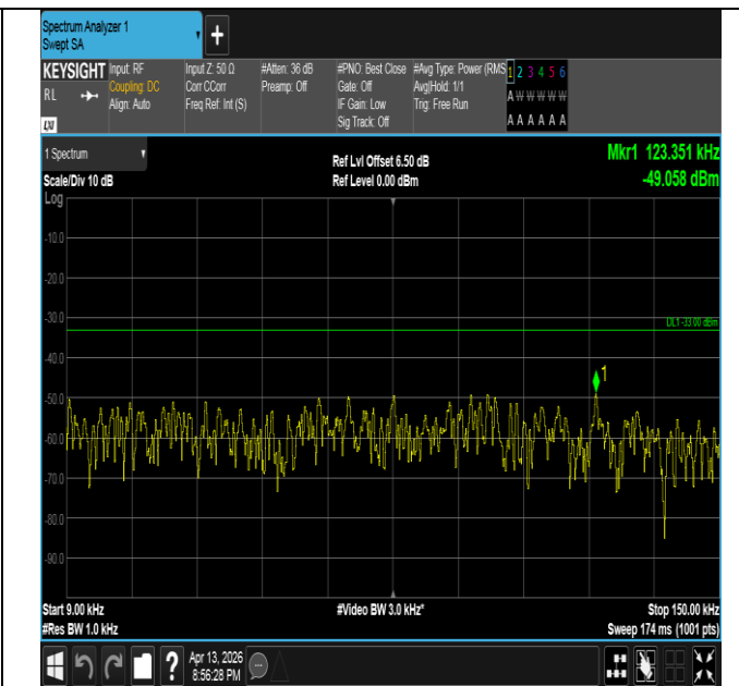
Band26(824-849)-5MHz-QPSK-26815-1RB#24-0.009~0.15-P
