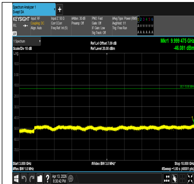
Band26(824-849)-3MHz-16QAM-26915-1RB#14-3000~10000 -PASS
