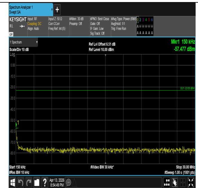
Band26(824-849)-5MHz-QPSK-26815-1RB#0-0.15~30-PASS
