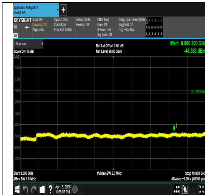
Band26(824-849)-5MHz-16QAM-26815-1RB#24-3000~10000 -PASS
