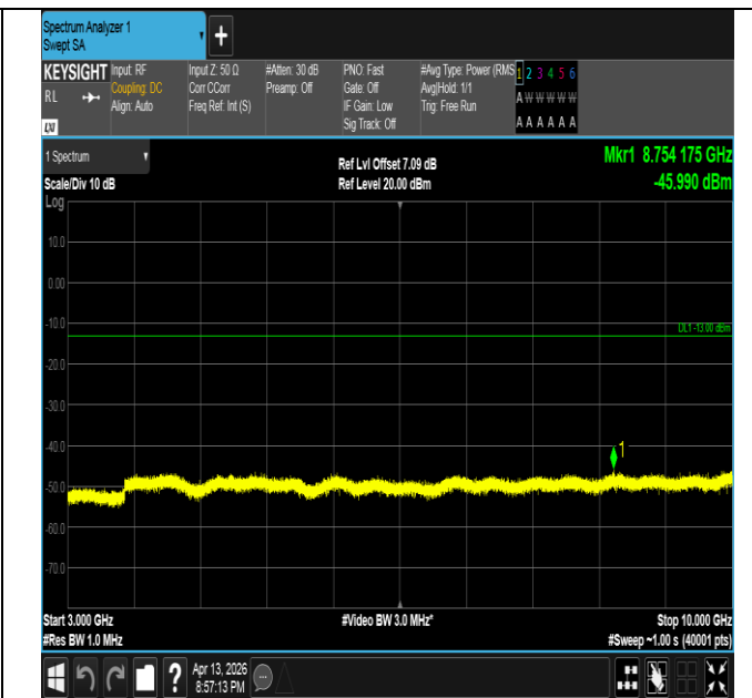
Band26(824-849)-5MHz-QPSK-26815-1RB#24-3000~10000-P
