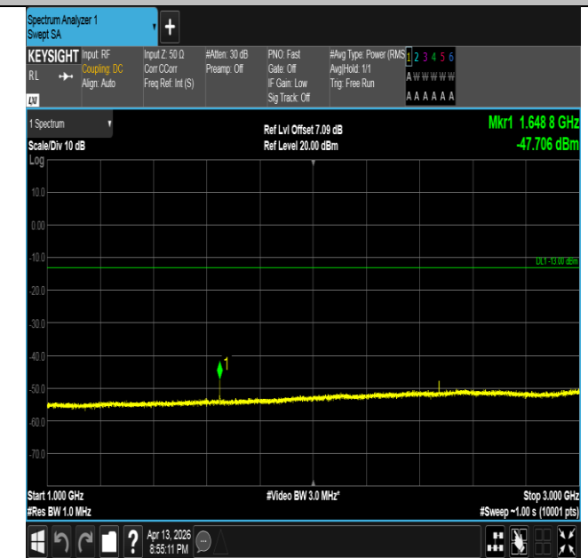
Band26(824-849)-5MHz-QPSK-26815-1RB#0-1000~3000-PA SS
