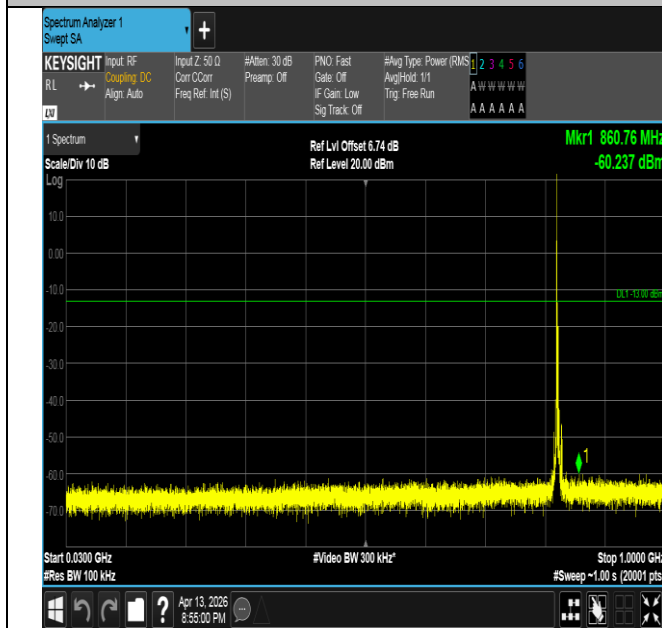
Band26(824-849)-5MHz-QPSK-26815-1RB#0-30~1000-PASS
