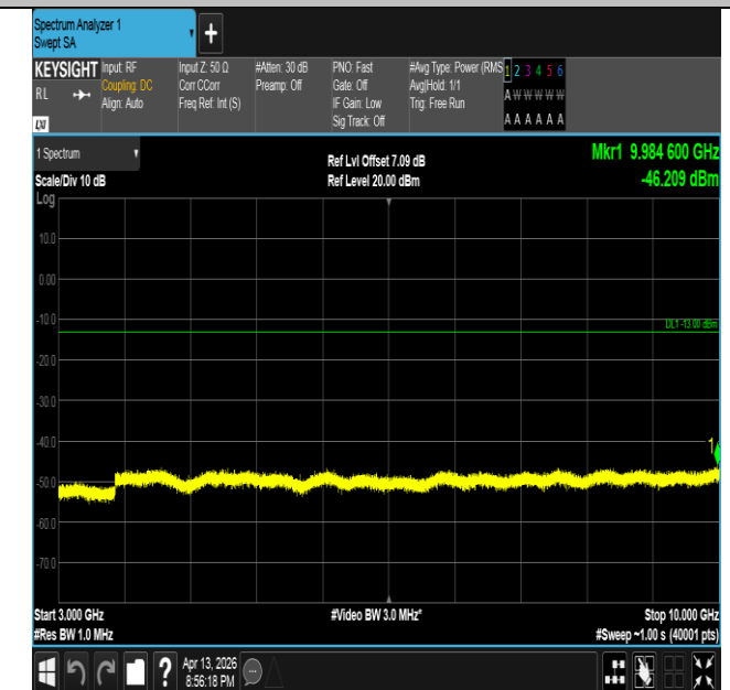
Band26(824-849)-5MHz-16QAM-26815-1RB#0-3000~10000-PASS
