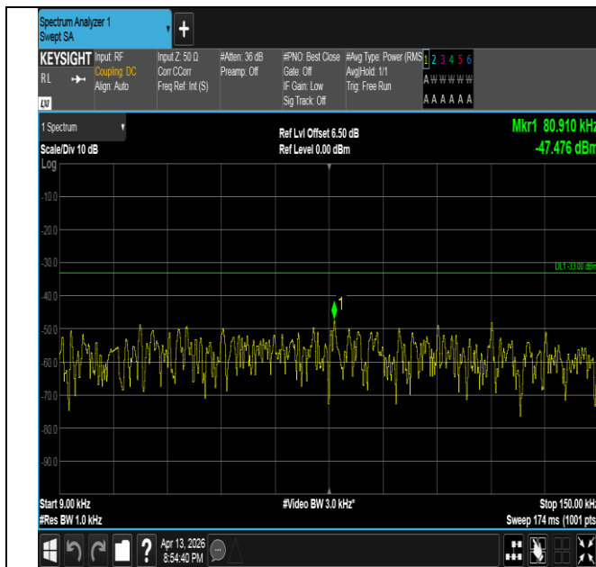
Band26(824-849)-5MHz-QPSK-26815-1RB#0-0.009~0.15-PA SS
