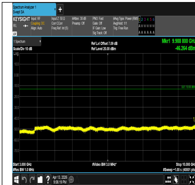
Band26(824-849)-5MHz-QPSK-27015-1RB#0-3000~10000-P
