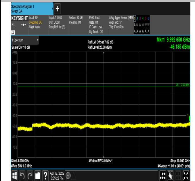
Band26(824-849)-5MHz-16QAM-26915-25RB#0-3000~10000
