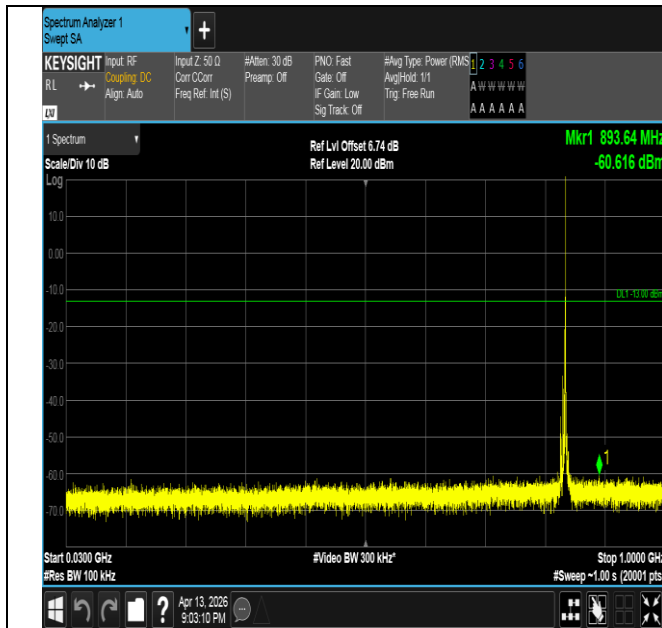
Band26(824-849)-5MHz-16QAM-26915-1RB#24-30~1000-PA SS
