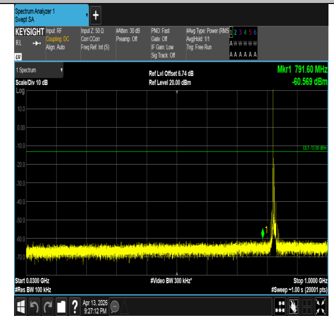
Band26(824-849)-10MHz-16QAM-26840-1RB#0-30~1000-PA SS
