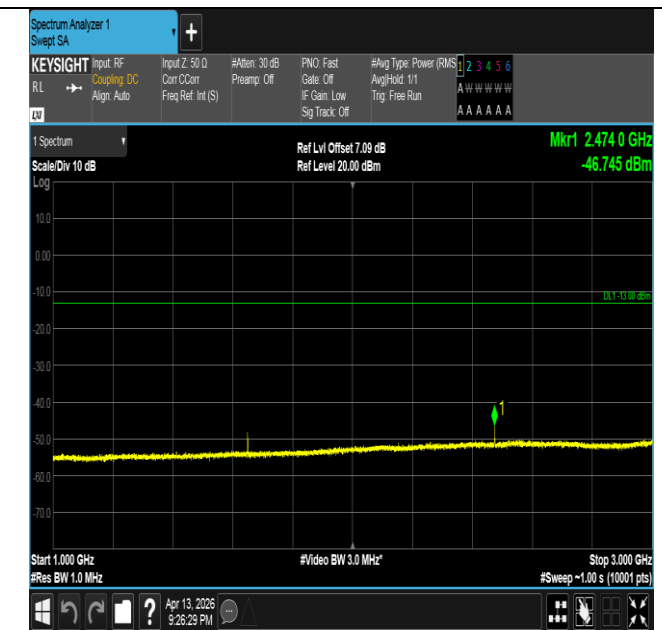
Band26(824-849)-10MHz-QPSK-26840-1RB#0-1000~3000-P
