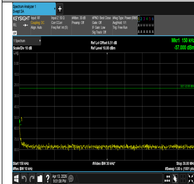
Band26(824-849)-5MHz-16QAM-26915-1RB#0-0.15~30-PAS S
