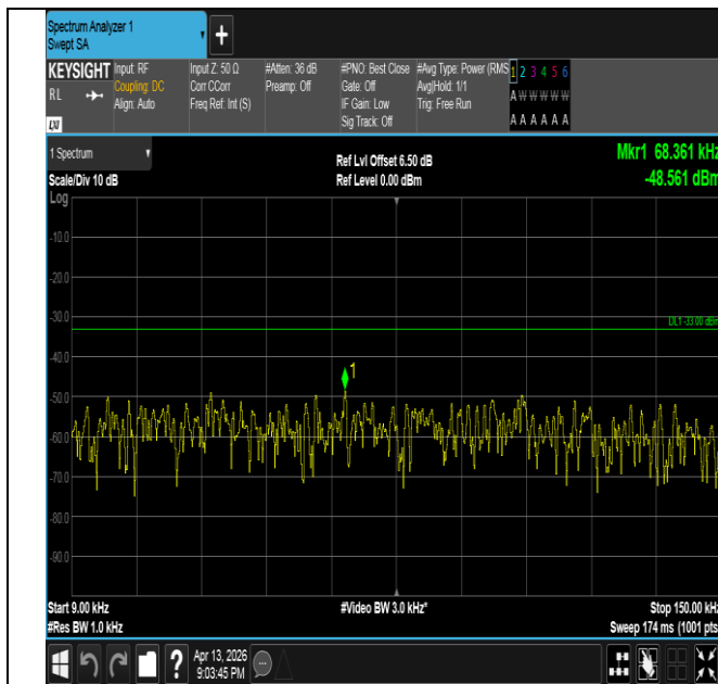
Band26(824-849)-5MHz-QPSK-26915-25RB#0-0.009~0.15-P ASS
