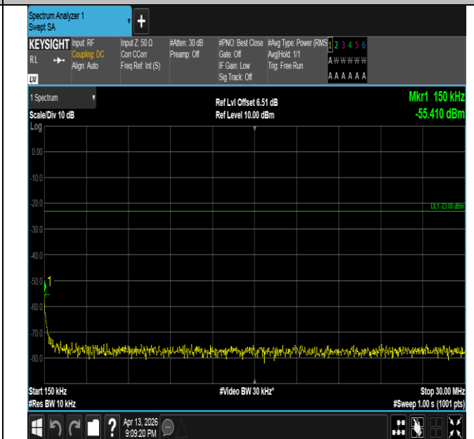
Band26(824-849)-5MHz-QPSK-27015-25RB#0-0.15~30-PAS
