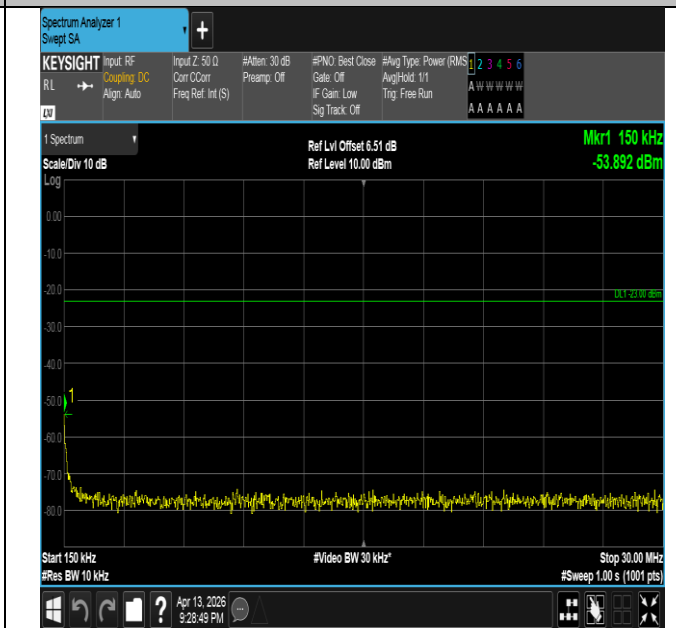
Band26(824-849)-10MHz-16QAM-26840-1RB#49-0.15~30-PA SS
