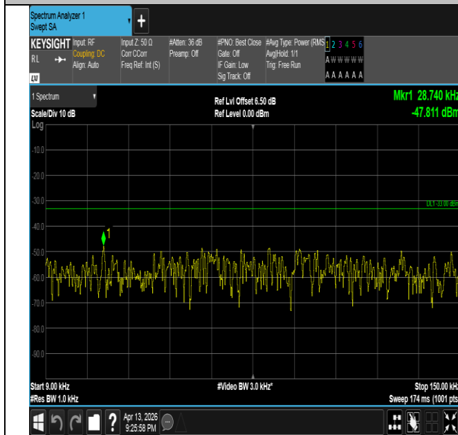
Band26(824-849)-10MHz-QPSK-26840-1RB#0-0.009~0.15-P ASS
