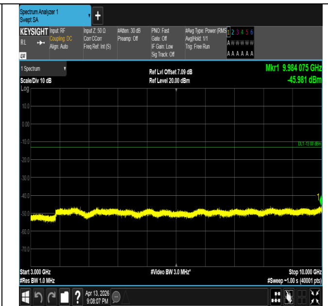
Band26(824-849)-5MHz-QPSK-27015-1RB#24-3000~10000-P
