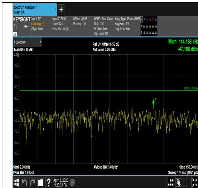
Band26(824-849)-10MHz-QPSK-26840-50RB#0-0.009~0.15- PASS
