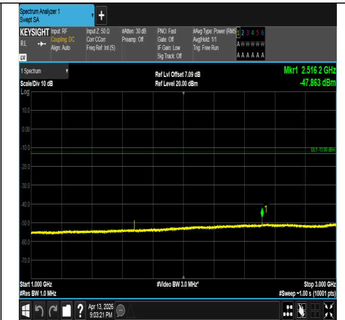
Band26(824-849)-5MHz-16QAM-26915-1RB#24-1000~3000- PASS
