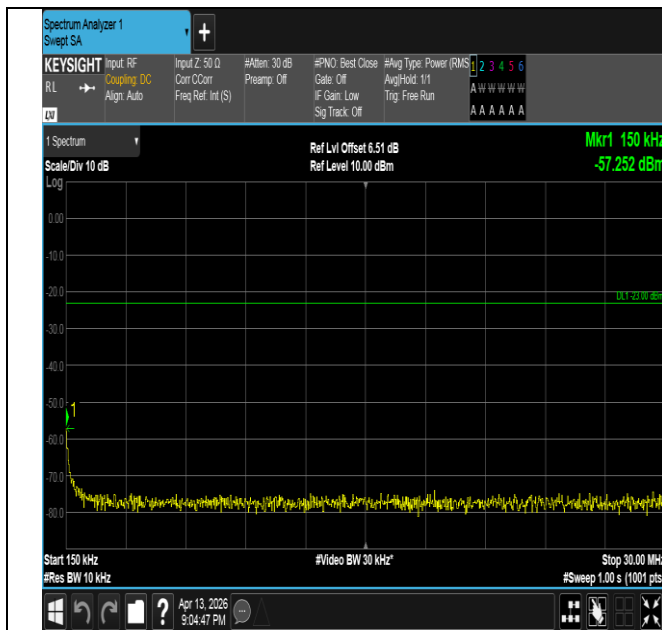
Band26(824-849)-5MHz-16QAM-26915-25RB#0-0.15~30-PA
