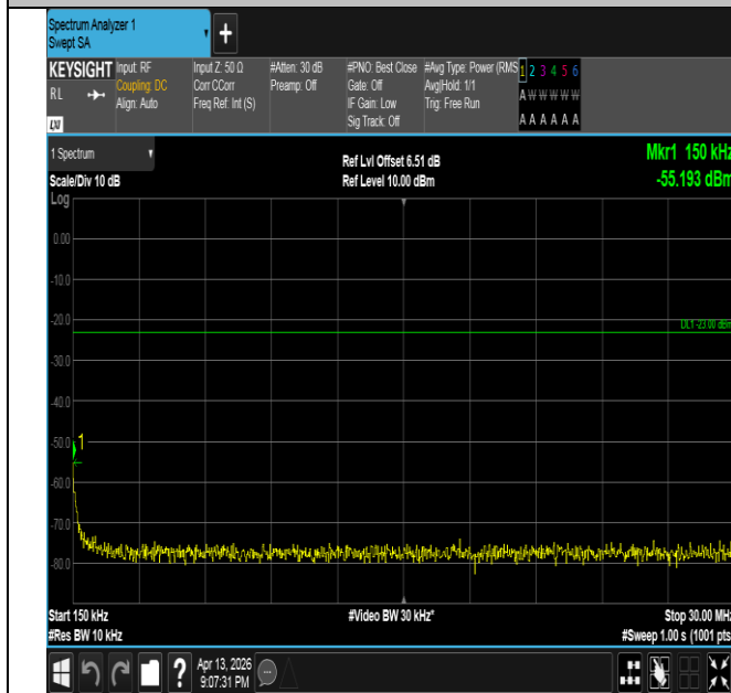
Band26(824-849)-5MHz-QPSK-27015-1RB#24-0.15~30-PAS
