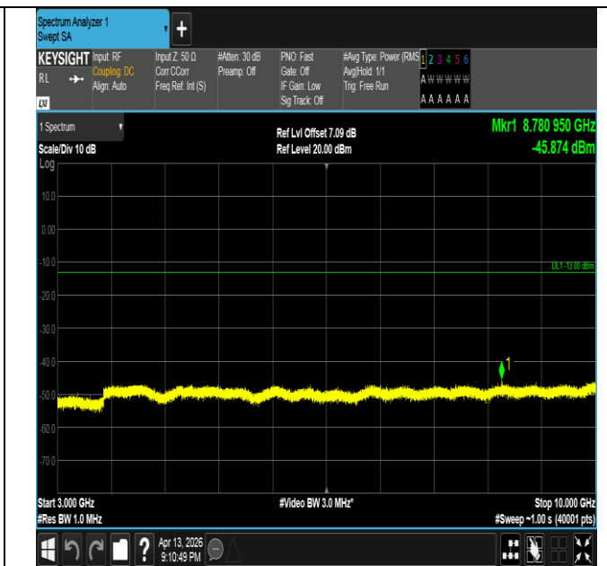
Band26(824-849)-5MHz-16QAM-27015-25RB#0-3000~10000 -PASS
