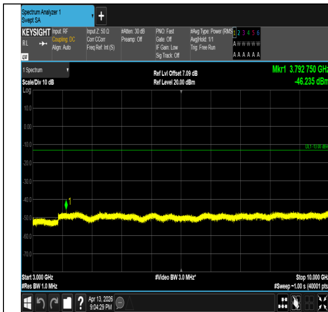
Band26(824-849)-5MHz-QPSK-26915-25RB#0-3000~10000- PASS
