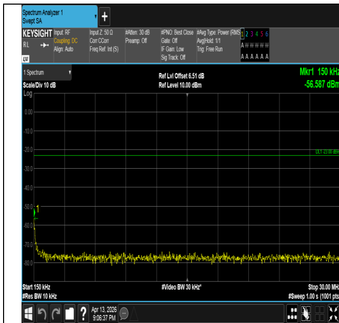
Band26(824-849)-5MHz-16QAM-27015-1RB#0-0.15~30-PAS
