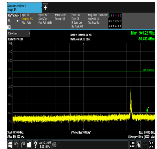
Band26(824-849)-5MHz-QPSK-26915-1RB#24-30~1000-PAS
