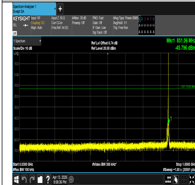
Band26(824-849)-5MHz-16QAM-27015-1RB#24-30~1000-PA SS
