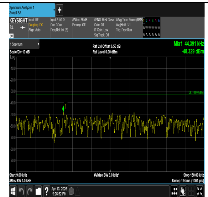
Band26(824-849)-10MHz-16QAM-26840-1RB#0-0.009~0.15- PASS
