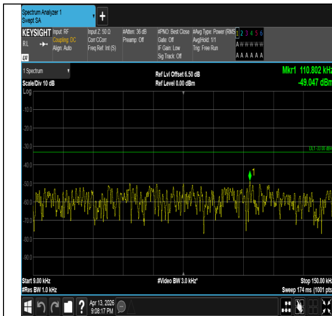
Band26(824-849)-5MHz-16QAM-27015-1RB#24-0.009~0.15- PASS
