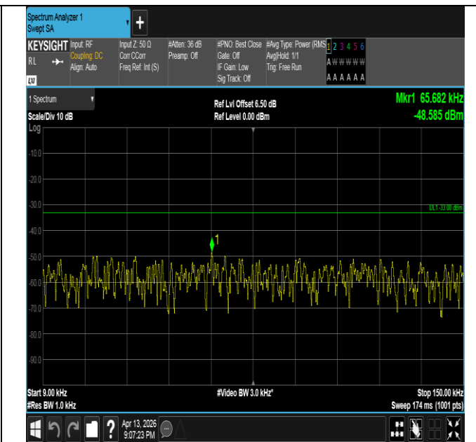
Band26(824-849)-5MHz-QPSK-27015-1RB#24-0.009~0.15-P
