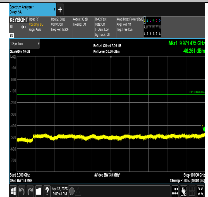
Band26(824-849)-5MHz-QPSK-26915-1RB#24-3000~10000-P
