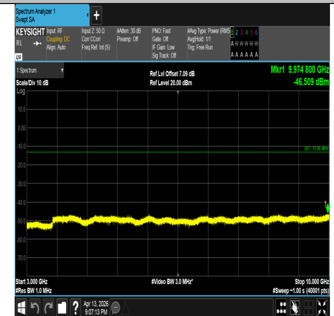
Band26(824-849)-5MHz-16QAM-27015-1RB#0-3000~10000-PASS
