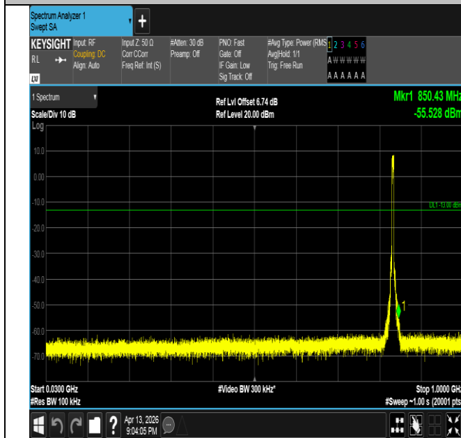
Band26(824-849)-5MHz-QPSK-26915-25RB#0-30~1000-PAS S
