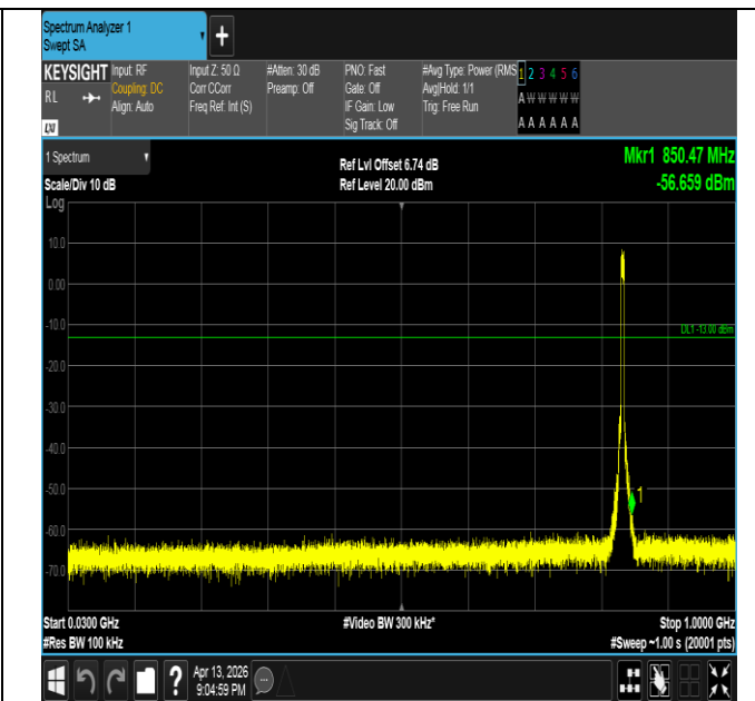
Band26(824-849)-5MHz-16QAM-26915-25RB#0-30~1000-PA
