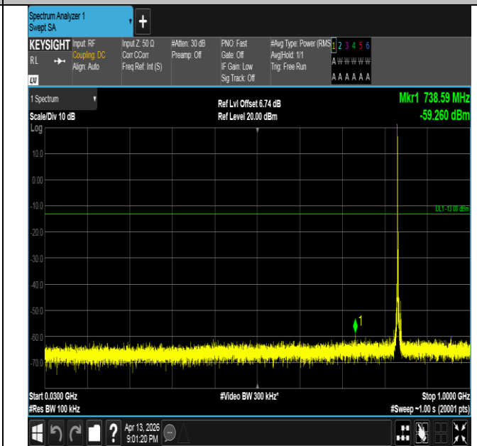
Band26(824-849)-5MHz-16QAM-26915-1RB#0-30~1000-PAS S
