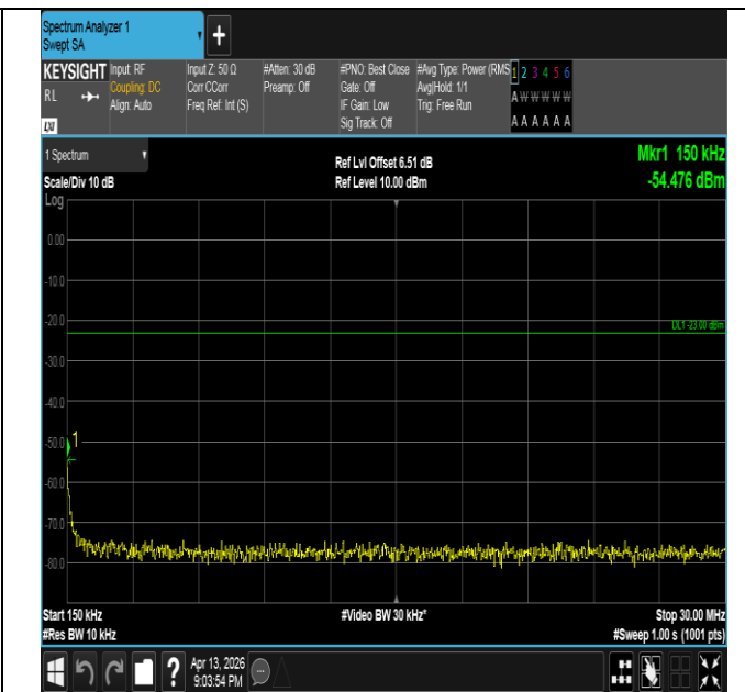
Band26(824-849)-5MHz-QPSK-26915-25RB#0-0.15~30-PAS S
