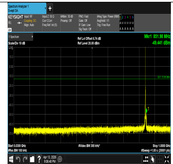
Band26(824-849)-5MHz-16QAM-27015-1RB#0-30~1000-PAS
