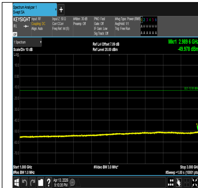
Band26(824-849)-5MHz-16QAM-27015-25RB#0-1000~3000- PASS
