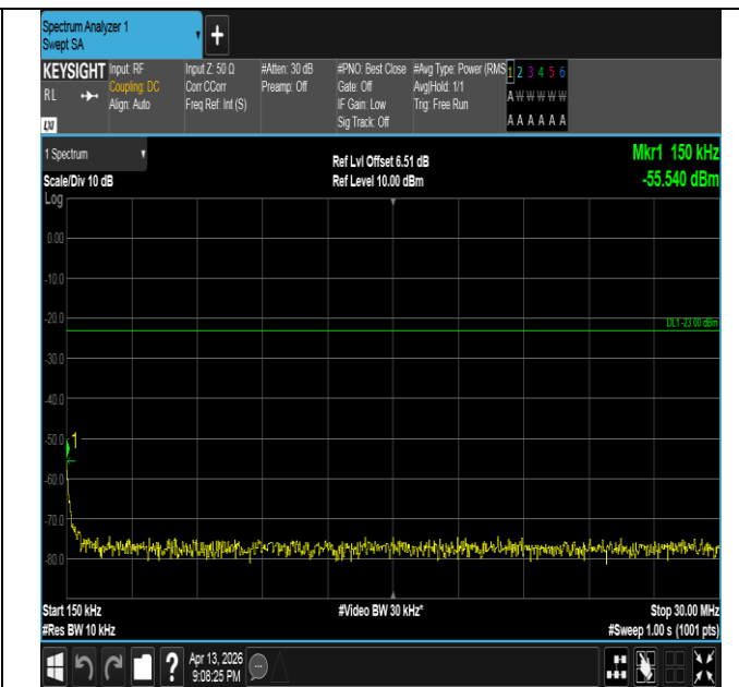
Band26(824-849)-5MHz-16QAM-27015-1RB#24-0.15~30-PAS S
