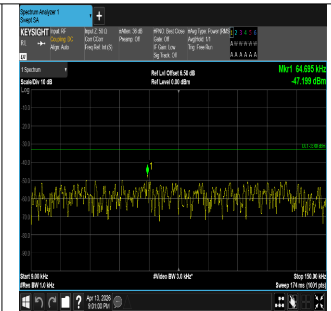
Band26(824-849)-5MHz-16QAM-26915-1RB#0-0.009~0.15-P ASS
