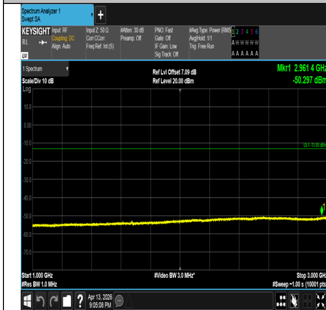
Band26(824-849)-5MHz-16QAM-26915-25RB#0-1000~3000-
