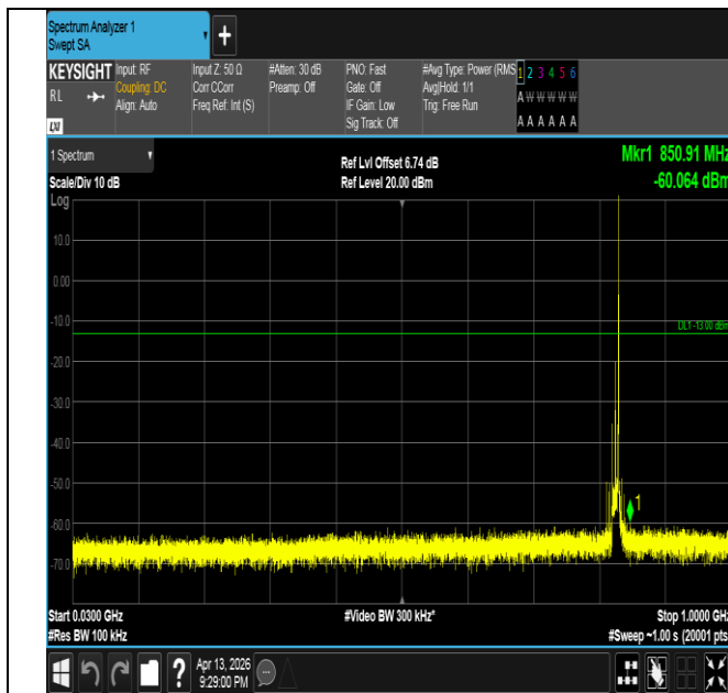
Band26(824-849)-10MHz-16QAM-26840-1RB#49-30~1000-P ASS
