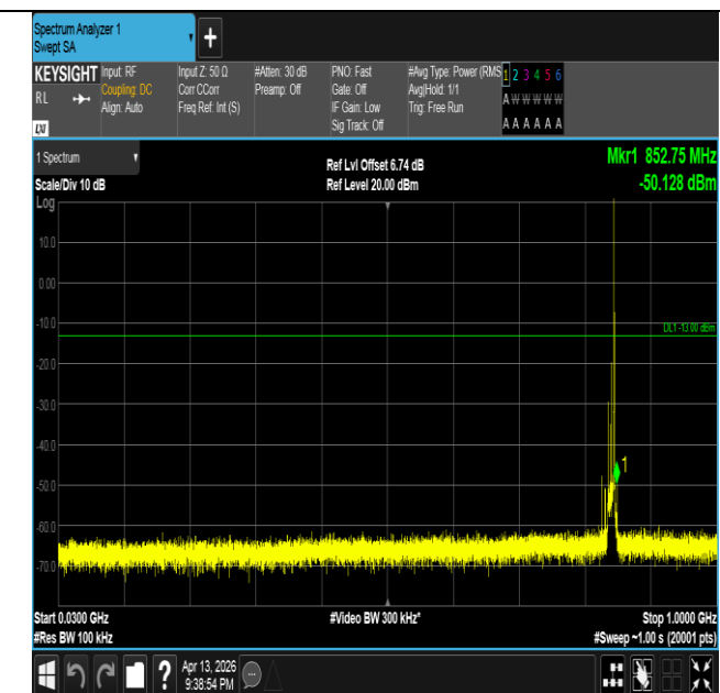
Band26(824-849)-10MHz-QPSK-26990-1RB#49-30~1000-PA
