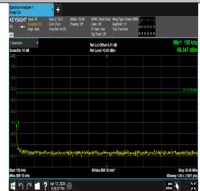
Band26(824-849)-10MHz-16QAM-26990-1RB#49-0.15~30-PA SS
