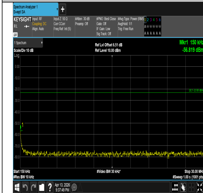
Band26(824-849)-10MHz-16QAM-26990-1RB#0-0.15~30-PA SS
