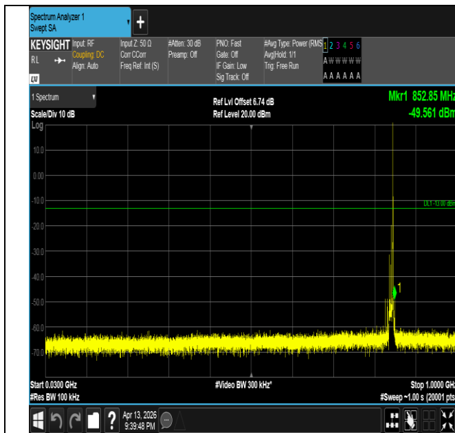
Band26(824-849)-10MHz-16QAM-26990-1RB#49-30~1000-P ASS
