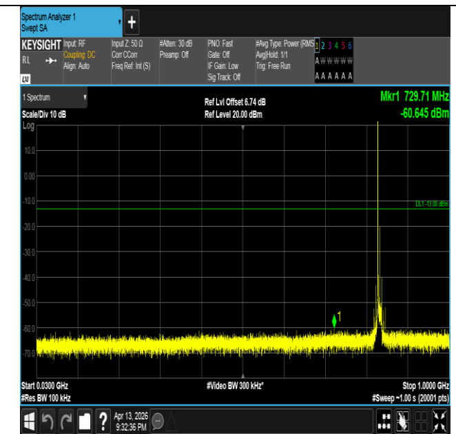
Band26(824-849)-10MHz-16QAM-26915-1RB#0-30~1000-PA
