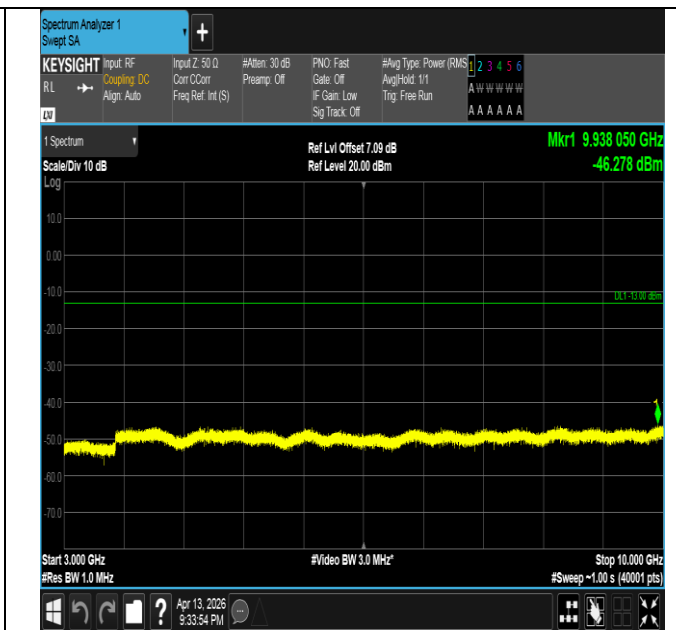
Band26(824-849)-10MHz-QPSK-26915-1RB#49-3000~10000- PASS
