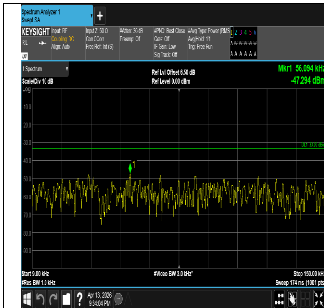
Band26(824-849)-10MHz-16QAM-26915-1RB#49-0.009~0.15
