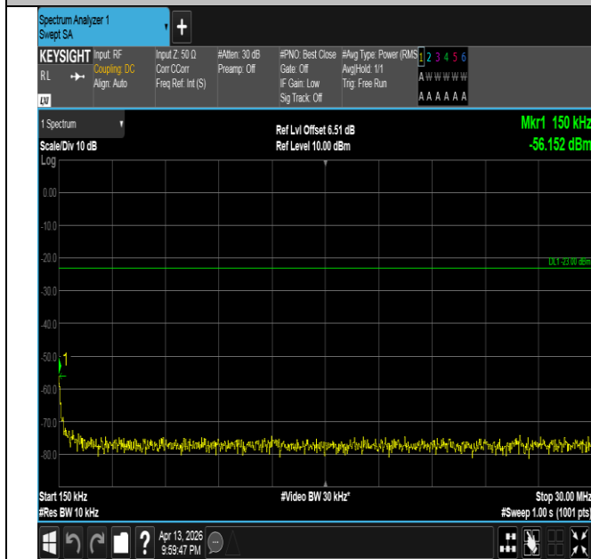
Band26(824-849)-15MHz-QPSK-26865-1RB#74-0.15~30-PA S
