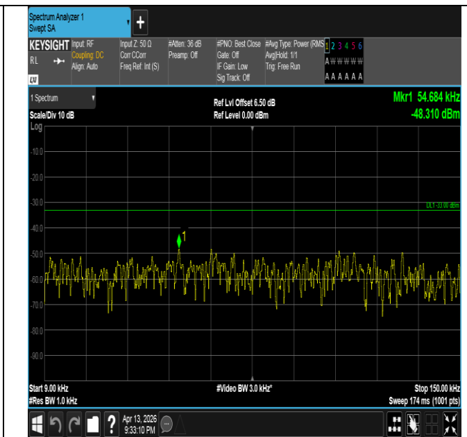
Band26(824-849)-10MHz-QPSK-26915-1RB#49-0.009~0.15-P ASS
