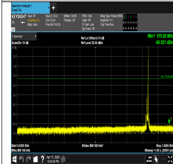
Band26(824-849)-10MHz-16QAM-26915-1RB#49-30~1000-P
