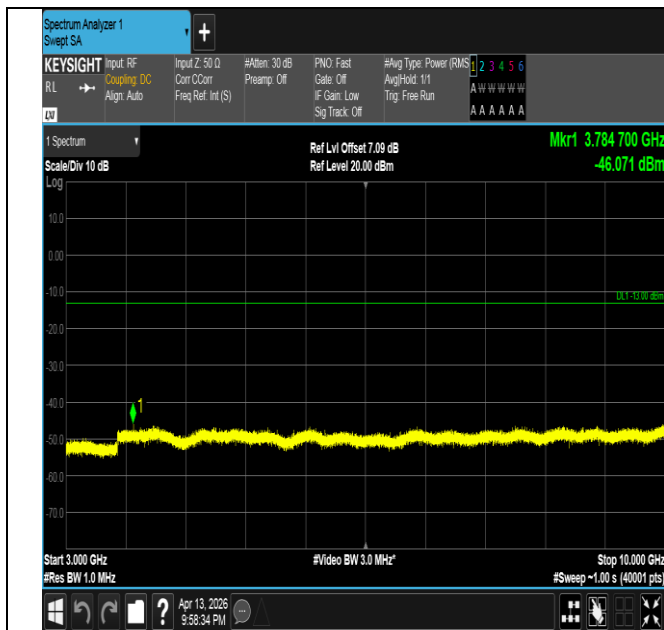
Band26(824-849)-15MHz-QPSK-26865-1RB#0-3000~10000- PASS
