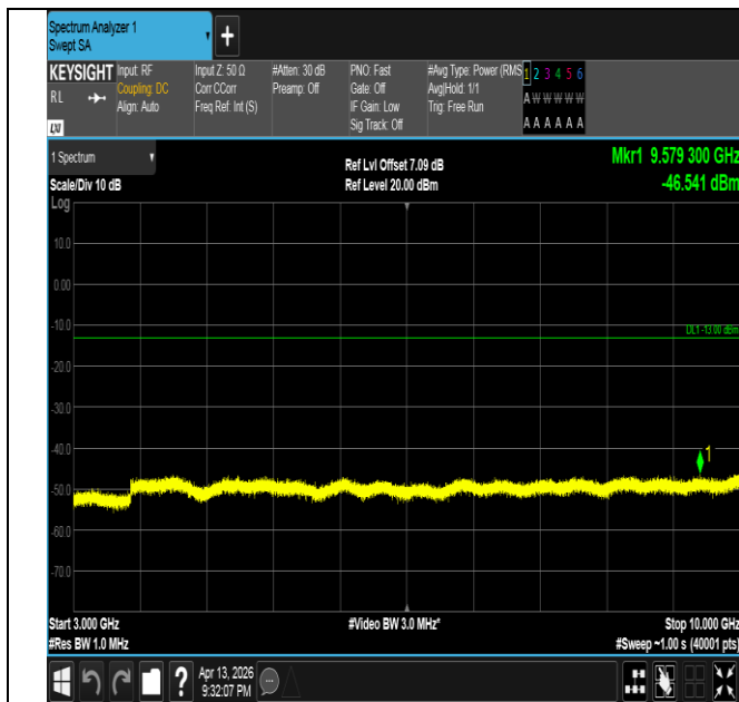
Band26(824-849)-10MHz-QPSK-26915-1RB#0-3000~10000- PASS
