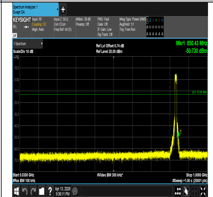
Band26(824-849)-10MHz-16QAM-26915-50RB#0-30~1000-P ASS
