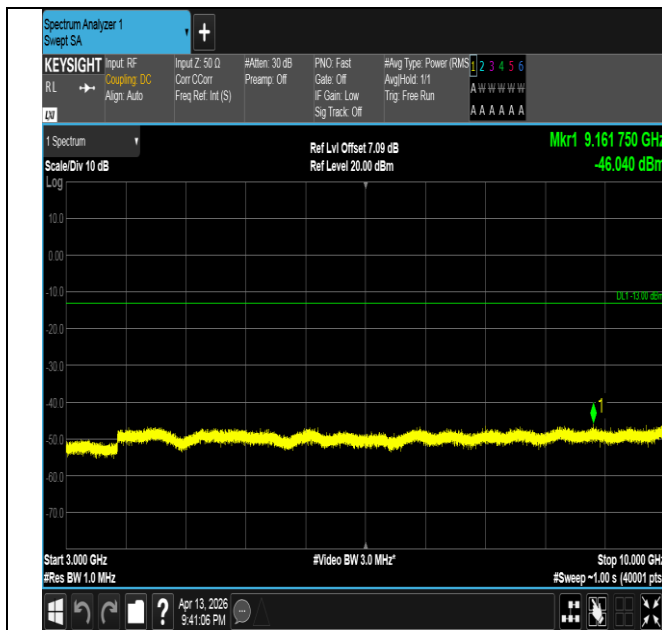
Band26(824-849)-10MHz-QPSK-26990-50RB#0-3000~10000- PASS
