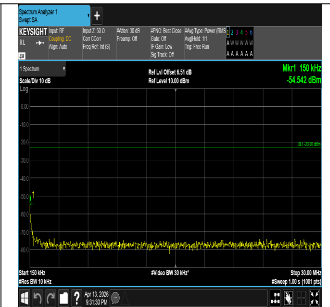
Band26(824-849)-10MHz-QPSK-26915-1RB#0-0.15~30-PAS
