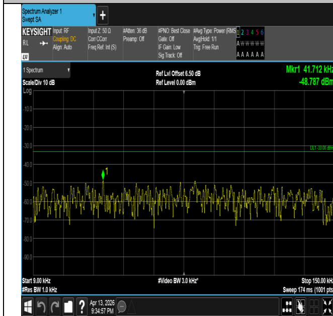
Band26(824-849)-10MHz-QPSK-26915-50RB#0-0.009~0.15- PASS
