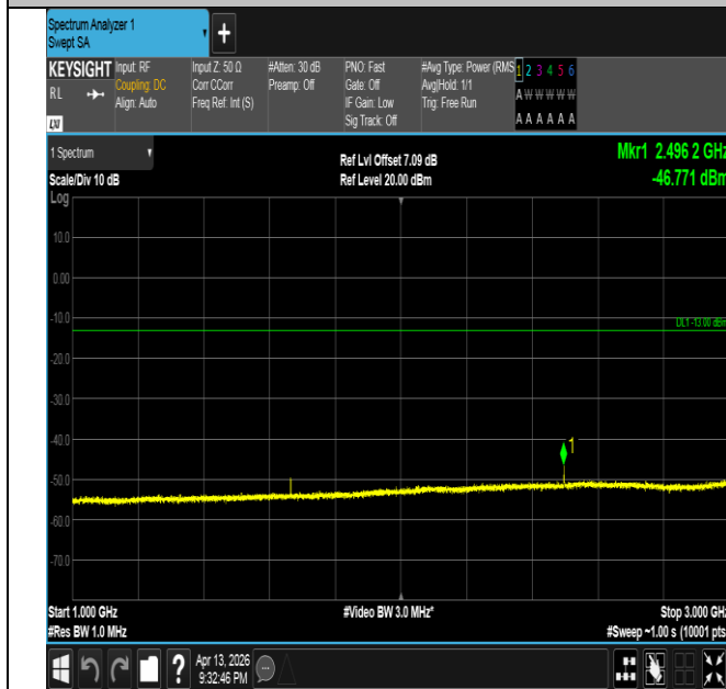
Band26(824-849)-10MHz-16QAM-26915-1RB#0-1000~3000-
