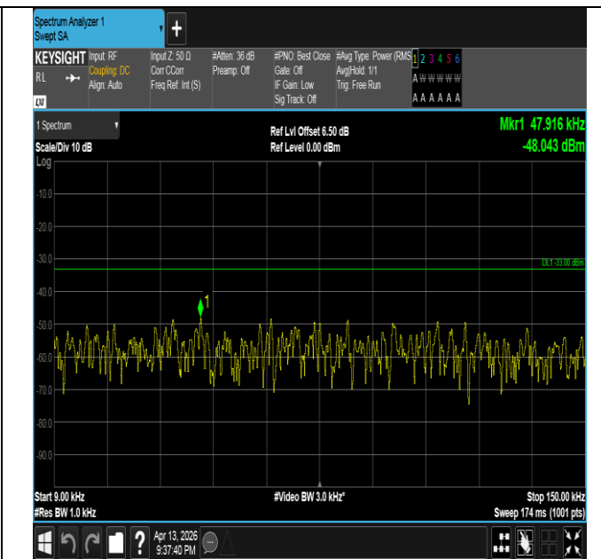
Band26(824-849)-10MHz-16QAM-26990-1RB#0-0.009~0.15- PASS
