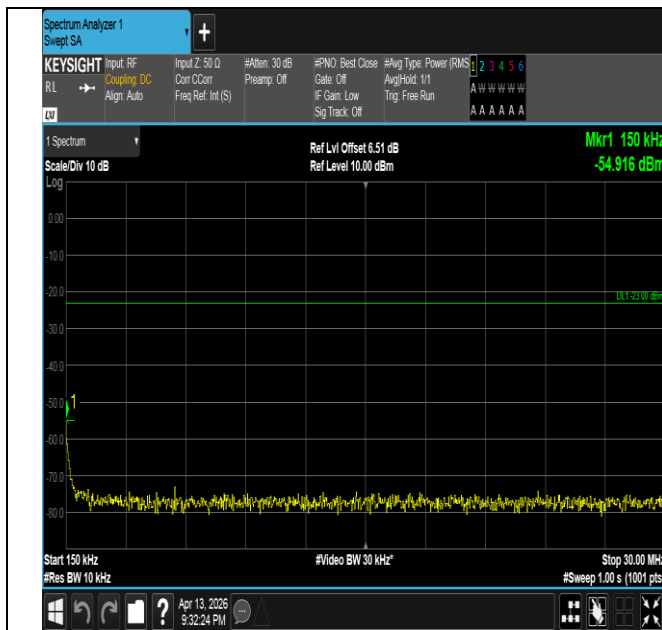
Band26(824-849)-10MHz-16QAM-26915-1RB#0-0.15~30-PA
