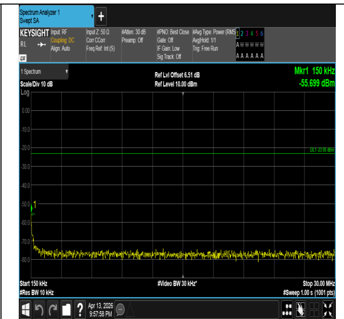
Band26(824-849)-15MHz-QPSK-26865-1RB#0-0.15~30-PAS
