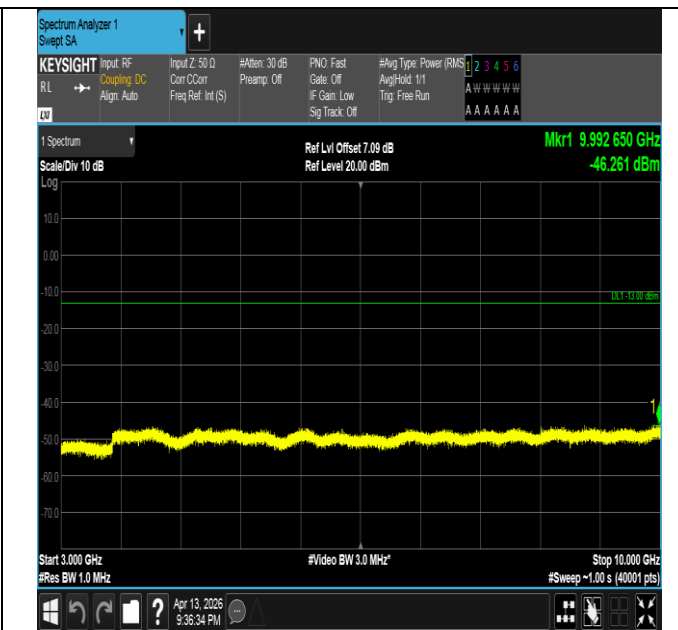
Band26(824-849)-10MHz-16QAM-26915-50RB#0-3000~1000
