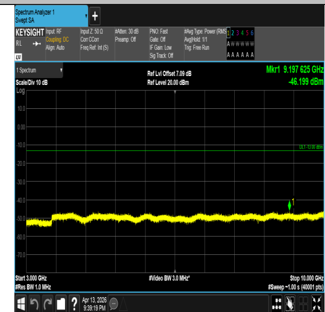
Band26(824-849)-10MHz-QPSK-26990-1RB#49-3000~10000-
