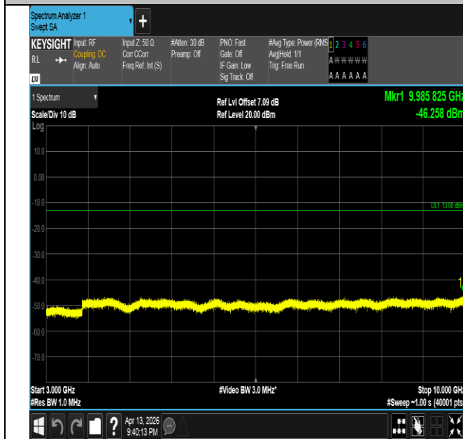
Band26(824-849)-10MHz-16QAM-26990-1RB#49-3000~1000 0-PASS
