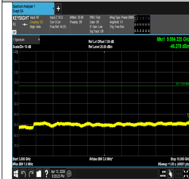
Band26(824-849)-10MHz-16QAM-26840-1RB#49-3000~1000 0-PASS
