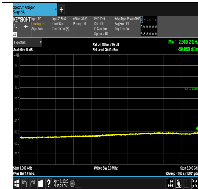
Band26(824-849)-10MHz-16QAM-26915-50RB#0-1000~3000
