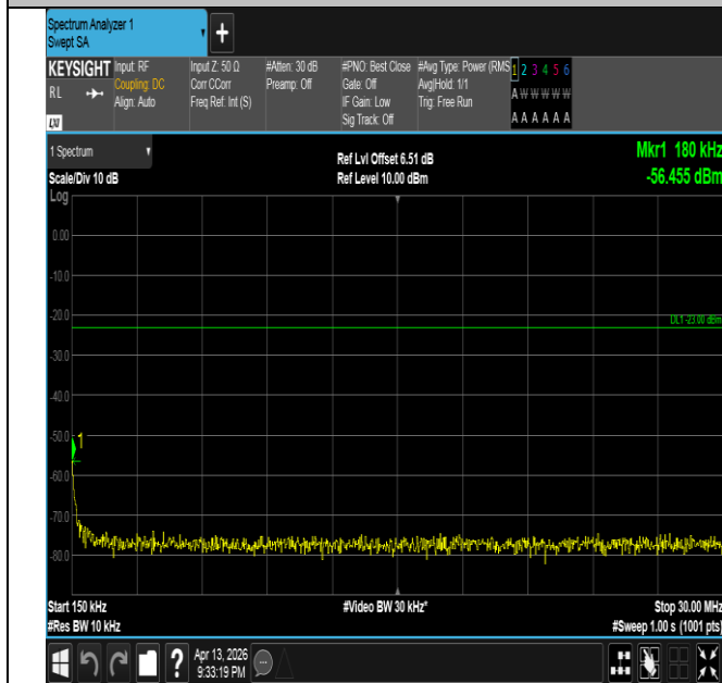
Band26(824-849)-10MHz-QPSK-26915-1RB#49-0.15~30-PA S
