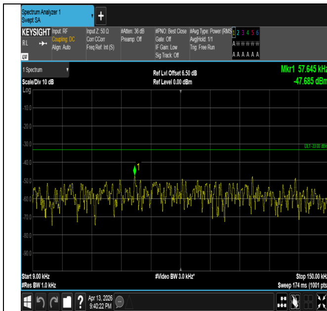
Band26(824-849)-10MHz-QPSK-26990-50RB#0-0.009~0.15- PASS
