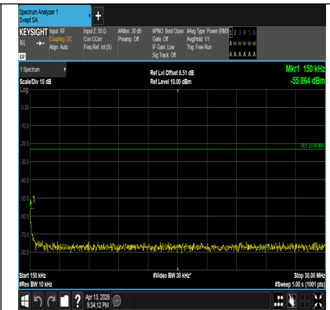
Band26(824-849)-10MHz-16QAM-26915-1RB#49-0.15~30-PA
