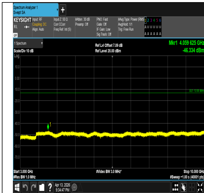
Band26(824-849)-10MHz-16QAM-26915-1RB#49-3000~1000 0-PASS
