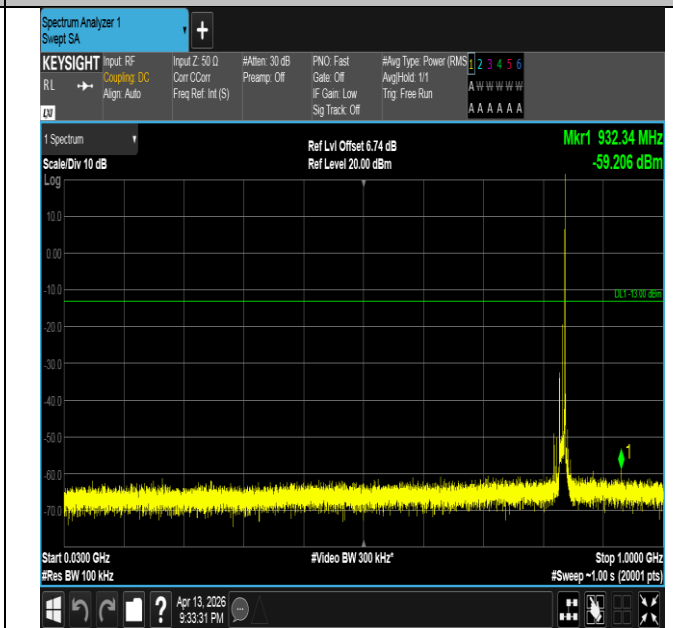
Band26(824-849)-10MHz-QPSK-26915-1RB#49-30~1000-PA SS
