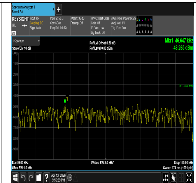
Band26(824-849)-15MHz-QPSK-26865-1RB#74-0.009~0.15-P ASS
