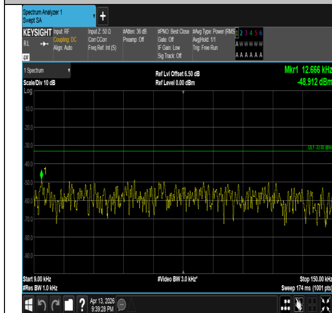
Band26(824-849)-10MHz-16QAM-26990-1RB#49-0.009~0.15 -PASS
