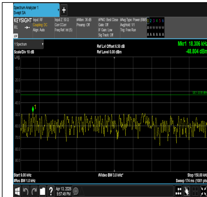
Band26(824-849)-15MHz-QPSK-26865-1RB#0-0.009~0.15-P
