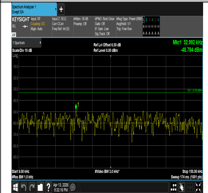
Band26(824-849)-10MHz-16QAM-26915-1RB#0-0.009~0.15- PASS
