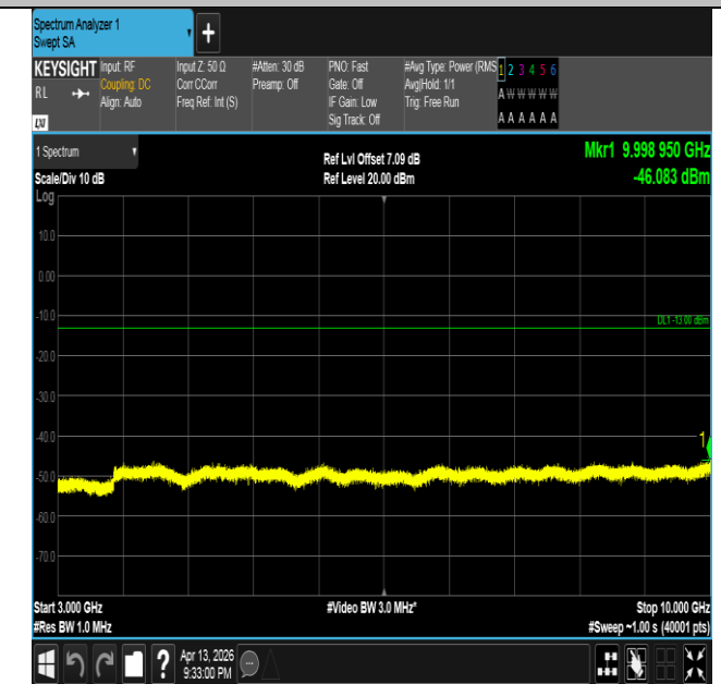
Band26(824-849)-10MHz-16QAM-26915-1RB#0-3000~10000
