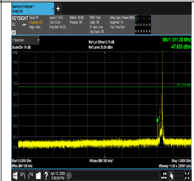
Band26(824-849)-15MHz-QPSK-26865-1RB#74-30~1000-PA SS
