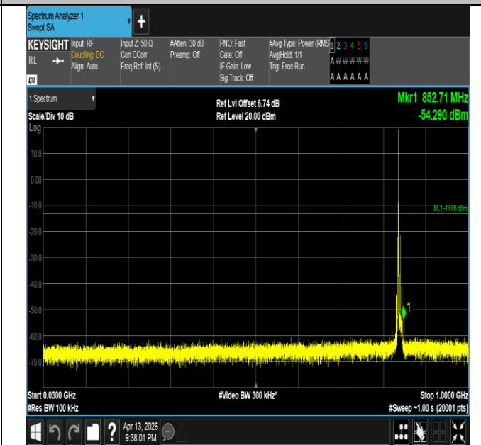
Band26(824-849)-10MHz-16QAM-26990-1RB#0-30~1000-PA SS
