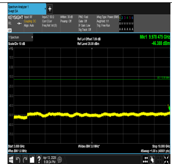
Band26(824-849)-10MHz-16QAM-26990-1RB#0-3000~10000 -PASS
