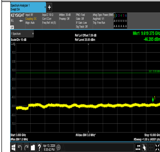
Band26(824-849)-10MHz-QPSK-26915-50RB#0-3000~10000- PASS
