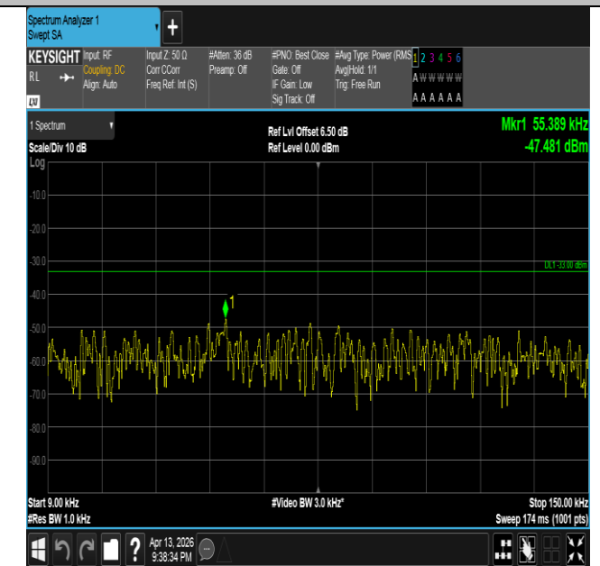
Band26(824-849)-10MHz-QPSK-26990-1RB#49-0.009~0.15-P
