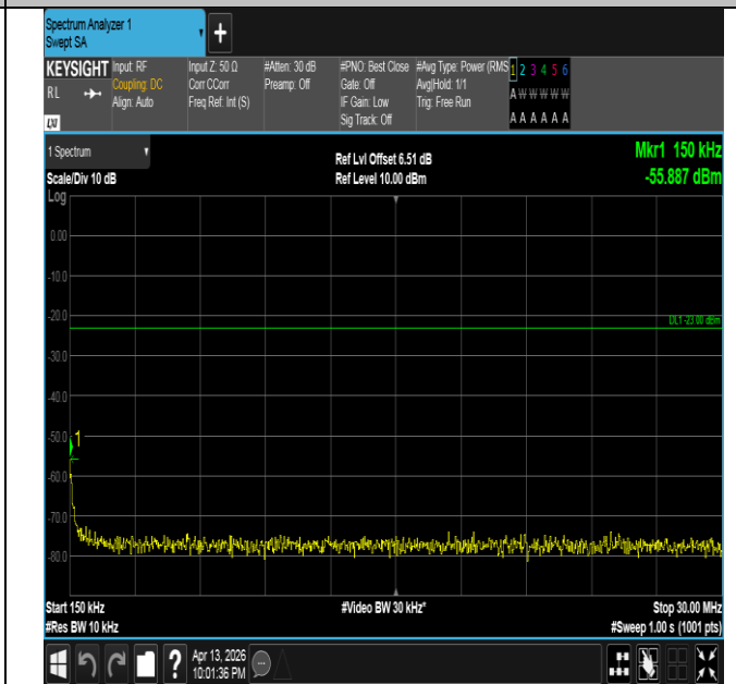
Band26(824-849)-15MHz-QPSK-26865-75RB#0-0.15~30-PAS S
