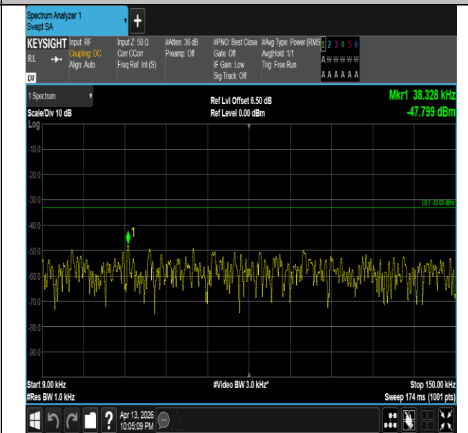
Band26(824-849)-15MHz-QPSK-26915-1RB#74-0.009~0.15-P
