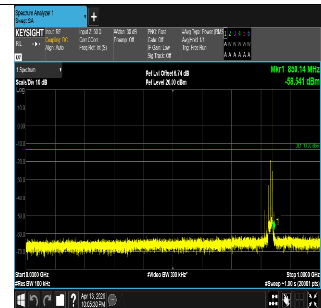
Band26(824-849)-15MHz-QPSK-26915-1RB#74-30~1000-PA
