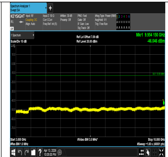
Band26(824-849)-15MHz-16QAM-26915-1RB#0-3000~10000 -PASS
