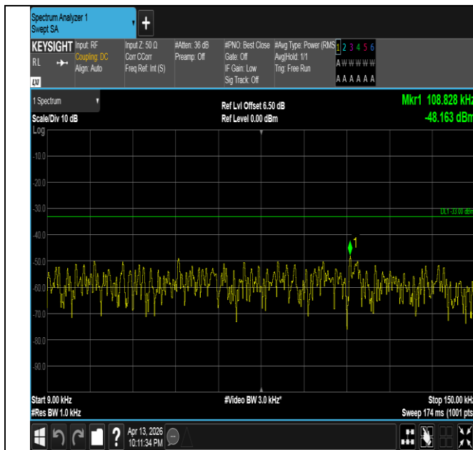
Band26(824-849)-15MHz-16QAM-26965-1RB#74-0.009~0.15
