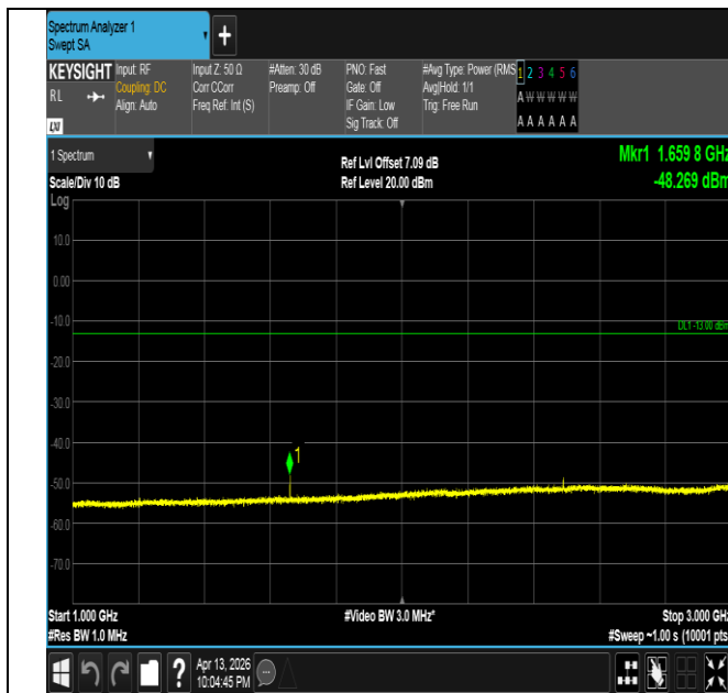
Band26(824-849)-15MHz-16QAM-26915-1RB#0-1000~3000- PASS
