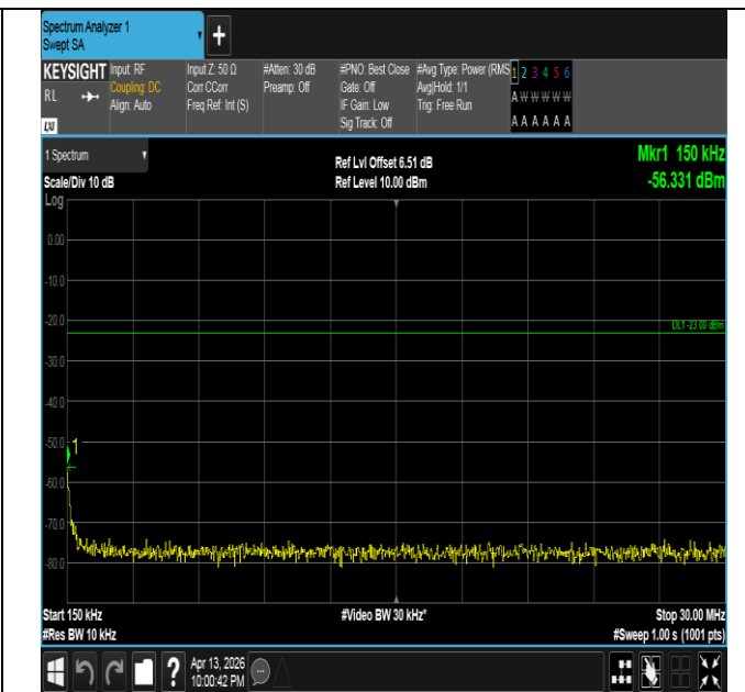
Band26(824-849)-15MHz-16QAM-26865-1RB#74-0.15~30-PA
