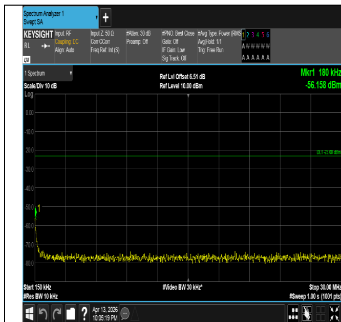
Band26(824-849)-15MHz-QPSK-26915-1RB#74-0.15~30-PAS
