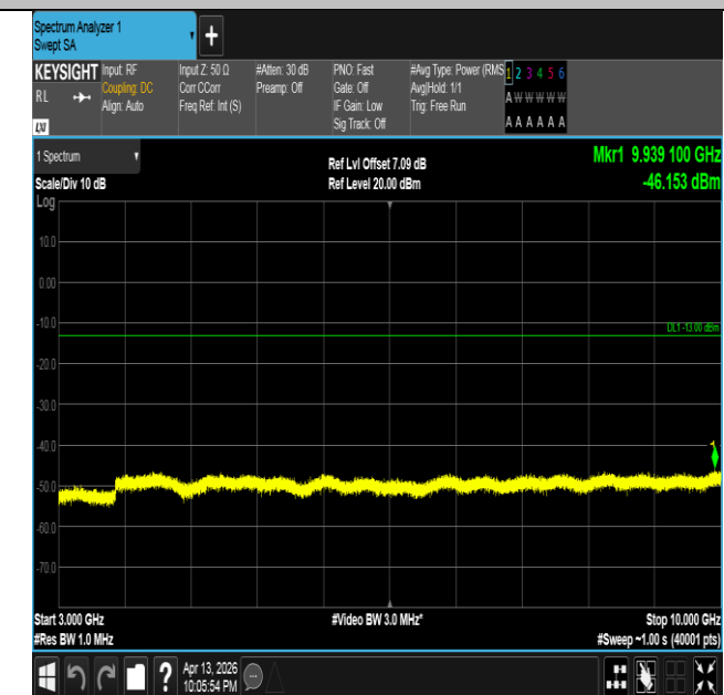
Band26(824-849)-15MHz-QPSK-26915-1RB#74-3000~10000-
