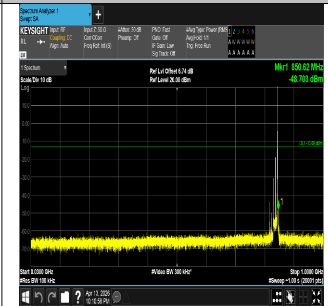
Band26(824-849)-15MHz-QPSK-26965-1RB#74-30~1000-PA SS
