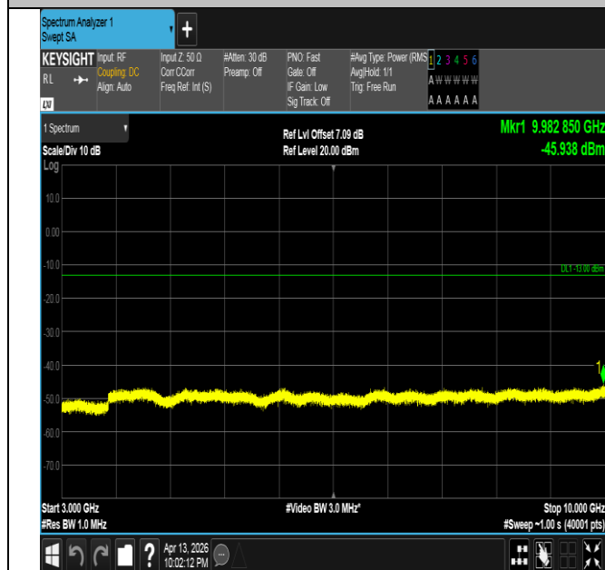
Band26(824-849)-15MHz-QPSK-26865-75RB#0-3000~10000-
