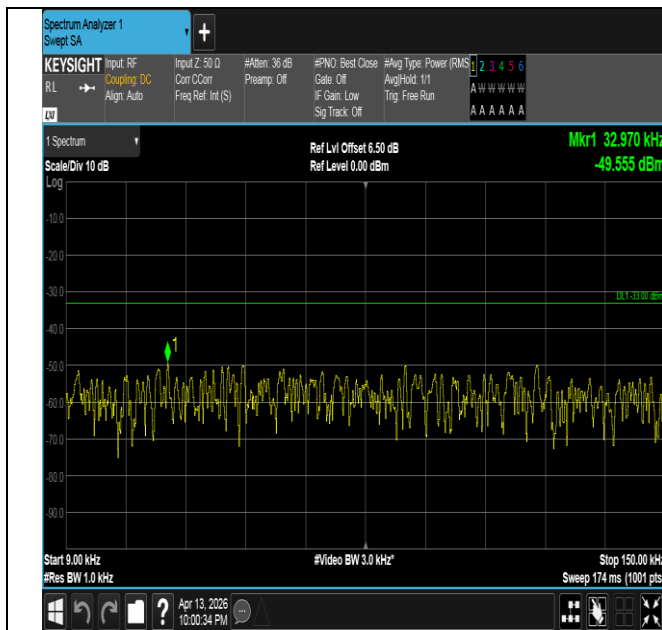
Band26(824-849)-15MHz-16QAM-26865-1RB#74-0.009~0.15
