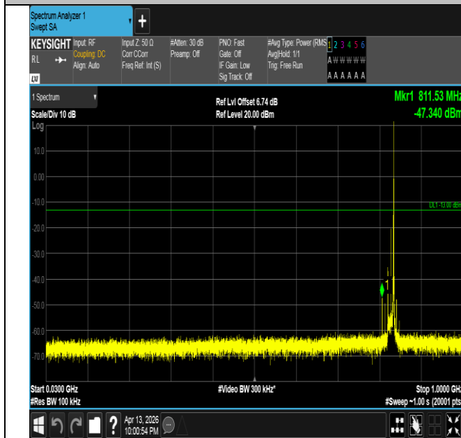
Band26(824-849)-15MHz-16QAM-26865-1RB#74-30~1000-P
