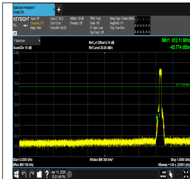
Band26(824-849)-15MHz-QPSK-26865-75RB#0-30~1000-PA
