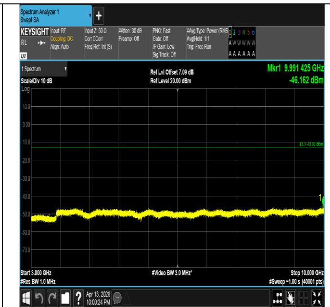
Band26(824-849)-15MHz-QPSK-26865-1RB#74-3000~10000- PASS
