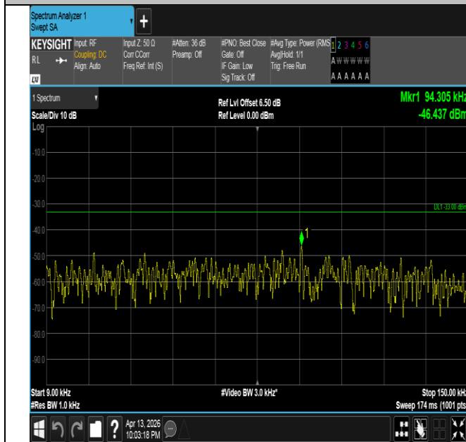
Band26(824-849)-15MHz-QPSK-26915-1RB#0-0.009~0.15-P
