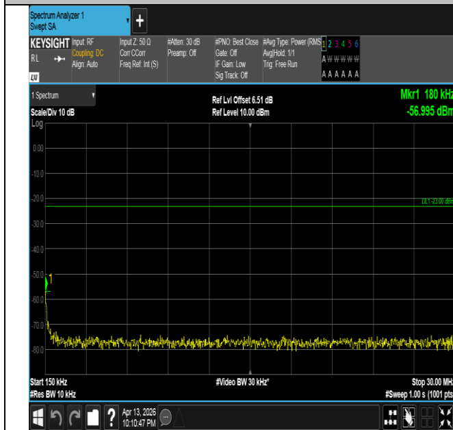
Band26(824-849)-15MHz-QPSK-26965-1RB#74-0.15~30-PA S
