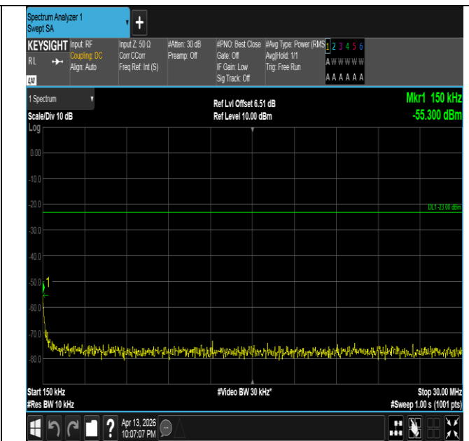
Band26(824-849)-15MHz-QPSK-26915-75RB#0-0.15~30-PAS S
