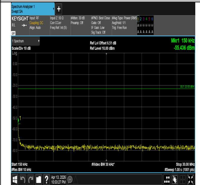
Band26(824-849)-15MHz-QPSK-26915-1RB#0-0.15~30-PAS
