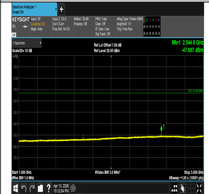
Band26(824-849)-15MHz-16QAM-26965-1RB#74-1000~3000
