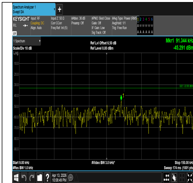
Band26(824-849)-15MHz-QPSK-26965-1RB#0-0.009~0.15-P
