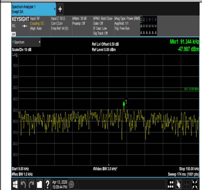
Band26(824-849)-15MHz-16QAM-26965-1RB#0-0.009~0.15- PASS
