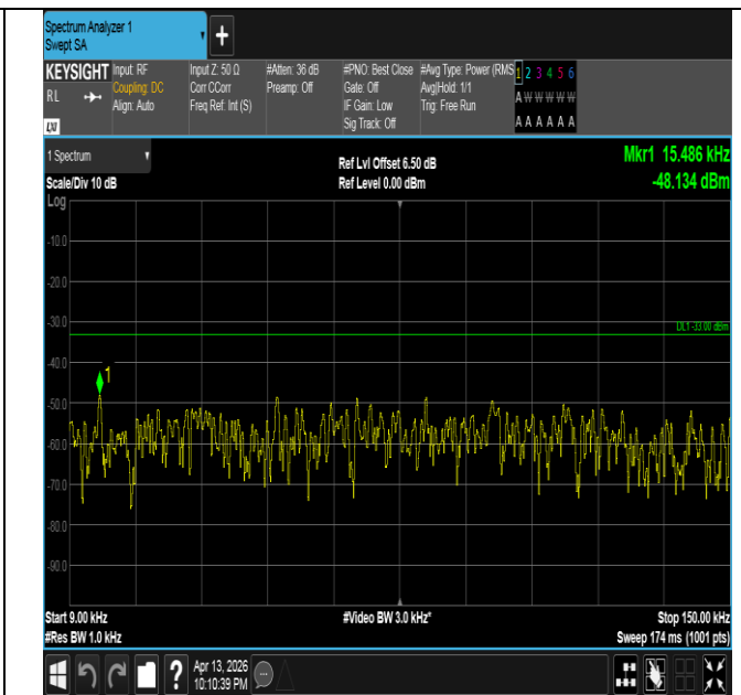
Band26(824-849)-15MHz-QPSK-26965-1RB#74-0.009~0.15-P ASS
