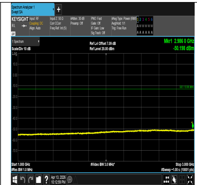
Band26(824-849)-15MHz-QPSK-26965-75RB#0-1000~3000-P ASS
