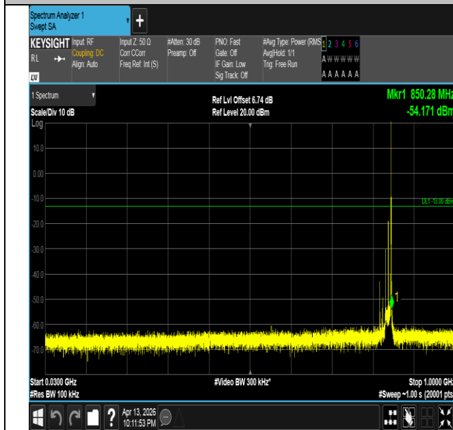
Band26(824-849)-15MHz-16QAM-26965-1RB#74-30~1000-P
