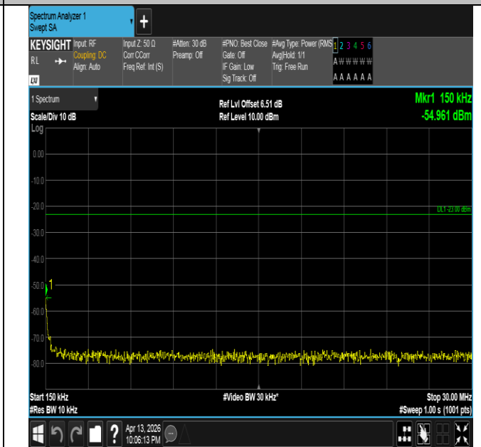
Band26(824-849)-15MHz-16QAM-26915-1RB#74-0.15~30-PA SS
