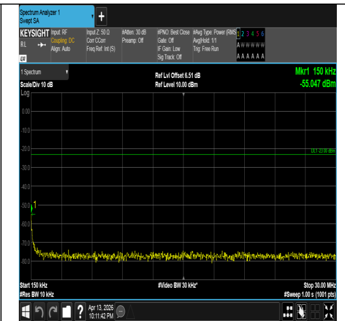
Band26(824-849)-15MHz-16QAM-26965-1RB#74-0.15~30-PA
