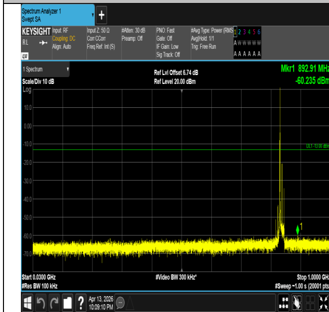
Band26(824-849)-15MHz-QPSK-26965-1RB#0-30~1000-PAS
