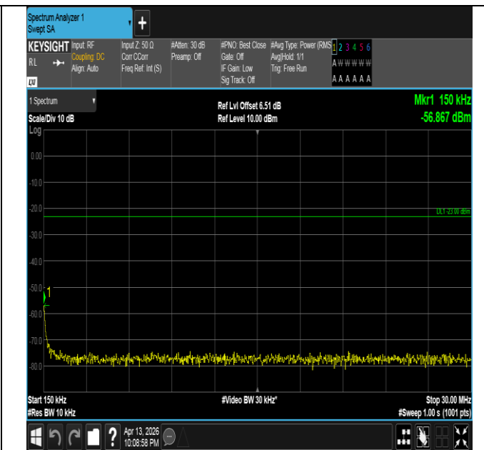
Band26(824-849)-15MHz-QPSK-26965-1RB#0-0.15~30-PAS
