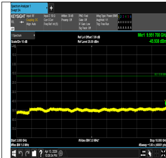
Band26(824-849)-15MHz-QPSK-26965-1RB#0-3000~10000- PASS
