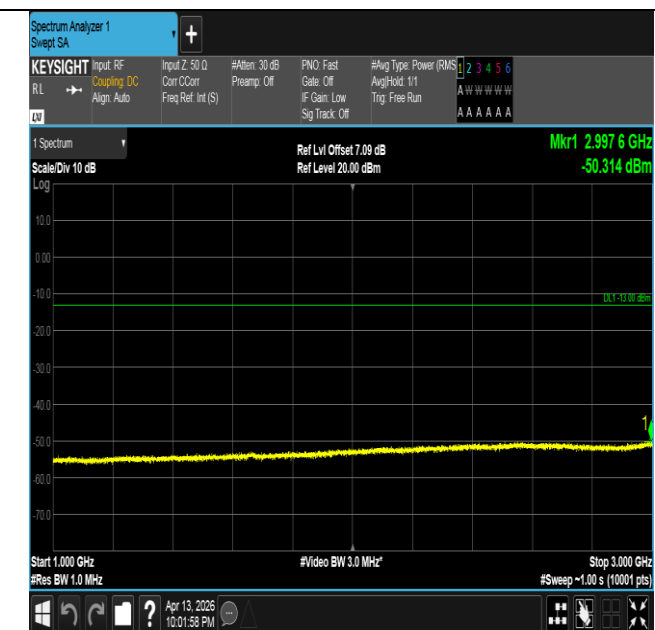
Band26(824-849)-15MHz-QPSK-26865-75RB#0-1000~3000-P
