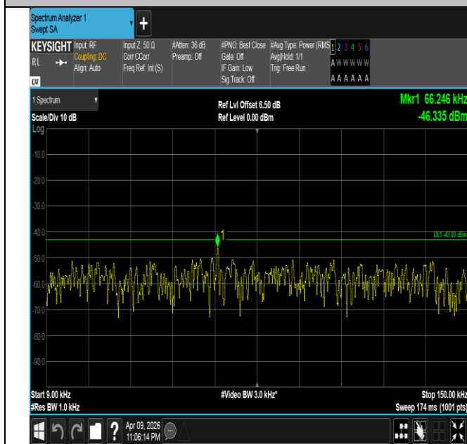
Band4-20MHz-16QAM-20300-1RB#99-0.009~0.15-PASS
