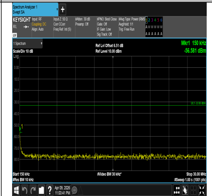
Band4-20MHz-QPSK-20300-1RB#0-0.15~30-PASS
