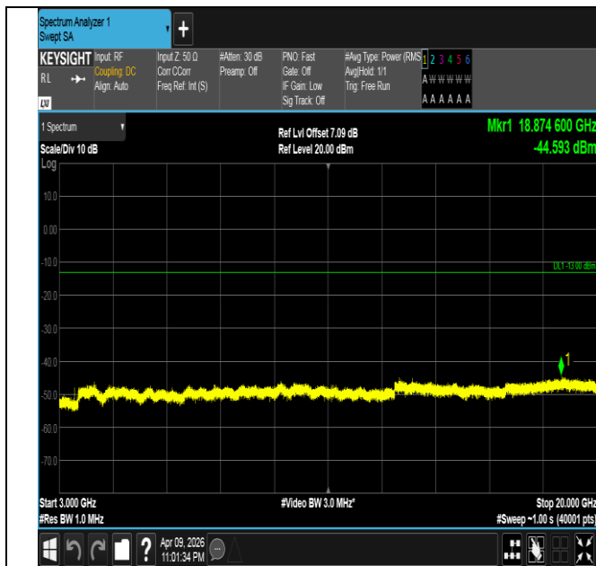
Band4-20MHz-16QAM-20175-1RB#99-3000~20000-PASS
