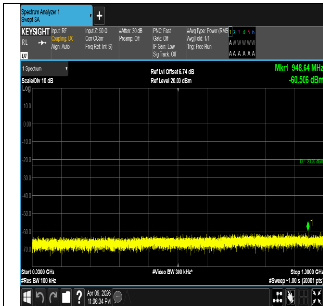
Band4-20MHz-16QAM-20300-1RB#99-30~1000-PASS
