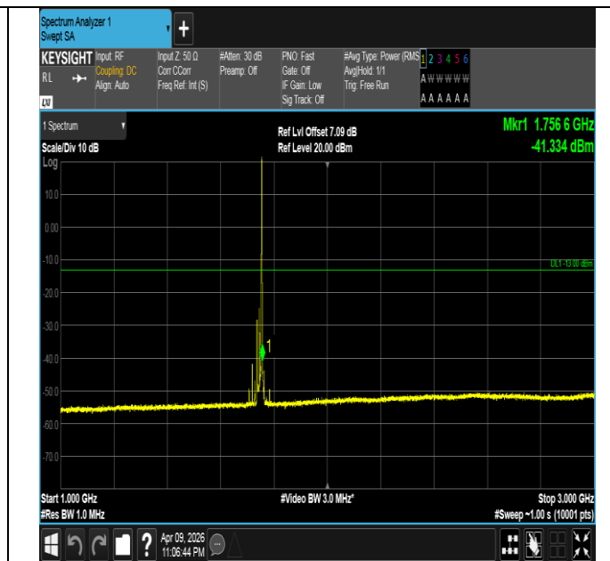
Band4-20MHz-16QAM-20300-1RB#99-1000~3000-PASS
