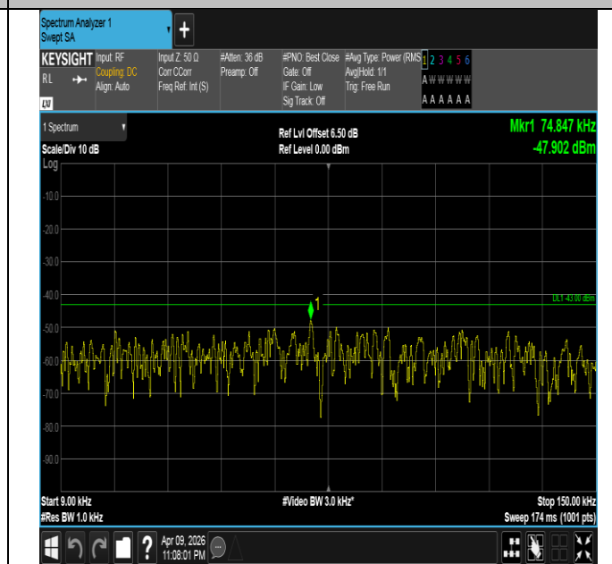
Band4-20MHz-16QAM-20300-100RB#0-0.009~0.15-PASS
