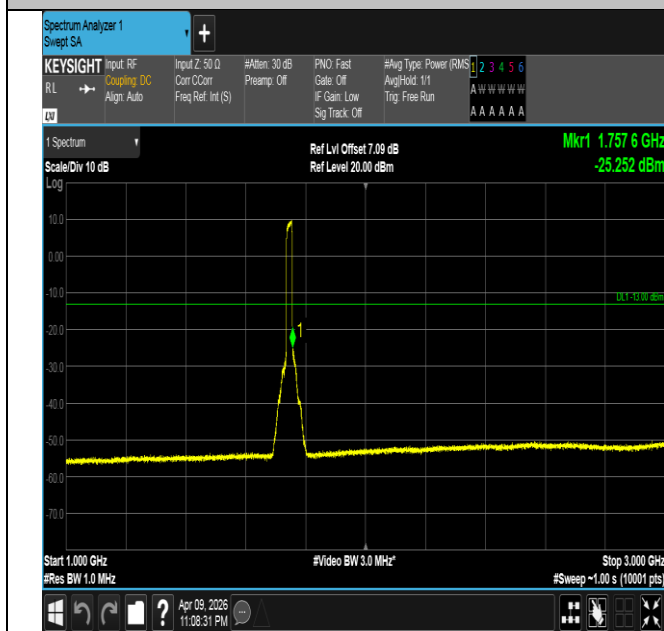
Band4-20MHz-16QAM-20300-100RB#0-1000~3000-PASS
