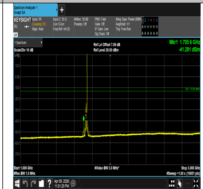
Band4-20MHz-16QAM-20175-1RB#99-1000~3000-PASS
