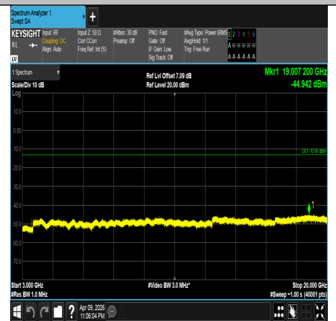
Band4-20MHz-QPSK-20300-1RB#99-3000~20000-PASS
