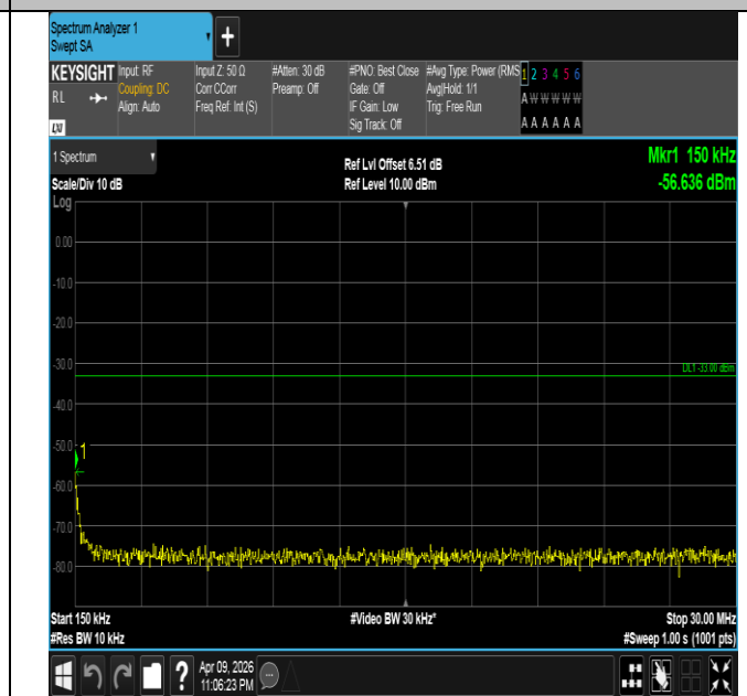
Band4-20MHz-16QAM-20300-1RB#99-0.15~30-PASS
