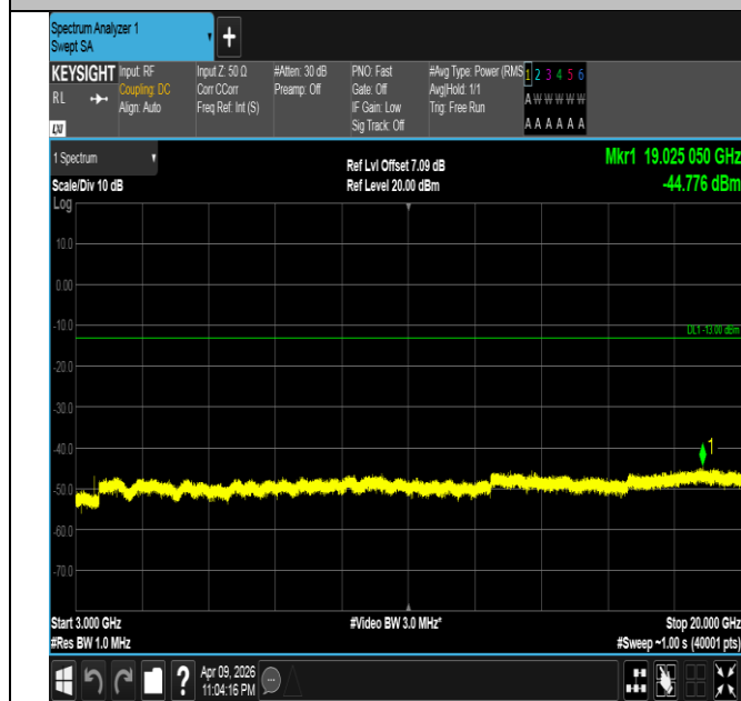
Band4-20MHz-QPSK-20300-1RB#0-3000~20000-PASS
