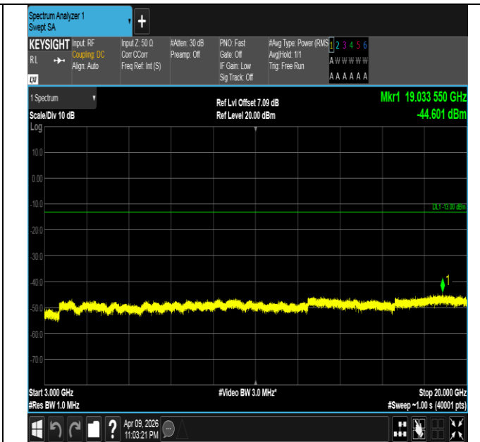
Band4-20MHz-16QAM-20175-100RB#0-3000~20000-PASS
