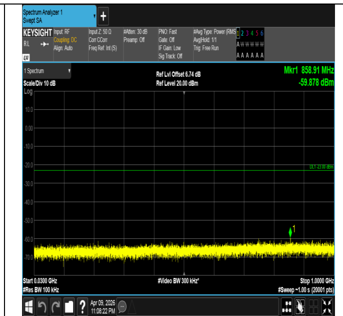
Band4-20MHz-16QAM-20300-100RB#0-30~1000-PASS
