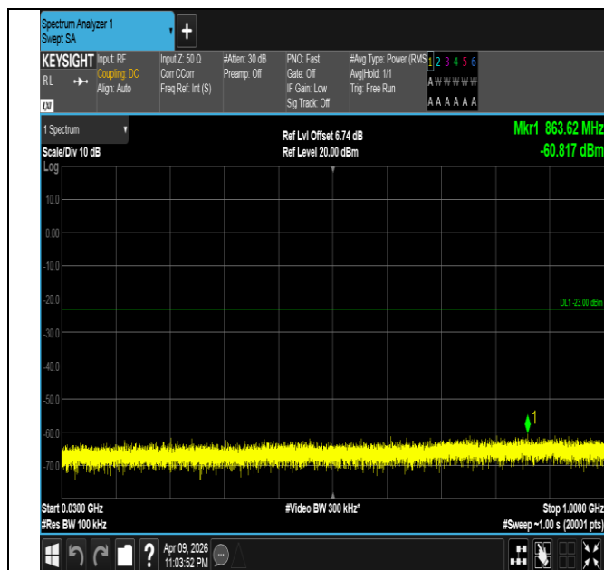
Band4-20MHz-QPSK-20300-1RB#0-30~1000-PASS
