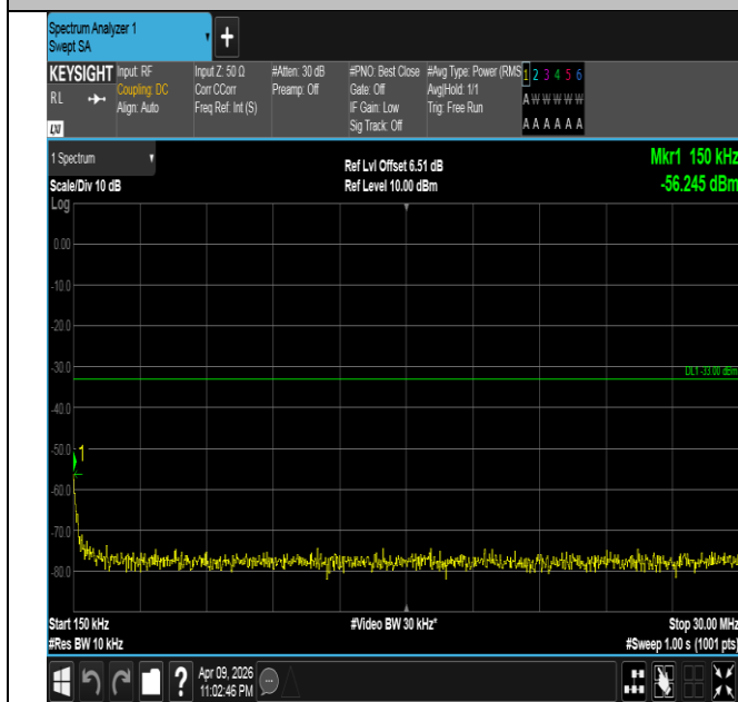
Band4-20MHz-16QAM-20175-100RB#0-0.15~30-PASS
