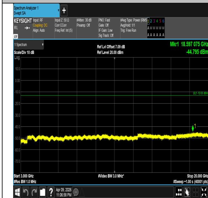
Band4-20MHz-16QAM-20300-1RB#99-3000~20000-PASS
