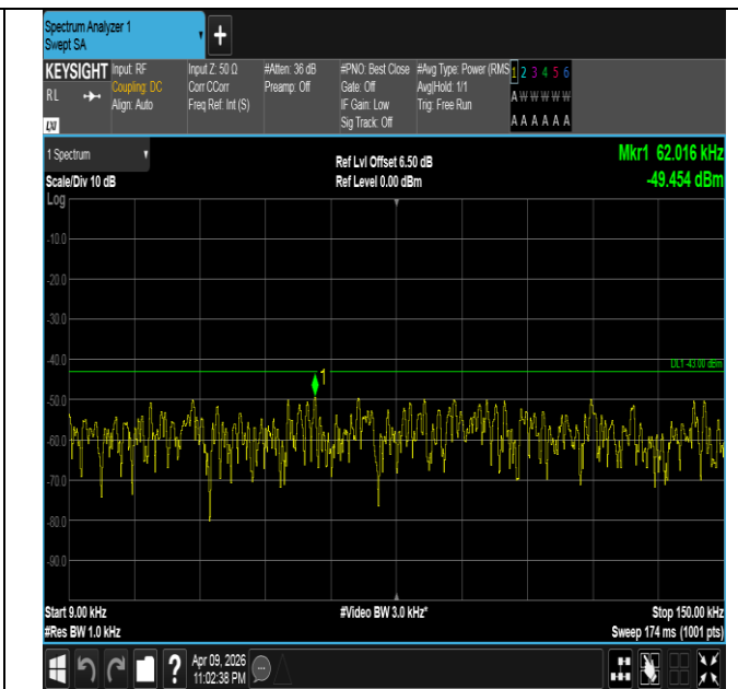
Band4-20MHz-16QAM-20175-100RB#0-0.009~0.15-PASS
