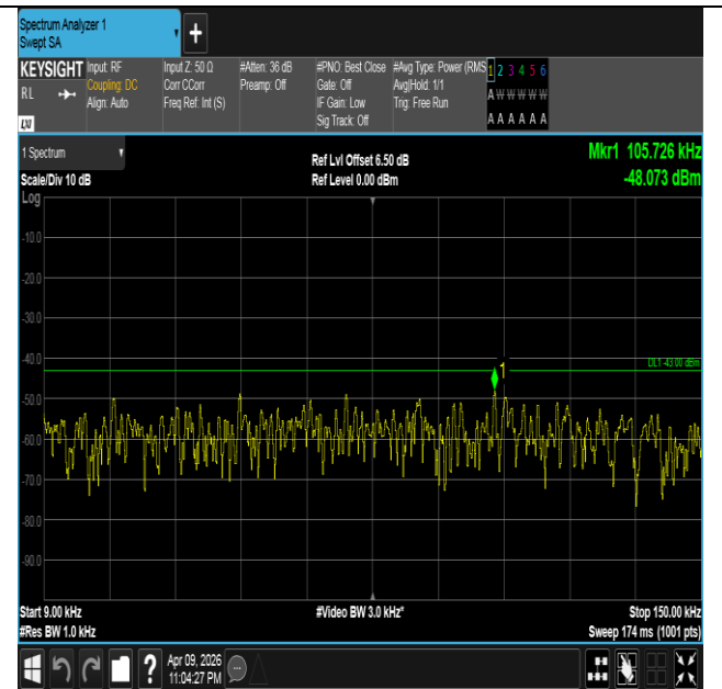
Band4-20MHz-16QAM-20300-1RB#0-0.009~0.15-PASS
