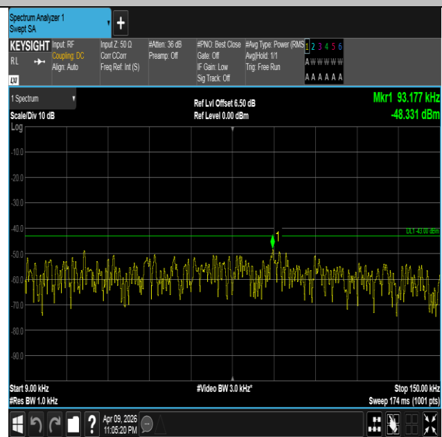
Band4-20MHz-QPSK-20300-1RB#99-0.009~0.15-PASS
