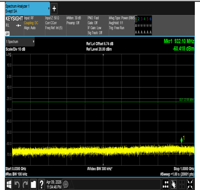
Band4-20MHz-16QAM-20300-1RB#0-30~1000-PASS
