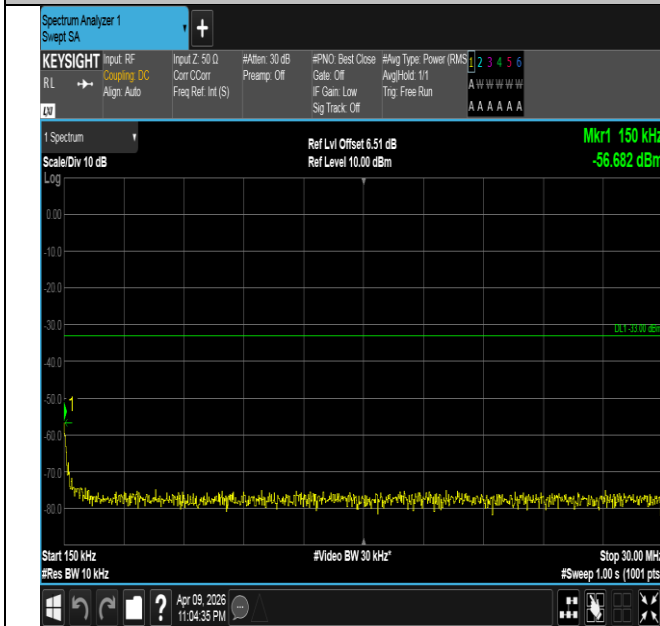
Band4-20MHz-16QAM-20300-1RB#0-0.15~30-PASS
