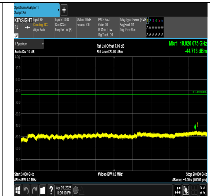
Band4-20MHz-16QAM-20300-1RB#0-3000~20000-PASS
