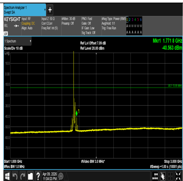
Band4-20MHz-QPSK-20300-1RB#0-1000~3000-PASS
