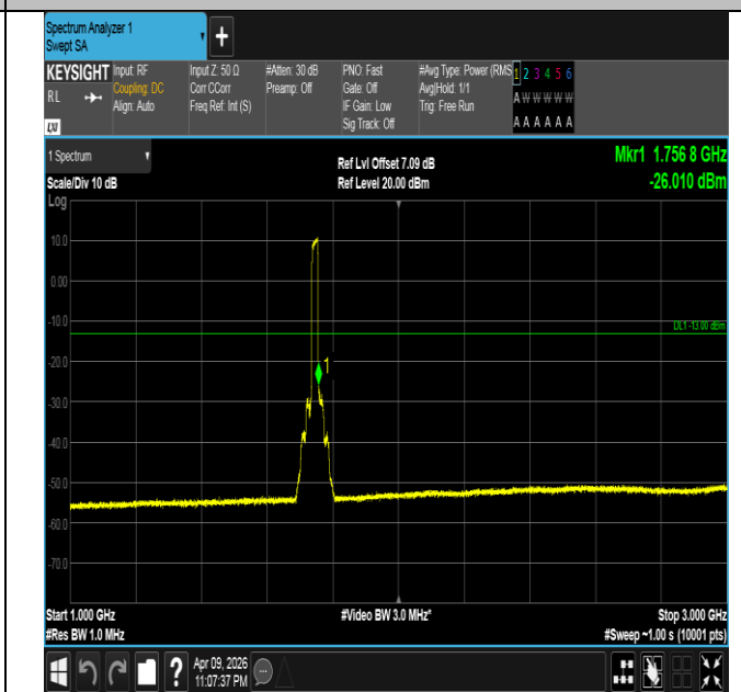
Band4-20MHz-QPSK-20300-100RB#0-1000~3000-PASS
