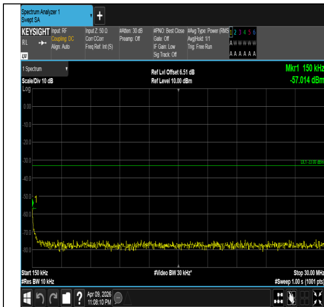
Band4-20MHz-16QAM-20300-100RB#0-0.15~30-PASS
