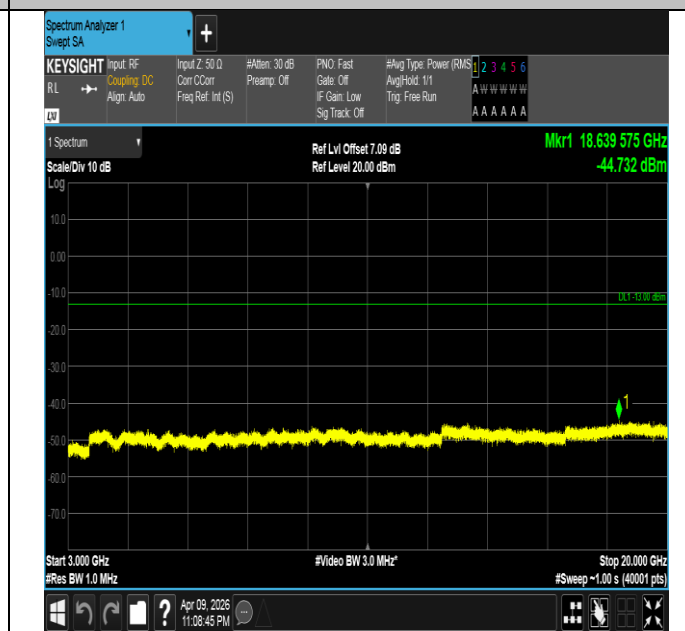
Band4-20MHz-16QAM-20300-100RB#0-3000~20000-PASS
