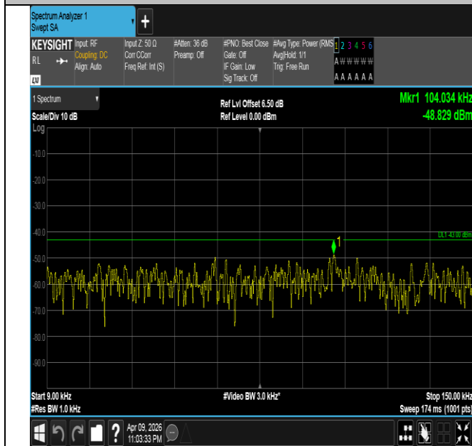
Band4-20MHz-QPSK-20300-1RB#0-0.009~0.15-PASS
