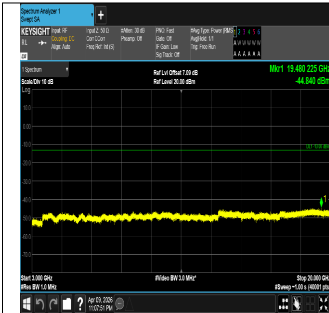
Band4-20MHz-QPSK-20300-100RB#0-3000~20000-PASS
