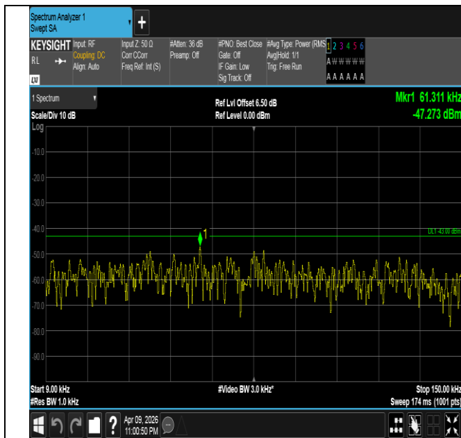
Band4-20MHz-16QAM-20175-1RB#99-0.009~0.15-PASS
