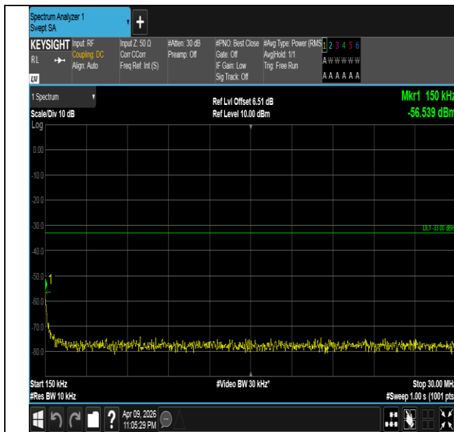
Band4-20MHz-QPSK-20300-1RB#99-0.15~30-PASS
