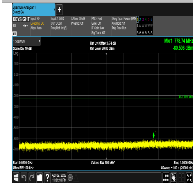
Band4-20MHz-16QAM-20175-1RB#99-30~1000-PASS
