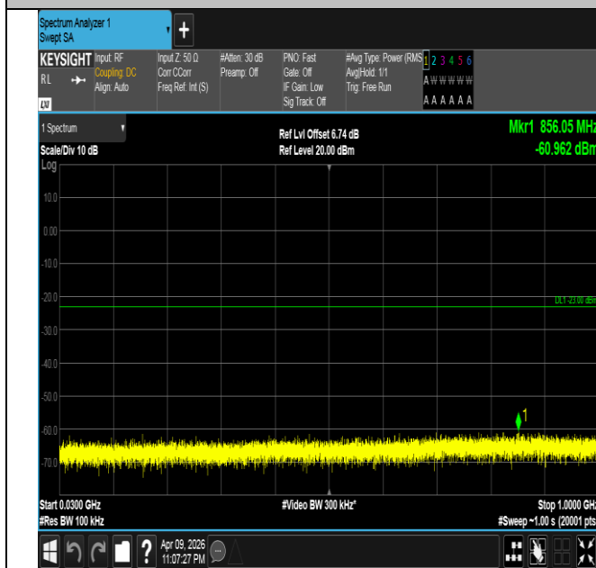
Band4-20MHz-QPSK-20300-100RB#0-30~1000-PASS
