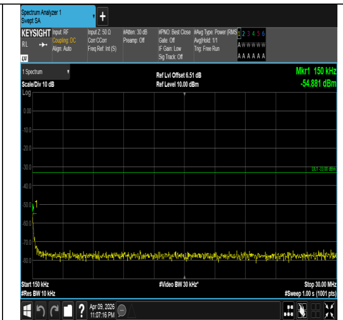
Band4-20MHz-QPSK-20300-100RB#0-0.15~30-PASS
