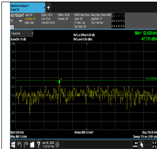
Band4-20MHz-QPSK-20300-100RB#0-0.009~0.15-PASS
