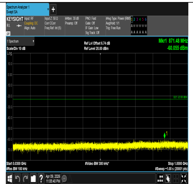
Band4-20MHz-QPSK-20300-1RB#99-30~1000-PASS
