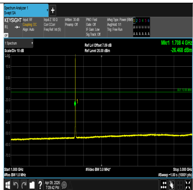
Band4-1.4MHz-QPSK-19957-6RB#0-1000~3000-PASS
