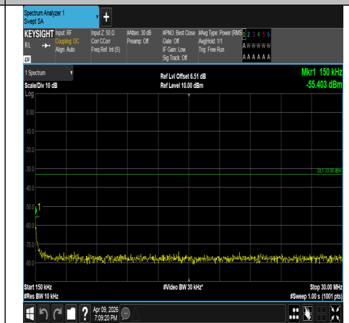
Band4-1.4MHz-QPSK-19957-6RB#0-0.15~30-PASS
