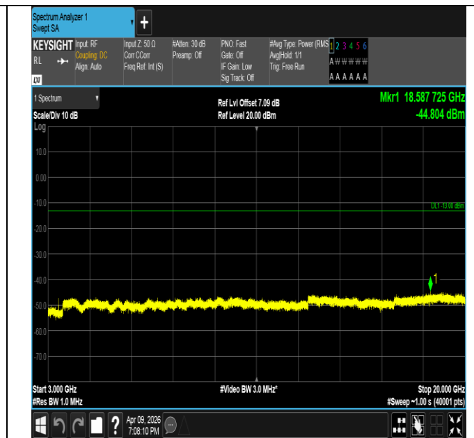
Band4-1.4MHz-QPSK-19957-1RB#5-3000~20000-PASS
