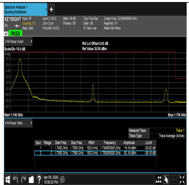
Band4-15MHz-16QAM-20325-1RB#0-PASS
