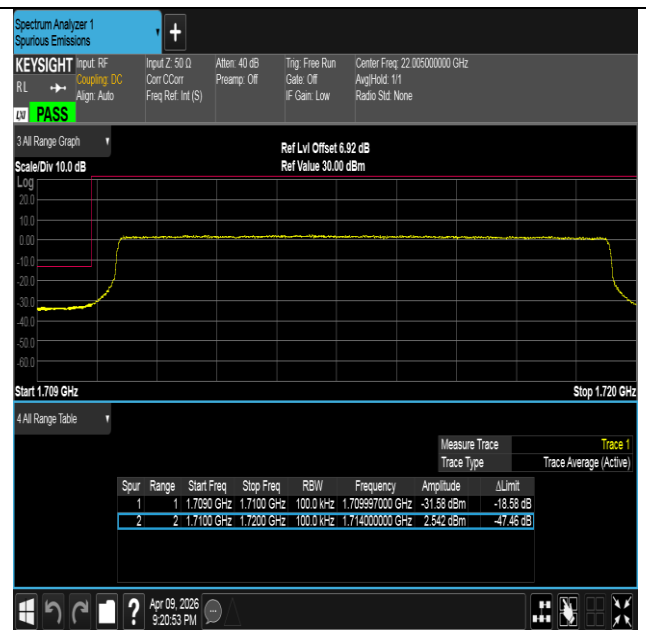
Band4-10MHz-16QAM-20000-50RB#0-PASS
