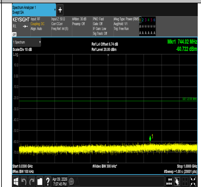
Band4-1.4MHz-QPSK-19957-1RB#5-30~1000-PASS
