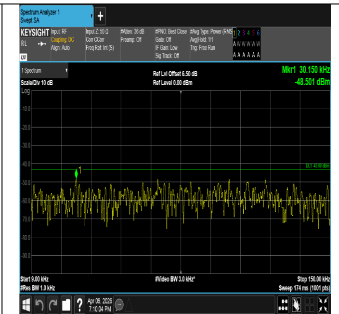
Band4-1.4MHz-16QAM-19957-6RB#0-0.009~0.15-PASS
