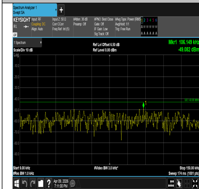
Band4-1.4MHz-QPSK-20175-1RB#0-0.009~0.15-PASS
