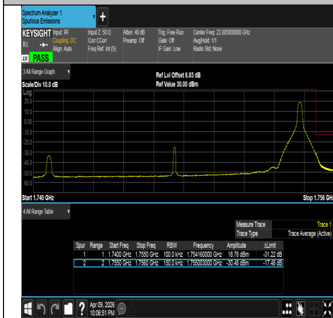
Band4-15MHz-16QAM-20325-1RB#74-PASS
