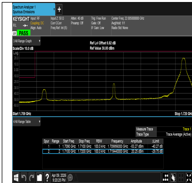
Band4-10MHz-16QAM-20000-1RB#49-PASS
