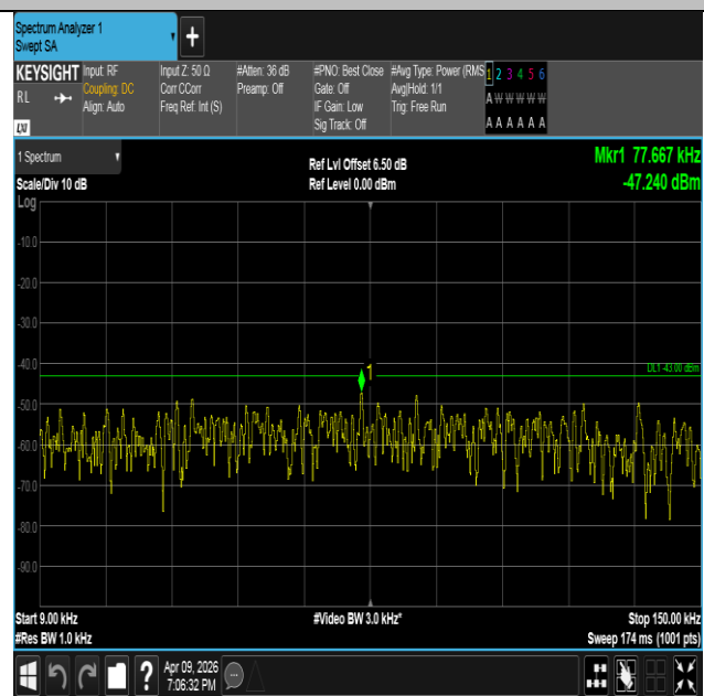
Band4-1.4MHz-16QAM-19957-1RB#0-0.009~0.15-PASS
