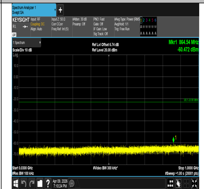
Band4-1.4MHz-16QAM-19957-6RB#0-30~1000-PASS
