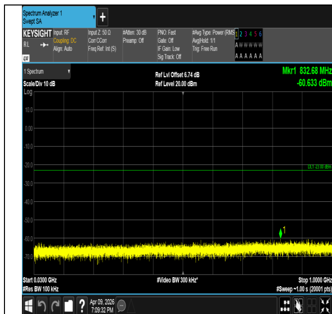
Band4-1.4MHz-QPSK-19957-6RB#0-30~1000-PASS
